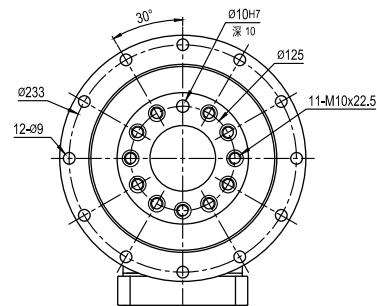
输出端/OUTPUT
