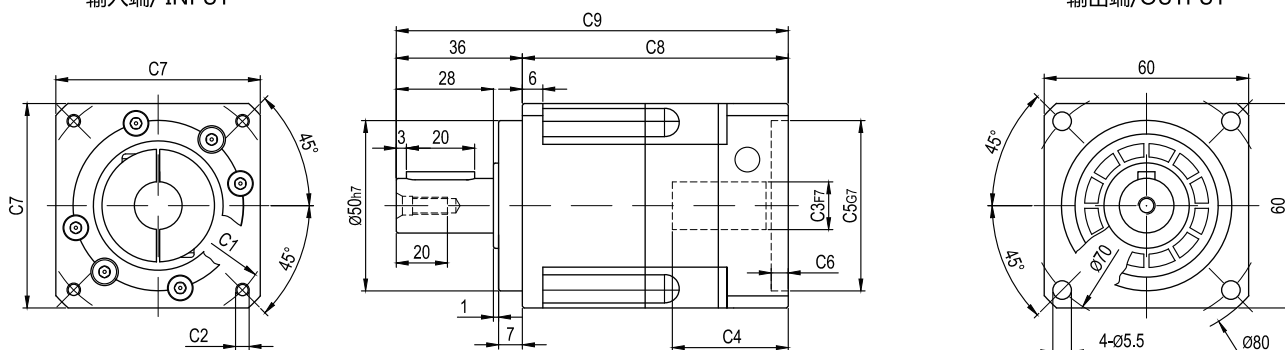
输出端/OUTPUT
