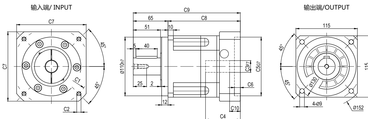
PGL115-L2
