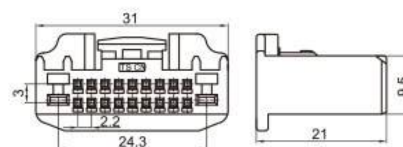
Type: TS7552-20P-21 Material: PA66 Matching Terminal: TSH009 / TSH143
