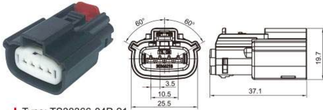
Type: TS30366-04P-21 Material: PA66 GF30% Matching Terminal: TSH047
