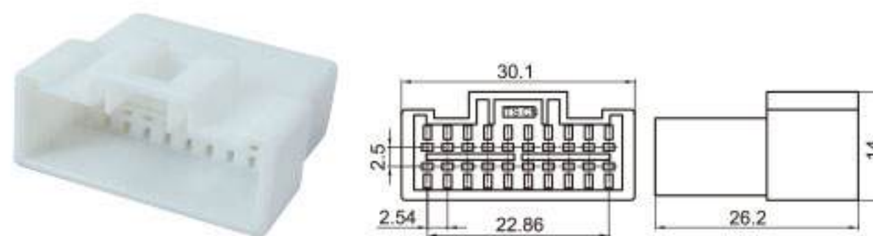
Type: TSPAN20-20P-11 Material: PA66 Matching Terminal: TSZ007B
