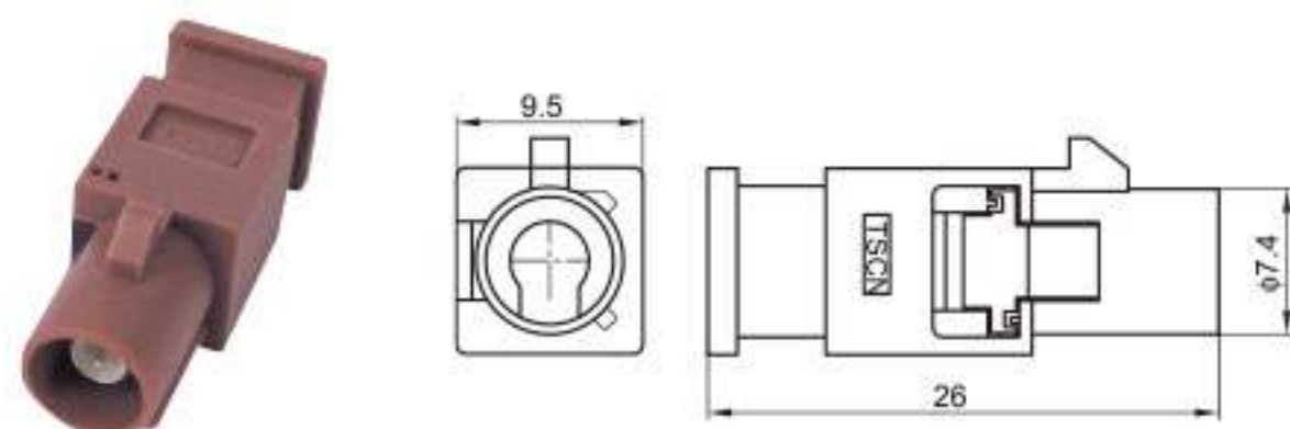
Type: TSVW10-01PM-AT-BN Material: PA66 Matching Terminal: TSTM0019 / TSTM0020
