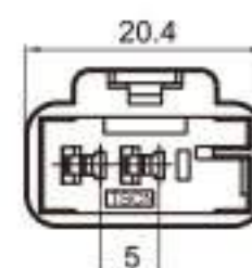
Type: TS30334-02P-11 Material: PA66 Matching Terminal: TSZ045
