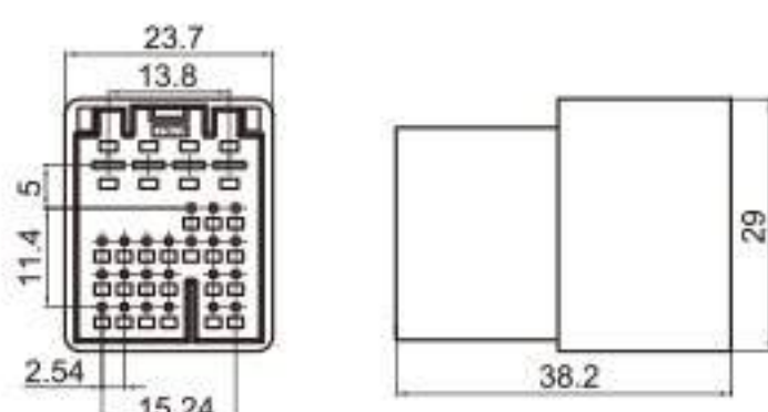
Type: TS30217-30P-11-1 Material: PBT GF15% Matching Terminal: TSDJ615B-2.8*0.8B / TSZ208
