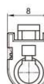
Type: TS1068-01PF-AT-3 Material: PA66 Matching Terminal: TSTF0003 / TSTF0004
