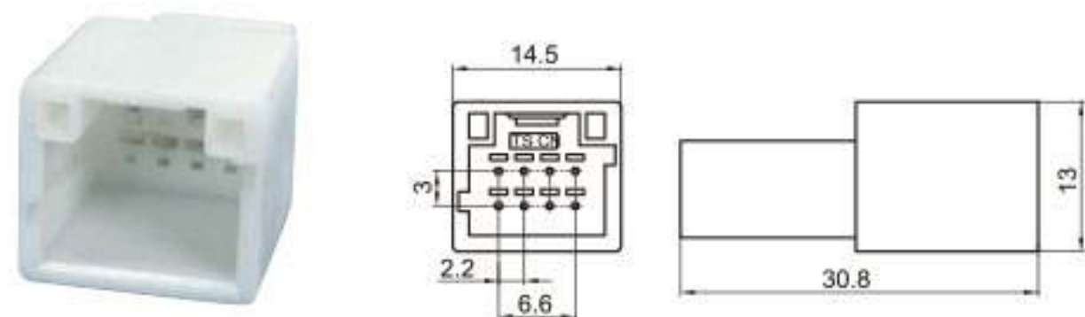
Type: TSTA08-08P-11-4 Material: PA66 Matching Terminal: TSZ208
