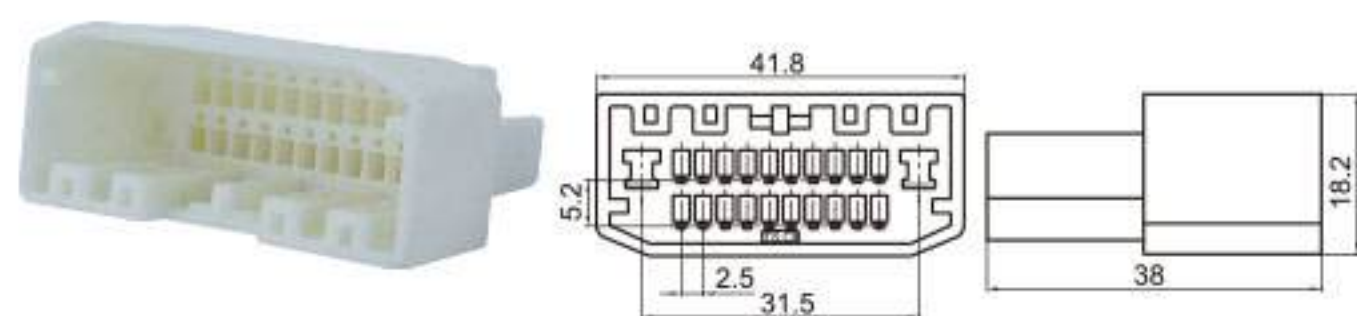
Type: TS6522-22P-11-1 Material: PA66 Matching Terminal: TSZ143 / TSZ145
