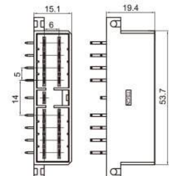
Type: TS1002-17PM-PKB Material: PA66 Matching Terminal: NIL
