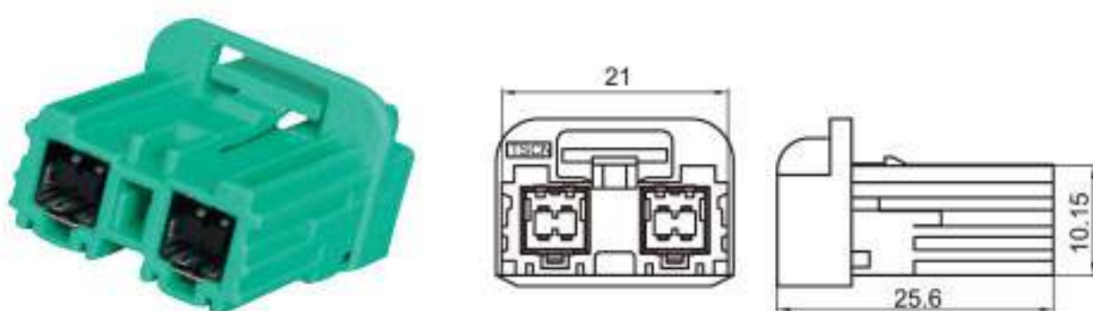
Type: TS1067-02PF-AT Material: PBT GF15% Matching Terminal: TSTF0008 / TSTF0010 / TSTF0011
