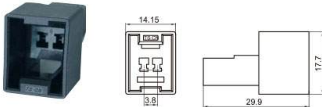
Type: TSLB03-02P-11 Material: PA66 GF30% Matching Terminal: TSZ011
