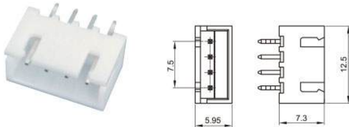
Type: TSXH-04A-PKS(02P-15P) Material: PA66 GF30% Matching Terminal: TSPM0015
