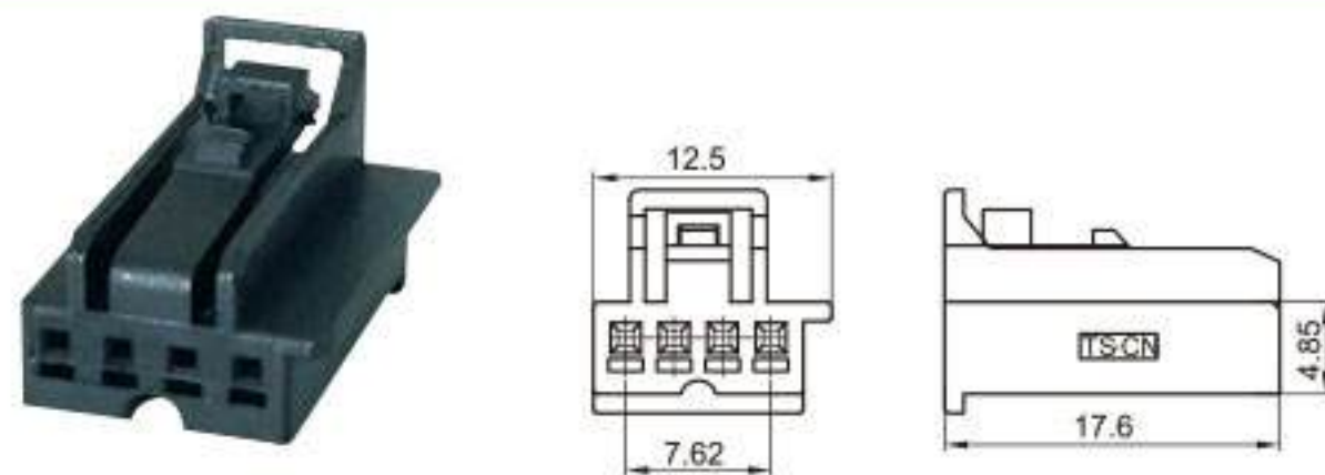
Type: TS30171-04P-21 Material: PA66 Matching Terminal: TSH143
