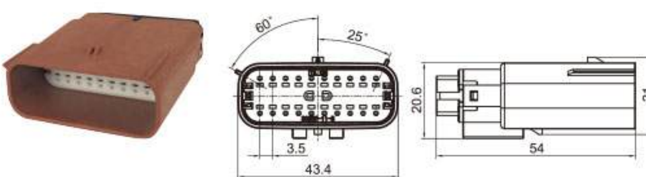
Type: TS30359-20P-11-2 Material: PA66 GF30% Matching Terminal: TSZ144A
