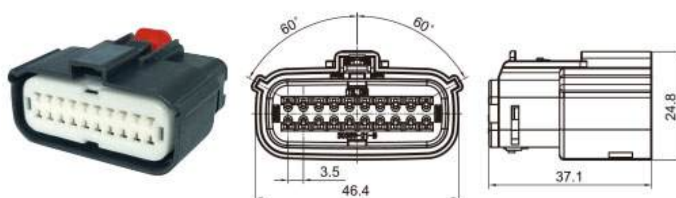
Type: TS30359-20P-21 Material: PA66 GF30% Matching Terminal: TSH047
