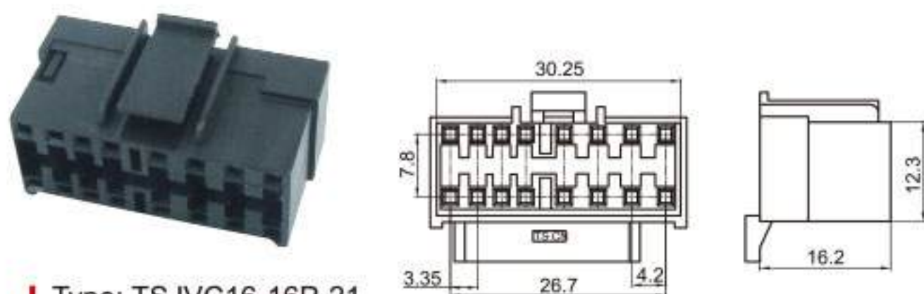
Type: TSJVC16-16P-21 Material: PA66 Matching Terminal: TSH504 / TSH503
