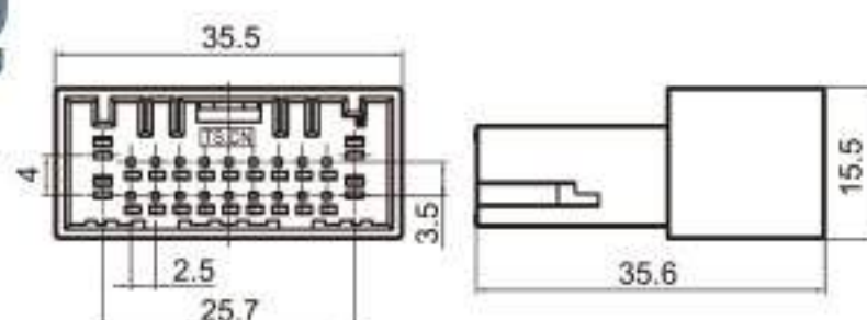
Type: TS30302-22P-11-1 Material: PBT Matching Terminal: TSZ040 / TSZ616
