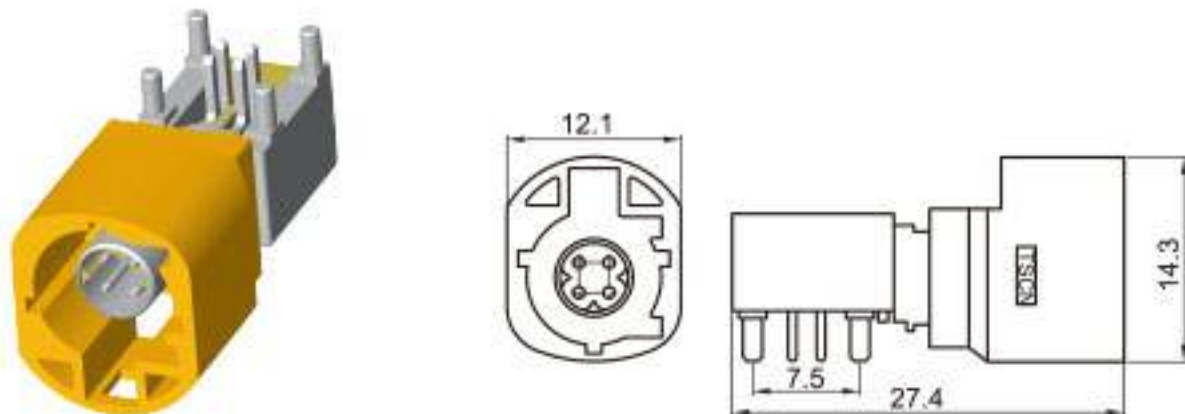
Type: TSVW10-04PM-AT-5OR Material: PA66 GF30% Matching Terminal: TSPM0021~TSPM0025
