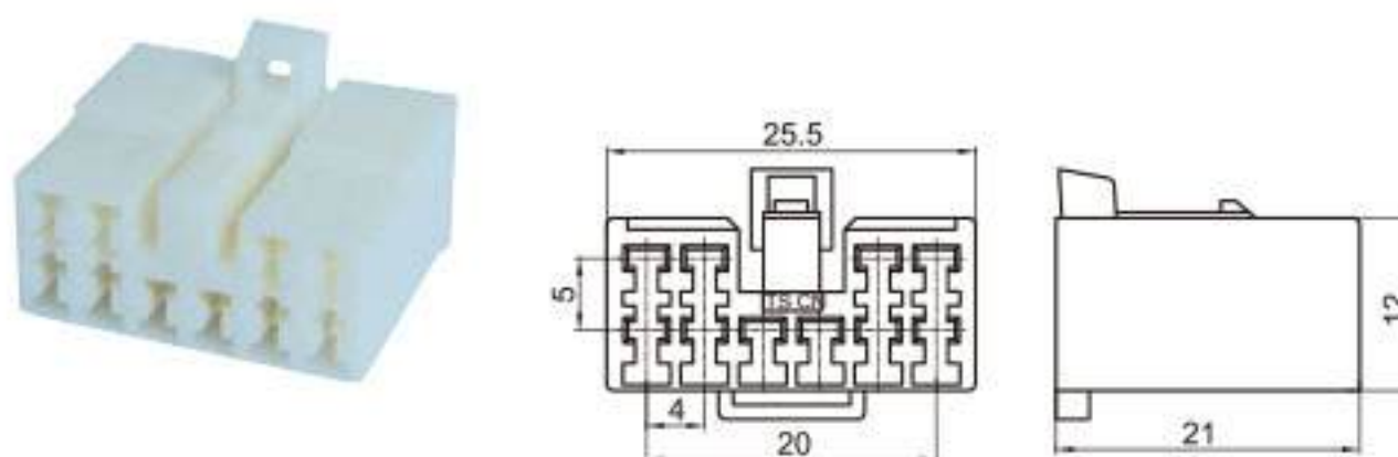
Type: TS1761-10P-21-2 Material: PA66 Matching Terminal: TSH009
