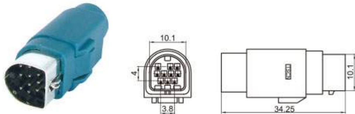
Type: TSALPH-10PM-AH Material: PA66 Matching Terminal: TSAM0014 / TSAM0015 / TS0079
