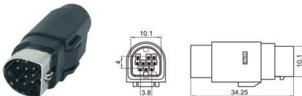
Type: TSALPH-10PM-AH-1 Material: PA66 Matching Terminal: TSAM0014 / TSAM0015 / TS0079
