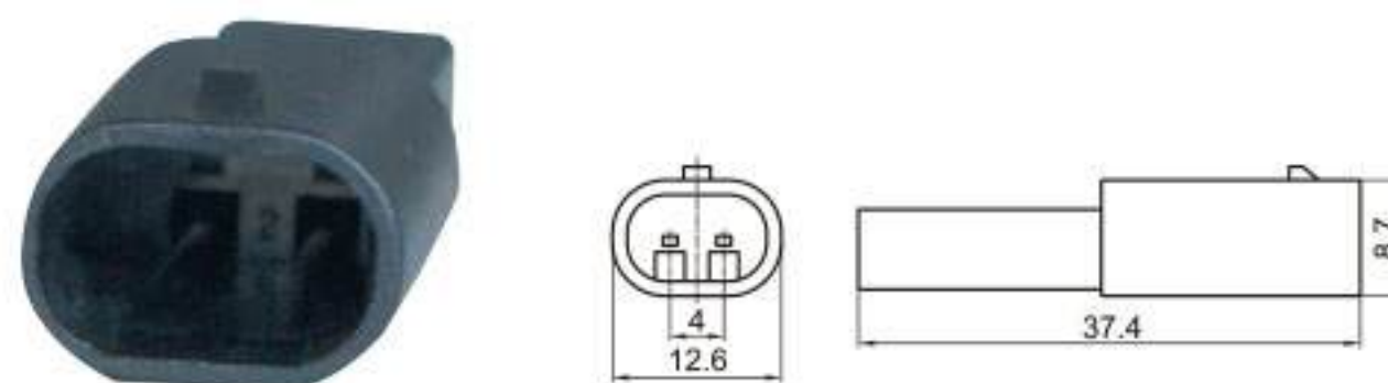
Type: TS30095-02P-11 Material: PA66 GF30% Matching Terminal: TSZ145
