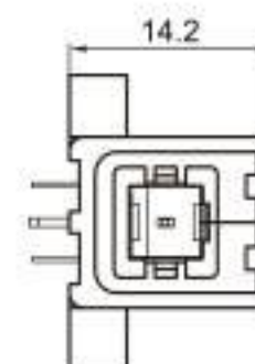
Type: TSFIAT10-01PM-PKB Material: PA66 GF30% Matching Terminal: TSPM0186 / TSPM0187
