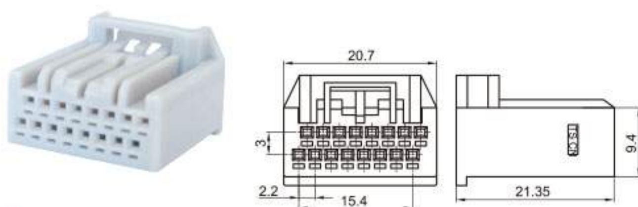
Type: TSCRV16-16P-21 Material: PA66 Matching Terminal: TSH143
