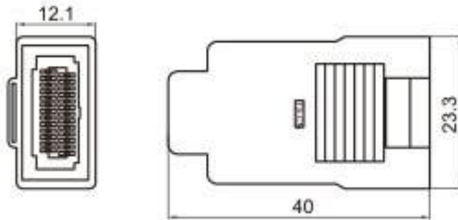
Type: TS30025-26PF-AH Material: PA66 Matching Terminal: TSAF0024 / TSAF0026
