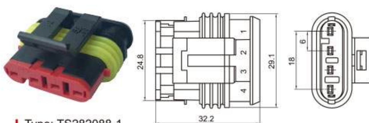
Type: TS282088-1 Material: PA66 Matching Terminal: NIL
