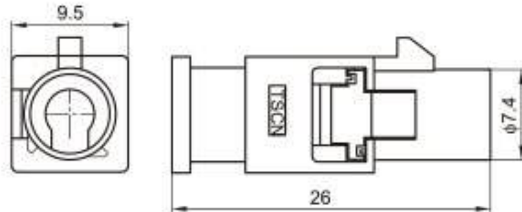
Type: TSVW10-01PM-AT-OR Material: PA66 Matching Terminal: TSTM0019 / TSTM0020
