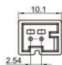
Type: TSLB39-02P-11-4 Material: PA66 GF30% Matching Terminal: TSZ208B
