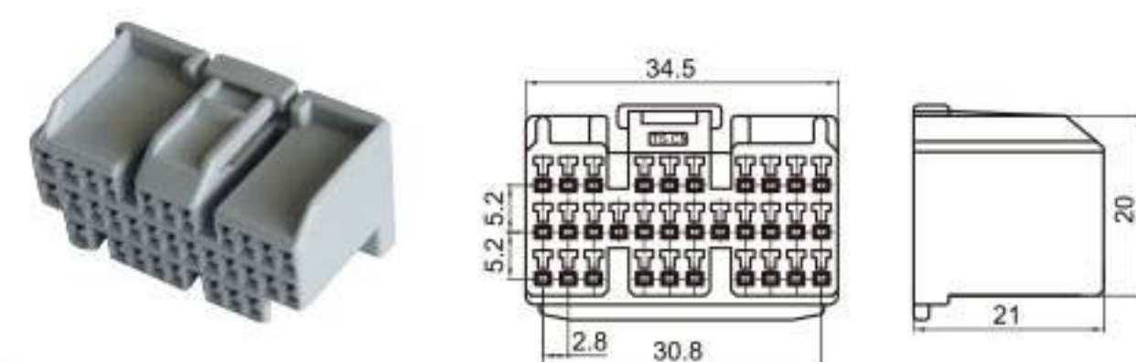
Type: TSWH104-31P-21 Material: PA66 Matching Terminal: TSH076
