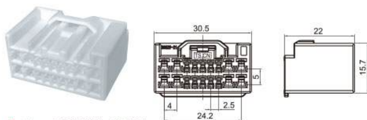
Type: TS30329-18P-21 Material: PBT Matching Terminal: TSH009 / TSH006
