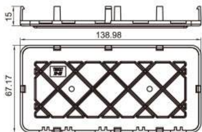
Type: TSBX37 Material: PBT Matching Terminal: NIL
