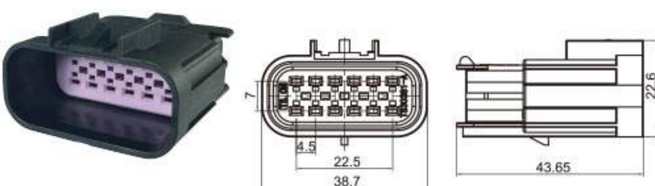
Type: TS30381-12P-11 Material: PA66 GF30% Matching Terminal: TS15326269
