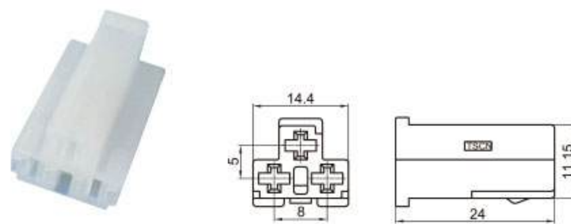
Type: TS30182-03P-21 Material: PA66 Matching Terminal: TSH019
