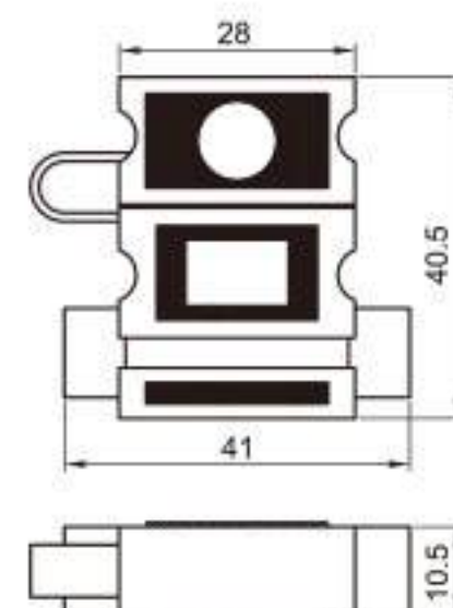
Type: TSBX12 Material: PBT Matching Terminal: TS7522-BS-2
