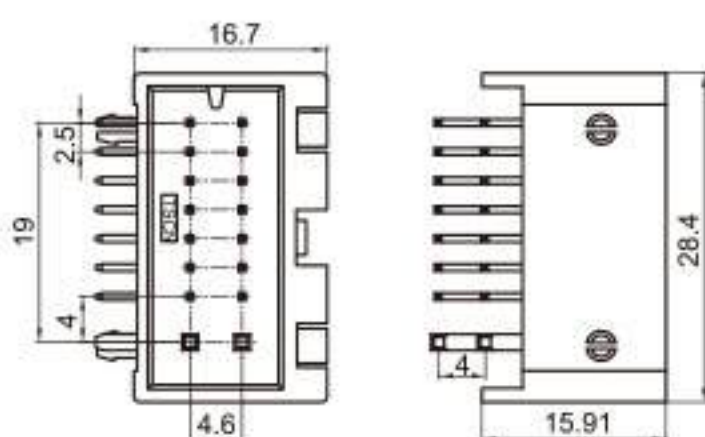
Type: TSCLR-16PM-PKB Material: PA66 Matching Terminal: TSPM0040 / TSPM0221~TSPM0223
