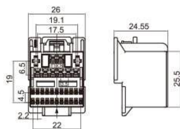
Type: TS30284-32P-11 Material: PA66 GF30% Matching Terminal: TSZ024 / TSZ144 / TSZ208B
