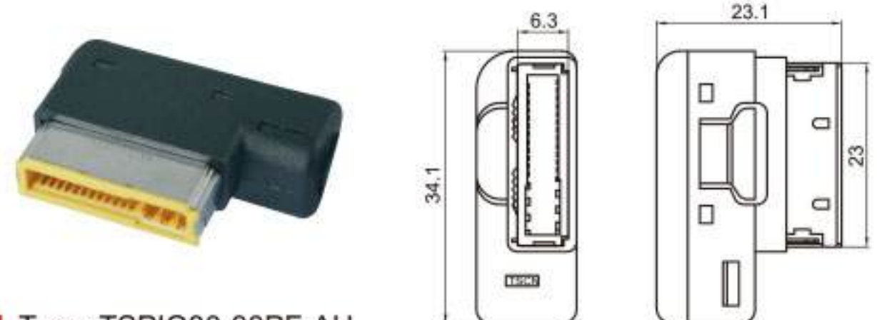
Type: TSPIO30-30PF-AH Material: PA66 GF15% Matching Terminal: TSAF0005 / TSAF0006 / TSAF0008
