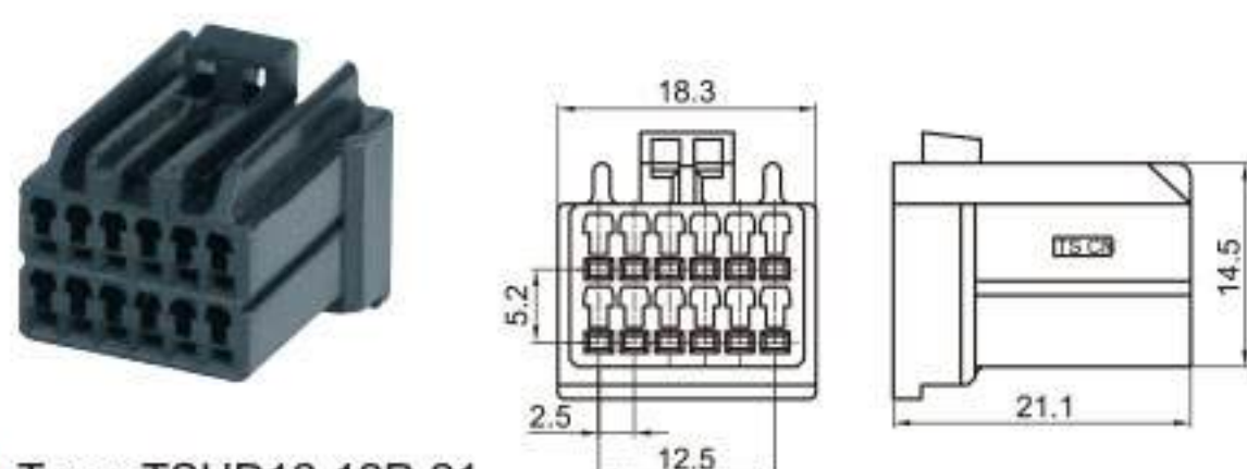
Type: TSHD12-12P-21 Material: PA66 Matching Terminal: TSH006
