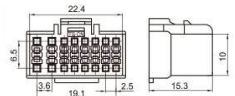
Type: TSPAN01A-16P-21 Material: PA66 GF30% Matching Terminal: TSH503 / TSH031B
