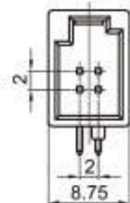
Type: TS30147-04PM-PKB-1 Material: PBT GF15% Matching Terminal: TSPM0140 / TSPM0077
