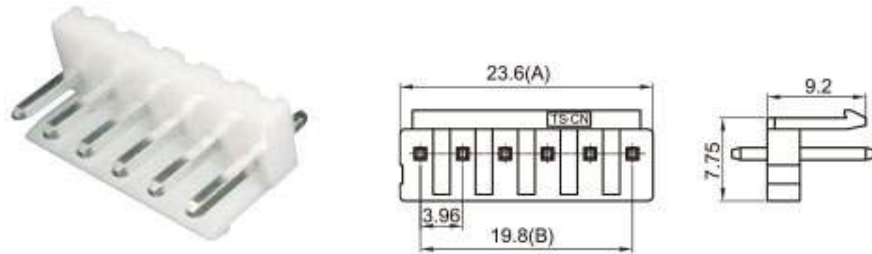
Type: TSVH-06PM-PKS(02P-15P) Material: PA66 Matching Terminal: TSPM0298
