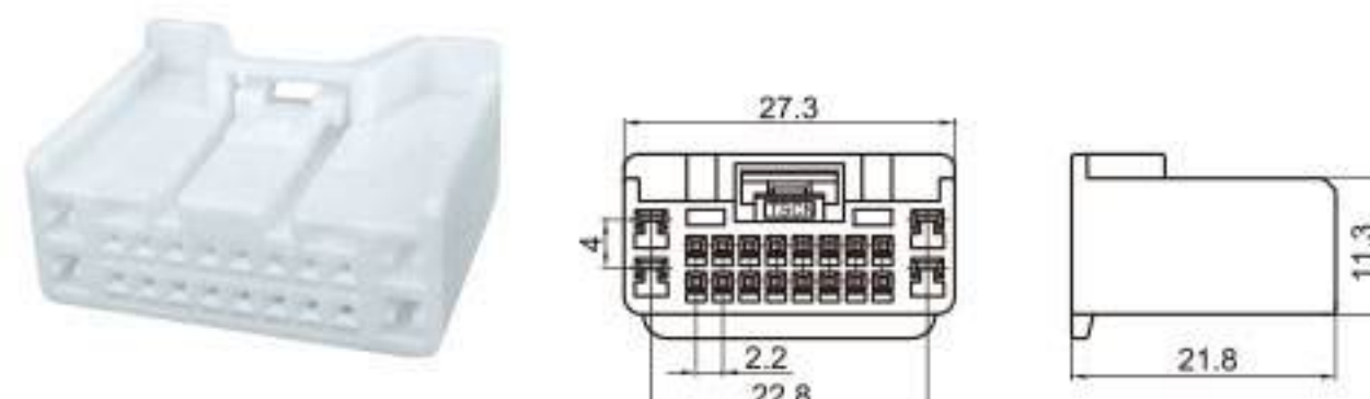
Type: TS30202-20P-21 Material: PA66 Matching Terminal: TSH541 / TSH143
