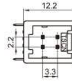
Type: TS30213-04PM-PKB Material: PBT GF15% Matching Terminal: TSPM0270~TSPM0274
