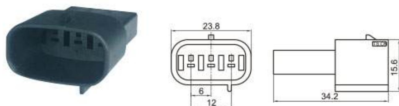
Type: TS30019-03P-11 Material: PA66 GF30% Matching Terminal: TSZ010B
