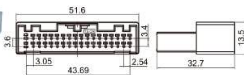
Type: TS30285-36P-11 Material: PBT GF30% Matching Terminal: TSZ040 / TSZ616
