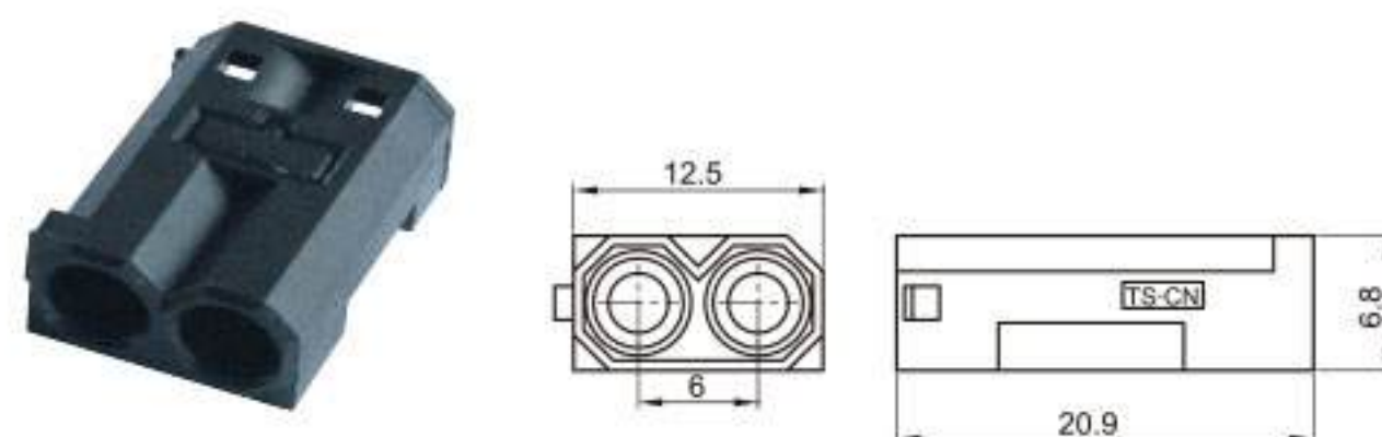
Type: TSBMGQ-A Material: PA66 GF15% Matching Terminal: TSBMGQ-B
