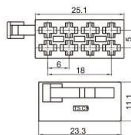
Type: TS1784A-08P-21-4BK Material: PA66 Matching Terminal: TSH019
