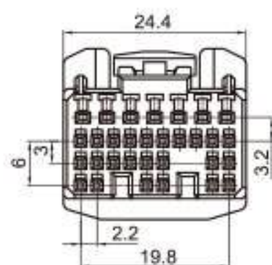
Type: TS30124-31P-21 Material: PA66 Matching Terminal: TSH076 / TSH143
