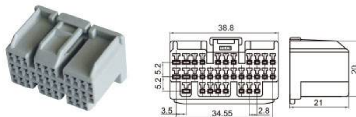
Type: TSWH104-32P-21 Material: PA66 Matching Terminal: TSH009 / TSH076
