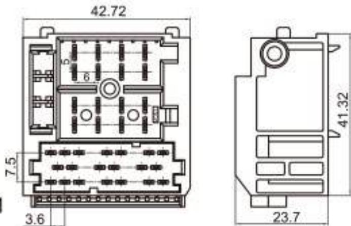
Type: TSVW36-36PM-PKS Material: PA66 GF30% Matching Terminal: TSPM0114~TSPM0118
