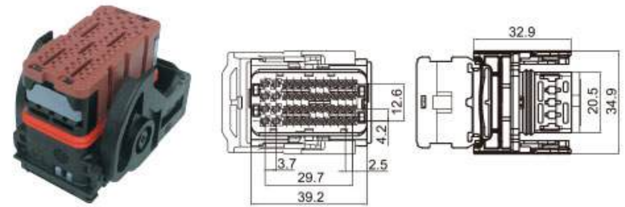
Type: TS30245-48P-21-2 Material: PA66 Matching Terminal: TSH632 / TS643221029
