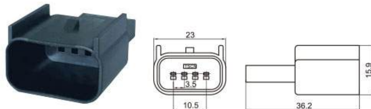
Type: TS30173-04P-11 Material: PBT Matching Terminal: TSZ040
