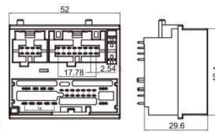
Type: TS5520-24PM-PKB Material: PA66 GF30% Matching Terminal: TSPM0009~TSPM0014
