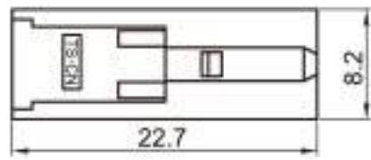
Type: TS2HD21-02PF-AT-1 Material: PA66 Matching Terminal: TSH143 / TSTF0007 / TSTM0004
