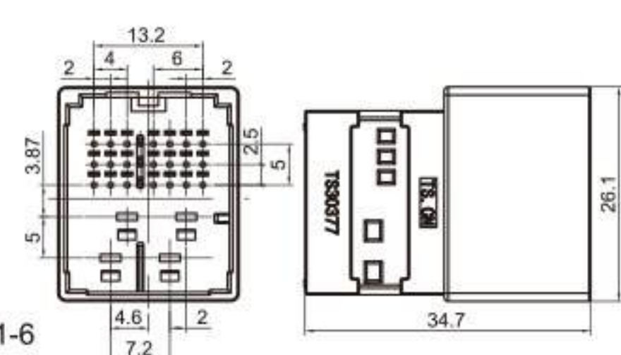
Type: TS30377-25P-21-5 Material: PA66 Matching Terminal: TSH019C / TSH606
