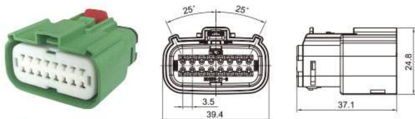
Type: TS30359-16P-21-3 Material: PA66 GF30% Matching Terminal: TSH047
