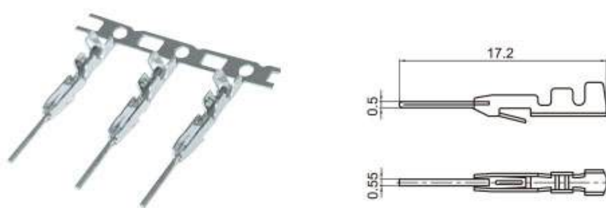
Type: TSZ534 Material: Brass
