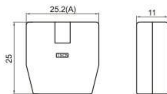
Type: TS43025-14P-21 黄盖 (06P-24P) Material: ABS Matching Terminal: NIL
