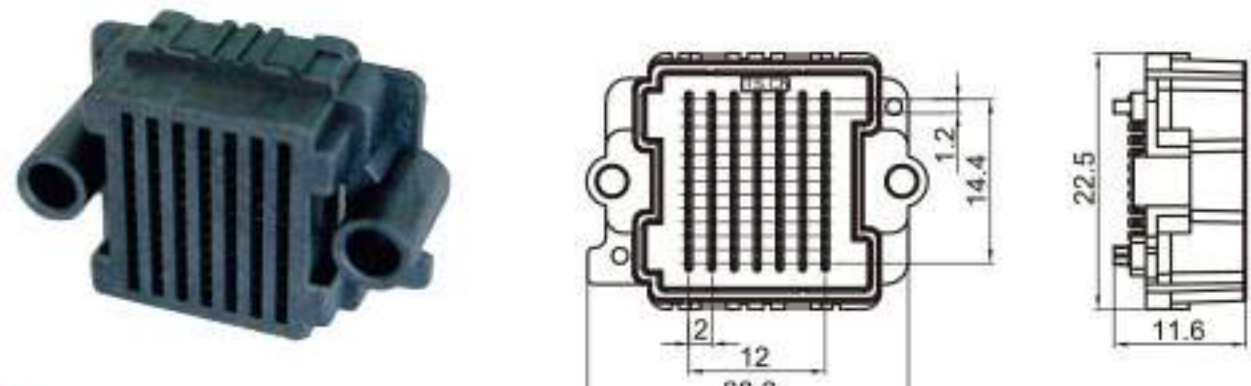
Type: TS30034-91PF-PKS Material: LCP GF30% Matching Terminal: TSPF0001 / TSPF0002
