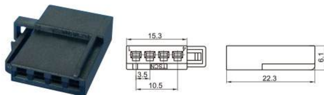
Type: TS30180-04P-21 Material: PA66 GF30% Matching Terminal: TSH593
