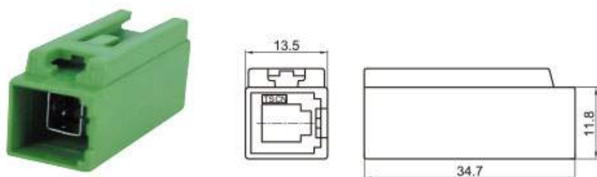
Type: TSTA10-01PM-AT Material: PA66 Matching Terminal: TSPM0012 / TSPM0013
