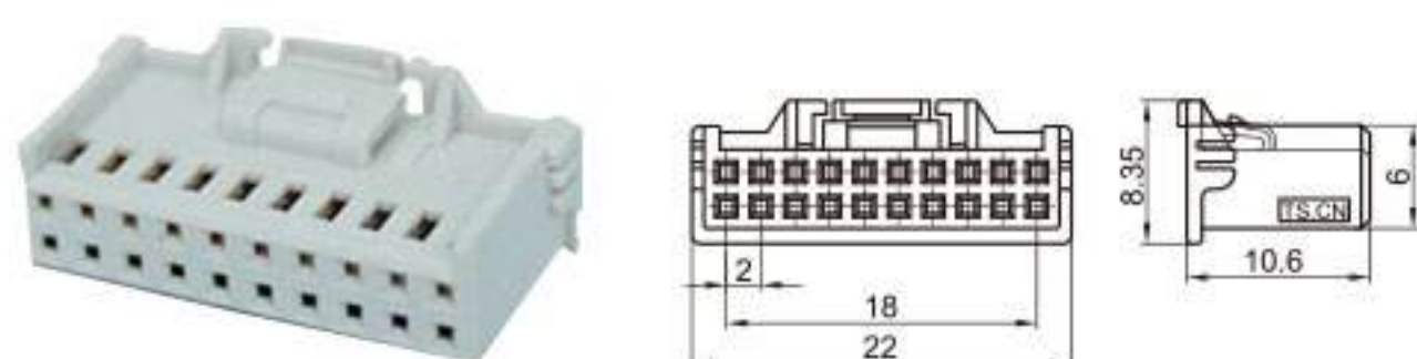
Type: TS30046-20P-21(QRA3) Material: PA66 GF15% Matching Terminal: TSPHB
