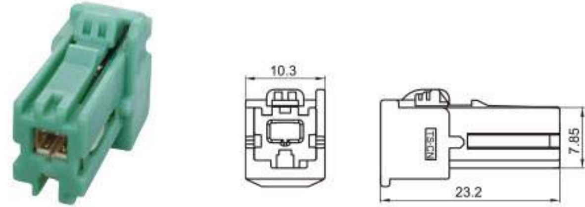
Type: TS30211-02PF-AT-2 Material: PBT Matching Terminal: TSTF0058 / TSTF0059 / TSTF0006
