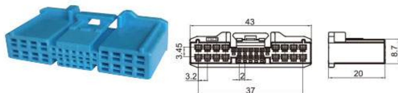
Type: TS30243-28P-21-4 Material: PA66 Matching Terminal: TSH593 / TSH606
