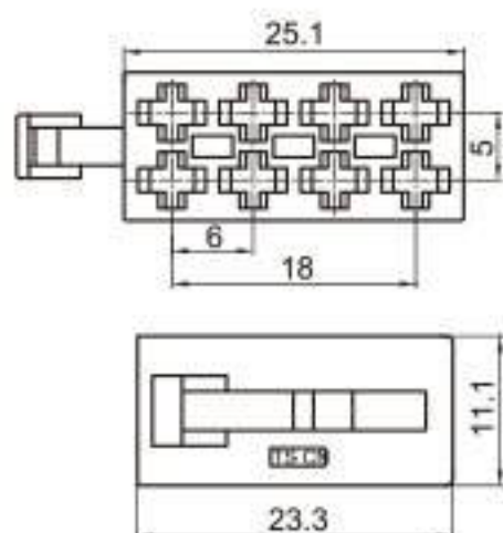
Type: TS1784A-08P-21-4BN Material: PA66 Matching Terminal: TSH019
