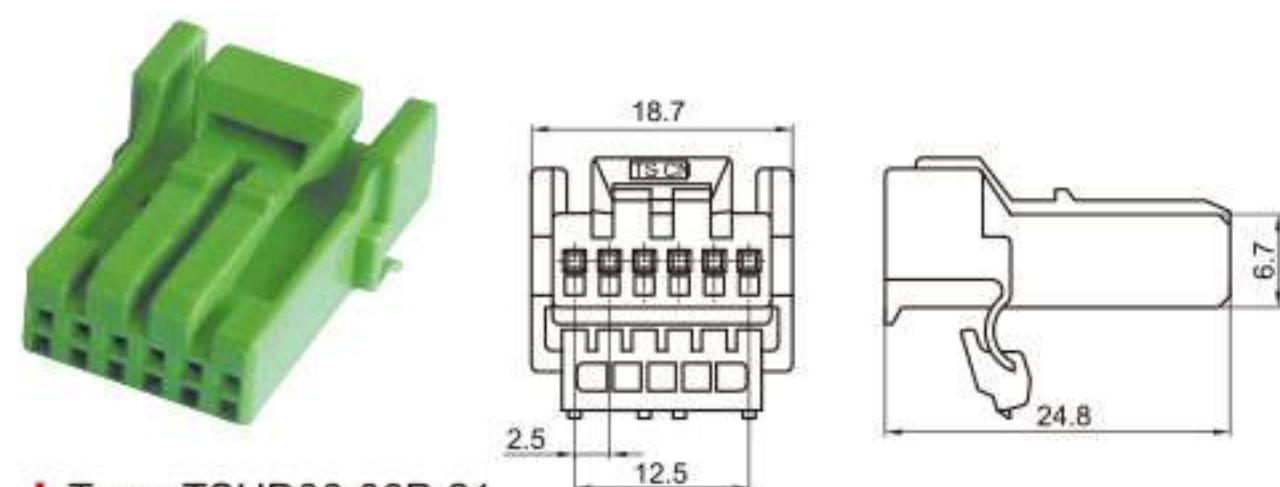
Type: TSHD06-06P-21 Material: PA66 Matching Terminal: TSH066
