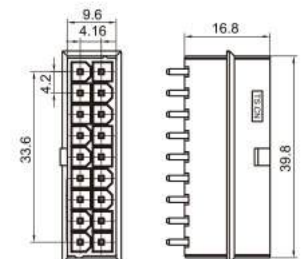
Type: TS30383-18PM-PKS Material: PA66 GF30% Matching Terminal: TSPM0341
