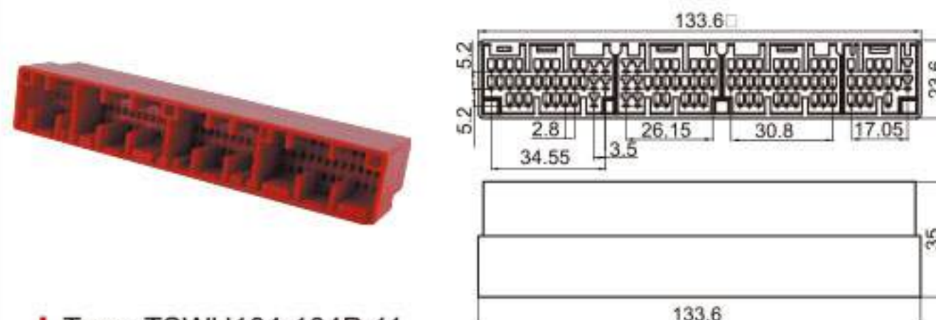
Type: TSWH104-104P-11 Material: PA66 Matching Terminal: TSZ007 / TSZ145
