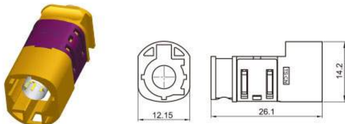
Type: TSVW10-04PM-AT-5BN-1 Material: PA66 GF15% Matching Terminal: TSPM0175 / TSTM0051
