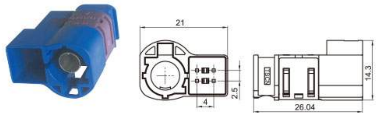
Type: TSVW10-08PM-AT-1BL Material: PBT GF15% Matching Terminal: TSPM0175 / TSTM0051 / TSZ208
