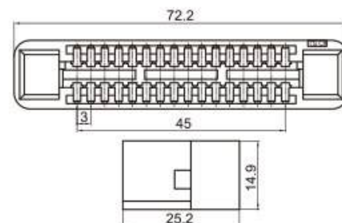
Type: TSGM07RB-32P-21 Material: PA66 Matching Terminal: TSH088
