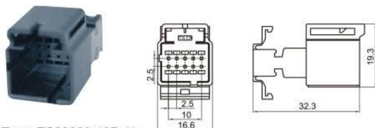
Type: TS30063-10P-11 Material: PA66 Matching Terminal: TSZ208B
