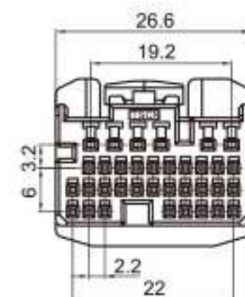
Type: TS30124-35P-21-1 Material: PA66 Matching Terminal: TSH076 / TSH143
