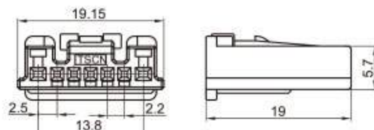
Type: TS30185-07P-21 Material: PA66 GF30% Matching Terminal: TSH076 / TSH143
