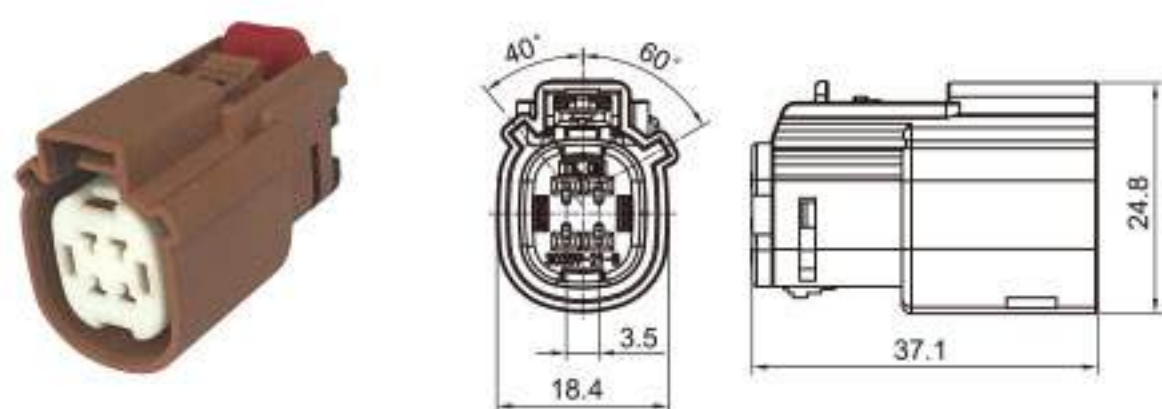
Type: TS30359-04P-21-2 Material: PA66 GF30% Matching Terminal: TSH047
