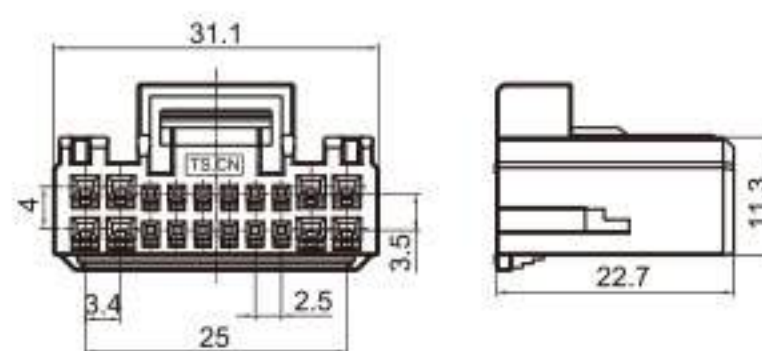
Type: TS30302-20P-21 Material: PBT Matching Terminal: TSH651 / TSH624
