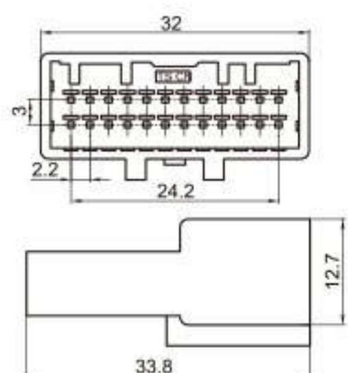
Type: TSTA24-24P-11-4 Material: PA66 Matching Terminal: TSZ208
