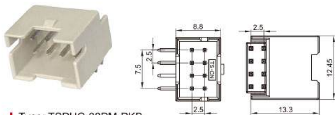
Type: TSPHC-08PM-PKB Material: PA66 GF15% Matching Terminal: TSPM0039 / TSPM0126
