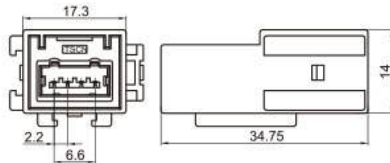
Type: TSTYUSB-04PM-AT-2 Material: ABS Matching Terminal: TSTM0017 / TSPM0016
