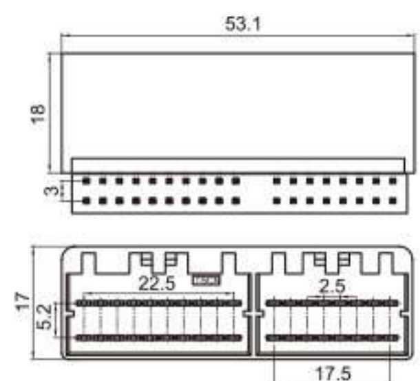
Type: TSHD36-36PM-PKB-1 Material: PA66 Matching Terminal: TSPM0088 / TSPM0089
