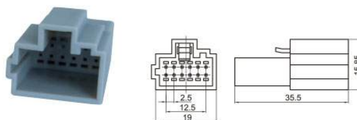
Type: TS30106-12P-11 Material: PA66 Matching Terminal: TSZ208B
