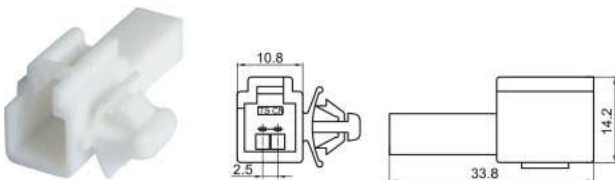
Type: TSLB04-02P-11 Material: PA66 Matching Terminal: TSZ145
