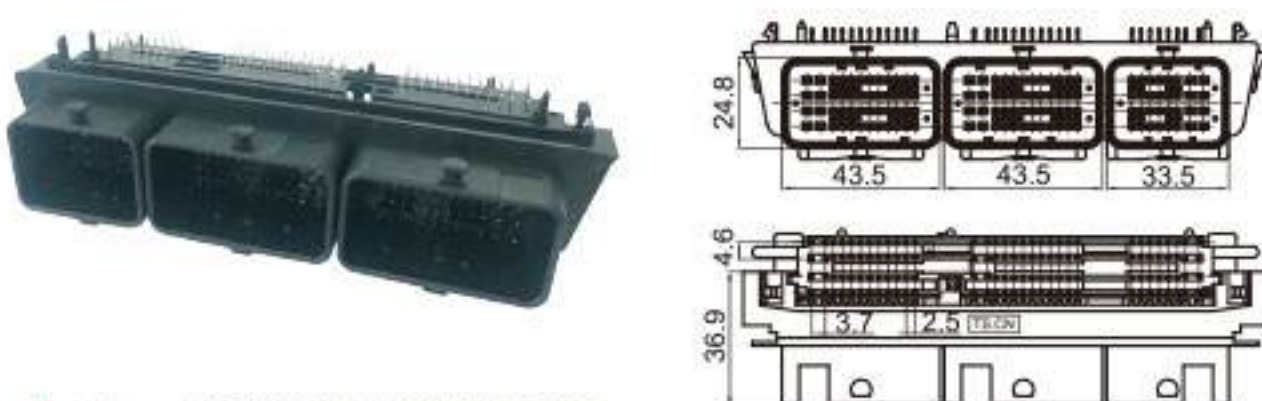
Type: TS30245-128PM-PKB Material: PA66 GF30% Matching Terminal: TSPM0277~TSPM0288
