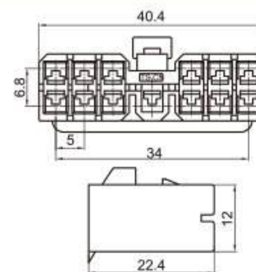
Type: TS1782-13P-21 Material: PA66 Matching Terminal: TSH017
