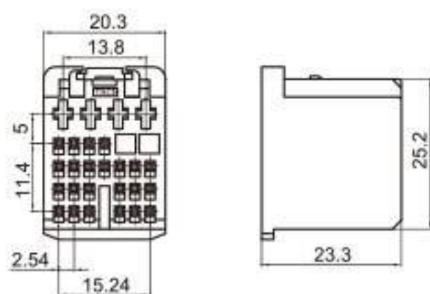
Type: TS30217-30P-21-5 Material: PBT GF10% Matching Terminal: TSH019 / TSH092
