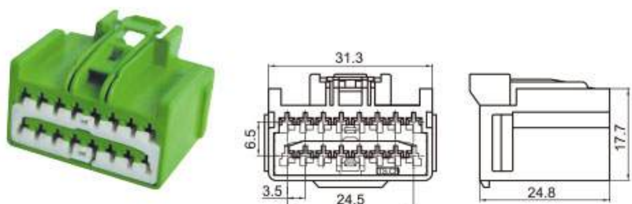
Type: TSVO16-16P-21-1 Material: PBT GF10% Matching Terminal: TSH047
