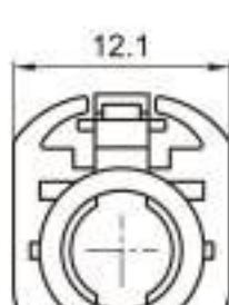
Type: TSVW20-04PF-AT-5BK Material: PA66 GF30% Matching Terminal: TSTF0048 / TSTF0049 / TSTF0050
