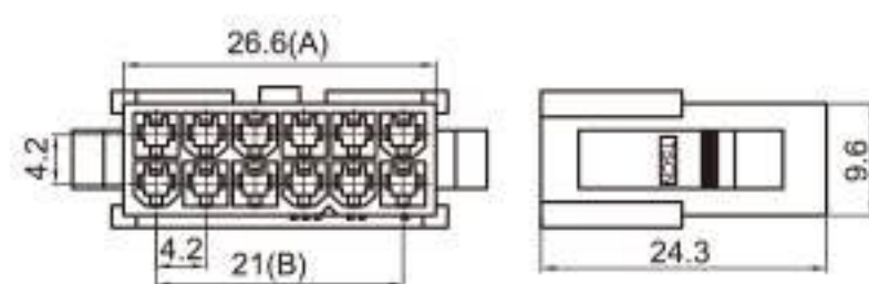
Type: TS5557-12P-11(02P-24P) Material: PA66 Matching Terminal: TSZ558
