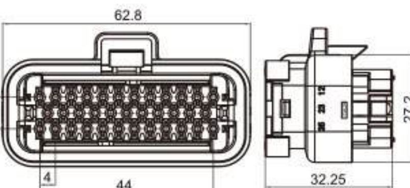
Type: TS30256-35P-21(TS3018) Material: ABS+PC Matching Terminal: TSH640
