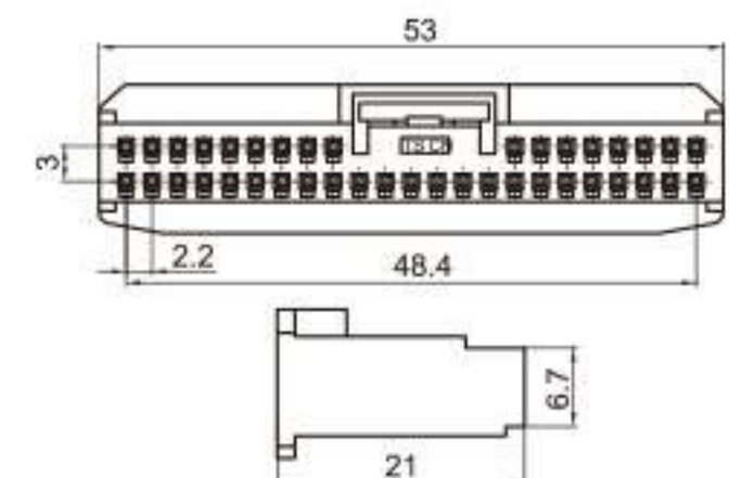
Type: TSTA40-40P-21-1 Material: PA66 Matching Terminal: TSH143
