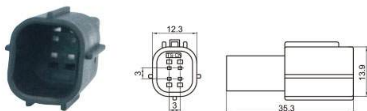
Type: TS1055-04P-11 Material: PA66 GF30% Matching Terminal: TSZ208
