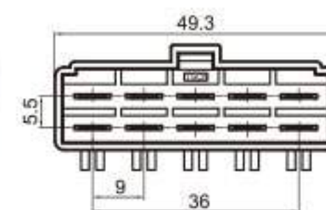
Type: TS30198-10PM-PKB Material: PA66 GF30% Matching Terminal: TSPM0308 / TSPM0309
