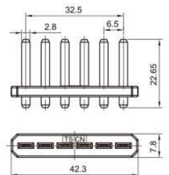
Type: TS30384-06PM-PKS Material: PA66 Matching Terminal: TSPM0342
