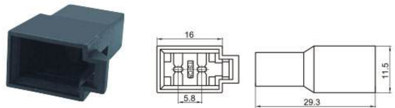
Type: TSLB21-02P-11 Material: PA66 Matching Terminal: TSZ024
