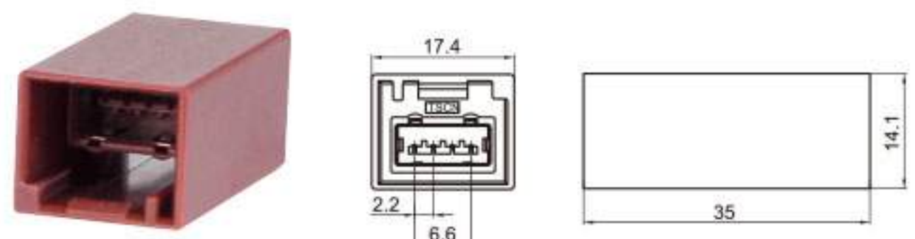
Type: TSTYUSB-04PM-AT Material: PA66 GF30% Matching Terminal: TSTM0017 / TSPM0016
