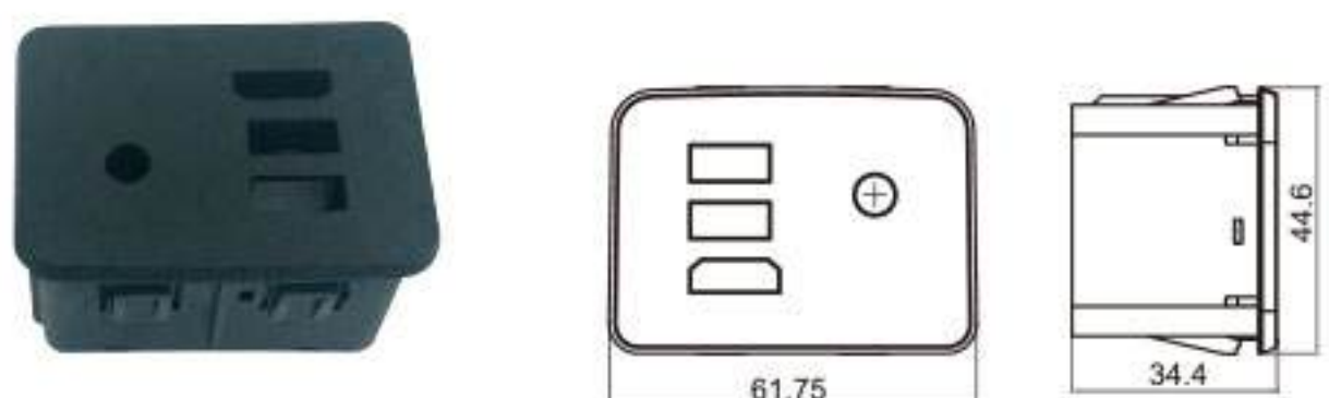
Type: TS30227 Material: PA66 GF30% Matching Terminal: TSHDMI-F / TSUSB-F / TS3.5-F
