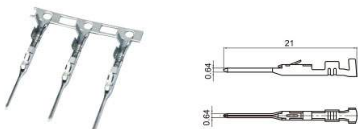
Type: TSZ537 Material: Brass
