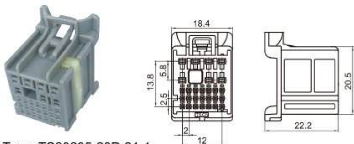
Type: TS30205-28P-21-1 Material: PA66 Matching Terminal: TSH606 / TSH092
