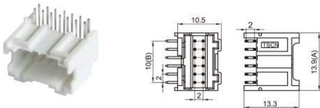
Type: TSPHS-14PM-PKB(10P-24P) Material: PBT GF15% Matching Terminal: TSPM0196 / TSPM0197
