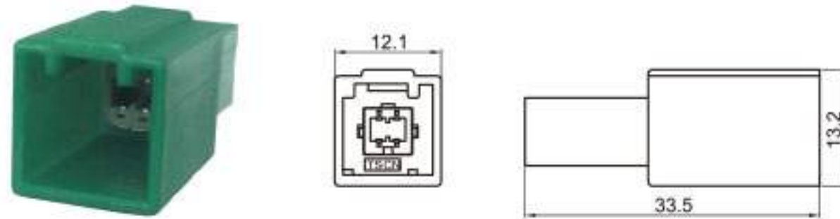
Type: TSTA04-04PM-AT-1 Material: PA66 GF30% Matching Terminal: TSTM0008-A / TSPM0218
