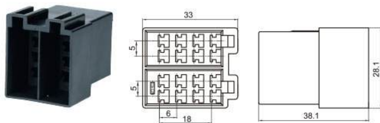
Type: TSVW16-16P-11 Material: PA66 Matching Terminal: TSZ054
