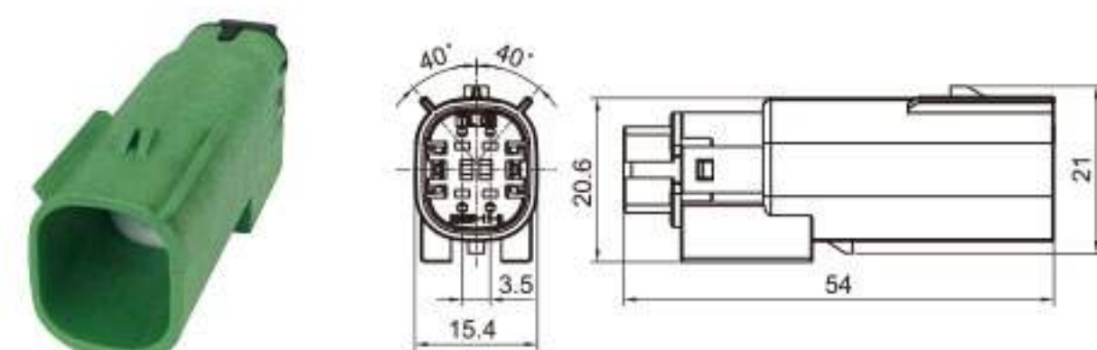
Type: TS30359-04P-11-3 Material: PA66 GF30% Matching Terminal: TSZ144A
