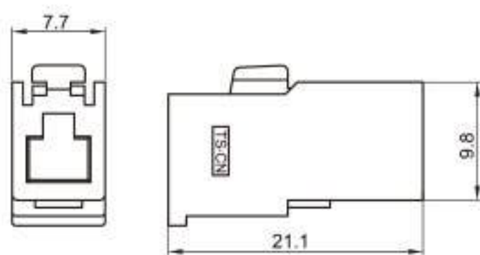
Type: TSK121-01PF-AT Material: PA66 Matching Terminal: TSTF0001 / TSTF0002
