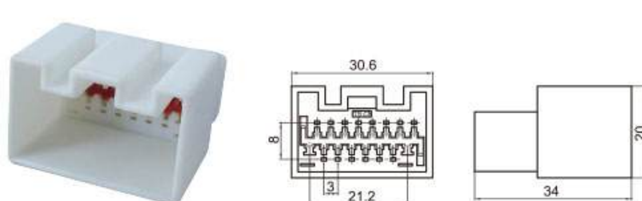
Type: TS1771-16P-11-1 Material: PA66 Matching Terminal: TSZ011 / TSZ018
