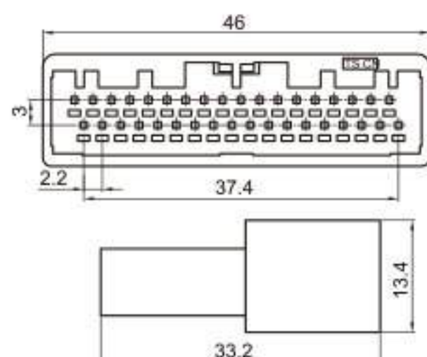
Type: TSCR36-36P-11-1 Material: PA66 Matching Terminal: TSZ208B
