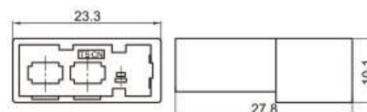
Type: TSN110-03PM-AT Material: PA66 Matching Terminal: TSZ040 / TSTM0001 / TSTM0002
