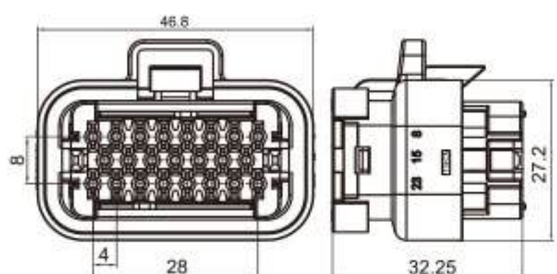
Type: TS30256-23P-21(TS3017) Material: ABS+PC Matching Terminal: TSH640
