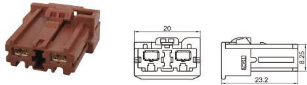
Type: TS30212-04PF-AT-1 Material: PBT Matching Terminal: TSTF0058 / TSTF0059 / TSTF0006
