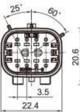
Type: TS30359-08P-11-1 Material: PA66 GF30% Matching Terminal: TSZ144A
