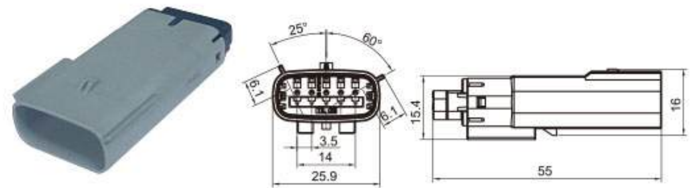
Type: TS30366-05P-11-1 Material: PA66 GF30% Matching Terminal: TSZ144A
