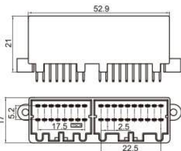
Type: TSHD36-36PM-PKS-2 Material: PA66 GF30% Matching Terminal: TSPM0091
