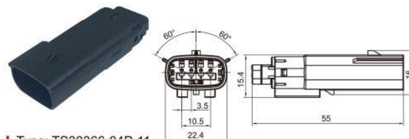
Type: TS30366-04P-11 Material: PA66 GF30% Matching Terminal: TSZ144A
