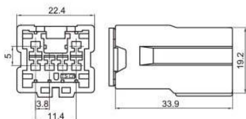
Type: TS7503-16P-11 Material: PA66 Matching Terminal: TSZ115 / TSZ050
