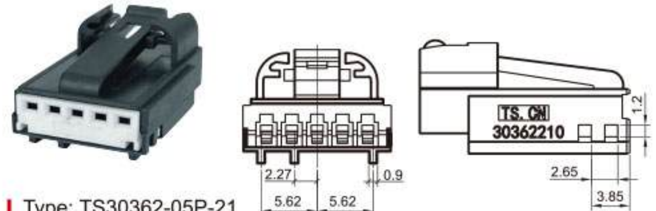
Type: TS30362-05P-21 Material: PA66 GF30% Matching Terminal: TSH006B
