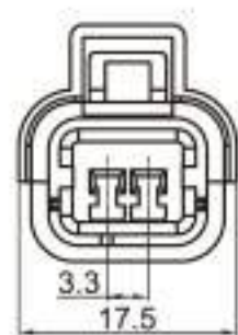
Type: TS30067-02P-21 Material: PA66 GF30% Matching Terminal: TSH047
