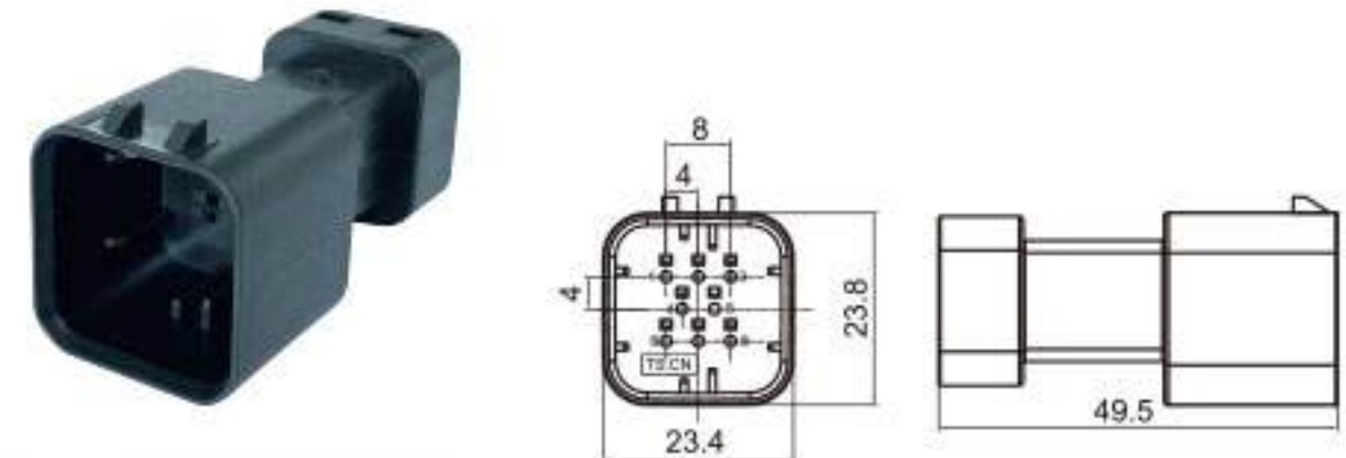
Type: TS30256-08P-11 Material: PBT GF15% Matching Terminal: TSZ072
