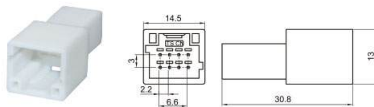
Type: TSRN08-08P-11-1 Material: PA66 Matching Terminal: TSZ208
