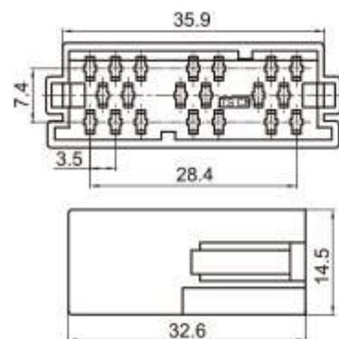
Type: TSAD20-20P-11 Material: PA66 Matching Terminal: TSZ040
