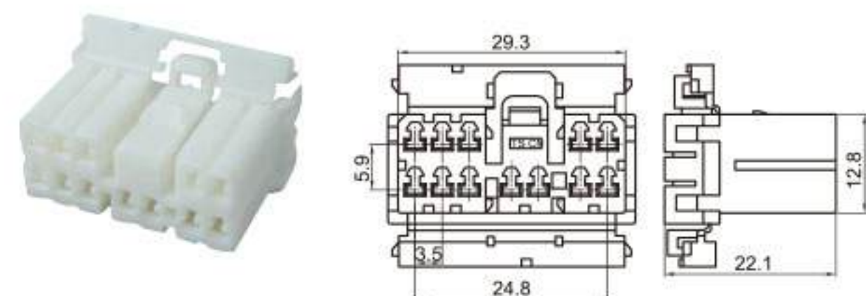
Type: TS7901-12P-21 Material: PA66 Matching Terminal: TSH016
