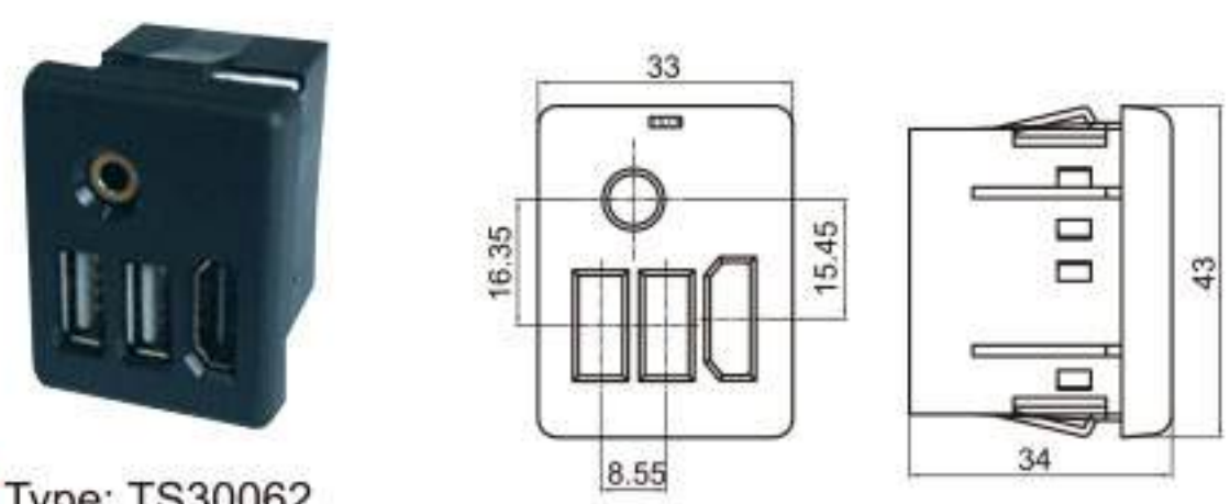
Type: TS30062 Material: PA66 GF30% Matching Terminal: TSHDMI-F / TSUSB-F / TS3.5-F
