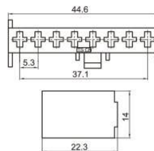
Type: TS1777-08P-21 Material: PA66 Matching Terminal: TSH019
