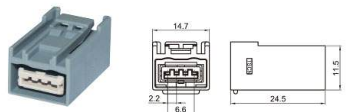
Type: TSTYUSB-04PF-AT Material: PA66 Matching Terminal: TSTF0021 / TSTF0006
