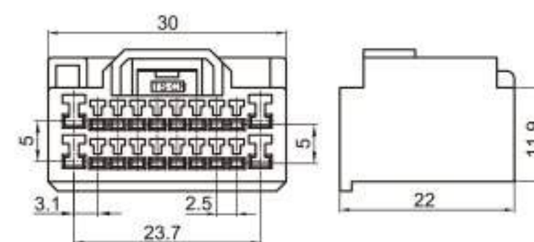
Type: TS7005-20P-21 Material: PA66 Matching Terminal: TSH009 / TSH006
