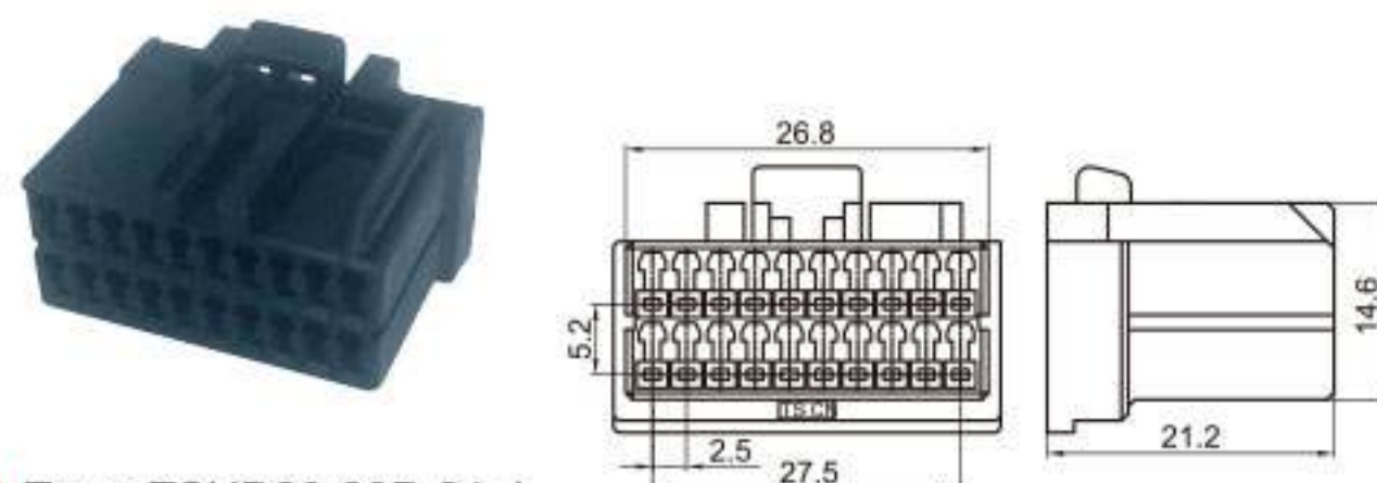
Type: TSHD20-20P-21-4 Material: PA66 Matching Terminal: TSH006
