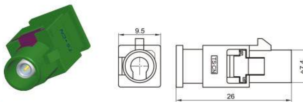
Type: TSVW10-01PM-AT-GN Material: PA66 Matching Terminal: TSTM0019 / TSTM0020
