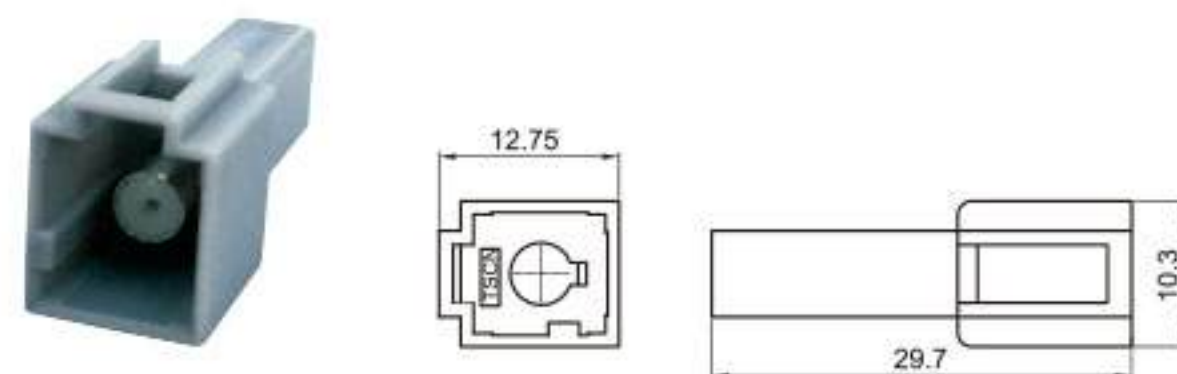
Type: TS30114-01PM-AT Material: PA66 Matching Terminal: TSTM0007/TSTF0004
