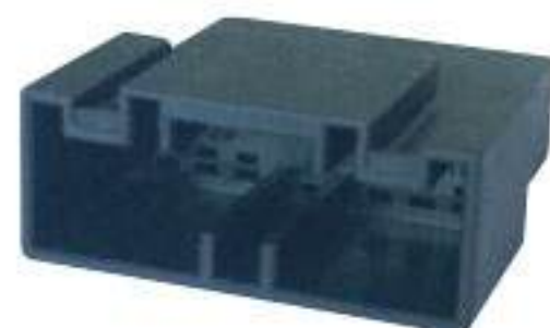
Type: TS30161-16P-11 Material: PA66 GF30% Matching Terminal: TSZ040 / TSZ208
