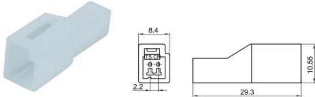
Type: TSLB13-02P-11 Material: PA66 Matching Terminal: NIL
