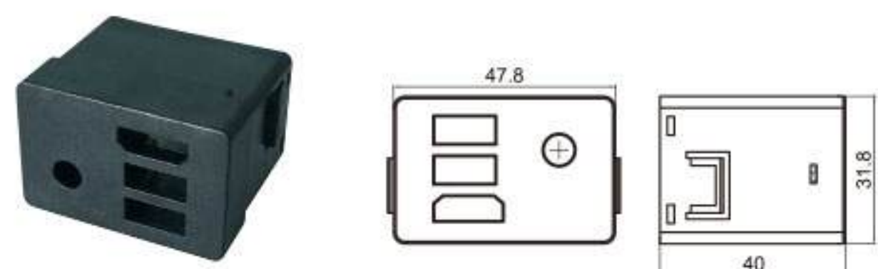
Type: TS30221 Material: PA66 GF30% Matching Terminal: TSHDMI-F / TSUSB-F / TS3.5-F
