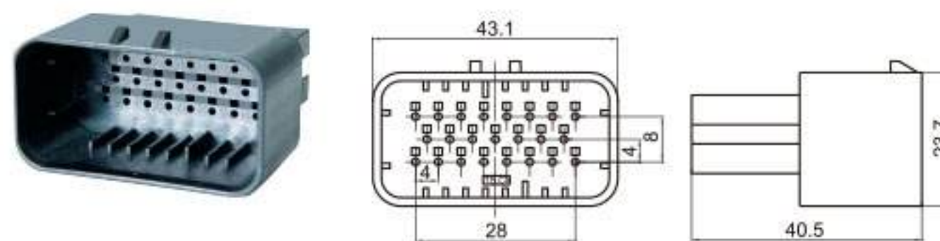
Type: TS3017-23P-11(30256) Material: PA66 GF30% Matching Terminal: TSZ072
