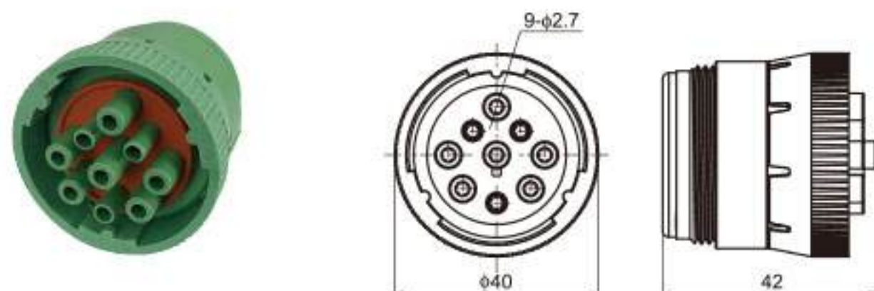
Type: TS30361-09P-21 Material: PA66 GF30% Matching Terminal: TSH646
