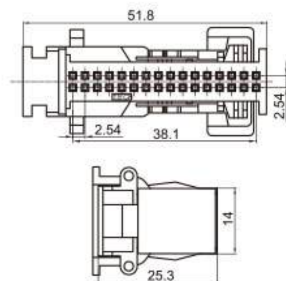
Type: TSAD32-32P-21-1 Material: PA66 Matching Terminal: TSH092
