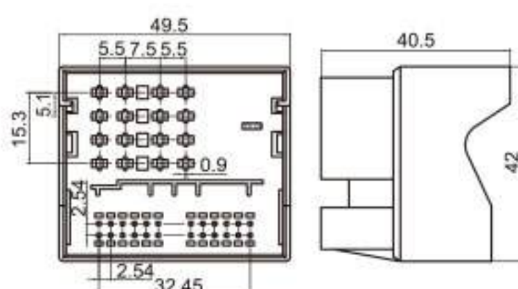
Type: TS9003-40P-11-6 Material: PA66 GF30% Matching Terminal: TSZ024 / TSZ208B
