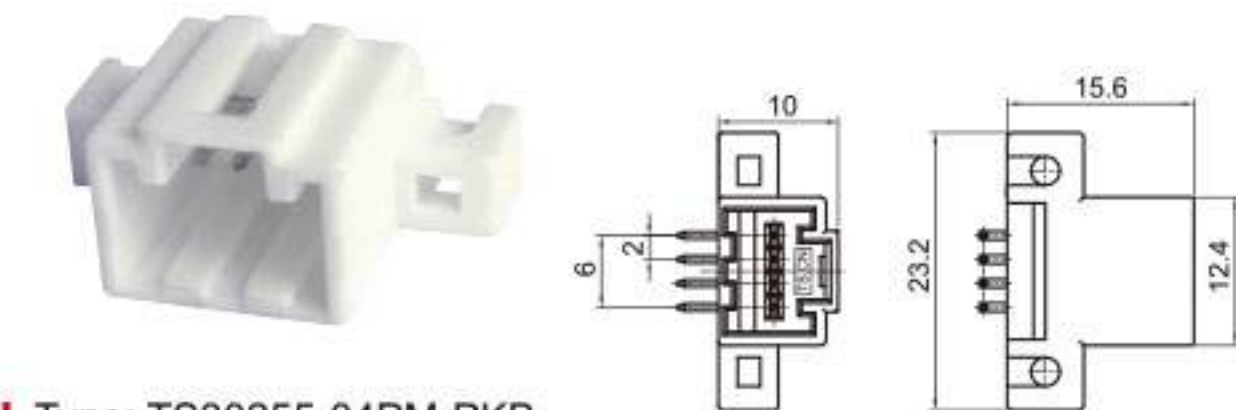
Type: TS30255-04PM-PKB Material: PBT GF15% Matching Terminal: TSPM0300
