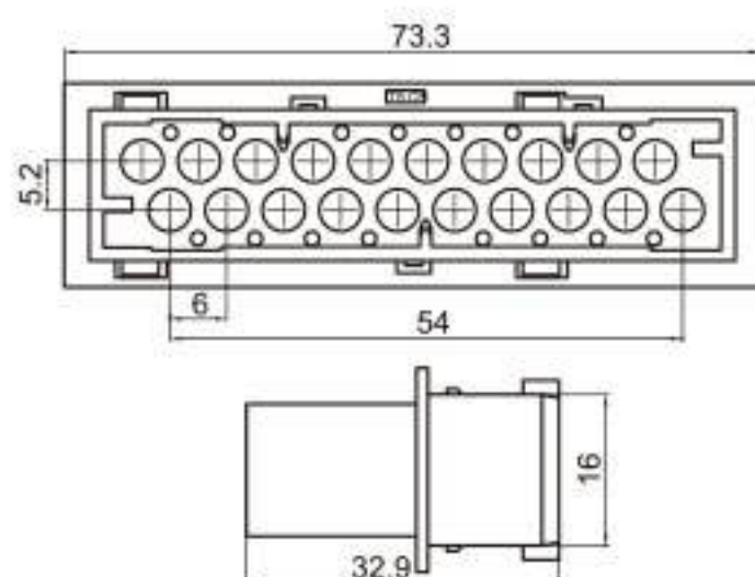
Type: TSBM20-20P-11 Material: PA66 GF30% Matching Terminal: TSZ036
