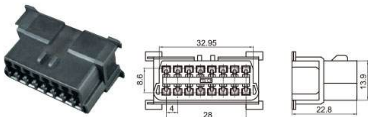
Type: TSOBD-16P-21-3 Material: PA66 GF30% Matching Terminal: TSH009
