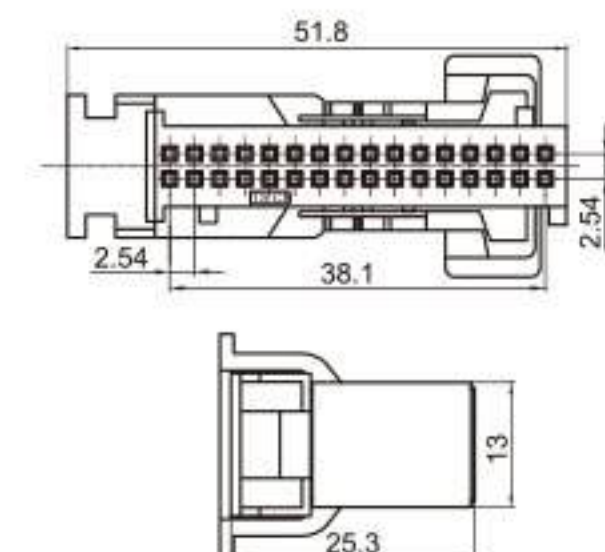
Type: TSAD32-32P-21-3 Material: PA66 Matching Terminal: TSH092
