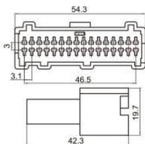
Type: TS2001-32P-11 Material: PA66 Matching Terminal: TSZ013
