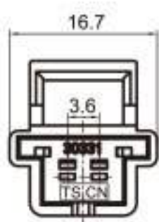
Type: TS30331-02P-11 Material: PA66 GF30% Matching Terminal: TSZ040
