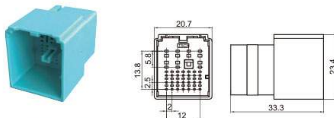
Type: TS30205-28P-11-2 Material: PA66 Matching Terminal: TSZ566 / TSZ561
