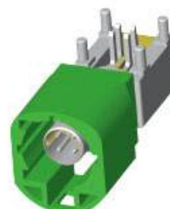
Type: TSVW10-04PM-AT-5GN Material: PA66 GF30% Matching Terminal: TSPM0021~TSPM0025
