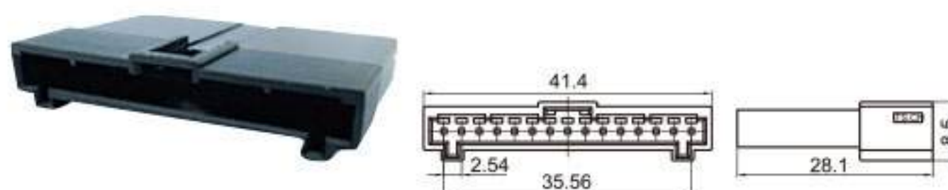
Type: TS30048-15P-11 Material: PA66 GF30% Matching Terminal: TSZ208
