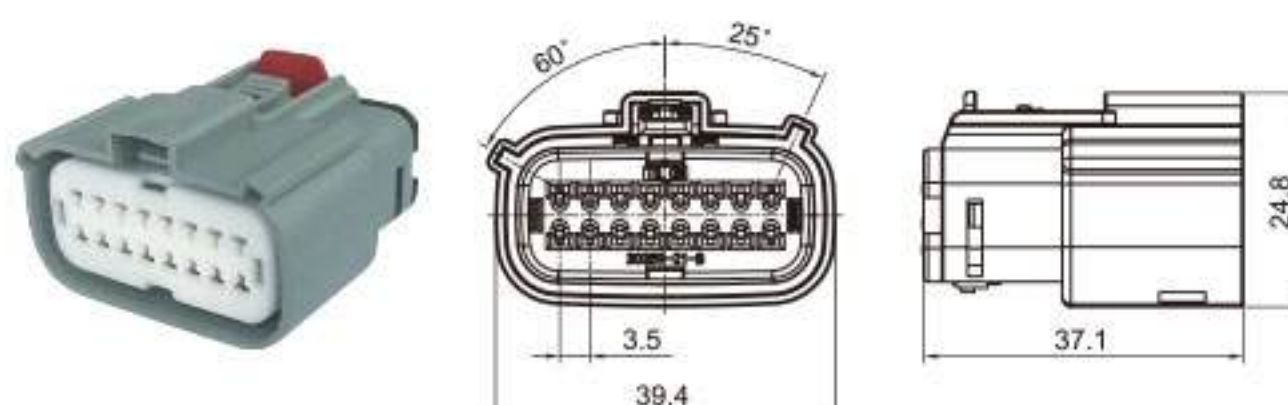
Type: TS30359-16P-21-1 Material: PA66 GF30% Matching Terminal: TSH047
