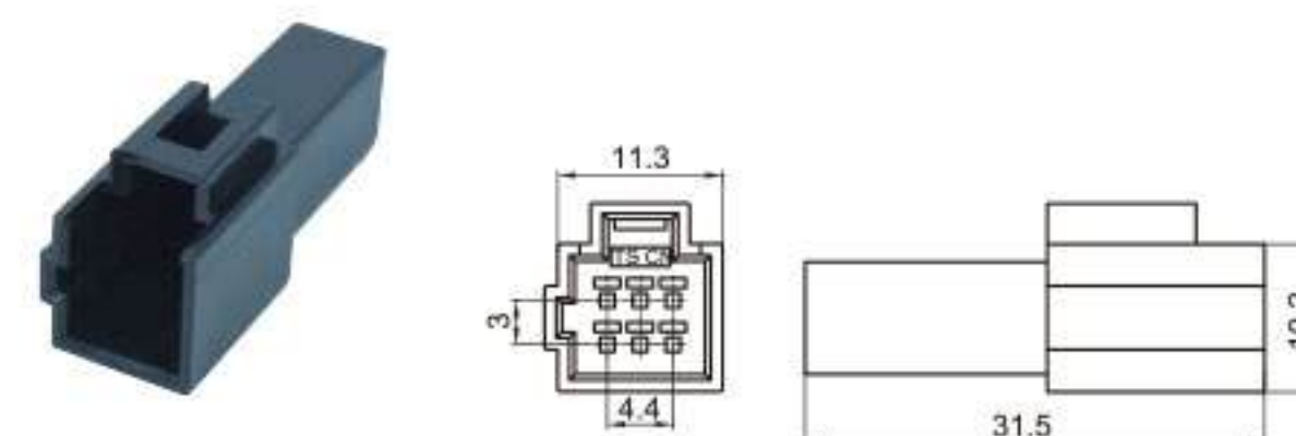
Type: TS3001-06P-11-1 Material: PA66 Matching Terminal: TSZ208
