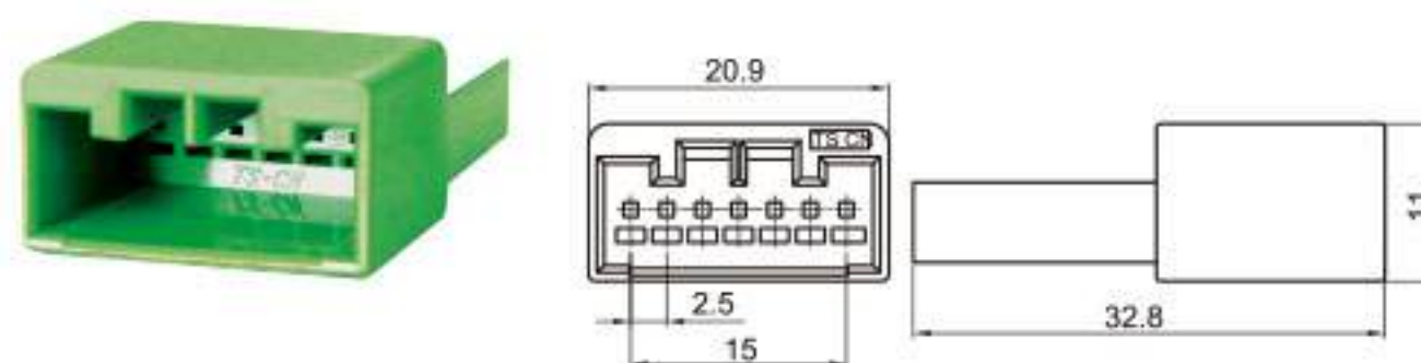
Type: TSHD07-07P-11 Material: PA66 Matching Terminal: TSZ208B
