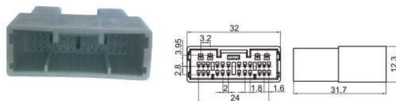
Type: TS30101-28P-11-2 Material: PA66 Matching Terminal: TSZ562 / TSZ556
