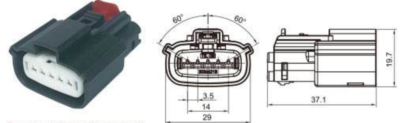
Type: TS30366-05P-21 Material: PA66 GF30% Matching Terminal: TSH047
