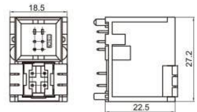
Type: TS30060-10PM-PKS Material: PA66 GF30% Matching Terminal: TSPM0217 / TSPM0215 / TSPM0077 / TSPM0039
