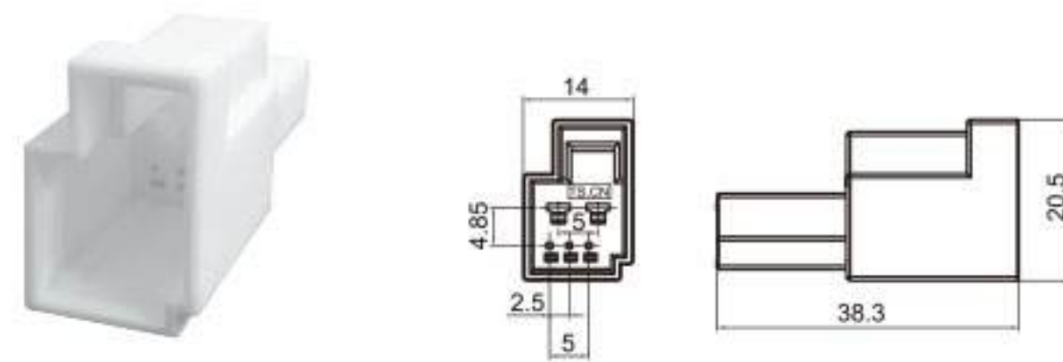
Type: TS30294-05P-11 Material: PBT Matching Terminal: TSZ024 / TSZ616
