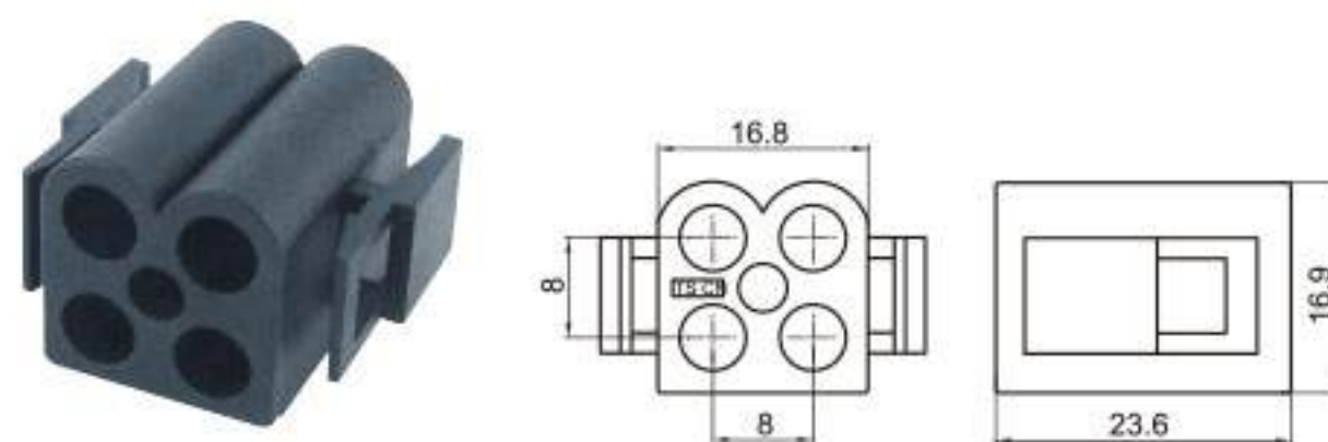
Type: TSVO04-04P-21 Material: PA66 GF15% Matching Terminal: TSH596
