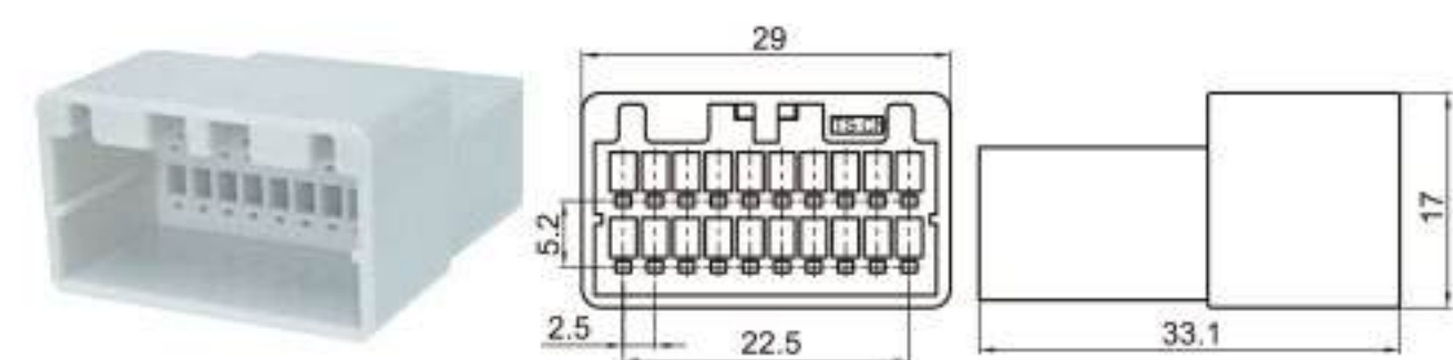
Type: TSHD20-20P-11-7 Material: PA66 Matching Terminal: TSZ145
