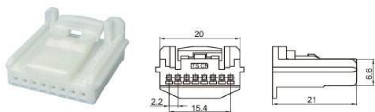
Type: TSTA08-08P-21-1 Material: PA66 Matching Terminal: TSH143
