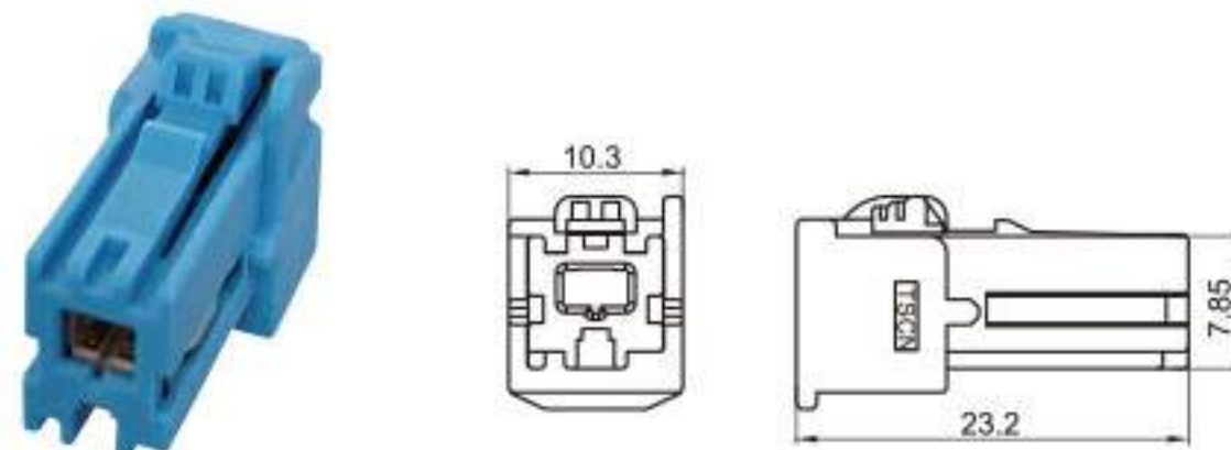
Type: TS30211-02PF-AT-1 Material: PBT Matching Terminal: TSTF0058 / TSTF0059 / TSTF0006
