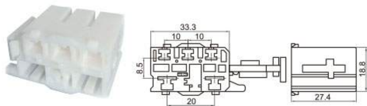
Type: TS30013-05P-21 Material: PBT Matching Terminal: TSH591 / TSH585
