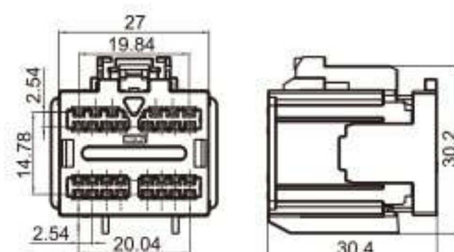
Type: TS30358-30P-21-1 Material: PBT GF10% Matching Terminal: TSH076 / TSH006B
