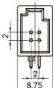
Type: TS30147-04PM-PKB-2 Material: PBT GF15% Matching Terminal: TSPM0140 / TSPM0077
