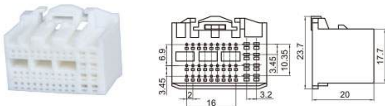
Type: TS30116-38P-21 Material: PA66 Matching Terminal: TSH593 / TSH606
