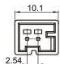
Type: TSLB39-02P-11-2 Material: PA66 GF30% Matching Terminal: TSZ208B
