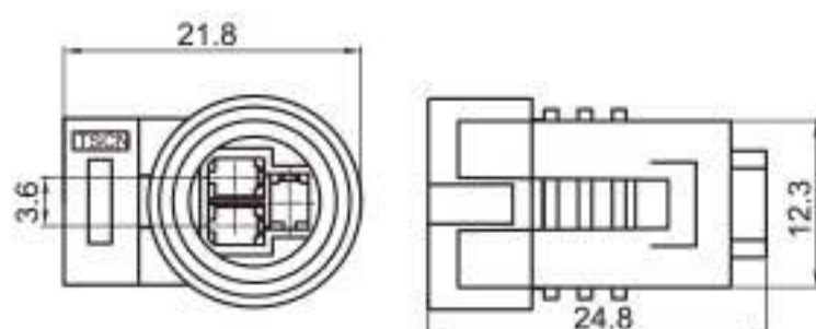
Type: TS30240-03P-21 Material: PBT Matching Terminal: TSDJ624-T1.5A
