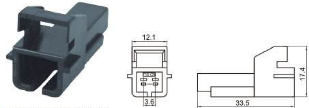
Type: TSLB07-02P-11 Material: PA66 GF30% Matching Terminal: TSZ040
