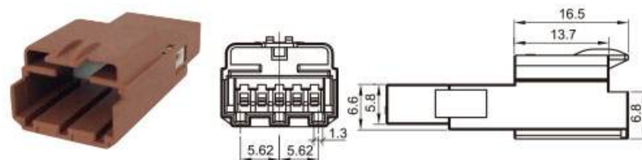
Type: TS30362-05P-11-2 Material: PA66 GF30% Matching Terminal: TSZ145
