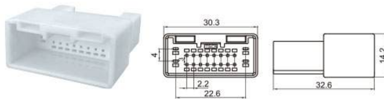
Type: TS30202-20P-11 Material: PA66 Matching Terminal: TSZ040 / TSZ208
