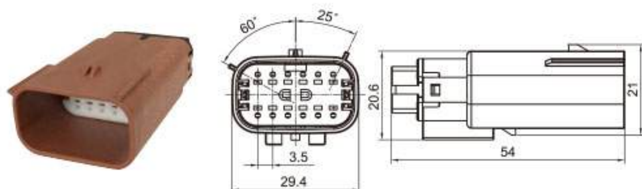
Type: TS30359-12P-11-2 Material: PA66 GF30% Matching Terminal: TSZ144A
