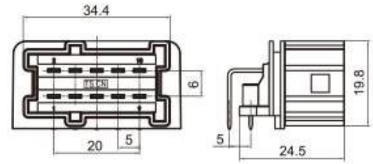
Type: TS30310-10PM-PKB Material: PBT GF15% Matching Terminal: TSPM0314 / TSPM0315
