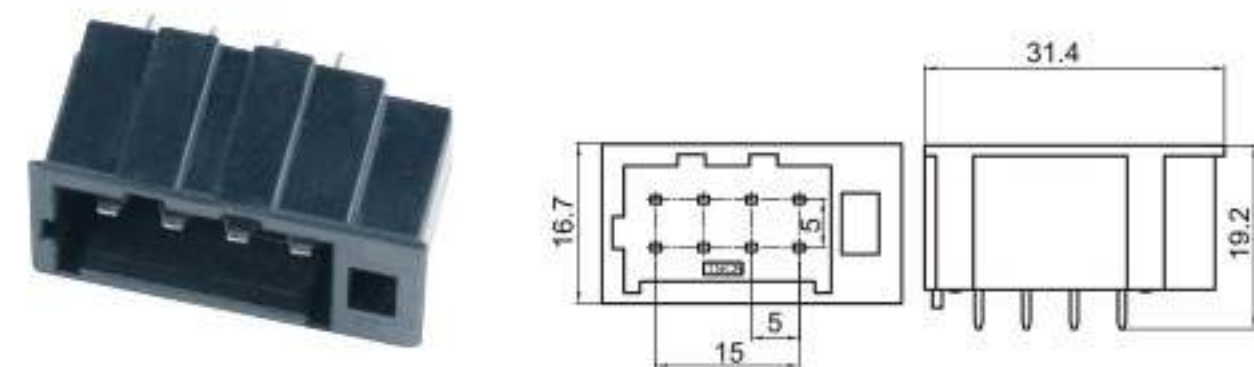
Type: TSABD-08PM-PKS-B Material: PA66 Matching Terminal: TSPM0127
