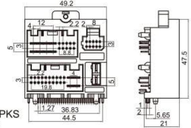
Type: TS30050-74PM-PKS Material: PA66 GF30% Matching Terminal: TSPM0121 / TSPM0207~TSPM0210
