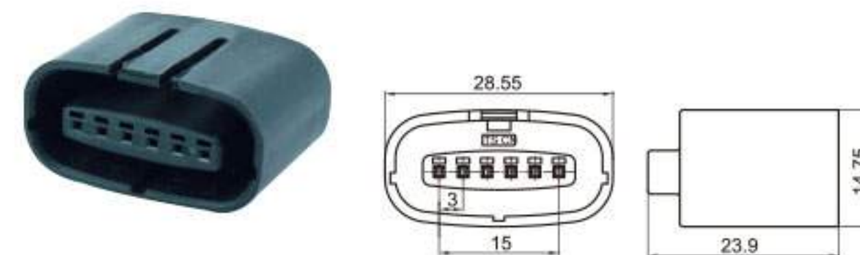
Type: TSTA06-06P-21-1 Material: PA66 GF30% Matching Terminal: TSH143
