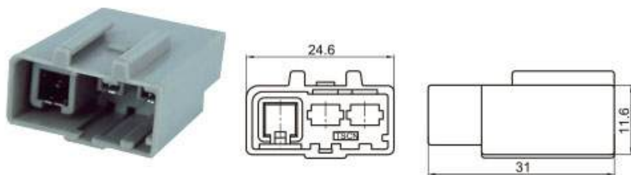
Type: TSSSANG10-03PM-AT Material: PA66 Matching Terminal: TSTM0012 / TSTM0013 / TSTM0001 / TSTM0002
