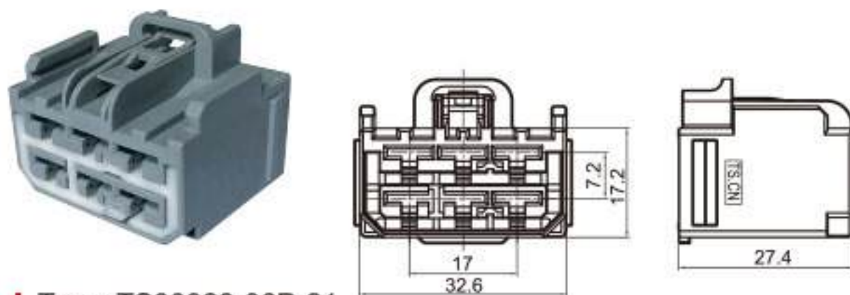
Type: TS30328-06P-21 Material: PBT Matching Terminal: TSH033B
