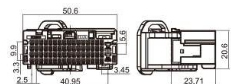
Type: TS30283-66P-21-1 Material: PBT Matching Terminal: TSH064 / TSH092
