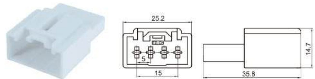
Type: TSLB22-04P-11 Material: PA66 Matching Terminal: TSZ024
