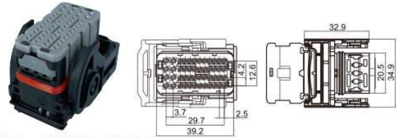
Type: TS30245-48P-21-1 Material: PA66 Matching Terminal: TSH632 / TS643221029
