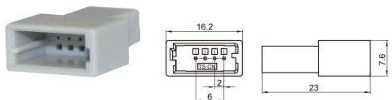
Type: TS1072-04P-11 Material: PA66 Matching Terminal: TSZ534
