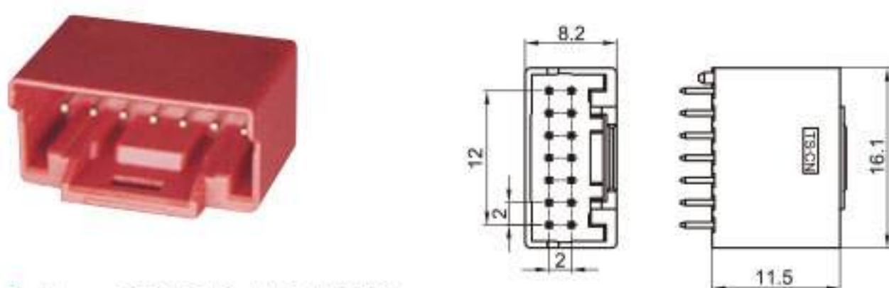
Type: TSQRA3-14PM-PKS Material: PA66 GF30% Matching Terminal: TSPM0145
