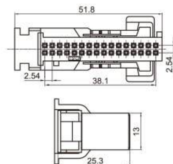
Type: TSAD32-32P-21-2 Material: PA66 Matching Terminal: TSH092
