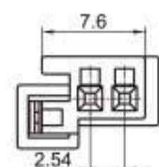
Type: TSLB39-02P-21-2 Material: PA66 GF30% Matching Terminal: TSH143
