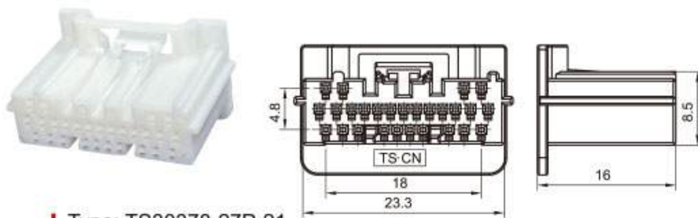
Type: TS30378-27P-21 Material: PA66 Matching Terminal: TSH600A
