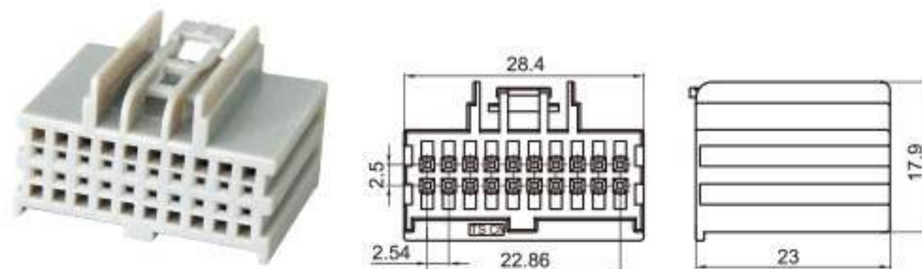
Type: TSGM20-20P-21-2 Material: PA66 GF30% Matching Terminal: TSH143
