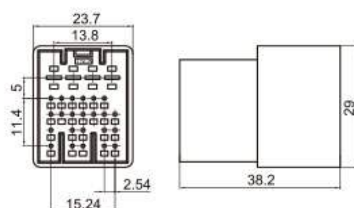
Type: TS30217-30P-11-6 Material: PBT GF15% Matching Terminal: TSDJ615B-2.8*0.8B / TSZ208
