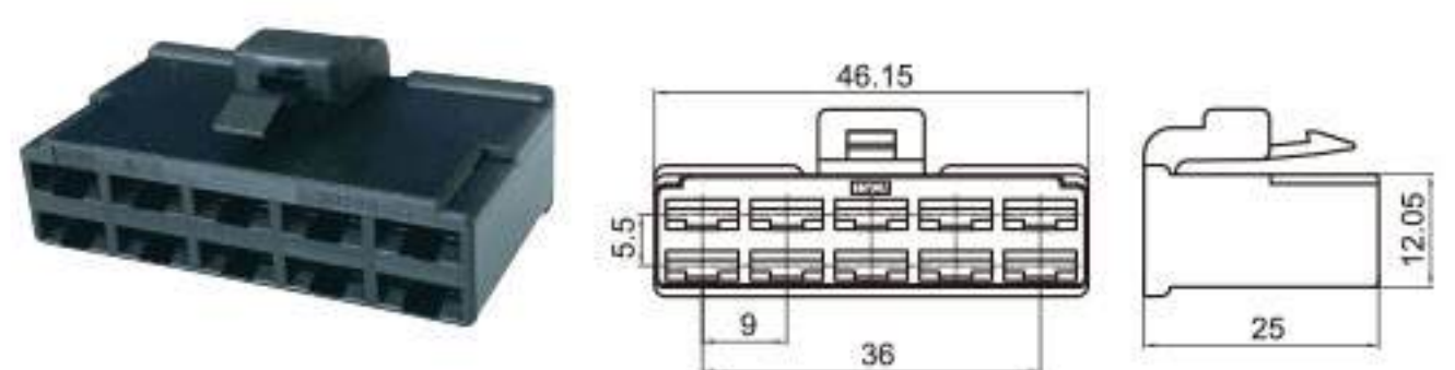
Type: TS30198-10P-21BK Material: PA66 Matching Terminal: TSH033A
