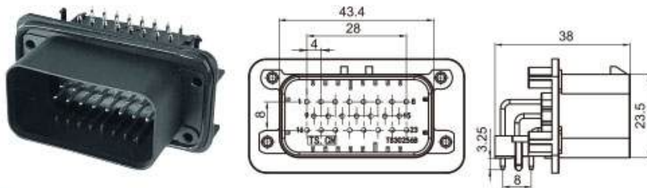
Type: TS30256-23PM-PKB Material: PBT Matching Terminal: TSPM0336~TSPM0338
