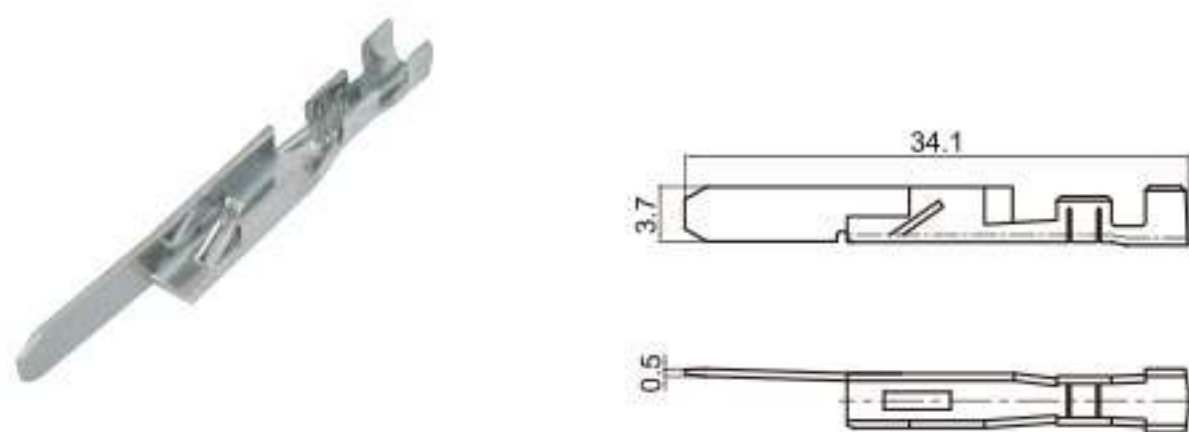
Type: TSZ019 Material: Brass
