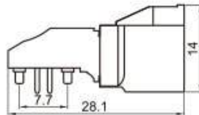
Type: TSVW10-08PM-AT Material: PBT GF30% Matching Terminal: TSPM0022 / TSPM0023 / TSPM0147 / TSPM0151
