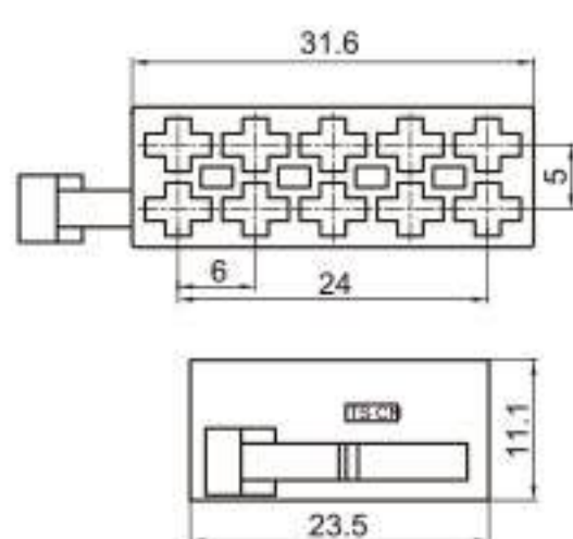
Type: TS9001-10P-21 Material: PA66 Matching Terminal: TSH019
