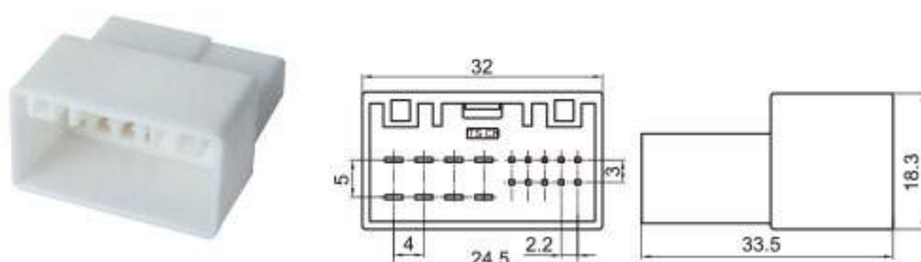
Type: TS7304-18P-11 Material: PA66 Matching Terminal: TSZ009 / TSZ208B
