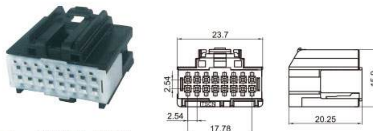
Type: TS30244-16P-21 Material: PBT Matching Terminal: TSH006
