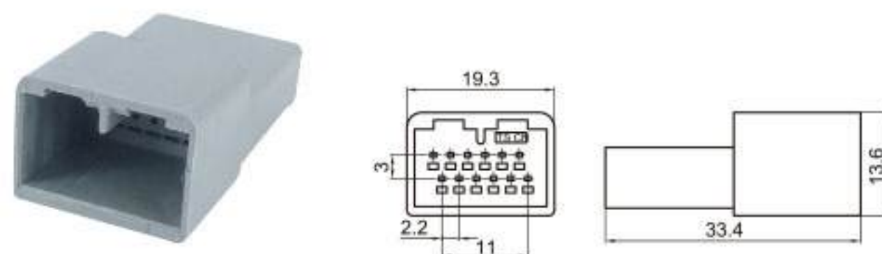
Type: TSCRV12-12P-11 Material: PA66 Matching Terminal: TSZ208B
