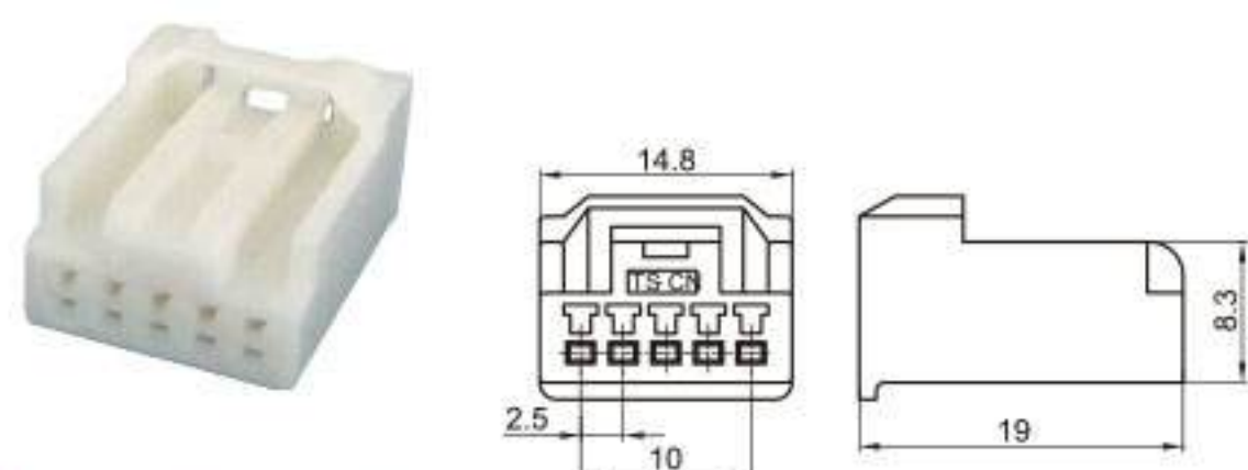
Type: TSTA05-05P-21-1 Material: PA66 Matching Terminal: TSH076
