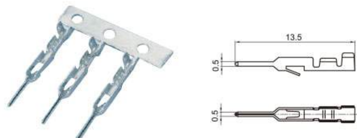
Type: TSZ210 Material: Phos.bronze
