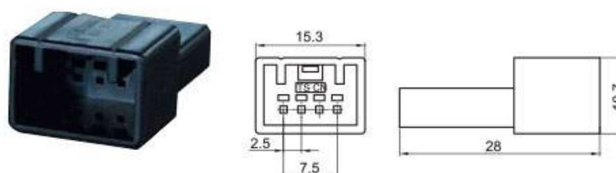
Type: TSTA04-04P-11-1 Material: PA66 Matching Terminal: TSZ208
