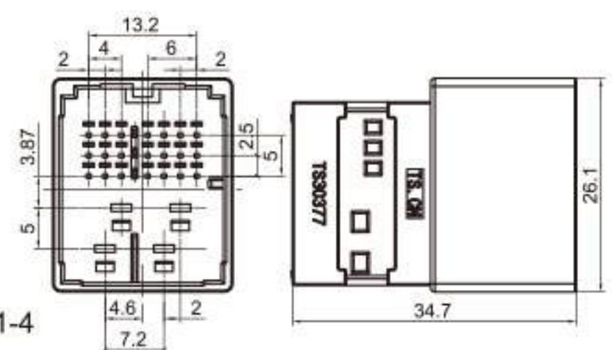
Type: TS30377-25P-21-3 Material: PA66 Matching Terminal: TSH019C / TSH606
