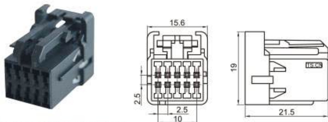
Type: TS30063-10P-21 Material: PA66 Matching Terminal: TSH592
