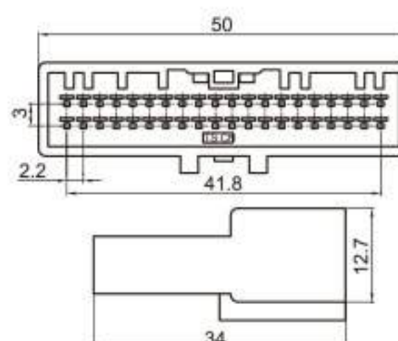
Type: TSTA40-40P-11-4 Material: PA66 Matching Terminal: TSZ208
