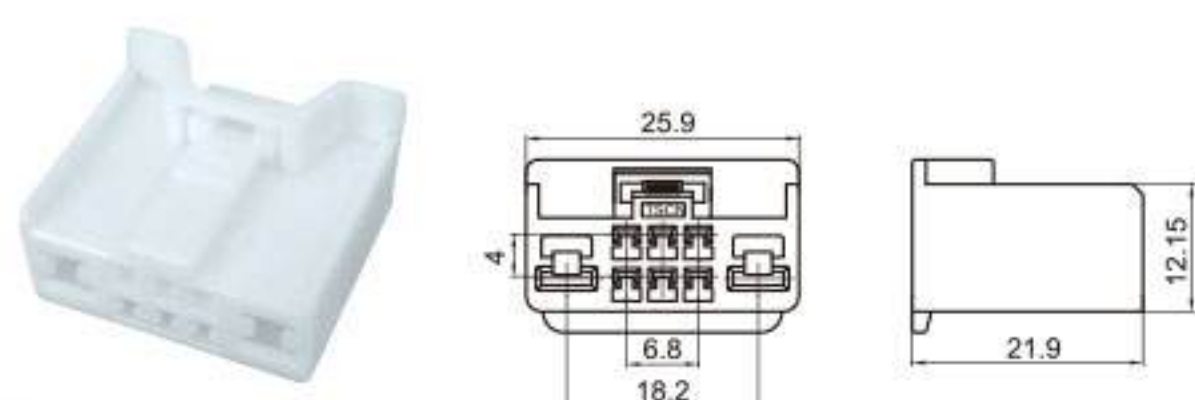
Type: TS30201-08P-21 Material: PA66 Matching Terminal: TSH541 / TSH585
