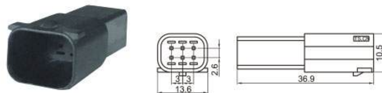
Type: TS30010-06P-11 Material: PA66 Matching Terminal: TSZ208B
