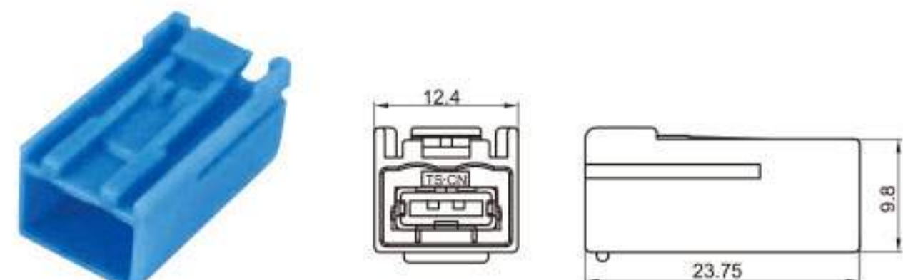
Type: TSKI41-02PF-AT Material: PA66 Matching Terminal: TSTF0005 / TSTF0006
