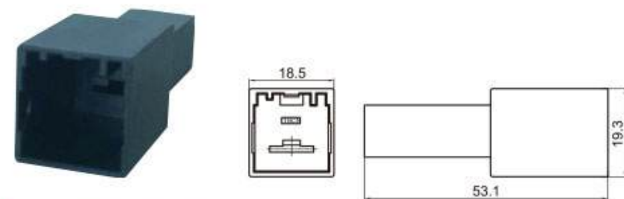
Type: TS30179-01P-11 Material: PBT GF15% Matching Terminal: TSDJ612-9.5*1.2C
