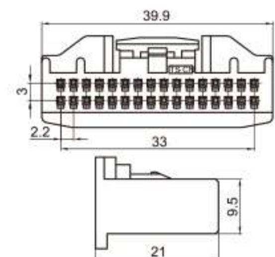
Type: TSTA32-32P-21 Material: PA66 Matching Terminal: TSH143
