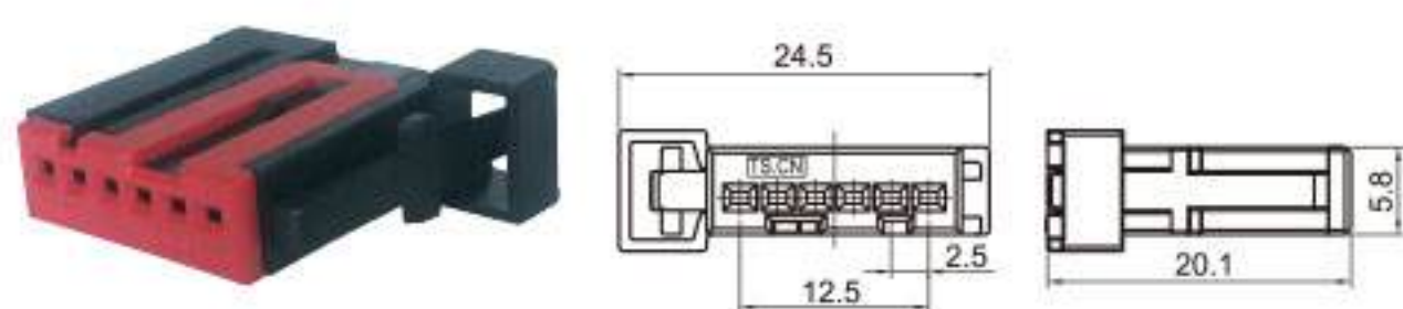
Type: TS30290-06P-21 Material: PA66 GF30% Matching Terminal: TSH624
