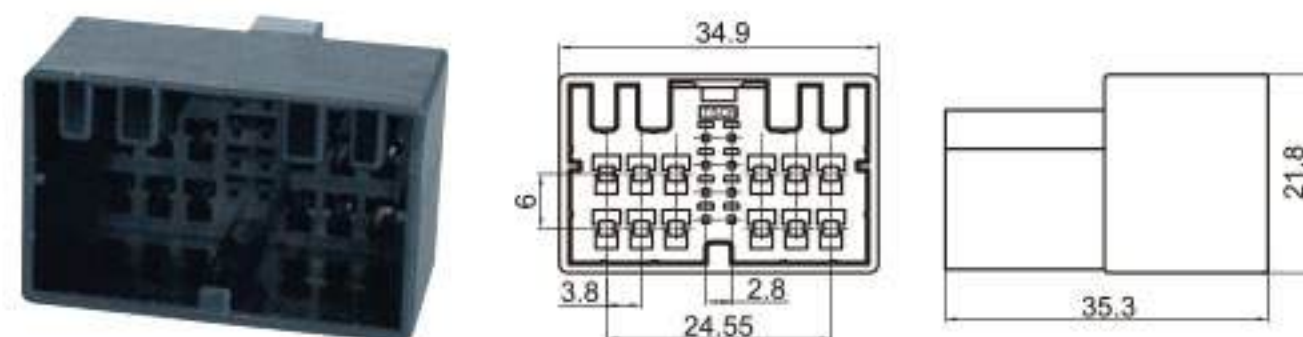
Type: TS30071-20P-11 Material: PA66 GF30% Matching Terminal: TSZ009 / TSZ208
