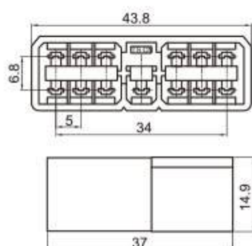
Type: TS1782-13P-11 Material: PA66 Matching Terminal: TSZ004
