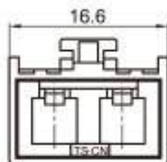
Type: TSVL20-02PF-AT Material: PA66 GF15% Matching Terminal: TSTF0014 / TF0015
