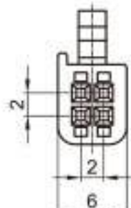
Type: TS30147-04P-21-1 Material: PA66 Matching Terminal: TSH009
