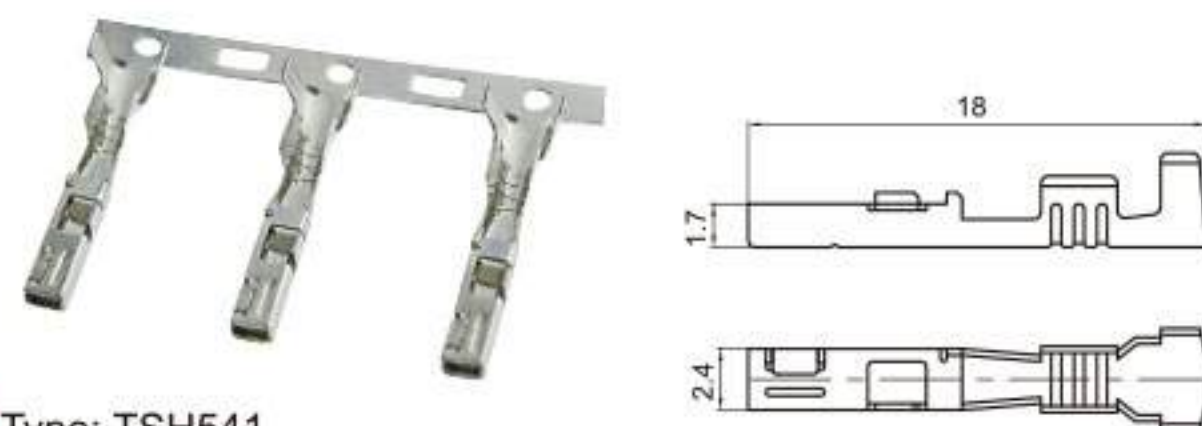
Type: TSH541 Material: Phos.bronze Applicable Thickness: 0.6
