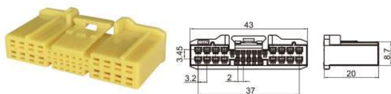
Type: TS30243-28P-21-6 Material: PA66 Matching Terminal: TSH593 / TSH606
