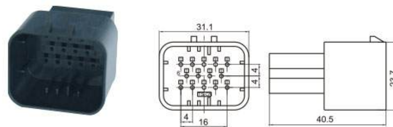
Type: TS3016-14P-11(30256) Material: PA66 GF30% Matching Terminal: TSZ072
