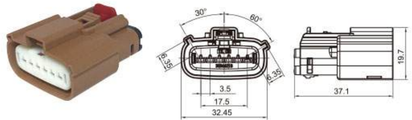
Type: TS30366-06P-21-2 Material: PA66 GF30% Matching Terminal: TSH047
