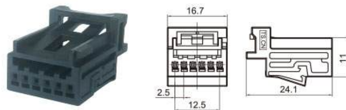
Type: TS30293-06P-21 Material: PBT GF10% Matching Terminal: TSH624
