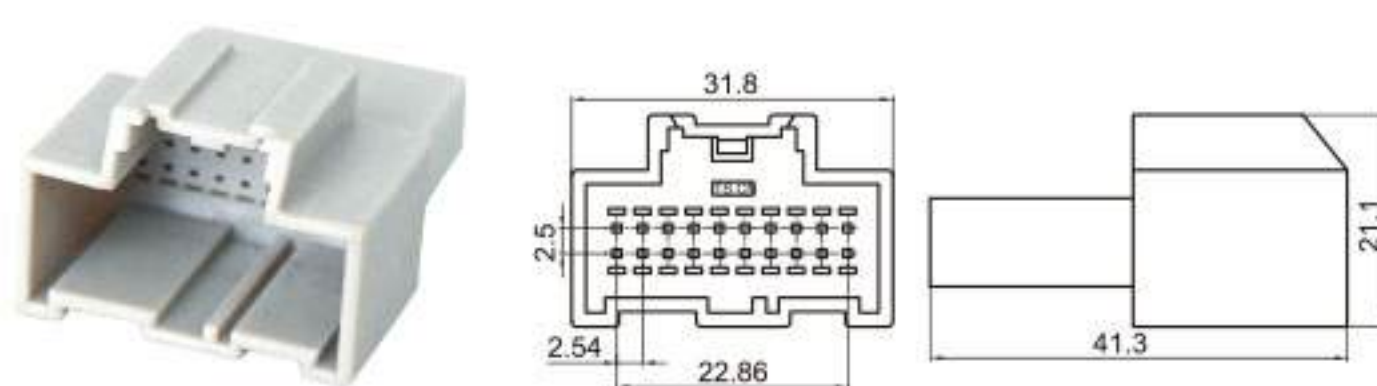
Type: TSGM20-20P-11-2 Material: PA66 GF30% Matching Terminal: TSZ208B
