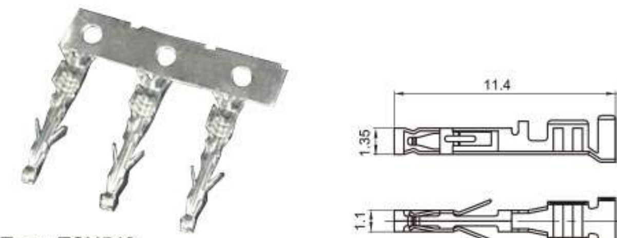
Type: TSH543 Material: Phos.bronze Applicable Thickness: 0.64
