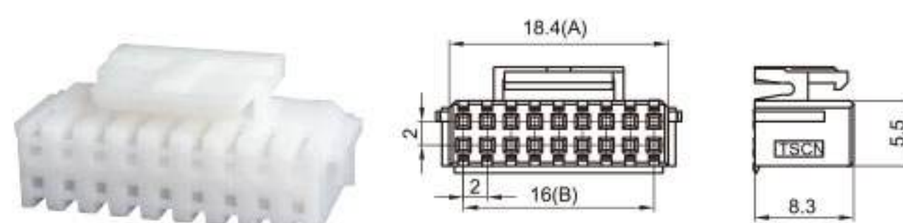
Type: TSPHB-18P-21(04P-40P) Material: PA66 Matching Terminal: TSPHB
