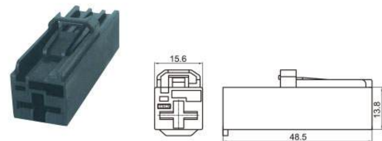
Type: TS30179-01P-21 Material: PBT GF15% Matching Terminal: TSDJ6128B-E9.5*1.2E
