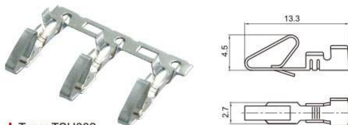
Type: TSH002 Material: Phos.bronze Applicable Thickness: 0.6~0.8
