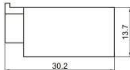
Type: TSVL10-02PM-AT Material: PA66 GF15% Matching Terminal: TSTM0012 / TSTM0013 / TSTM0014
