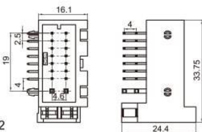
Type: TSCLR-16PM-PKB-1 Material: PA66 Matching Terminal: TSPM0040 / TSPM0221~TSPM0223
