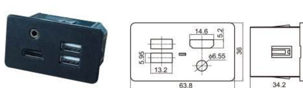
Type: TS30100 Material: ABS Matching Terminal: TSHDMI-F / TSUSB-F / TS3.5-F
