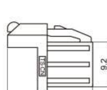
Type: TSVW20-04PF-AT-5BL Material: PA66 GF30% Matching Terminal: TSTF0048 / TSTF0049 / TSTF0050
