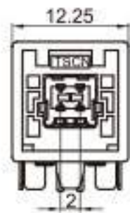
Type: TSTA04-04PM-AT-PKB Material: PA66 GF15% Matching Terminal: TSPM0050 / TSPM0053
