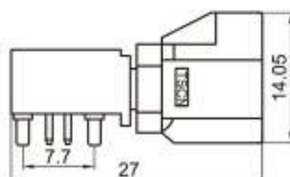
Type: TSVW10-06PM-AT Material: PBT GF30% Matching Terminal: TSPM0027 / TSPM0151 / TSPM0151-A
