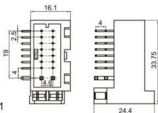
Type: TSCLR-16PM-PKB Material: PA66 Matching Terminal: TSPM0040 / TSPM0221~TSPM0223
