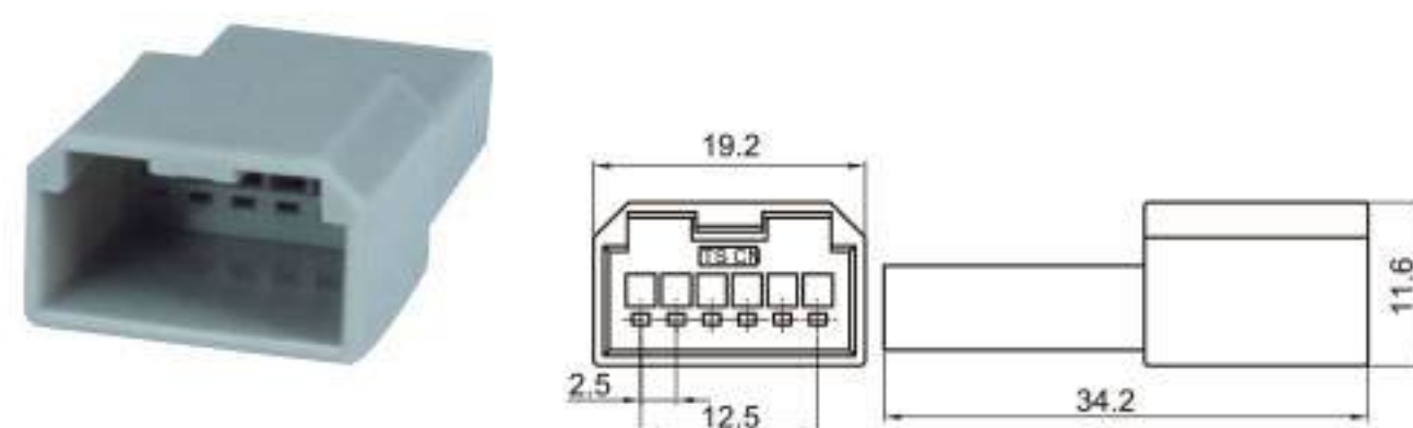
Type: TSHD06-06P-11-4 Material: PA66 Matching Terminal: TSZ145
