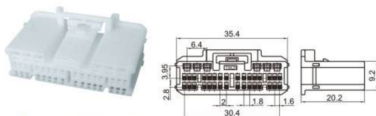
Type: TS30101-38P-21 Material: PA66 Matching Terminal: TSH593 / TSH600
