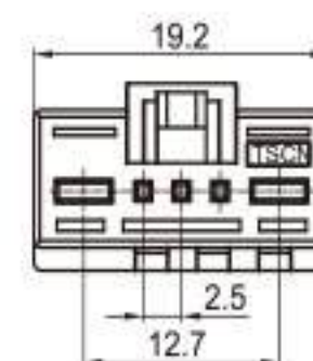
Type: TS30149-05P-21 Material: PA66 GF30% Matching Terminal: TSH091 / TSH092
