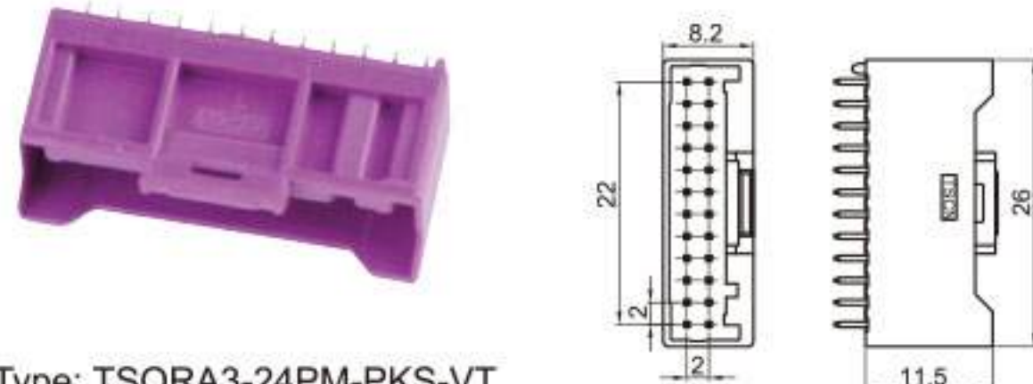
Type: TSQRA3-24PM-PKS-VT Material: PA66 GF15% Matching Terminal: TSPM0145
