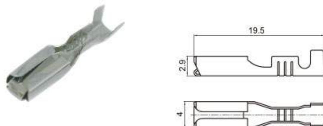
Type: TSH001 Material: Phos.bronze Applicable Thickness: 0.6
