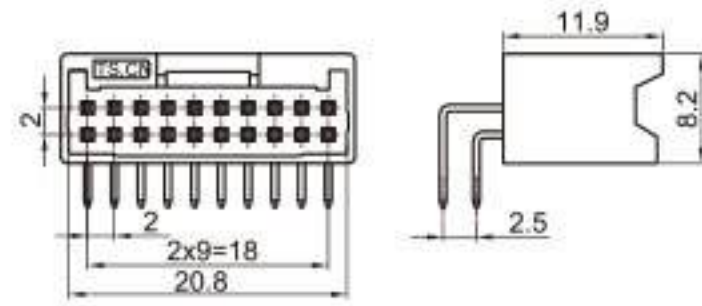
Type: TS30046-20PM-PKB(QRA3) Material: PA66 GF15% Matching Terminal: TSPM0143 / TSPM0144
