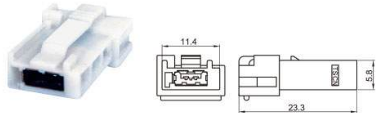
Type: TSKC3123-02PF-AT Material: PA66 GF30% Matching Terminal: TSTF0022 / TSTM0006
