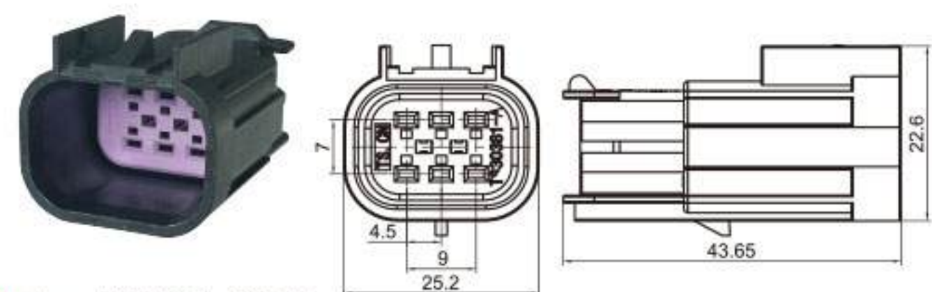
Type: TS30381-06P-11 Material: PA66 GF30% Matching Terminal: TS15326269
