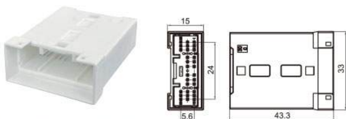
Type: TS30101-30PM-PKS-6 Material: PBT GF15% Matching Terminal: TSPM0305
