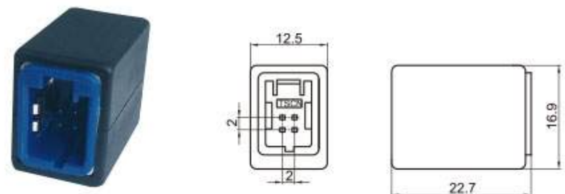
Type: TSMA04-04PM-AH-2 Material: PA66 GF30% Matching Terminal: TSAF0029 / TSPM0030
