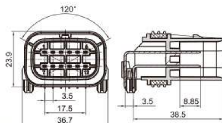
Type: TS30359-12PM-PKB Material: PBT GF15% Matching Terminal: TSPM0333/TSPM0334
