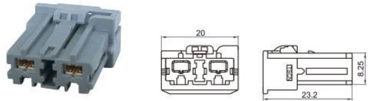
Type: TS30212-04PF-AT Material: PBT Matching Terminal: TSTF0058 / TSTF0059 / TSTF0006
