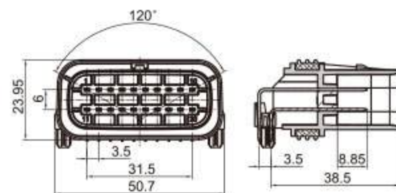
Type: TS30359-20PM-PKB Material: PBT GF15% Matching Terminal: TSPM0333 / TSPM0334
