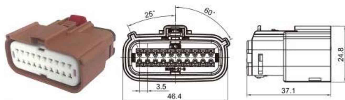
Type: TS30359-20P-21-2 Material: PA66 GF30% Matching Terminal: TSH047
