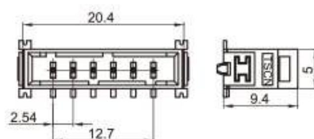
Type: TS30231-06PM-PKB Material: PPS Matching Terminal: TSPM0262 / TSPM0263
