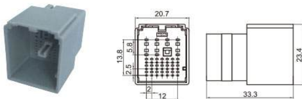
Type: TS30205-28P-11-1 Material: PA66 Matching Terminal: TSZ566 / TSZ561
