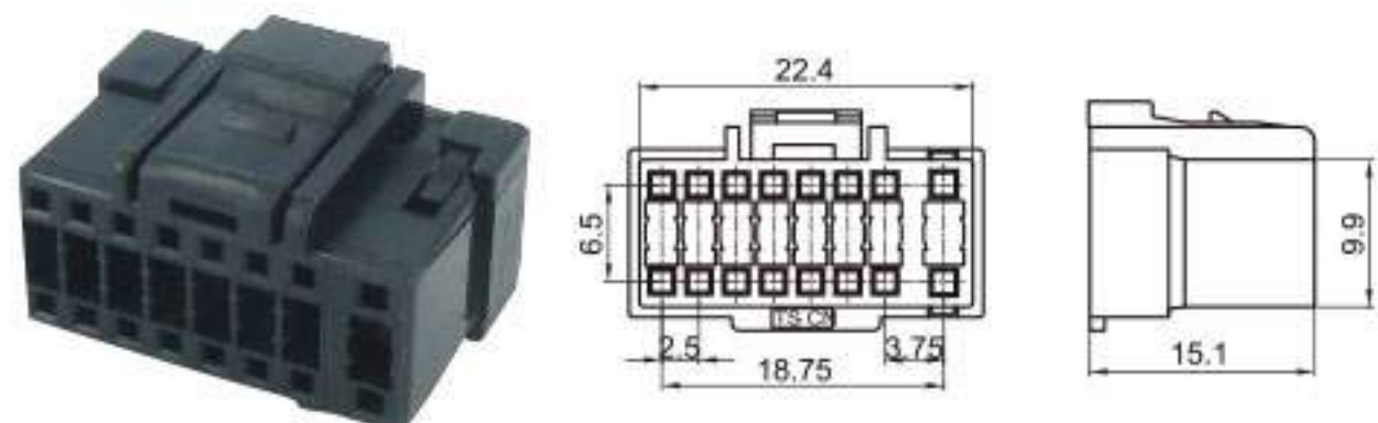
Type: TSALP04-16P-21 Material: PA66 GF15% Matching Terminal: TSH503 / TSH031B
