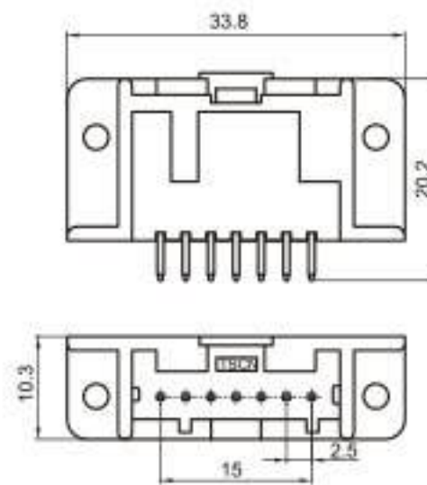
Type: TS3003-07PM-PKS Material: PA66 GF30% Matching Terminal: TSPM0140
