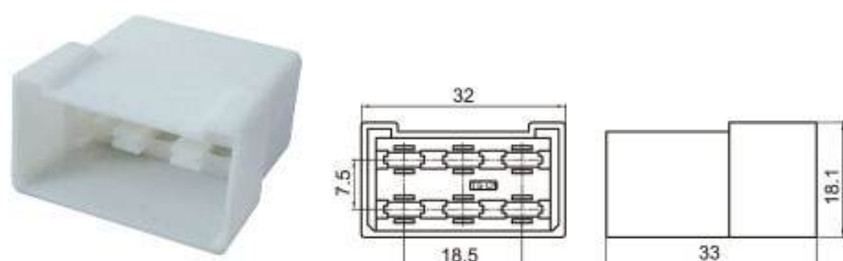
Type: TSFIAT-06P-11 Material: PA66 Matching Terminal: TSZ538A
