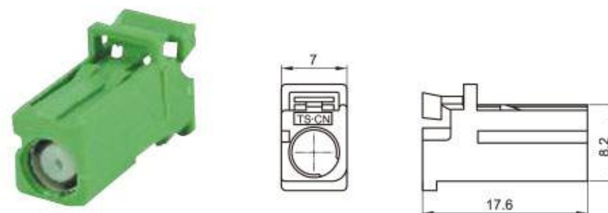
Type: TSGT16-01PF-AT-2 Material: PA66 Matching Terminal: TSTF0017 / TSTF0004
