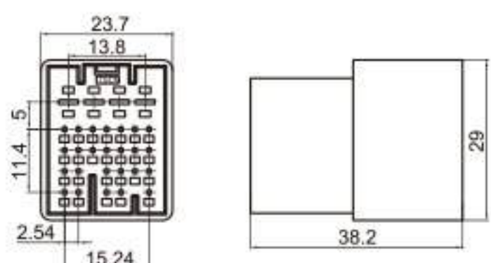
Type: TS30217-30P-11-7 Material: PBT GF15% Matching Terminal: TSDJ615B-2.8*0.8B / TSZ208
