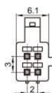
Type: TSHY66-04P-21 Material: PA66 Matching Terminal: TSHY66
