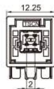
Type: TSTA04-04PM-AT-PKB-3 Material: PA66 GF15% Matching Terminal: TSPM0050 / TSPM0053
