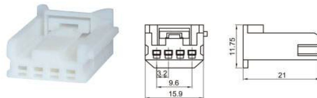
Type: TS30096-04P-21 Material: PA66 Matching Terminal: TSH593
