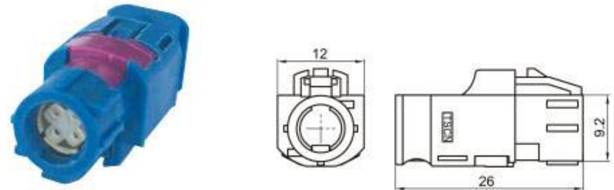
Type: TSVW20-04PF-AT-5BL-1 Material: PA66 GF30% Matching Terminal: TSTF0051 / TSTF0052
