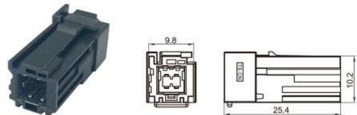
Type: TSTA04-04PF-AT-4 Material: PBT 1100 Matching Terminal: TSTF0008 / TSTF0010 / TSTF0011
