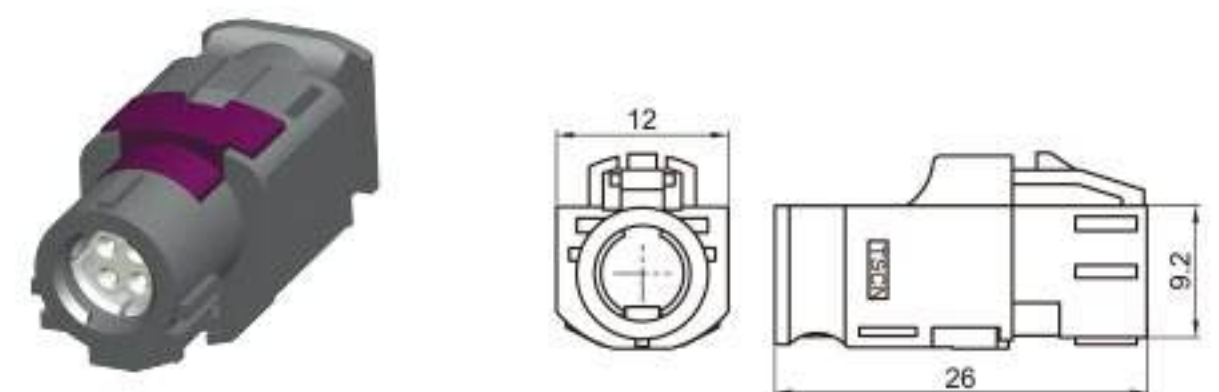
Type: TSVW20-04PF-AT-5GY-1 Material: PA66 GF30% Matching Terminal: TSTF0051 / TSTF0052
