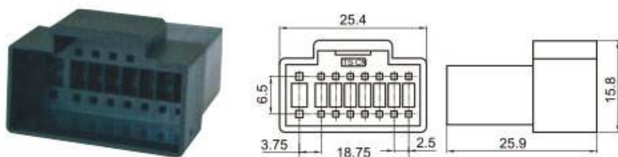
Type: TSALP04-16P-11 Material: PA66 GF30% Matching Terminal: TSZ532 / TSZ533
