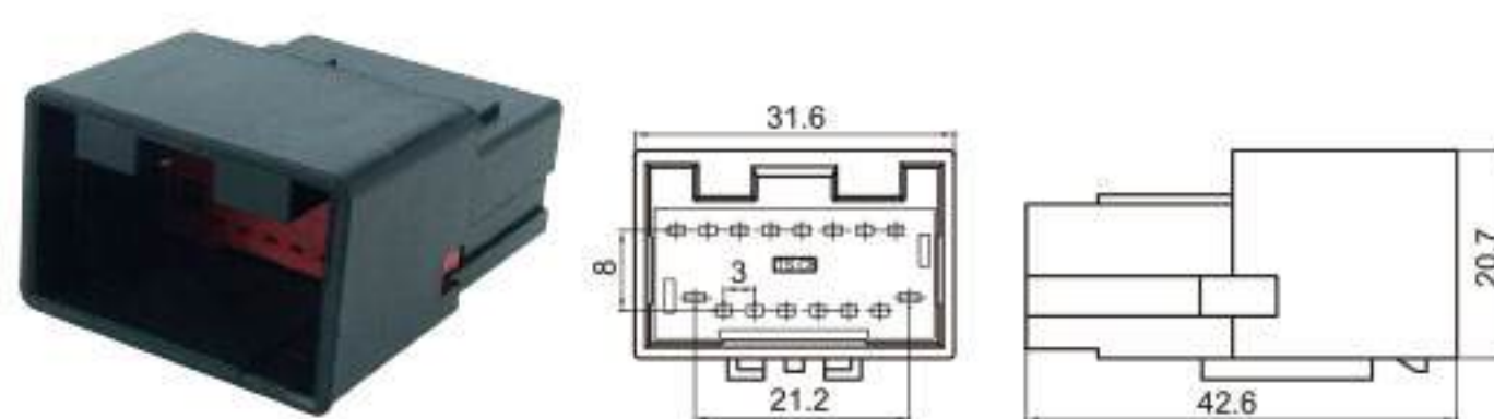
Type: TS1771-16P-11-2 Material: PA66 Matching Terminal: TSZ144 / TSZ185
