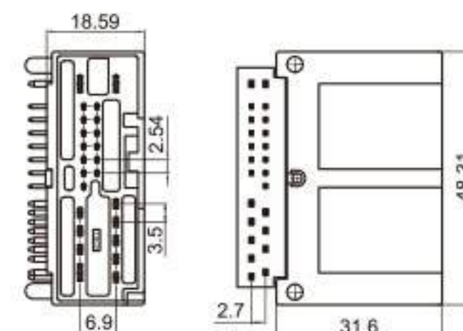
Type: TS5520-16PM-PKB Material: PA66 GF30% Matching Terminal: TSPM0009 / TSPM0012
