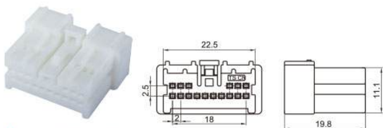
Type: TSNI16-16P-21 Material: PA66 Matching Terminal: TSH143
