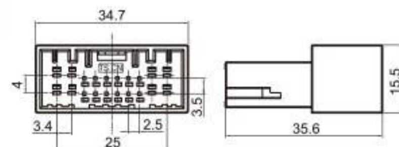
Type: TS30302-20P-11 Material: PBT Matching Terminal: TSZ040 / TSZ616
