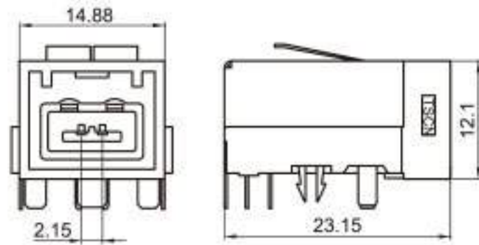
Type: TSKI10-02PM-AT-PKB Material: PBT GF15% Matching Terminal: TSPM0054~TSPM0056
