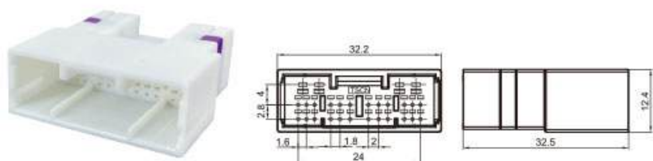
Type: TS30101-28P-11-7 Material: PA66 Matching Terminal: TSZ562 / TSZ615
