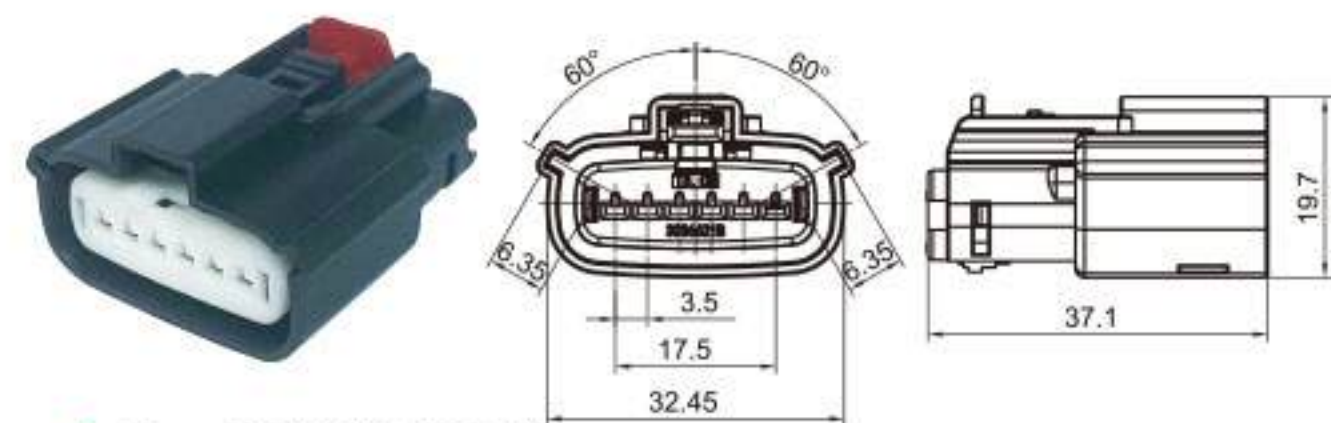
Type: TS30366-06P-21 Material: PA66 GF30% Matching Terminal: TSH047
