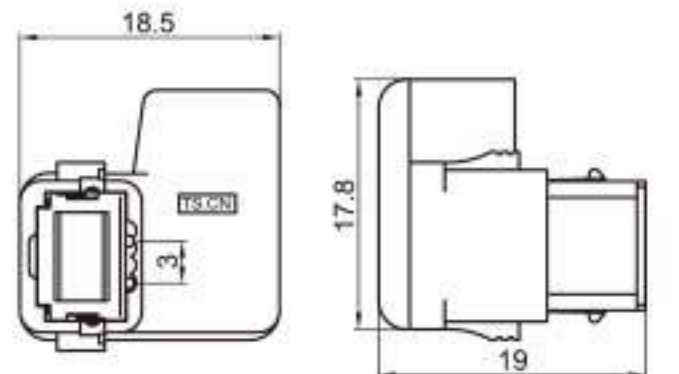
Type: TS30053-10PM-AH-1 Material: PA66 GF30% Matching Terminal: TSAF0007 / TSAM0018 / TSAM0019
