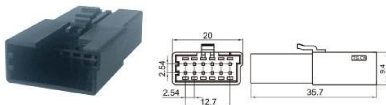
Type: TS30069-12P-11 Material: PA66 GF30% Matching Terminal: TSZ208
