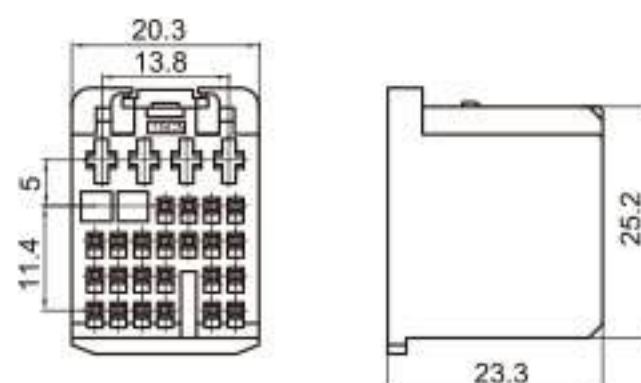
Type: TS30217-30P-11-2 Material: PBT GF15% Matching Terminal: TSDJ615B-2.8*0.8B / TSZ208
