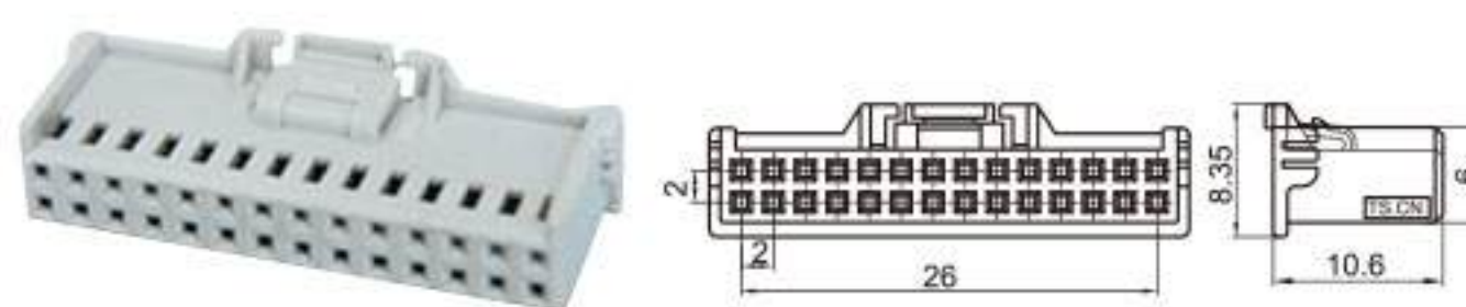
Type: TS30047-28P-21(QRA3) Material: PA66 GF15% Matching Terminal: TSPHB
