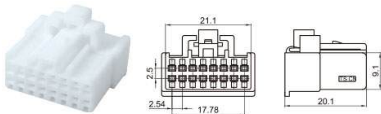
Type: TSPAN16-16P-21 Material: PA66 Matching Terminal: TSH053
