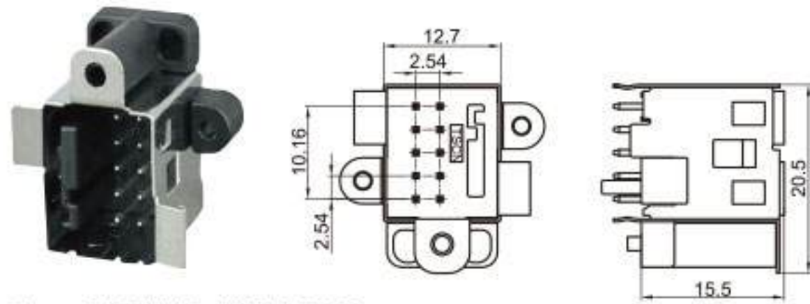
Type: TSRW10-10PM-PKS Material: PA66 GF30% Matching Terminal: TSPM0126 / TSPM0146
