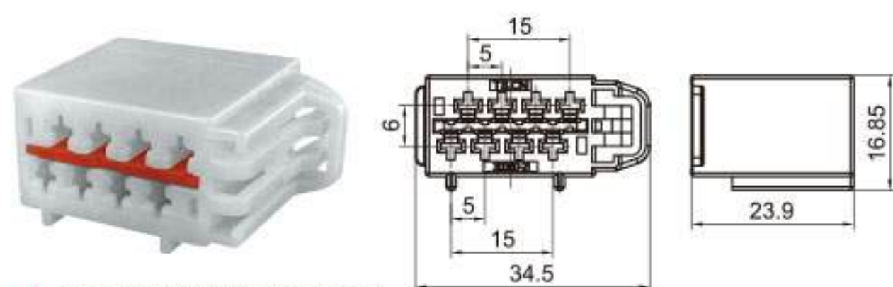
Type: TS30360-08P-21-2 Material: ABS Matching Terminal: TSH085
