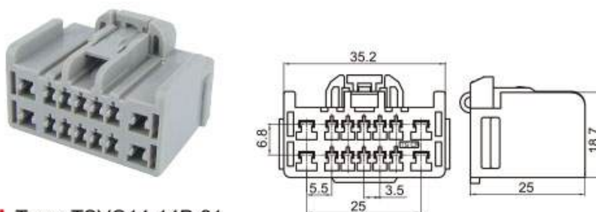
Type: TSVO14-14P-21 Material: PA66 Matching Terminal: TSH085 / TSH047
