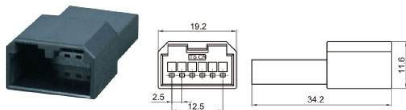
Type: TSHD06-06P-11-1 Material: PA66 Matching Terminal: TSZ145
