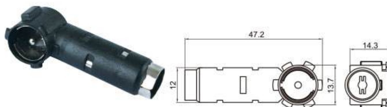
Type: TSVW21-01PF-AT Material: ABS Matching Terminal: NIL
