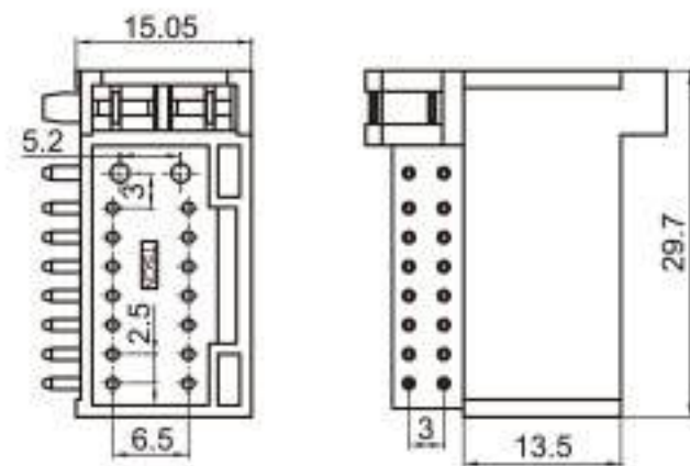
Type: TSKEN-16PM-PKB-1 Material: PA66 GF30% Matching Terminal: TSPM0103~TSPM0108
