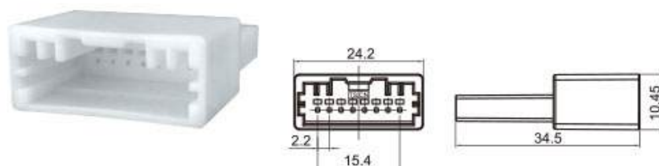
Type: TS30291-08P-11 Material: PA66 Matching Terminal: TSZ208
