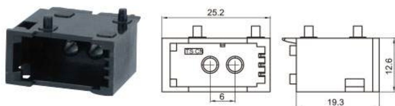
Type: TSBMGQ-02PM-AH Material: PA66 GF15% Matching Terminal: NIL
