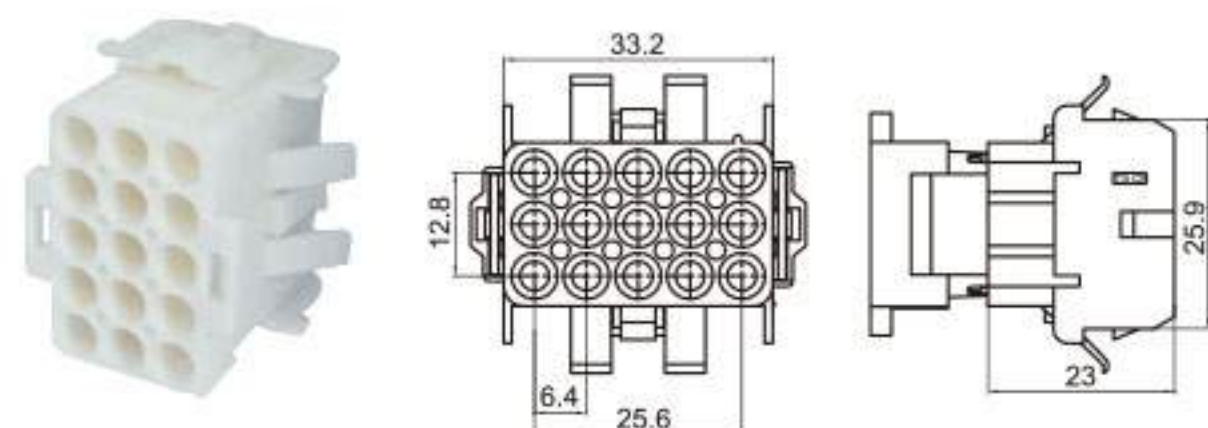
Type: TSPP15-15P-21 Material: PA66 GF15% Matching Terminal: TSH536
