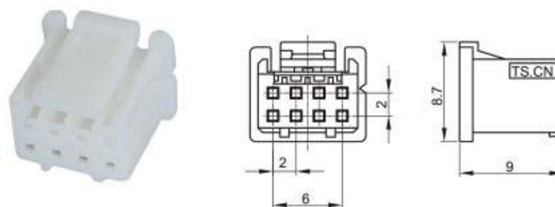
Type: TS30021-08P-21(10P) Material: PA66 Matching Terminal: TSH595
