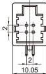
Type: TS30147-04PM-PKB Material: PBT GF15% Matching Terminal: TSPM0140 / TSPM0077
