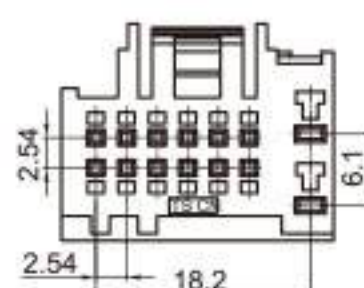
Type: TS2105-14P-21 Material: PA66 GF30% Matching Terminal: TSH008/TSH143B
