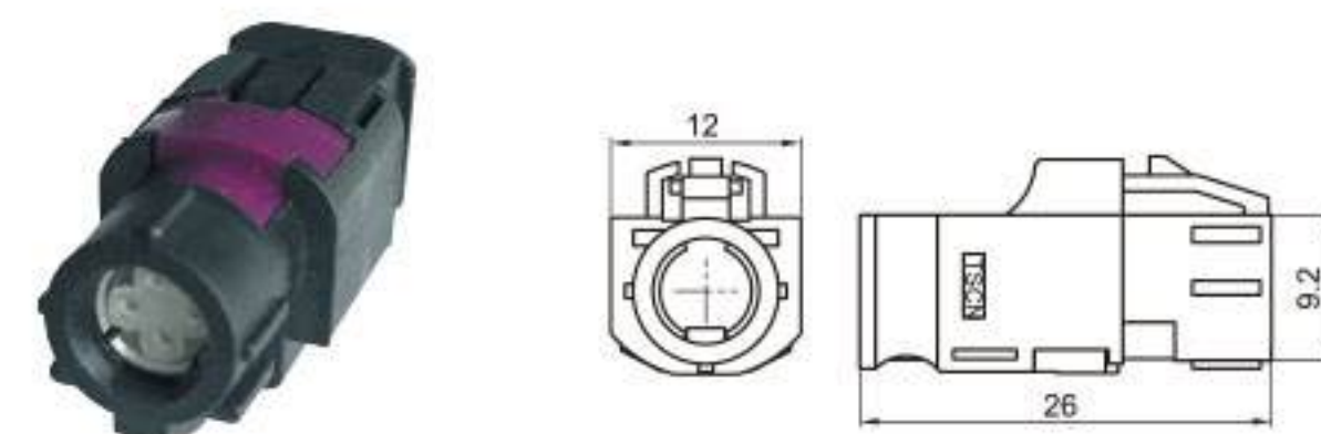
Type: TSVW20-04PF-AT-5BK-1 Material: PA66 GF30% Matching Terminal: TSTF0051 / TSTF0052
