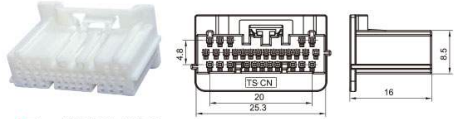
Type: TS30378-30P-21 Material: PA66 Matching Terminal: TSH600A
