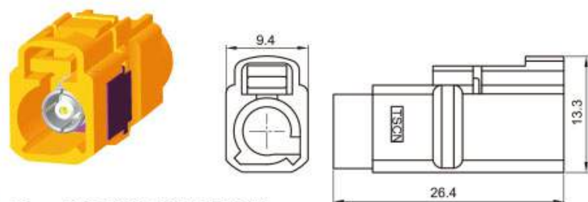
Type: TSVW20-01PF-AT-OR Material: PA66 GF30% Matching Terminal: TSTF0025 / TSTF0026
