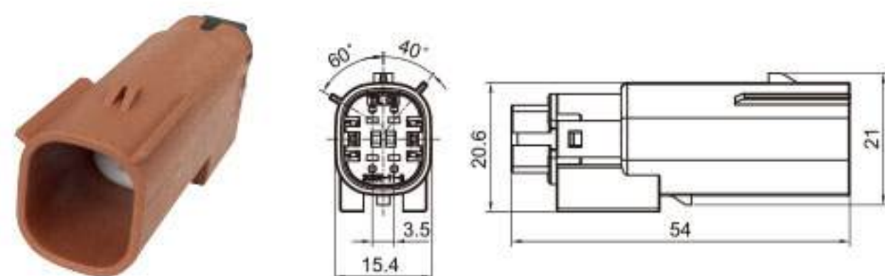
Type: TS30359-04P-11-2 Material: PA66 GF30% Matching Terminal: TSZ144A
