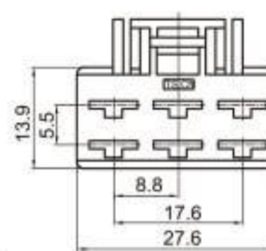
Type: TS30002-06P-21 Material: PBT 1100 Matching Terminal: TSH033A
