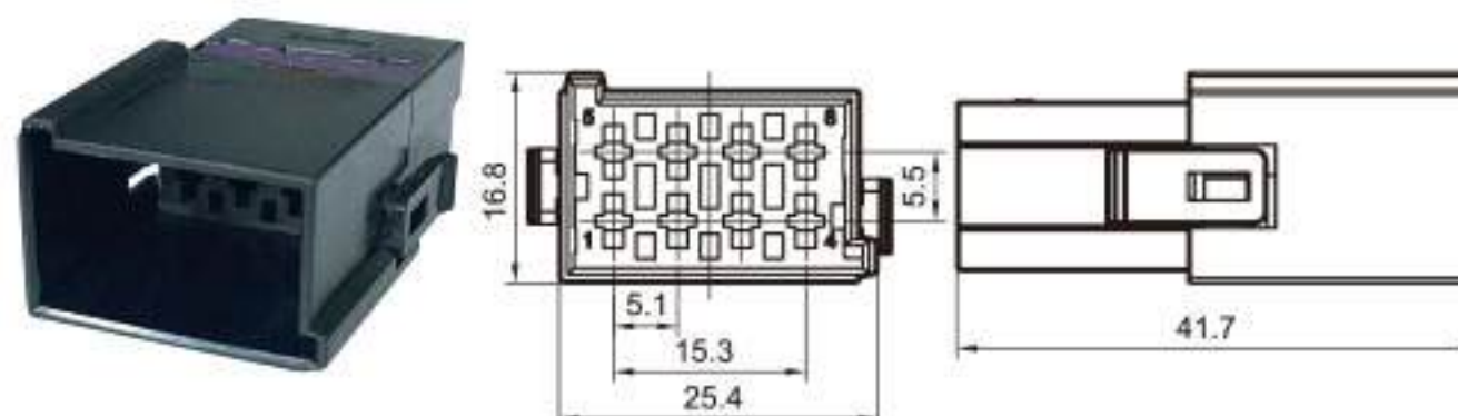
Type: TS30372-08P-11 Material: PA66 Matching Terminal: TSZ024
