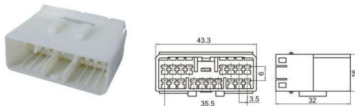
Type: TS8405-18P-11 Material: PA66 Matching Terminal: TSZ011
