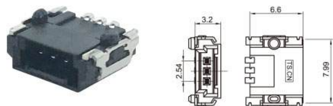
Type: TS30278-03PM-PKB Material: PPS Matching Terminal: TSPM0306 / TSPM0307
