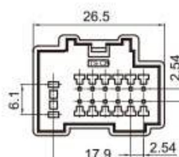
Type: TS2105-14P-11 Material: PA66 GF30% Matching Terminal: TSZ040 / TSZ018B
