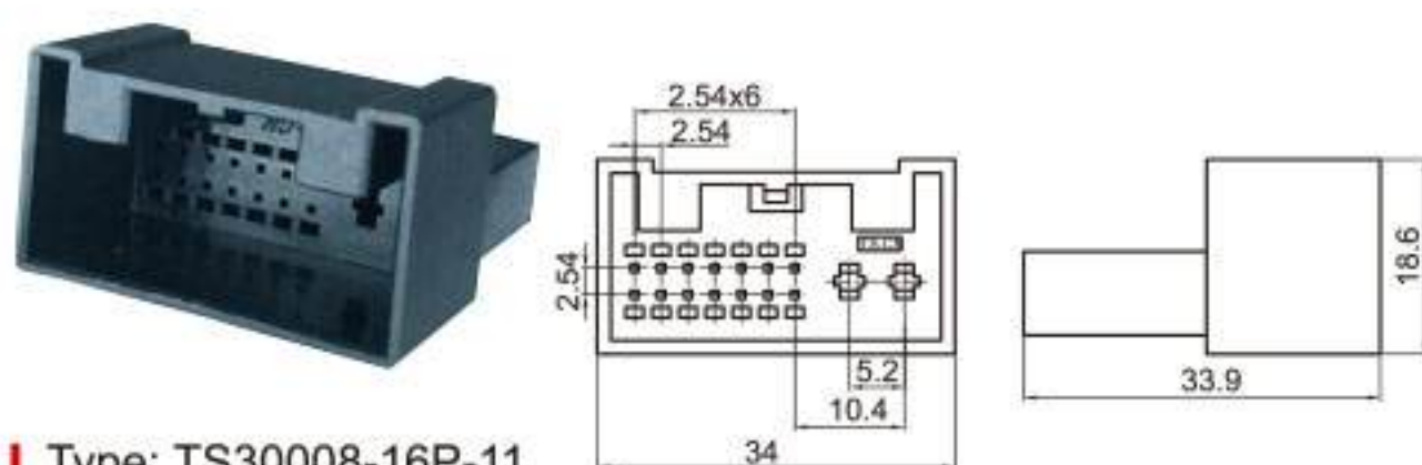
Type: TS30008-16P-11 Material: PBT GF15% Matching Terminal: TSZ024 / TSZ208B
