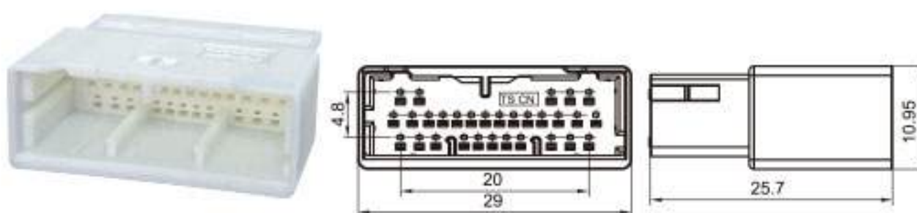
Type: TS30378-30P-11 Material: PA66 Matching Terminal: TSZ556
