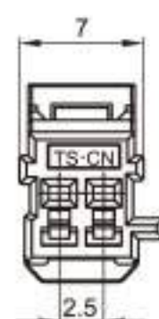
Type: TS30333-02P-21 Material: PBT Matching Terminal: TSH076
