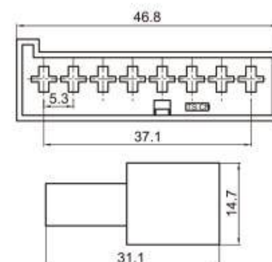
Type: TS1777-08P-11-1 Material: PA66 Matching Terminal: TSZ024
