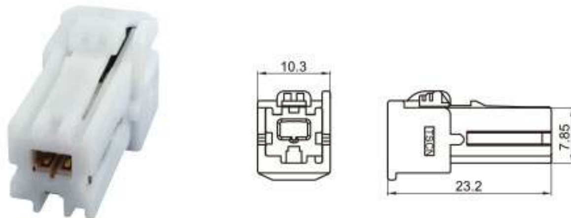
Type: TS30211-02PF-AT Material: PBT Matching Terminal: TSTF0058 / TSTF0059 / TSTF0006
