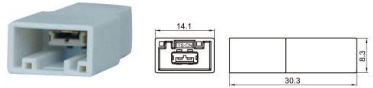
Type: TSKC3123-02PM-AT Material: PA66 GF30% Matching Terminal: TSTM0021 / TSTM0022
