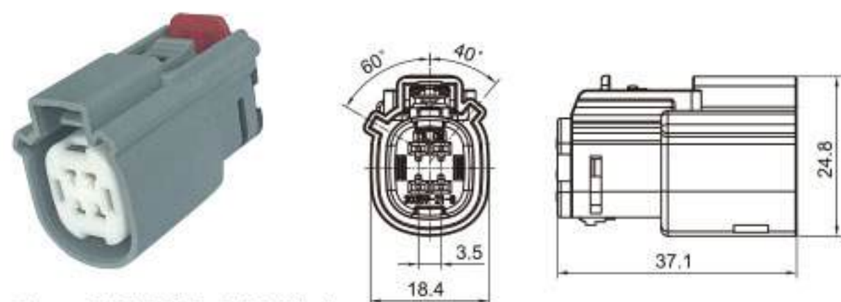
Type: TS30359-04P-21-1 Material: PA66 GF30% Matching Terminal: TSH047
