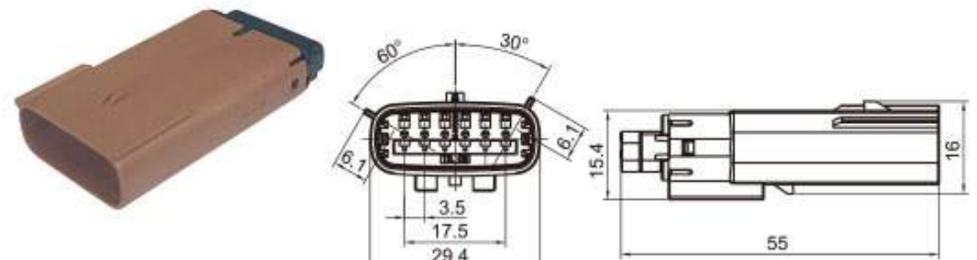
Type: TS30366-06P-11-2 Material: PA66 GF30% Matching Terminal: TSZ144A
