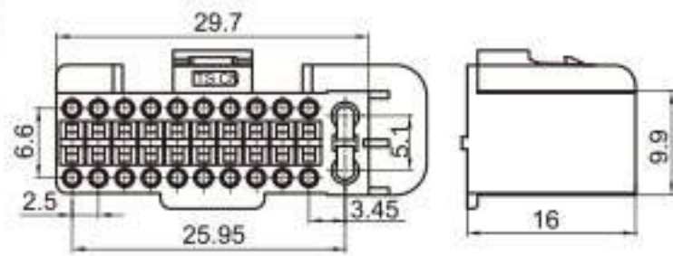
Type: TSKEN22-22P-21 Material: PA66 GF30% Matching Terminal: TSH032 / TSH031
