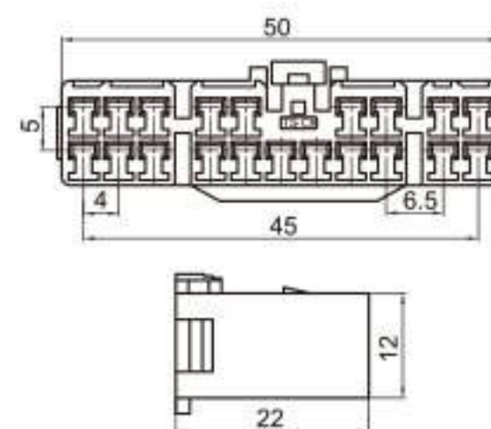
Type: TS7712-20P-21 Material: PA66 Matching Terminal: TSH064
