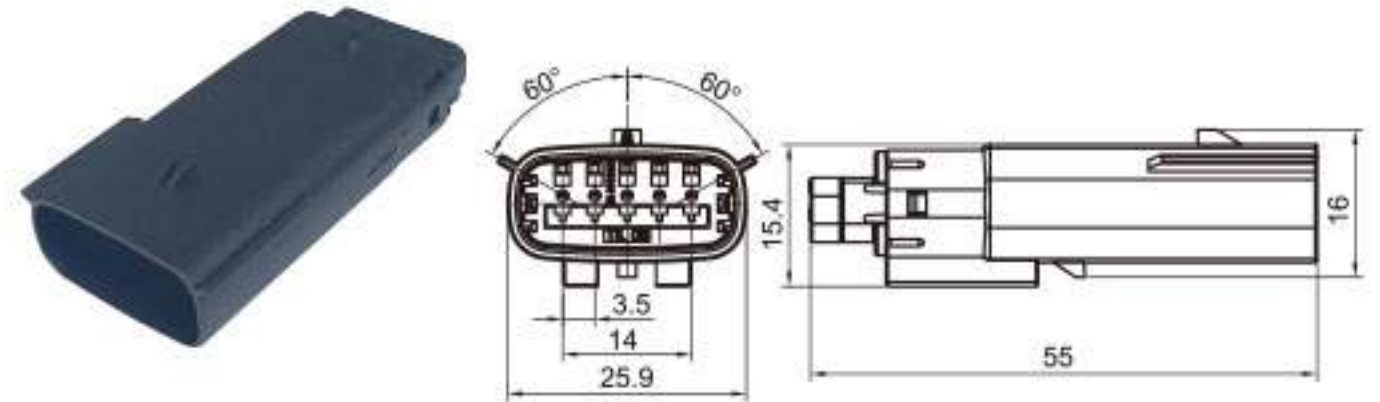
Type: TS30366-05P-11 Material: PA66 GF30% Matching Terminal: TSZ144A
