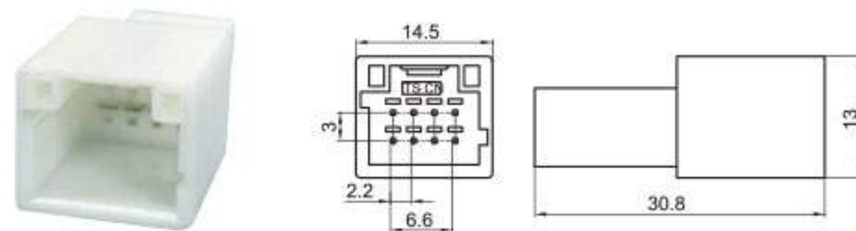
Type: TSTA08-08P-11-3 Material: PA66 Matching Terminal: TSZ208
