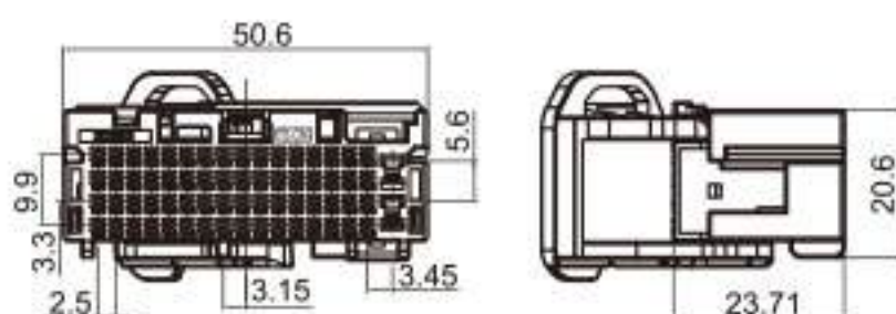
Type: TS30283-66P-21-2 Material: PBT Matching Terminal: TSH064 / TSH092
