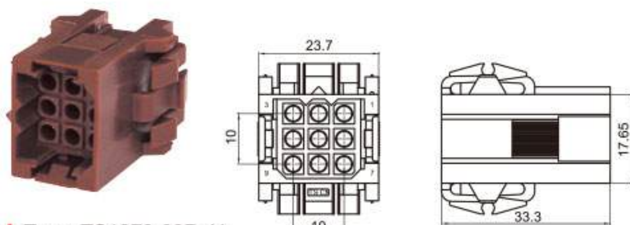
Type: TS1073-09P-11 Material: PA66 Matching Terminal: NIL
