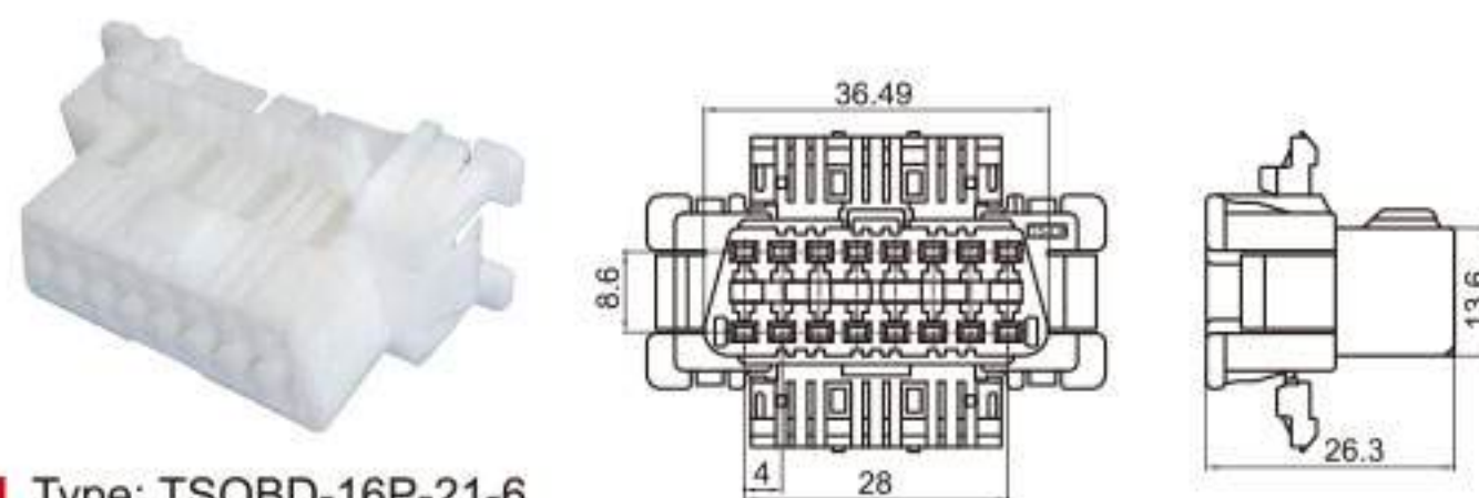
Type: TSOBD-16P-21-6 Material: PA66 Matching Terminal: TSH610
