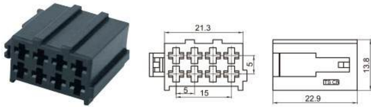
Type: TSABD-08P-21-A Material: PA66 Matching Terminal: TSH019A
