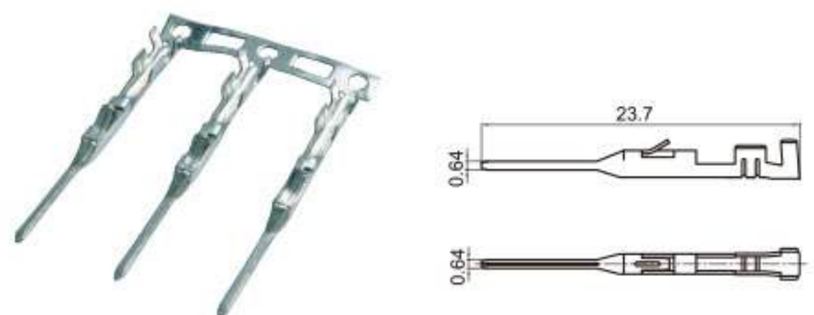
Type: TSZ208B Material: Brass
