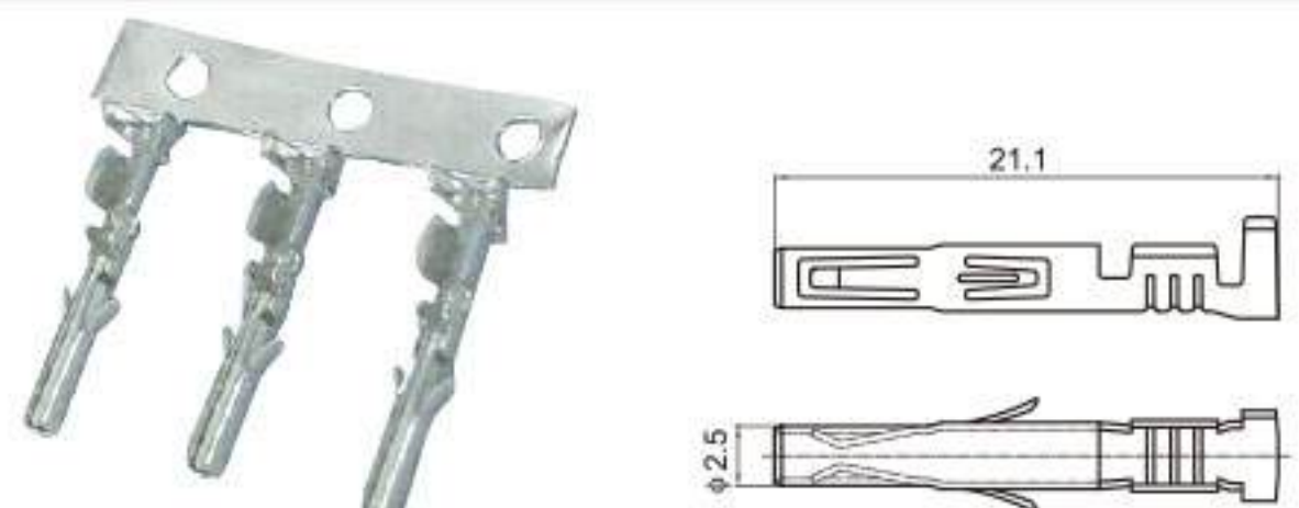
Type: TSH535 Material: Phos.bronze Applicable Thickness: \phi 1.3
