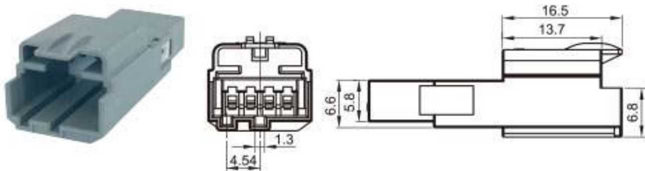
Type: TS30362-04P-11-1 Material: PA66 GF30% Matching Terminal: TSZ145
