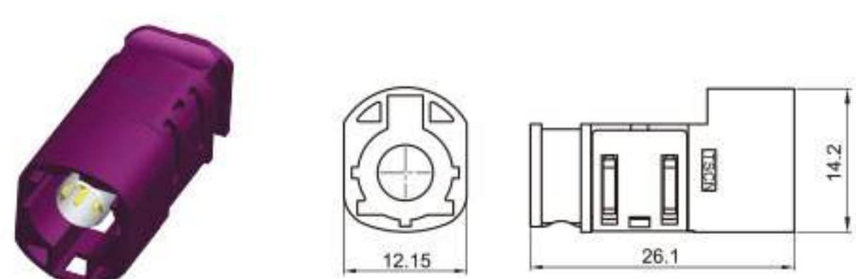
Type: TSVW10-04PM-AT-5VT-1 Material: PA66 GF15% Matching Terminal: TSPM0175 / TSTM0051
