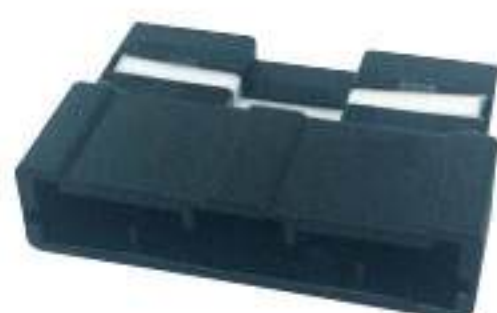
Type: TS30210-24P-11 Material: PA66 GF30% Matching Terminal: TSZ556
