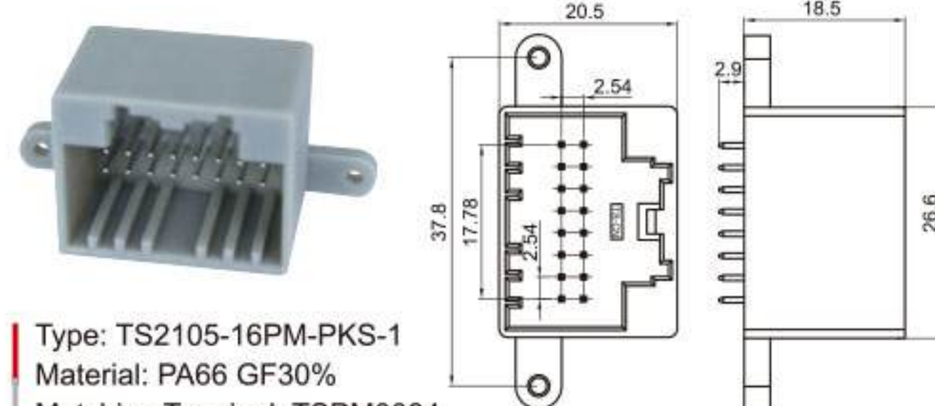
Type: TS2105-16PM-PKS Material: PA66 GF30% Matching Terminal: TSPM0084
