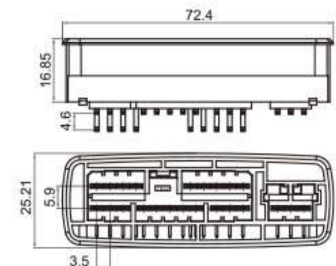
Type: TS8113-20PM-PKB Material: PA66 Matching Terminal: TSPM0001~TSPM0004
