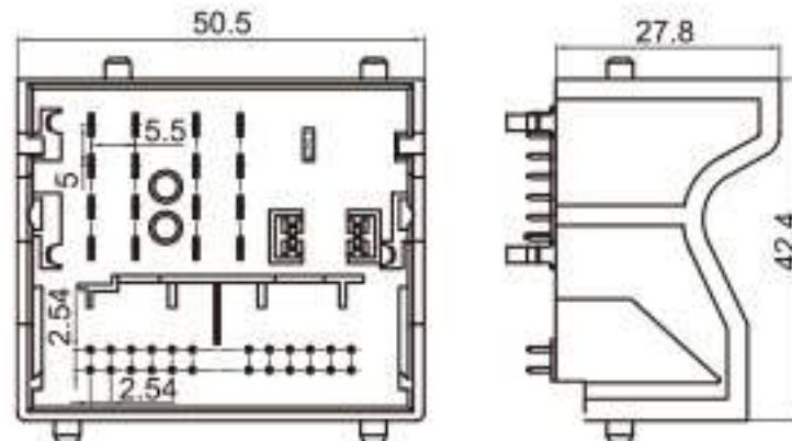
Type: TS9003-40PM-PKS-1 Material: PA66 GF30% Matching Terminal: TSPM0057 / TSPM0119 / TSPM0120
