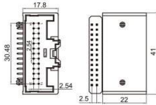
Type: TS5524-26PM-PKB Material: PA66 GF30% Matching Terminal: TSPM0085 / TSPM0122
