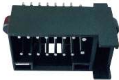
Type: TSKEN-16PM-PKS Material: PA66 GF30% Matching Terminal: TSPM0120 / TSPM0239 / TSPM0240
