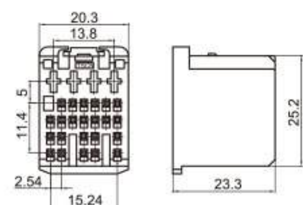
Type: TS30217-30P-21-6 Material: PBT GF10% Matching Terminal: TSH019 / TSH092
