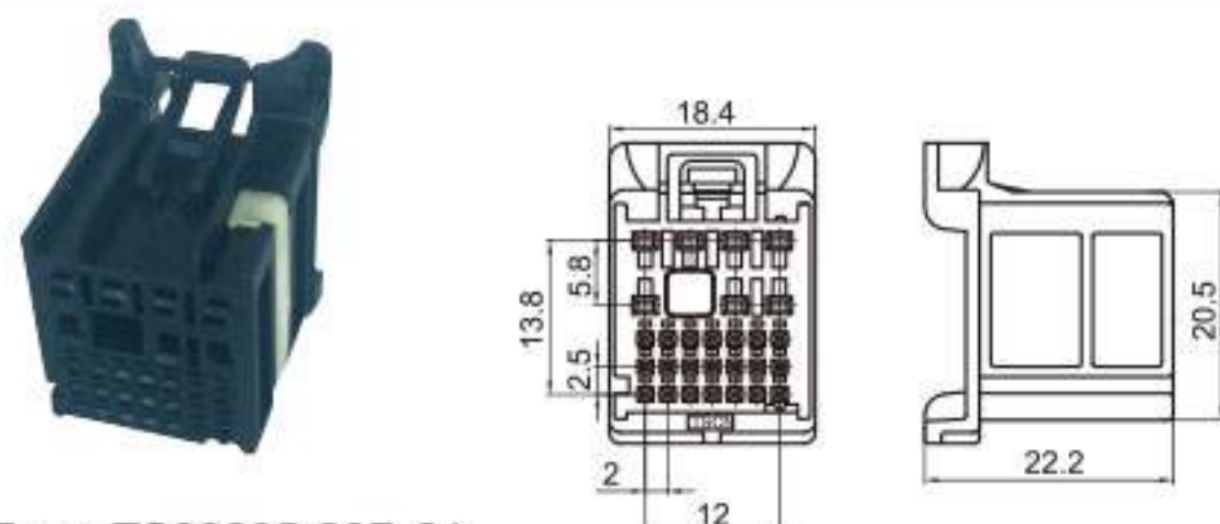
Type: TS30205-28P-21 Material: PA66 Matching Terminal: TSH092 / TSH606
