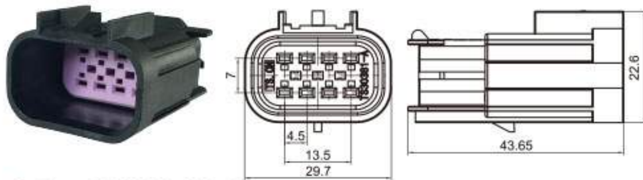
Type: TS30381-08P-11 Material: PA66 GF30% Matching Terminal: TS15326269
