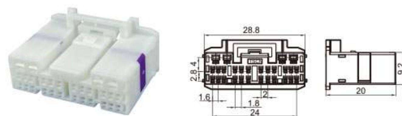
Type: TS30101-28P-21-4 Material: PA66 Matching Terminal: TSH593 / TSH600A
