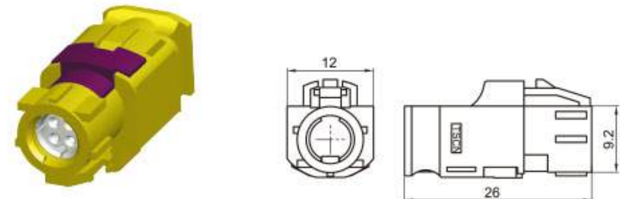
Type: TSVW20-04PF-AT-5CU-1 Material: PA66 GF30% Matching Terminal: TSTF0051 / TSTF0052
