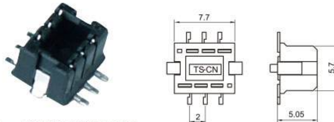
Type: TSTKCW-06PM-PKB Material: PA66 GF30% Matching Terminal: TSPM0124 / TSPM0125
