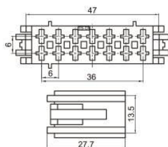
Type: TSBZ14-14P-21 Material: PA66 Matching Terminal: TSH019
