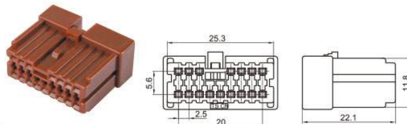
Type: TSHY16-16P-21 Material: PA66 Matching Terminal: TSH006
