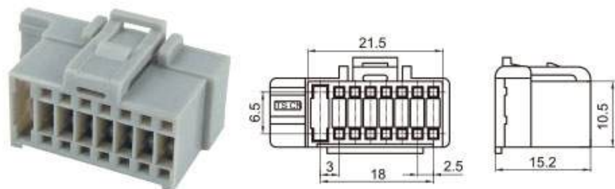
Type: TSPAN16C-16P-21 Material: PA66 Matching Terminal: TSH114 / TSH113
