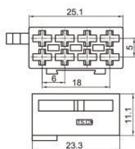
Type: TS1784A-08P-21-2BK Material: PA66 Matching Terminal: TSH019
