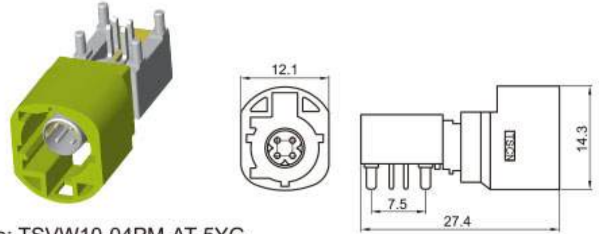
Type: TSVW10-04PM-AT-5YG Material: PA66 GF30% Matching Terminal: TSPM0021~TSPM0025
