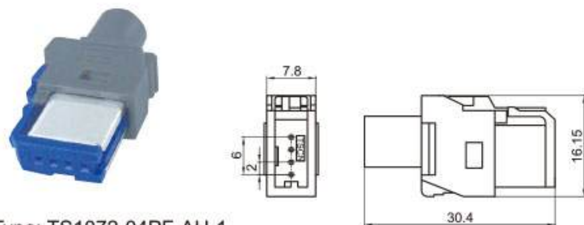
Type: TS1072-04PF-AH-1 Material: PA66 Matching Terminal: TSAF0031 / TSPH
