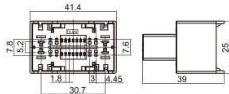
Type: TS30279-26P-11 Material: PA66 Matching Terminal: TSZ024 / TSZ566 / TSZ556
