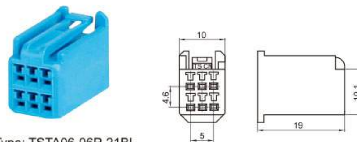
Type: TSTA06-06P-21BL Material: PA66 Matching Terminal: TSH076
