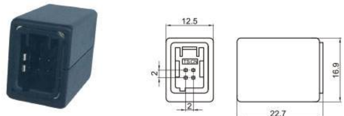
Type: TSMA04-04PM-AH Material: PA66 GF30% Matching Terminal: TSPM0029 / TSPM0030
