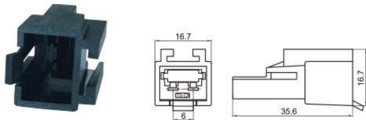
Type: TSLB14-02P-11 Material: PA66 GF30% Matching Terminal: TSZ006
