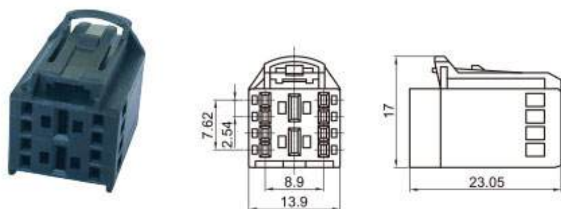
Type: TS30141-10P-21-1 Material: PBT GF15% Matching Terminal: TSH019/TSH092
