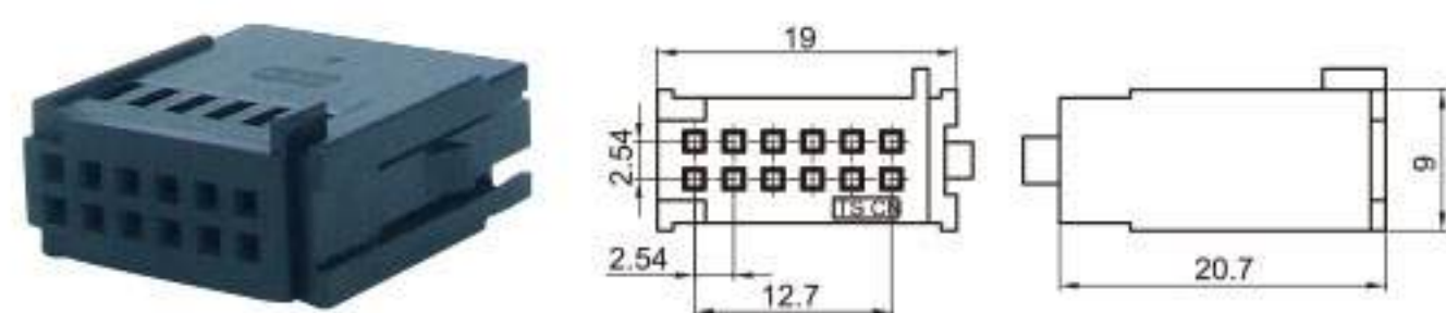
Type: TSVW12-12P-21-1WT Material: PA66 Matching Terminal: TSH143
