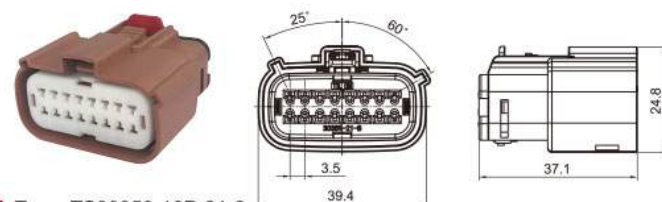
Type: TS30359-16P-21-2 Material: PA66 GF30% Matching Terminal: TSH047
