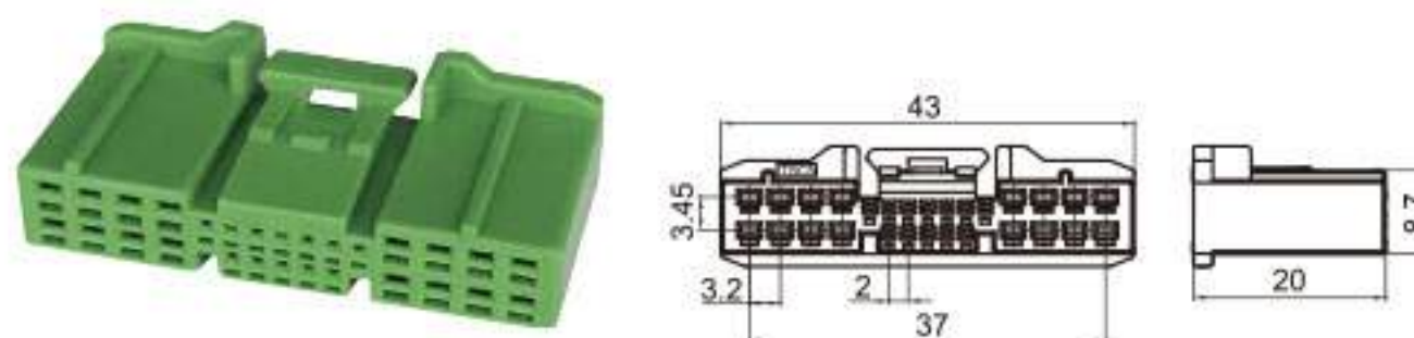
Type: TS30243-28P-21-7 Material: PA66 Matching Terminal: TSH593 / TSH606
