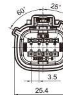
Type: TS30359-08P-21-1 Material: PA66 GF30% Matching Terminal: TSH047
