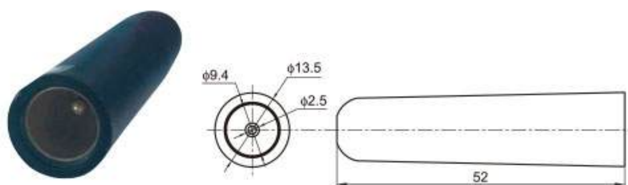
Type: TSFD17-01PM-AT Material: ABS Matching Terminal: TSTF0013 / TSTF0062
