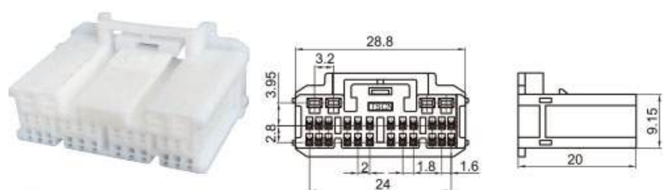
Type: TS30101-28P-21 Material: PA66 Matching Terminal: TSH593 / TSH600
