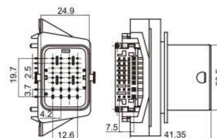
Type: TS30245-32PM-PKB Material: PA66 Matching Terminal: TSPM0289~TSPM0296
