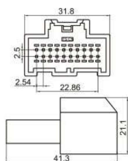
Type: TSGM20-20P-11-5 Material: PA66 GF30% Matching Terminal: TSZ208B
