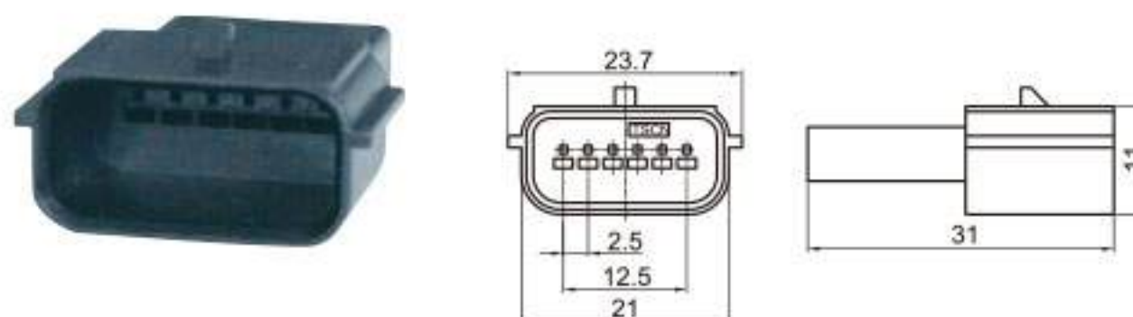
Type: TS30121-06P-11 Material: PA66 GF30% Matching Terminal: TSZ208B
