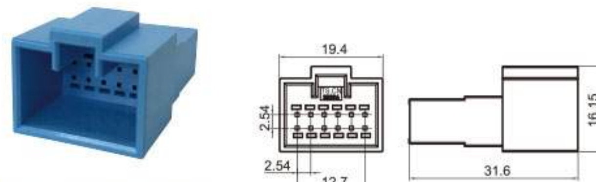
Type: TS30296-12P-11 Material: PBT GF15% Matching Terminal: TSZ616
