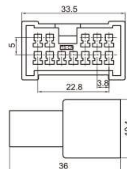
Type: TS7550-12P-11 Material: PA66 Matching Terminal: TSZ009
