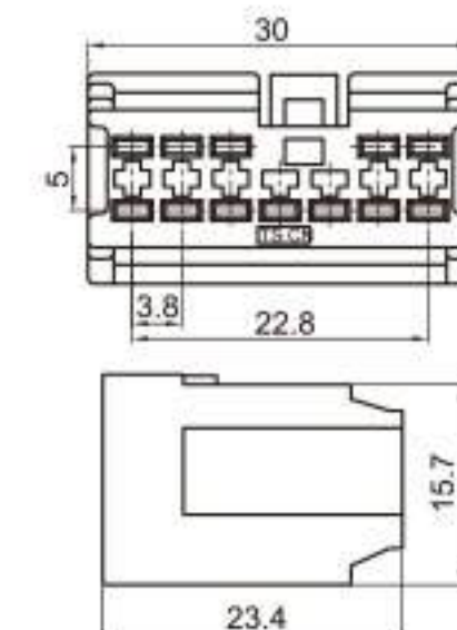
Type: TS7550-12P-21 Material: PA66 Matching Terminal: TSH064
