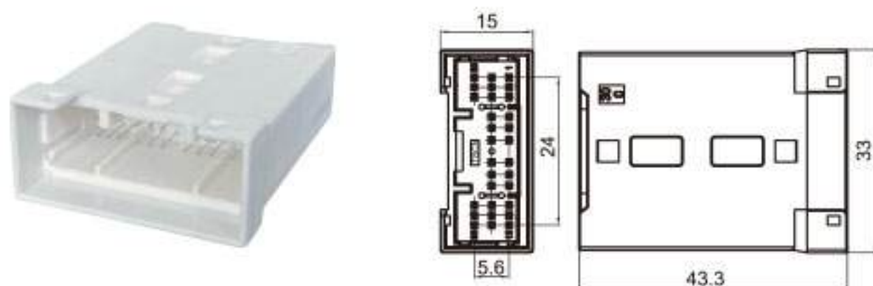
Type: TS30101-30PM-PKS-8 Material: PBT GF15% Matching Terminal: TSPM0305
