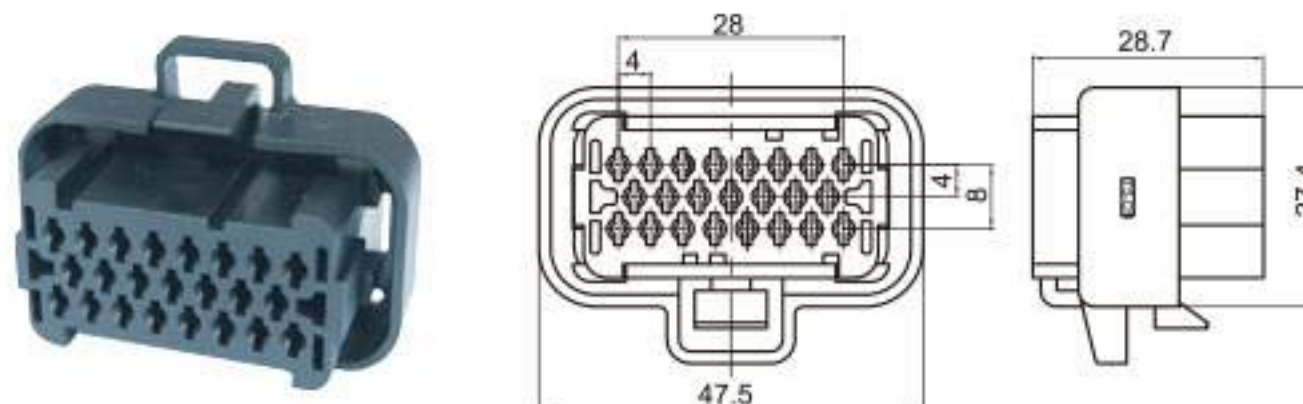
Type: TS3017-23P-21(30256) Material: PA66 Matching Terminal: TSH535
