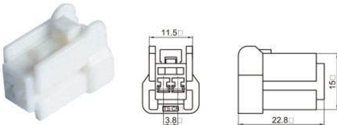
Type: TSLB03-02P-21 Material: PA66 Matching Terminal: TSH015
