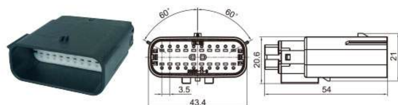
Type: TS30359-20P-11 Material: PA66 GF30% Matching Terminal: TSZ144A
