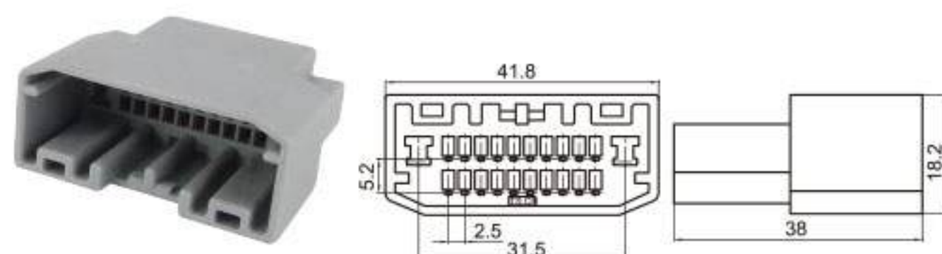
Type: TS6522-22P-11 Material: PA66 Matching Terminal: TSZ143 / TSZ145
