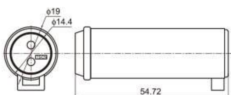
Type: TSN101-02PM-AT Material: ABS Matching Terminal: TSTM0025 / TSTM0026
