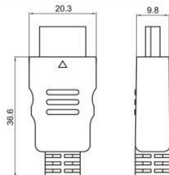
Type: TSHDMI 公 Material: PVC Matching Terminal: TSHDMI-M
