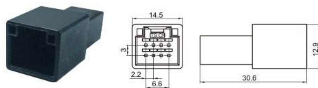
Type: TSTA08-08P-11-5 Material: PA66 Matching Terminal: TSZ208
