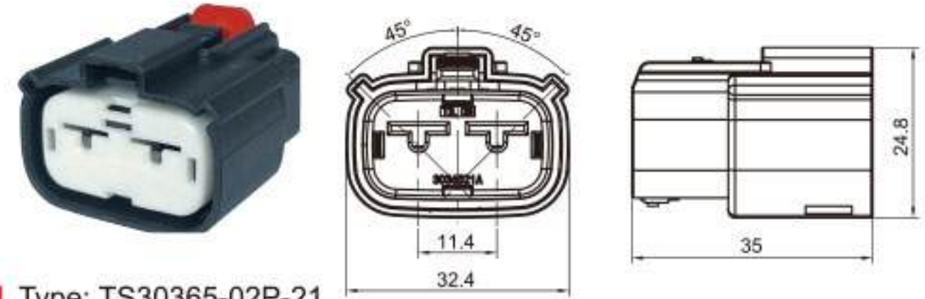
Type: TS30365-02P-21 Material: PA66 GF30% Matching Terminal: TSH591
