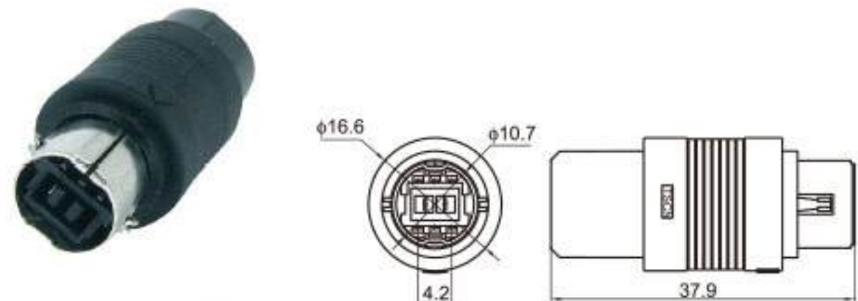
Type: TSSONY-08PF-AH-1 Material: PA66 GF30% Matching Terminal: TSAF0001 / TSH042 / TSH041
