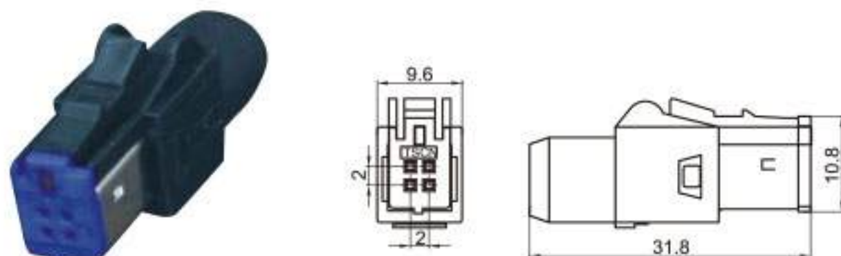
Type: TSMA04-04PF-AH-2 Material: PA66 GF15% Matching Terminal: TSAF0013 / TSPH
