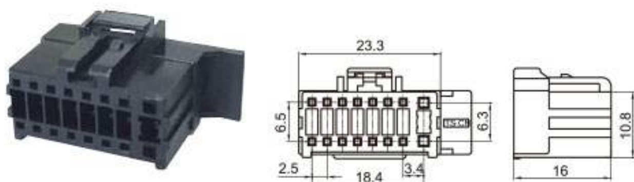
Type: TSJVC-16P-21 Material: PA66 GF30% Matching Terminal: TSH119B / TSH118
