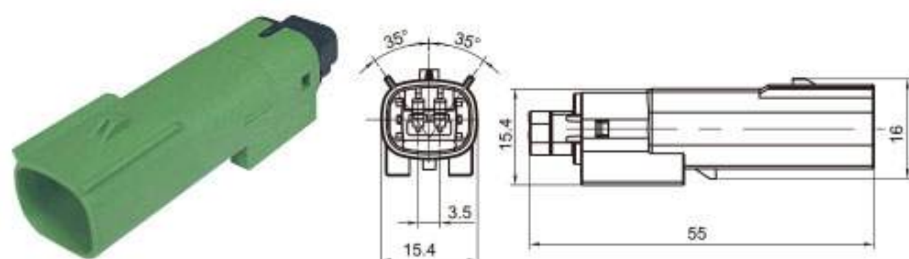
Type: TS30366-02P-11-3 Material: PA66 GF30% Matching Terminal: TSZ144A
