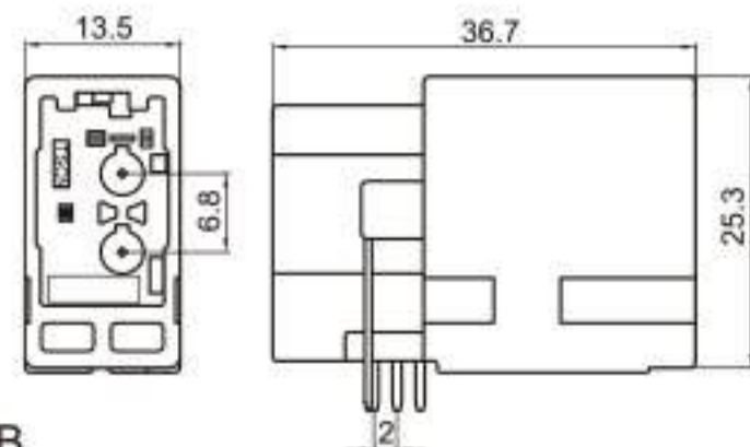
Type: TSLX03-03PM-AT-PKB Material: PBT GF30% Matching Terminal: TSPM0092~TSPM0097
