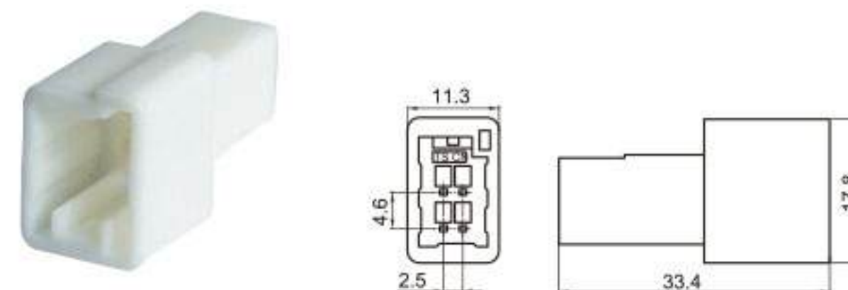
Type: TSTA04-04P-11 Material: PA66 Matching Terminal: TSZ145
