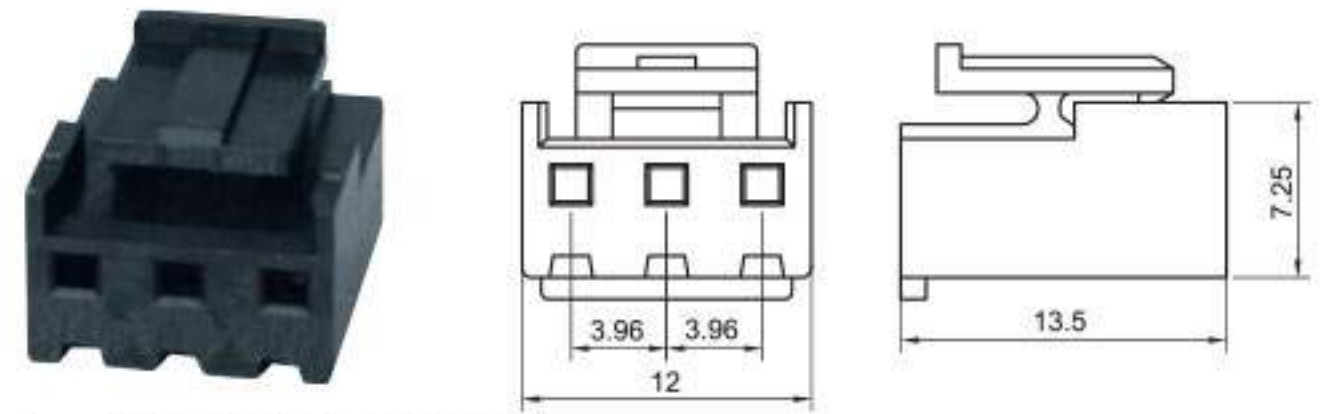
Type: TSVH-03P-21(02P-15P) Material: PA66 Matching Terminal: TSVH
