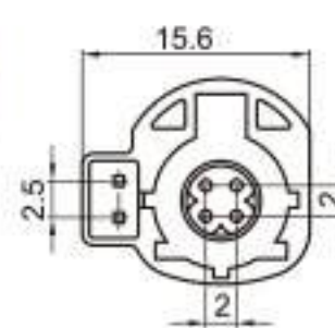
Type: TSVW10-06PM-AT Material: PBT GF30% Matching Terminal: TSPM0027 / TSPM0151 / TSPM0151-A
