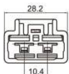
Type: TS30191-02P-11 Material: PA66 GF15% Matching Terminal: TSDJ611-7.8D
