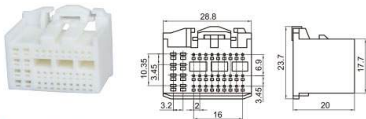
Type: TS30116-35P-21 Material: PA66 Matching Terminal: TSH593 / TSH606
