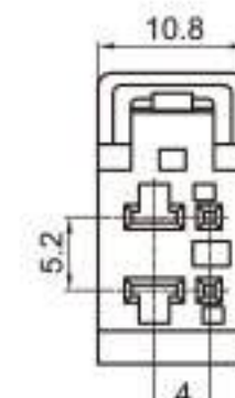
Type: TS30148-04P-21GN Material: PBT Matching Terminal: TSH091 / TSH092
