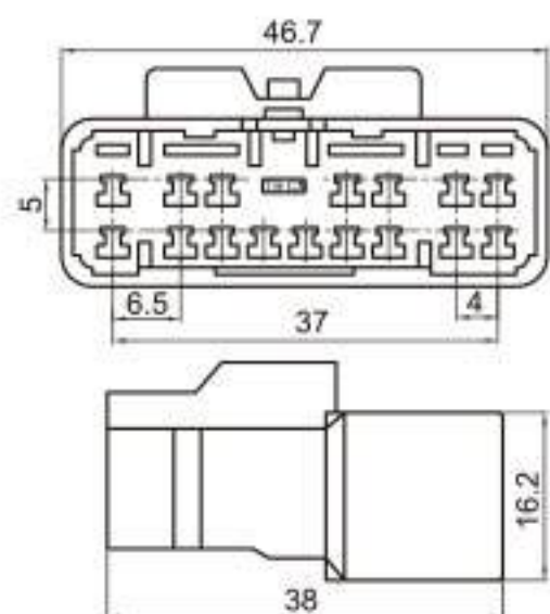
Type: TS7712-16P-11 Material: PA66 Matching Terminal: TSZ045
