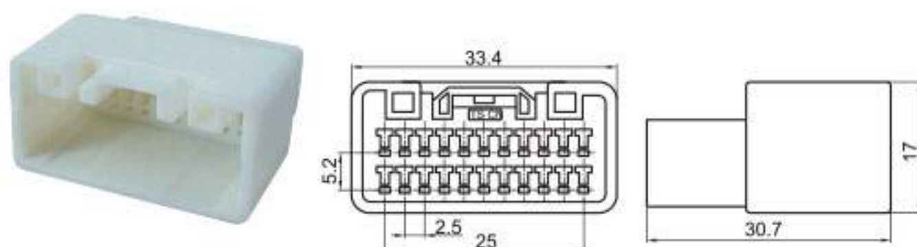
Type: TSMI22-22P-11 Material: PA66 Matching Terminal: TSZ018
