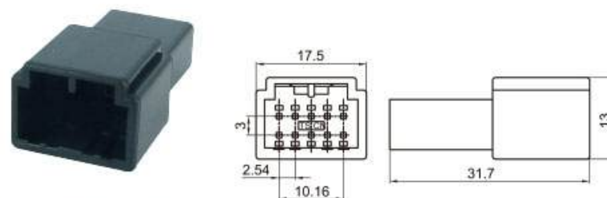
Type: TSNITL-10P-11 Material: PA66 Matching Terminal: TSZ116
