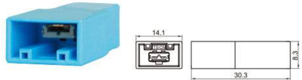
Type: TSKC3123-02PM-AT-1 Material: PA66 GF30% Matching Terminal: TSTM0021 / TSTM0022
