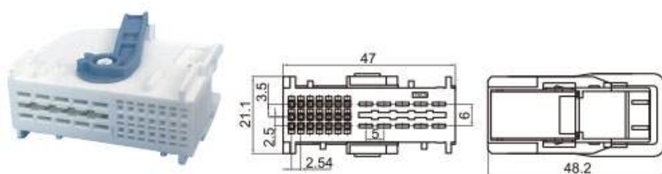
Type: TS30102-31P-21 Material: PBT GF15% Matching Terminal: TSH019/TSH143
