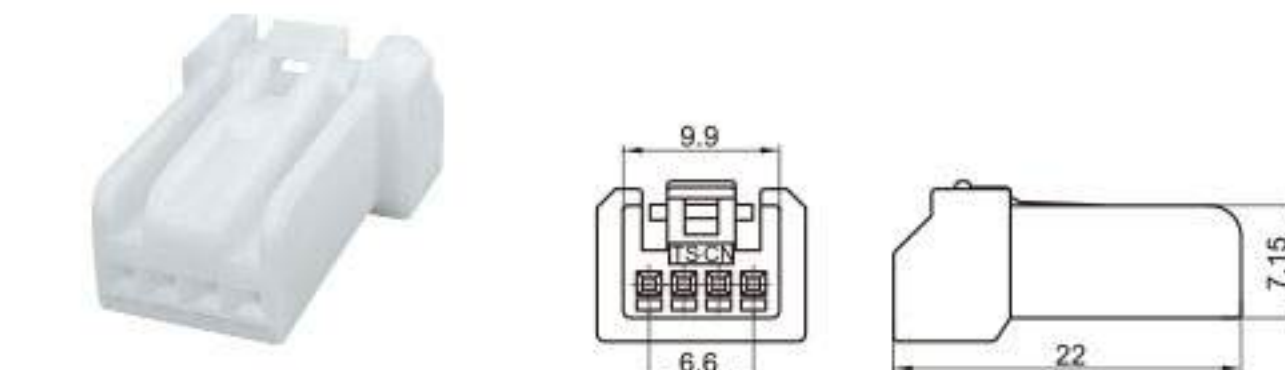
Type: TS30203-04P-21 Material: PA66 Matching Terminal: TSH143
