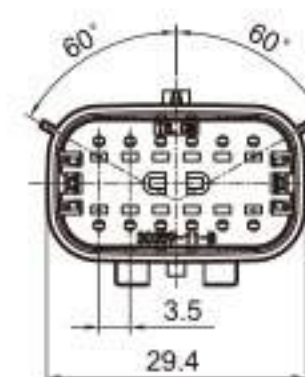
Type: TS30359-12P-11 Material: PA66 GF30% Matching Terminal: TSZ144A
