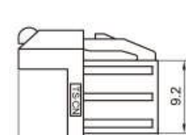
Type: TSVW20-04PF-AT-5GY Material: PA66 GF30% Matching Terminal: TSTF0048 / TSTF0049 / TSTF0050
