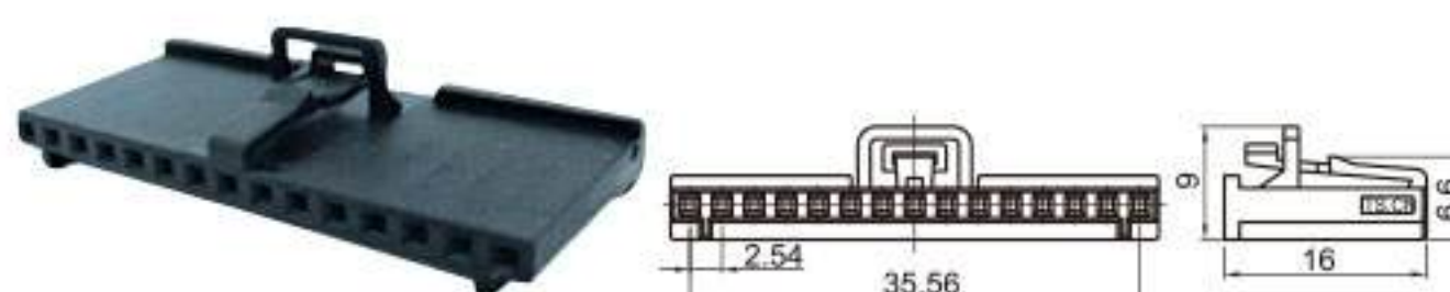
Type: TS30048-15P-21 Material: PA66 GF30% Matching Terminal: TSH069
