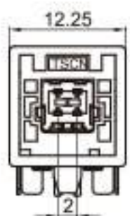
Type: TSTA04-04PM-AT-PKB-2 Material: PBT GF15% Matching Terminal: TSPM0050 / TSPM0053
