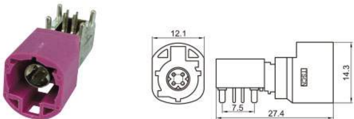
Type: TSVW10-04PM-AT-5PK Material: PA66 GF30% Matching Terminal: TSPM0021~TSPM0025
