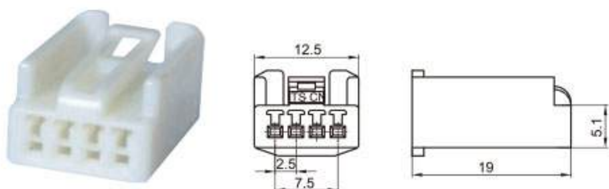
Type: TSTA04-04P-21-2 Material: PA66 Matching Terminal: TSH076
