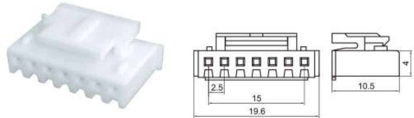
Type: TSHA-07P-21(02P-15P) Material: PA66 Matching Terminal: TSC3
