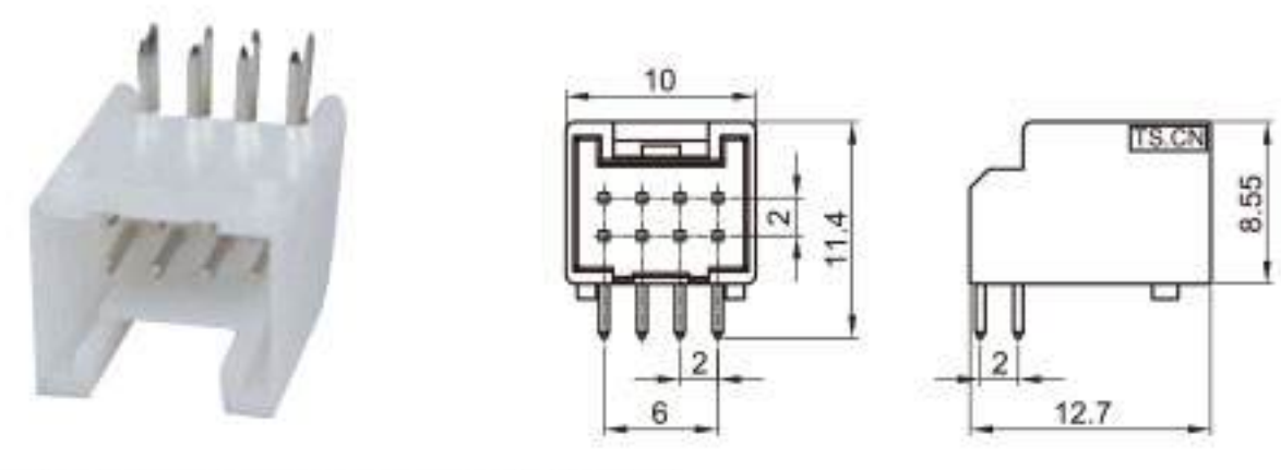
Type: TS30021-08PM-PKB(10PM) Material: PA66 Matching Terminal: TSPM0141 / TSPM0194
