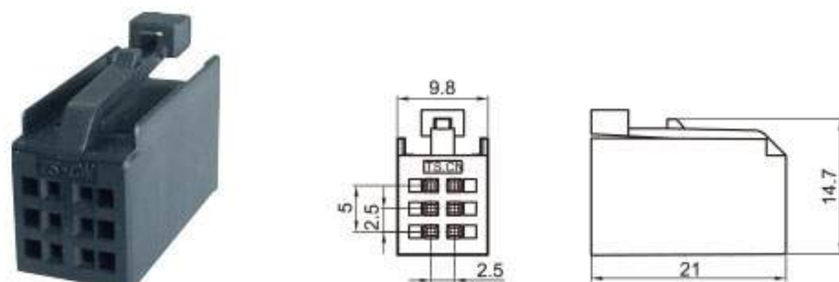
Type: TS30009-06P-21 Material: PBT GF15% Matching Terminal: TSH143
