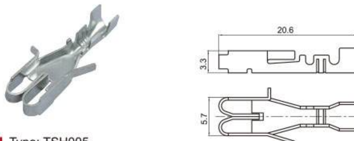
Type: TSH005 Material: Brass Applicable Thickness: 0.5
