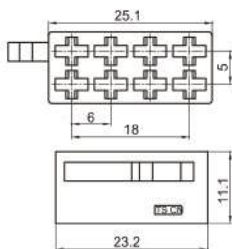
Type: TS1784A-08P-21BK Material: PA66 Matching Terminal: TSH019
