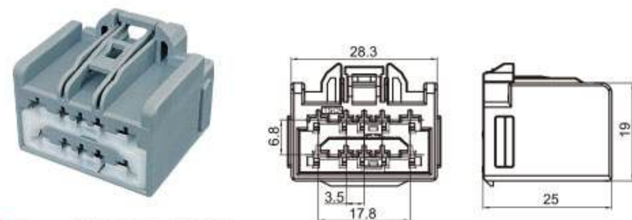
Type: TS30337-10P-21 Material: PBT GF15% Matching Terminal: TSH085 / TSH047
