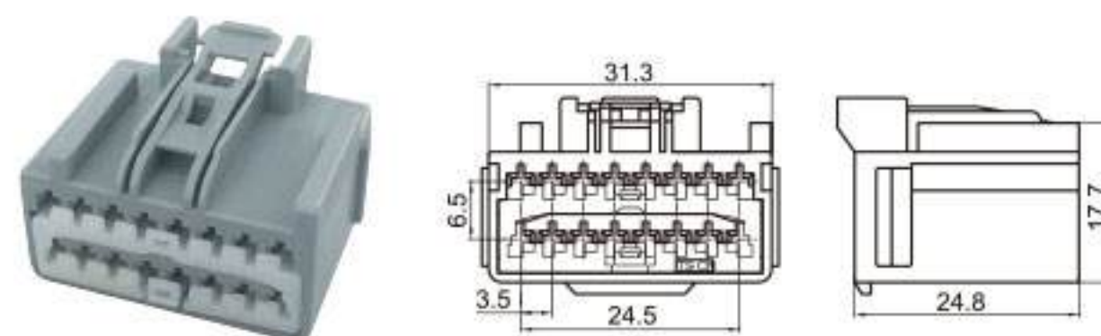
Type: TSVO16-16P-21-3 Material: PBT GF10% Matching Terminal: TSH047
