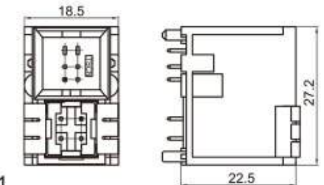
Type: TS30060-10PM-PKS-1 Material: PA66 GF30% Matching Terminal: TSPM0217 / TSPM0215 / TSPM0077 / TSPM0039
