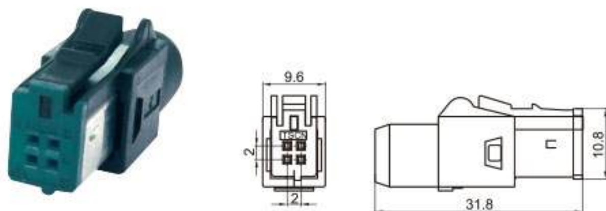
Type: TSMA04-04PF-AH-1 Material: PA66 GF15% Matching Terminal: TSAF0013 / TSPM0030
