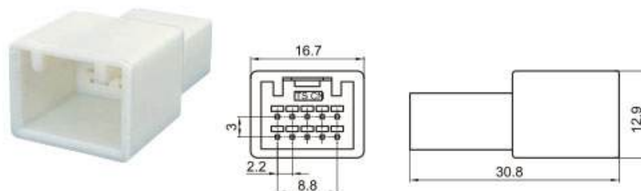
Type: TSTA10-10P-11-2 Material: PA66 Matching Terminal: TSZ208
