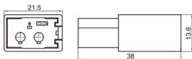
Type: TSLX11-03PM-AT Material: PA66 Matching Terminal: TSZ208 / TSTM0003 / TSTM0004
