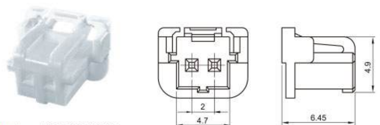
Type: TS502351200 Material: PA66 Matching Terminal: TS502128000
