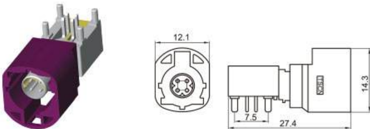
Type: TSVW10-04PM-AT-5VT Material: PA66 GF30% Matching Terminal: TSPM0021~TSPM0025
