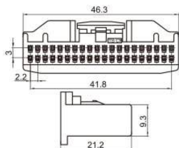
Type: TSTA40-40P-21 Material: PA66 Matching Terminal: TSH143
