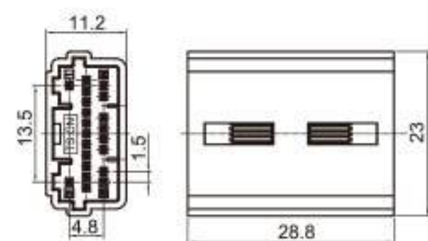
Type: TS30258-21PM-PKS Material: PBT GF15% Matching Terminal: TSPM6078 / TSPM0305
