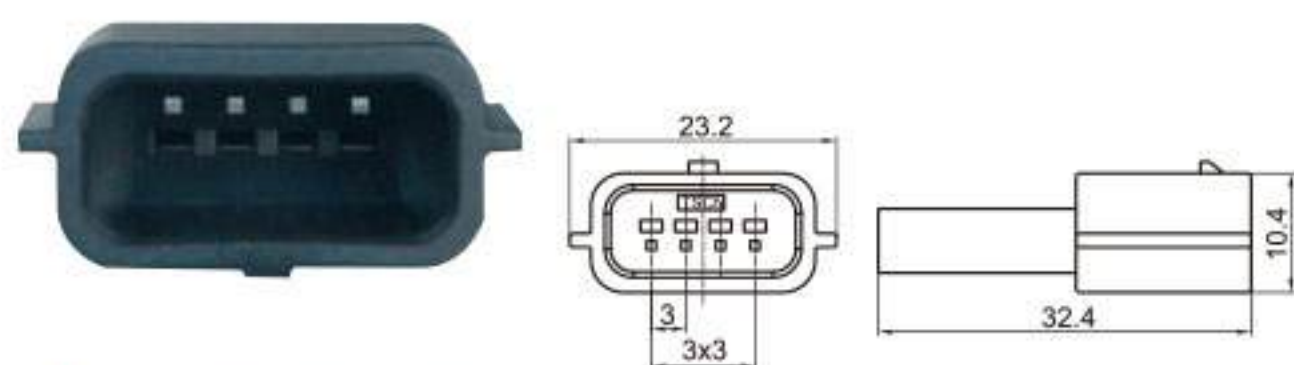
Type: TS30090-04P-11 Material: PA66 GF30% Matching Terminal: TSZ208
