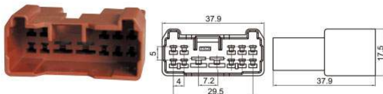
Type: TS30091-12P-11 Material: PBT GF10% Matching Terminal: TSZ028 / TSZ045
