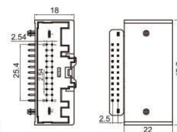
Type: TS5522-08PM-PKB Material: PA66 GF30% Matching Terminal: TSPM0009 / TSPM0012
