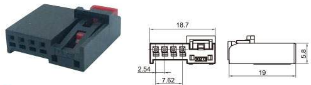
Type: TS30273-04P-21 Material: PBT Matching Terminal: TSH092
