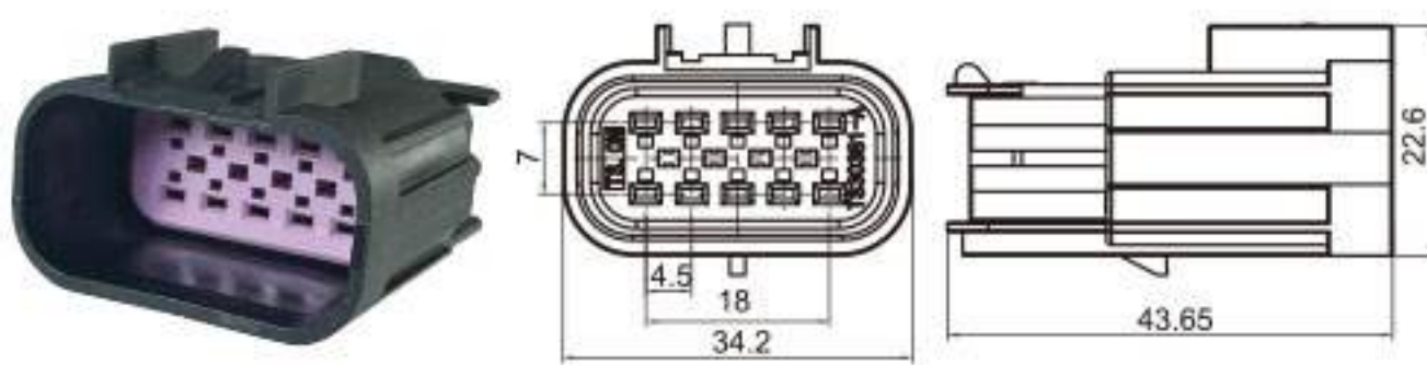
Type: TS30381-10P-11 Material: PA66 GF30% Matching Terminal: TS15326269
