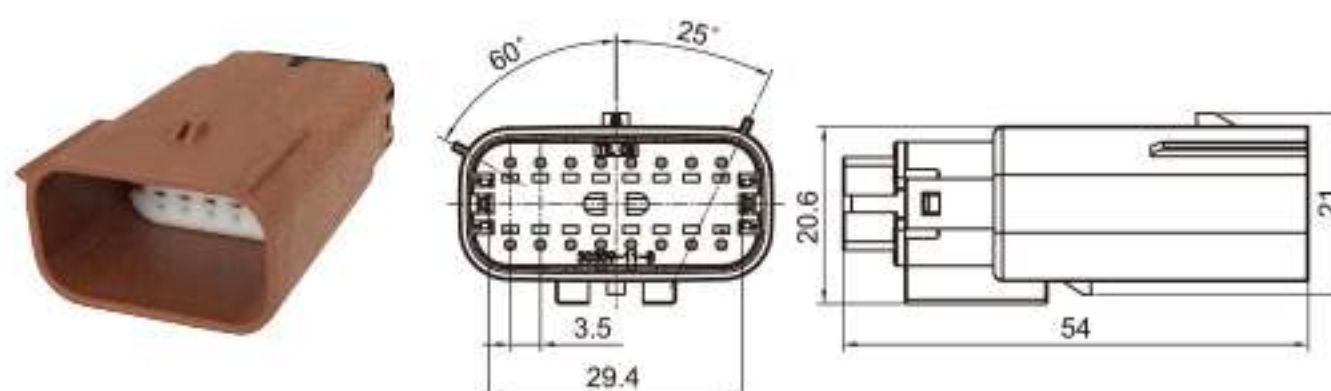
Type: TS30359-16P-11-2 Material: PA66 GF30% Matching Terminal: TSZ144A
