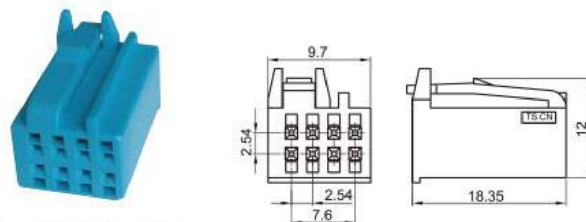
Type: TS30020-08P-21 Material: PBT GF15% Matching Terminal: TSH143
