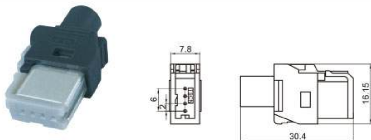
Type: TS1072-04PF-AH Material: PA66 Matching Terminal: TSAF0031 / TSPH
