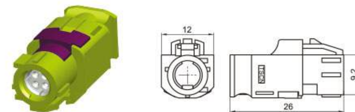
Type: TSVW20-04PF-AT-5YG-1 Material: PA66 GF30% Matching Terminal: TSTF0051 / TSTF0052
