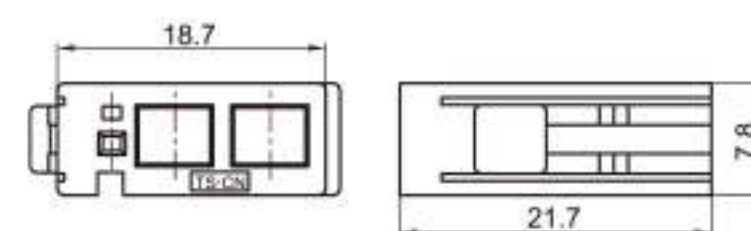
Type: TSSB20-03PF-AT Material: PA66 Matching Terminal: TSH053 / TSTF0001 / TSTF0002
