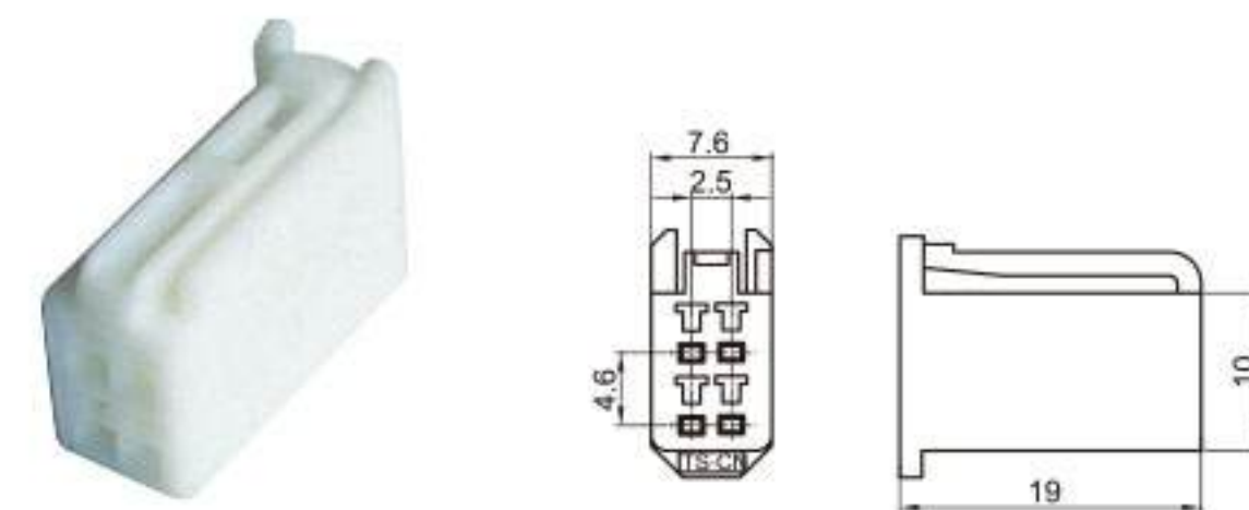
Type: TSTA04-04P-21 Material: PA66 Matching Terminal: TSH076
