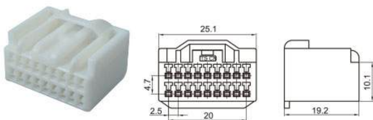
Type: TSMI18-18P-21 Material: PA66 Matching Terminal: TSH006
