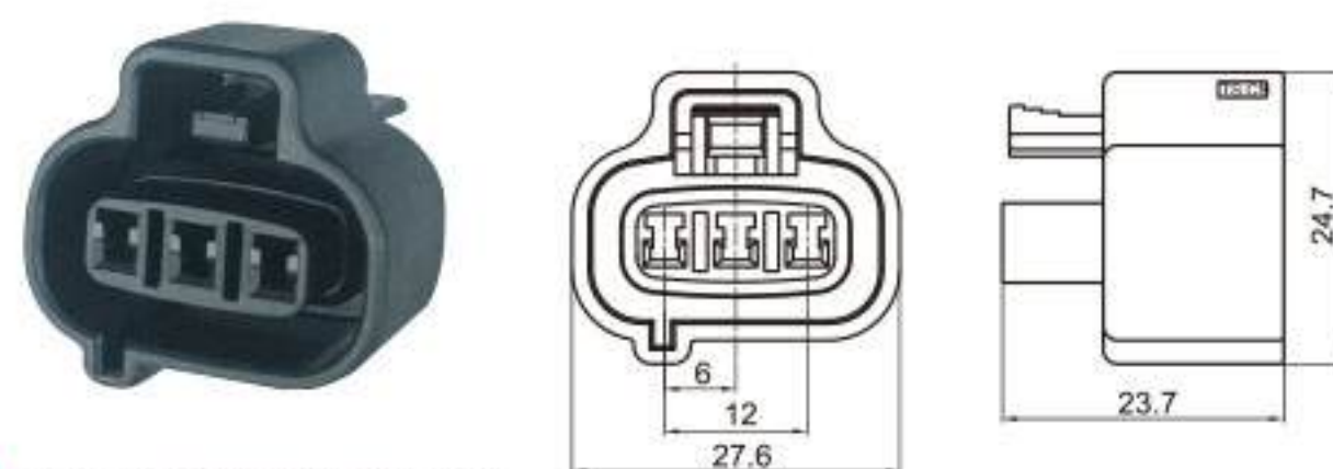
Type: TS30019-03P-21 Material: PA66 Matching Terminal: TSH064
