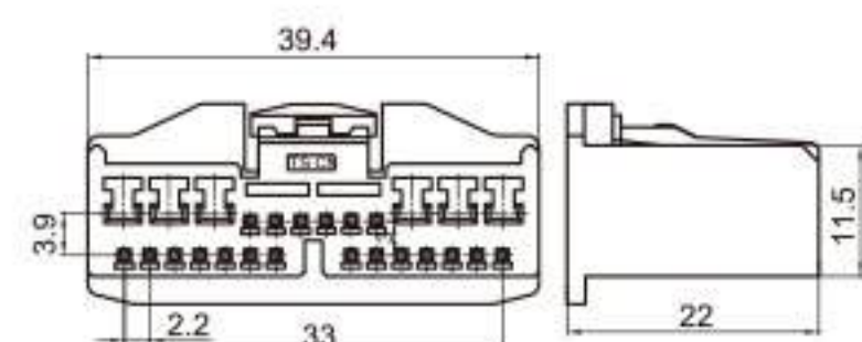
Type: TSTA26-26P-21 Material: PA66 Matching Terminal: TSH064 / TSH143
