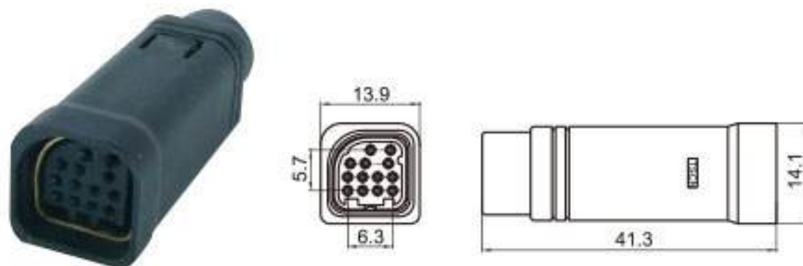
Type: TSPIOH-13PF-AH Material: PA66 Matching Terminal: TSAF0030 / TSAF0034
