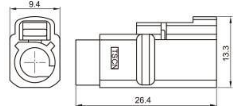
Type: TSVW20-01PF-AT-BK Material: PA66 GF30% Matching Terminal: TSTF0025 / TSTF0026
