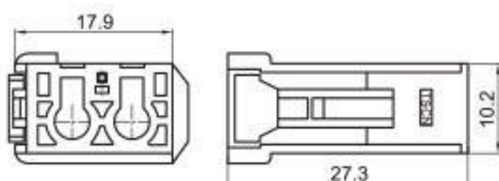
Type: TSLX21-03PF-AT Material: PA66 Matching Terminal: TSH143 / TSTF0003 / TSTF0004
