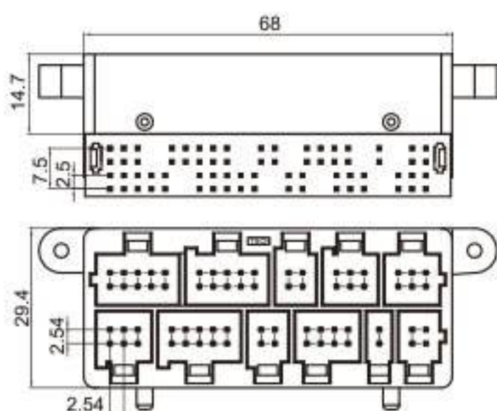
Type: TSHY66-66PM-PKB Material: PA66 Matching Terminal: TSPM0078 / TSPM0085
