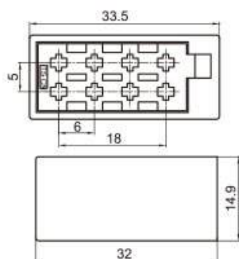
Type: TS1784A-08P-11BK Material: PA66 Matching Terminal: TSZ024
