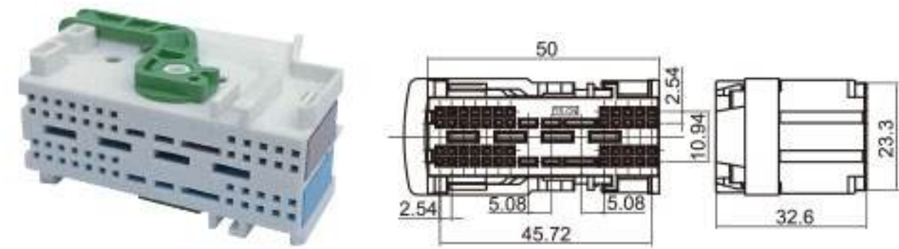
Type: TS30271-54P-21 Material: PBT GF15% Matching Terminal: TS968073-2 / TS968075-2 / TSH624
