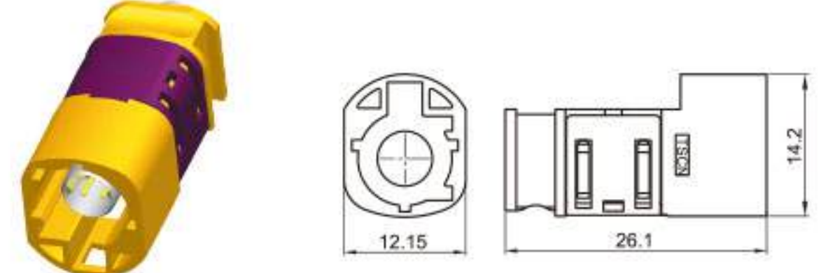
Type: TSVW10-04PM-AT-5OR-1 Material: PA66 GF15% Matching Terminal: TSPM0175 / TSTM0051
