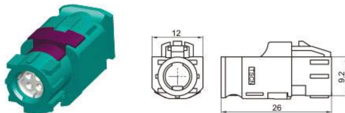
Type: TSVW20-04PF-AT-5WB-1 Material: PA66 GF30% Matching Terminal: TSTF0051 / TSTF0052
