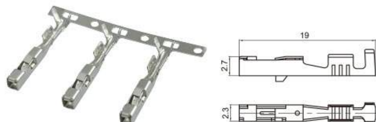
Type: TSH008 Material: Phos.bronze Applicable Thickness: 0.6~0.8
