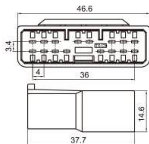
Type: TS1720-16P-11 Material: PA66 Matching Terminal: TSZ010
