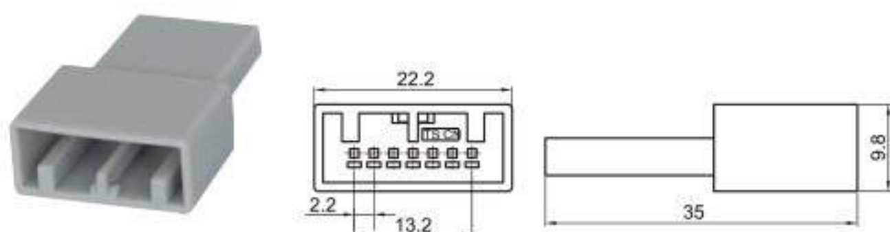
Type: TSCRV07-07P-11 Material: PA66 Matching Terminal: TSZ208B
