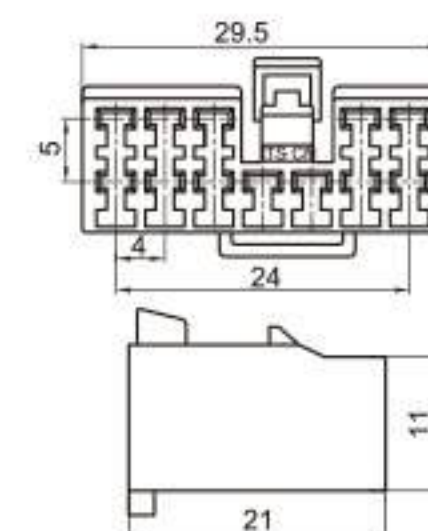
Type: TS7992-12P-21 Material: PA66 Matching Terminal: TSH009
