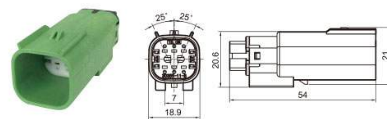
Type: TS30359-06P-11-3 Material: PA66 GF30% Matching Terminal: TSZ144A
