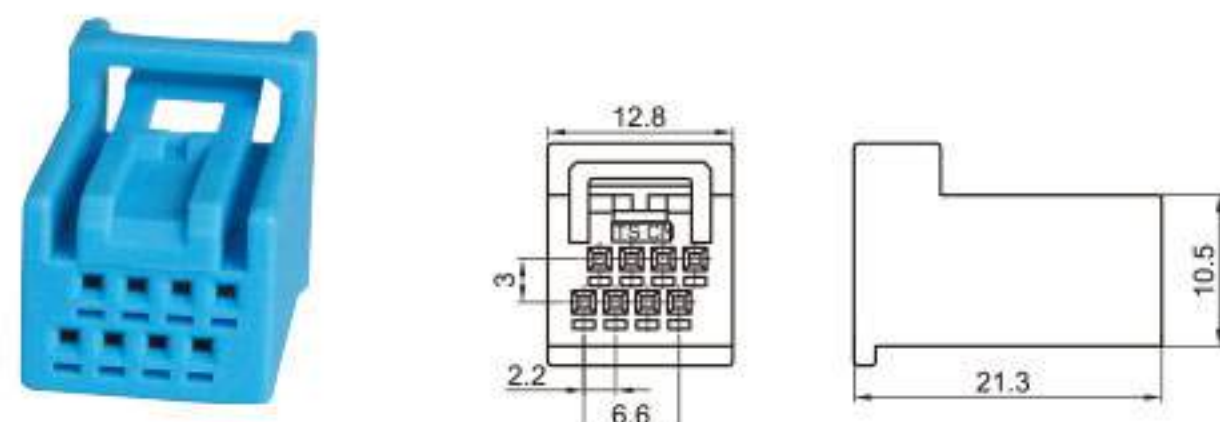
Type: TSCRV08-08P-21-1 Material: PA66 Matching Terminal: TSH143
