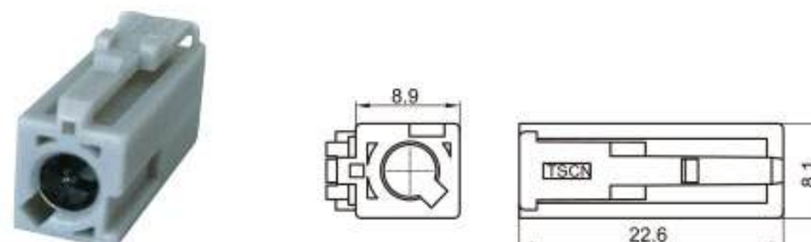
Type: TS30114-01PF-AT Material: PA66 Matching Terminal: TSTF0007/TSTM0004
