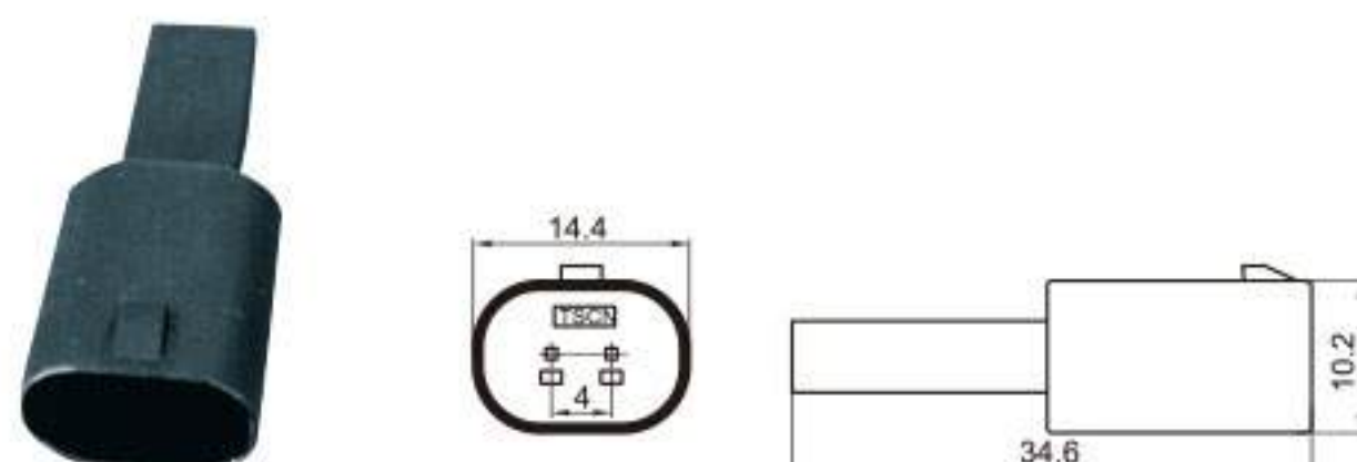
Type: TS30177-02P-11 Material: PA66 GF30% Matching Terminal: TSZ208
