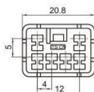
Type: TS1761-06P-11 Material: PA66 Matching Terminal: TSZ003
