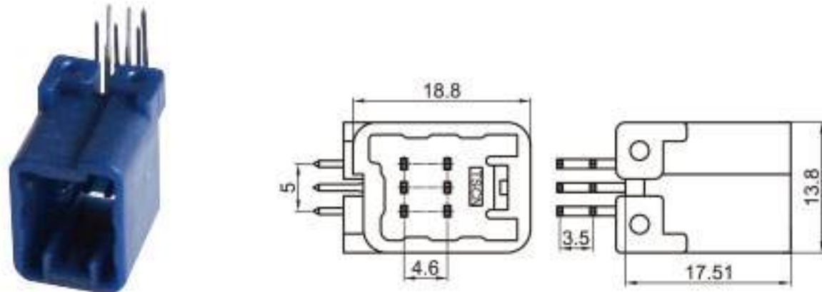
Type: TSTA06-06PM-PKB Material: PA66 GF30% Matching Terminal: TSPM0042 / TSPM0043
