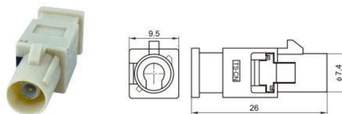
Type: TSVW10-01PM-AT-BE Material: PA66 Matching Terminal: TSTM0019 / TSTM0020
