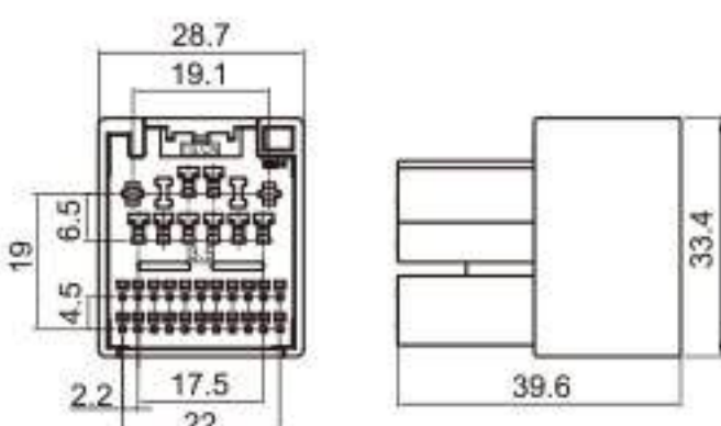
Type: TS30284-32P-11-1 Material: PA66 GF30% Matching Terminal: TSZ024 / TSZ144 / TSZ208B
