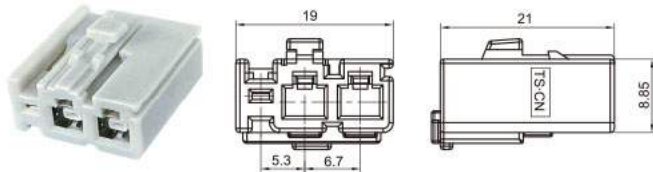
Type: TS30388-03PF-AT Material: PA66 Matching Terminal: TSH015 / TSTF0001
