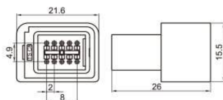
Type: TSNI10-10P-11 Material: PA66 GF30% Matching Terminal: TSZ540 / TSZ537
