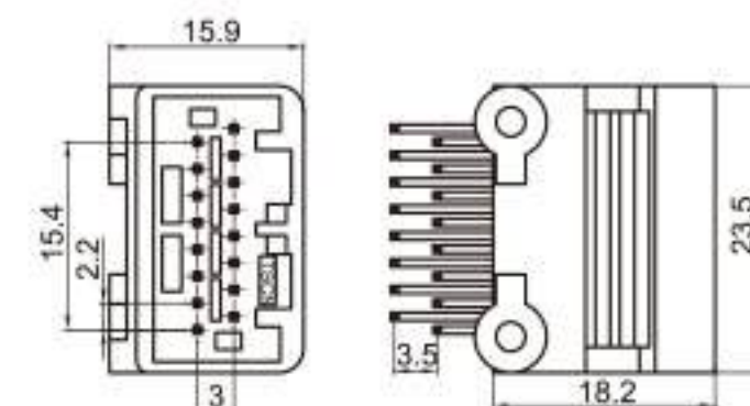
Type: TSCRV-16PM-PKB Material: PA66 Matching Terminal: TSPM0062 / TSPM0063
