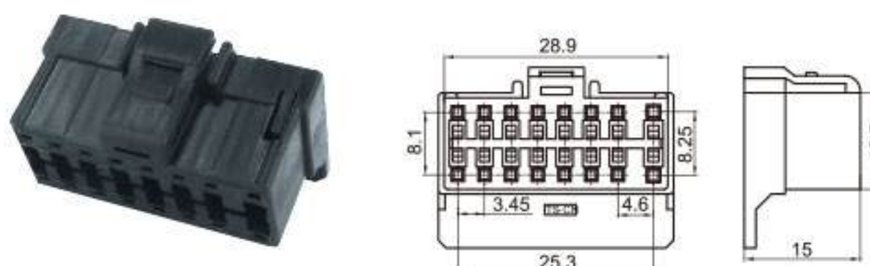
Type: TSPIO01A-16P-21 Material: PA66 GF30% Matching Terminal: TSH504 / TSH503
