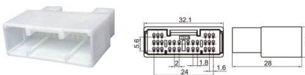
Type: TS30101-30P-11-1 Material: PA66 Matching Terminal: TSZ556
