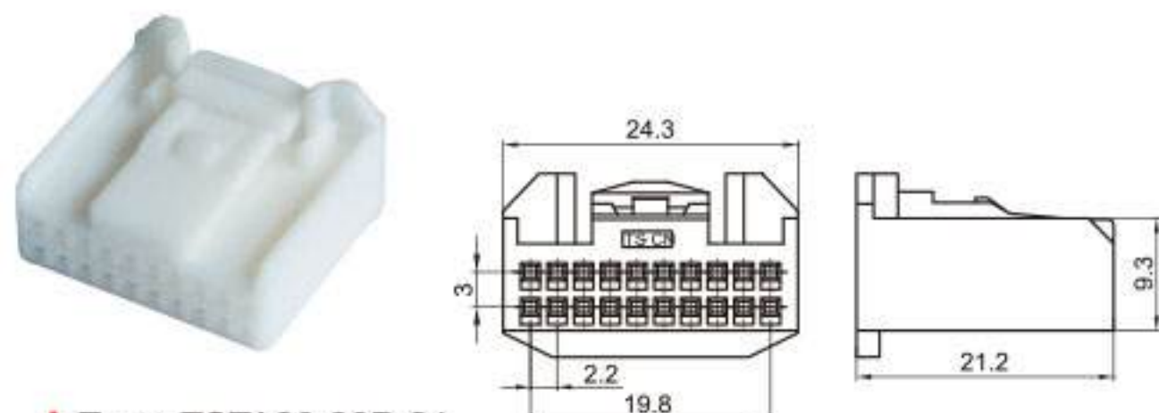
Type: TSTA20-20P-21 Material: PA66 Matching Terminal: TSH143
