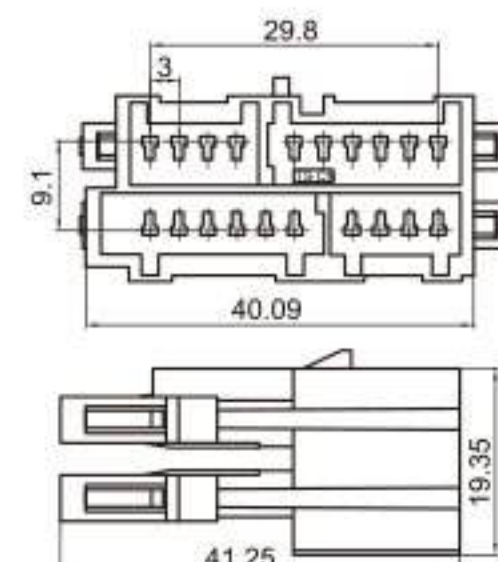
Type: TS1858-20P-11 Material: PA66 Matching Terminal: TSZ013
