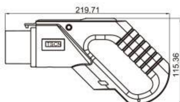
Type: TS30247(交流充电枪) Material: PA66 GF30% Matching Terminal: TS30247-K / TS30247-L / TS30247-M
