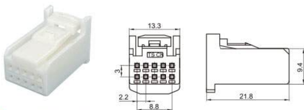
Type: TSTA10-10P-21-2 Material: PA66 Matching Terminal: TSH143
