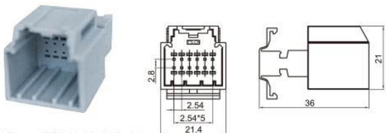
Type: TS30041-12P-11 Material: PA66 Matching Terminal: TSZ208B
