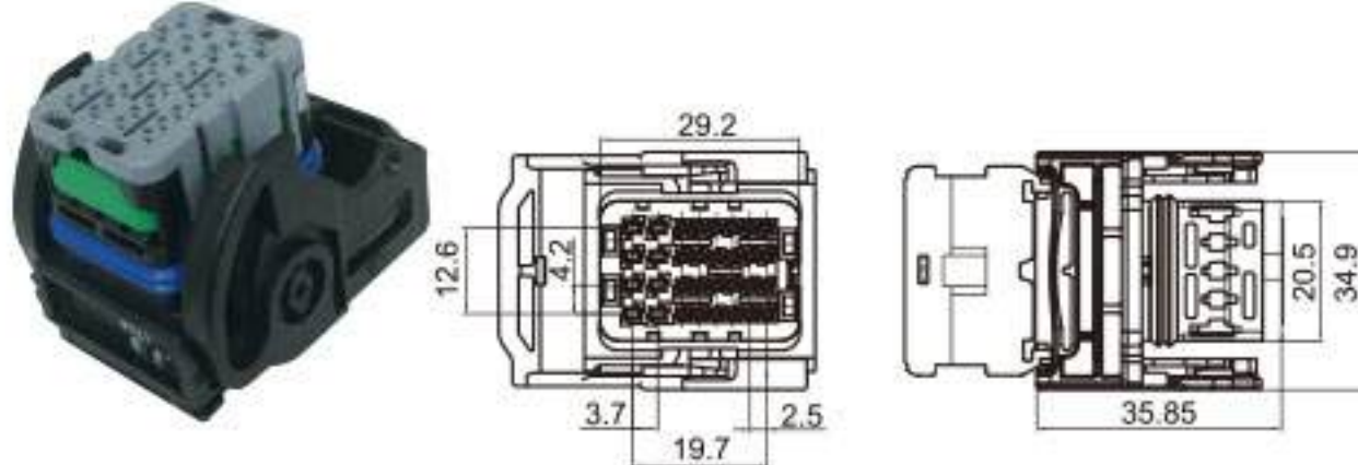
Type: TS30245-32P-21-1 Material: PA66 Matching Terminal: TSH632 / TS643221029
