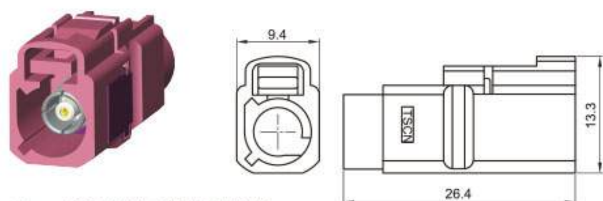
Type: TSVW20-01PF-AT-PK Material: PA66 GF30% Matching Terminal: TSTF0025 / TSTF0026
