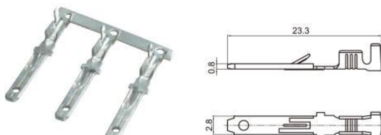
Type: TSZ024 Material: Brass
