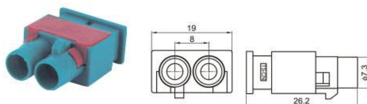
Type: TSVW10-02PM-AT-2 Material: PA66 Matching Terminal: TSTM0019 / TSTM0020
