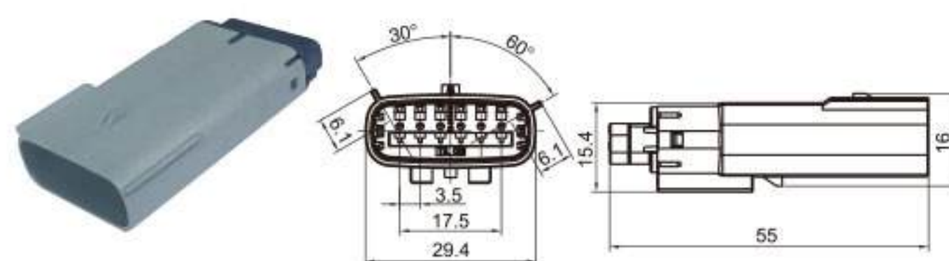
Type: TS30366-06P-11-1 Material: PA66 GF30% Matching Terminal: TSZ144A
