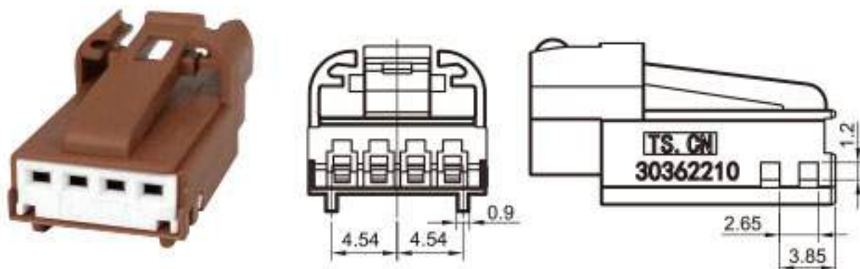
Type: TS30362-04P-21-2 Material: PA66 GF30% Matching Terminal: TSH006B
