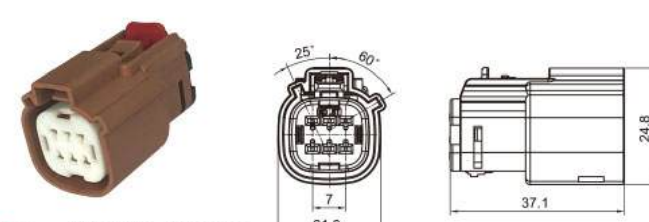
Type: TS30359-06P-21-2 Material: PA66 GF30% Matching Terminal: TSH047
