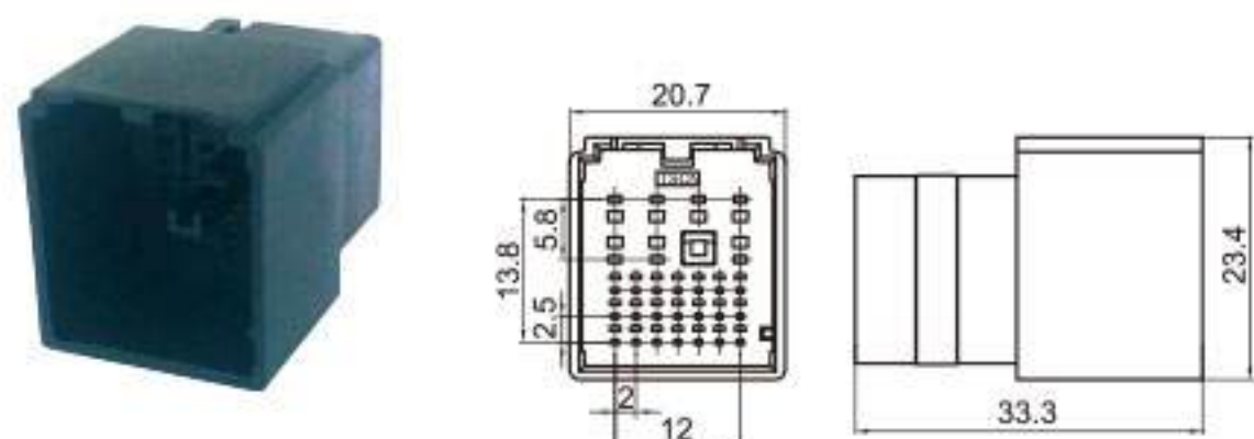
Type: TS30205-28P-11 Material: PA66 Matching Terminal: TSZ566 / TSZ561
