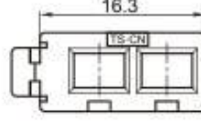
Type: TSK120-02PF-AT Material: PA66 Matching Terminal: TSTF0001 / TSTF0002
