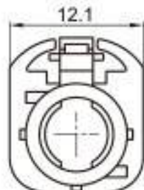
Type: TSVW20-04PF-AT-5WT Material: PA66 GF30% Matching Terminal: TSTF0048 / TSTF0049 / TSTF0050
