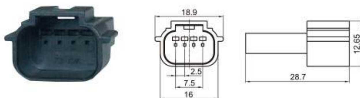
Type: TS30094-04P-11 Material: PA66 GF30% Matching Terminal: TSZ208
