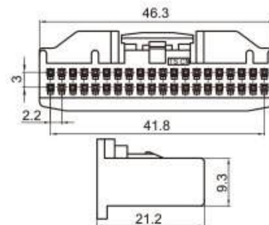
Type: TSTA40-40P-21-3 Material: PA66 Matching Terminal: TSH143
