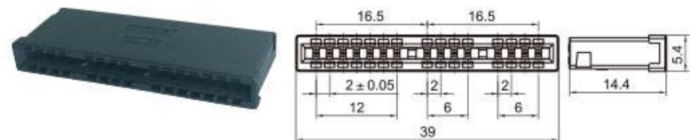
Type: TS30380-30P-21 Material: PA66 GF30% Matching Terminal: TSH650
