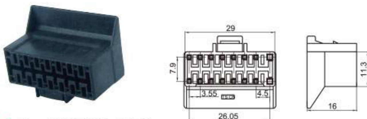
Type: TSPAN16D-16P-21 Material: PA66 GF15% Matching Terminal: TSH114 / TSH113
