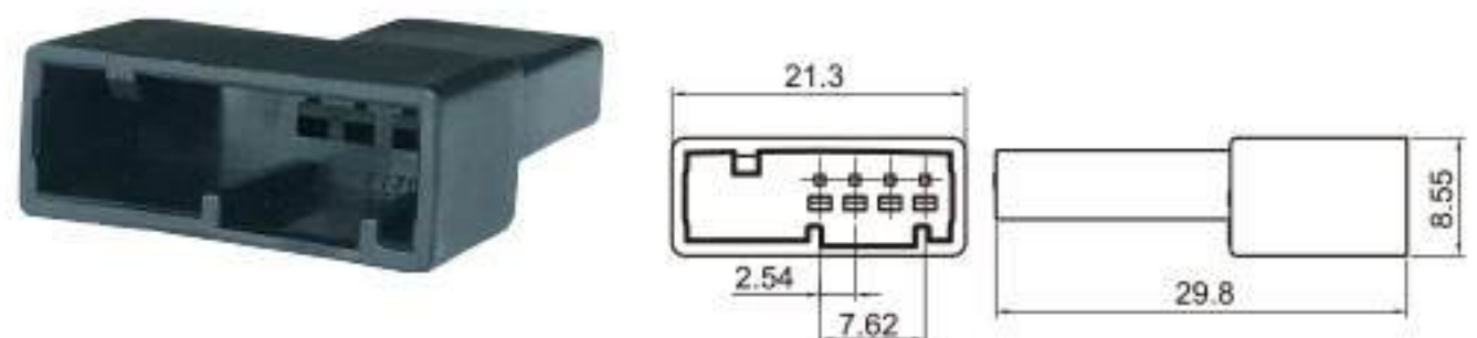
Type: TS30273-04P-11 Material: PBT Matching Terminal: TSZ208
