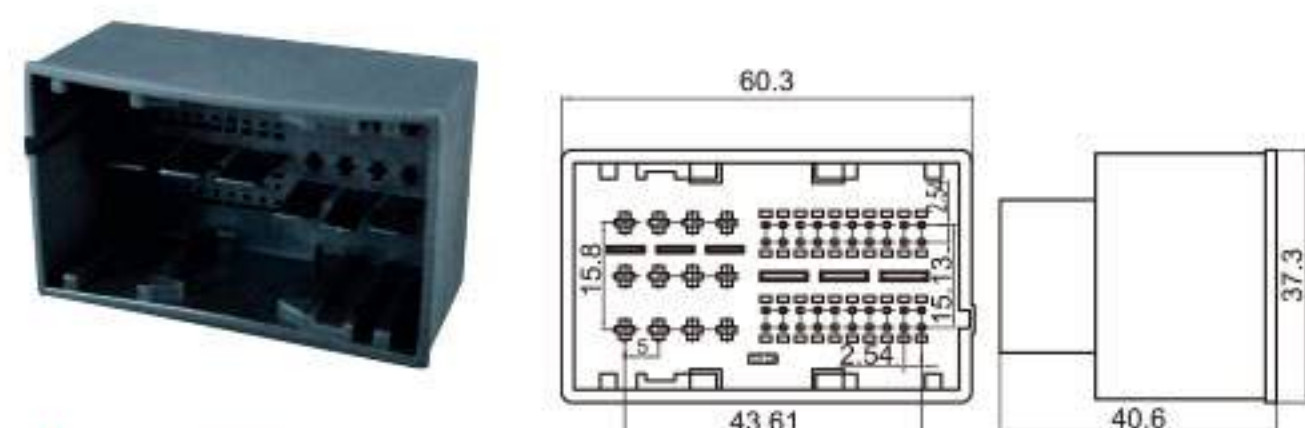
Type: TS6523-52P-11 Material: PA66 GF30% Matching Terminal: TSZ024 / TSZ208B
