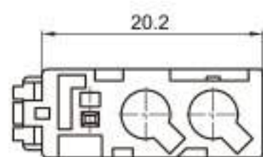
Type: TS2HD21-03PF-AT Material: PA66 Matching Terminal: TSH143 / TSTF0007 / TSTM0004
