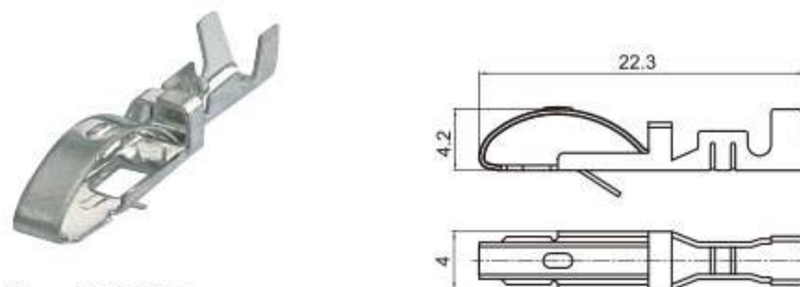
Type: TSH004 Material: Brass Applicable Thickness: 0.5
