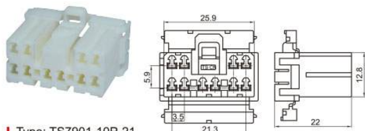
Type: TS7901-10P-21 Material: PA66 Matching Terminal: TSH016
