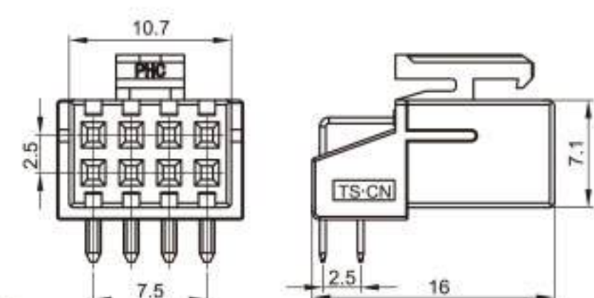
Type: TSPHC-08PF-PKB Material: PA66 Matching Terminal: TSH641 / TSH642
