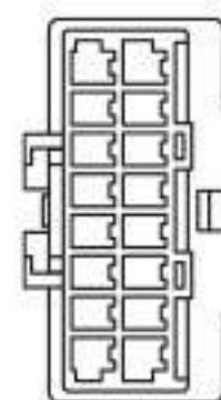
Type: TS7166S-16P-11 Material: PA66 Matching Terminal: TSDJ611-F2.2
