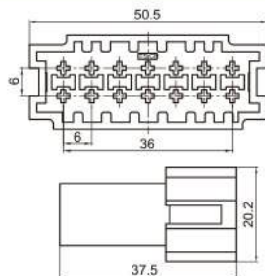
Type: TSBZ14-14P-11 Material: PA66 Matching Terminal: TSZ024
