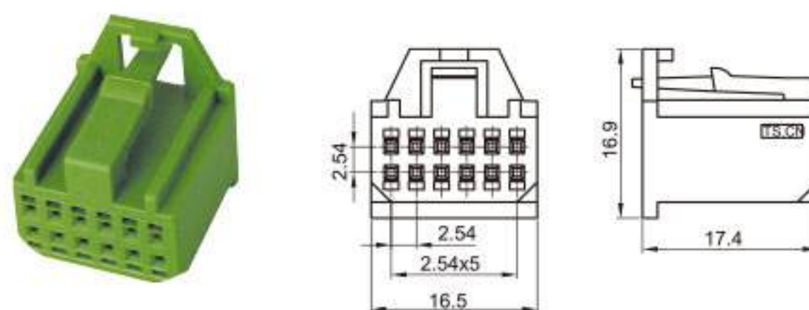
Type: TS30023-12P-21 Material: PBT Matching Terminal: TSH143
