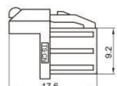
Type: TSVW20-04PF-AT-5BN Material: PA66 GF30% Matching Terminal: TSTF0048 / TSTF0049 / TSTF0050
