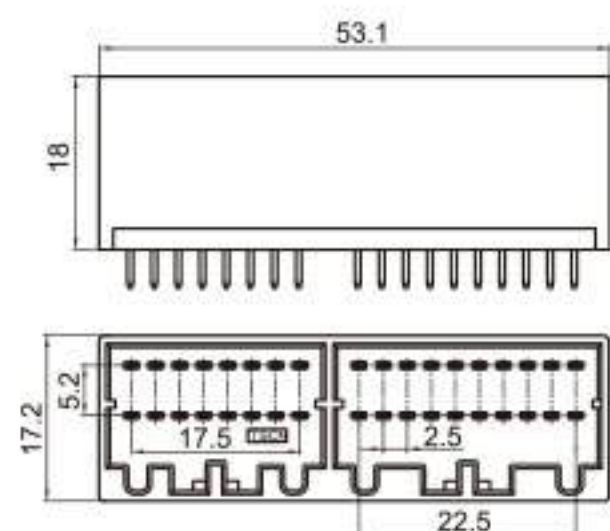
Type: TSHD36-36PM-PKS Material: PA66 Matching Terminal: TSPM0090
