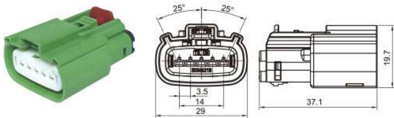
Type: TS30366-05P-21-3 Material: PA66 GF30% Matching Terminal: TSH047
