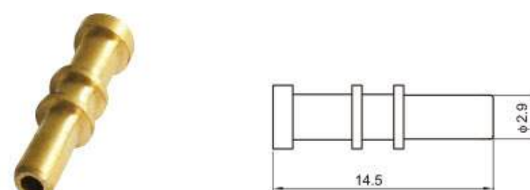
Type: TSBMGQ-C Material: Brass Matching Terminal: NIL
