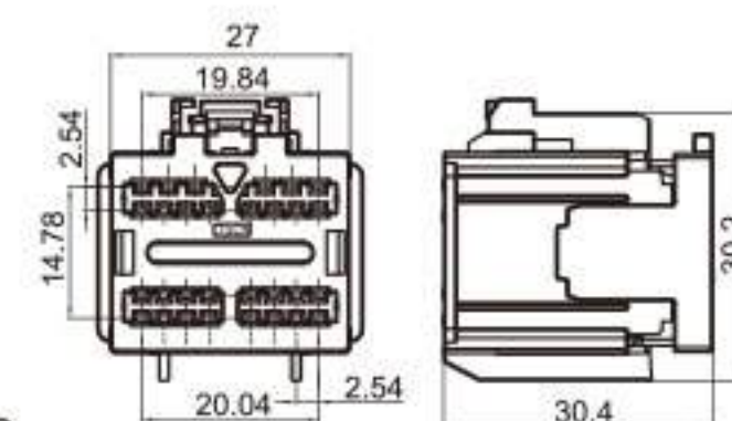
Type: TS30358-30P-21-3 Material: PBT GF10% Matching Terminal: TSH076 / TSH006B
