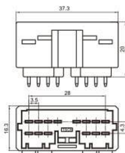
Type: TS7001-14PM-PKS Material: PA66 Matching Terminal: TSPM0049
