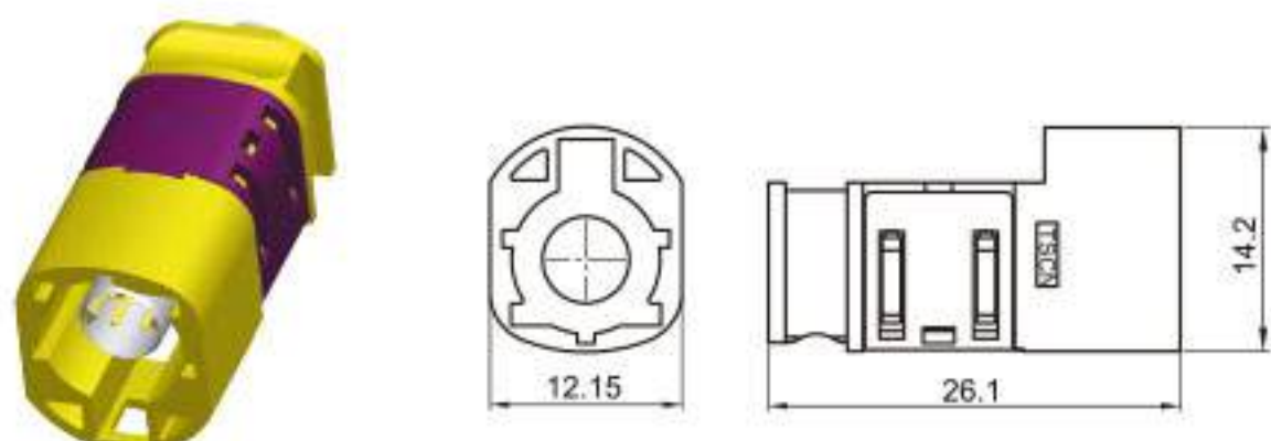
Type: TSVW10-04PM-AT-5CU-1 Material: PA66 GF15% Matching Terminal: TSPM0175 / TSTM0051
