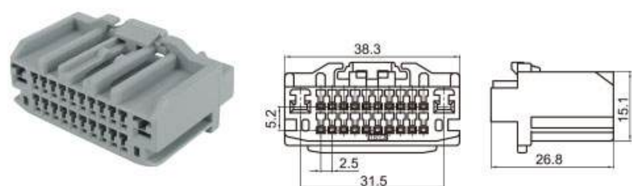
Type: TS6522-22P-21 Material: PA66 Matching Terminal: TSH085 / TSH006
