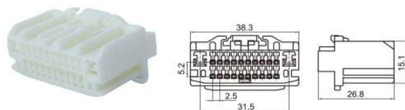
Type: TS6522-22P-21-1 Material: PA66 Matching Terminal: TSH085 / TSH006
