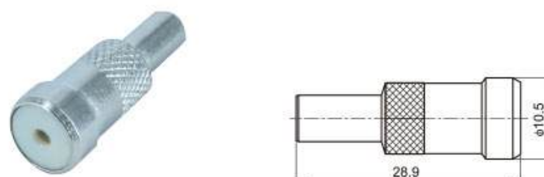
Type: TSVW02-01PF-AT Material: BRASS Matching Terminal: TSTF0027
