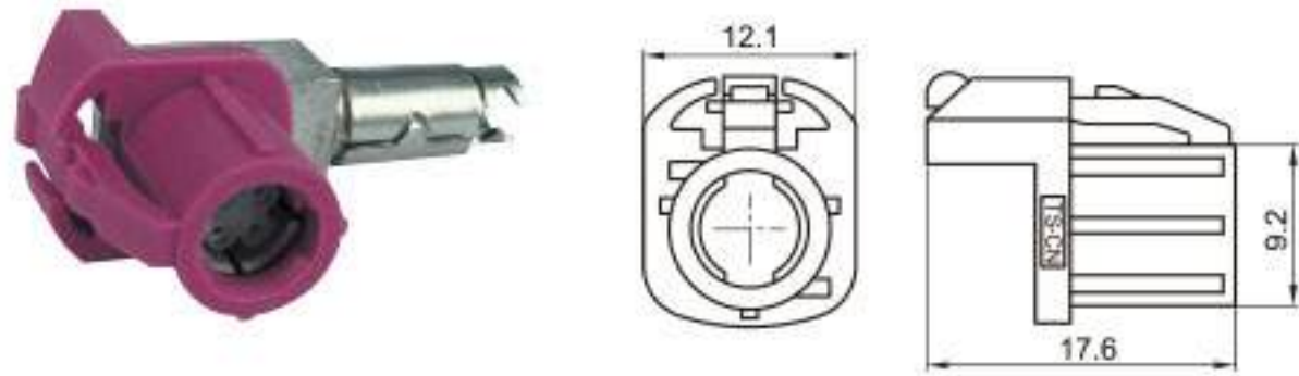
Type: TSVW20-04PF-AT-5PK Material: PA66 GF30% Matching Terminal: TSTF0048 / TSTF0049 / TSTF0050
