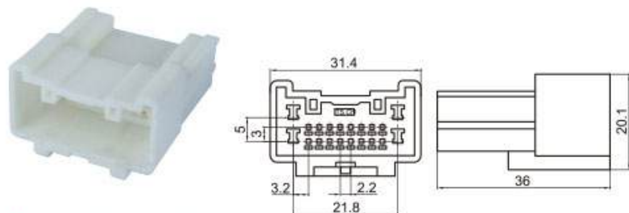
Type: TSTA20-20P-11-2 Material: PA66 Matching Terminal: TSZ045 / TSZ208
