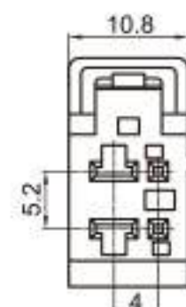
Type: TS30148-04P-21CR Material: PBT Matching Terminal: TSH091 / TSH092
