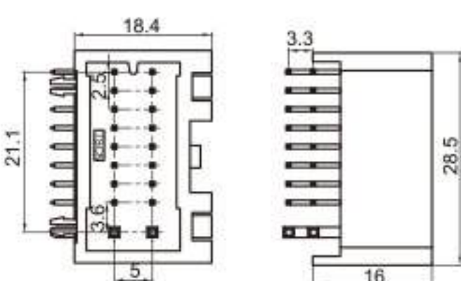
Type: TSCLR-18PM-PKB Material: PA66 Matching Terminal: TSPM0034~TSPM0037
