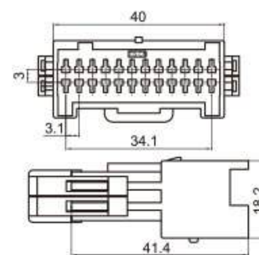
Type: TS2102-24P-11 Material: PA66 Matching Terminal: TSZ013
