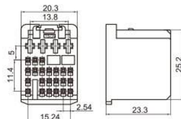
Type: TS30217-30P-11-3 Material: PBT GF15% Matching Terminal: TSDJ615B-2.8*0.8B / TSZ208
