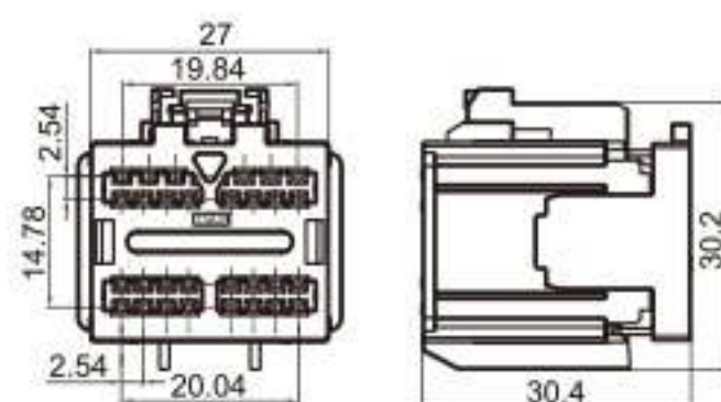
Type: TS30358-30P-21 Material: PBT GF15% Matching Terminal: TSH076 / TSH006B
