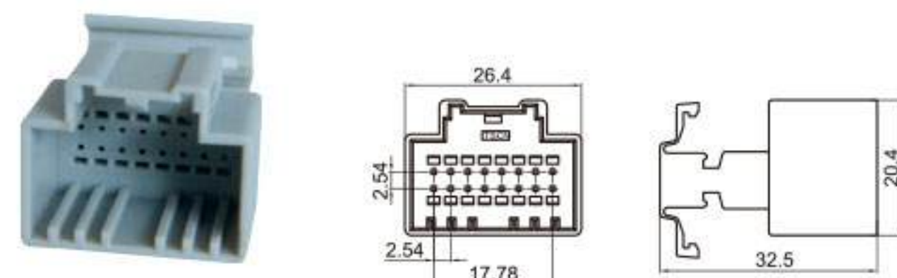
Type: TS30075-16P-11(2015) Material: PA66 GF15% Matching Terminal: TSZ208B
