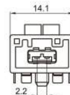
Type: TSKC3123-02PM-PKB Material: PBT GF30% Matching Terminal: TSTM017~TSPM0019
