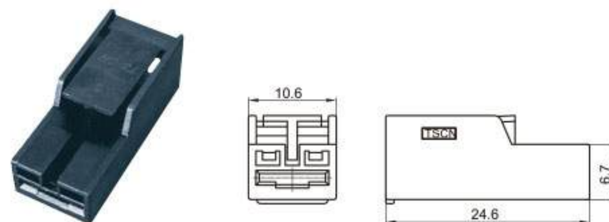
Type: TS30181-01P-21 Material: PA66 GF30% Matching Terminal: TSH613
