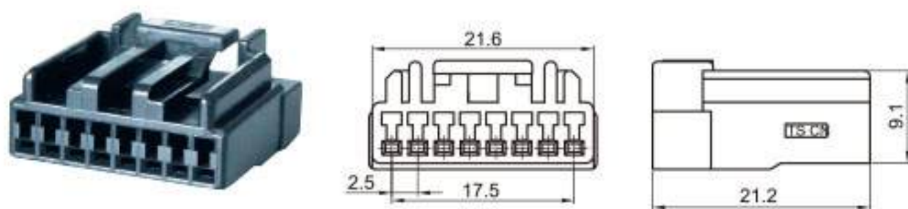
Type: TSHD08-08P-21 Material: PA66 GF30% Matching Terminal: TSH076
