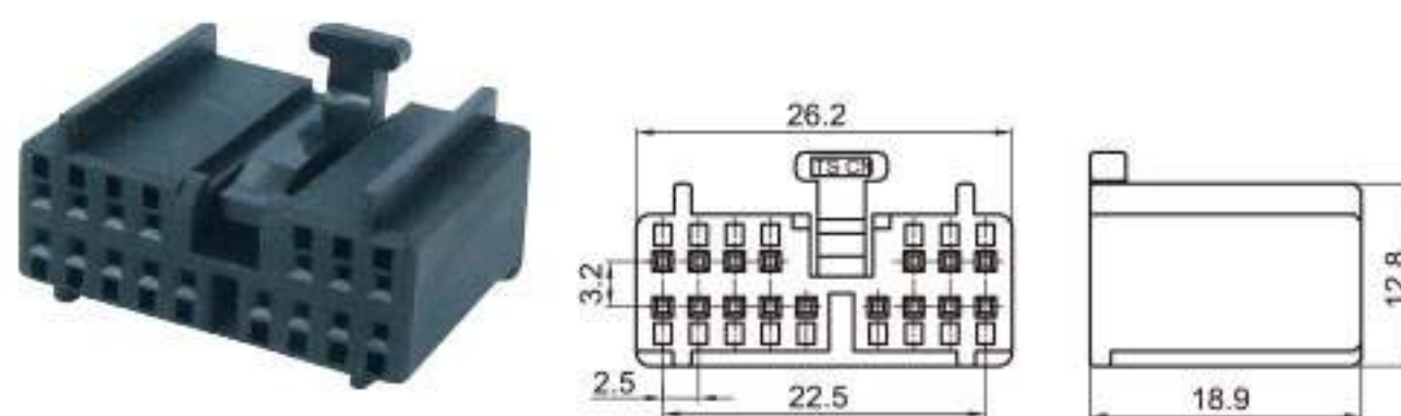
Type: TSHD16-16P-21 Material: PA66 Matching Terminal: TSH143
