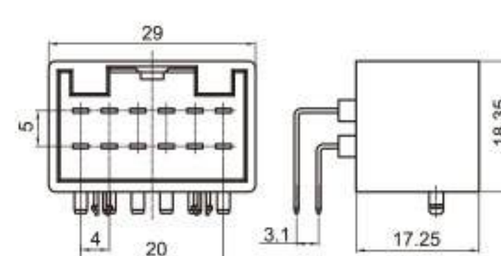
Type: TS30135-12PM-PKB Material: PBT GF15% Matching Terminal: TSPM0241 / PM0242
