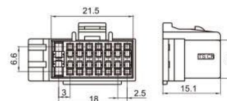
Type: TSSY16-16P-21 Material: PA66 GF30% Matching Terminal: TSH114 / TSH113
