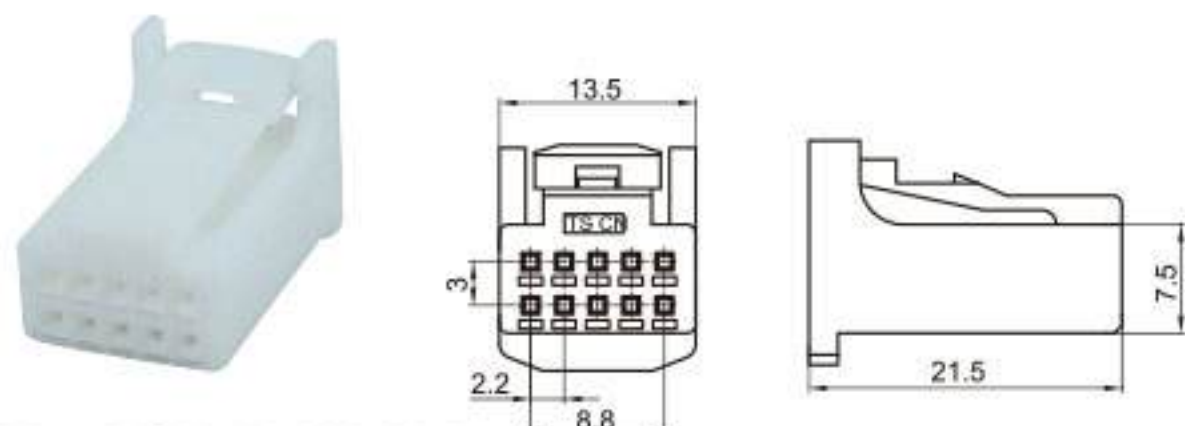
Type: TSTA10-10P-21-1 Material: PA66 Matching Terminal: TSH143
