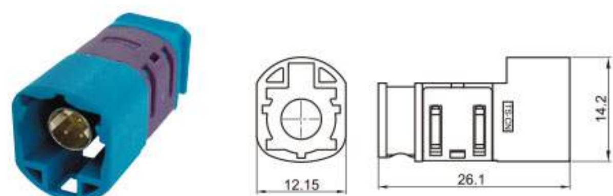
Type: TSVW10-04PM-AT-5LG-1 Material: PA66 GF15% Matching Terminal: TSPM0175 / TSTM0051
