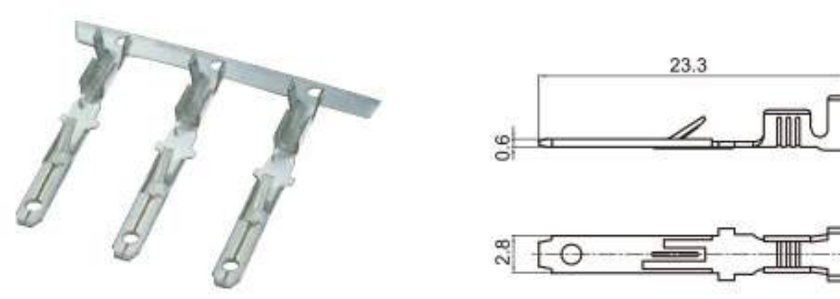
Type: TSZ024B Material: Brass
