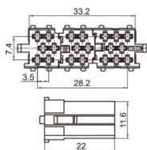
Type: TSAD20-20P-21 Material: PA66 Matching Terminal: TSH054
