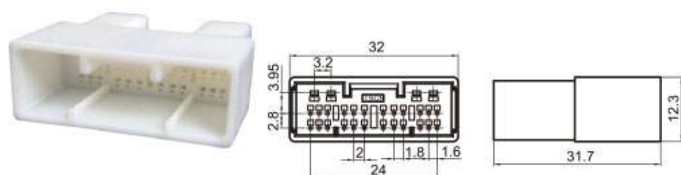
Type: TS30101-28P-11 Material: PA66 Matching Terminal: TSZ562 / TSZ556
