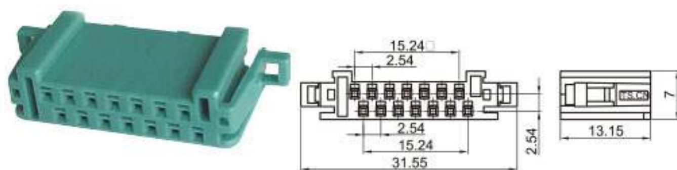
Type: TS30014-14P-21 Material: PBT GF15% Matching Terminal: TSPHB
