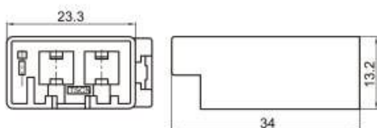
Type: TSLX10-03PM-AT Material: PA66 GF15% Matching Terminal: TSTM0016 / TSTM0015 / TSTM0013
