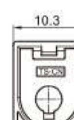
Type: TS1068-01PM-AT-3 Material: PA66 GF30% Matching Terminal: TSTM0003 / TSTM0004
