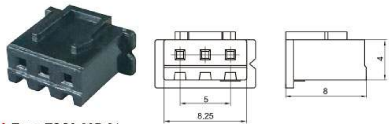
Type: TSC3-03P-21 Material: PA66 Matching Terminal: TSC3
