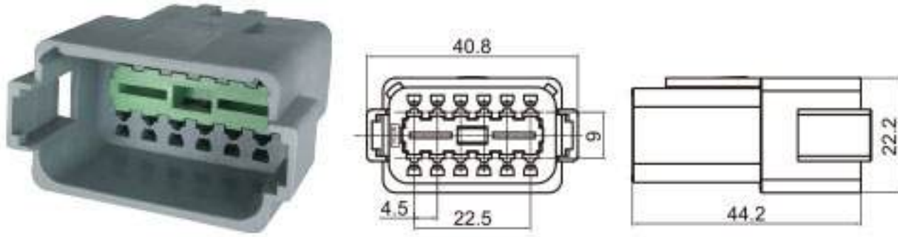
Type: TS30267-12P-11 Material: PBT GF15% Matching Terminal: TSZ621
