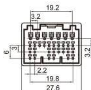
Type: TS30124-31P-11 Material: PA66 Matching Terminal: TSZ145 / TSZ208
