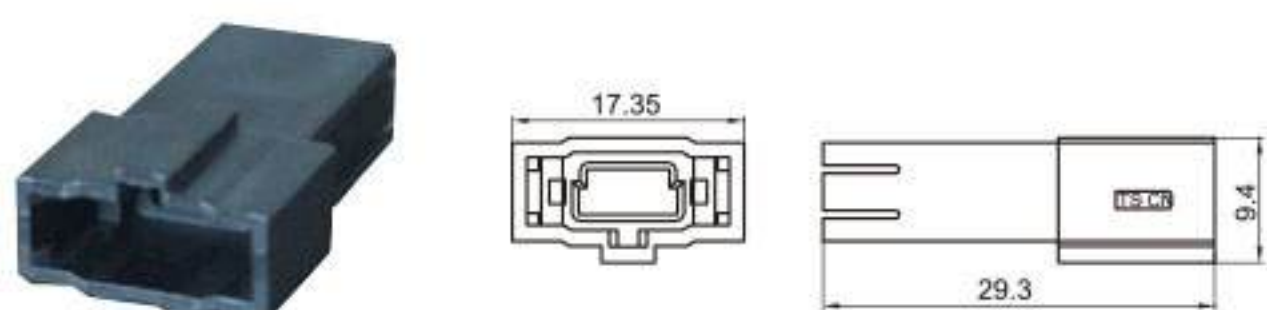
Type: TS1056-MINIUSB-21 Material: PA66 GF15% Matching Terminal: TSMINIUSB-F
