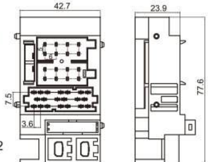
Type: TSVW36-36PM-PKS-1 Material: PA66 GF30% Matching Terminal: TSPM0109~TSPM0113
