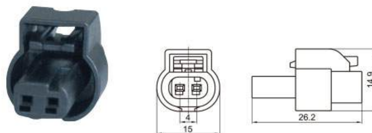
Type: TS30095-02P-21 Material: PA66 GF30% Matching Terminal: TSH092
