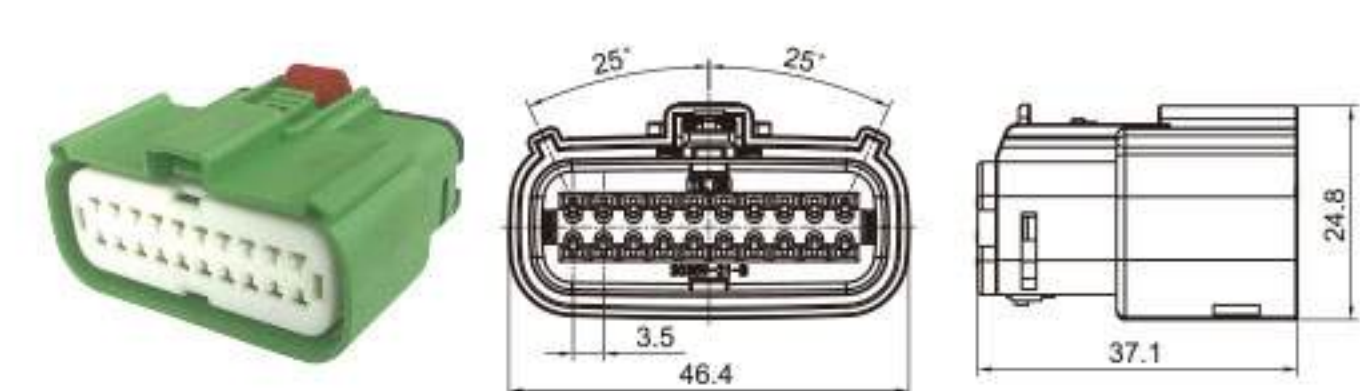
Type: TS30359-20P-21-3 Material: PA66 GF30% Matching Terminal: TSH047
