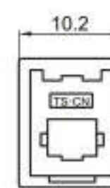
Type: TSK111-01PM-AT Material: PA66 Matching Terminal: TSTM0001 / TSTM0002
