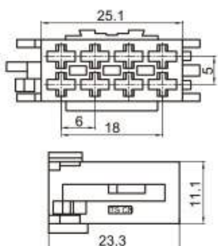
Type: TS1784A-08P-21-3BN Material: PA66 Matching Terminal: TSH019
