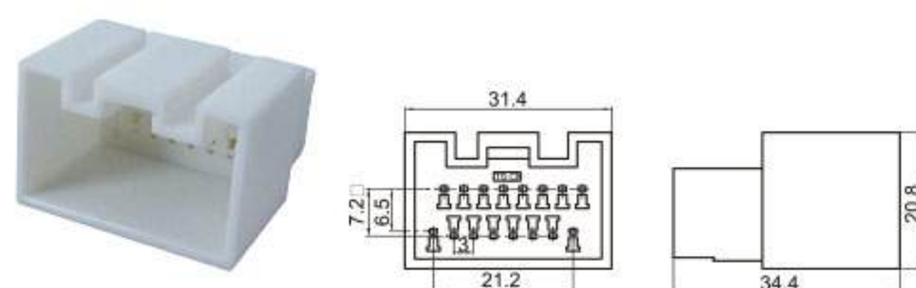
Type: TS1771-16P-11 Material: PA66 Matching Terminal: TSZ018
