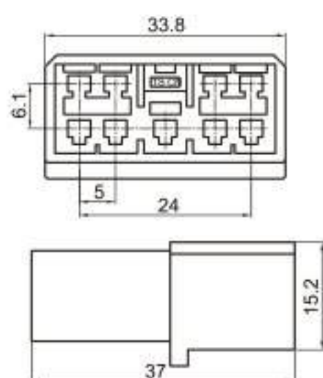
Type: TS1780-09P-11 Material: PA66 Matching Terminal: TSZ016
