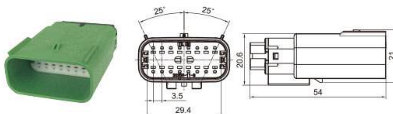
Type: TS30359-16P-11-3 Material: PA66 GF30% Matching Terminal: TSZ144A
