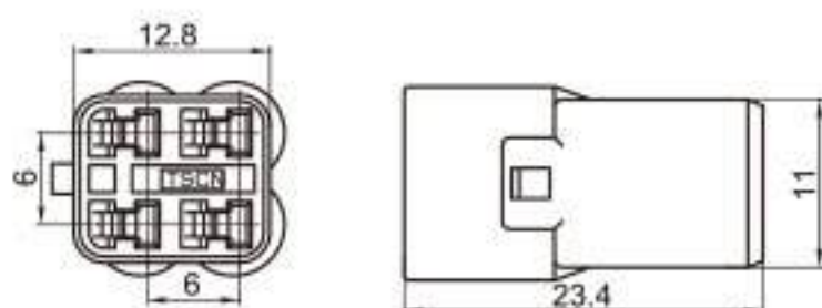
Type: TS30239-04P-21 Material: PBT Matching Terminal: TSDJ7045F-2.2-21
