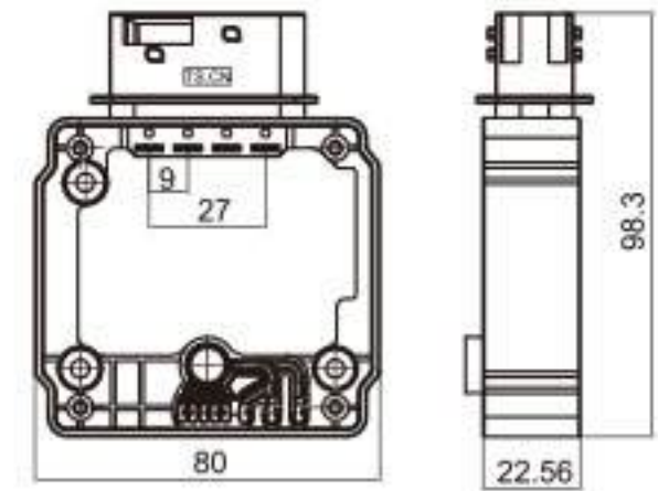
Type: TS30311-10PM-PKB Material: PBT GF15% Matching Terminal: TSPM0314 / TSPM0316
