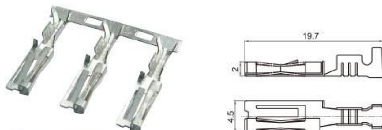
Type: TSH003 Material: Phos.bronze Applicable Thickness: \phi 1.0
