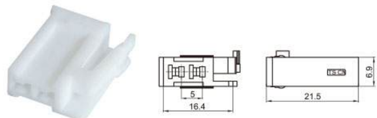
Type: TSLB10-02P-21 Material: PBT 1100 Matching Terminal: TSH064
