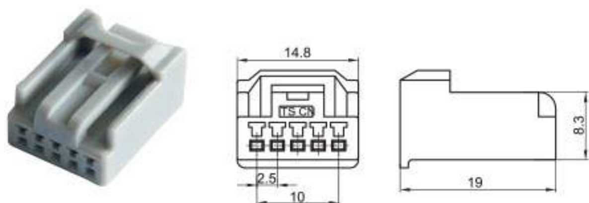
Type: TSTA05-05P-21 Material: PA66 Matching Terminal: TSH076
