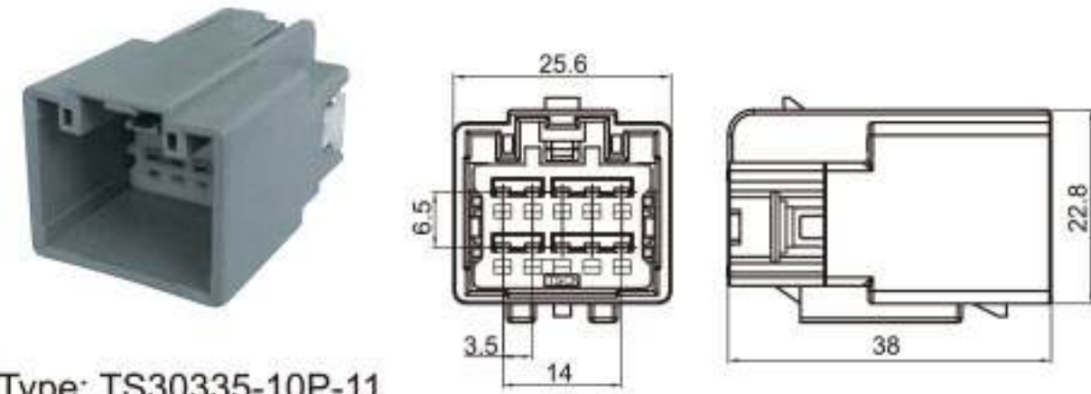
Type: TS30335-10P-11 Material: PBT GF15% Matching Terminal: TSZ144A
