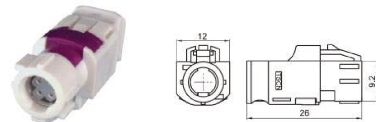
Type: TSVW20-04PF-AT-5WT-1 Material: PA66 GF30% Matching Terminal: TSTF0051 / TSTF0052
