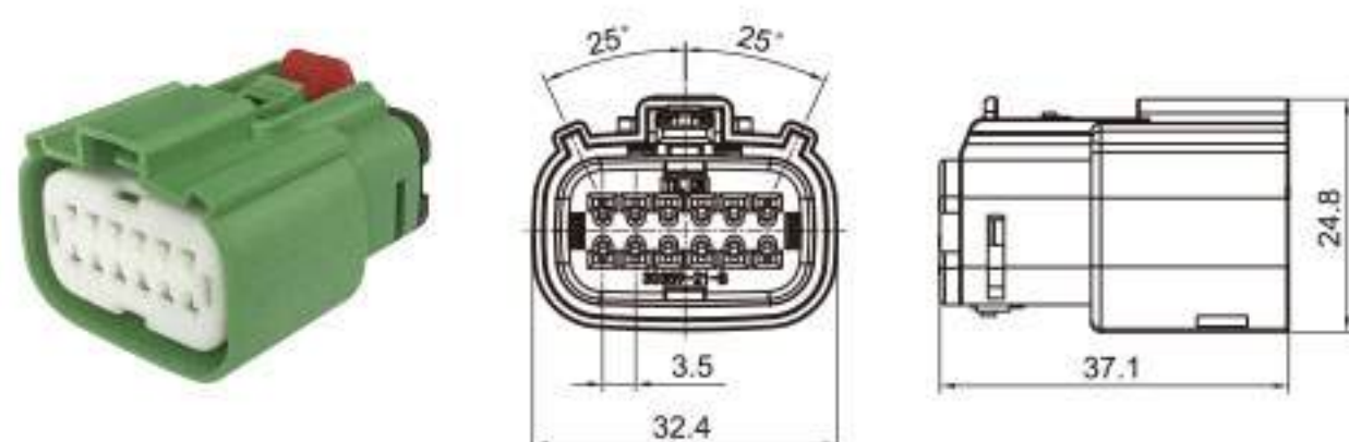
Type: TS30359-12P-21-3 Material: PA66 GF30% Matching Terminal: TSH047
