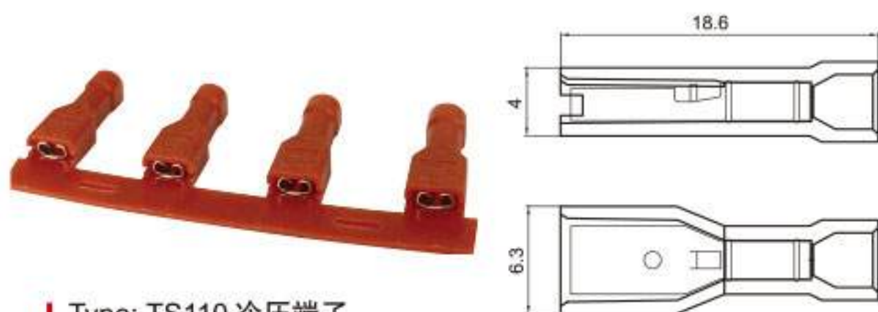
Type: TS110 冷压端子 Material: Brass Applicable Thickness: 0.5~0.8
