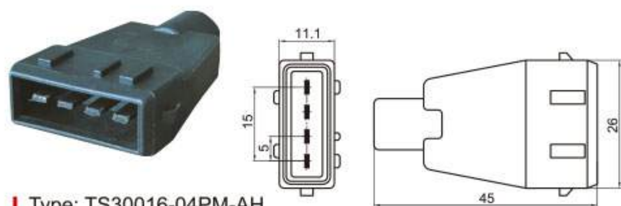
Type: TS30016-04PM-AH Material: ABS Matching Terminal: TSAM0017
