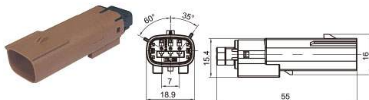
Type: TS30366-03P-11-2 Material: PA66 GF30% Matching Terminal: TSZ144A
