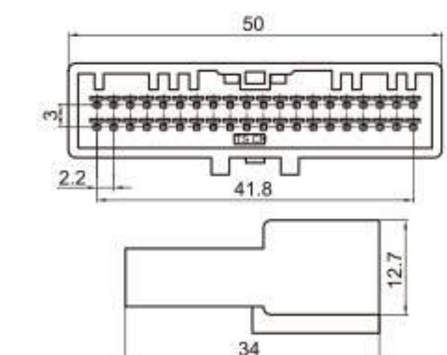
Type: TSTA40-40P-11-3 Material: PA66 Matching Terminal: TSZ208
