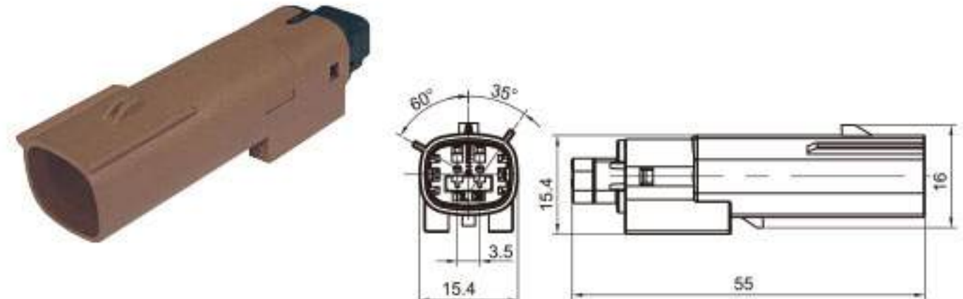
Type: TS30366-02P-11-2 Material: PA66 GF30% Matching Terminal: TSZ144A
