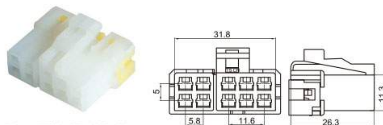
Type: TS1763-10P-21 Material: PA66 Matching Terminal: TSH011
