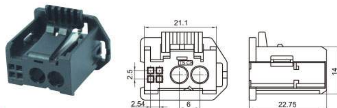
Type: TSBMGQ-06P-21 Material: PA66 GF15% Matching Terminal: TSH092
