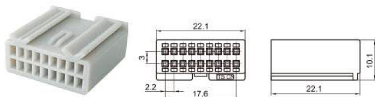
Type: TSCR18-18P-21 Material: PA66 Matching Terminal: TSH143
