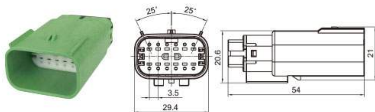
Type: TS30359-12P-11-3 Material: PA66 GF30% Matching Terminal: TSZ144A
