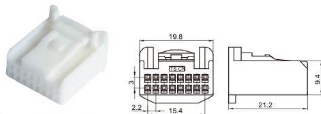
Type: TSTA16-16P-21 Material: PA66 Matching Terminal: TSH143
