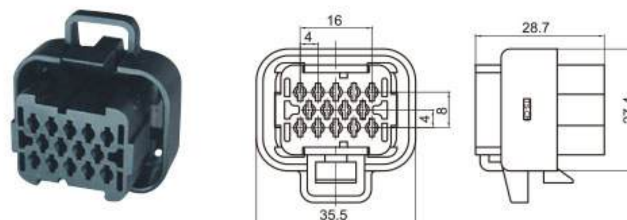
Type: TS3016-14P-21(30256) Material: PA66 Matching Terminal: TSH535
