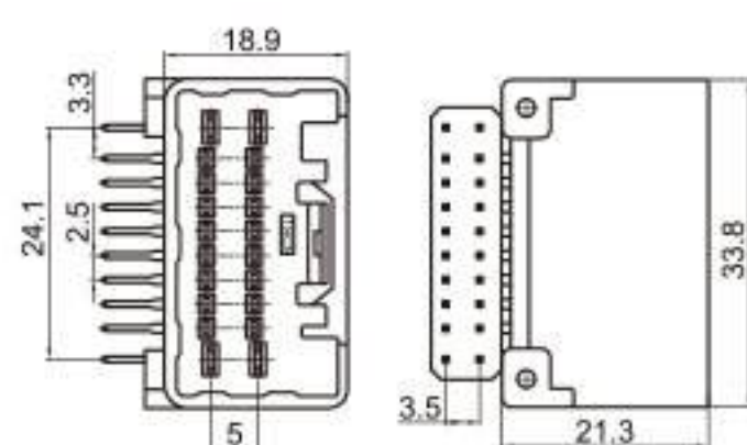
Type: TS7005-20PM-PKB Material: PA66 Matching Terminal: TSPM0001~TSPM0004
