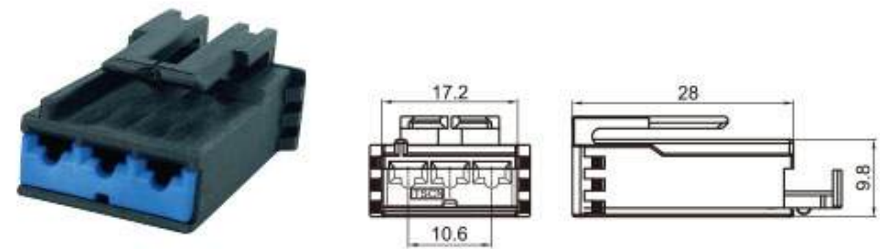
Type: TS30336-03P-21 Material: PA66 GF30% Matching Terminal: TSH085A
