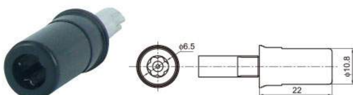
Type: TSCR20-01PF-AT Material: ABS Matching Terminal: TSTF0031 / TSTF0032
