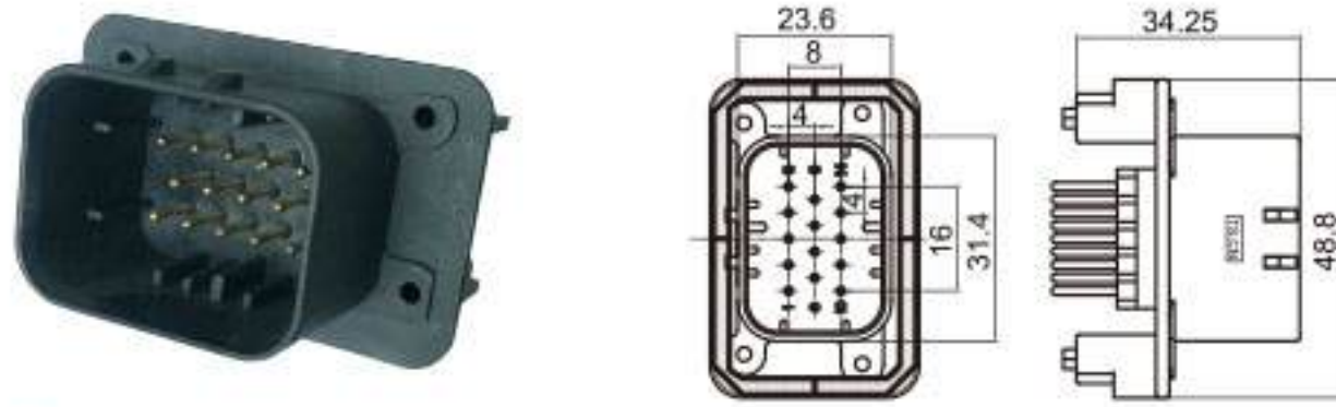
Type: TS30256-14PM-PKS(TS3016) Material: PBT GF30% Matching Terminal: TSPM0304
