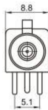
Type: TSVW10-01PM-PKB Material: PBT GF15% Matching Terminal: TSPM0169~TSPM0172
