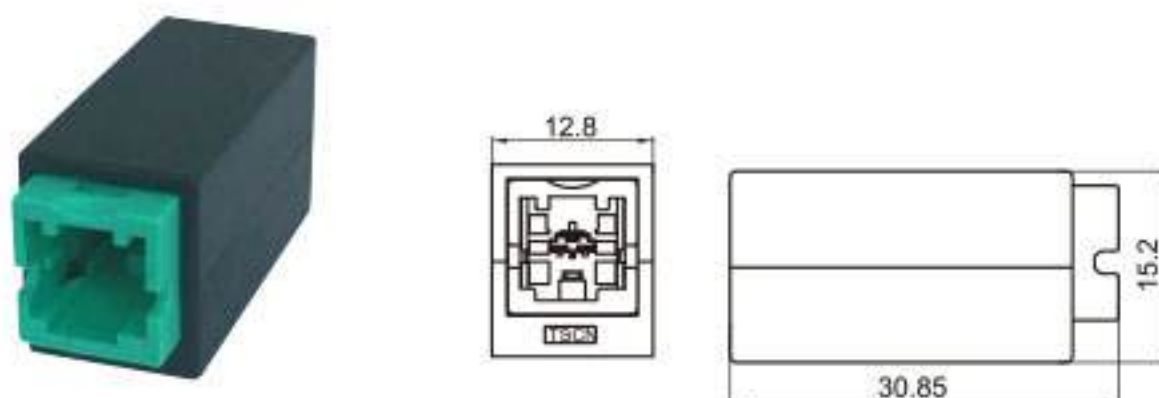
Type: TS30211-02PM-AT-2 Material: PBT GF15% Matching Terminal: TSPM0266~TSPM0269
