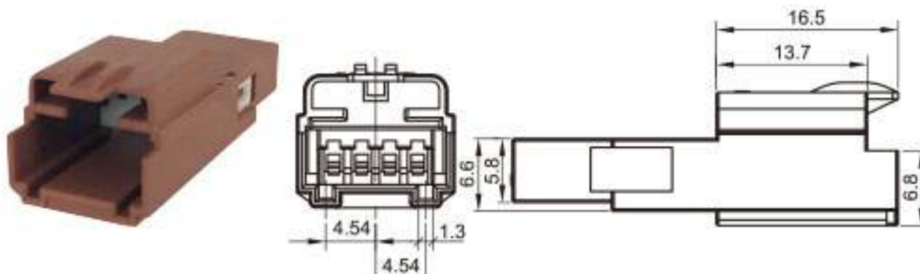
Type: TS30362-04P-11-2 Material: PA66 GF30% Matching Terminal: TSZ145
