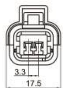
Type: TS30067-02P-21-1 Material: PA66 GF30% Matching Terminal: TSH047
