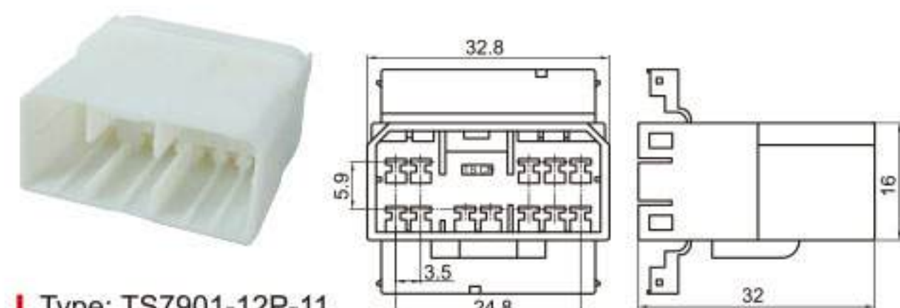
Type: TS7901-12P-11 Material: PA66 Matching Terminal: TSZ011
