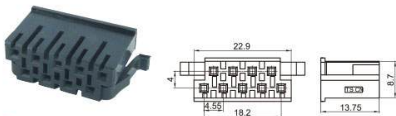
Type: TSJVC09-09P-21 Material: PA66 Matching Terminal: TSH045
