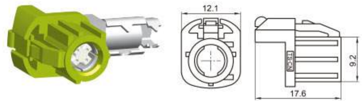
Type: TSVW20-04PF-AT-5YG Material: PA66 GF30% Matching Terminal: TSTF0048 / TSTF0049 / TSTF0050
