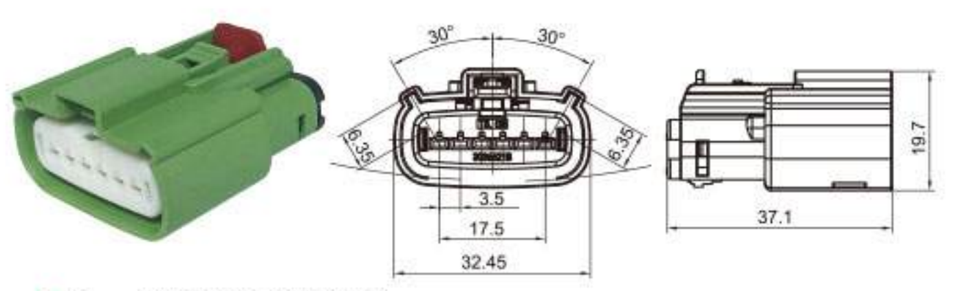
Type: TS30366-06P-21-3 Material: PA66 GF30% Matching Terminal: TSH047
