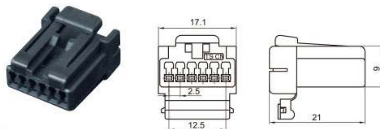
Type: TSHD06-06P-21-1 Material: PA66 Matching Terminal: TSH006
