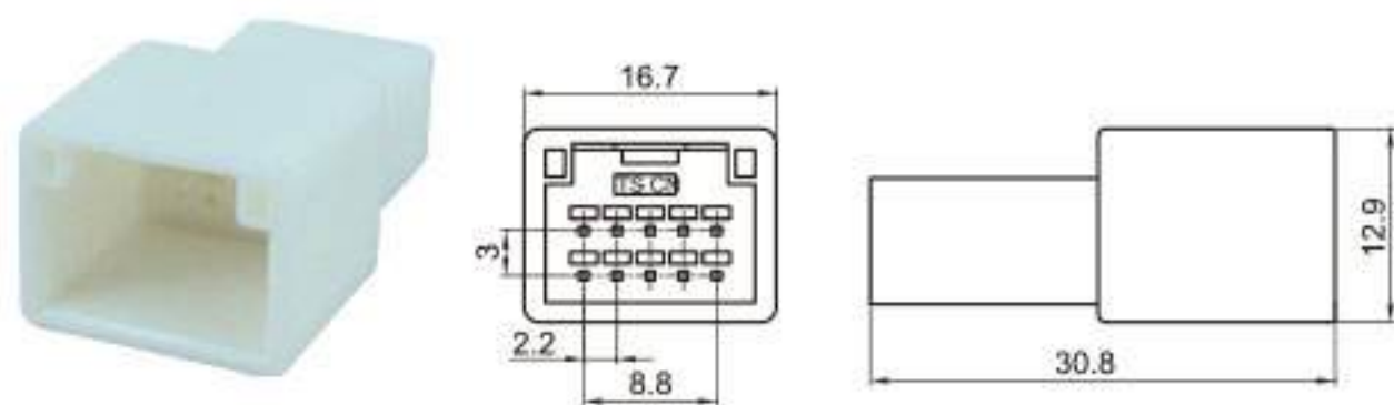
Type: TSTA10-10P-11-1 Material: PA66 Matching Terminal: TSZ208
