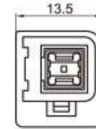
Type: TSFIAT10-01PM-AT-1 Material: PA66 Matching Terminal: TSTF0014/TSTF0015
