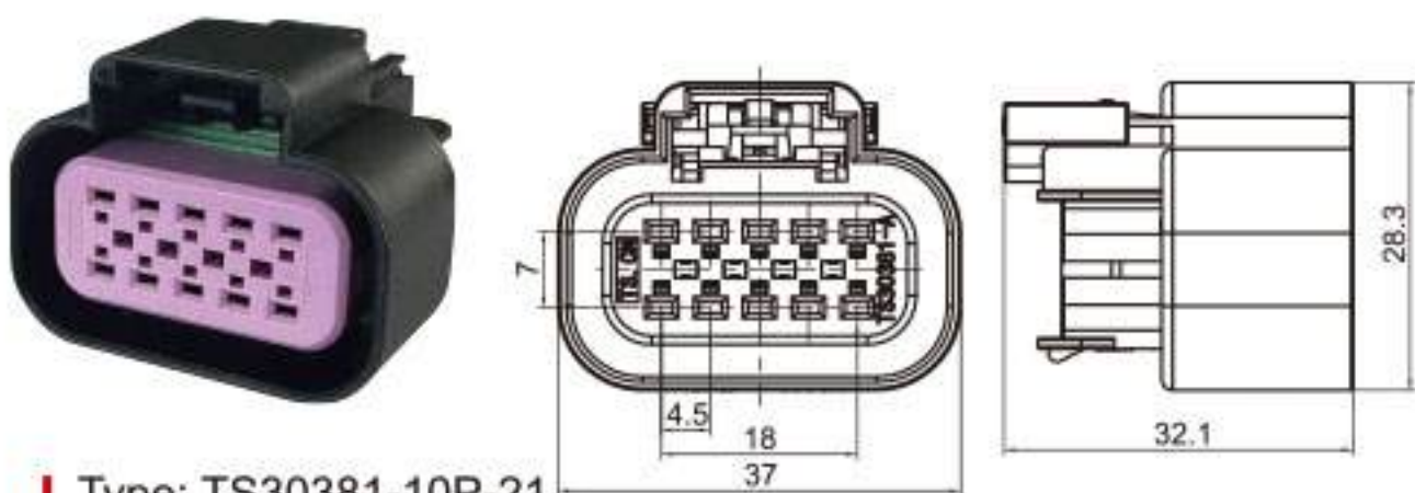
Type: TS30381-10P-21 Material: PA66 GF30% Matching Terminal: TSDJ625-F1.5A
