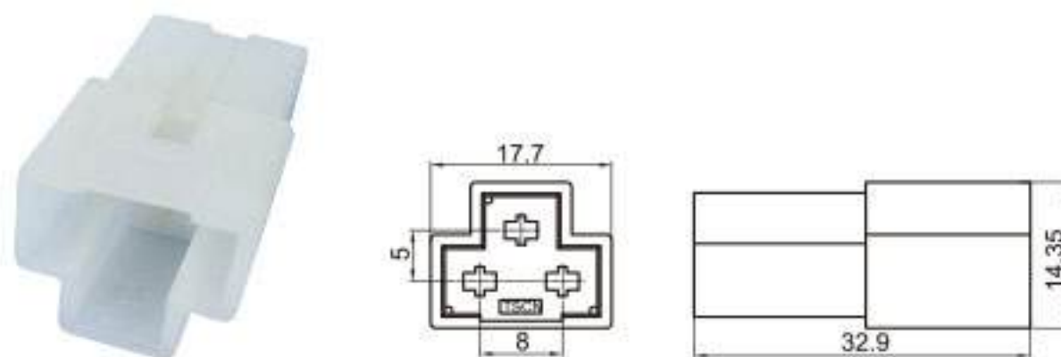
Type: TS30182-03P-11 Material: PA66 Matching Terminal: TSZ024
