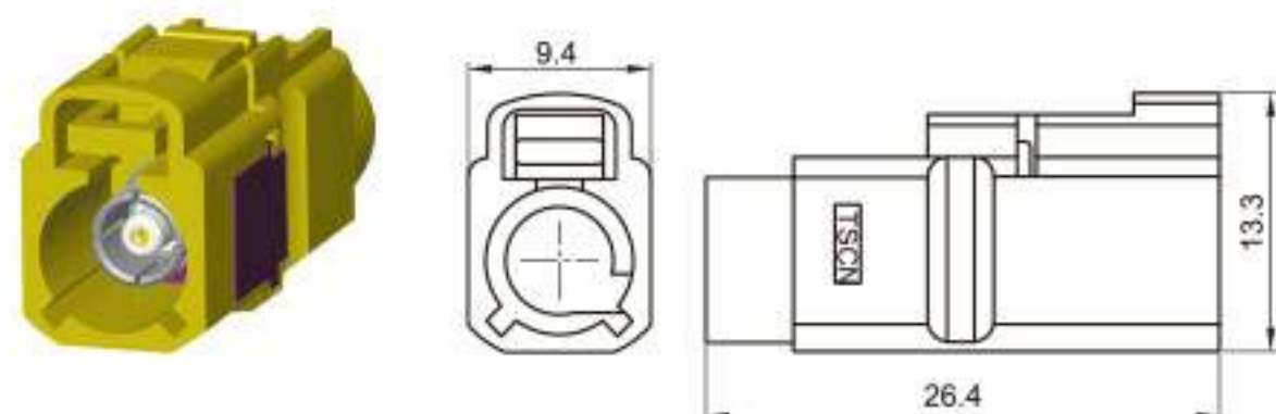
Type: TSVW20-01PF-AT-CU Material: PA66 GF30% Matching Terminal: TSTF0025 / TSTF0026
