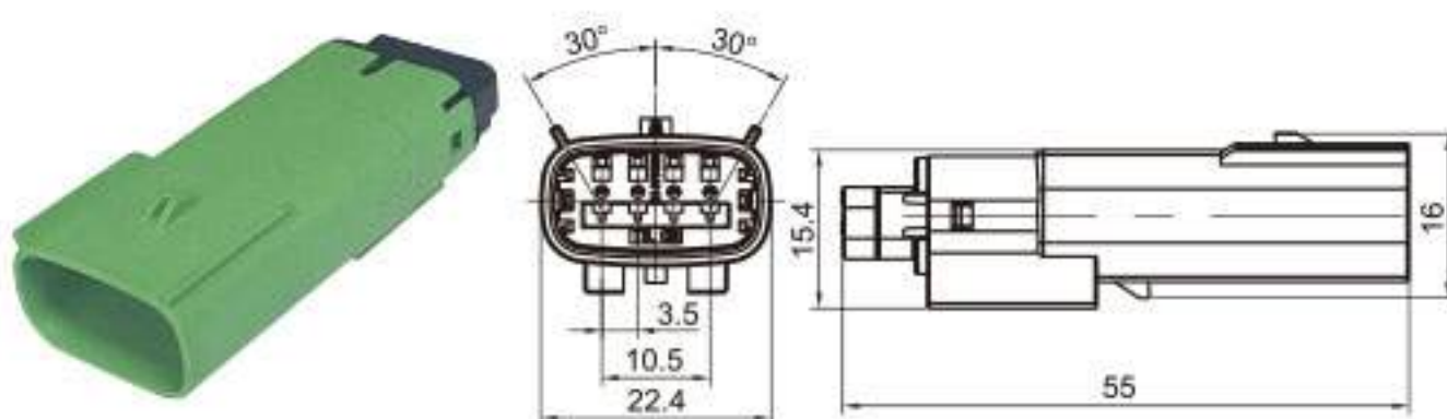
Type: TS30366-04P-11-3 Material: PA66 GF30% Matching Terminal: TSZ144A
