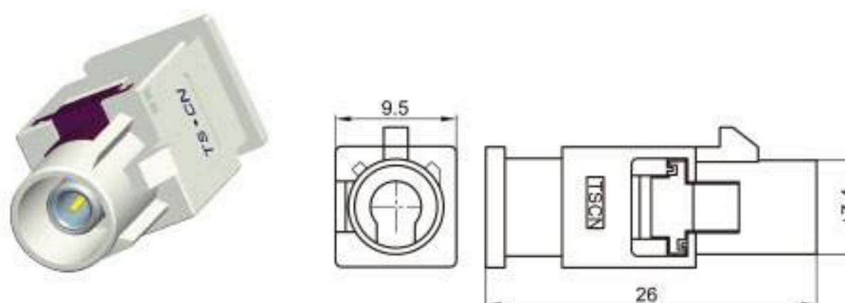
Type: TSVW10-01PM-AT-WT Material: PA66 Matching Terminal: TSTM0019 / TSTM0020
