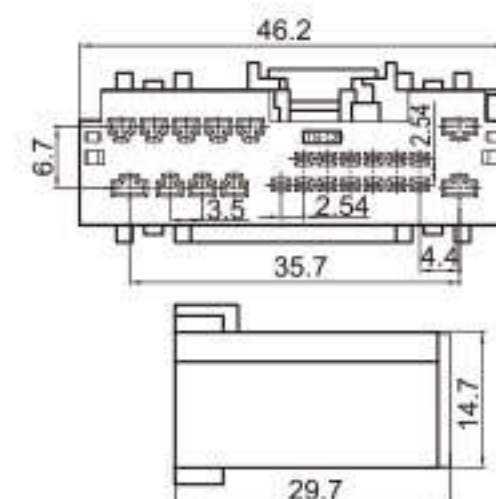
Type: TS5520-24P-11 Material: PA66 GF30% Matching Terminal: TSZ143 / TSZ144 / TSZ145
