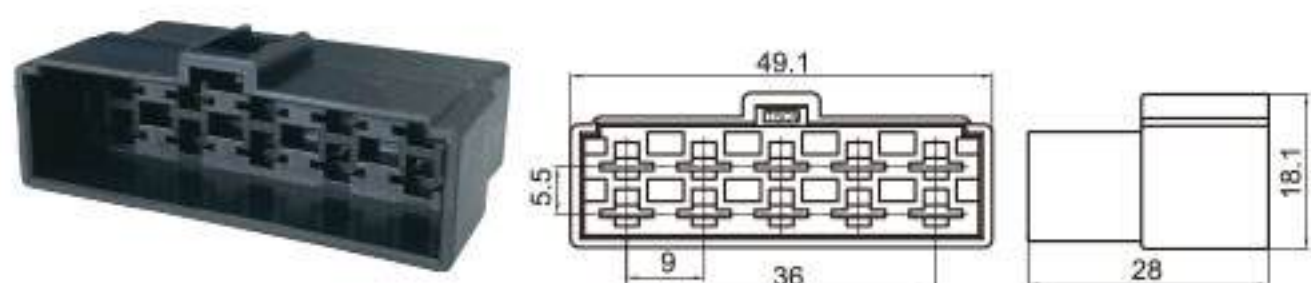
Type: TS30198-10P-11BK Material: PA66 Matching Terminal: TSZ538A
