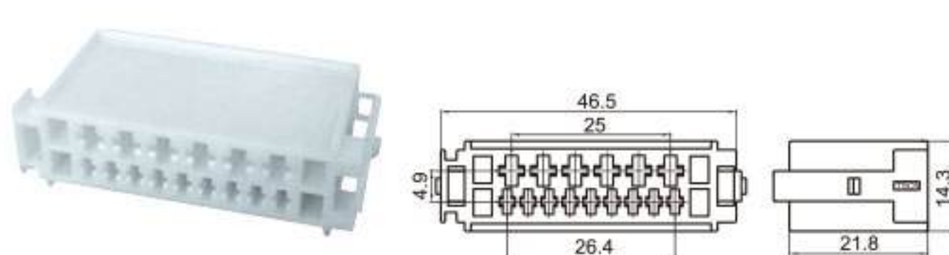
Type: TS30204-15P-21 Material: PA66 Matching Terminal: TSH019 / TSH054
