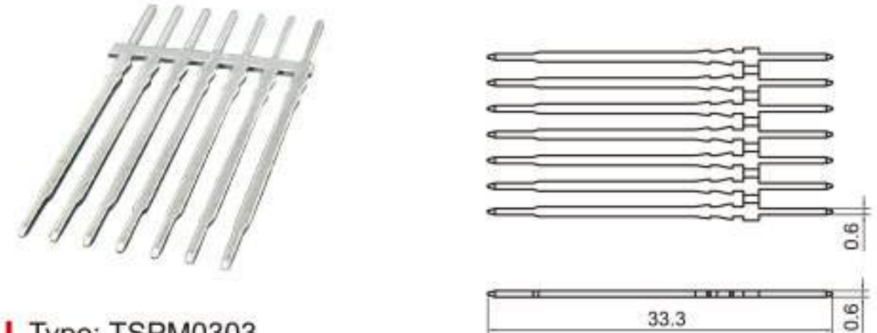
Type: TSPM0303 Material: Brass
