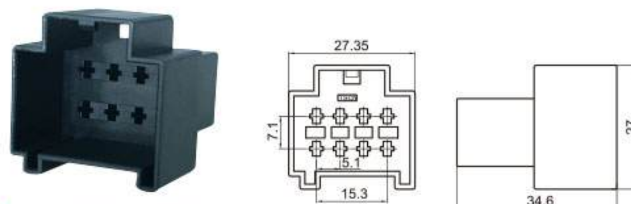
Type: TS30174-08P-11 Material: PA66 Matching Terminal: TSH019
