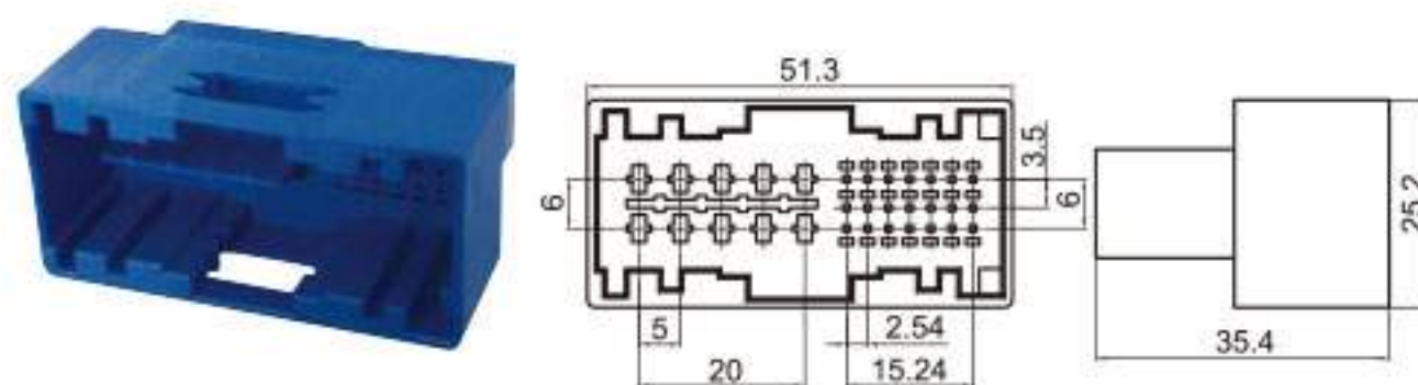
Type: TS30103-31P-11 Material: PBT 3015 Matching Terminal: TSZ024 / TSZ208
