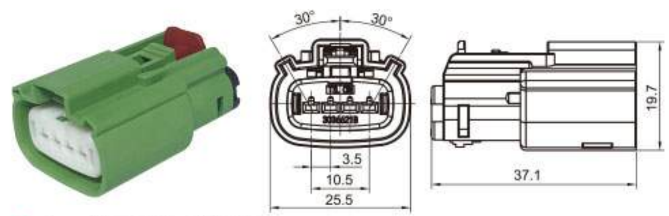
Type: TS30366-04P-21-3 Material: PA66 GF30% Matching Terminal: TSH047
