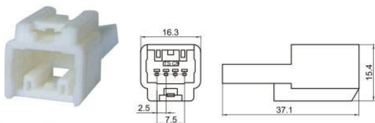
Type: TSTA04-04P-11-2 Material: PA66 Matching Terminal: TSZ208
