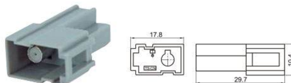
Type: TSHD11-02PM-AT-1 Material: PA66 Matching Terminal: TSZ208B / TSTM0007 / TSTF0004
