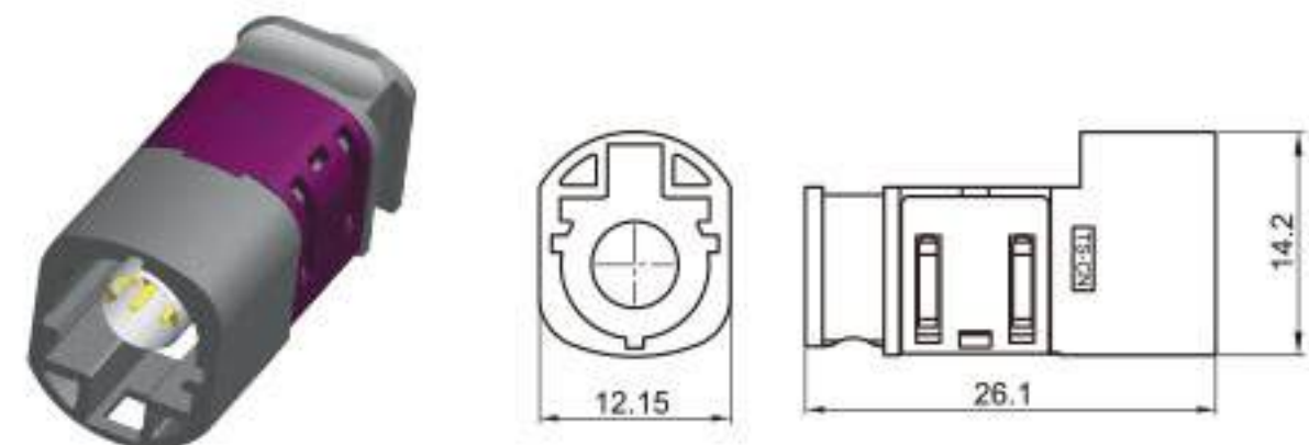
Type: TSVW10-04PM-AT-5GY-1 Material: PA66 GF15% Matching Terminal: TSPM0175 / TSTM0051
