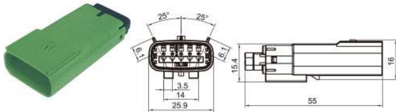
Type: TS30366-05P-11-3 Material: PA66 GF30% Matching Terminal: TSZ144A
