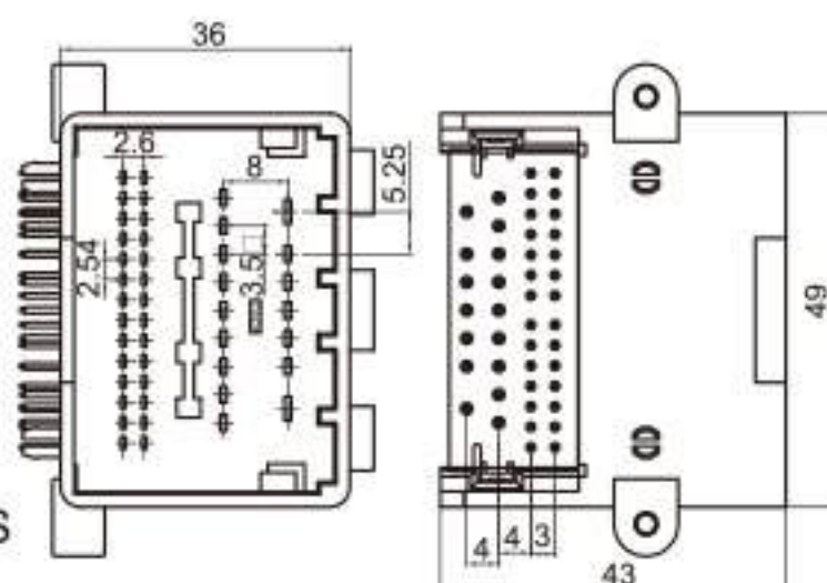
Type: TSKL44-44PM-PKS Material: PA66 GF30% Matching Terminal: NIL
