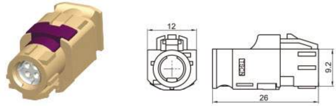
Type: TSVW20-04PF-AT-5BE-1 Material: PA66 GF30% Matching Terminal: TSTF0051 / TSTF0052
