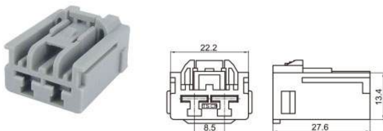
Type: TSVO02-02P-21 Material: PA66 Matching Terminal: TSH033B
