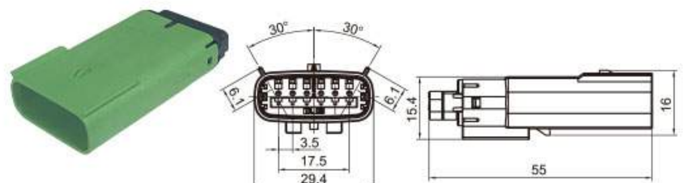
Type: TS30366-06P-11-3 Material: PA66 GF30% Matching Terminal: TSZ144A
