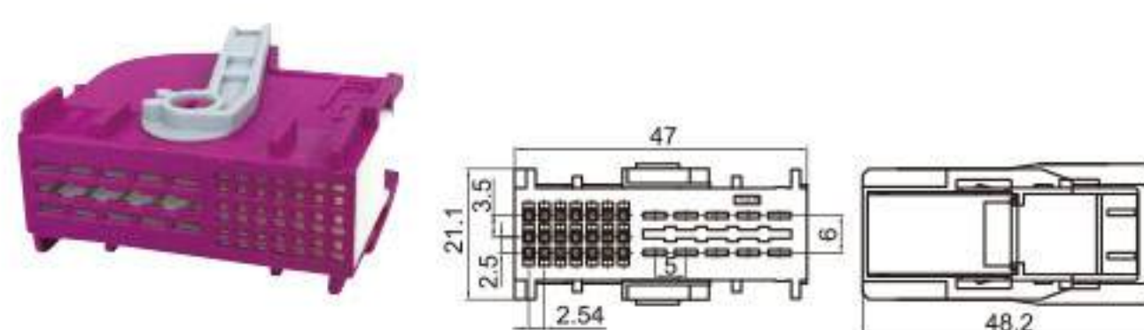
Type: TS30104-31P-21 Material: PBT GF15% Matching Terminal: TSH019 / TSH143
