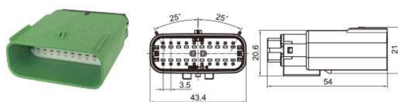
Type: TS30359-20P-11-3 Material: PA66 GF30% Matching Terminal: TSZ144A
