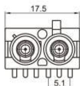
Type: TSVW10-02PM-AT-3 Material: PBT GF15% Matching Terminal: TSPM0169 / TSPM0172
