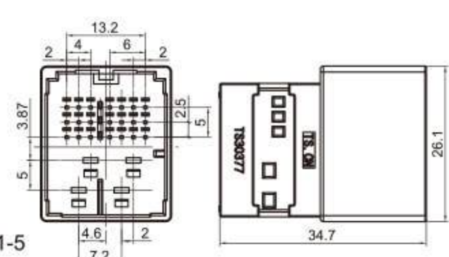
Type: TS30377-25P-21-4 Material: PA66 Matching Terminal: TSH019C / TSH606
