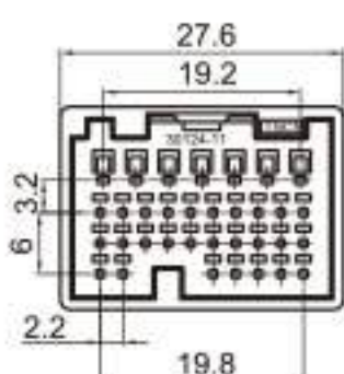
Type: TS30124-34P-11 Material: PA66 Matching Terminal: TSZ145 / TSZ208
