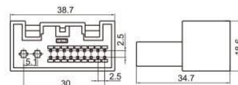
Type: TS30167-20P-11 Material: PA66 GF30% Matching Terminal: TSZ024 / TSZ208B
