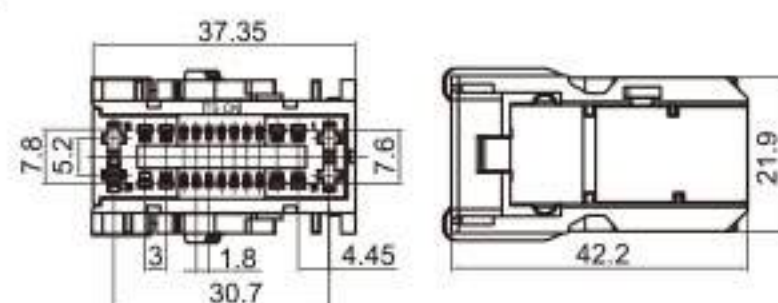
Type: TS30279-26P-21 Material: PA66 Matching Terminal: TSH019 / TSH593 / TSH606
