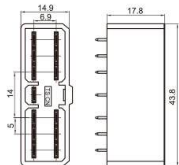
Type: TS1692-13PM-PKB Material: PA66 Matching Terminal: NIL
