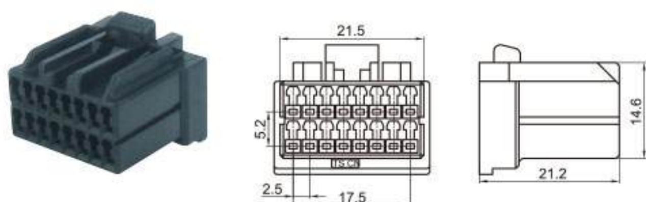
Type: TSHD16-16P-21-2 Material: PA66 Matching Terminal: TSH006
