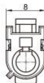
Type: TS1068-01PF-AT-1 Material: PA66 Matching Terminal: TSTF0003 / TSTF0004
