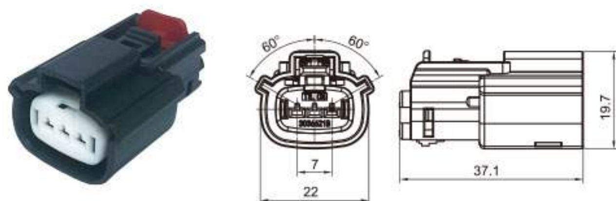
Type: TS30366-03P-21 Material: PA66 GF30% Matching Terminal: TSH047
