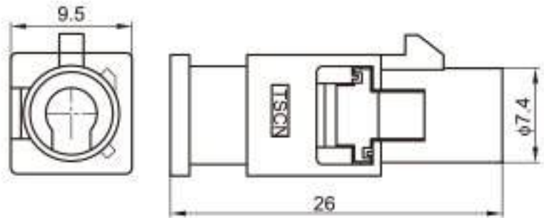
Type: TSVW10-01PM-AT-PK Material: PA66 Matching Terminal: TSTM0019 / TSTM0020
