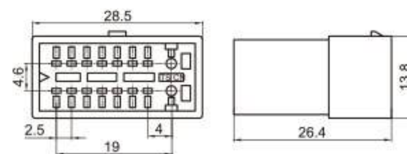
Type: TSCLR16-16P-11 Material: PA66 GF30% Matching Terminal: TSZ032 / TSZ007B
