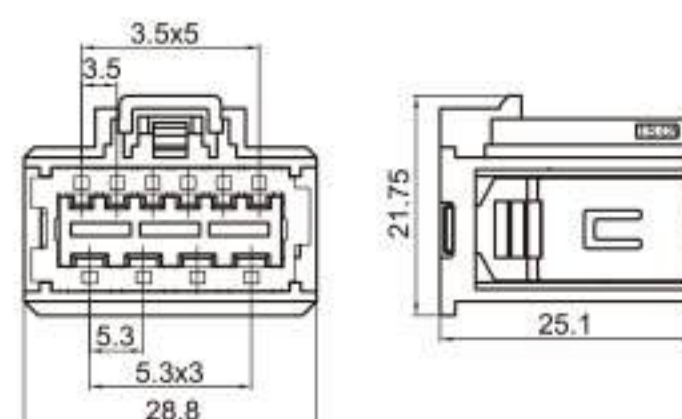
Type: TS30039-10P-21 Material: PA66 GF30% Matching Terminal: TSH085 / TSH047
