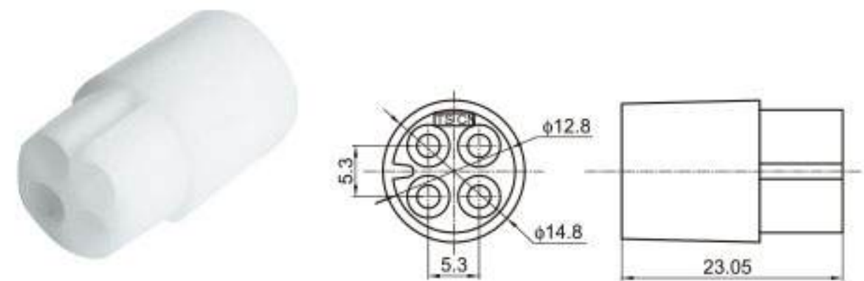
Type: TSLB20-04P-21 Material: PA66 Matching Terminal: NIL
