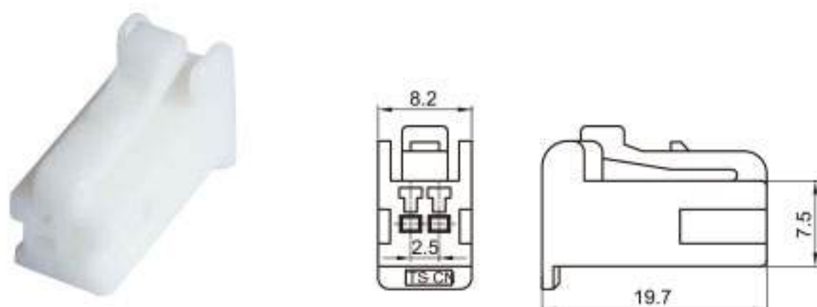
Type: TSLB18-02P-21 Material: PA66 Matching Terminal: NIL
