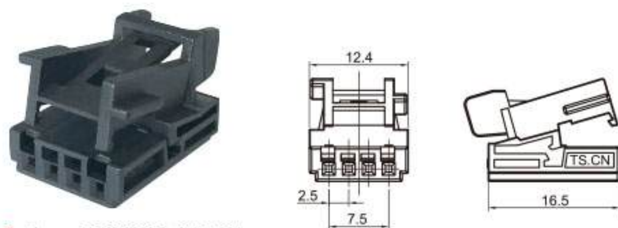
Type: TS30292-04P-21 Material: PA66 GF30% Matching Terminal: TSH624
