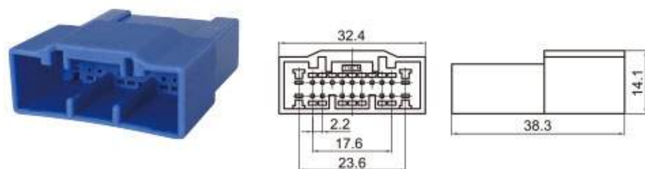
Type: TS30118-20P-11BL Material: PA66 Matching Terminal: TSZ144 / TSZ208
