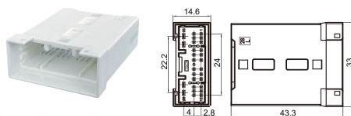
Type: TS30101-28PM-PKS-5 Material: PBT GF15% Matching Terminal: TSPM0331 / TSPM0305
