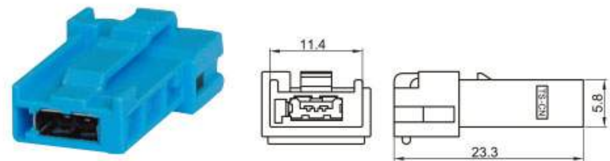
Type: TSKC3123-02PF-AT-1 Material: PA66 GF30% Matching Terminal: TSTF0022 / TSTM0006
