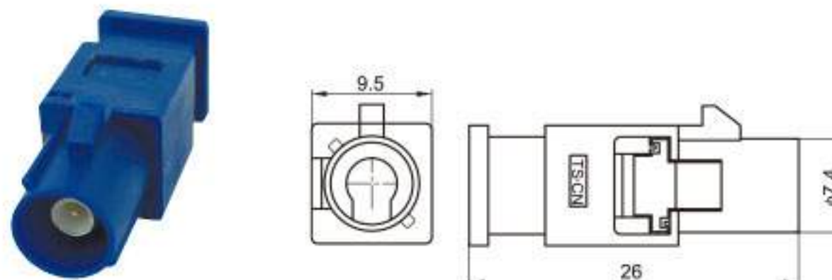
Type: TSVW10-01PM-AT-BL Material: PA66 Matching Terminal: TSTM0019 / TSTM0020
