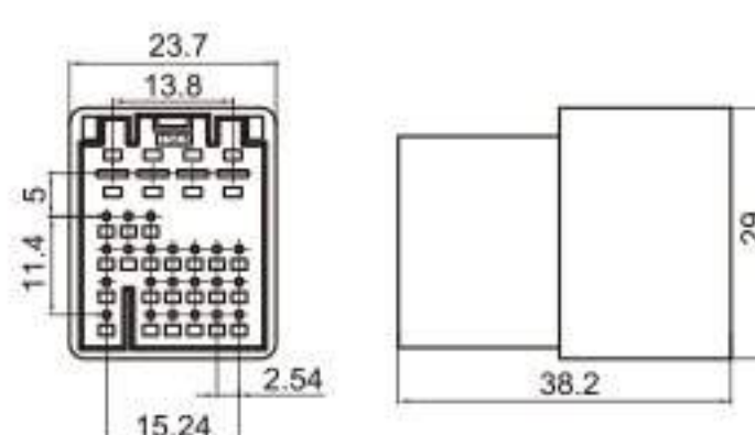
Type: TS30217-30P-11-4 Material: PBT GF15% Matching Terminal: TSDJ615B-2.8*0.8B / TSZ208
