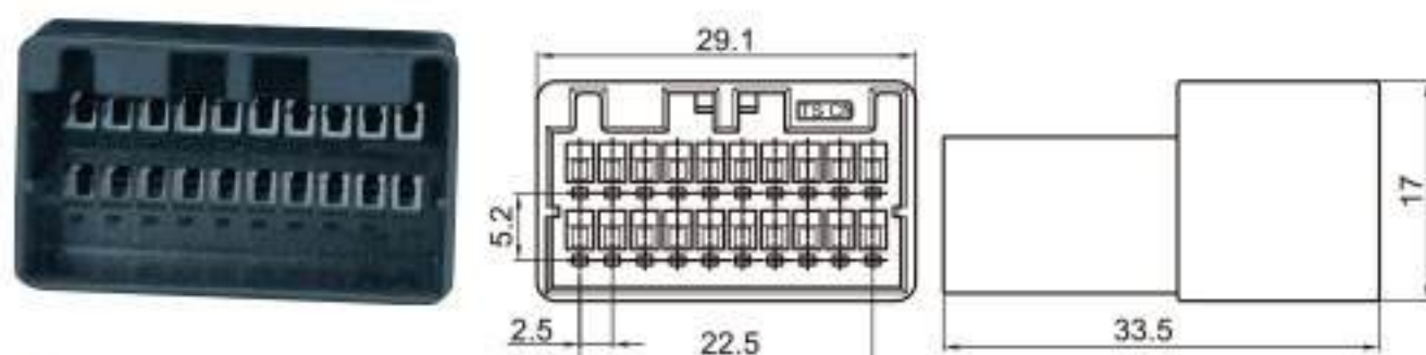
Type: TSHD20-20P-11-5 Material: PA66 Matching Terminal: TSZ145
