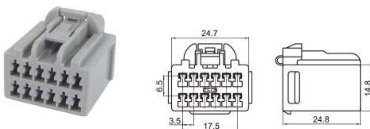
Type: TSVO12-12P-21 Material: PA66 Matching Terminal: TSH047
