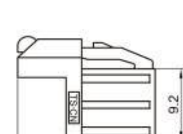
Type: TSVW20-04PF-AT-5GN Material: PA66 GF30% Matching Terminal: TSTF0048 / TSTF0049 / TSTF0050
