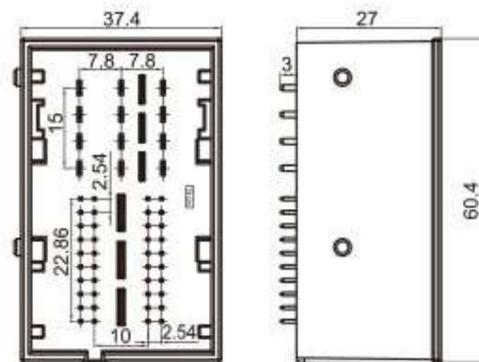
Type: TS6523-52PM-PKS Material: PA66 Matching Terminal: NIL
