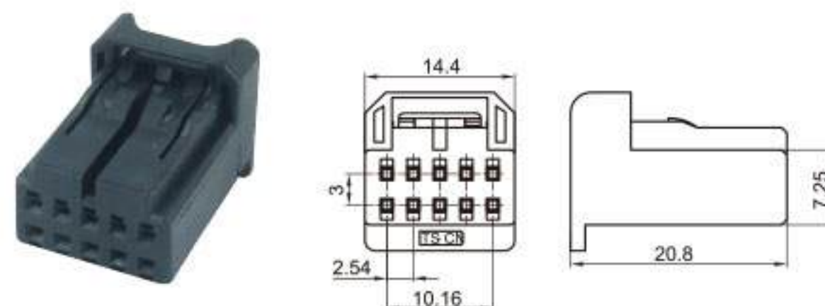
Type: TSNITL-10P-21 Material: PA66 Matching Terminal: TSH143
