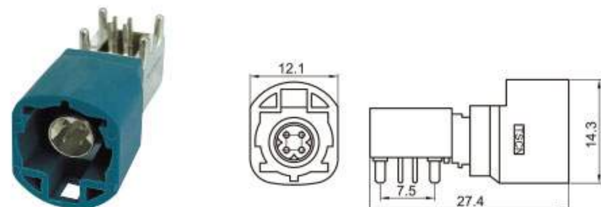
Type: TSVW10-04PM-AT-5WB Material: PA66 GF30% Matching Terminal: TSPM0021~TSPM0025
