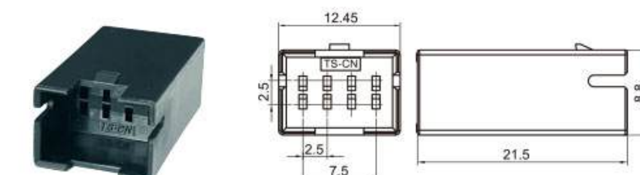
Type: TSPHC-08P-11 Material: PA66 Matching Terminal: TS25044-RT
