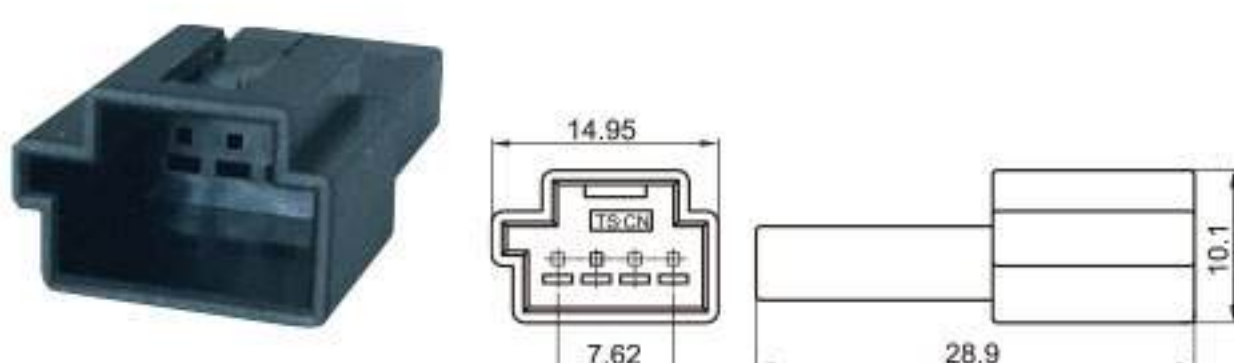
Type: TS30171-04P-11 Material: PA66 Matching Terminal: TSZ208B
