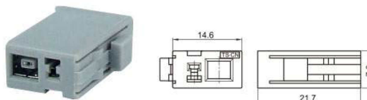
Type: TSHD20-02PF-AT Material: PA66 Matching Terminal: TSH009 / TSTF0001 / TSTF0002
