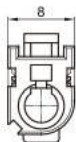
Type: TS1068-01PF-AT Material: PA66 Matching Terminal: TSTF0003 / TSTF0004
