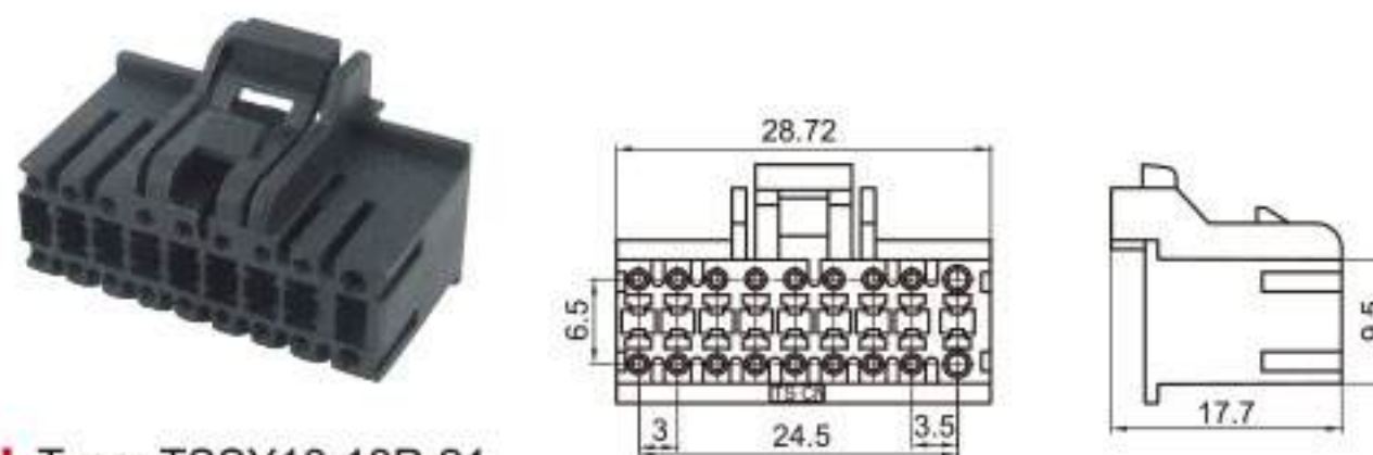
Type: TSSY18-18P-21 Material: PA66 Matching Terminal: TSH031
