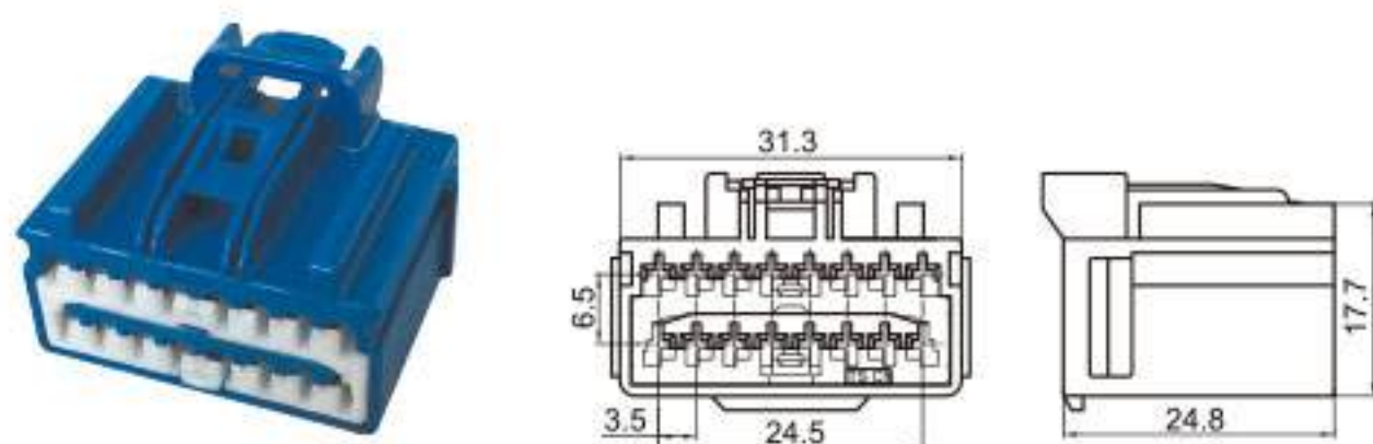
Type: TSVO16-16P-21-2 Material: PBT GF10% Matching Terminal: TSH047
