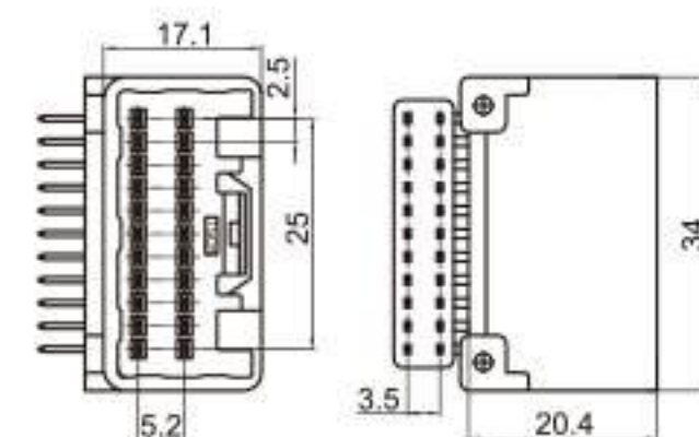
Type: TSMI22-22PM-PKB Material: PA66 Matching Terminal: TSPM0001 / TSPM0003
