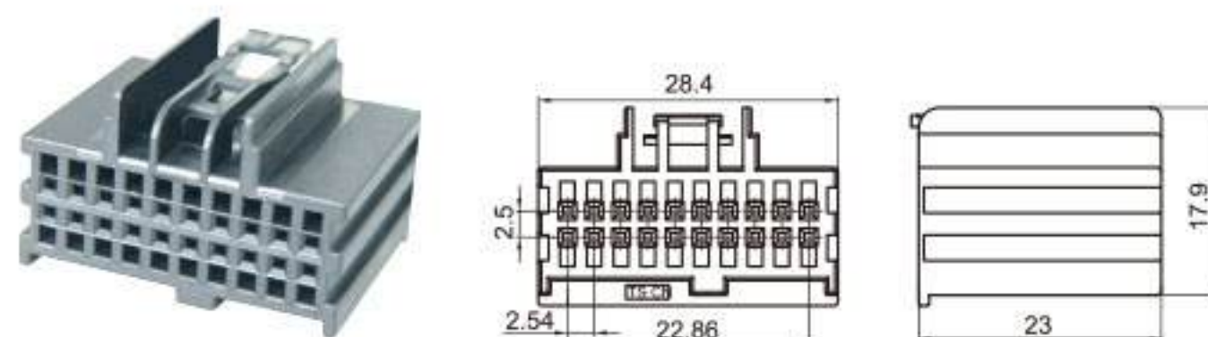
Type: TSGM20-20P-21-1 Material: PA66 GF30% Matching Terminal: TSH143
