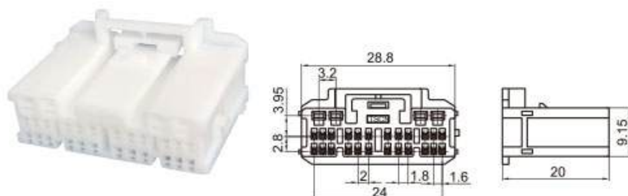
Type: TS30101-28P-21-1 Material: PA66 Matching Terminal: TSH593 / TSH600
