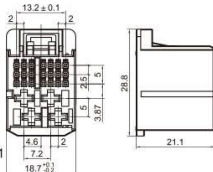
Type: TS30377-25P-11-1 Material: PA66 Matching Terminal: TSZ550 / TSZ561A
