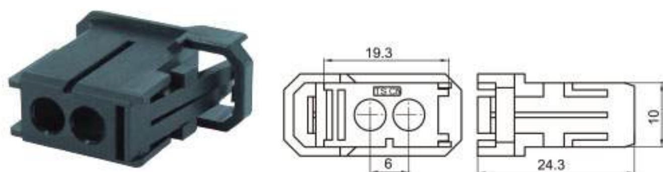
Type: TSBMGQ-02P-21 Material: PA66 Matching Terminal: NIL
