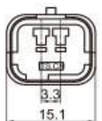
Type: TS30067-02P-11-1 Material: PA66 GF30% Matching Terminal: TSZ144
