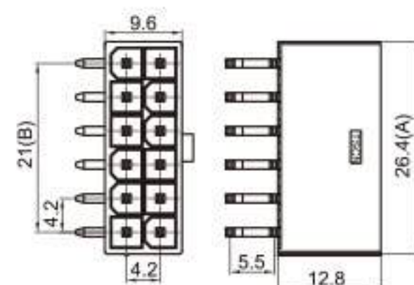
Type: TS5557-12PM-PKB(02P-24P) Material: PA66 Matching Terminal: TSPM0311 / TSPM3012
