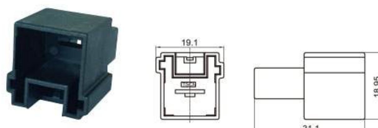
Type: TS30144-01P-11 Material: PA66 Matching Terminal: TSZ611
