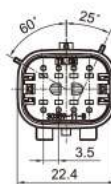
Type: TS30359-08P-11-2 Material: PA66 GF30% Matching Terminal: TSZ144A
