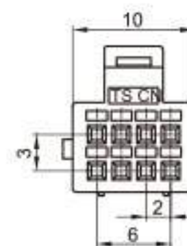
Type: TSHY66-08P-21BL Material: PA66 Matching Terminal: TSHY66
