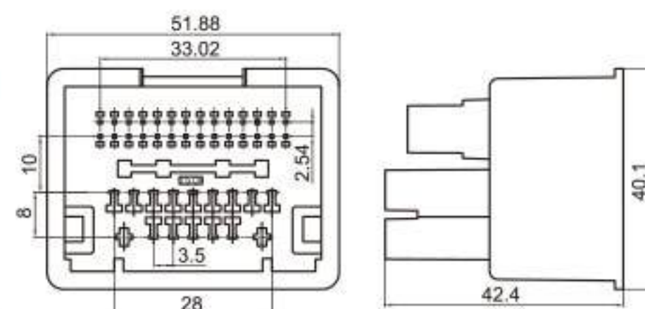
Type: TSKL44-44P-11 Material: PA66 GF30% Matching Terminal: TSZ024 / TSZ144 / TSZ208B
