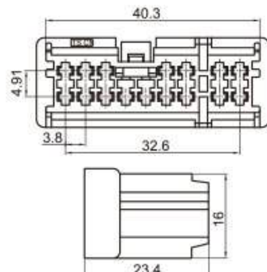
Type: TS7301A-16P-21-2 Material: PA66 Matching Terminal: TSH009
