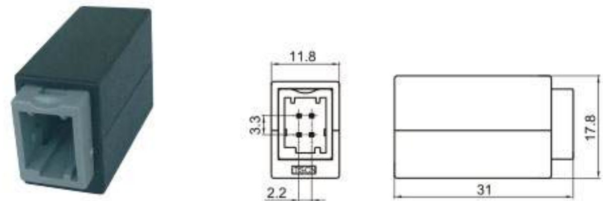
Type: TS30213-04PM-AT Material: PBT GF15% Matching Terminal: TSPM0270~TSPM0274
