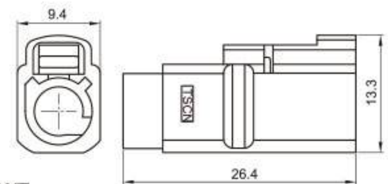
Type: TSVW20-01PF-AT-WT Material: PA66 GF30% Matching Terminal: TSTF0025 / TSTF0026
