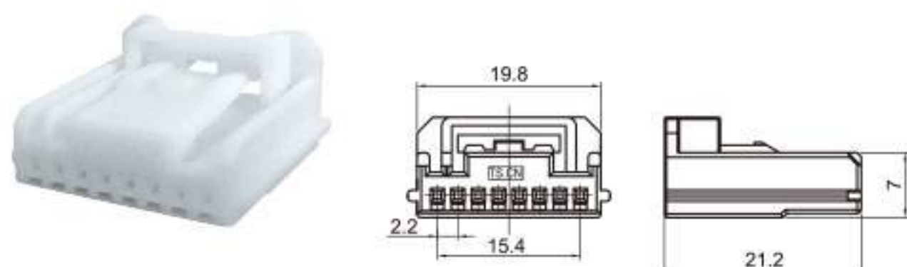
Type: TS30291-08P-21 Material: PA66 Matching Terminal: TSH143
