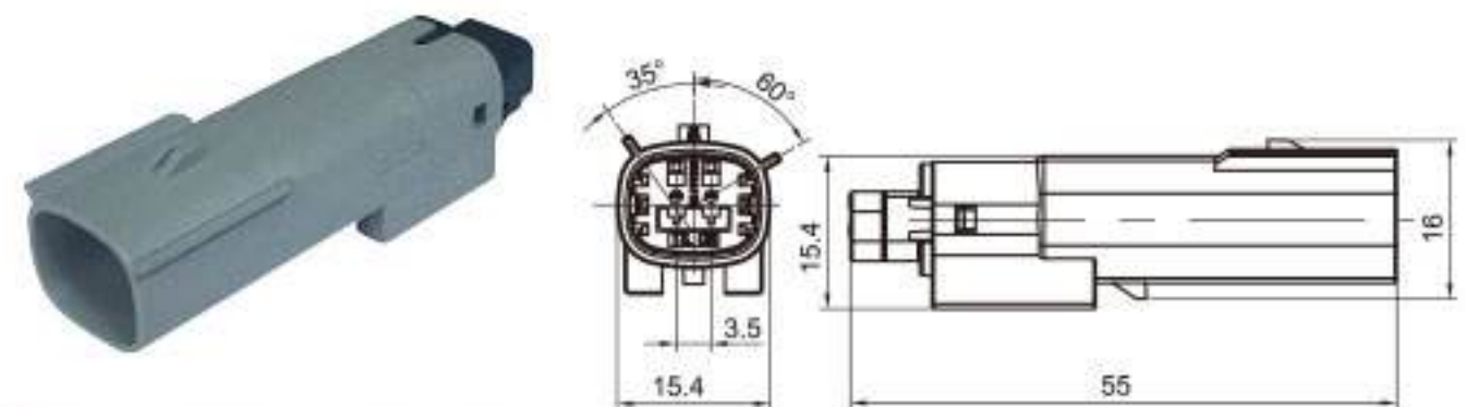
Type: TS30366-02P-11-1 Material: PA66 GF30% Matching Terminal: TSZ144A
