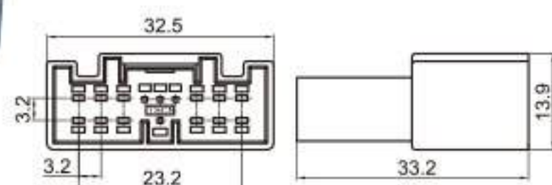
Type: TS30161-16P-11 Material: PA66 GF30% Matching Terminal: TSZ040 / TSZ208
