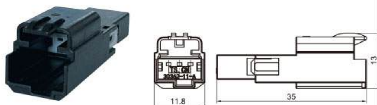
Type: TS30362-03P-11 Material: PA66 GF30% Matching Terminal: TSZ145
