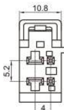
Type: TS30148-04P-21BK Material: PBT Matching Terminal: TSH091 / TSH092
