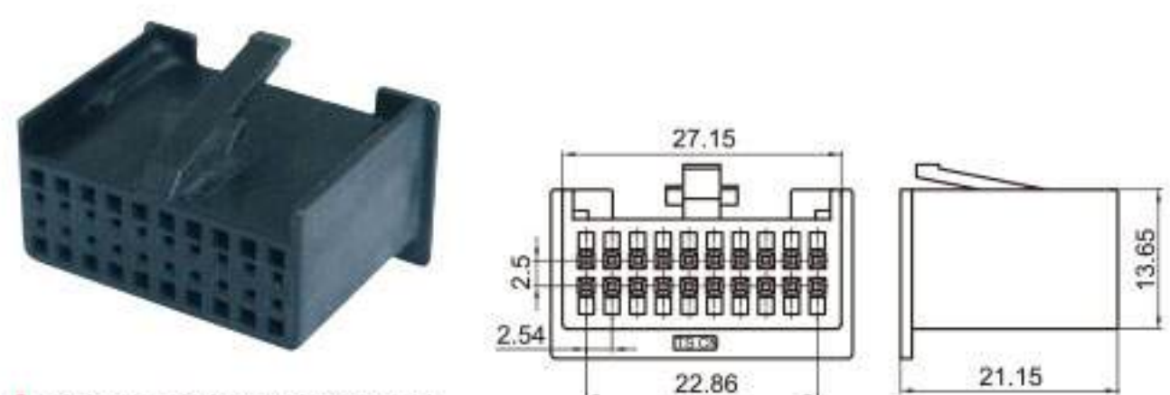
Type: TSGM20-20P-21 Material: PA66 GF30% Matching Terminal: TSH143
