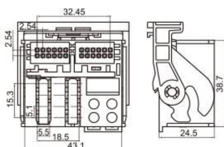
Type: TS9003-40P-11-1 Material: PA66 GF30% Matching Terminal: TSZ054B / TSZ208B
