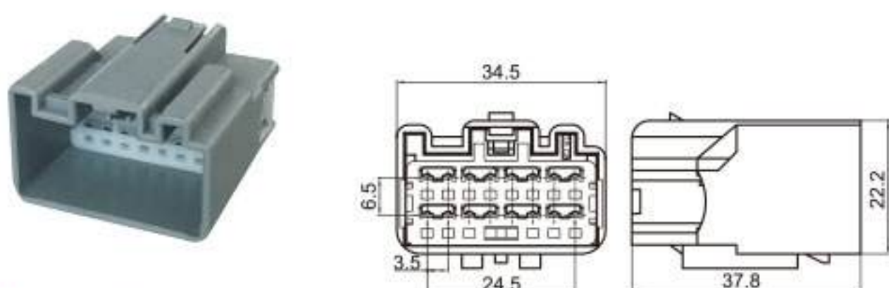
Type: TSVO16-16P-11-3 Material: PBT GF10% Matching Terminal: TSZ144
