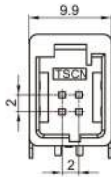
Type: TSMA04-04PM-PKS-2 Material: PA66 GF30% Matching Terminal: TSPM0030 / TSPM0029
