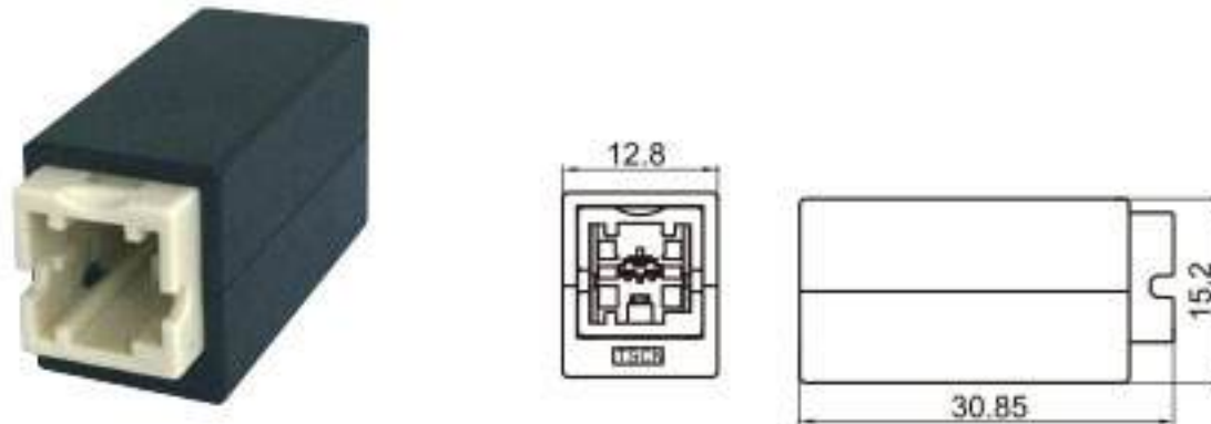
Type: TS30211-02PM-AT Material: PBT GF15% Matching Terminal: TSPM0269
