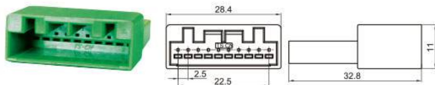
Type: TSHD10-10P-11 Material: PA66 Matching Terminal: TSZ208B
