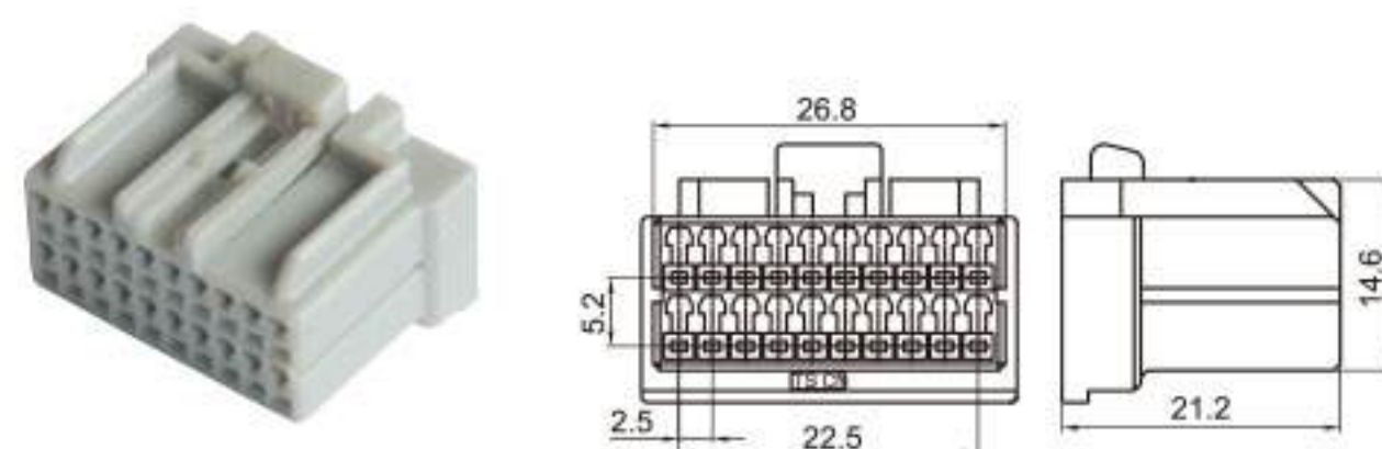
Type: TSHD20-20P-21-3 Material: PA66 Matching Terminal: TSH006
