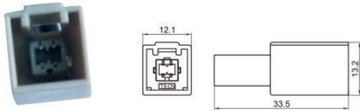
Type: TSTA04-04PM-AT Material: PA66 GF30% Matching Terminal: TSTM0008-A / TSPM0218
