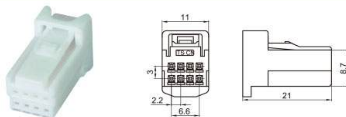
Type: TSTA08-08P-21-2 Material: PA66 Matching Terminal: TSH143
