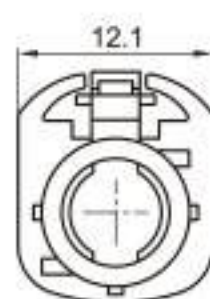
Type: TSVW20-04PF-AT-5BL Material: PA66 GF30% Matching Terminal: TSTF0048 / TSTF0049 / TSTF0050
