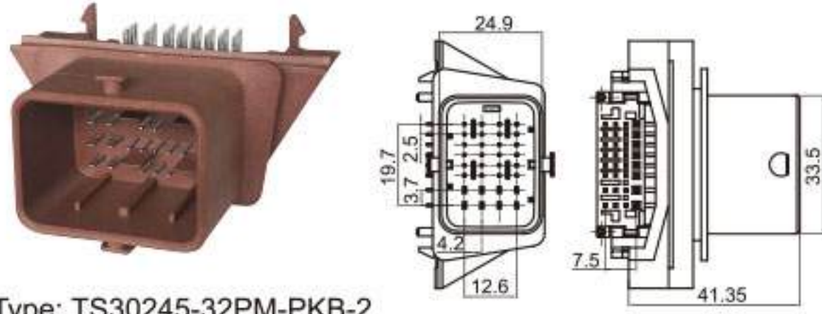
Type: TS30245-32PM-PKB-2 Material: GF30% PBT Matching Terminal: TSPM0289~TSPM0296
