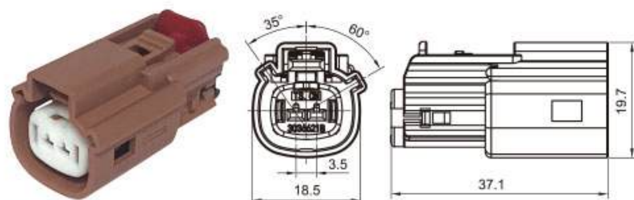
Type: TS30366-02P-21-2 Material: PA66 GF30% Matching Terminal: TSH047
