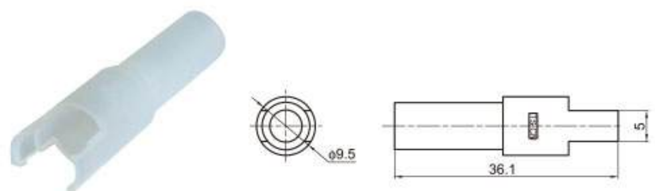
Type: TSLB24-01P-11 Material: PA66 Matching Terminal: NIL
