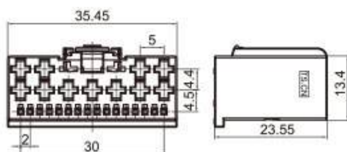
Type: TS30299-27P-21 Material: PA66 Matching Terminal: TS1241390-1 / TSHY66
