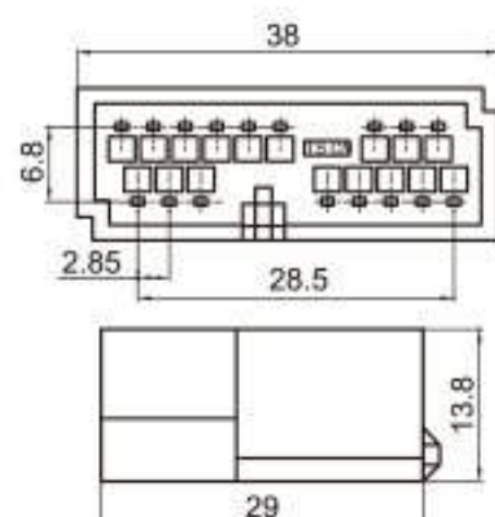
Type: TSFD17-17P-11 Material: PA66 Matching Terminal: TSZ018
