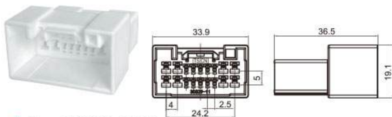
Type: TS30329-18P-11 Material: PBT Matching Terminal: TSZ003 / TSZ018
