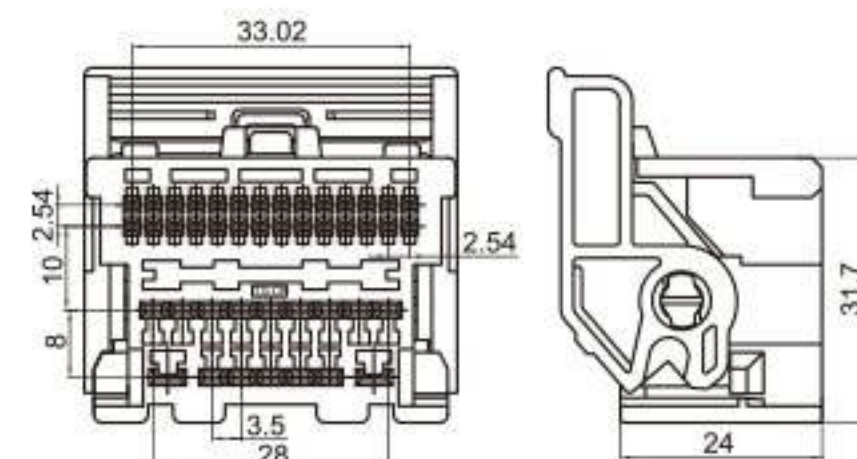
Type: TSKL44-44P-21 Material: PA66 GF30% Matching Terminal: TSH085 / TSH008 / TSH143
