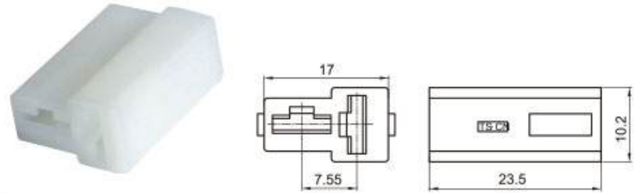
Type: TSLB05-02P-21 Material: PA66 Matching Terminal: TSH033
