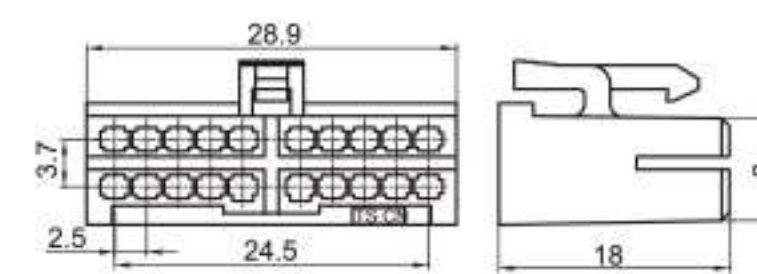
Type: TSJEN-20P-21-1 Material: PA66 GF15% Matching Terminal: TSH034 / TSH060
