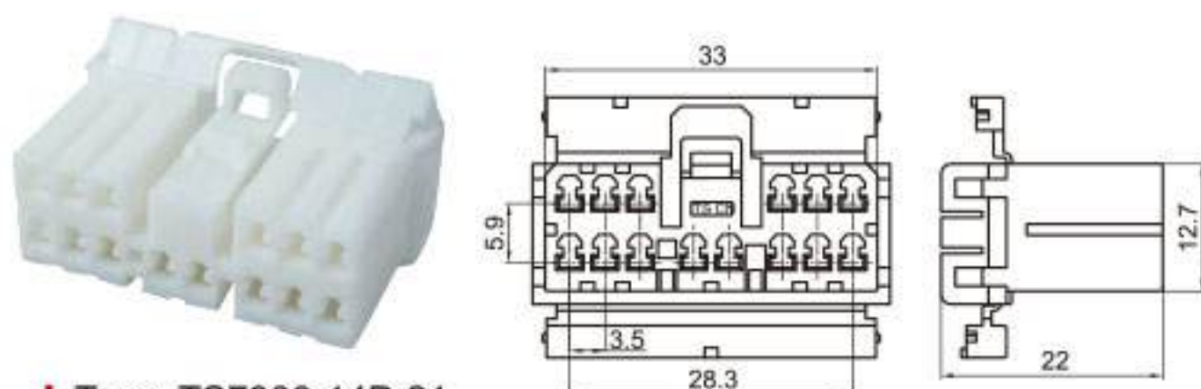
Type: TS7300-14P-21 Material: PA66 Matching Terminal: TSH016
