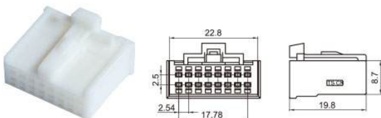
Type: TSPAN16-16P-21-1 Material: PA66 Matching Terminal: TSH053
