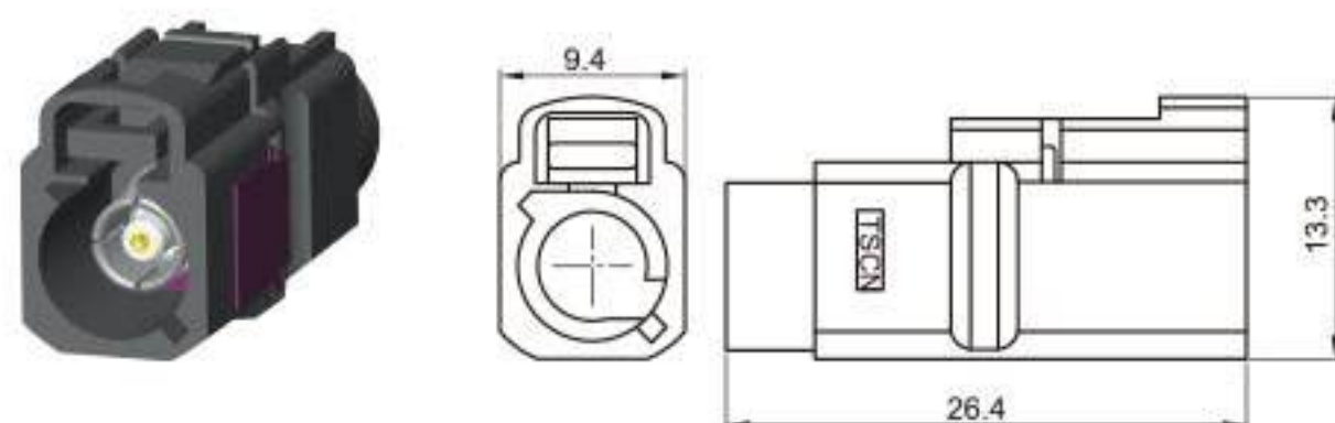
Type: TSVW20-01PF-AT-GY Material: PA66 GF30% Matching Terminal: TSTF0025 / TSTF0026
