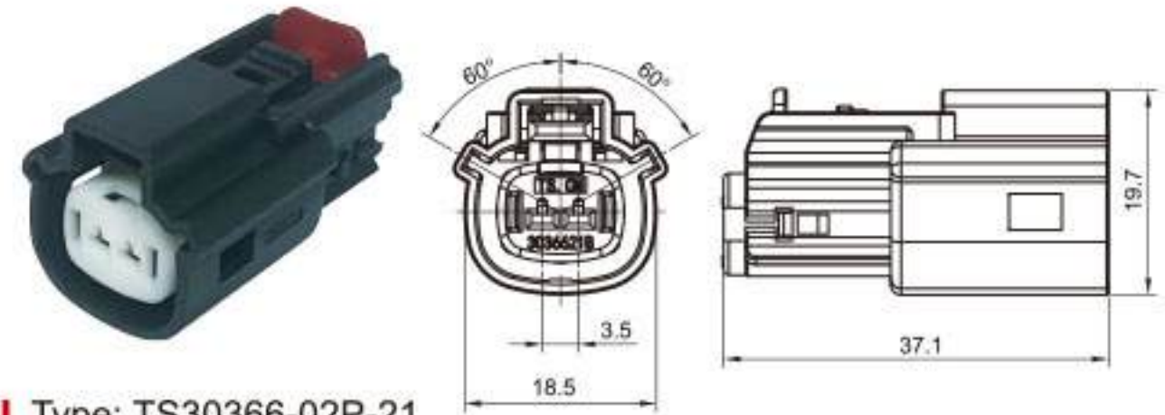
Type: TS30366-02P-21 Material: PA66 GF30% Matching Terminal: TSH047
