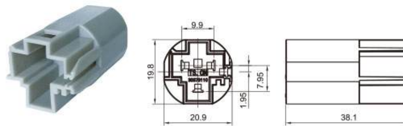
Type: TS30373-03P-11 Material: PA66 Matching Terminal: TSZ054A
