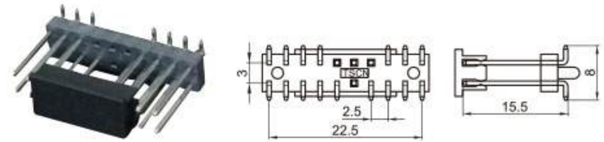
Type: TS57591-16PM-PKB Material: LCP GF30% Matching Terminal: TSPM0139
