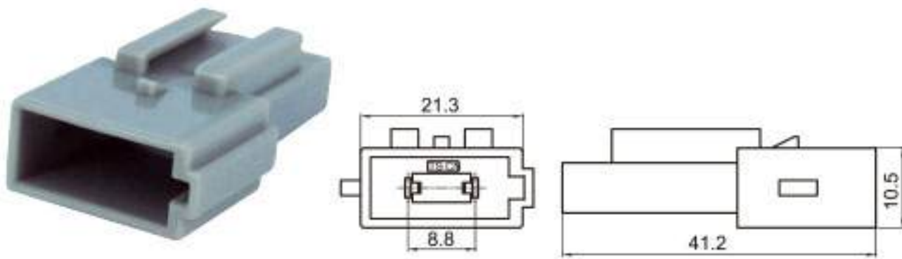
Type: TSLB12-02P-11 Material: ABS Matching Terminal: TSZ006
