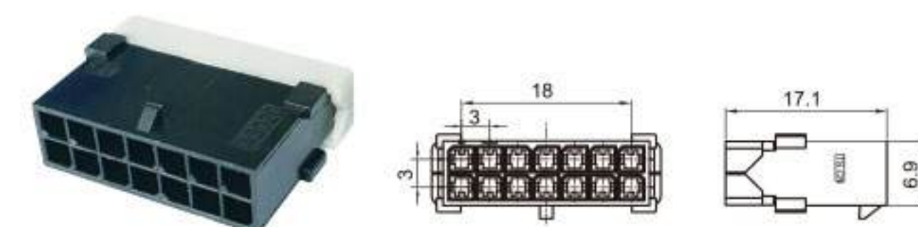
Type: TS43025-14P-11-3(04P-24P) Material: PA66 Matching Terminal: TSZ160
