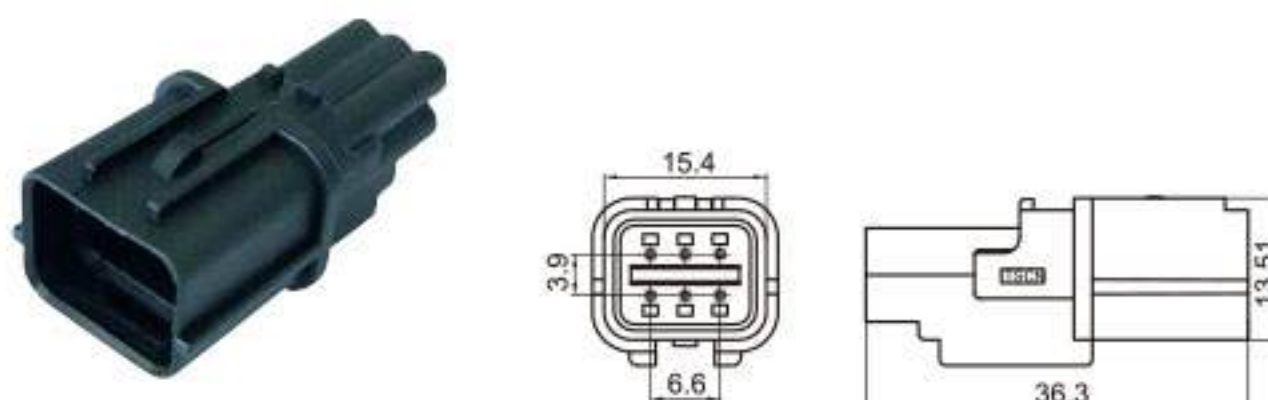
Type: TS30207-06P-11 Material: PBT GF15% Matching Terminal: TSZ537
