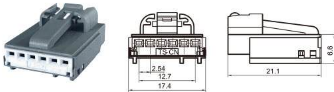
Type: TS30362-06P-21-1 Material: PA66 GF30% Matching Terminal: TSH006B
