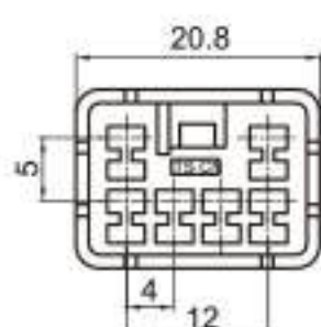
Type: TS1761-06P-11-1 Material: PA66 Matching Terminal: TSZ003
