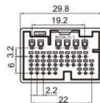
Type: TS30124-35P-11-1 Material: PA66 Matching Terminal: TSZ145 / TSZ208
