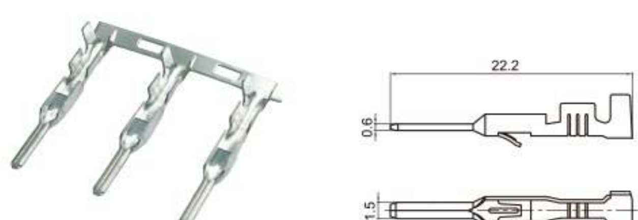
Type: TSZ040 Material: Brass
