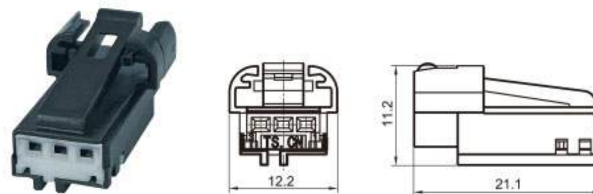
Type: TS30362-03P-21 Material: PA66 GF30% Matching Terminal: TSH006B
