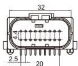
Type: TS30160-18PM-PKB Material: PBT GF30% Matching Terminal: TSPM0148 / TSPM0149
