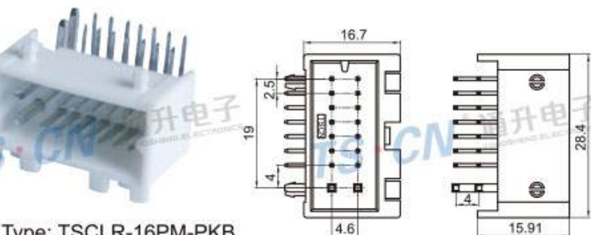
Type: TSCLR-16PM-PKB Material: PA66 Matching Terminal: TSPM0040 / TSPM0221~TSPM0223
