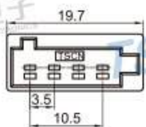
Type: TS30180-04P-11 Material: PA66 GF30% Matching Terminal: TSZ040
