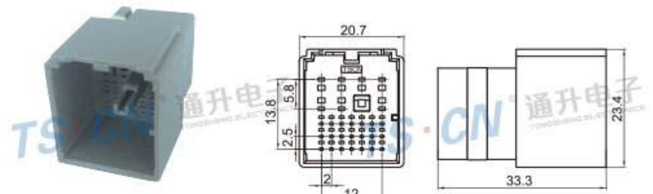
Type: TS30205-28P-11-3 Material: PA66 Matching Terminal: TSZ566 / TSZ561
