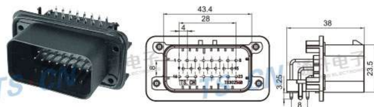
Type: TS30256-23PM-PKB Material: PBT Matching Terminal: TSPM0336~TSPM0338
