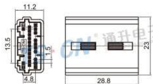
Type: TS30258-21PM-PKS Material: PBT GF15% Matching Terminal: TSPM6078 / TSPM0305
