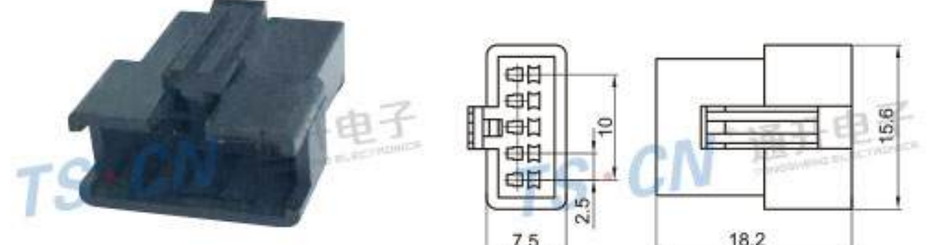
Type: TSSM-05P-11(02P-12P) Material: PA66 Matching Terminal: TSZSM
