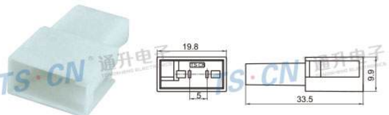
Type: TSLB10-02P-11(TA) Material: PA66 Matching Terminal: TSZ115
