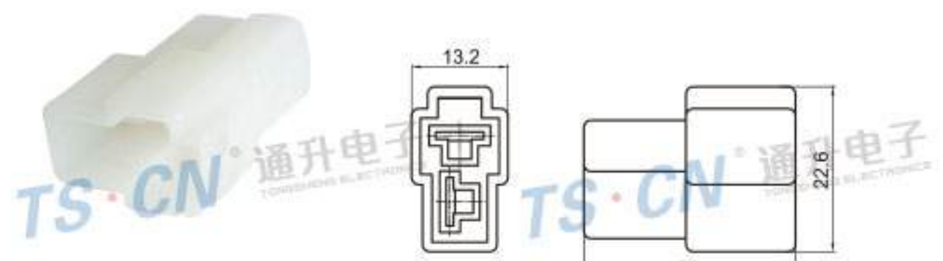
Type: TS7021-6.3-11 Material: PA66 Matching Terminal: TS611-6.3B
