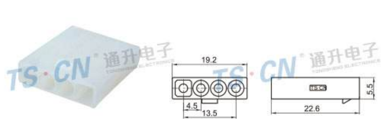
Type: TSOTP-04P-11 Material: PA66 Matching Terminal: NIL
