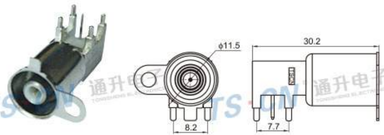
Type: TSCR10-01PM-PKB Material: PA66 Matching Terminal: TSPM0176~TSPM0178
