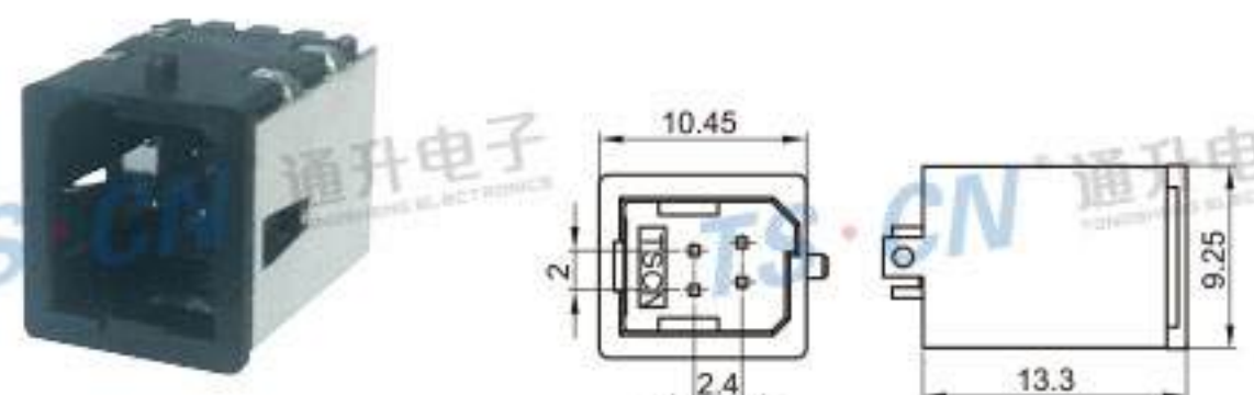
Type: TS30068-04PM-PKS Material: PA66 GF30% Matching Terminal: TSPM0224 / TSPM0030
