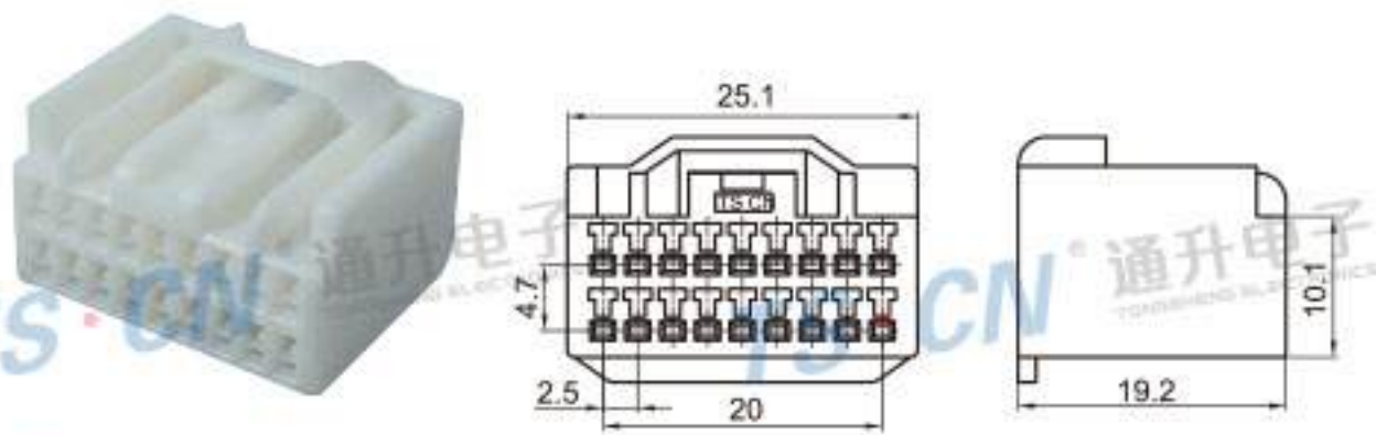
Type: TSMI18-18P-21 Material: PA66 Matching Terminal: TSH006
