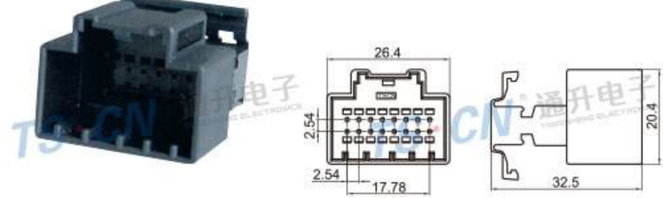
Type: TS30073-16P-11(2015) Material: PA66 GF15% Matching Terminal: TSZ208B
