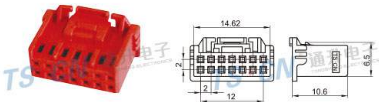
Type: TSQRA3-14P-21 Material: PA66 GF15% Matching Terminal: TSPHB
