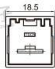
Type: TS30179-01P-11 Material: PBT GF15% Matching Terminal: TSDJ612-9.5*1.2C
