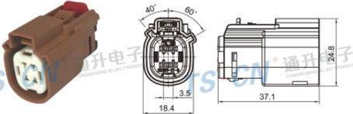
Type: TS30359-04P-21-2 Material: PA66 GF30% Matching Terminal: TSH047
