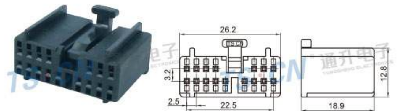
Type: TSHD16-16P-21 Material: PA66 Matching Terminal: TSH143
