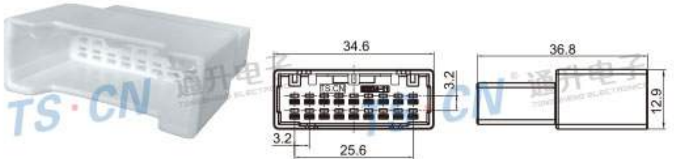
Type: TS30324-18P-11 Material: PBT Matching Terminal: TSZ562
