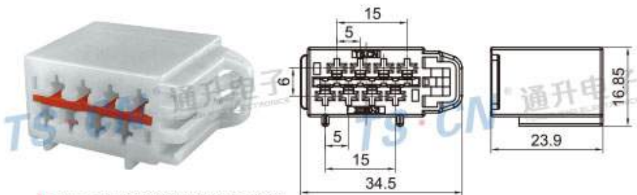
Type: TS30360-08P-21-2 Material: ABS Matching Terminal: TSH085
