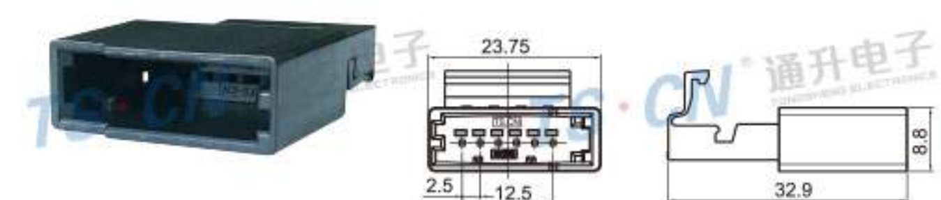
Type: TS30290-06P-11 Material: PA66 Matching Terminal: TSZ616
