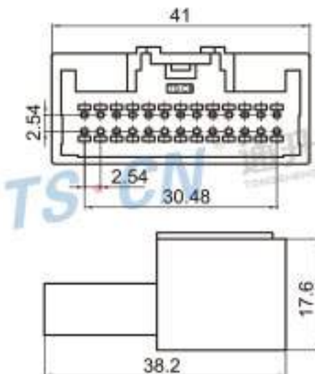
Type: TS5524-26P-11 Material: PA66 GF30% Matching Terminal: TSZ08B
