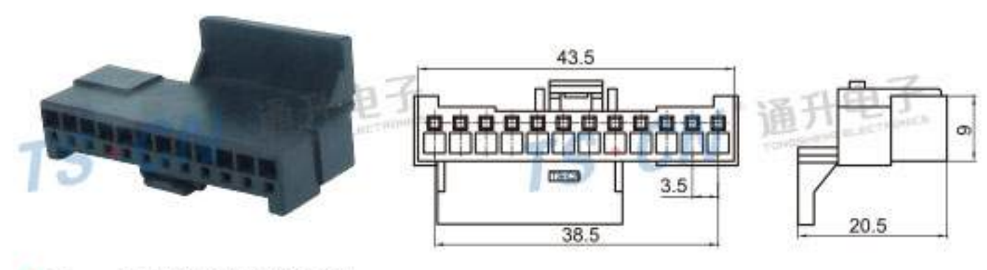
Type: TSPI12A-12P-21 Material: PA66 GF15% Matching Terminal: TSH511
