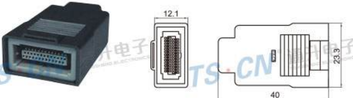
Type: TS30025-26PF-AH Material: PA66 Matching Terminal: TSAF0024 / TSAF0026
