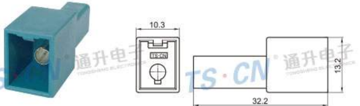
Type: TS1068-01PM-AT-4 Material: PA66 GF30% Matching Terminal: TSTM0003 / TSTM0004
