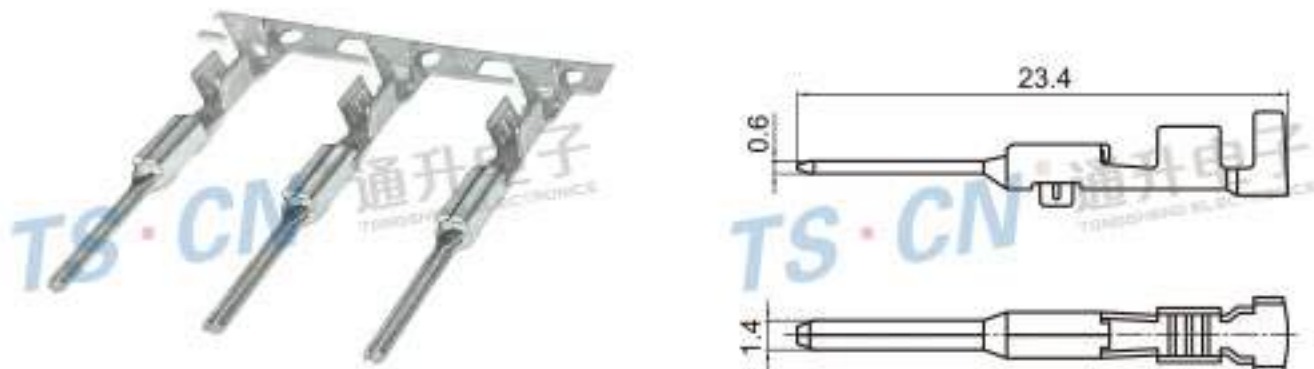
Type: TSZ619 Material: Brass
