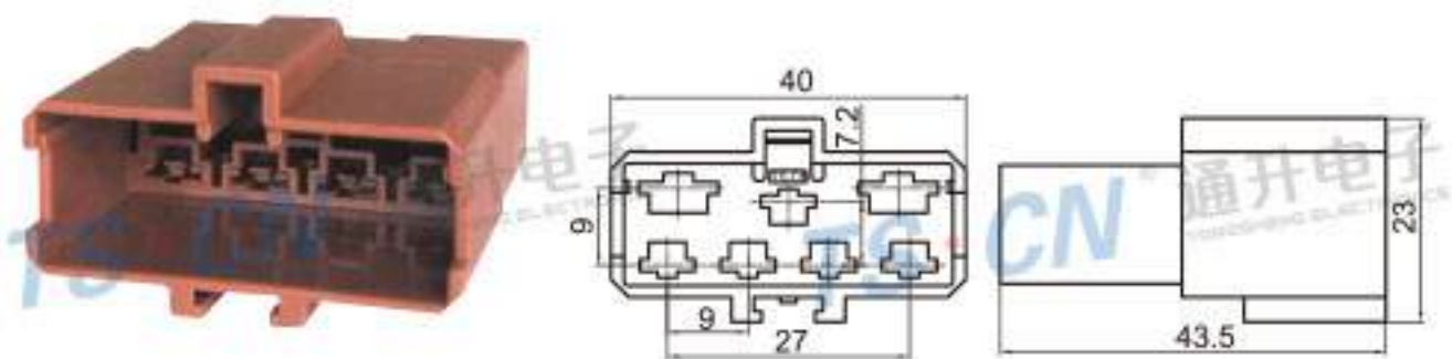
Type: TS30012-07P-11 Material: PA66 Matching Terminal: TSZ555 / TSZ565
