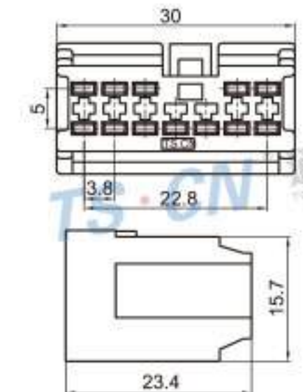
Type: TS7550-12P-21 Material: PA66 Matching Terminal: TSH064
