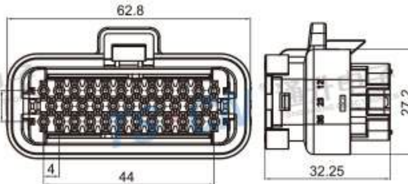
Type: TS30256-35P-21(TS3018) Material: ABS+PC Matching Terminal: TSH640
