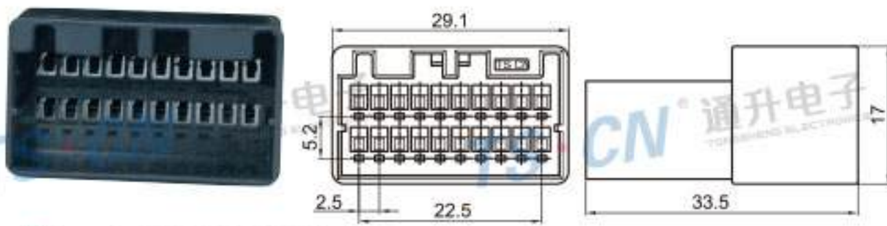
Type: TSHD20-20P-11-5 Material: PA66 Matching Terminal: TSZ145
