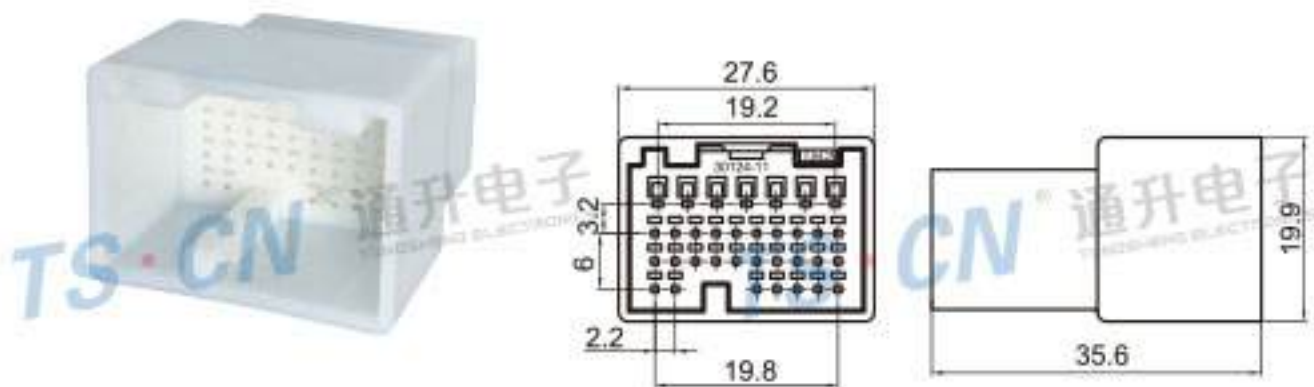
Type: TS30124-34P-11 Material: PA66 Matching Terminal: TSZ145 / TSZ208
