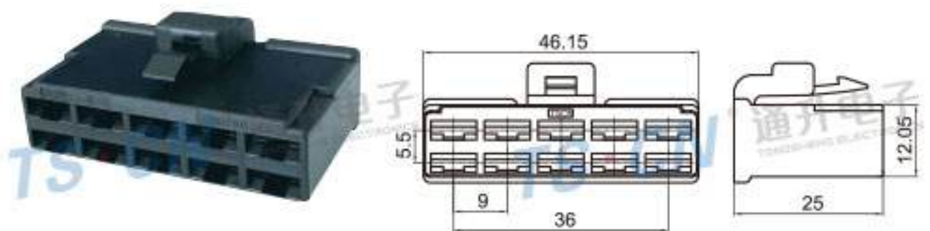
Type: TS30198-10P-21BK Material: PA66 Matching Terminal: TSH033A
