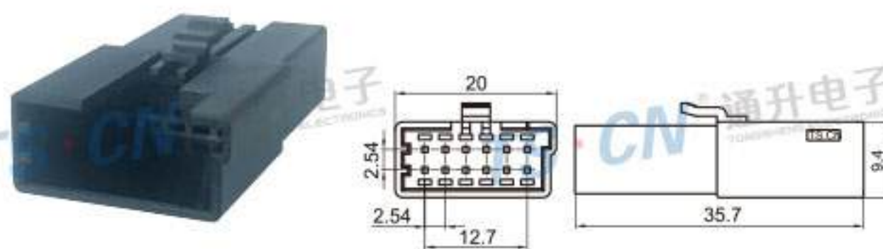
Type: TS30069-12P-11 Material: PA66 GF30% Matching Terminal: TSZ208
