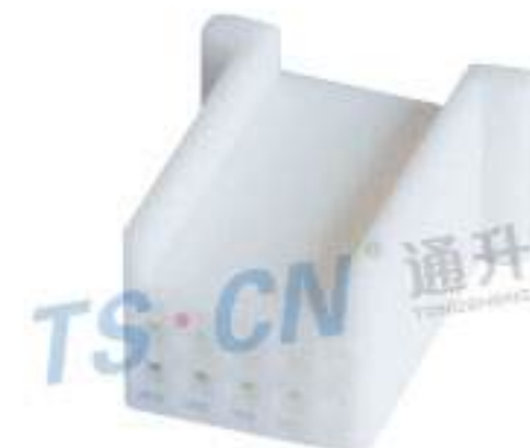
Type: TSROWE-10P-21 Material: PA66 Matching Terminal: TSH143
