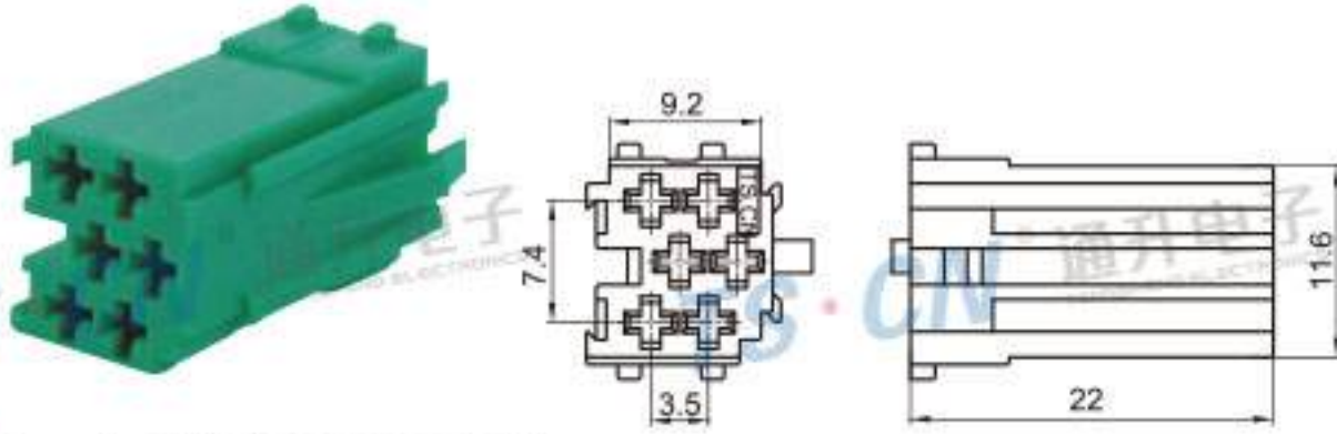
Type: TSVW06-06P-21GN Material: PA66 Matching Terminal: TSH054
