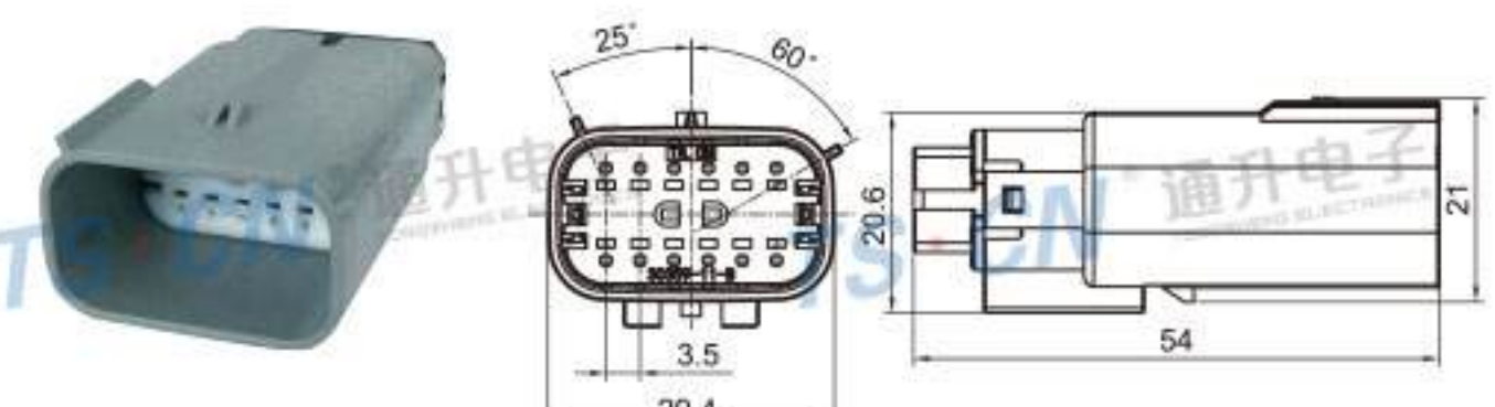
Type: TS30359-12P-11-1 Material: PA66 GF30% Matching Terminal: TSZ144A
