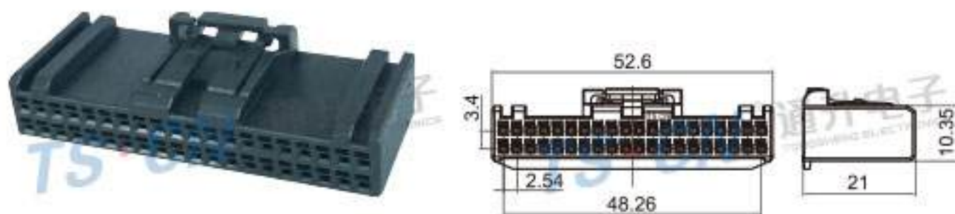
Type: TS30285-40P-21 Material: PBT GF10% Matching Terminal: TSH624
