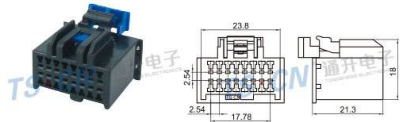
Type: TS2105-16P-21-1 Material: PA66 GF30% Matching Terminal: TSH006
