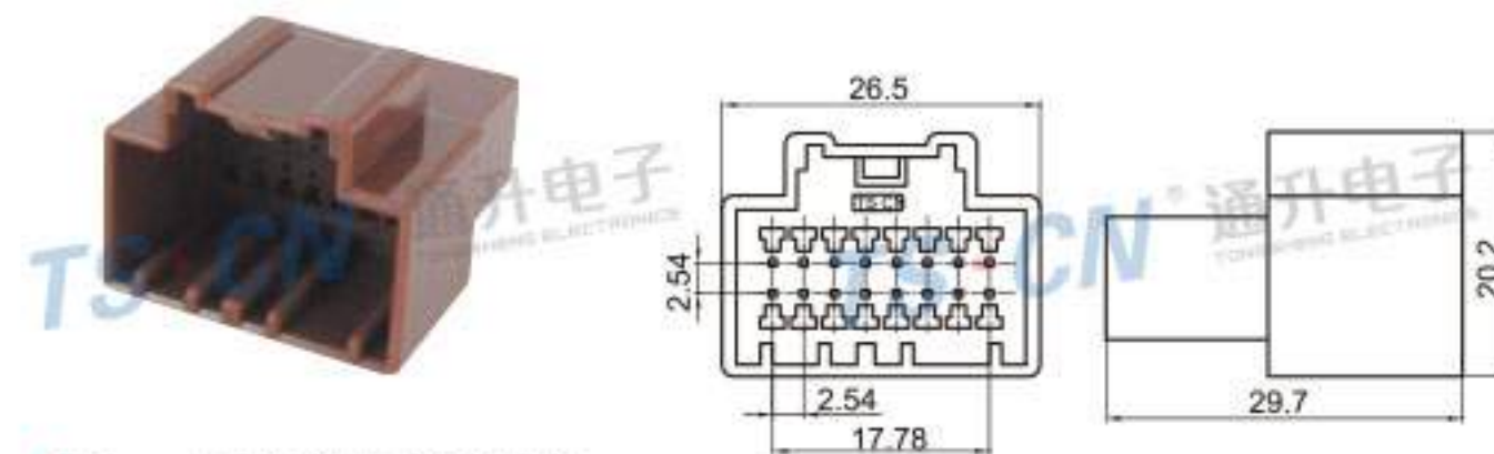
Type: TS2105-16P-11BN Material: PA66 Matching Terminal: TSZ018B
