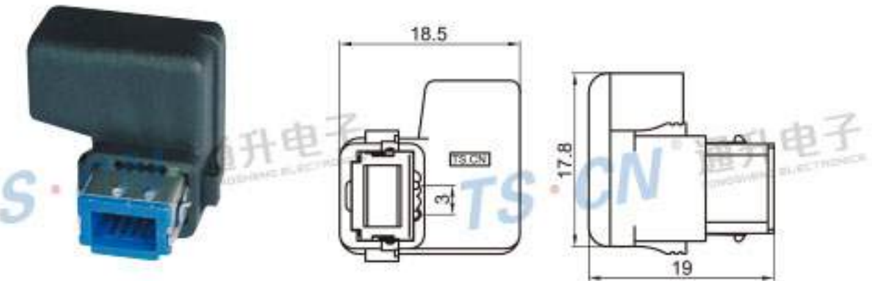
Type: TS30053-10PM-AH-1 Material: PA66 GF30% Matching Terminal: TSAF0007 / TSAM0018 / TSAM0019
