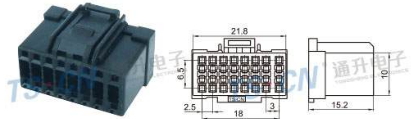
Type: TSPAN05-16P-21 Material: PA66 GF15% Matching Terminal: TSH031B
