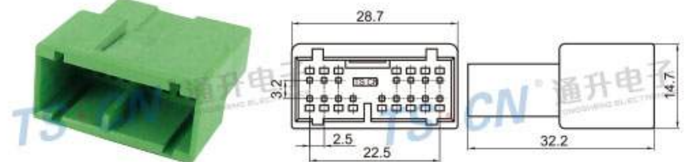
Type: TSHD16-16P-11 Material: PA66 Matching Terminal: TSZ116
