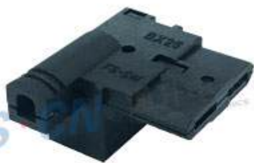
Type: TSBX25 Material: PA66 GF30% Matching Terminal: TSH626 / TSH627
