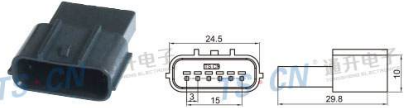
Type: TSHD06-06P-11-3 Material: PA66 GF30% Matching Terminal: TSZ208B
