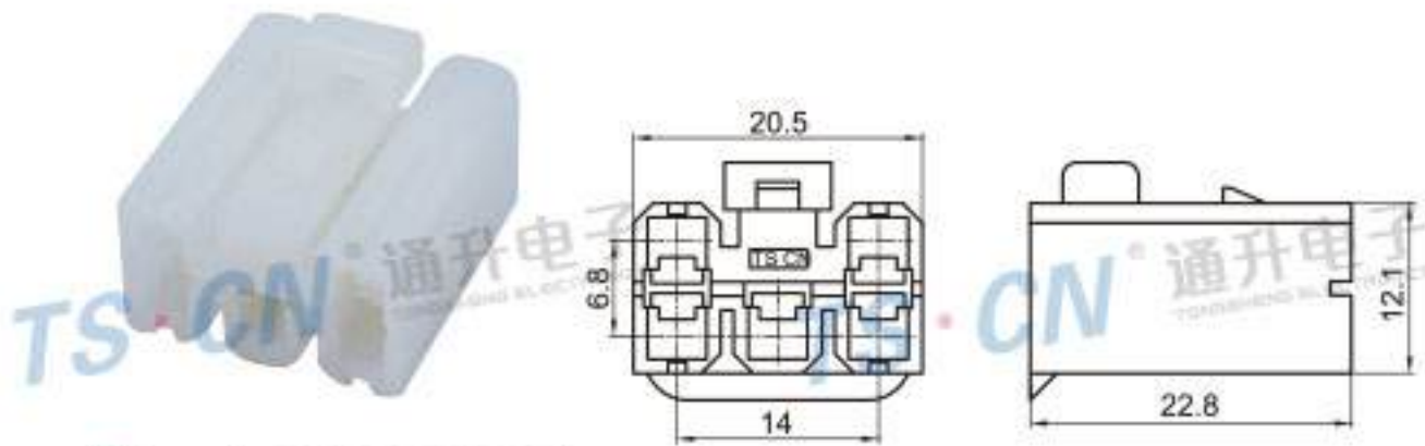
Type: TS1398-05P-21 Material: PA66 Matching Terminal: TSH017
