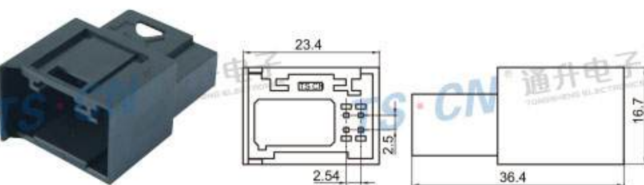
Type: TSBMGQ-06P-11 Material: PA66 GF15% Matching Terminal: TSZ208
