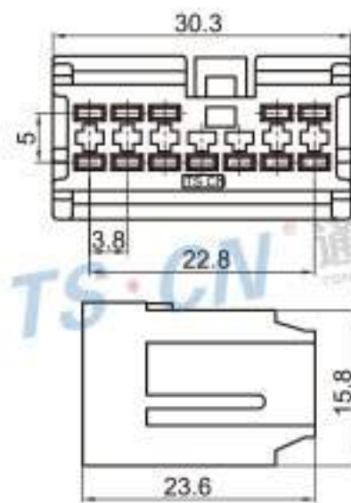
Type: TS7550-12P-21-1 Material: PA66 Matching Terminal: TSH064
