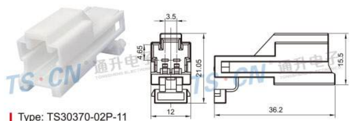
Type: TS30370-02P-11 Material: PA66 Matching Terminal: TSZ007
