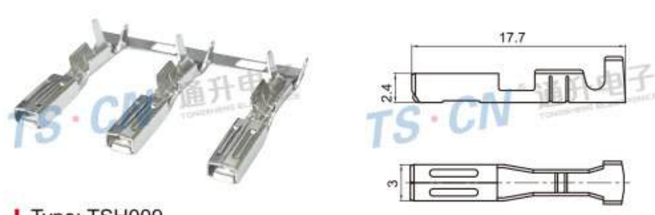
Type: TSH009 Material: Phos.bronze Applicable Thickness: 0.6~0.8
