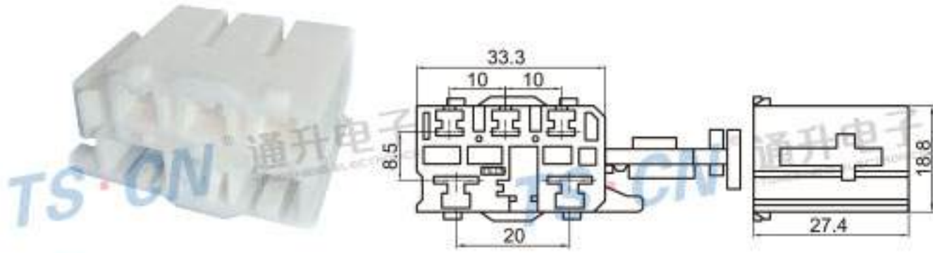
Type: TS30013-05P-21 Material: PBT Matching Terminal: TSH591 / TSH585
