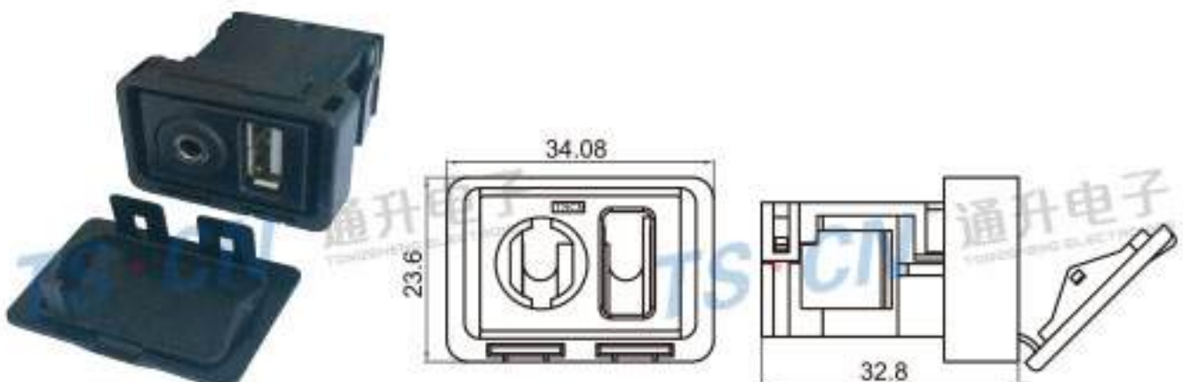
Type: TSAP-1 Material: ABS Matching Terminal: TSUSB-F / TS3.5-F
