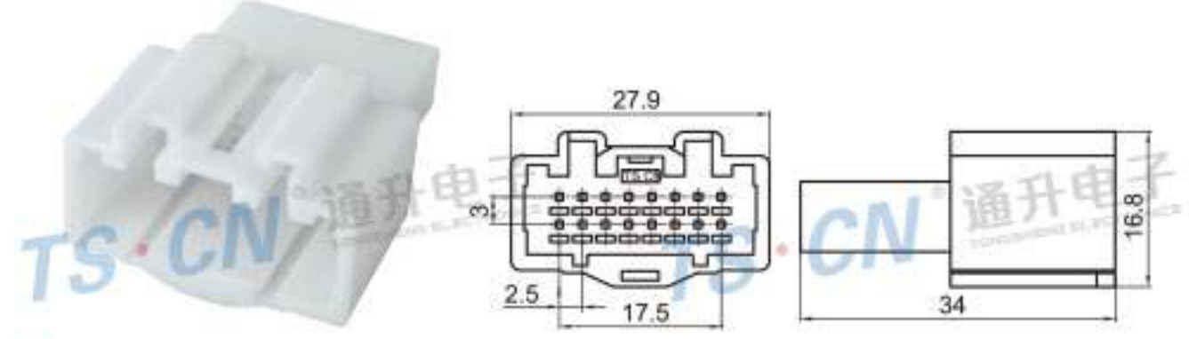
Type: TSMA1609-16P-11 Material: PA66 Matching Terminal: TSZ208B
