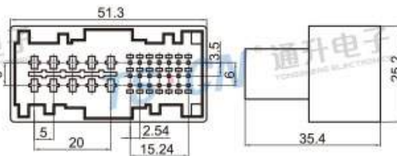
Type: TS30102-31P-11 Material: PBT GF15% Matching Terminal: TSZ024 / TSZ208
