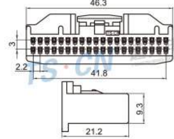
Type: TSTA40-40P-21-3 Material: PA66 Matching Terminal: TSH143
