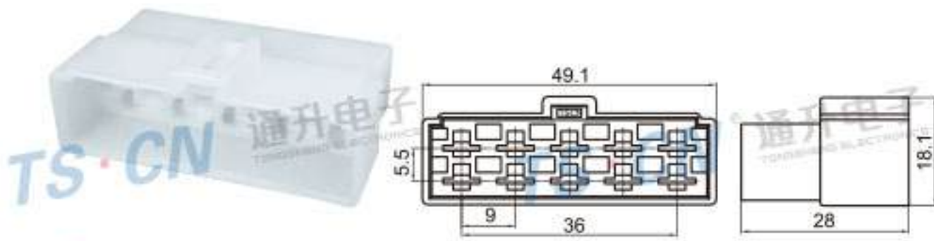
Type: TS30198-10P-11 Material: PA66 Matching Terminal: TSZ538A
