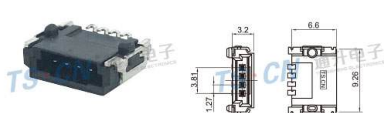
Type: TS30278-04PM-PKB Material: PPS Matching Terminal: TSPM0306 / TSPM0307
