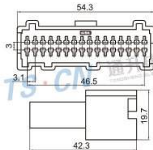
Type: TS2001-32P-11 Material: PA66 Matching Terminal: TSZ013
