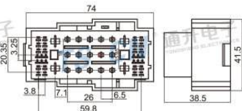
Type: TS30168-51P-11 Material: PA66 GF30% Matching Terminal: TSZ538A / TSZ024 / TSZ040 / TSZ208B
