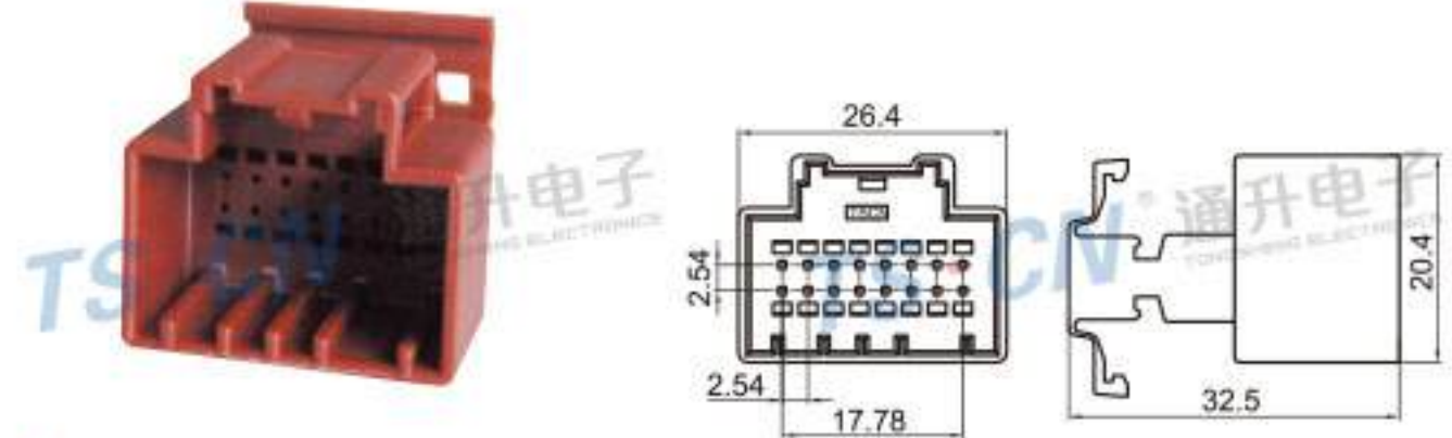
Type: TS30074-16P-11(2015) Material: PA66 GF15% Matching Terminal: TSZ208B
