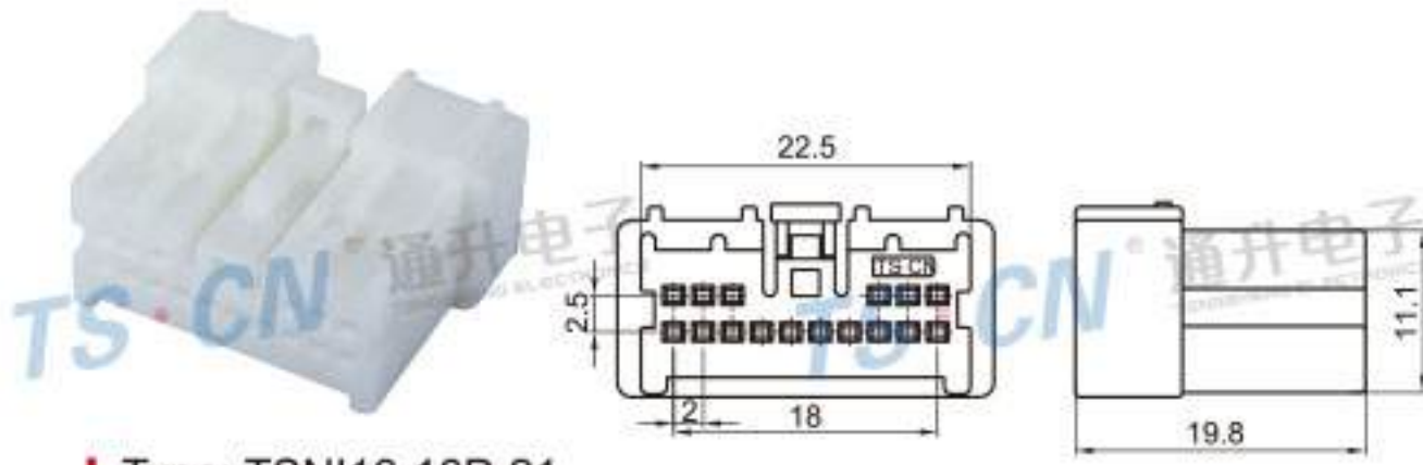
Type: TSNI16-16P-21 Material: PA66 Matching Terminal: TSH143
