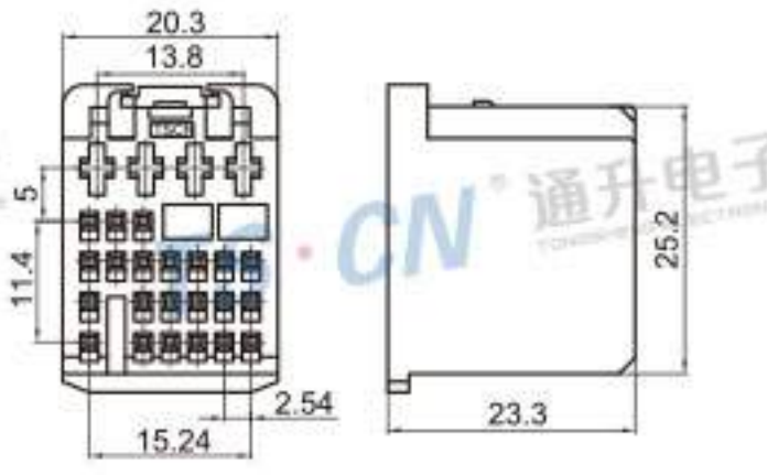
Type: TS30217-30P-11-3 Material: PBT GF15% Matching Terminal: TSDJ615B-2.8*0.8B / TSZ208
