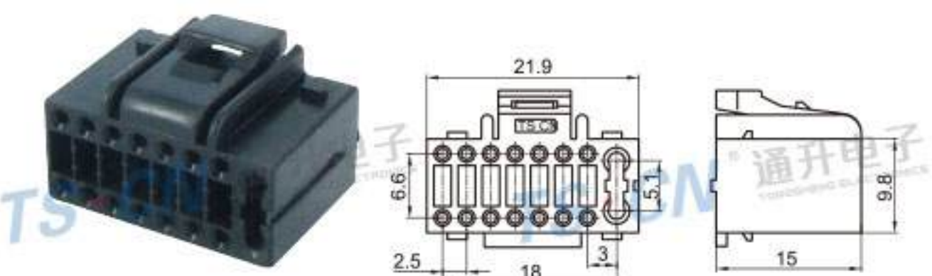
Type: TSKEN16-16P-21 Material: PA66 GF30% Matching Terminal: TSH032 / TSH031
