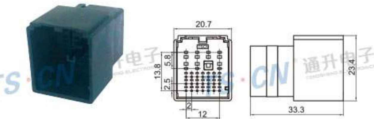
Type: TS30205-28P-11 Material: PA66 Matching Terminal: TSZ566 / TSZ561
