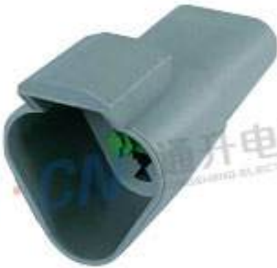
Type: TS30267-03P-11 Material: PBT GF15% Matching Terminal: TSZ621
