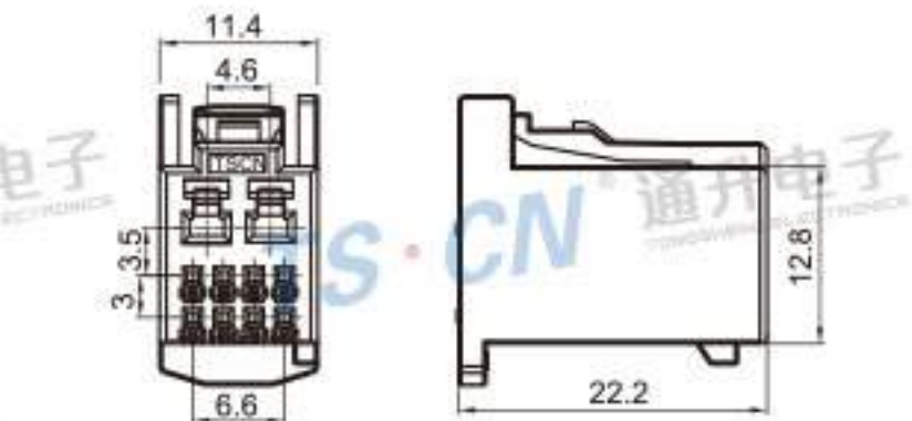
Type: TS30348-10P-21 Material: PBT Matching Terminal: TSH064 / TSH631
