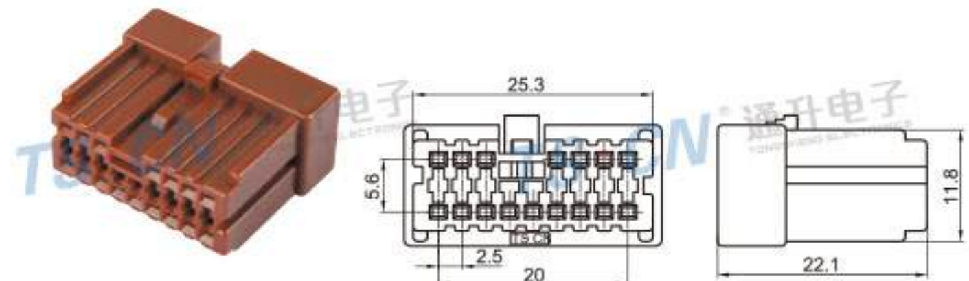
Type: TSHY16-16P-21 Material: PA66 Matching Terminal: TSH006
