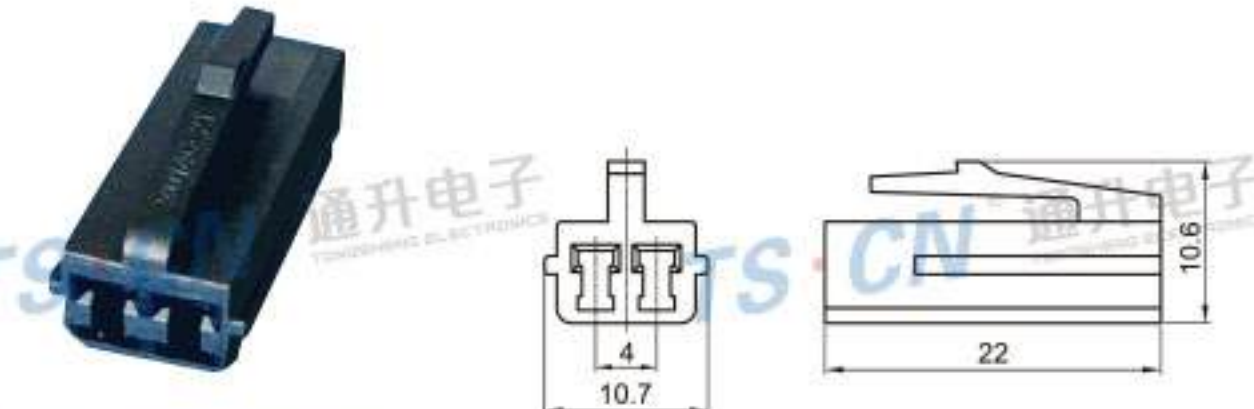
Type: TS30146-02P-21 Material: PA66 Matching Terminal: TSH009
