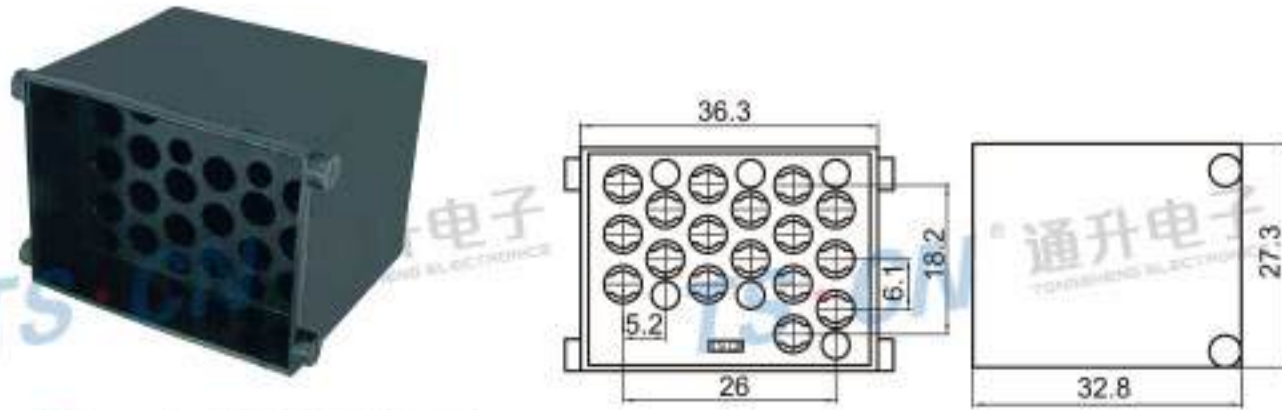
Type: TS8590-17P-11 Material: PA66 GF30% Matching Terminal: TSZ036
