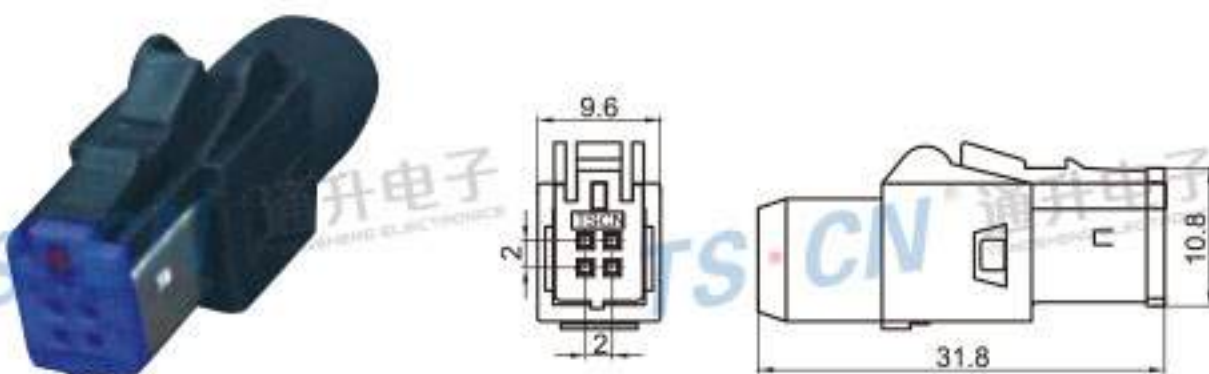
Type: TSMA04-04PF-AH-2 Material: PA66 GF15% Matching Terminal: TSAF0013 / TSPH
