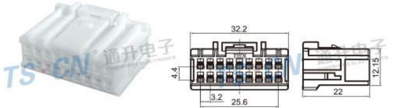
Type: TS30320-18P-21 Material: PBT Matching Terminal: TSH593
