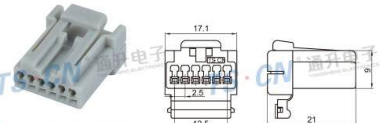
Type: TSHD06-06P-21-4 Material: PA66 Matching Terminal: TSH006
