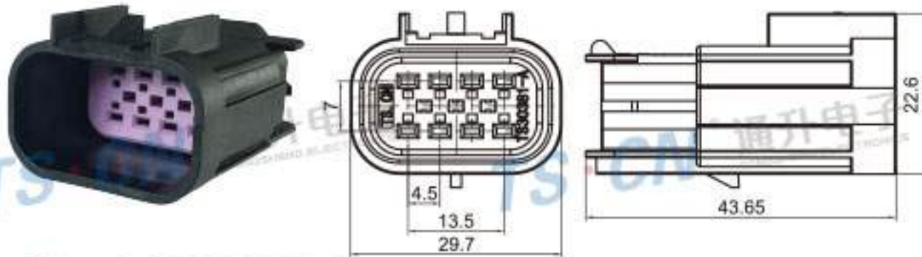
Type: TS30381-08P-11 Material: PA66 GF30% Matching Terminal: TS15326269
