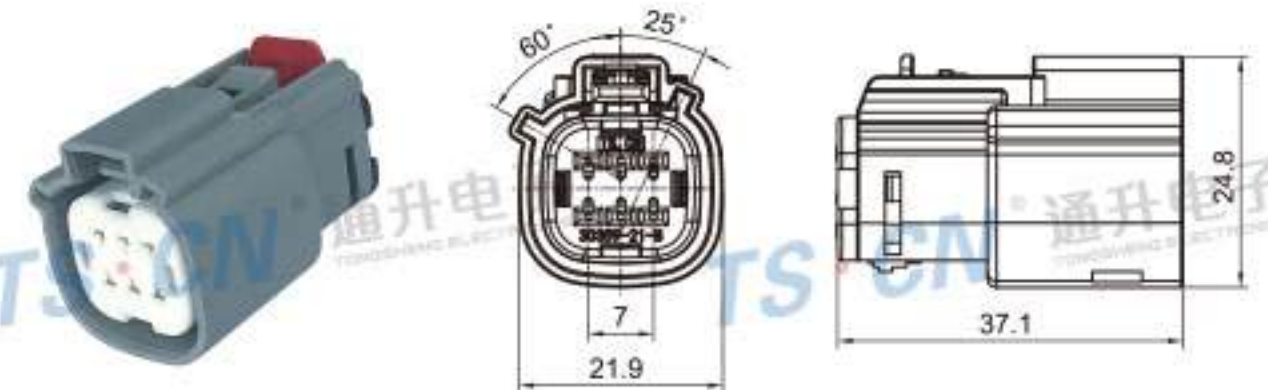
Type: TS30359-06P-21-1 Material: PA66 GF30% Matching Terminal: TSH047
