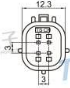
Type: TS1055-04P-11 Material: PA66 GF30% Matching Terminal: TSZ208
