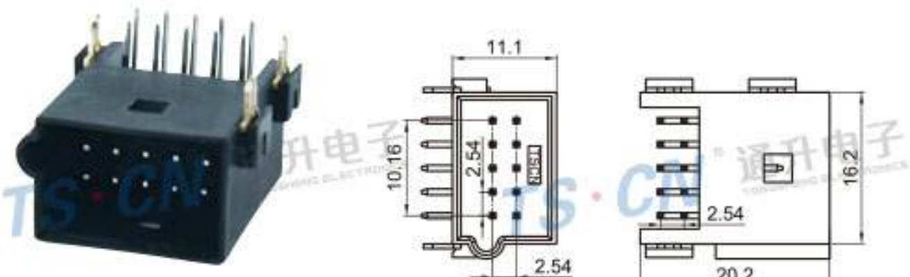
Type: TSBM10-10PM-PKB Material: PA66 GF15% Matching Terminal: TSPM0062 / TSPM0066 / TSPM0123
