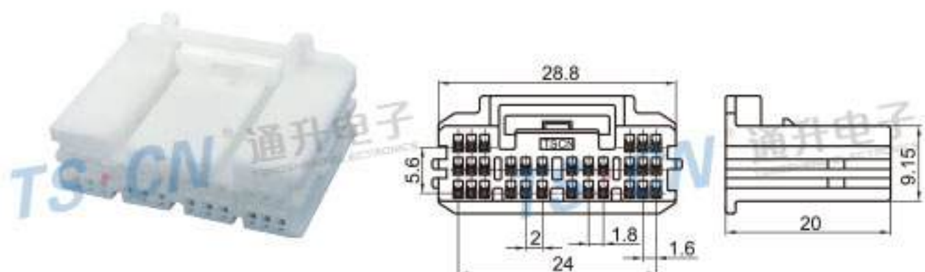
Type: TS30101-30P-21-3 Material: PA66 Matching Terminal: TSH600
