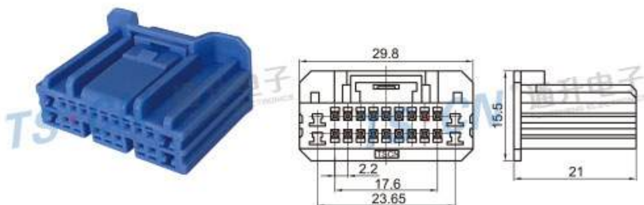
Type: TS30118-20P-21BL Material: PA66 Matching Terminal: TSH541 / TSH143
