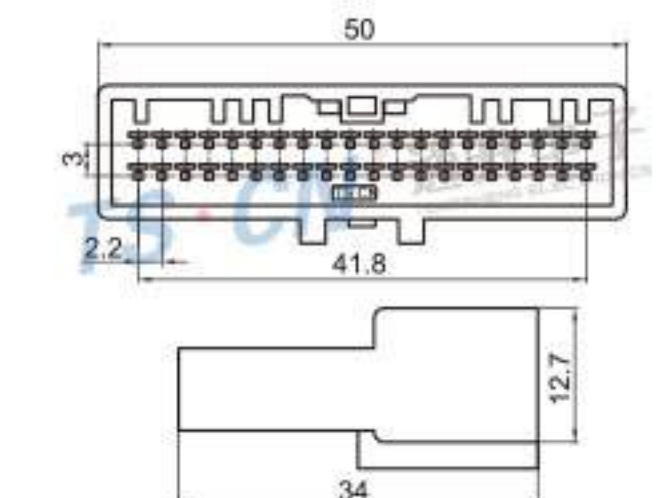
Type: TSTA40-40P-11-3 Material: PA66 Matching Terminal: TSZ208
