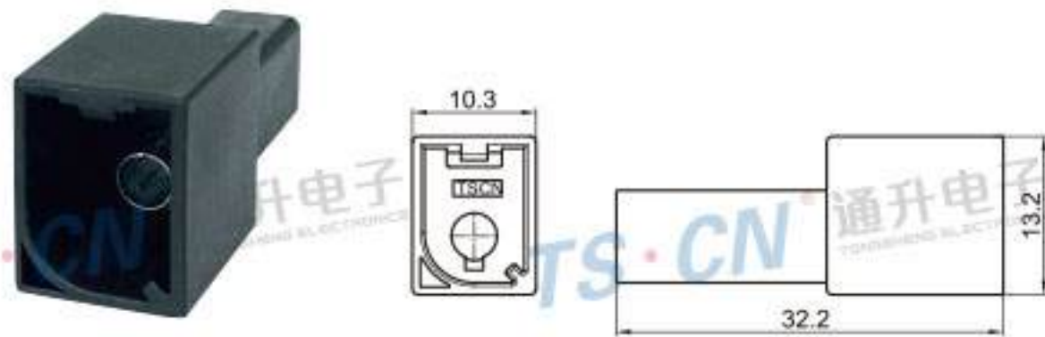
Type: TS1068-01PM-AT Material: PA66 GF30% Matching Terminal: TSTM0003 / TSTM0004
