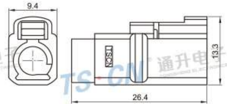
Type: TSVW20-01PF-AT-RD Material: PA66 GF30% Matching Terminal: TSTF0025 / TSTF0026
