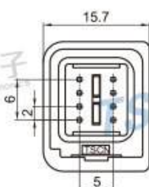
Type: TSNI08-08PM-PKS Material: PA66 GF30% Matching Terminal: TSPM0057 / TSPM0058
