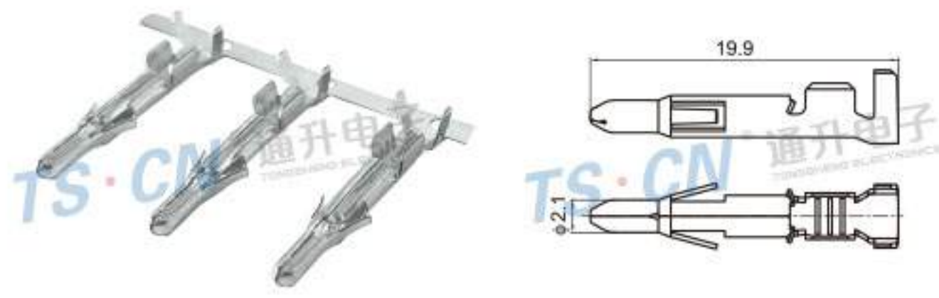
Type: TSZ571 Material: Brass
