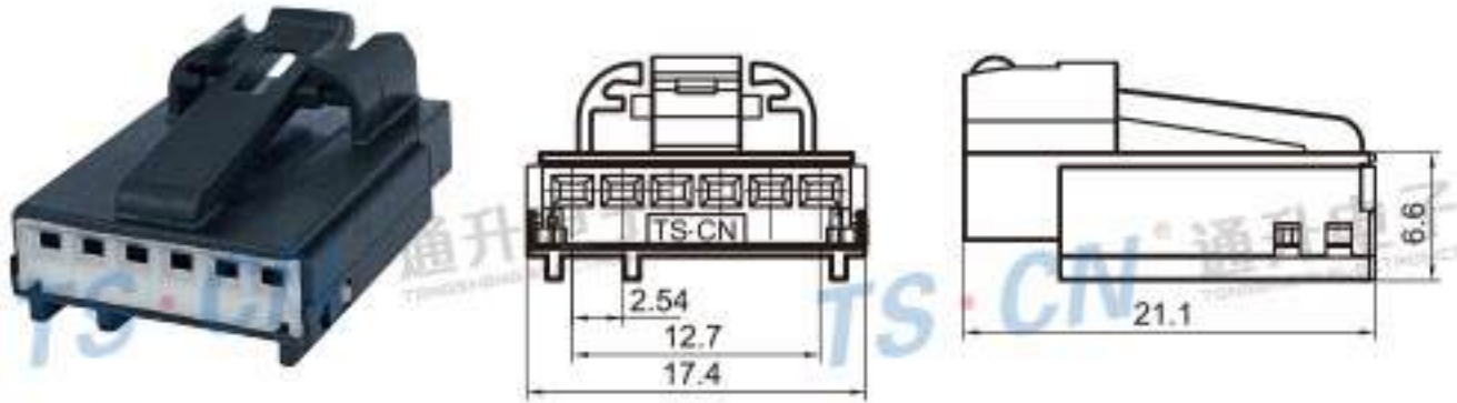
Type: TS30362-06P-21 Material: PA66 GF30% Matching Terminal: TSH006B
