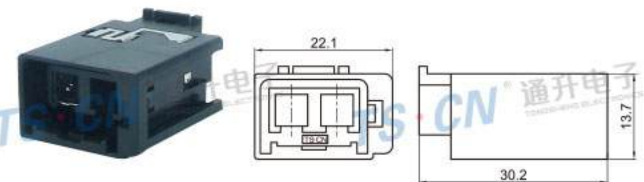
Type: TSVL10-02PM-AT Material: PA66 GF15% Matching Terminal: TSTM0012 / TSTM0013 / TSTM0014
