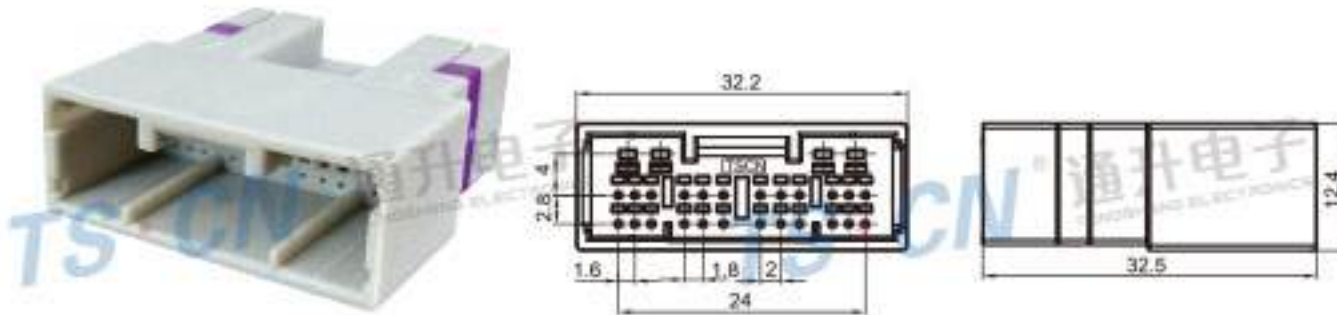
Type: TS30101-28P-11-6 Material: PA66 Matching Terminal: TSZ562 / TSZ615
