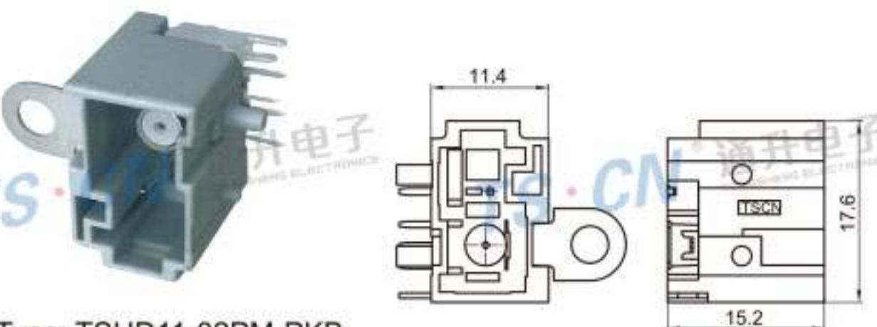
Type: TSHD11-02PM-PKB Material: PBT GF30% Matching Terminal: TSPM0148~TSPM0166
