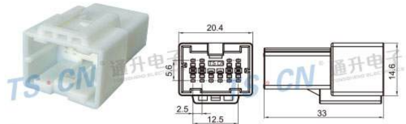
Type: TSNI10-10P-11-1 Material: PA66 Matching Terminal: TSZ145
