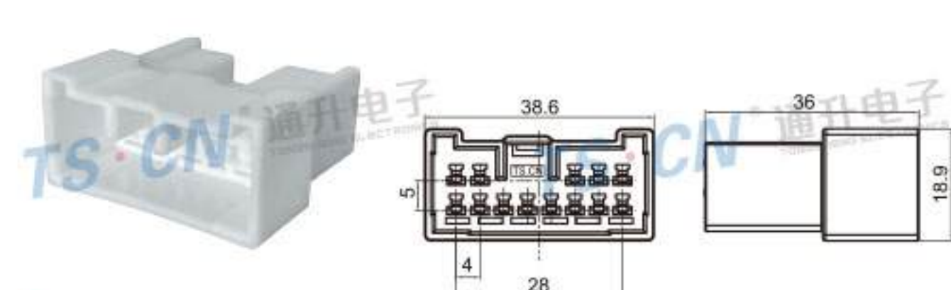
Type: TS30319-13P-11 Material: PBT Matching Terminal: TSZ045
