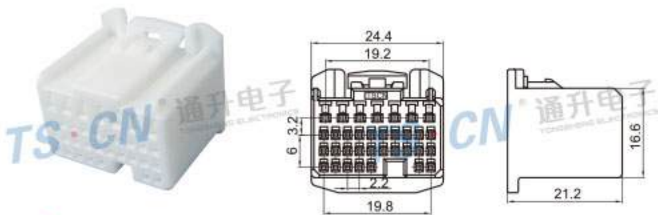
Type: TS30124-34P-21 Material: PA66 Matching Terminal: TSH076 / TSH143
