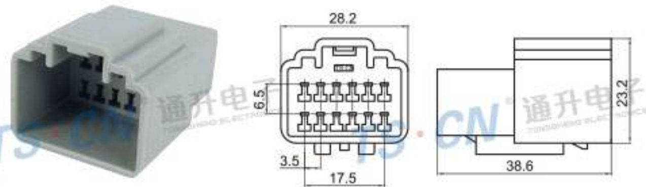
Type: TSVO12-12P-11 Material: PA66 Matching Terminal: TSZ144
