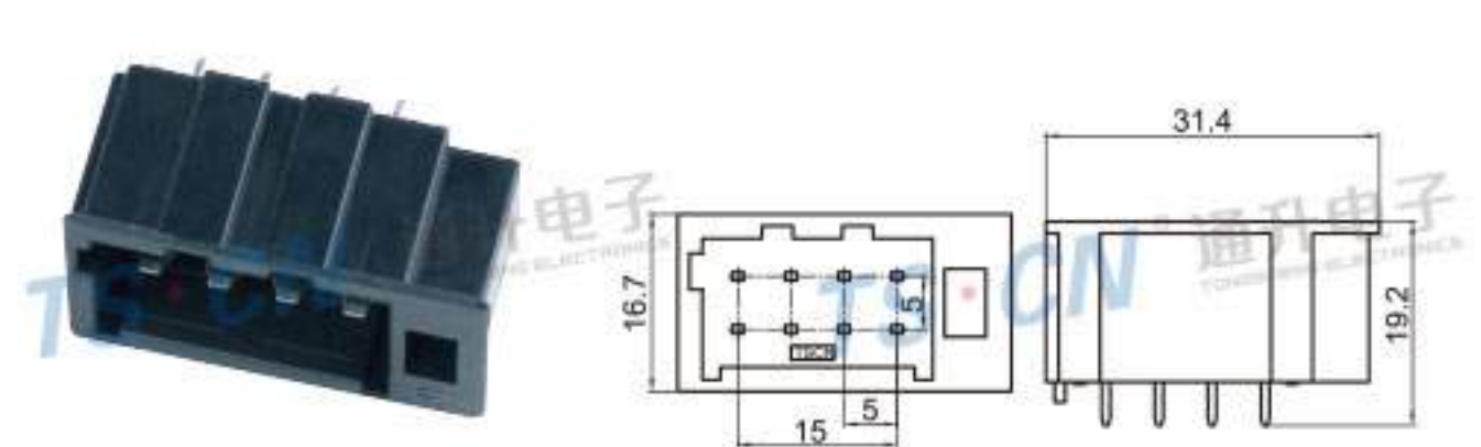
Type: TSABD-08PM-PKS-D Material: PA66 Matching Terminal: TSPM0127
