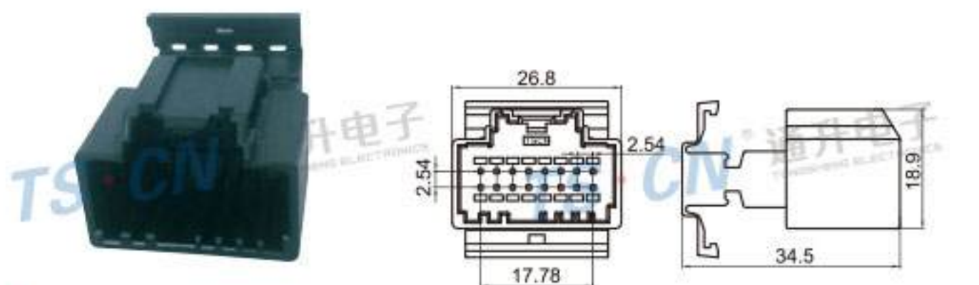
Type: TS30244-16P-11 Material: PA66 Matching Terminal: TSZ208B
