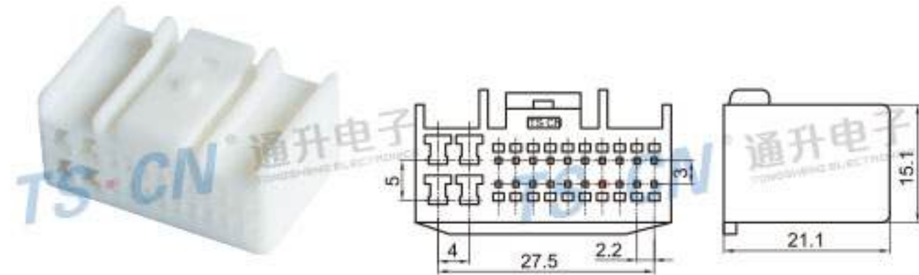
Type: TS7304-24P-21 Material: PA66 Matching Terminal: TSH064 / TSH143
