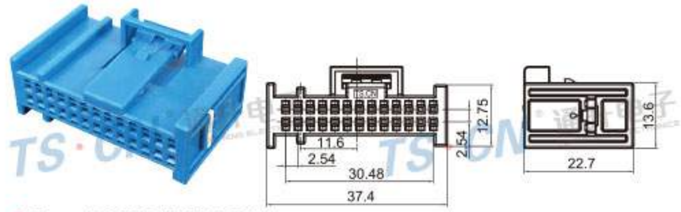
Type: TS30316-26P-21-1 Material: PA66 GF30% Matching Terminal: TSH624
