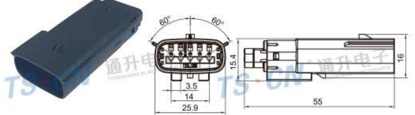
Type: TS30366-05P-11 Material: PA66 GF30% Matching Terminal: TSZ144A
