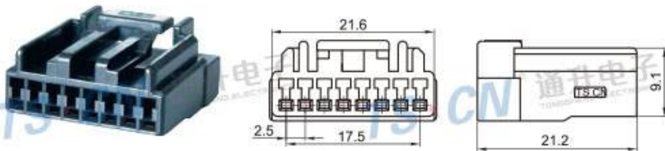
Type: TSHD08-08P-21 Material: PA66 GF30% Matching Terminal: TSH076
