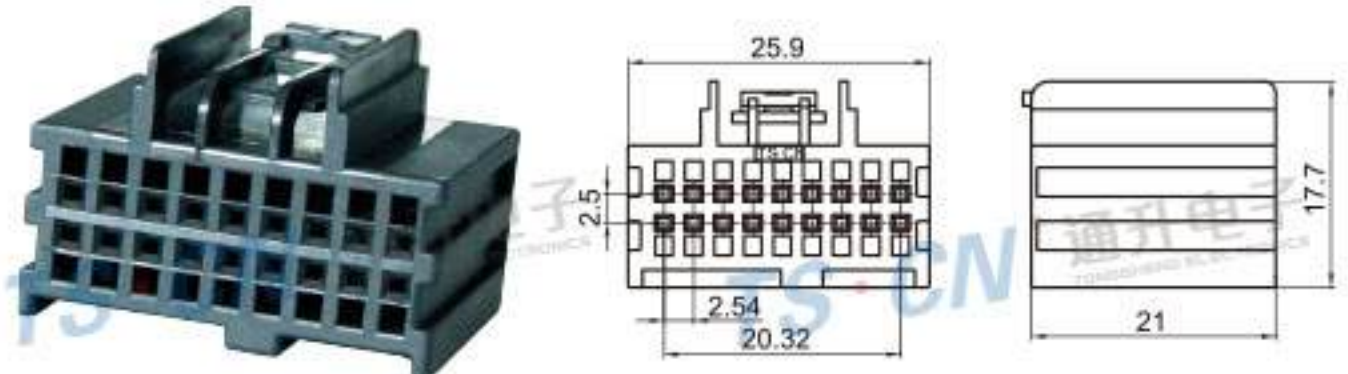
Type: TSGM18-18P-21 Material: PA66 GF15% Matching Terminal: TSH143
