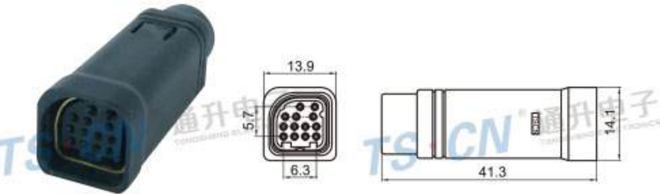
Type: TSPIOH-13PF-AH Material: PA66 Matching Terminal: TSAF0030 / TSAF0034
