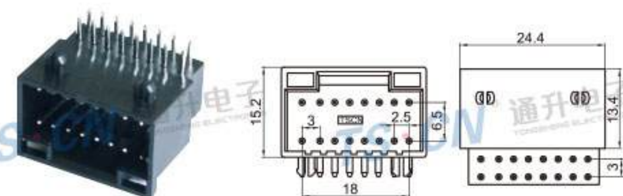
Type: TSALP-16PM-PKB-2 Material: PBT GF30% Matching Terminal: TSPM0167 / TSPM0168
