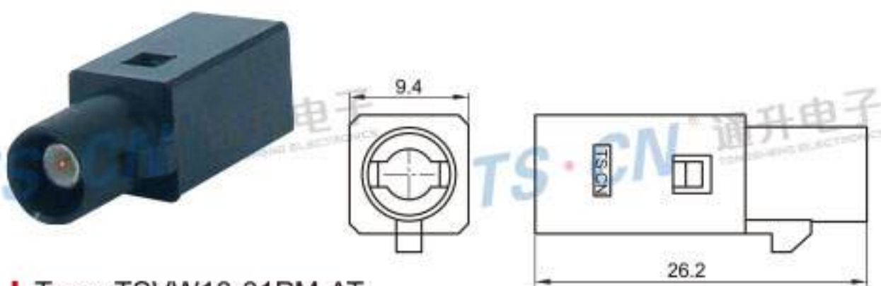
Type: TSVW10-01PM-AT Material: PA66 Matching Terminal: TSTM0018 / TSTM0019
