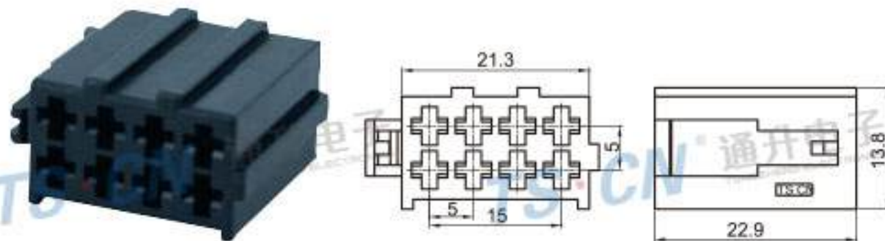
Type: TSABD-08P-21-B Material: PA66 Matching Terminal: TSH019A
