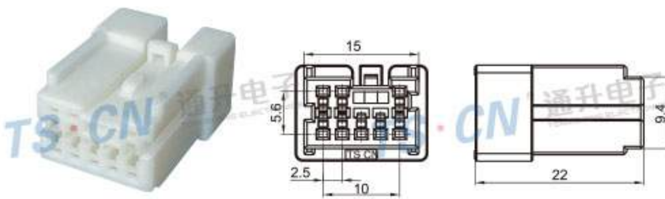
Type: TSNI08-08P-21-2 Material: PA66 Matching Terminal: TSH076
