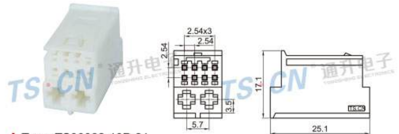
Type: TS30022-10P-21 Material: PA66 Matching Terminal: TSH019 / TSH143
