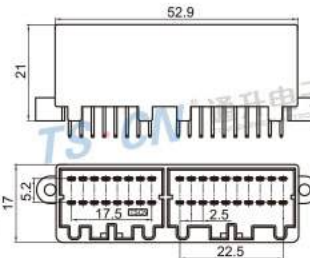
Type: TSHD36-36PM-PKB-2 Material: PA66 Matching Terminal: TSPM0088 / TSPM0089
