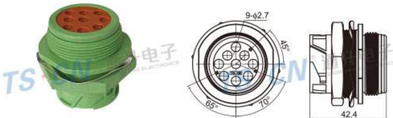
Type: TS30361-09P-11 Material: PA66 GF30% Matching Terminal: TSZ621
