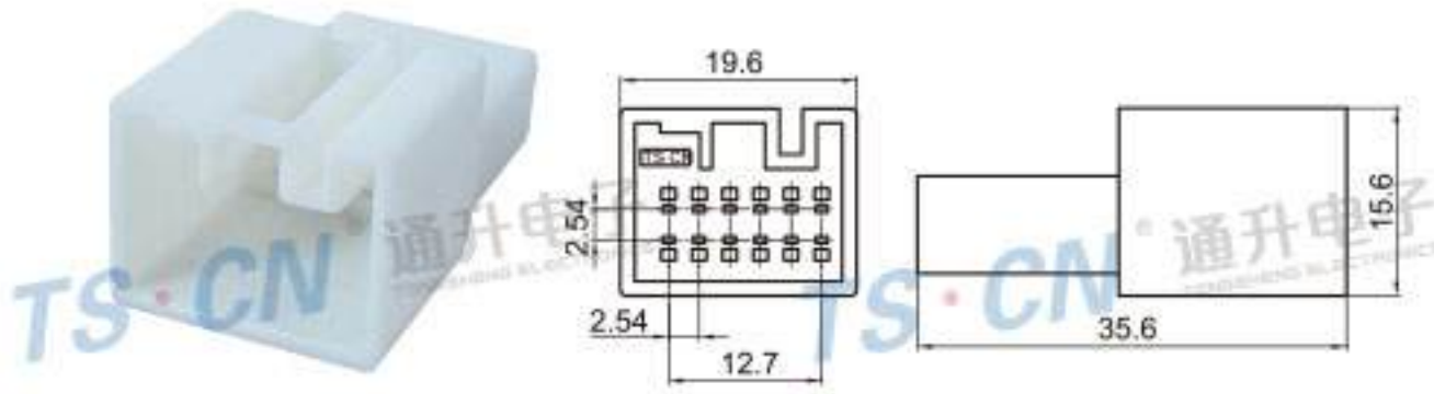
Type: TSVW12-12P-11WT Material: PA66 Matching Terminal: TSZ116
