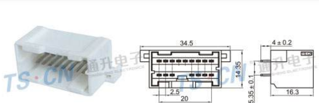
Type: TS30030-16PM-PKS Material: PA66 GF30% Matching Terminal: TSPM0090
