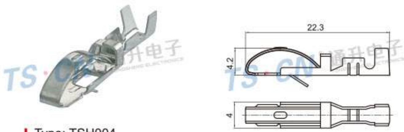
Type: TSH004 Material: Brass Applicable Thickness: 0.5
