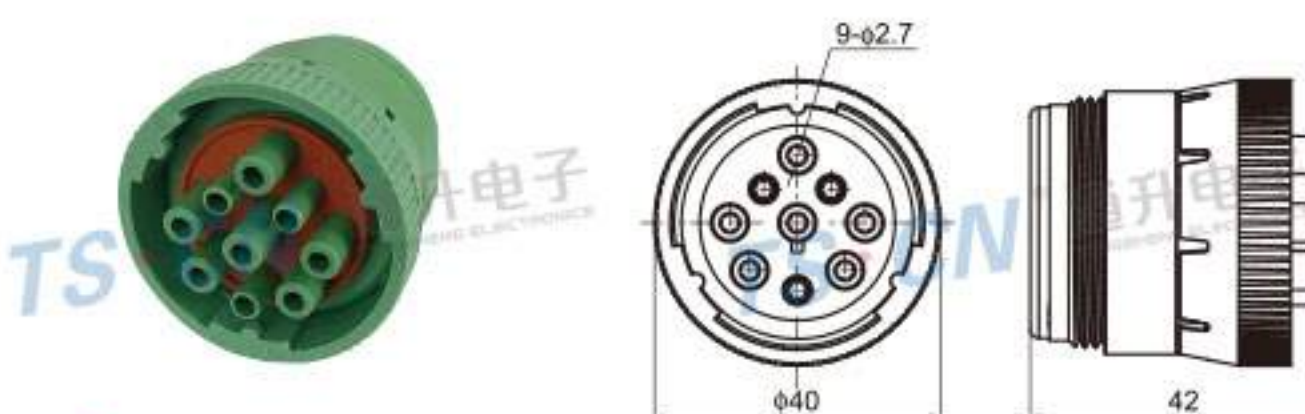
Type: TS30361-09P-21 Material: PA66 GF30% Matching Terminal: TSH646
