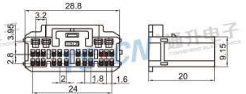
Type: TS30101-28P-21-1 Material: PA66 Matching Terminal: TSH593 / TSH600
