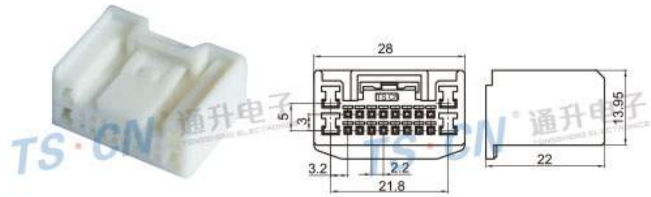
Type: TSTA20-20P-21-2 Material: PA66 Matching Terminal: TSH064 / TSH143
