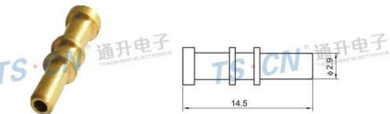
Type: TSBMGQ-C Material: Brass Matching Terminal: NIL
