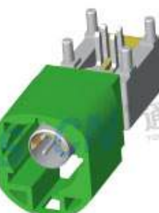
Type: TSVW10-04PM-AT-5GN Material: PA66 GF30% Matching Terminal: TSPM0021~TSPM0025
