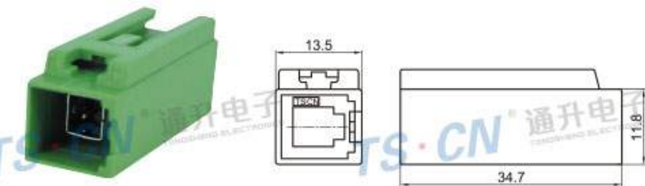
Type: TSTA10-01PM-AT Material: PA66 Matching Terminal: TSPM0012 / TSPM0013
