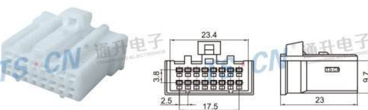
Type: TSMA16-16P-21 Material: PA66 Matching Terminal: TSH053
