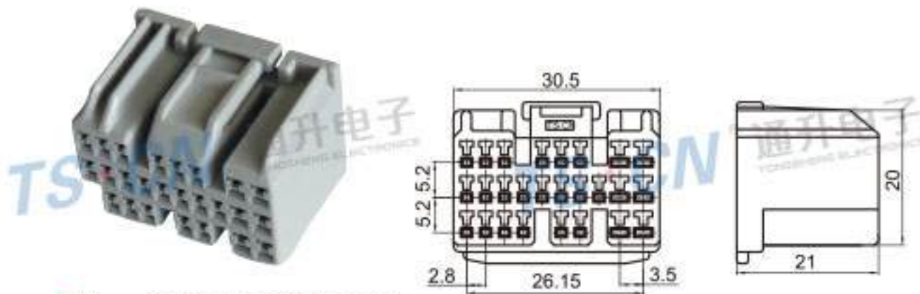
Type: TSWH104-25P-21 Material: PA66 Matching Terminal: TSH009 / TSH076
