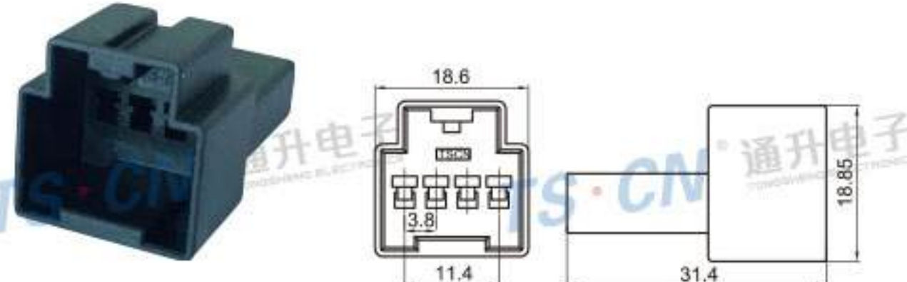
Type: TS30145-04P-11 Material: PA66 GF30% Matching Terminal: TSZ009
