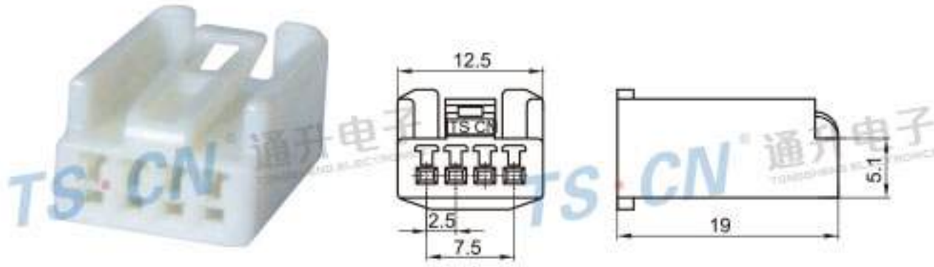
Type: TSTA04-04P-21-2 Material: PA66 Matching Terminal: TSH076
