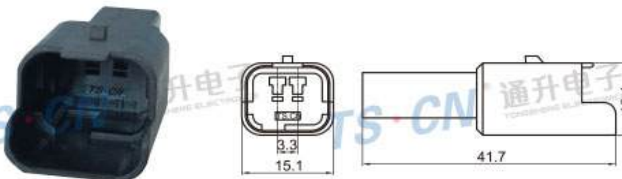
Type: TS30067-02P-11-1 Material: PA66 GF30% Matching Terminal: TSZ144
