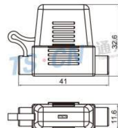
Type: TSBX32 Material: PA66 Matching Terminal: TSH634
