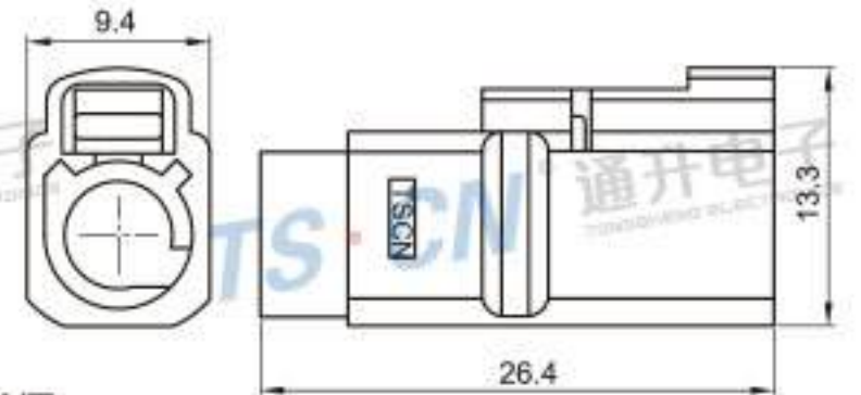
Type: TSVW20-01PF-AT-WT Material: PA66 GF30% Matching Terminal: TSTF0025 / TSTF0026
