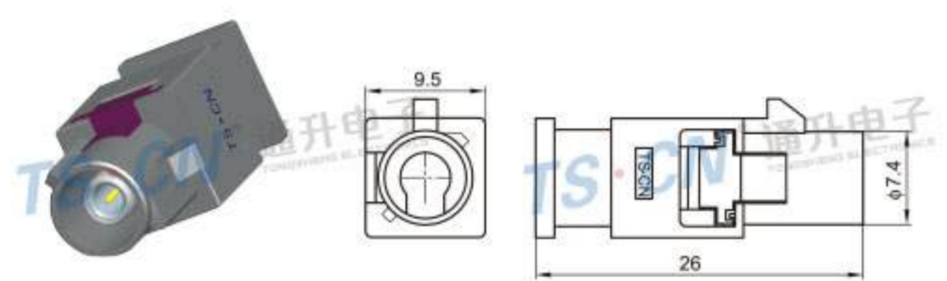
Type: TSVW10-01PM-AT-GY Material: PA66 Matching Terminal: TSTM0019 / TSTM0020
