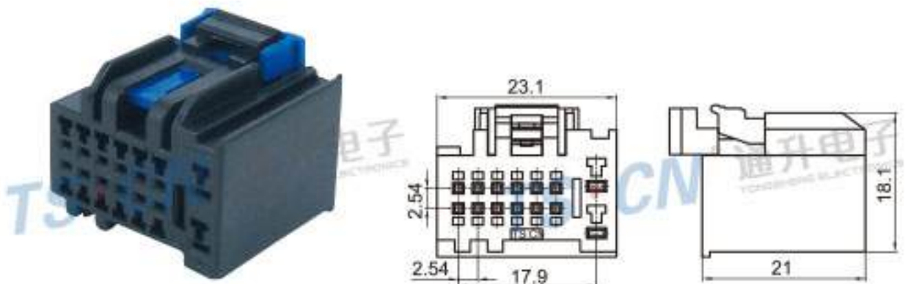
Type: TS2105-14P-21-1 Material: PA66 GF30% Matching Terminal: TSH006/TSH009
