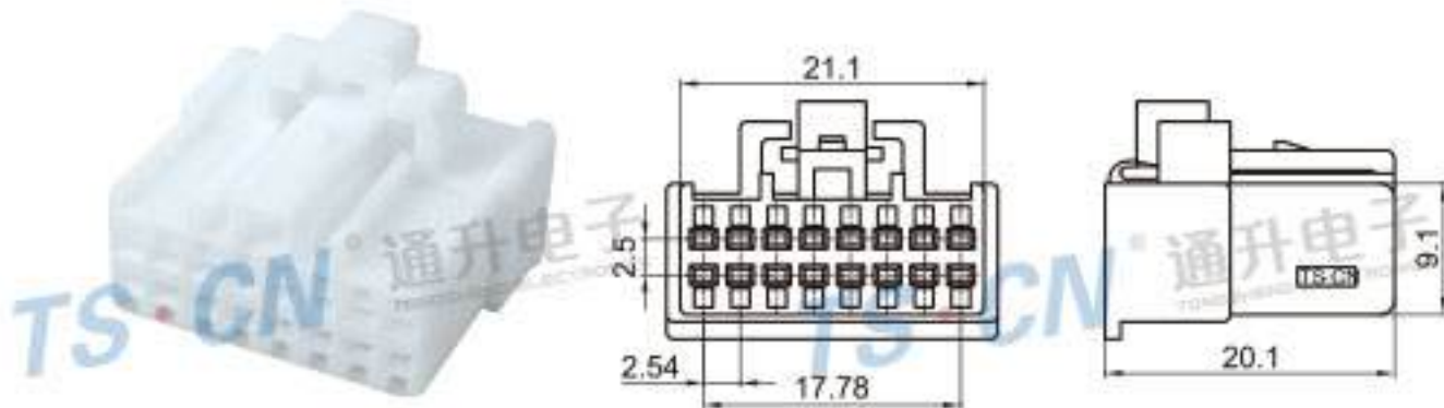
Type: TSPAN16-16P-21 Material: PA66 Matching Terminal: TSH053
