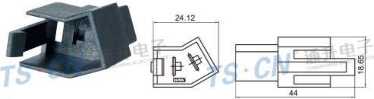
Type: TSLB30-02P-11 Material: PA66 GF30% Matching Terminal: TSZ538
