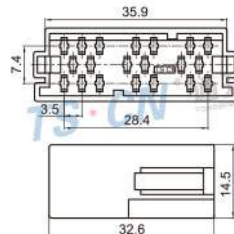
Type: TSAD20-20P-11 Material: PA66 Matching Terminal: TSZ040
