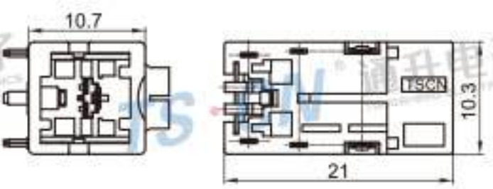
Type: TS30211-02PM-PKB-1 Material: PBT GF15% Matching Terminal: TSPM0266~TSPM0269
