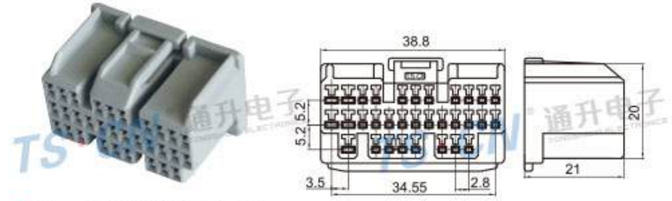
Type: TSWH104-32P-21 Material: PA66 Matching Terminal: TSH009 / TSH076
