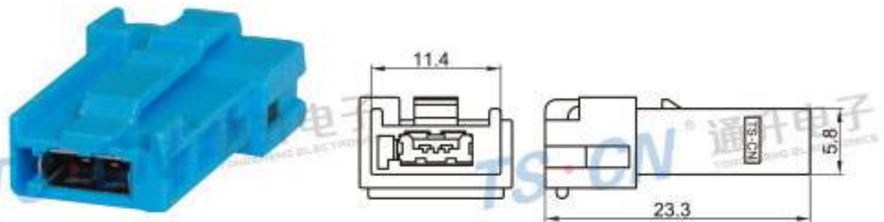
Type: TSKC3123-02PF-AT-1 Material: PA66 GF30% Matching Terminal: TSTF0022 / TSTM0006
