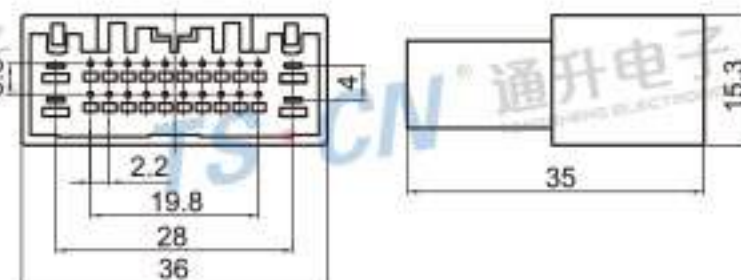
Type: TS30131-24P-11 Material: PA66 Matching Terminal: TSZ559 / TSZ208B
