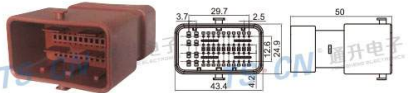
Type: TS30245-48P-11-2 Material: PA66 GF30% Matching Terminal: TSZ040B / TSZ208
