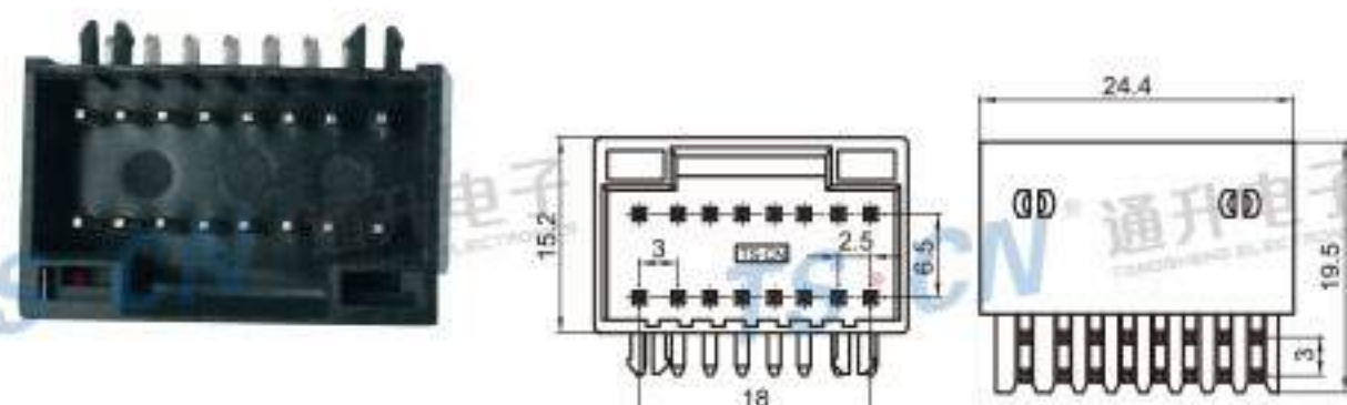
Type: TSALP-16PM-PKB Material: PBT GF30% Matching Terminal: TSPM0167 / TSPM0168
