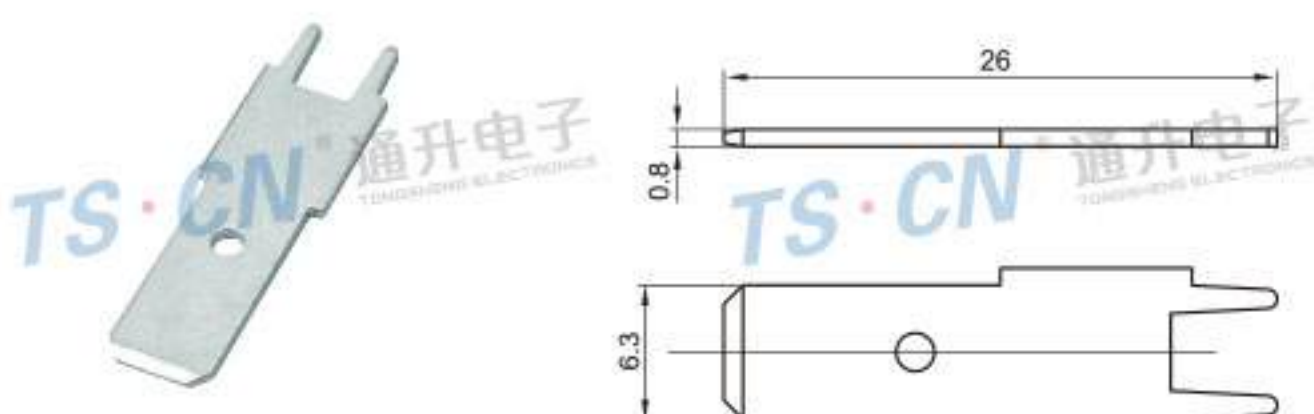
Type: TS623 Material: Brass
