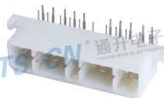
Type: TS1002-21PM-PKB Material: PA66 Matching Terminal: NIL
