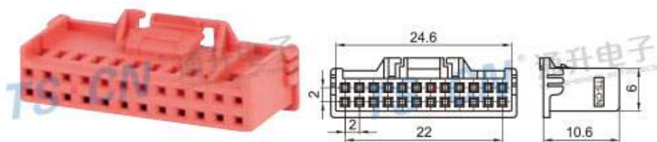
Type: TSQRA3-24P-21RD Material: PA66 GF15% Matching Terminal: TSPHB
