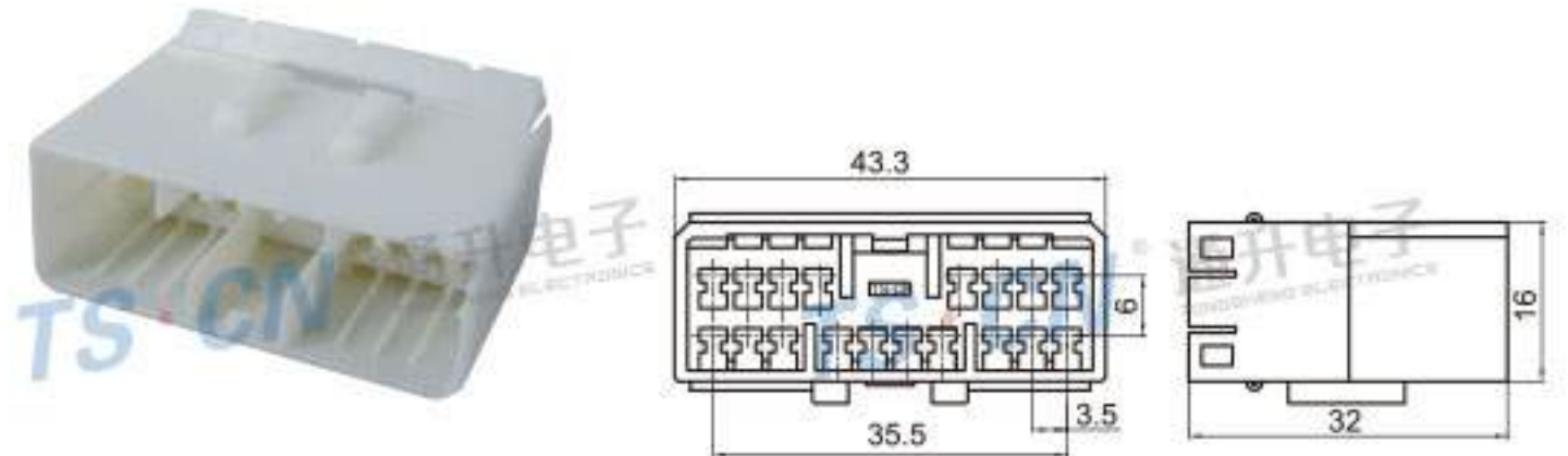
Type: TS8405-18P-11 Material: PA66 Matching Terminal: TSZ011
