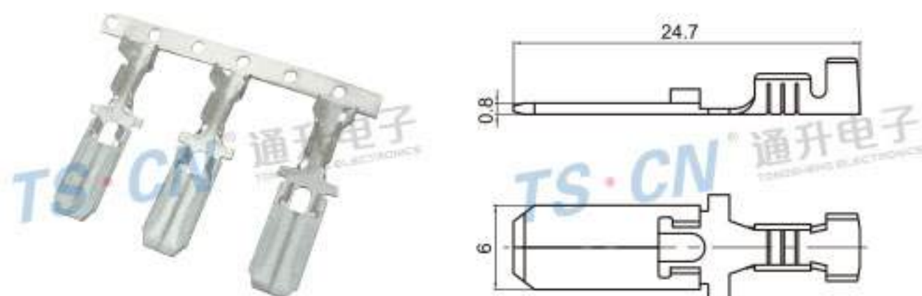
Type: TSZ565 Material: Brass
