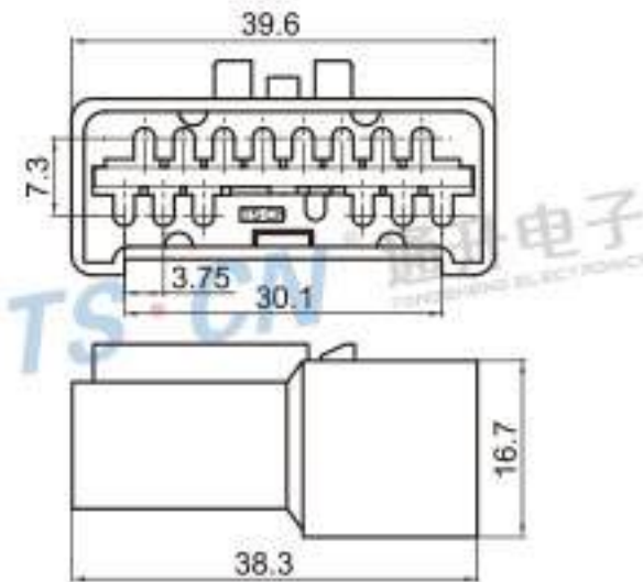
Type: TS5513-14P-11 Material: ABS Matching Terminal: TSZ014
