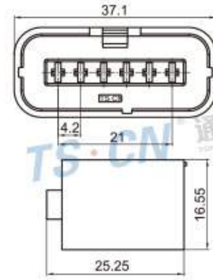
Type: TSVW06-06P-21 Material: PA66 Matching Terminal: TSH054
