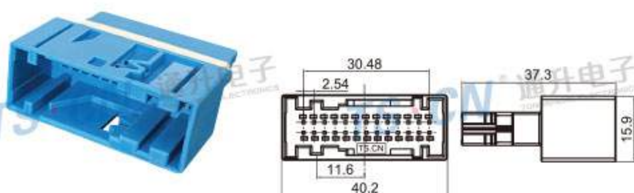
Type: TS30316-26P-11-1 Material: PA66 GF30% Matching Terminal: TSZ616
