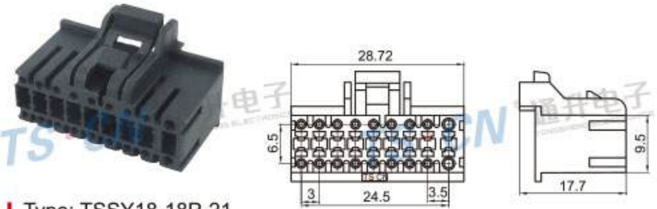
Type: TSSY18-18P-21 Material: PA66 Matching Terminal: TSH031
