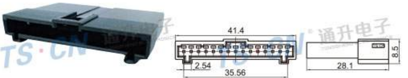
Type: TS30048-15P-11 Material: PA66 GF30% Matching Terminal: TSZ208
