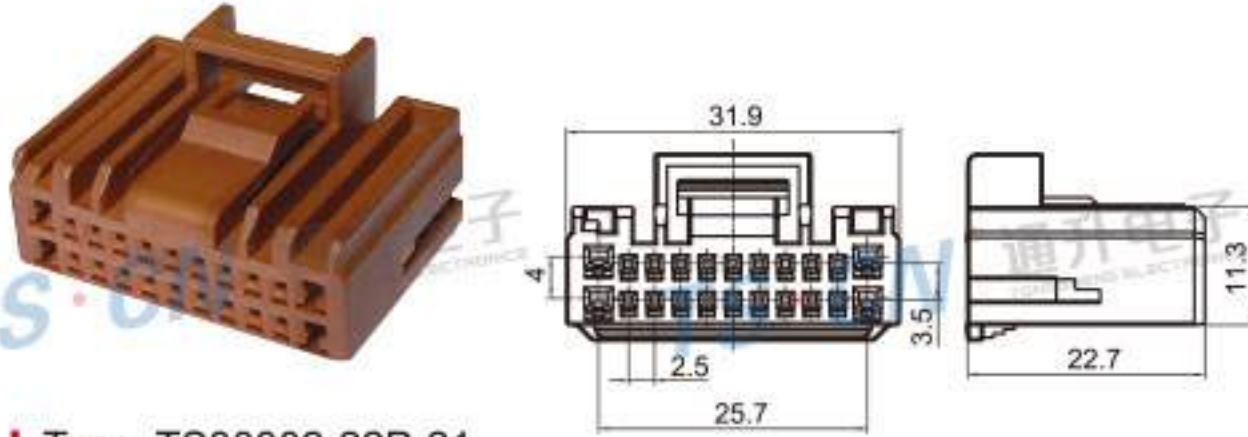
Type: TS30302-22P-21 Material: PBT Matching Terminal: TSH651 / TSH624
