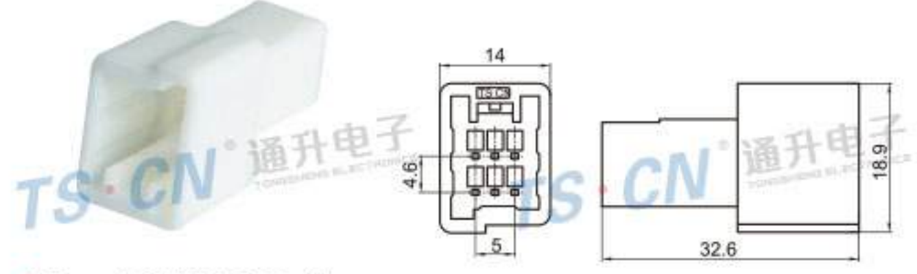
Type: TSTA06-06P-11 Material: PA66 Matching Terminal: TSZ145
