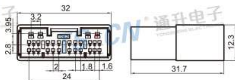
Type: TS30101-28P-11 Material: PA66 Matching Terminal: TSZ562 / TSZ556
