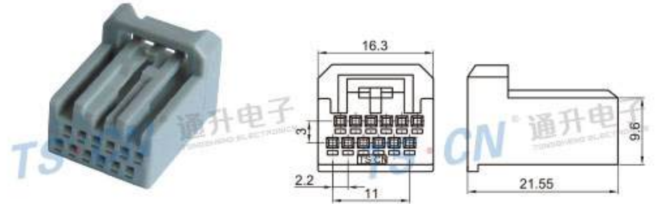
Type: TSCRV12-12P-21 Material: PA66 Matching Terminal: TSH143
