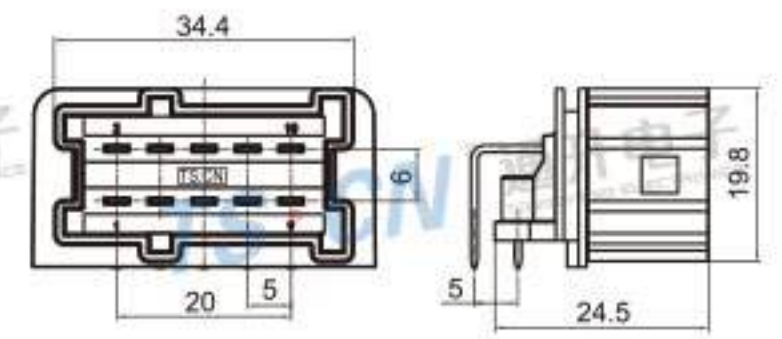
Type: TS30310-10PM-PKB Material: PBT GF15% Matching Terminal: TSPM0314 / TSPM0315
