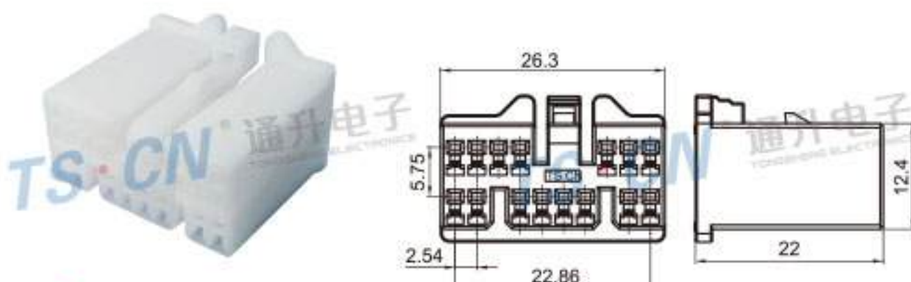
Type: TS8112-15P-21 Material: PA66 Matching Terminal: TSH076
