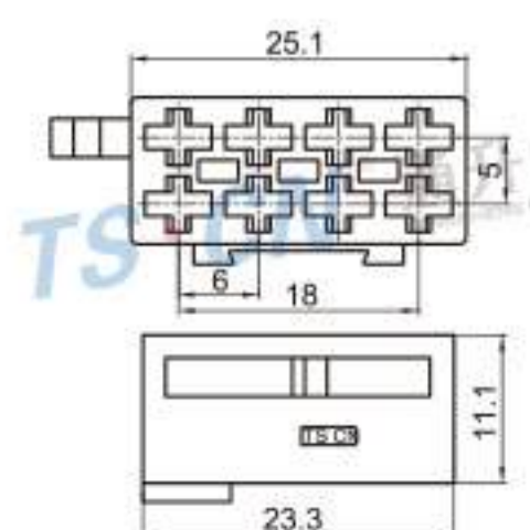
Type: TS1784A-08P-21-2BK Material: PA66 Matching Terminal: TSH019
