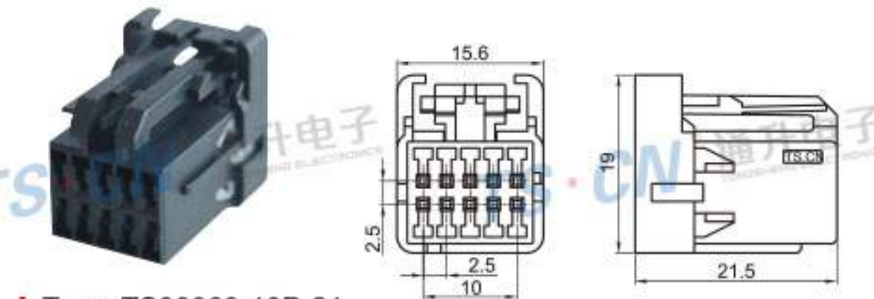
Type: TS30063-10P-21 Material: PA66 Matching Terminal: TSH592
