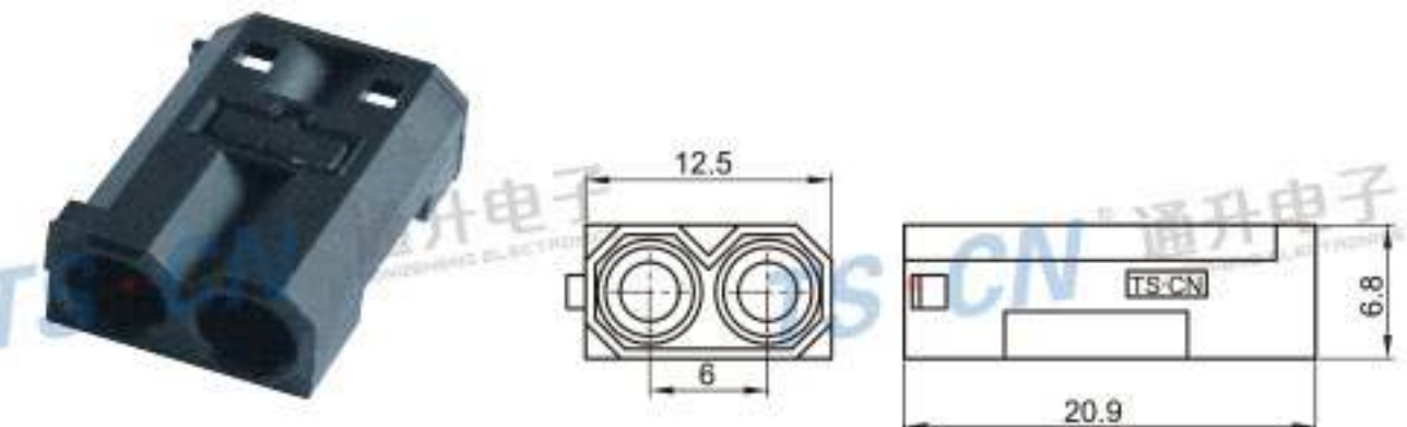
Type: TSBMGQ-A Material: PA66 GF15% Matching Terminal: TSBMGQ-B
