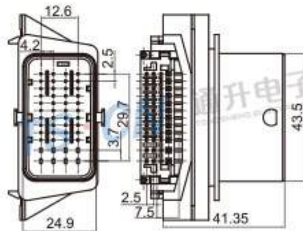
Type: TS30245-48PM-PKB Material: GF30% PBT Matching Terminal: TSPM0289-TSPM0296
