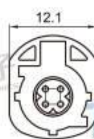
Type: TSVW10-04PM-AT-5BL Material: PA66 GF30% Matching Terminal: TSPM0021~TSPM0025
