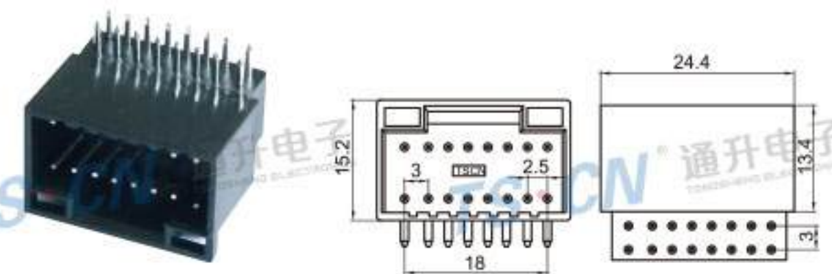
Type: TSALP-16PM-PKB-1 Material: PBT GF30% Matching Terminal: TSPM0167 / TSPM0168
