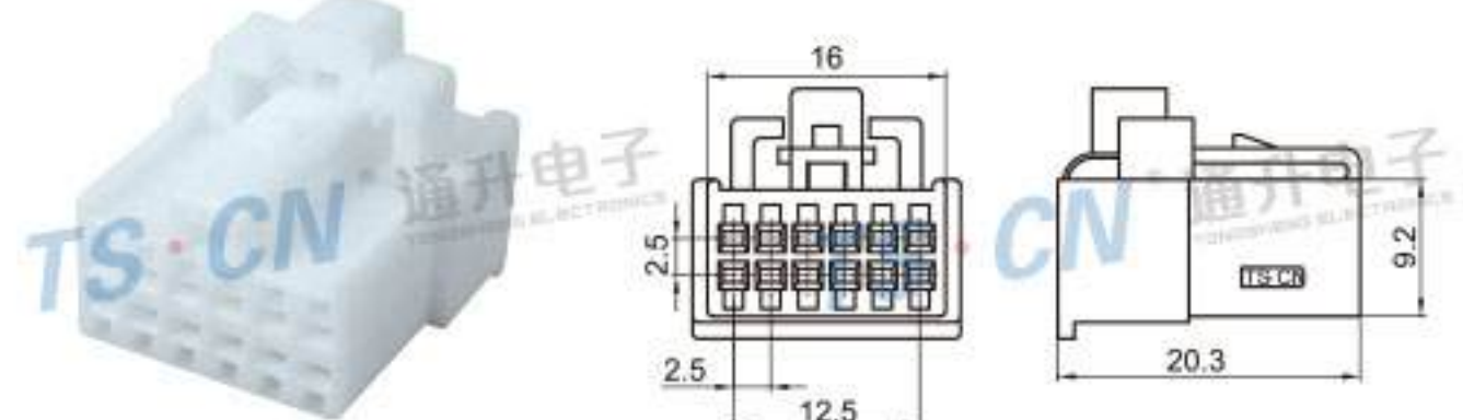
Type: TSPAN12-12P-21 Material: PA66 Matching Terminal: TSH053
