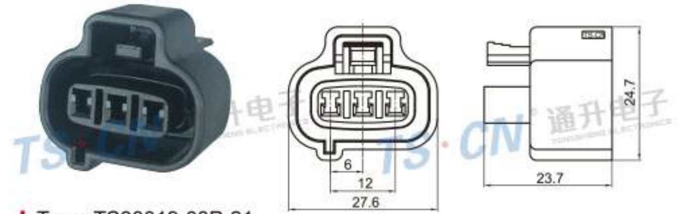
Type: TS30019-03P-21 Material: PA66 Matching Terminal: TSH064
