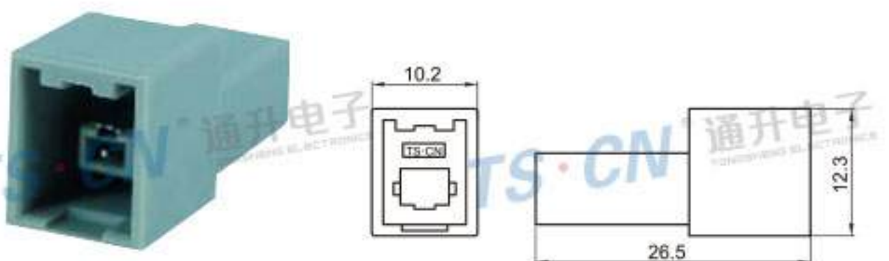
Type: TSK111-01PM-AT Material: PA66 Matching Terminal: TSTM0001 / TSTM0002
