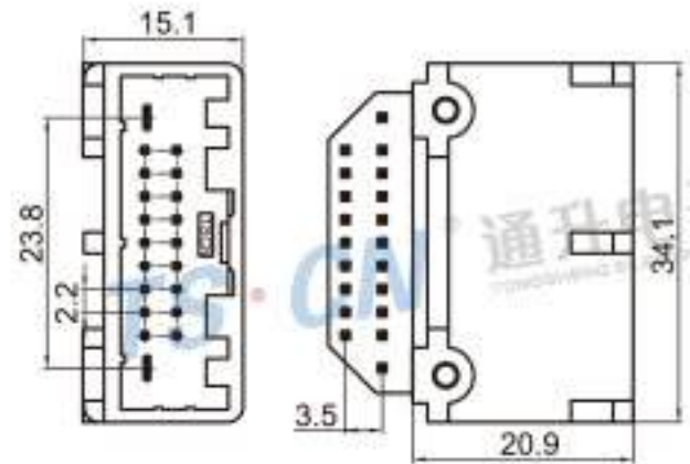
Type: TS7552-20PM-PKB Material: PA66 Matching Terminal: TSPM0002 / TSPM0040 / TSPM0041
