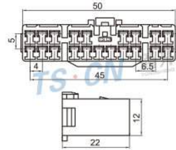
Type: TS7712-20P-21 Material: PA66 Matching Terminal: TSH064
