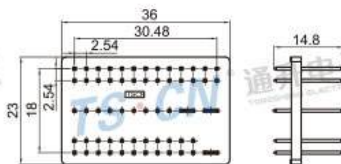
Type: TS30248-60PM-PKS Material: PBT GF30% Matching Terminal: TSPM0198 / TSPM0297
