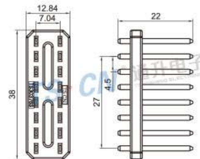
Type: TS30376-16PM-PKS Material: PA66 GF30% Matching Terminal: TSPM0340
