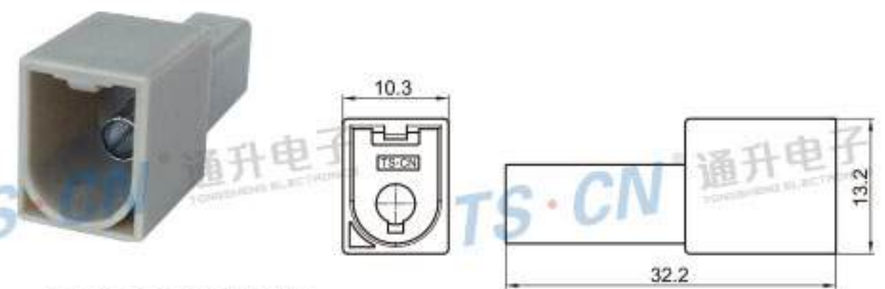
Type: TS1068-01PM-AT-3 Material: PA66 GF30% Matching Terminal: TSTM0003 / TSTM0004
