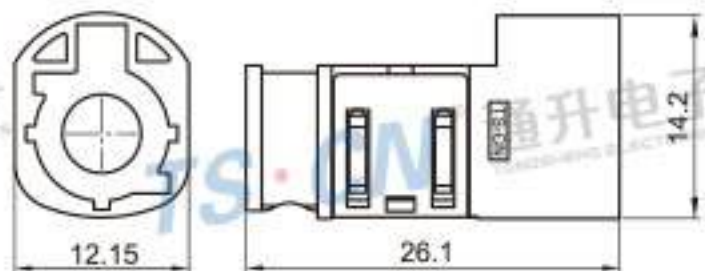
Type: TSVW10-04PM-AT-5BL-1 Material: PA66 GF15% Matching Terminal: TSPM0175 / TSTM0051
