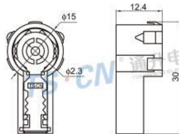
Type: TSVW03-01PM-AT Material: ABS Matching Terminal: TSTM0023 / TSTM0024
