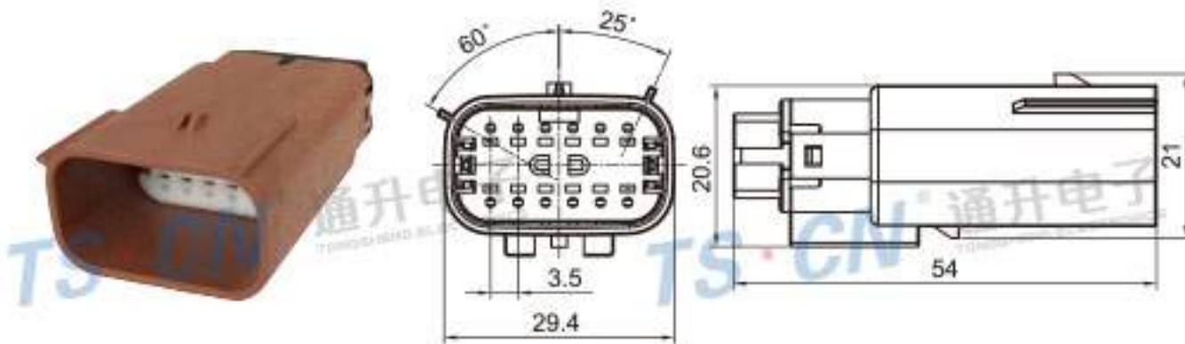
Type: TS30359-12P-11-2 Material: PA66 GF30% Matching Terminal: TSZ144A
