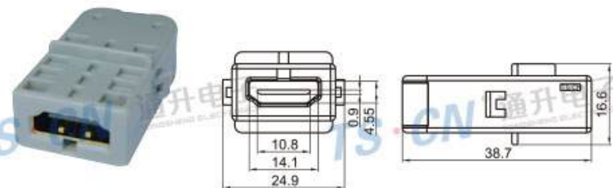
Type: TS30026-19PF-AH Material: PA66 Matching Terminal: TSAF0027 / TSAF0028
