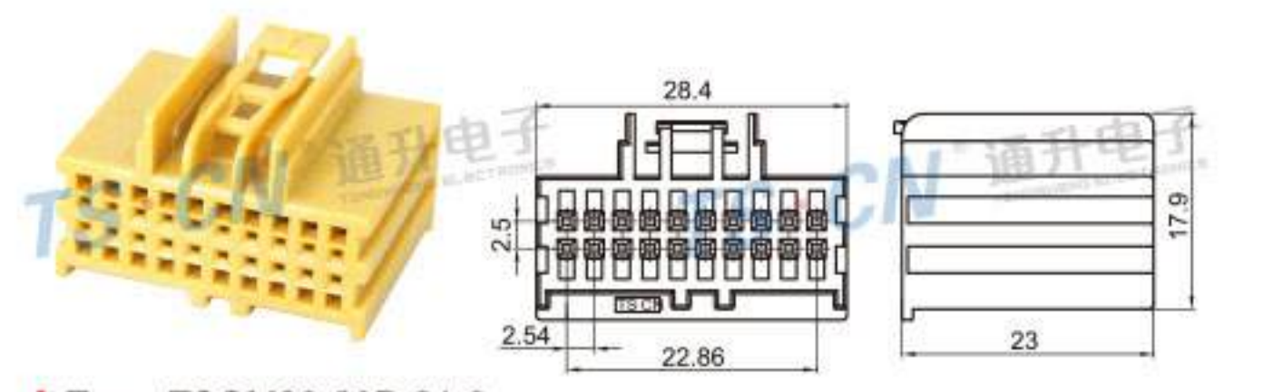
Type: TSGM20-20P-21-3 Material: PA66 GF30% Matching Terminal: TSH143
