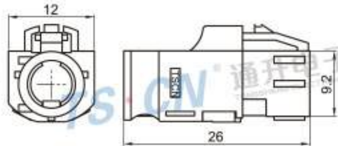
Type: TSVW20-04PF-AT-5OR-1 Material: PA66 GF30% Matching Terminal: TSTF0051 / TSTF0052
