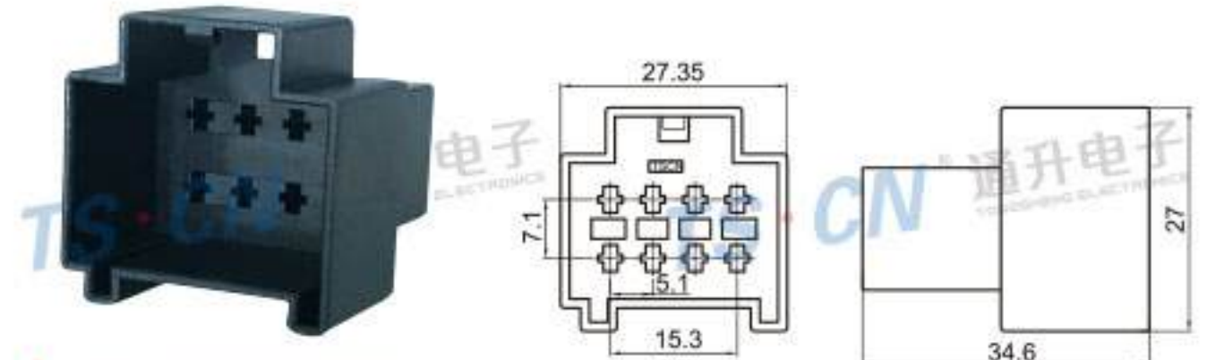
Type: TS30174-08P-11 Material: PA66 Matching Terminal: TSH019
