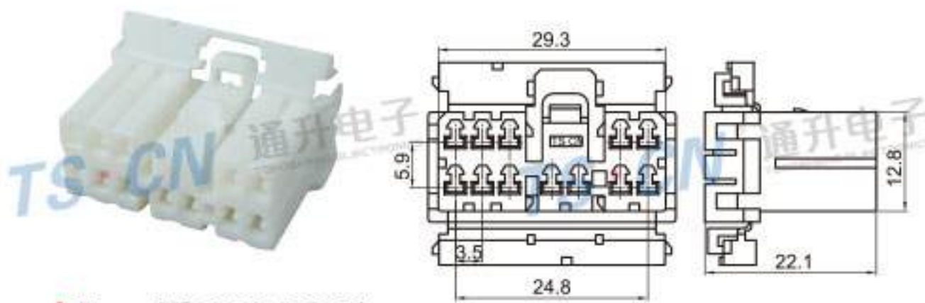
Type: TS7901-12P-21 Material: PA66 Matching Terminal: TSH016
