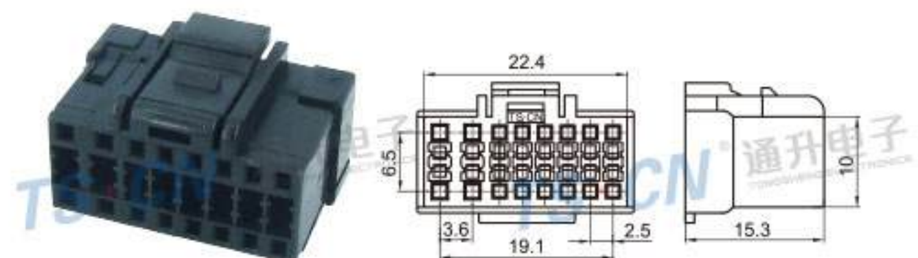
Type: TSPAN01A-16P-21 Material: PA66 GF30% Matching Terminal: TSH503 / TSH031B
