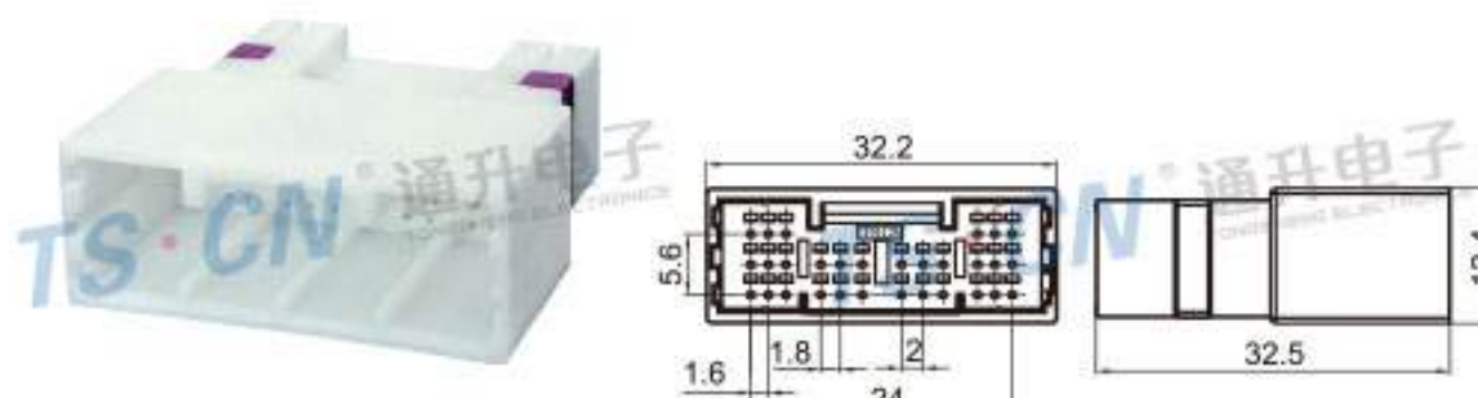
Type: TS30101-30P-11-7 Material: PA66 Matching Terminal: TSZ615
