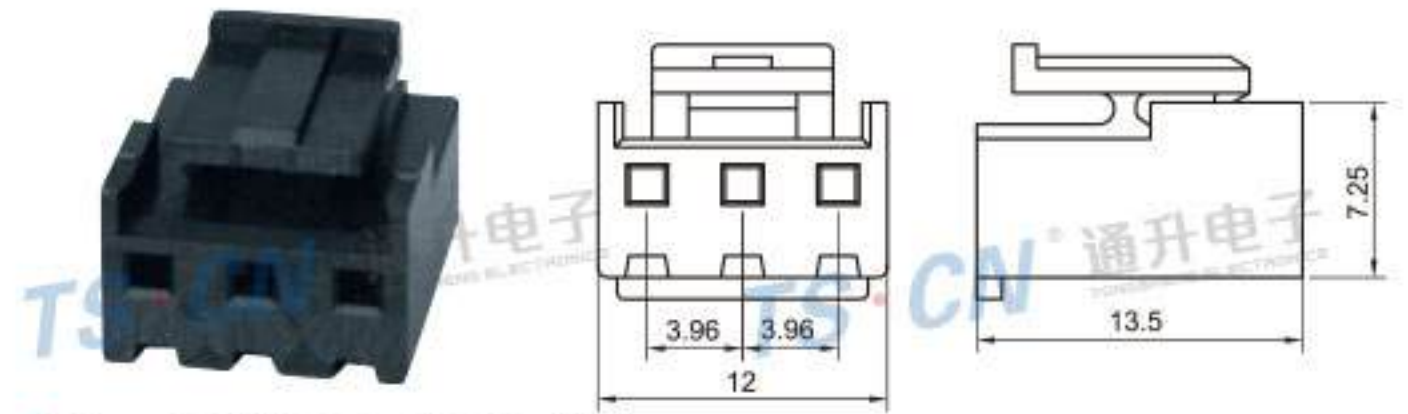
Type: TSVH-03P-21(02P-15P) Material: PA66 Matching Terminal: TSVH
