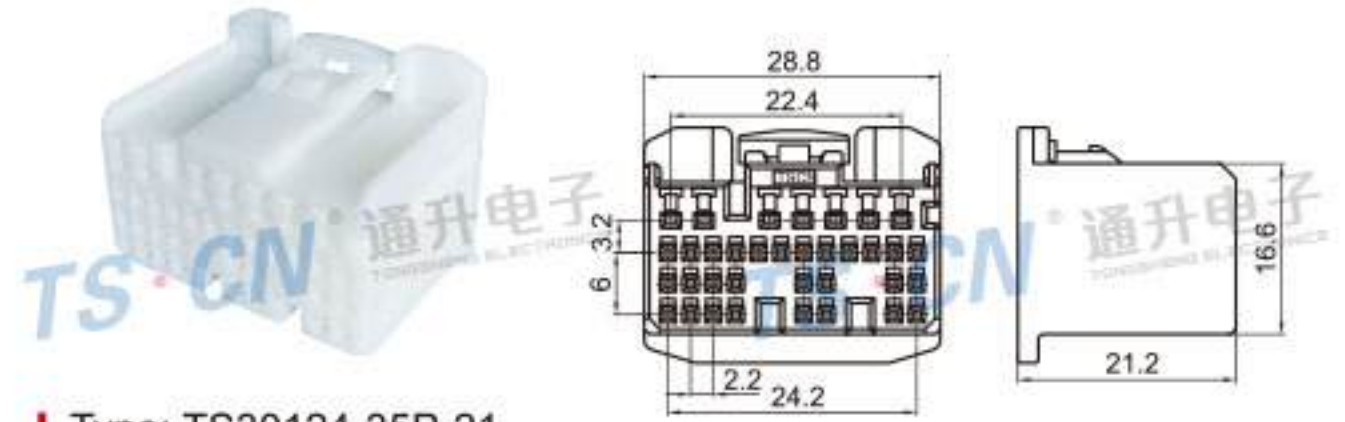
Type: TS30124-35P-21 Material: PA66 Matching Terminal: TSH076 / TSH143
