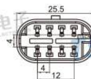
Type: TS30224-08P-11 Material: PA66 GF30% Matching Terminal: TSZ007B
