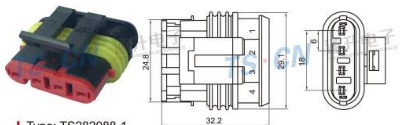
Type: TS282088-1 Material: PA66 Matching Terminal: NIL
