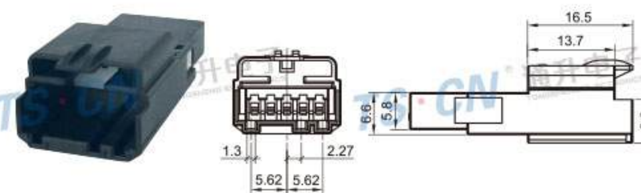
Type: TS30362-05P-11 Material: PA66 GF30% Matching Terminal: TSZ145
