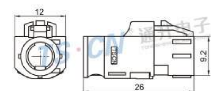
Type: TSVW20-04PF-AT-5GN-1 Material: PA66 GF30% Matching Terminal: TSTF0051 / TSTF0052
