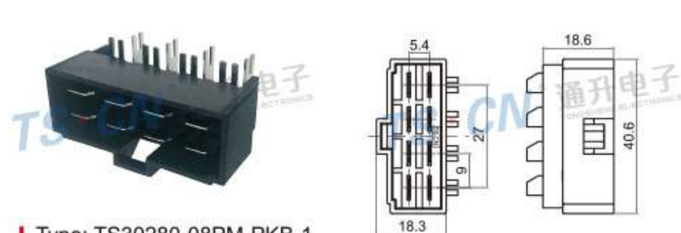
Type: TS30280-08PM-PKB-1 Material: PA66 GF30% Matching Terminal: TSPM0308 / TSPM0309
