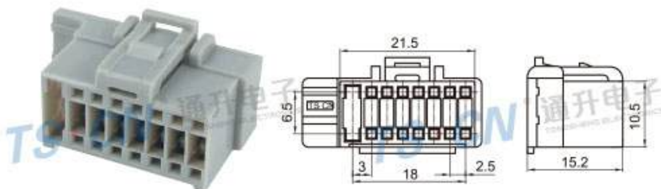
Type: TSPAN16C-16P-21 Material: PA66 Matching Terminal: TSH114 / TSH113
