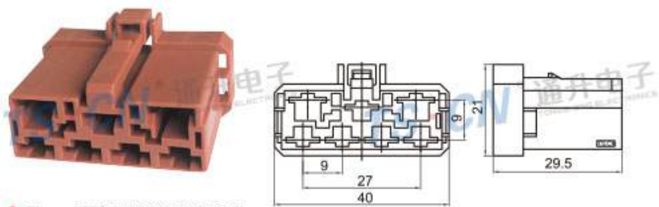
Type: TS30012-07P-21 Material: PA66 Matching Terminal: TSH589A / TSH590
