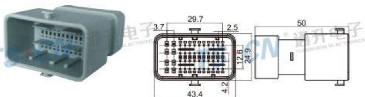
Type: TS30245-48P-11-1 Material: PA66 GF30% Matching Terminal: TSZ040B / TSZ208
