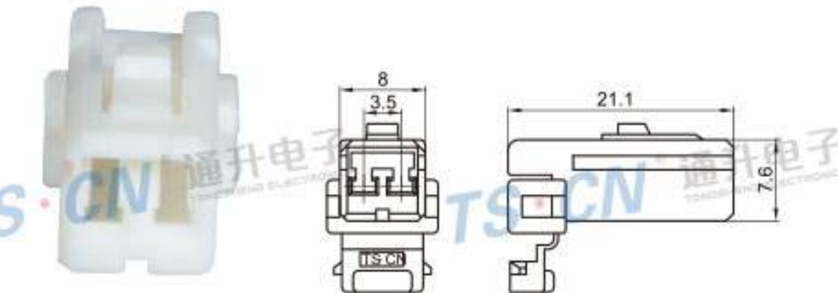
Type: TSLB27-02P-21 Material: PA66 Matching Terminal: TSH016
