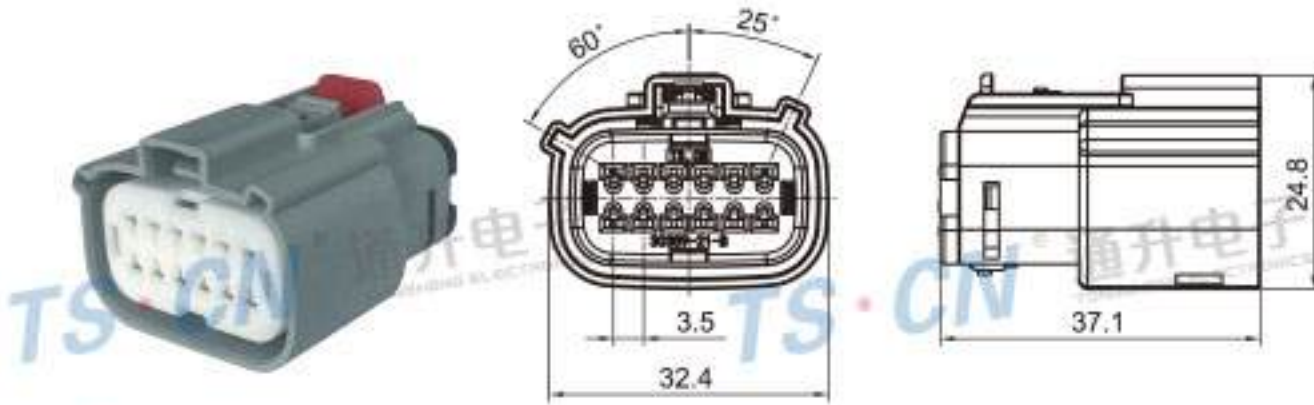
Type: TS30359-12P-21-1 Material: PA66 GF30% Matching Terminal: TSH047
