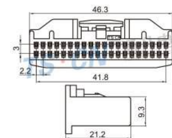
Type: TSTA40-40P-21-5 Material: PA66 Matching Terminal: TSH143
