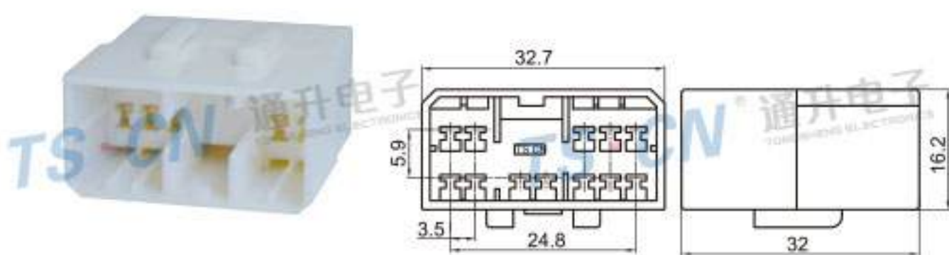
Type: TS7901-12P-11-1 Material: PA66 Matching Terminal: TSZ011
