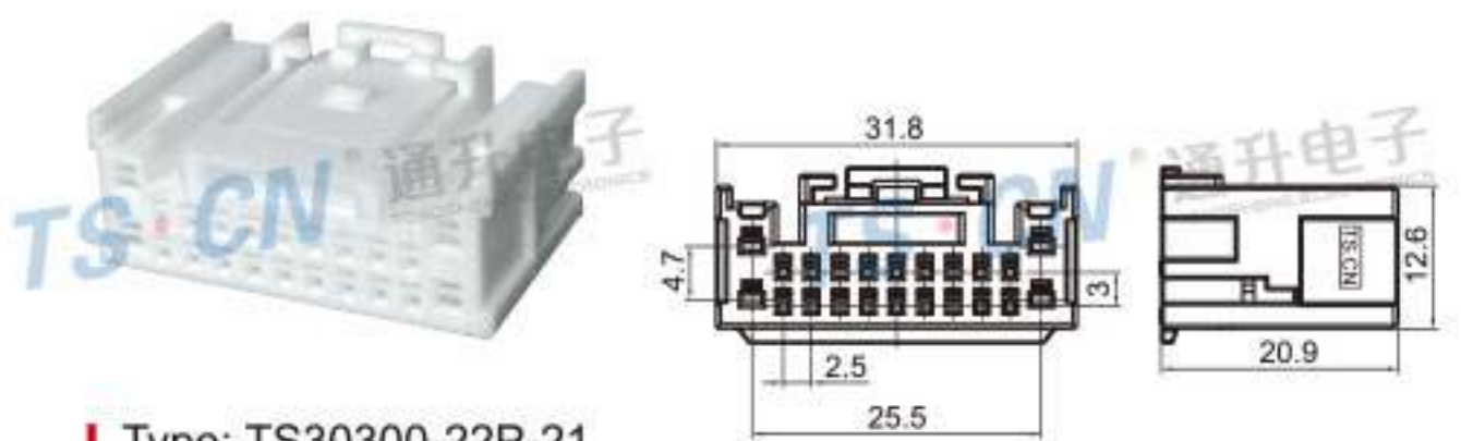
Type: TS30300-22P-21 Material: PBT Matching Terminal: TSH593 / TSH143
