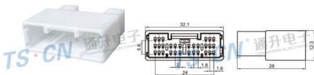
Type: TS30101-30P-11-2 Material: PA66 Matching Terminal: TSZ556
