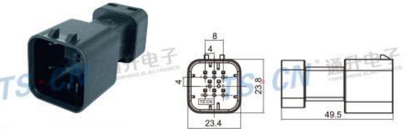
Type: TS30256-08P-11 Material: PBT GF15% Matching Terminal: TSZ072
