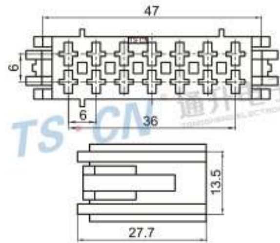
Type: TSBZ14-14P-21 Material: PA66 Matching Terminal: TSH019
