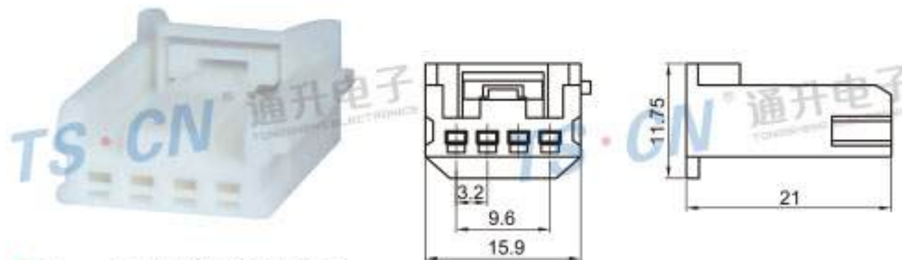
Type: TS30096-04P-21 Material: PA66 Matching Terminal: TSH593
