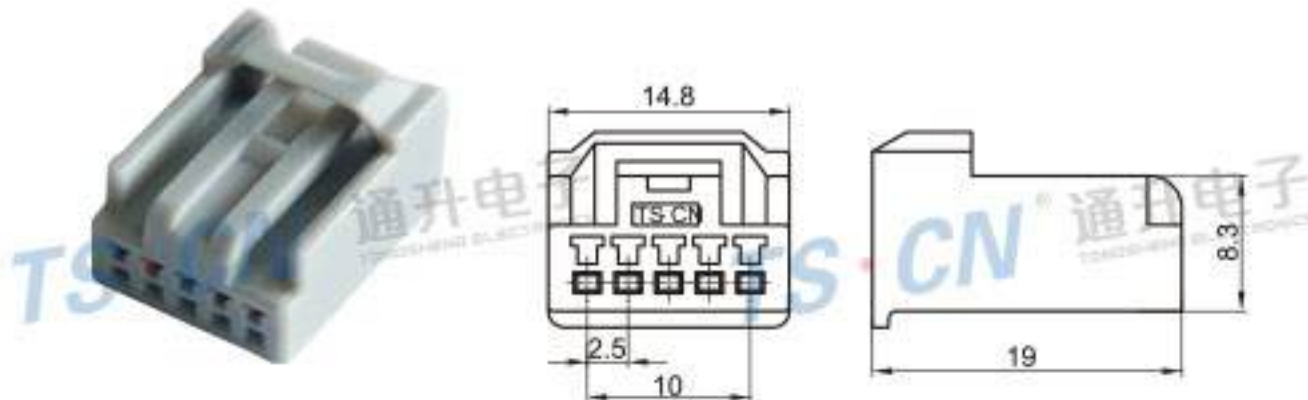
Type: TSTA05-05P-21 Material: PA66 Matching Terminal: TSH076
