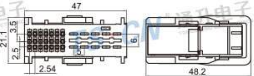
Type: TS30104-31P-21 Material: PBT GF15% Matching Terminal: TSH019 / TSH143
