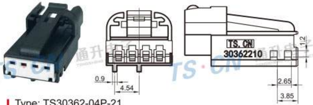
Type: TS30362-04P-21 Material: PA66 GF30% Matching Terminal: TSH006B
