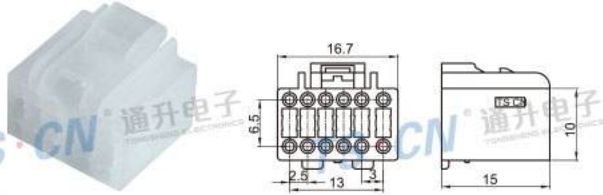
Type: TSALP12-12P-21 Material: PA66 Matching Terminal: TSH031
