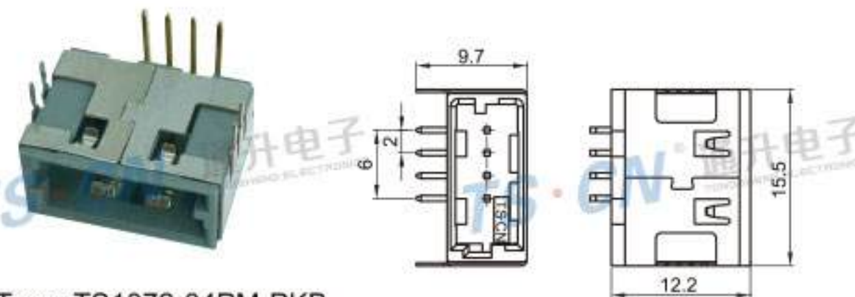
Type: TS1072-04PM-PKB Material: PBT GF15% Matching Terminal: TSPM0243 / TSPM0237-B
