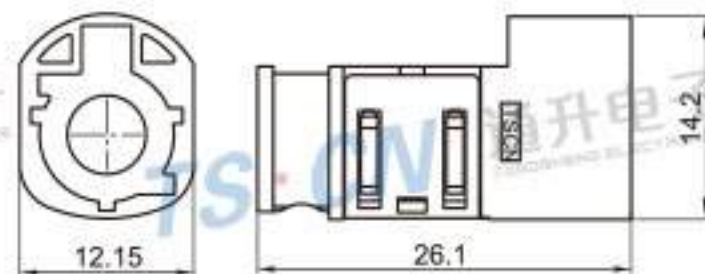
Type: TSVW10-04PM-AT-5BE-1 Material: PA66 GF15% Matching Terminal: TSPM0175 / TSTM0051
