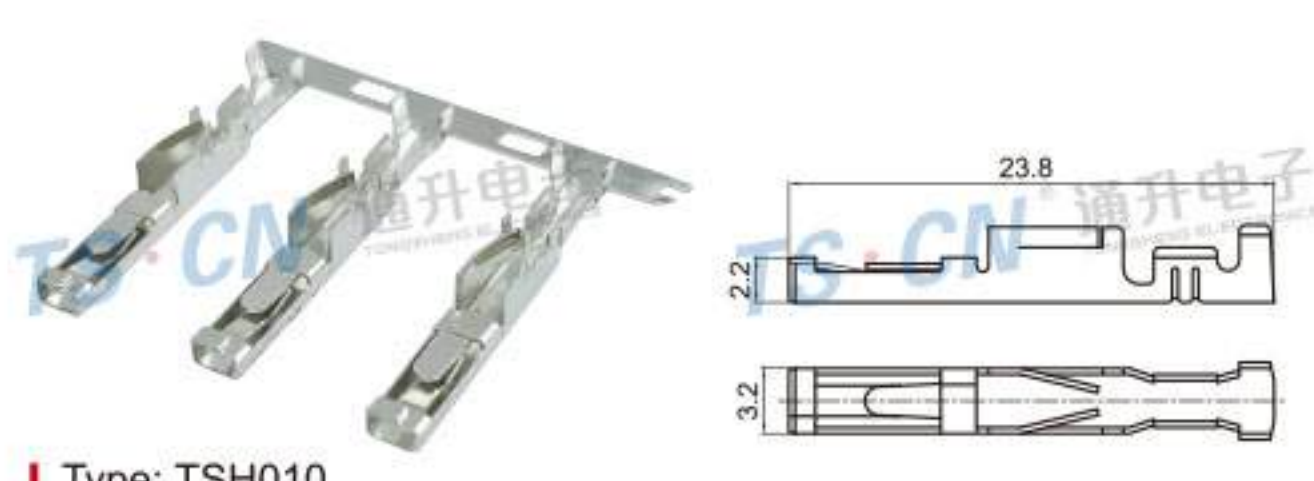
Type: TSH010 Material: Phos.bronze Applicable Thickness: 0.6
