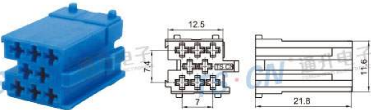
Type: TSVW08-08P-21 Material: PA66 Matching Terminal: TSH054
