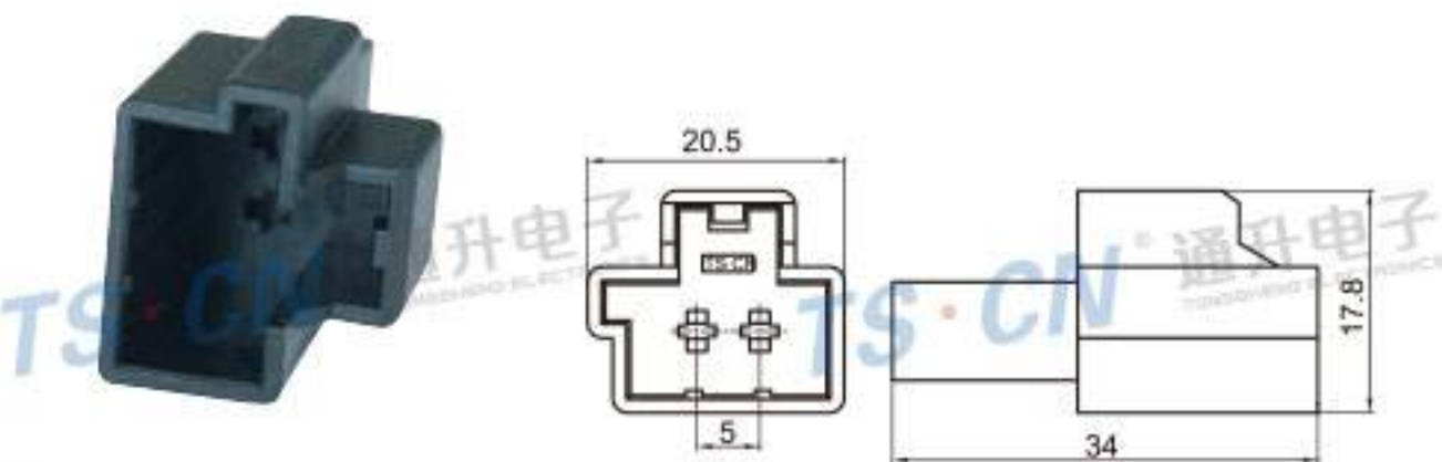
Type: TSLB34-02P-11 Material: PA66 GF30% Matching Terminal: TSZ024
