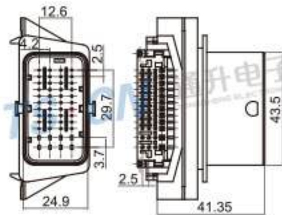
Type: TS30245-48PM-PKB-1 Material: GF30% PBT Matching Terminal: TSPM0289~TSPM0296
