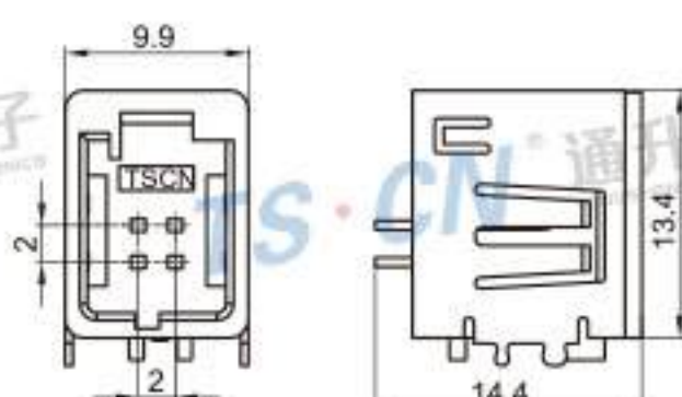
Type: TSMA04-04PM-PS-1 Material: PA66 GF30% Matching Terminal: TSPM0030 / TSPM0029
