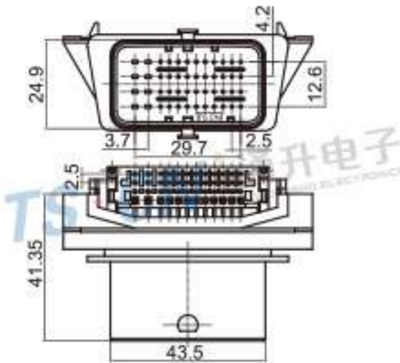
Type: TS30245-32PM-PKB-3 Material: GF30% PBT Matching Terminal: TSPM0289~TSPM0296
