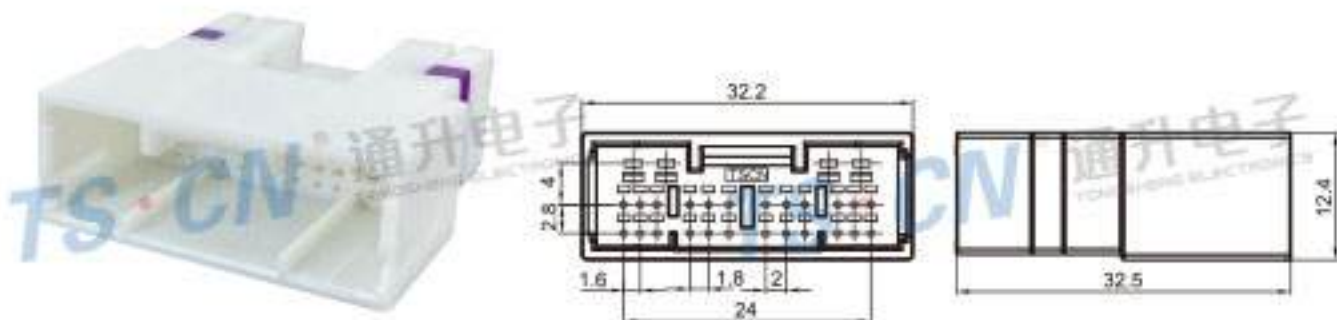
Type: TS30101-28P-11-7 Material: PA66 Matching Terminal: TSZ562 / TSZ615
