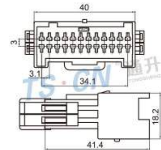
Type: TS2102-24P-11 Material: PA66 Matching Terminal: TSZ013
