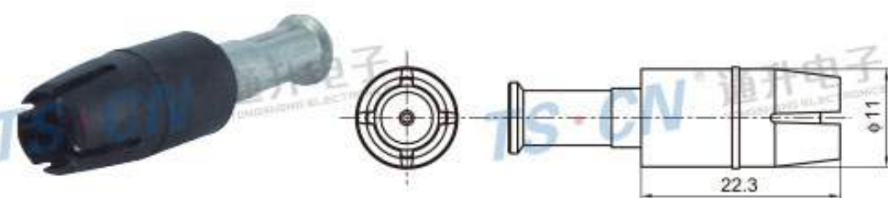
Type: TSFIAT10-01PM-AT Material: PA66 GF30% Matching Terminal: TSTM0012/TSTM0013
