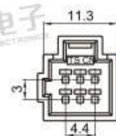
Type: TS3001-06P-11-1 Material: PA66 Matching Terminal: TSZ208
