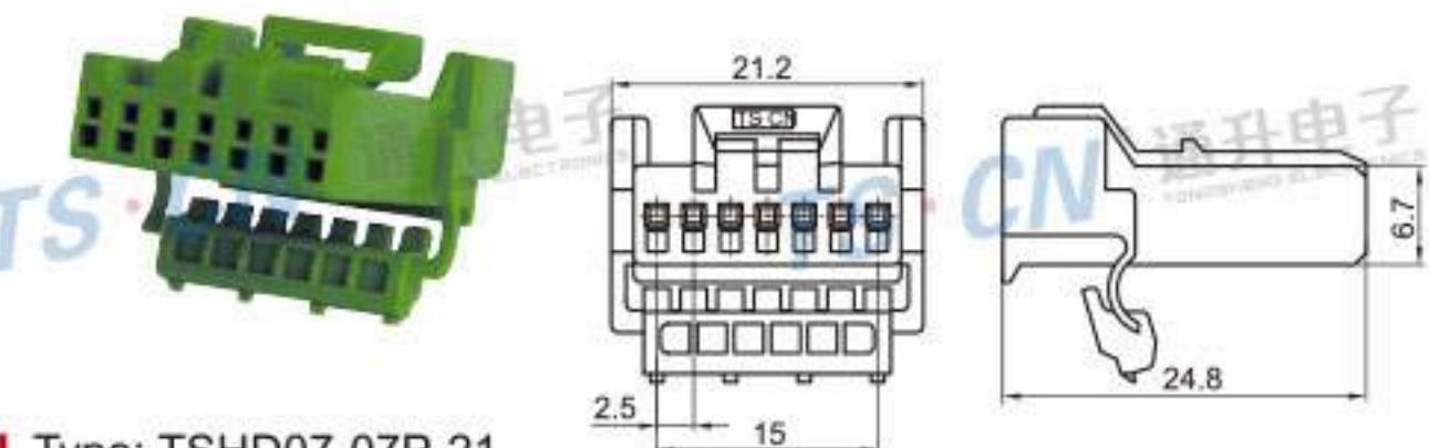
Type: TSHD07-07P-21 Material: PA66 Matching Terminal: TSH066
