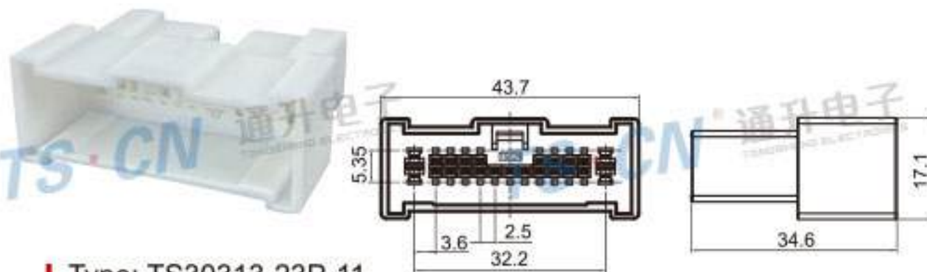
Type: TS30313-23P-11 Material: PA66 Matching Terminal: TSZ009 / TSZ145
