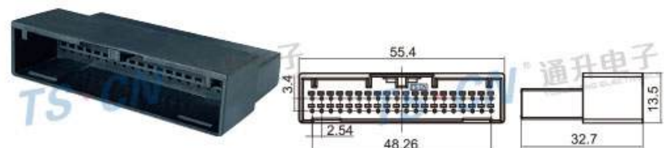
Type: TS30285-40P-11-1 Material: PBT GF30% Matching Terminal: TSZ616
