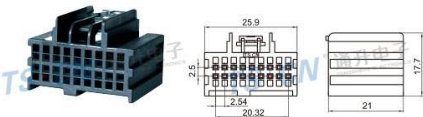
Type: TSGM18-18P-21-1 Material: PA66 GF15% Matching Terminal: TSH143
