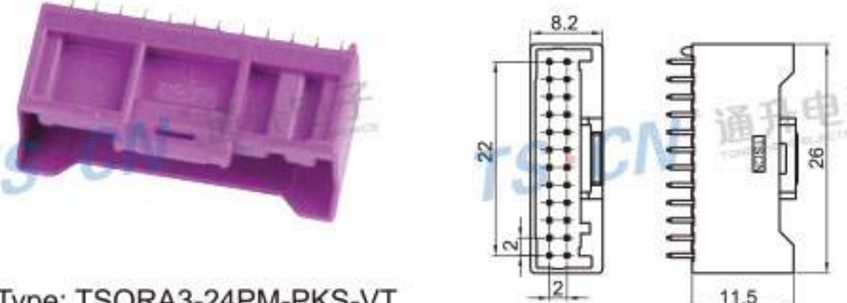
Type: TSQRA3-24PM-PKS-VT Material: PA66 GF15% Matching Terminal: TSPM0145
