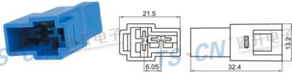
Type: TSLB25-02P-11 Material: PA66 Matching Terminal: TSZ538A
