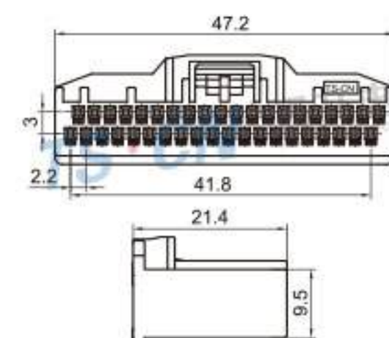
Type: TSCRV40-40P-21 Material: PA66 Matching Terminal: TSH143
