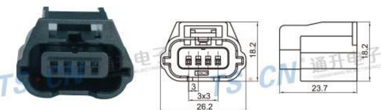
Type: TS30090-04P-21 Material: PA66 GF30% Matching Terminal: TSH143
