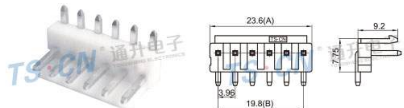
Type: TSVH-06PM-PKB(02P-15P) Material: PA66 Matching Terminal: TSPM0098
