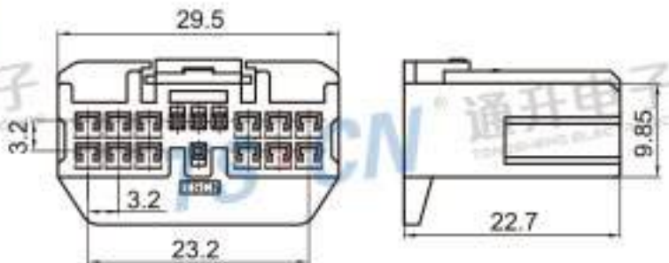
Type: TS30161-16P-21 Material: PA66 GF30% Matching Terminal: TSH541 / TSH143
