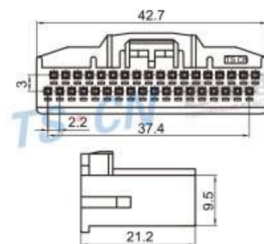
Type: TSCRV36-36P-21-1 Material: PA66 Matching Terminal: TSH143D
