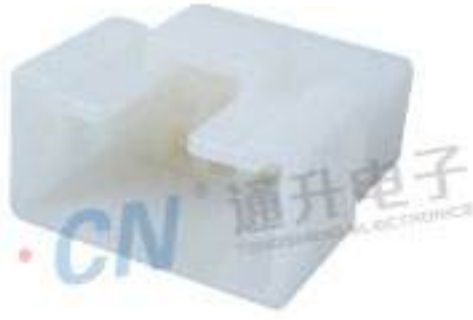
Type: TS1388-10P-11 Material: PA66 Matching Terminal: TS1388
