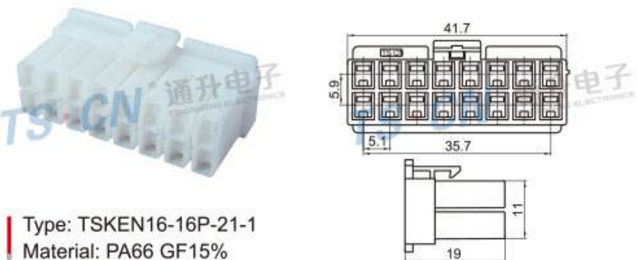
Type: TSKEN16-16P-21-1 Material: PA66 GF15% Matching Terminal: TSH032 / TSH031
