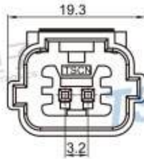
Type: TS30178-02P-21 Material: PA66 GF30% Matching Terminal: TSH143
