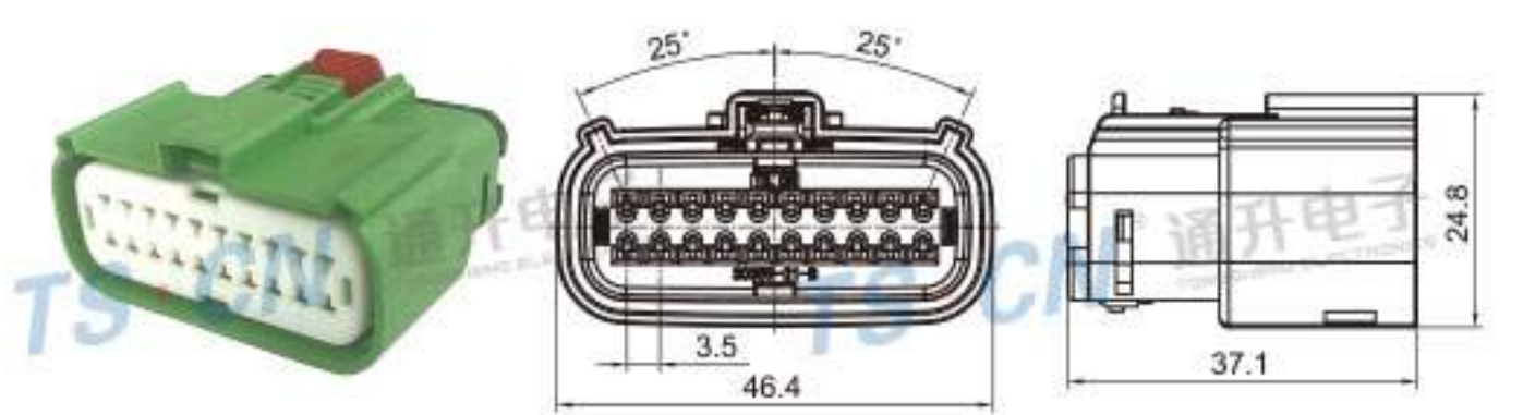
Type: TS30359-20P-21-3 Material: PA66 GF30% Matching Terminal: TSH047
