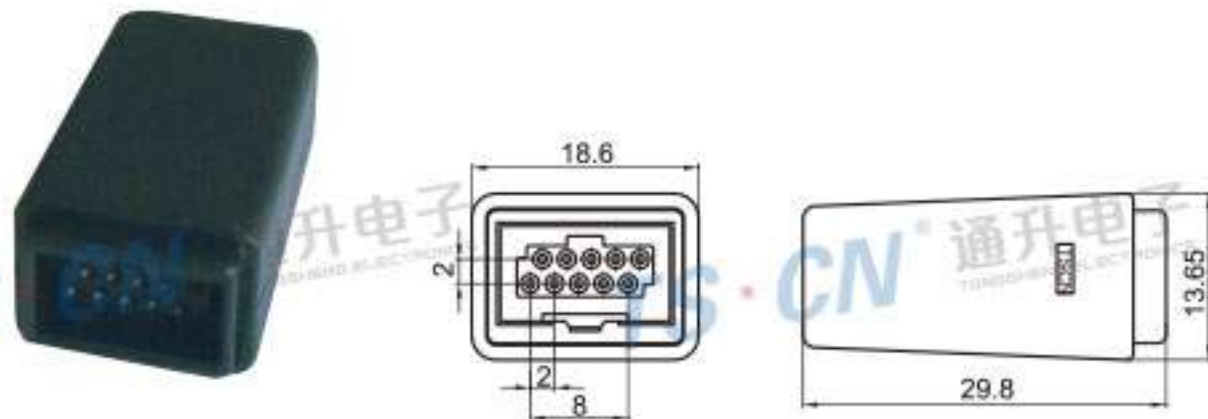
Type: TS3004-10PF-AH Material: PA66 Matching Terminal: TSH501
