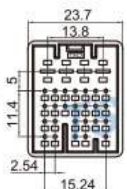
Type: TS30217-30P-11-7 Material: PBT GF15% Matching Terminal: TSDJ615B-2.8*0.8B / TSZ208
