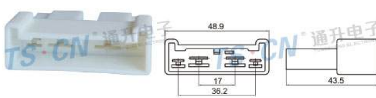
Type: TS30097-04P-11 Material: PBT GF10% Matching Terminal: TSDJ611-7.8D / TS614-G4.8
