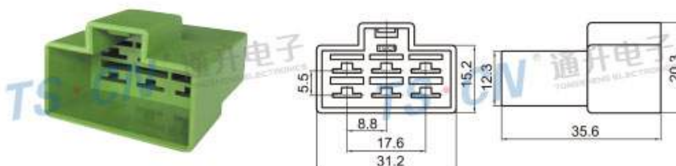
Type: TS30002-06P-11-1 Material: PBT GF15% Matching Terminal: TSZ538-A
