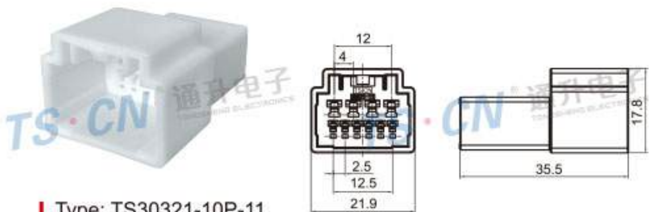
Type: TS30321-10P-11 Material: PBT Matching Terminal: TSZ045 / TSZ018A
