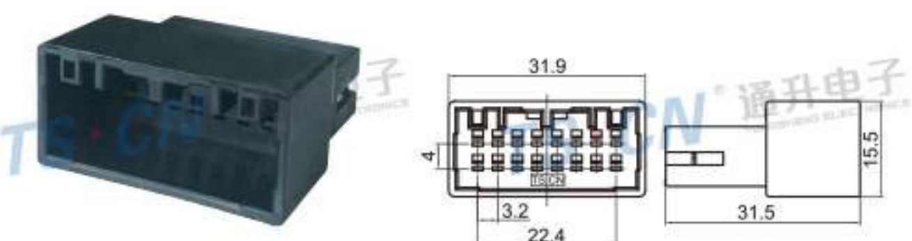
Type: TS30274-16P-11 Material: PBT Matching Terminal: TSZ040
