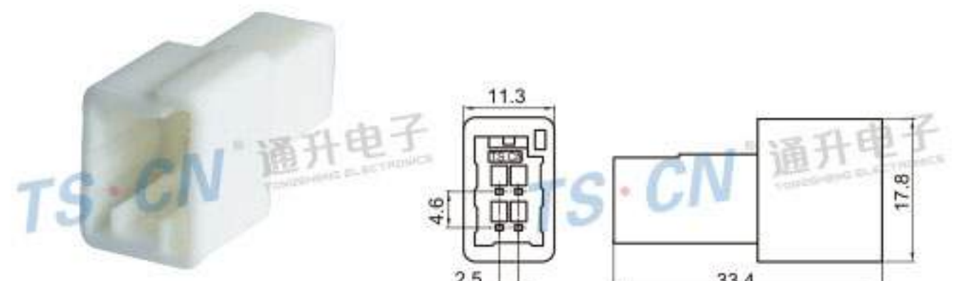
Type: TSTA04-04P-11 Material: PA66 Matching Terminal: TSZ145
