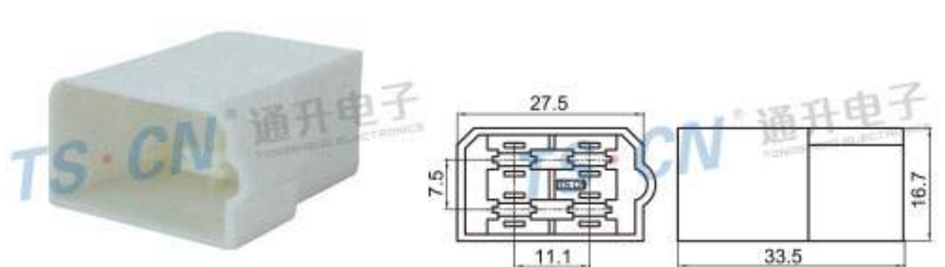
Type: TSFIAT-04P-11 Material: PA66 Matching Terminal: TSZ538A
