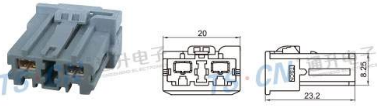
Type: TS30212-04PF-AT Material: PBT Matching Terminal: TSTF0058 / TSTF0059 / TSTF0006
