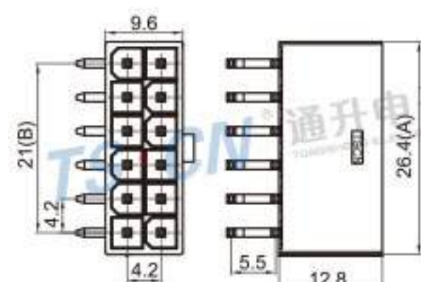
Type: TS5557-12PM-PKB(02P-24P) Material: PA66 Matching Terminal: TSPM0311 / TSPM3012
