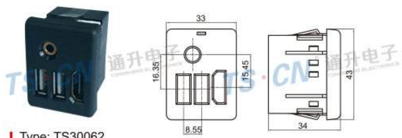
Type: TS30062 Material: PA66 GF30% Matching Terminal: TSHDMI-F / TSUSB-F / TS3.5-F
