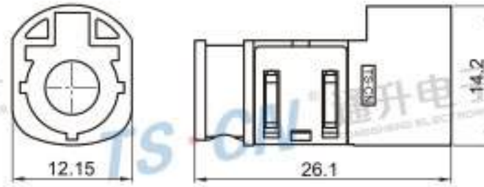
Type: TSVW10-04PM-AT-5BK-1 Material: PA66 GF15% Matching Terminal: TSPM0175 / TSTM0051
