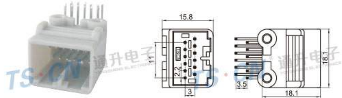
Type: TSCRV-12PM-PKB Material: PA66 Matching Terminal: TSPM0062 / TSPM0063
