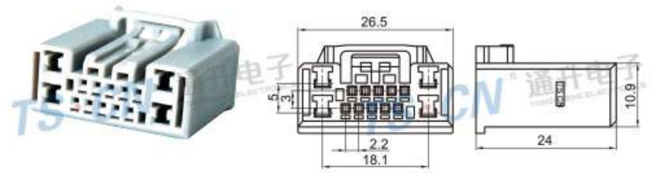
Type: TSCRV14-14P-21 Material: PA66 Matching Terminal: TSH064 / TSH143
