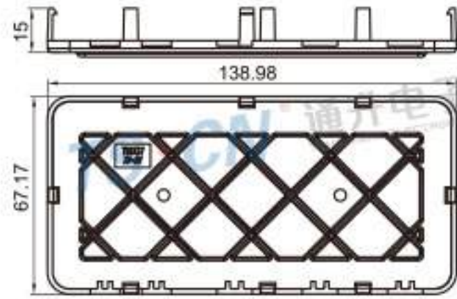
Type: TS BX37 Material: PBT Matching Terminal: NIL
