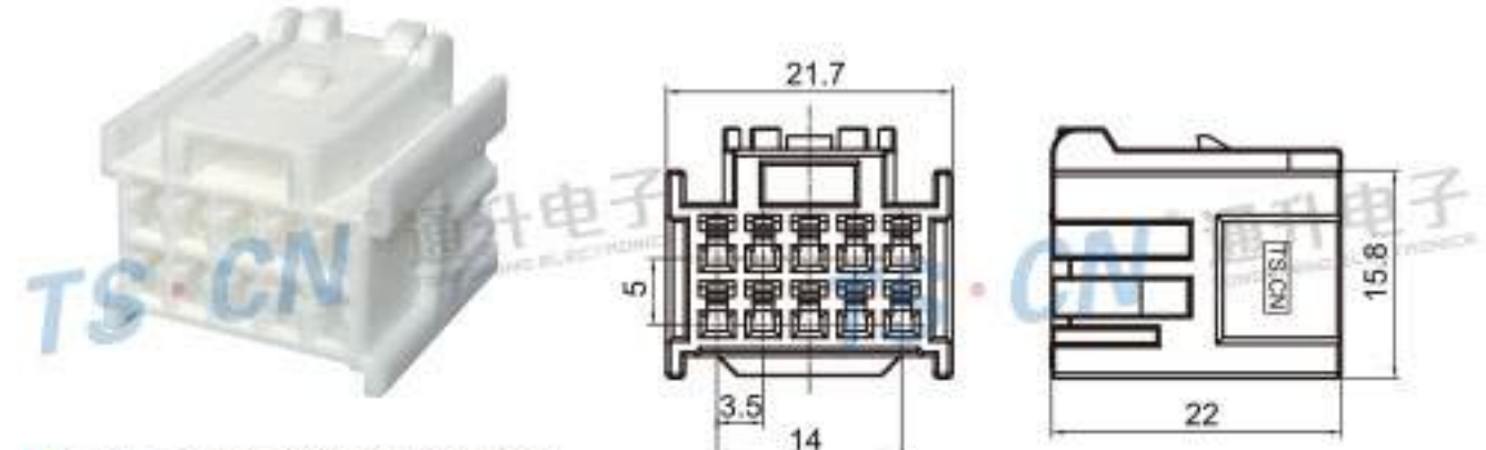
Type: TS30301-10P-21 Material: PBT Matching Terminal: TSH628
