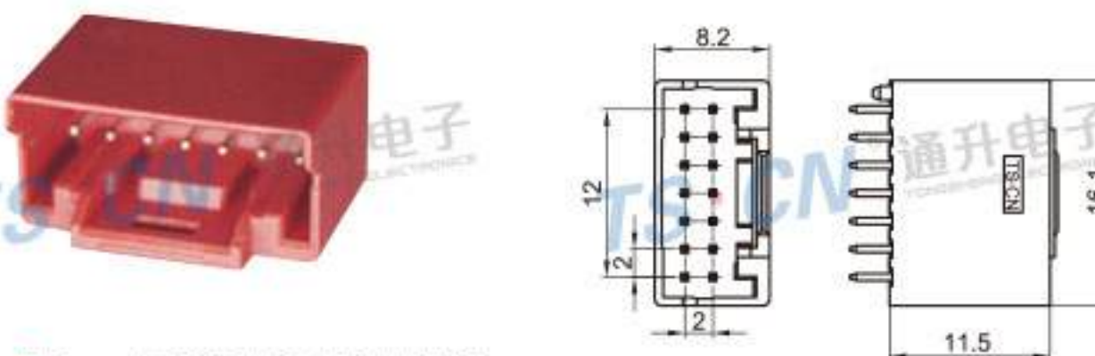
Type: TSQRA3-14PM-PKS Material: PA66 GF30% Matching Terminal: TSPM0145
