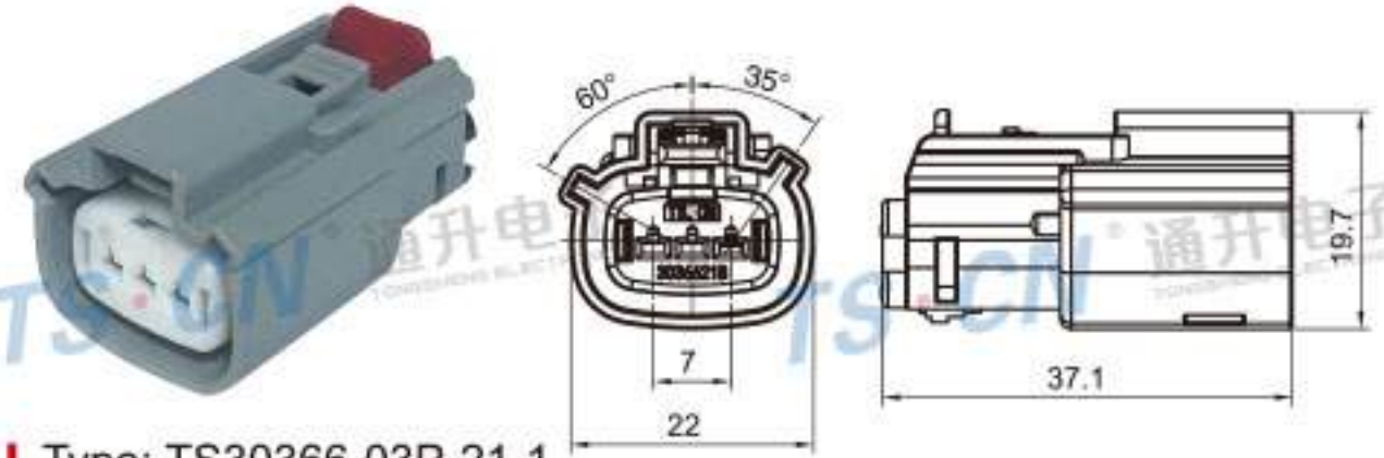
Type: TS30366-03P-21-1 Material: PA66 GF30% Matching Terminal: TSH047
