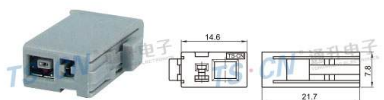
Type: TSHD20-02PF-AT Material: PA66 Matching Terminal: TSH009 / TSTF0001 / TSTF0002
