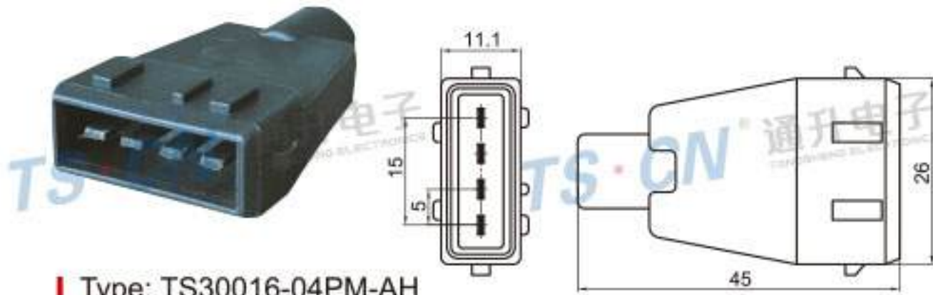
Type: TS30016-04PM-AH Material: ABS Matching Terminal: TSAM0017
