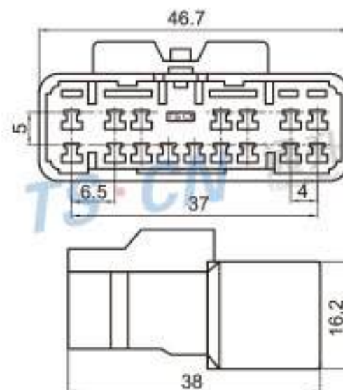
Type: TS7712-16P-11 Material: PA66 Matching Terminal: TSZ045
