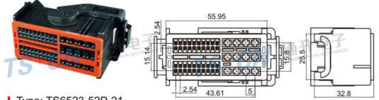
Type: TS6523-52P-21 Material: PA66 GF30% Matching Terminal: TSH019 / TSH143
