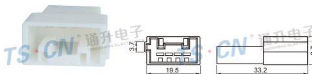
Type: TS30096-04P-11(AD26) Material: PA66 Matching Terminal: TSZ040
