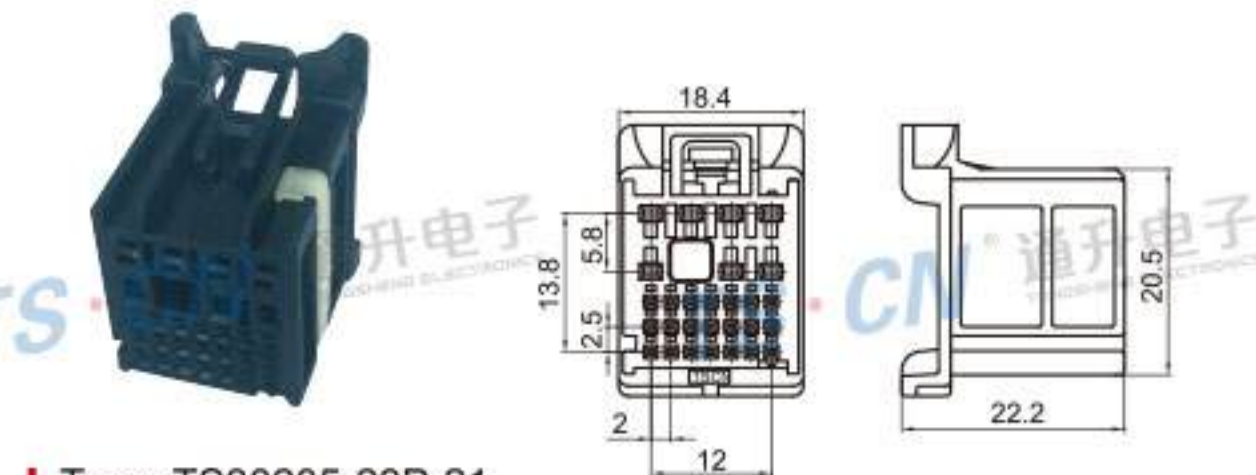
Type: TS30205-28P-21 Material: PA66 Matching Terminal: TSH092 / TSH606
