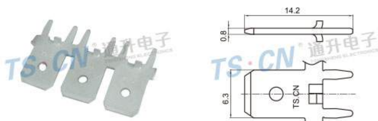
Type: TSZ567 Material: Brass
