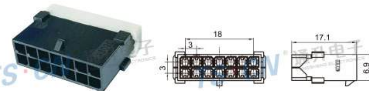
Type: TS43025-14P-11-3(04P-24P) Material: PA66 Matching Terminal: TSZ160
