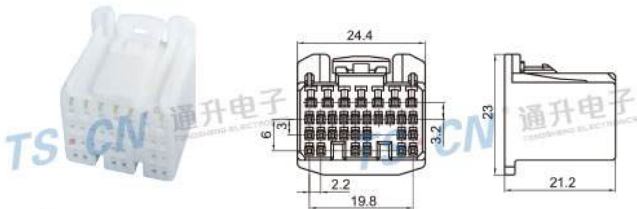
Type: TS30124-31P-21 Material: PA66 Matching Terminal: TSH076 / TSH143
