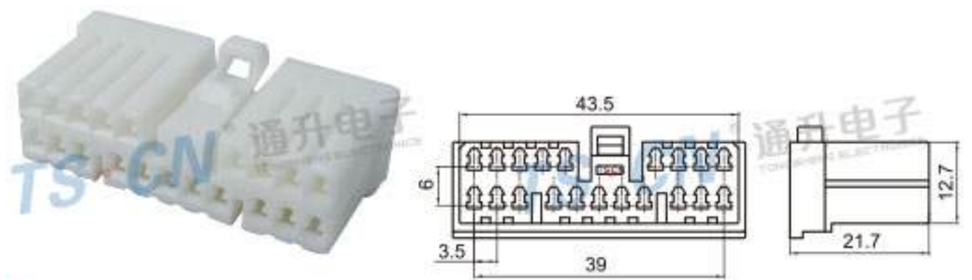
Type: TSDA20-20P-21 Material: PA66 Matching Terminal: TSH016
