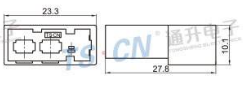
Type: TSNI10-03PM-AT Material: PA66 Matching Terminal: TSZ040 / TSTM0001 / TSTM0002
