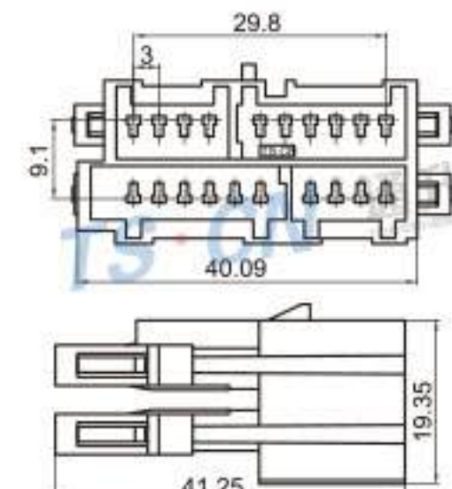
Type: TS1858-20P-11 Material: PA66 Matching Terminal: TSZ013
