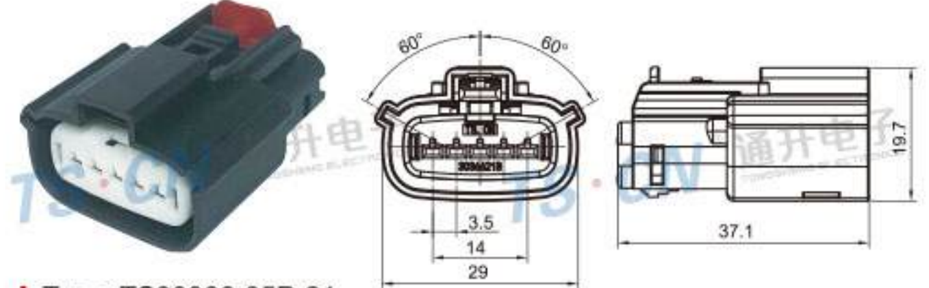
Type: TS30366-05P-21 Material: PA66 GF30% Matching Terminal: TSH047
