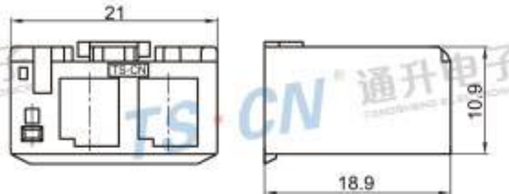
Type: TSLX20-03PF-AT Material: PA66 GF15% Matching Terminal: TSTF0016 / TSTF0015
