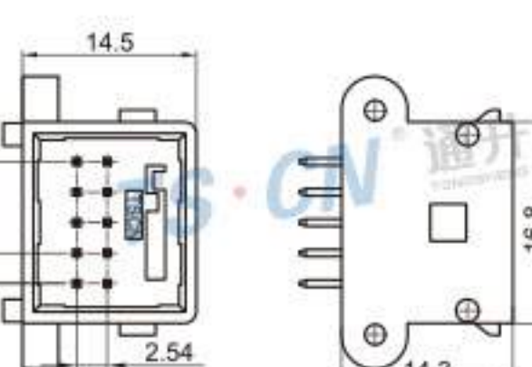
Type: TSROWE-10PM-PKB Material: PA66 Matching Terminal: TSPM0040 / TSPM0147
