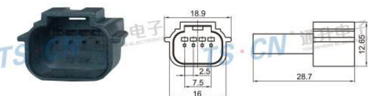
Type: TS30094-04P-11 Material: PA66 GF30% Matching Terminal: TSZ208
