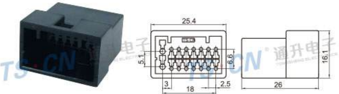
Type: TSKEN16-16P-11 Material: PA66 GF30% Matching Terminal: TSZ032 / TSZ031
