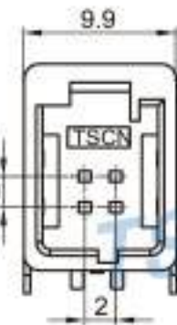
Type: TSMA04-04PM-PKS-2 Material: PA66 GF30% Matching Terminal: TSPM0030 / TSPM0029
