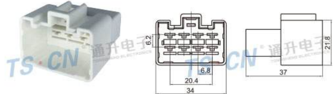
Type: TS30003-08P-11 Material: PBT GF15% Matching Terminal: TSZ028
