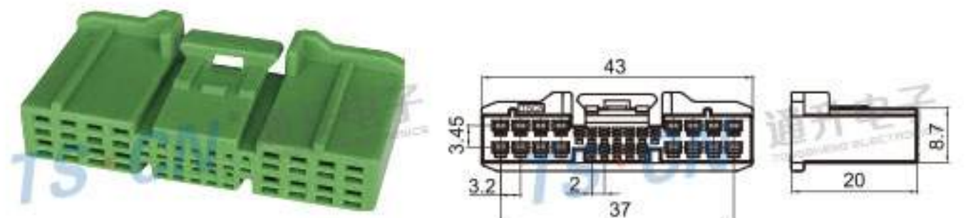
Type: TS30243-28P-21-7 Material: PA66 Matching Terminal: TSH593 / TSH606
