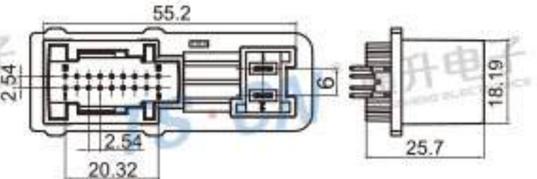
Type: TS30235-20PM-PKS Material: PBT GF15% Matching Terminal: TSPM0275 / TSPM0276
