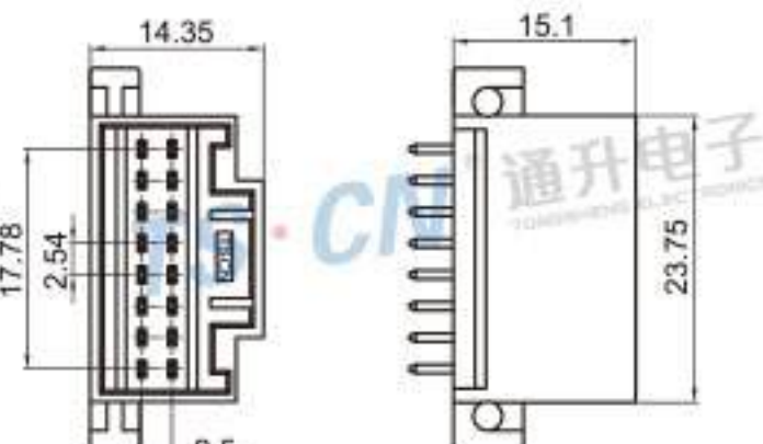
Type: TSPAN-16PM-PKS Material: PA66 Matching Terminal: TSPM0044~TSPM0046
