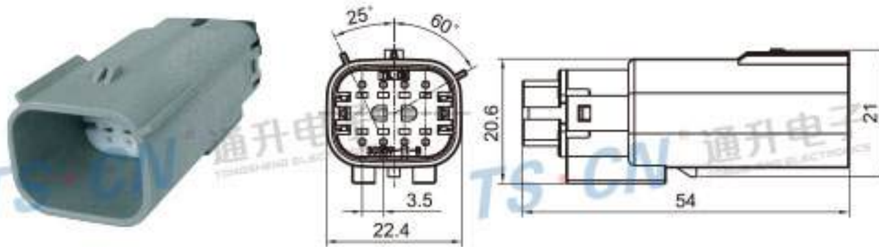
Type: TS30359-08P-11-1 Material: PA66 GF30% Matching Terminal: TSZ144A
