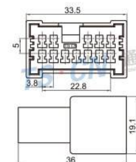
Type: TS7550-12P-11-1 Material: PA66 Matching Terminal: TSZ009
