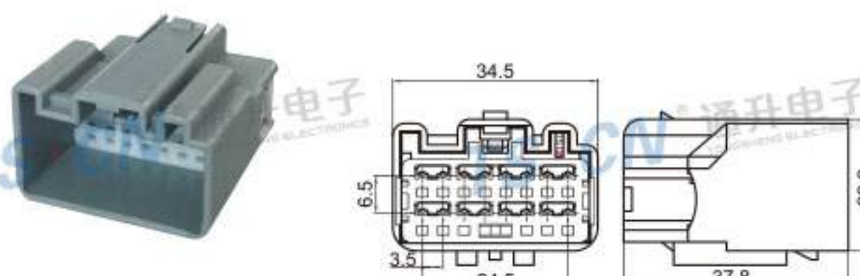
Type: TSVO16-16P-11-3 Material: PBT GF10% Matching Terminal: TSZ144
