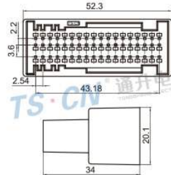
Type: TSFD54-54P-11 Material: PA66 GF30% Matching Terminal: TSZ208B
