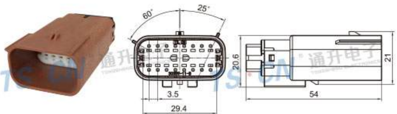
Type: TS30359-16P-11-2 Material: PA66 GF30% Matching Terminal: TSZ144A
