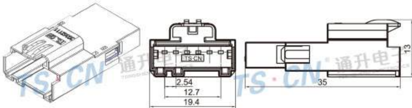
Type: TS30362-06P-11-1 Material: PA66 GF30% Matching Terminal: TSZ145
