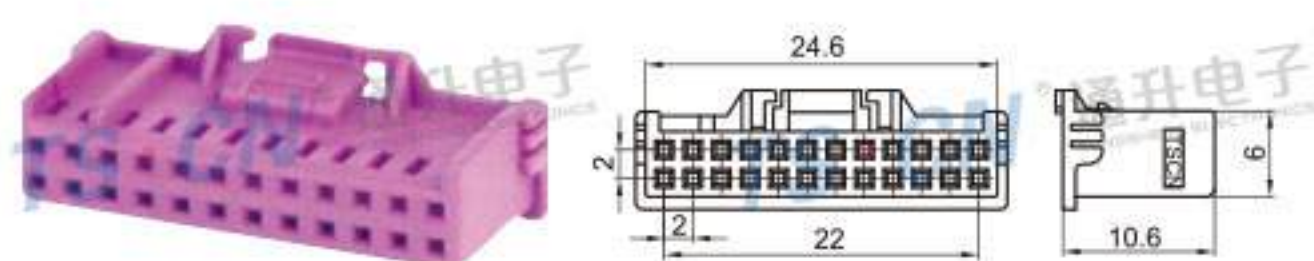
Type: TSQRA3-24P-21VT Material: PA66 GF15% Matching Terminal: TSPHB
