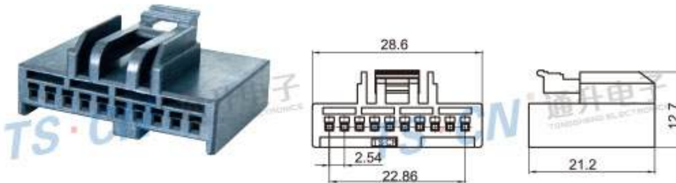
Type: TS2105-10P-21 Material: PA66 GF15% Matching Terminal: TSH143
