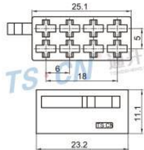
Type: TS1784A-08P-21BK Material: PA66 Matching Terminal: TSH019
