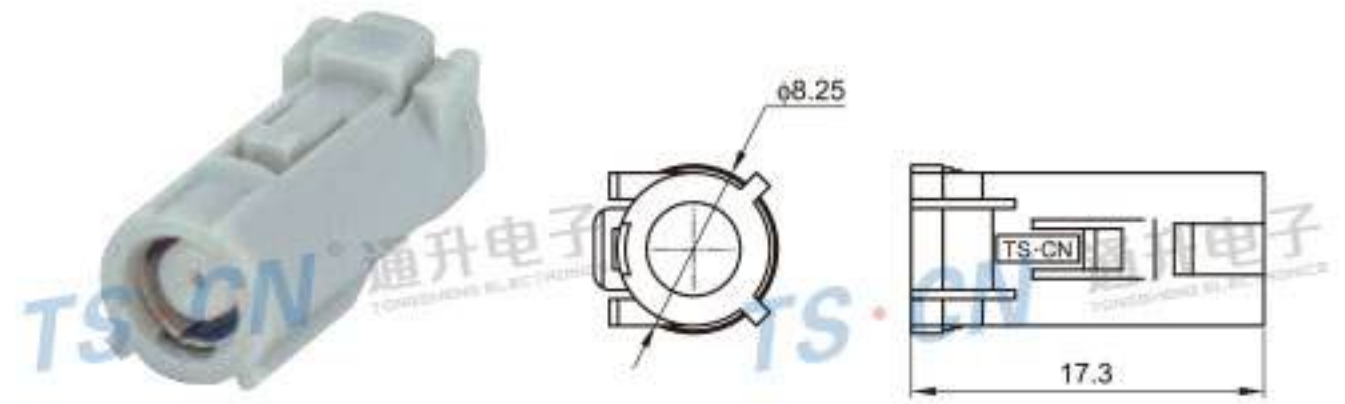
Type: TSGT16-01PF-AT Material: PA66 Matching Terminal: TSTF0017 / TSTF0004
