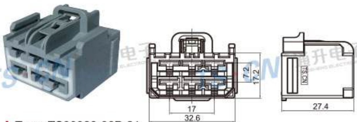
Type: TS30328-06P-21 Material: PBT Matching Terminal: TSH033B
