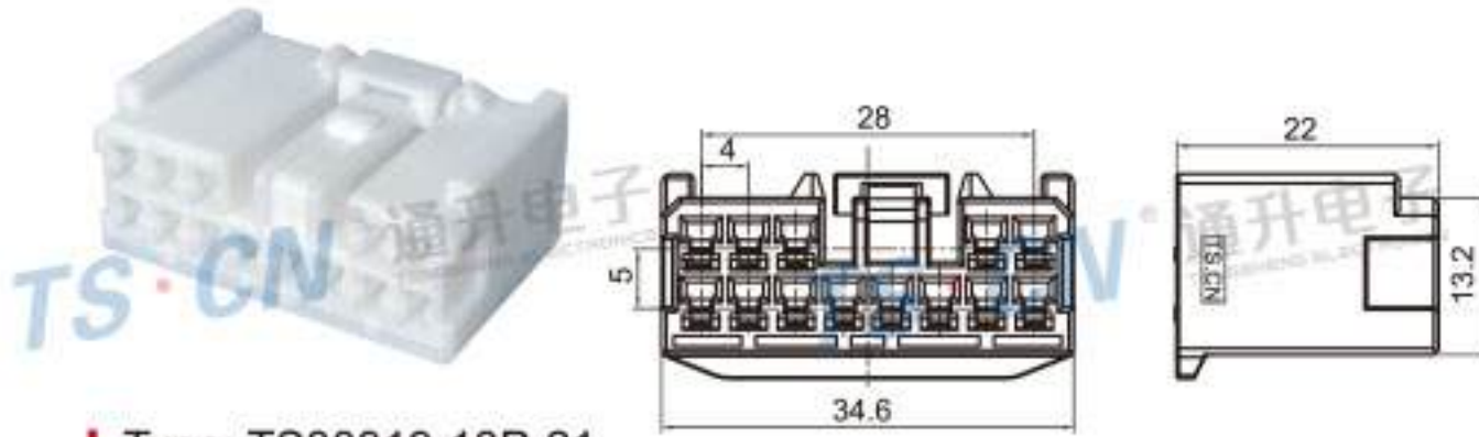
Type: TS30319-13P-21 Material: PBT Matching Terminal: TSH064
