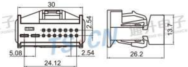
Type: TS30230-16P-21-2 Material: PBT Matching Terminal: TSH091 / TSH092
