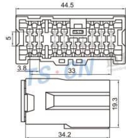
Type: TS7550-16P-11 Material: PA66 Matching Terminal: TSZ009
