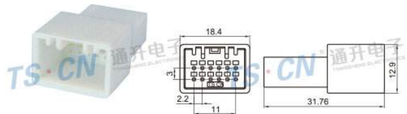
Type: TSNI12-12P-11 Material: PA66 Matching Terminal: TSZ208
