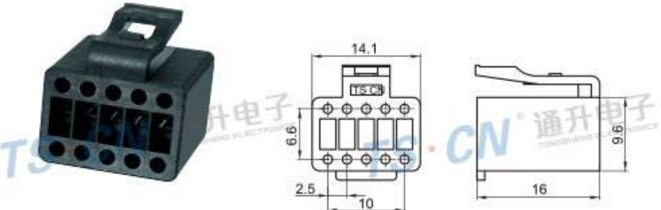
Type: TSKEN10-10P-21 Material: PA66 GF30% Matching Terminal: TSH031
