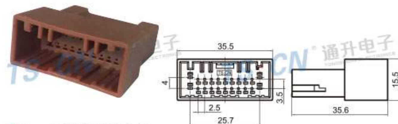
Type: TS30302-22P-11 Material: PBT Matching Terminal: TSZ040 / TSZ616
