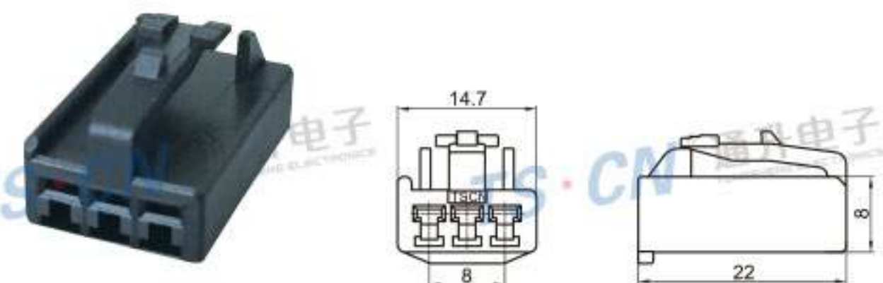
Type: TS30170-03P-21 Material: PA66 GF30% Matching Terminal: TSH009
