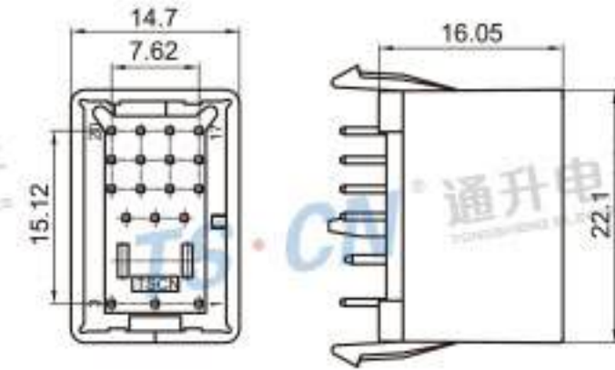
Type: TS30165-20PM-PKS Material: PA66 GF30% Matching Terminal: TSPM0084 / TSPM0250
