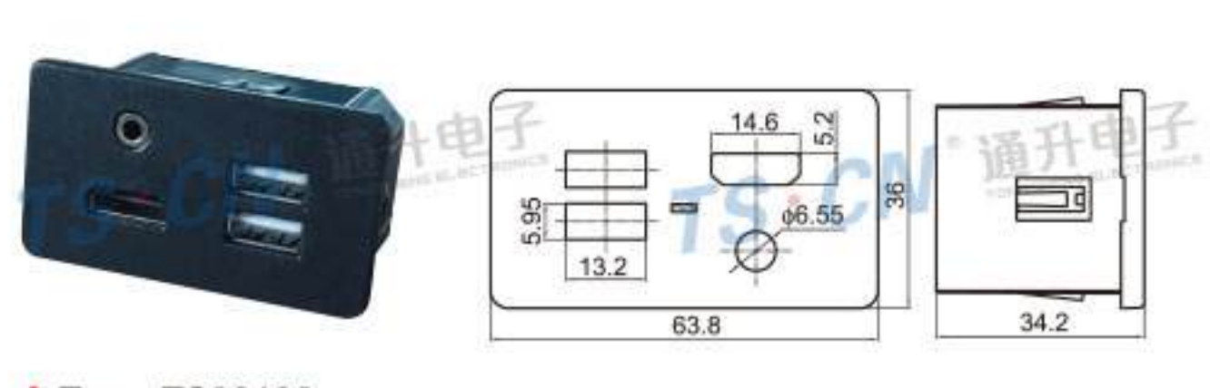
Type: TS30100 Material: ABS Matching Terminal: TSHDMI-F / TSUSB-F / TS3.5-F
