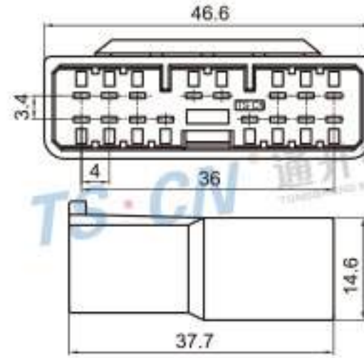
Type: TS1720-16P-11 Material: PA66 Matching Terminal: TSZ010
