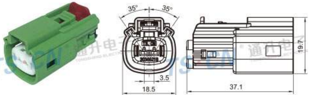
Type: TS30366-02P-21-3 Material: PA66 GF30% Matching Terminal: TSH047
