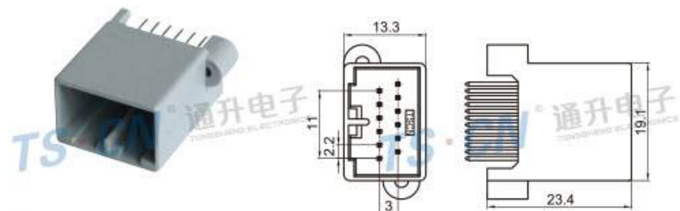
Type: TSCRV-12PM-PKS Material: PA66 Matching Terminal: TSPM0214
