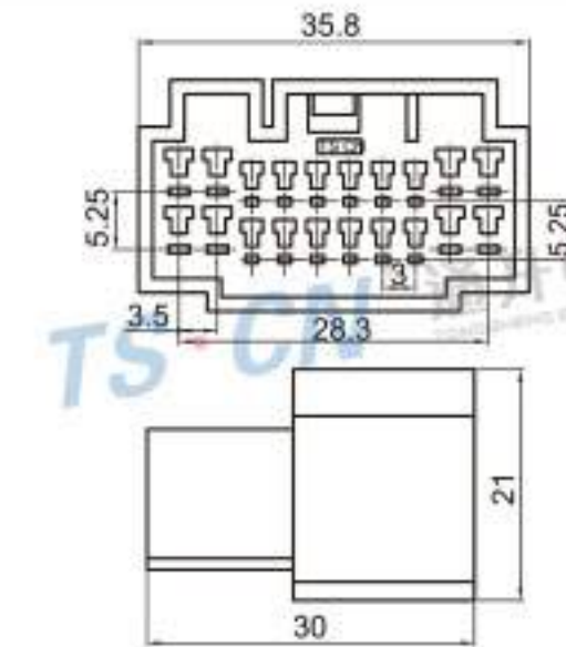
Type: TS1721-20P-11 Material: PA66 Matching Terminal: TSZ018
