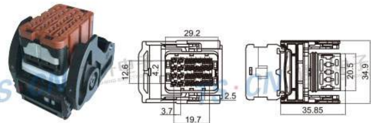
Type: TS30245-32P-21-2 Material: PA66 Matching Terminal: TSH632~TS643221029
