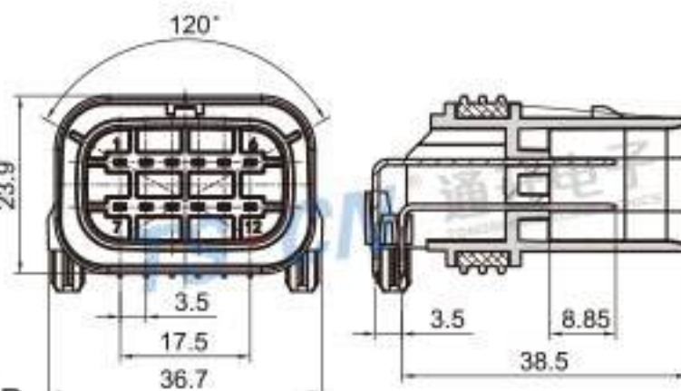
Type: TS30359-12PM-PKB Material: PBT GF15% Matching Terminal: TSPM0333/TSPM0334
