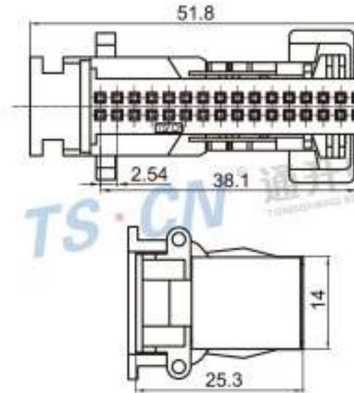
Type: TSAD32-32P-21-1 Material: PA66 Matching Terminal: TSH092
