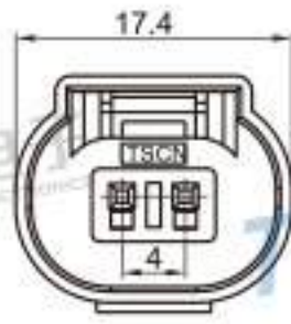
Type: TS30177-02P-21 Material: PA66 GF30% Matching Terminal: TSH143
