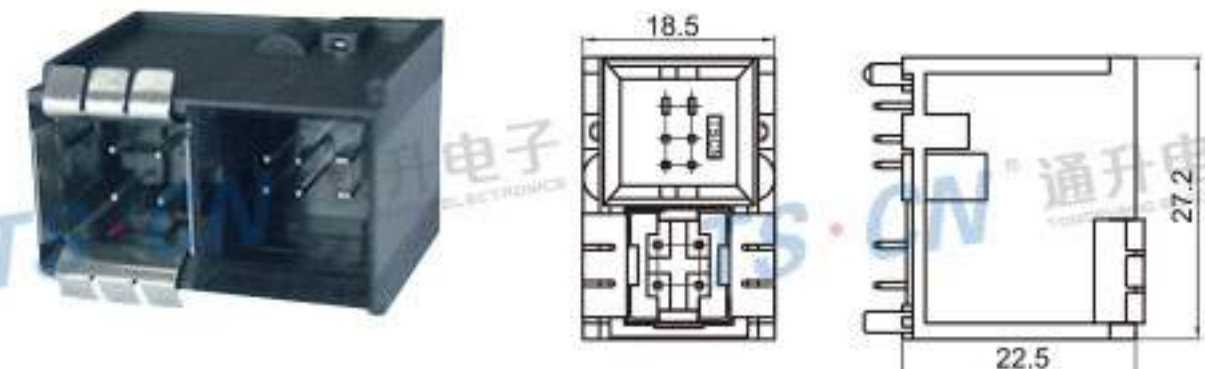
Type: TS30060-10PM-PKS Material: PA66 GF30% Matching Terminal: TSPM0217 / TSPM0215 / TSPM0077 / TSPM0039
