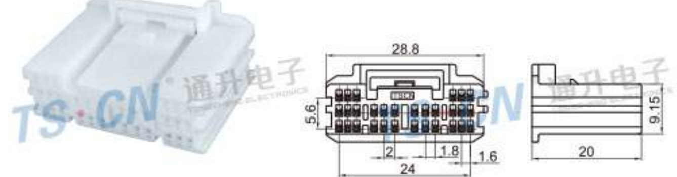
Type: TS30101-30P-21 Material: PA66 Matching Terminal: TSH600
