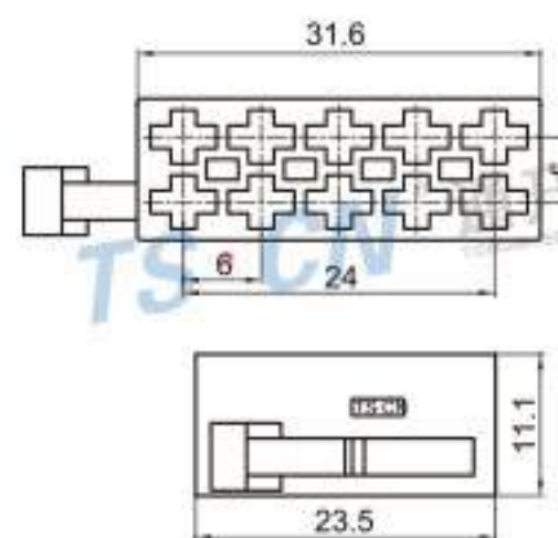
Type: TS9001-10P-21 Material: PA66 Matching Terminal: TSH019
