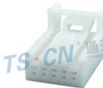
Type: TS30188-05P-21 Material: PA66 Matching Terminal: TSH143
