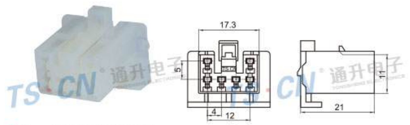
Type: TS1761-06P-21-1 Material: PA66 Matching Terminal: TSH009
