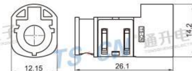
Type: TSVW10-04PM-AT-5GY-1 Material: PA66 GF15% Matching Terminal: TSPM0175 / TSTM0051
