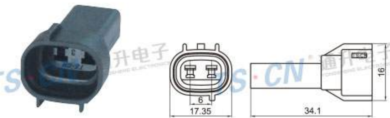
Type: TS30064-02P-11 Material: PA66 GF30% Matching Terminal: TSZ045
