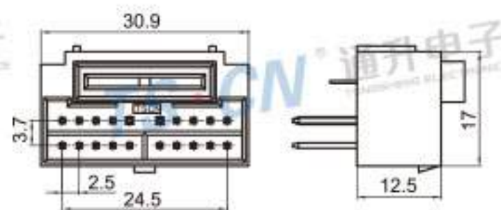
Type: TSJEN-20PM-PKS Material: PBT GF30% Matching Terminal: TSPM0231 / TSPM0098
