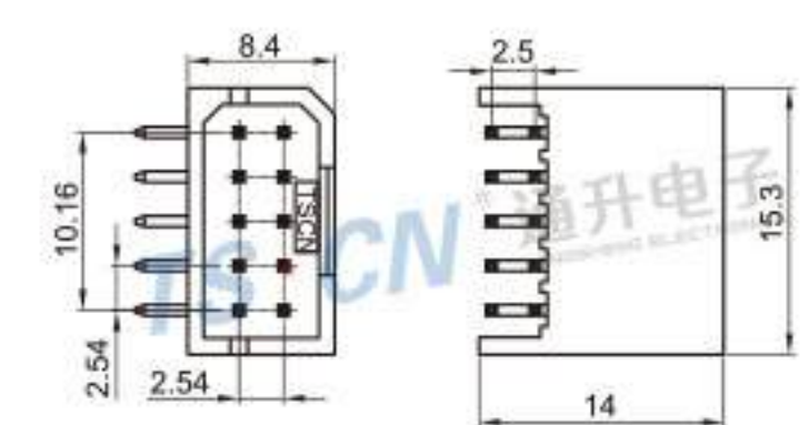
Type: TSCH10-10PM-PKB(10P-24P) Material: PA66 Matching Terminal: TSPM0084 / TSPM0128
