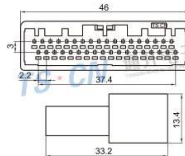
Type: TSCRV36-36P-11-1 Material: PA66 Matching Terminal: TSZ208B
