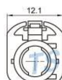
Type: TSVW20-04PF-AT-5GN Material: PA66 GF30% Matching Terminal: TSTF0048 / TSTF0049 / TSTF0050
