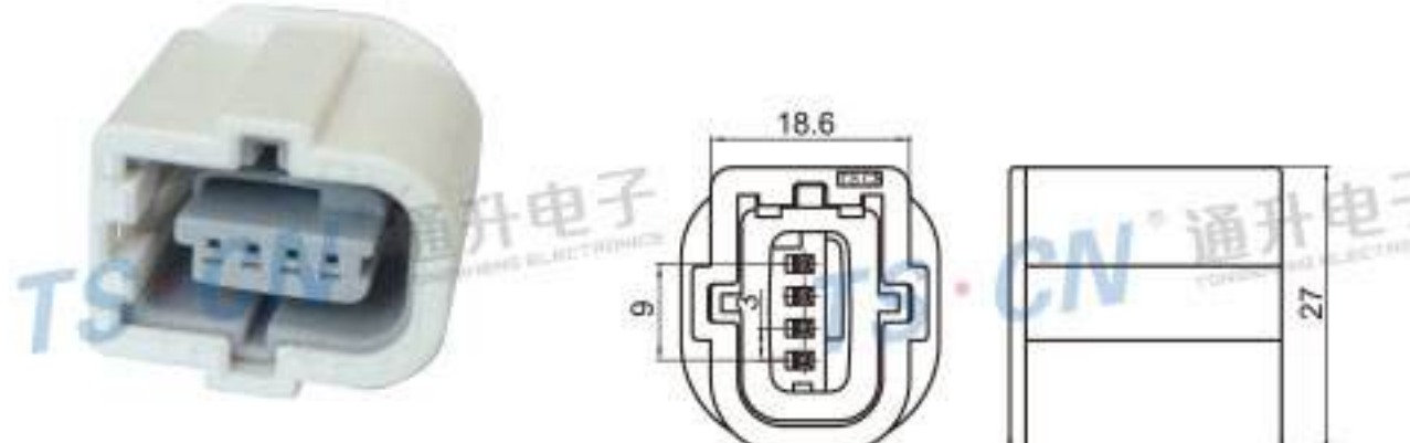
Type: TS1050-04P-21 Material: PA66 Matching Terminal: TSH143
