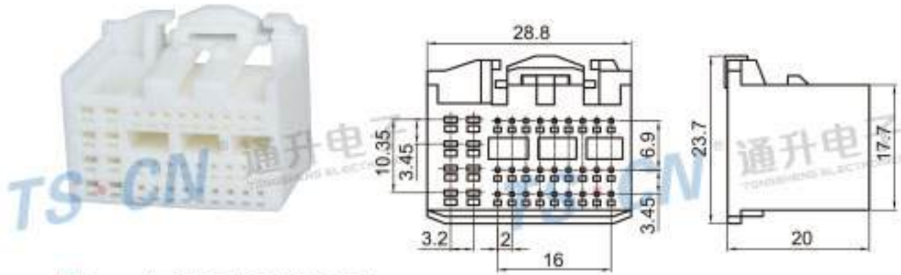
Type: TS30116-35P-21 Material: PA66 Matching Terminal: TSH593 / TSH606
