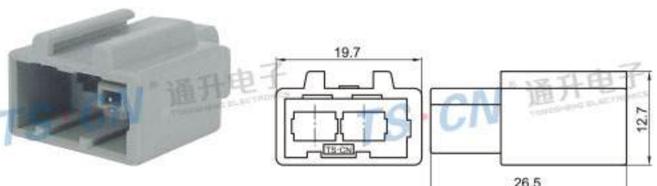
Type: TSK110-02PM-AT Material: PA66 Matching Terminal: TSTM0001 / TSTM0002
