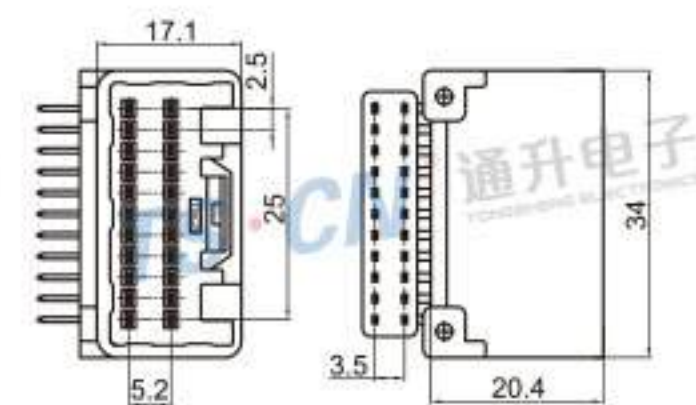
Type: TSMI22-22PM-PKB Material: PA66 Matching Terminal: TSPM0001 / TSPM0003
