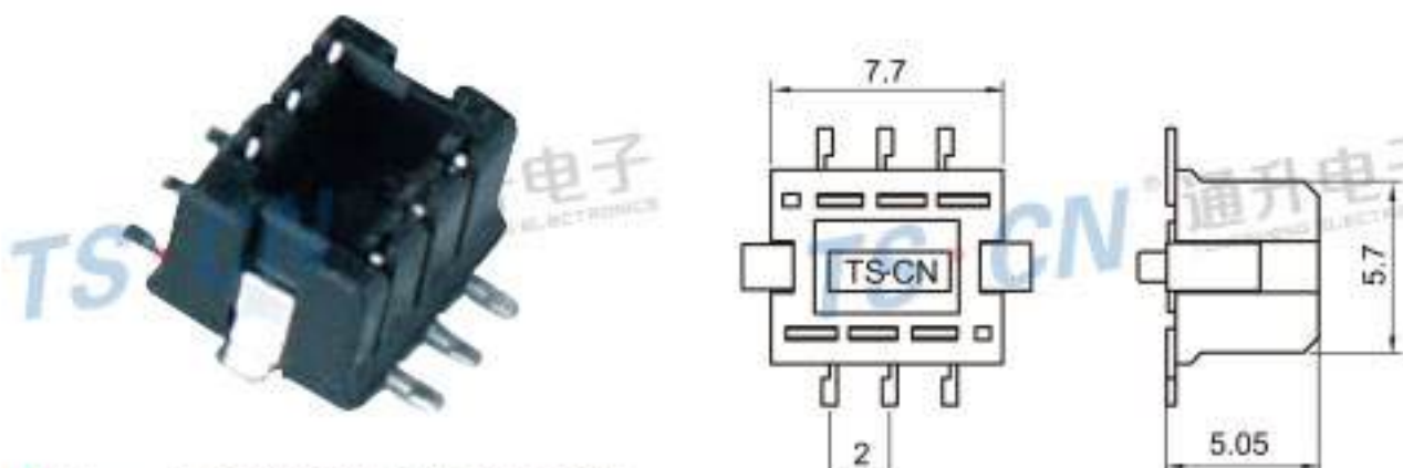
Type: TSTKCW-06PM-PKB Material: PA66 GF30% Matching Terminal: TSPM0124 / TSPM0125
