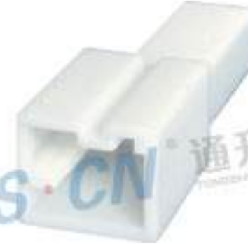
Type: TSLB39-02P-11-5 Material: PA66 GF30% Matching Terminal: TSZ208B
