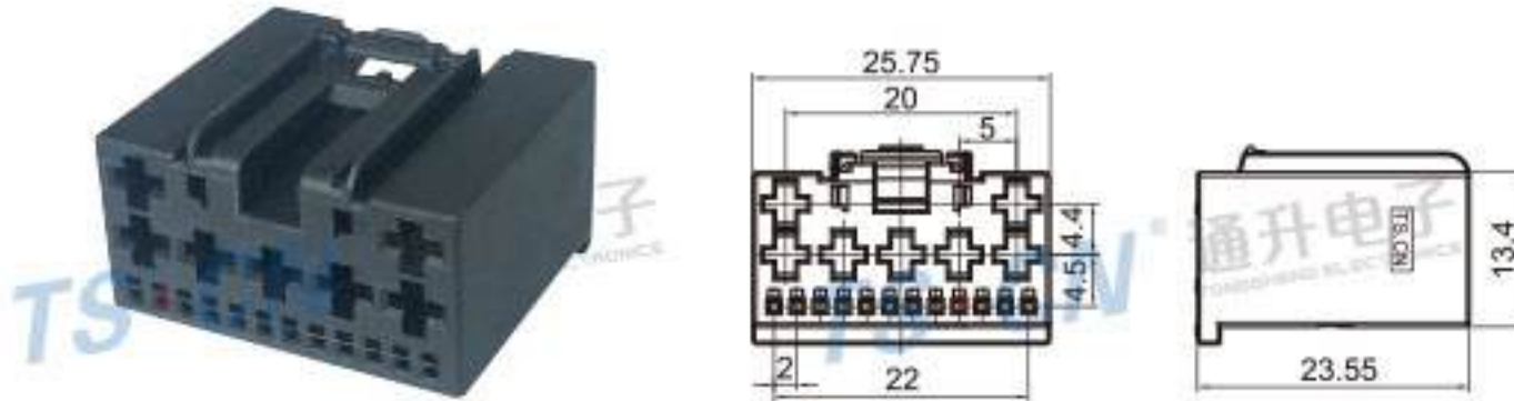
Type: TS30299-19P-21 Material: PA66 Matching Terminal: TS1241390-1 / TSHY66
