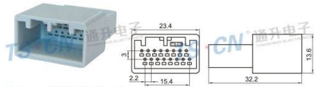
Type: TSCRV16-16P-11 Material: PA66 A206FN Matching Terminal: TSZ208B
