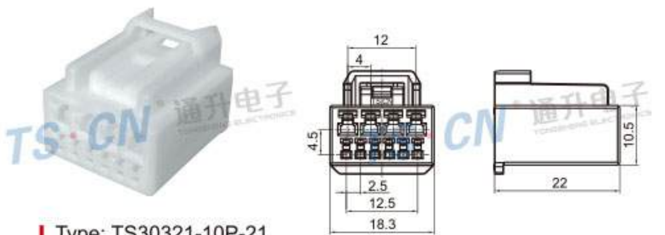
Type: TS30321-10P-21 Material: PBT Matching Terminal: TSH064 / TSH076
