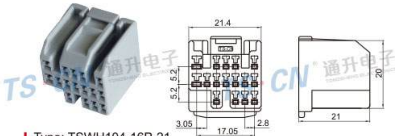
Type: TSWH104-16P-21 Material: PA66 Matching Terminal: TSH076
