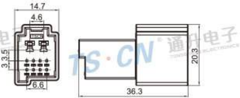
Type: TS30348-10P-11 Material: PBT Matching Terminal: TSZ045 / TSZ208
