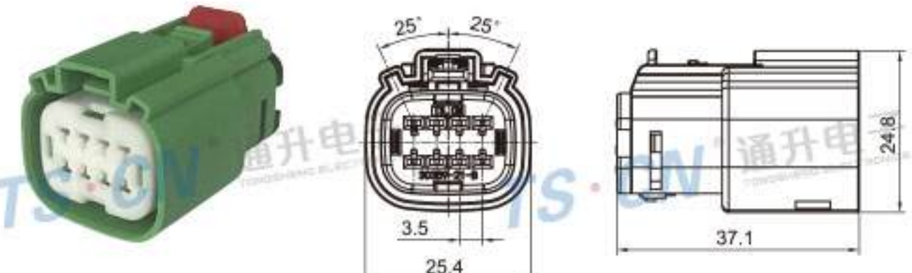
Type: TS30359-08P-21-3 Material: PA66 GF30% Matching Terminal: TSH047
