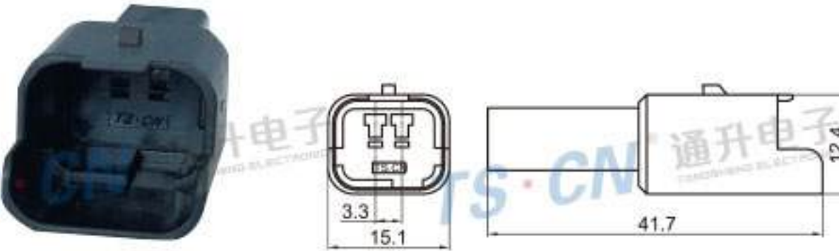
Type: TS30067-02P-11 Material: PA66 GF30% Matching Terminal: TSZ144
