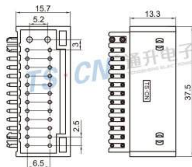
Type: TSKEN-16PM-PKB-2 Material: PA66 GF30% Matching Terminal: TSPM0103~TSPM0108
