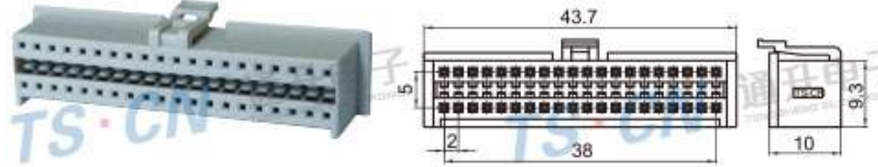
Type: TS1008-40P-21 Material: PA66 GF30% Matching Terminal: TSH540
