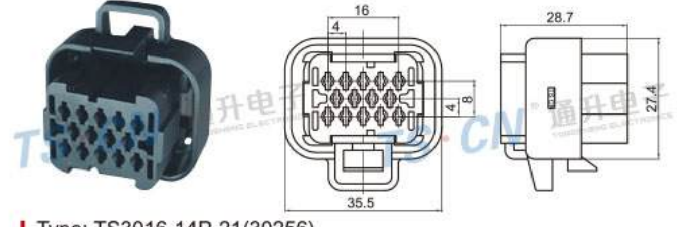
Type: TS3016-14P-21(30256) Material: PA66 Matching Terminal: TSH535
