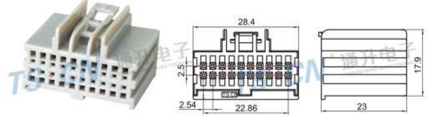
Type: TSGM20-20P-21-2 Material: PA66 GF30% Matching Terminal: TSH143
