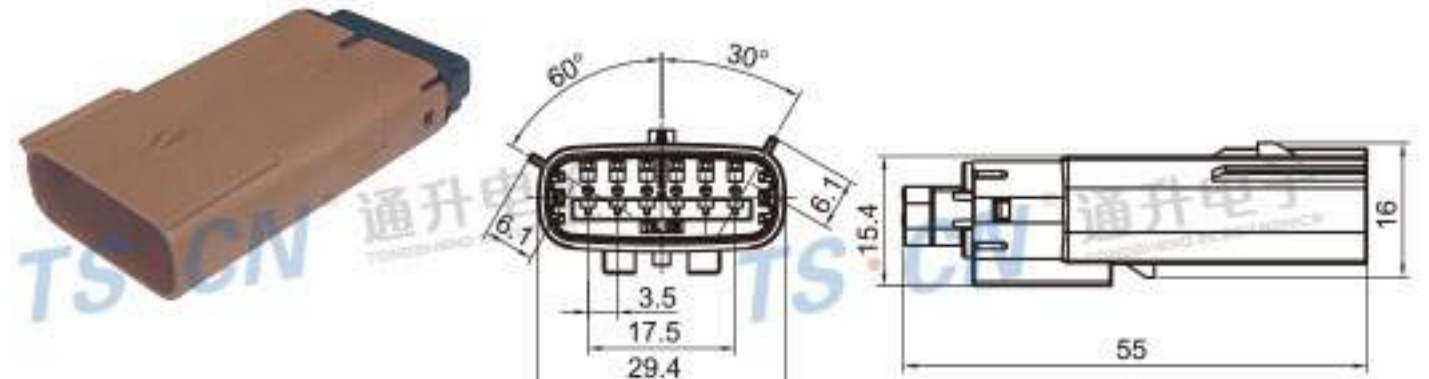
Type: TS30366-06P-11-2 Material: PA66 GF30% Matching Terminal: TSZ144A
