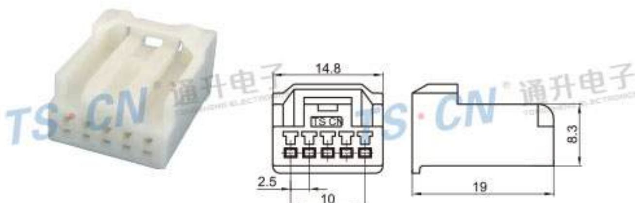
Type: TSTA05-05P-21-1 Material: PA66 Matching Terminal: TSH076
