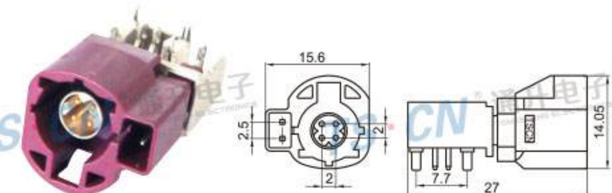
Type: TSVW10-06PM-AT Material: PBT GF30% Matching Terminal: TSPM0027 / TSPM0151 / TSPM0151-A
