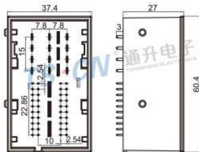
Type: TS6523-52PM-PSK Material: PA66 Matching Terminal: NIL
