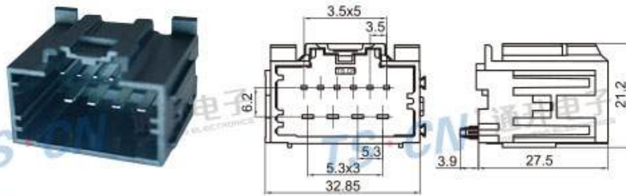
Type: TS30039-10PM-PKS Material: PBT GF15% Matching Terminal: TSPM0202 / TSPM0203
