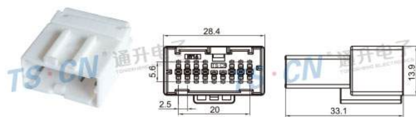
Type: TSHY16-16P-11 Material: PA66 Matching Terminal: TSZ145
