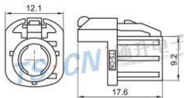
Type: TSVW20-04PF-AT-5YG Material: PA66 GF30% Matching Terminal: TSTF0048 / TSTF0049 / TSTF0050
