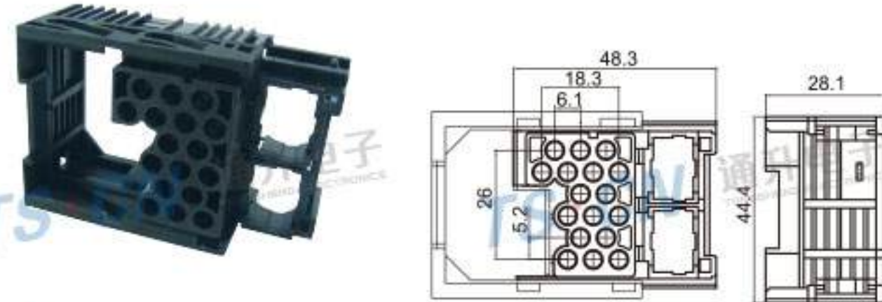
Type: TS8590-17P-21 Material: PA66 GF30% Matching Terminal: TSH078
