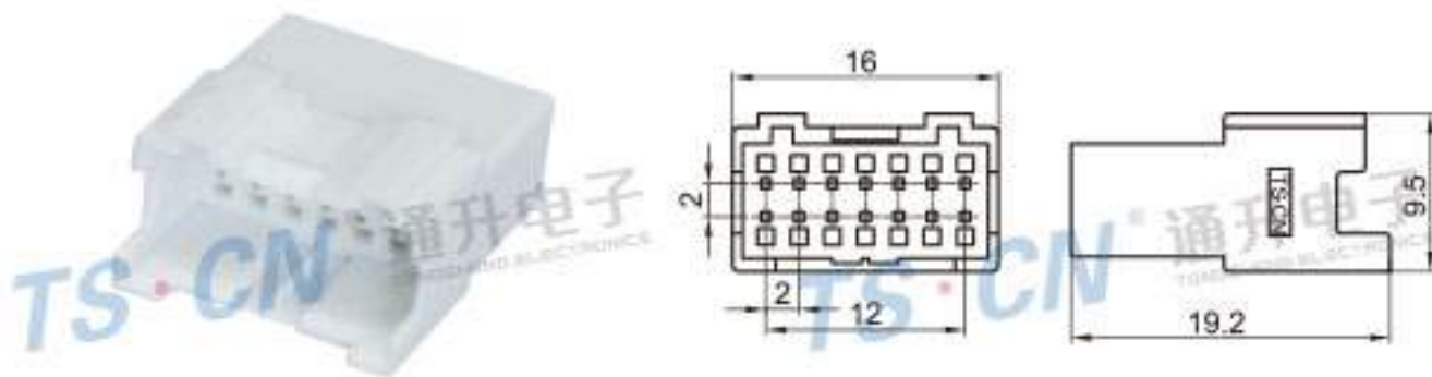
Type: TSPHS-14P-11(10P-24P) Material: PBT GF15% Matching Terminal: TSZ210
