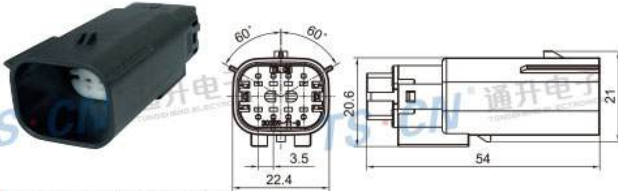
Type: TS30359-08P-11 Material: PA66 GF30% Matching Terminal: TSZ144A
