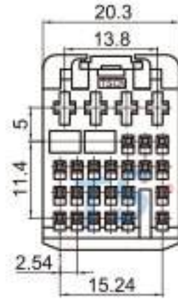
Type: TS30217-30P-21-4 Material: PBT GF10% Matching Terminal: TSH019 / TSH092
