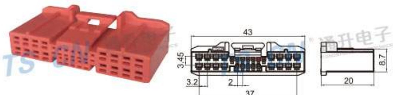
Type: TS30243-28P-21-5 Material: PA66 Matching Terminal: TSH593 / TSH606
