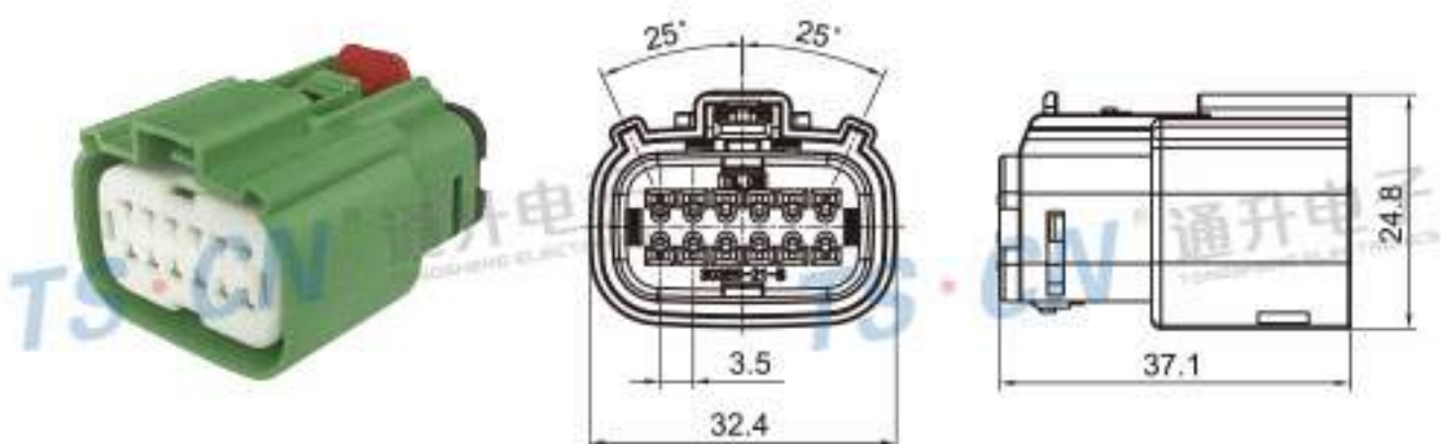
Type: TS30359-12P-21-3 Material: PA66 GF30% Matching Terminal: TSH047
