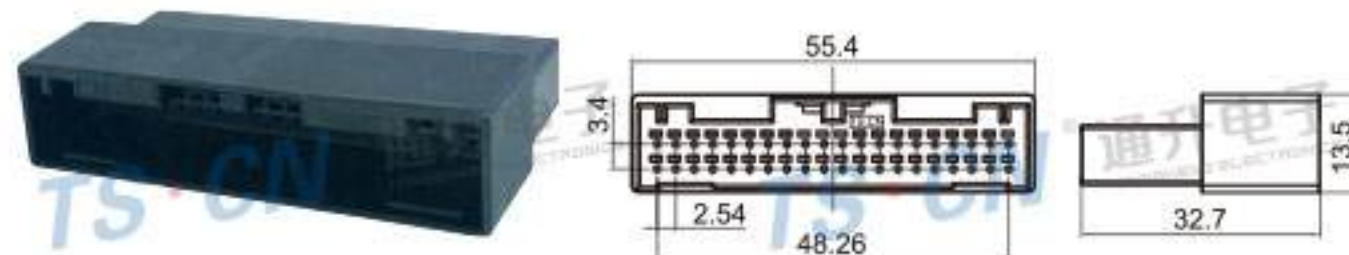
Type: TS30285-40P-11 Material: PBT GF30% Matching Terminal: TSZ616
