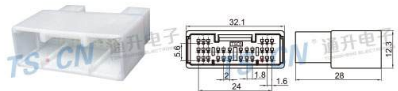
Type: TS30101-30P-11-1 Material: PA66 Matching Terminal: TSZ556
