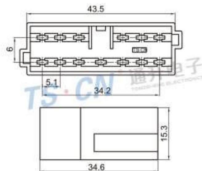
Type: TSCIT-13P-11 Material: PA66 Matching Terminal: TSZ024
