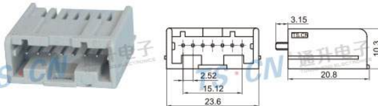
Type: TS30043-07PM-PKS Material: PA66 GF30% Matching Terminal: TSPM0085
