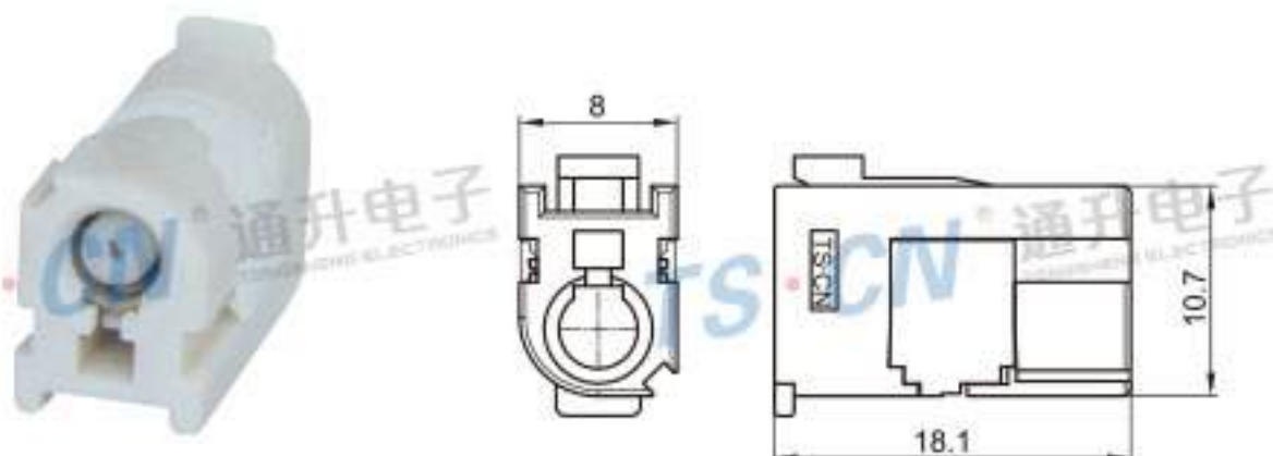
Type: TS1068-01PF-AT-2 Material: PA66 Matching Terminal: TSTF0003 / TSTF0004
