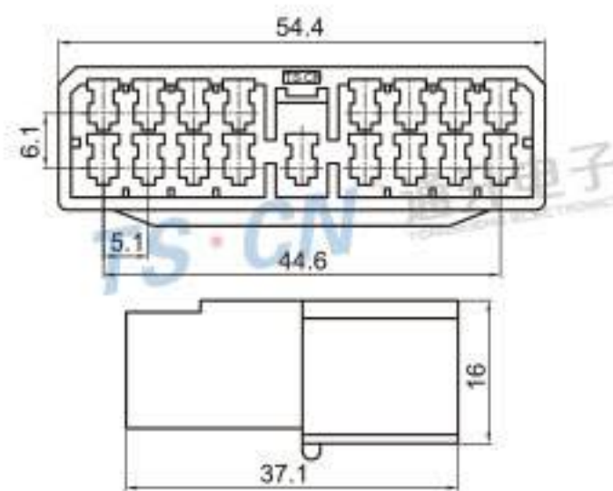
Type: TSHD17-17P-11 Material: PA66 Matching Terminal: TSZ800
