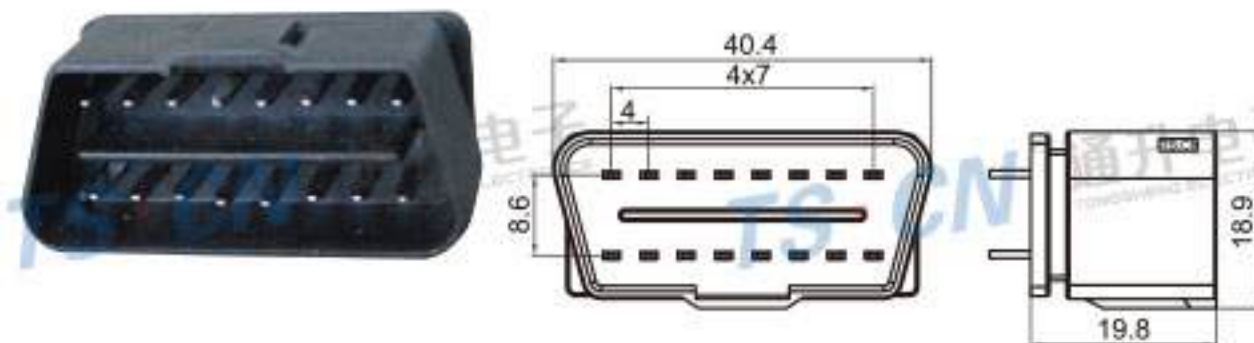
Type: TS30055-16PM-PKS Material: PA66 GF30% Matching Terminal: TSPM0211
