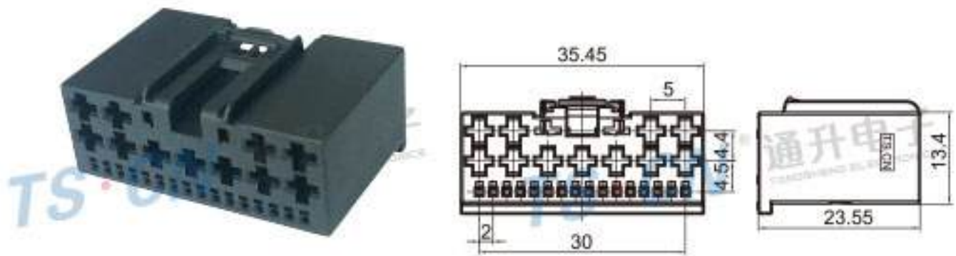
Type: TS30299-27P-21 Material: PA66 Matching Terminal: TS1241390-1 / TSHY66
