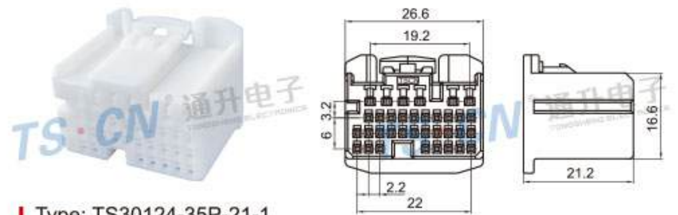
Type: TS30124-35P-21-1 Material: PA66 Matching Terminal: TSH076 / TSH143
