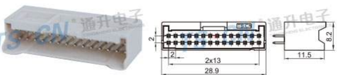
Type: TS30047-28PM-PKS(QRA3) Material: PA66 GF15% Matching Terminal: TSPM0145
