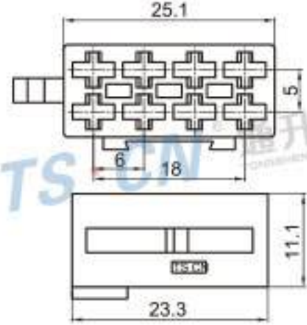
Type: TS1784A-08P-21-2BN Material: PA66 Matching Terminal: TSH019
