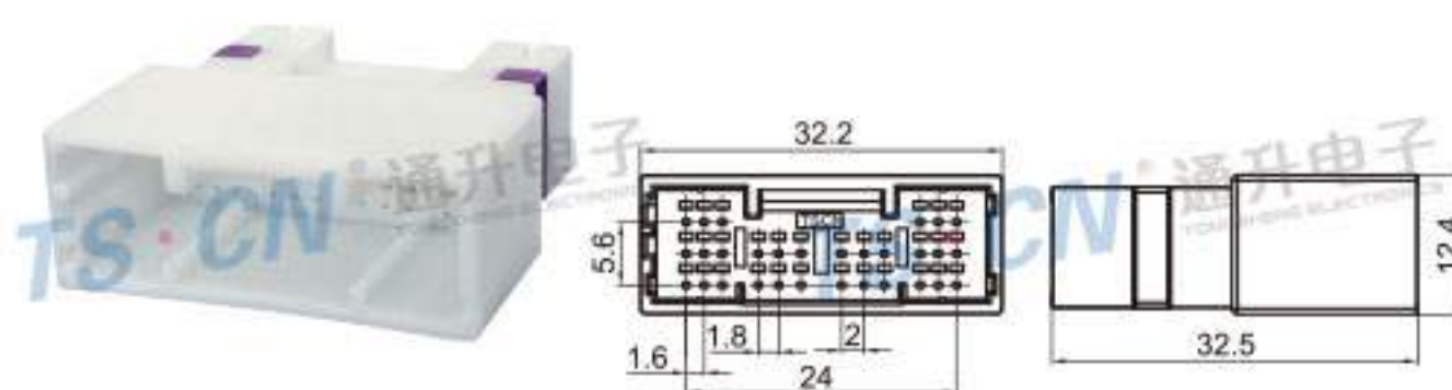
Type: TS30101-30P-11-4 Material: PA66 Matching Terminal: TSZ615
