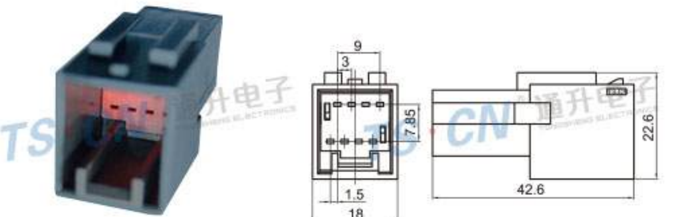
Type: TS30058-08P-11(5700) Material: PA66 Matching Terminal: TSZ185
