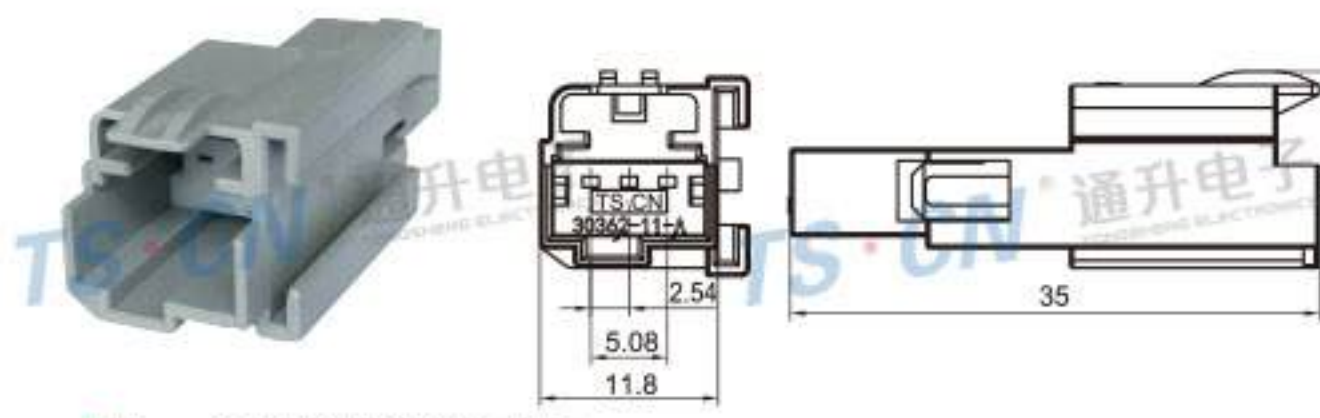
Type: TS30362-03P-11-4 Material: PA66 GF30% Matching Terminal: TSZ145
