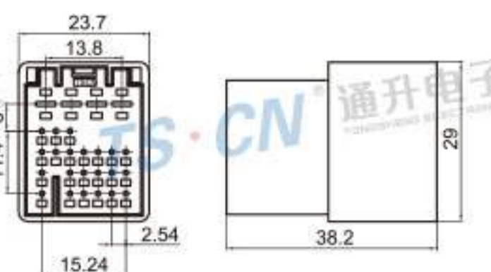
Type: TS30217-30P-11-4 Material: PBT GF15% Matching Terminal: TSDJ615B-2.8*0.8B / TSZ208
