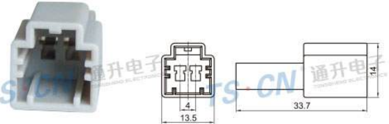
Type: TS30093-02P-11 Material: PA66 Matching Terminal: TSZ009
