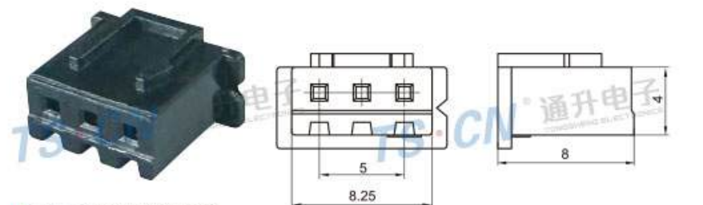
Type: TSC3-03P-21 Material: PA66 Matching Terminal: TSC3
