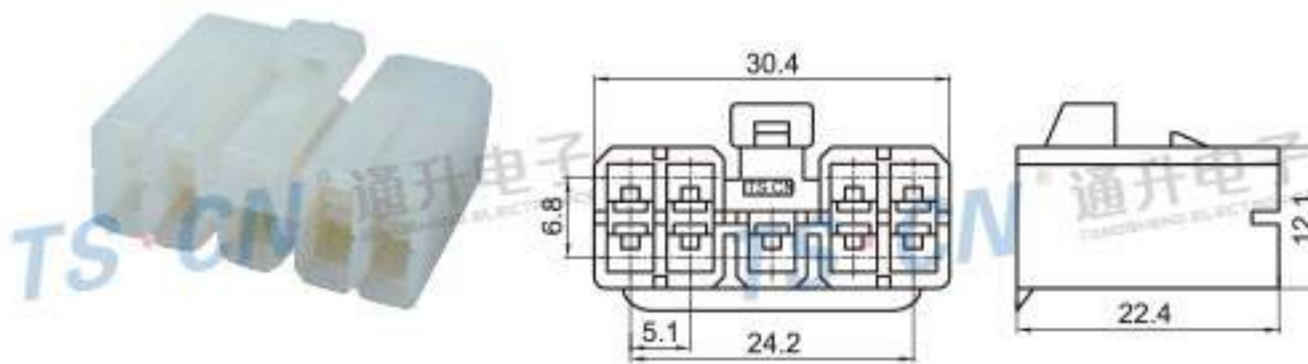
Type: TS1398-09P-21 Material: PA66 Matching Terminal: TSH017
