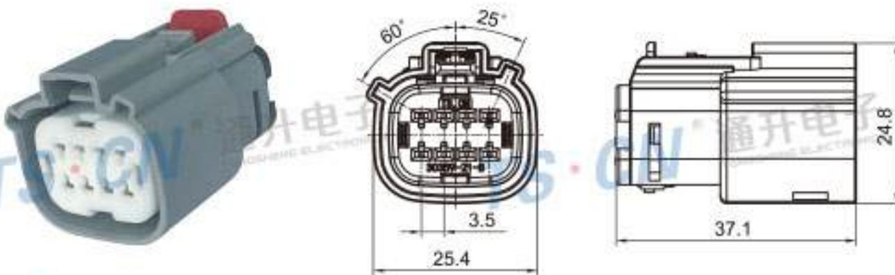
Type: TS30359-08P-21-1 Material: PA66 GF30% Matching Terminal: TSH047
