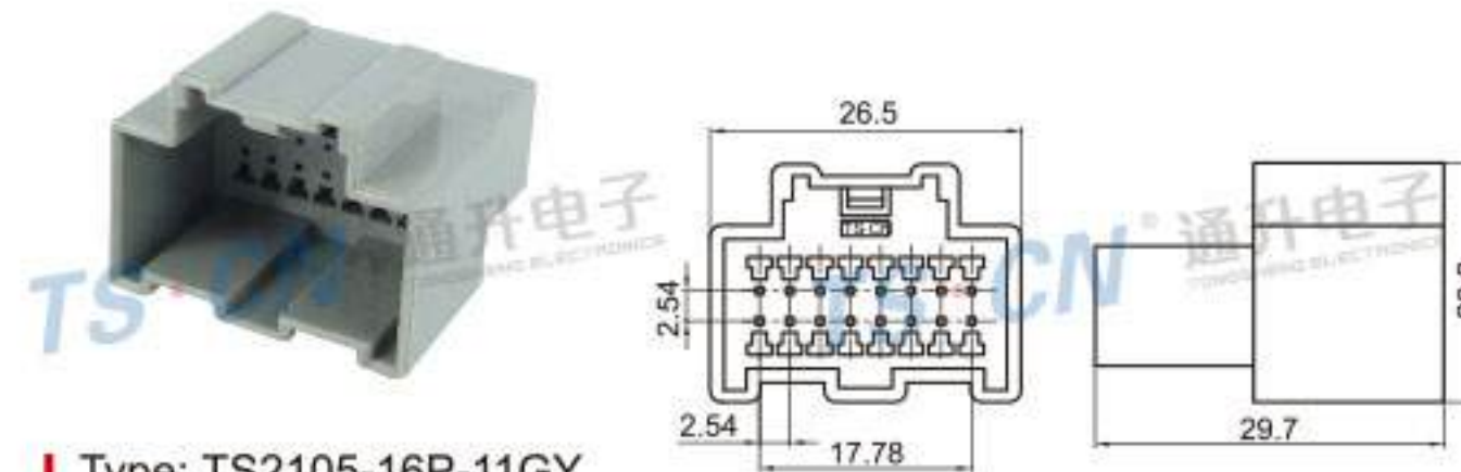
Type: TS2105-16P-11GY Material: PA66 Matching Terminal: TSZ018B
