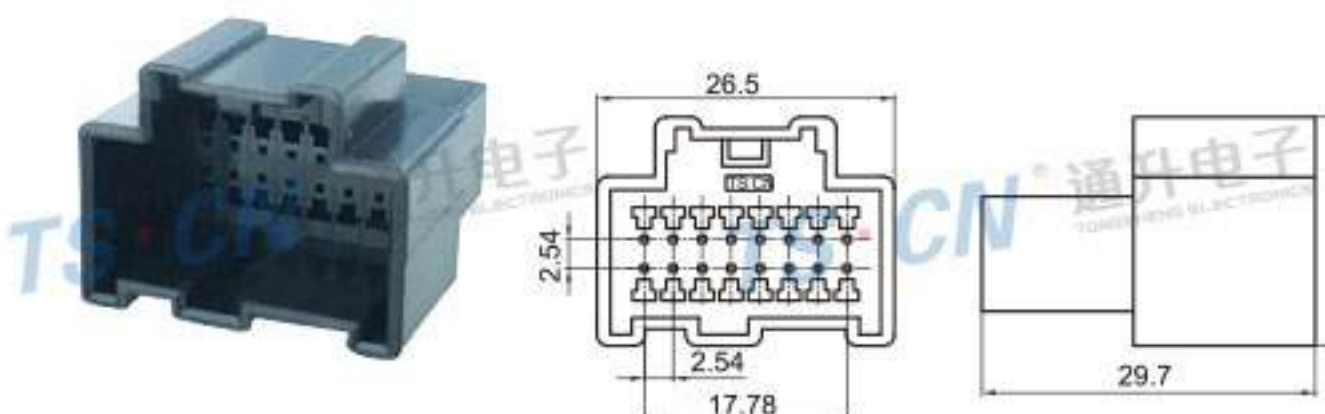
Type: TS2105-16P-11 Material: PA66 GF30% Matching Terminal: TSZ018B
