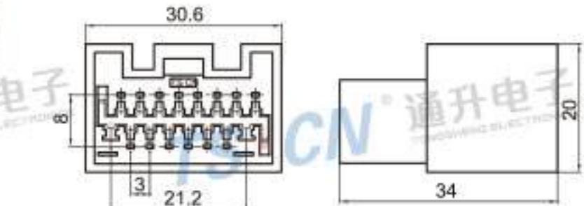
Type: TS1771-16P-11-1 Material: PA66 Matching Terminal: TSZ011 / TSZ018
