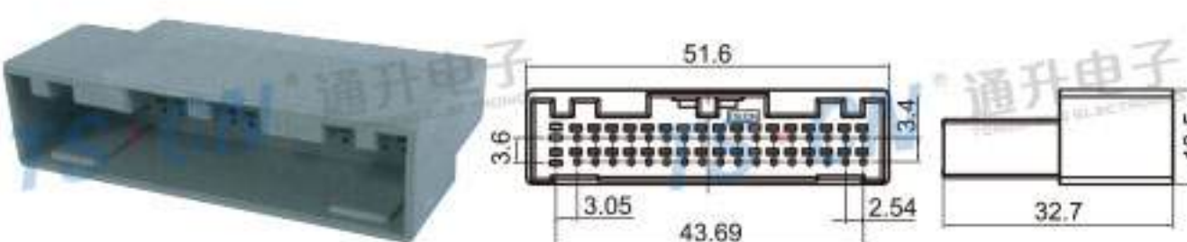
Type: TS30285-36P-11 Material: PBT GF30% Matching Terminal: TSZ040 / TSZ616
