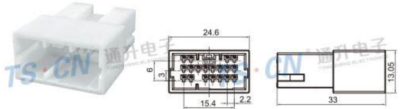
Type: TS30306-19P-11 Material: PA66 Matching Terminal: TSZ618
