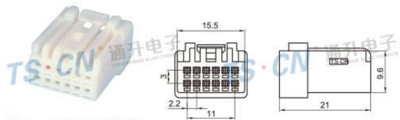
Type: TSNI12-12P-21 Material: PA66 Matching Terminal: TSH143
