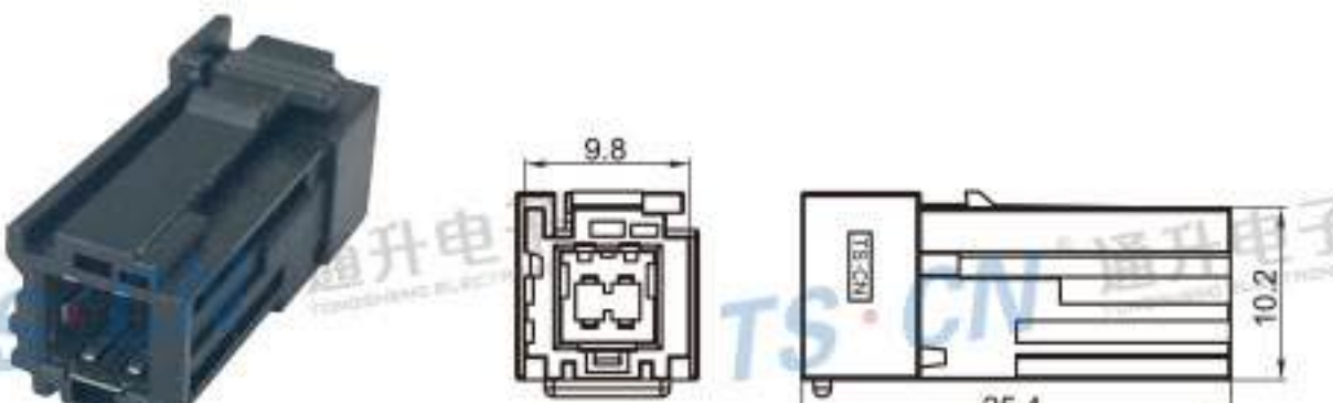
Type: TSTA04-04PF-AT-4 Material: PBT 1100 Matching Terminal: TSTF0008 / TSTF0010 / TSTF0011
