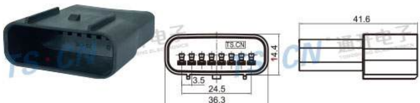
Type: TS30325-08P-11 Material: PBT Matching Terminal: TSZ144A
