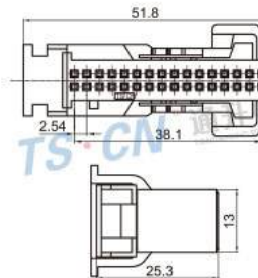
Type: TSAD32-32P-21-2 Material: PA66 Matching Terminal: TSH092
