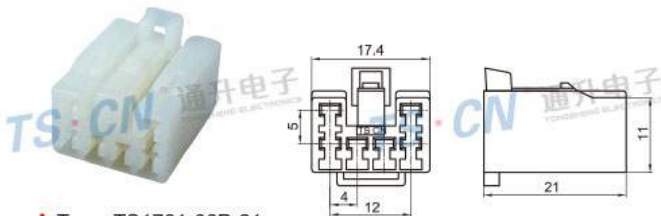
Type: TS1761-06P-21 Material: PA66 Matching Terminal: TSH009
