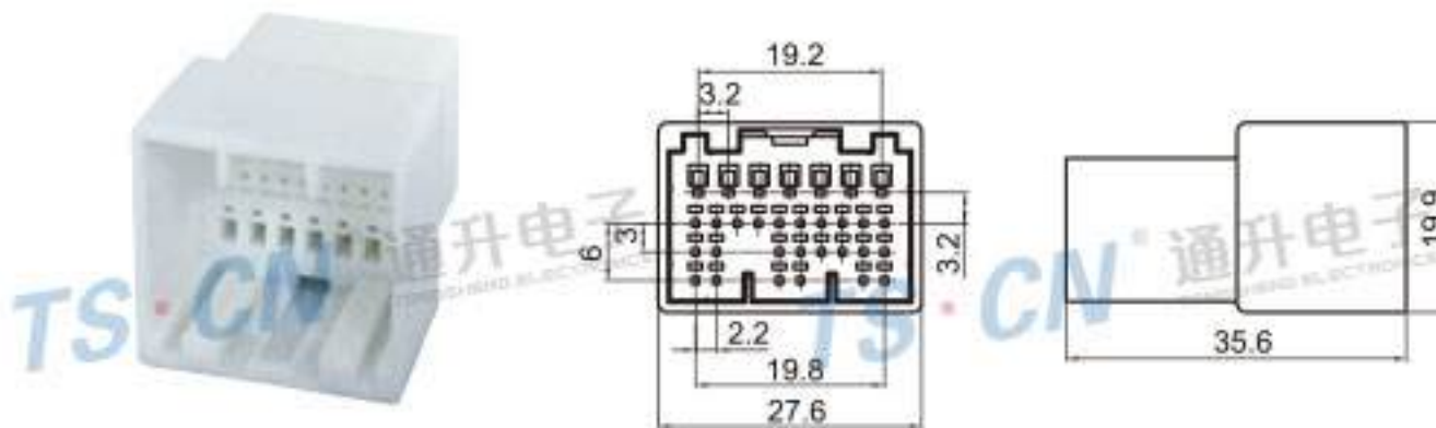
Type: TS30124-31P-11 Material: PA66 Matching Terminal: TSZ145 / TSZ208
