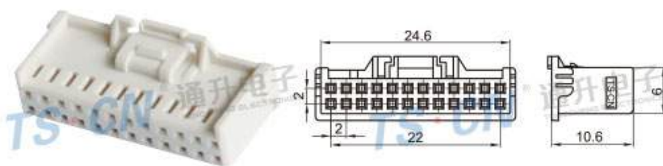
Type: TSQRA3-24P-21(12P-28P) Material: PA66 GF30% Matching Terminal: TSPHB
