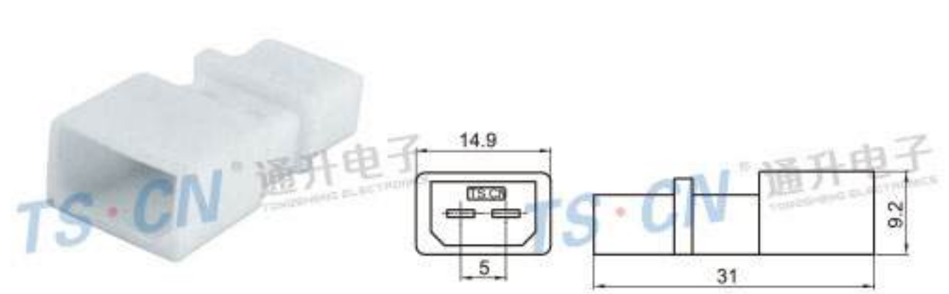
Type: TS7022-3.5-11-1 Material: PA66 Matching Terminal: NIL
