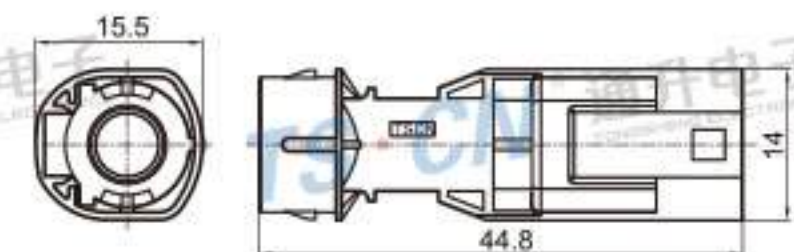
Type: TS30166-04PM-AT Material: PA66 GF30% Matching Terminal: TSTF0051-B / TSPM0175
