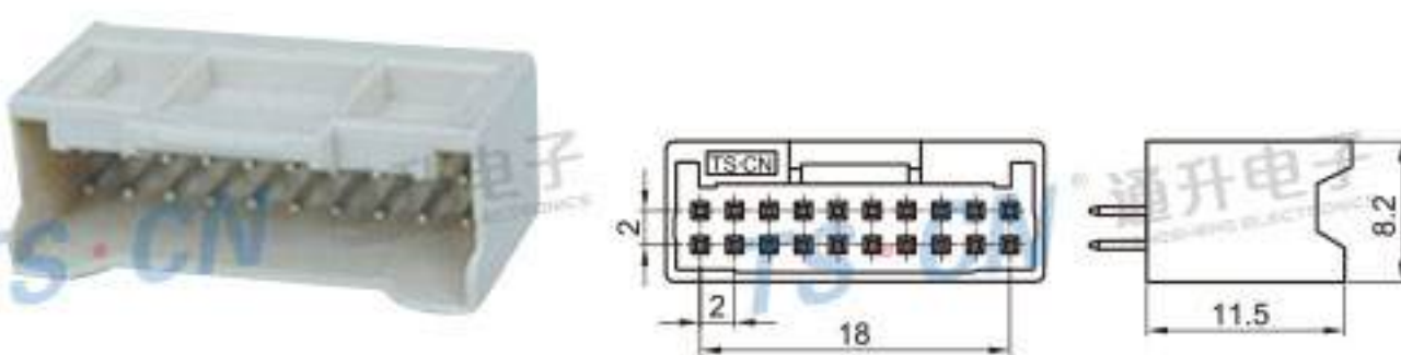
Type: TS30046-20PM-PKS(QRA3) Material: PA66 GF15% Matching Terminal: TSPM0145
