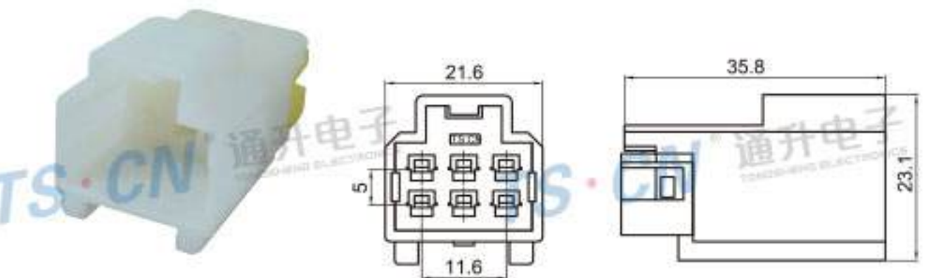
Type: TS1763-06P-11 Material: PA66 Matching Terminal: TSZ012
