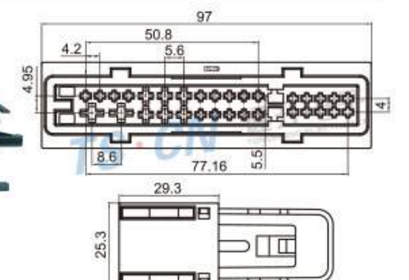
Type: TSAD32-32P-11 Material: PA66 GF30% Matching Terminal: TSZ028 / TSZ024 / TSZ040
