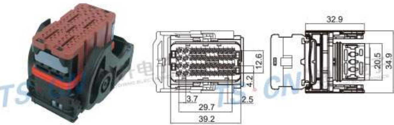
Type: TS30245-48P-21-2 Material: PA66 Matching Terminal: TSH632 / TS643221029
