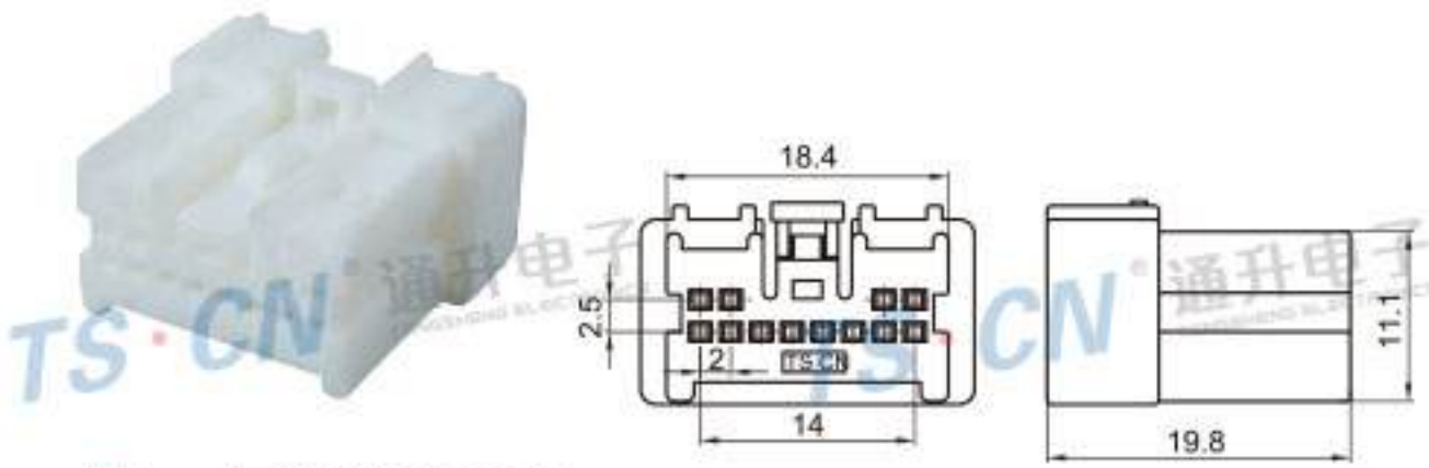
Type: TSNI07-12P-21 Material: PA66 Matching Terminal: TSH143
