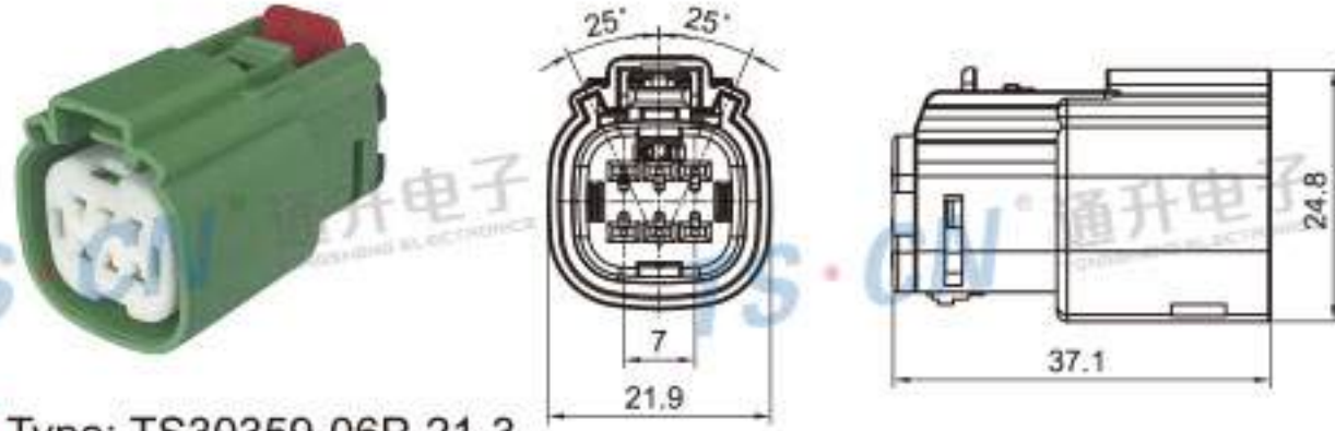
Type: TS30359-06P-21-3 Material: PA66 GF30% Matching Terminal: TSH047
