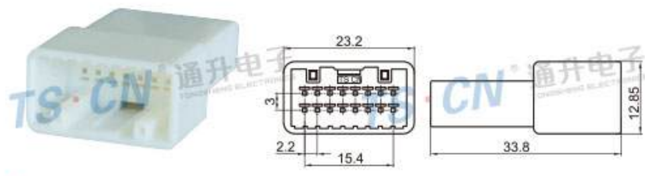
Type: TSTA16-16P-11-1 Material: PA66 Matching Terminal: TSZ208
