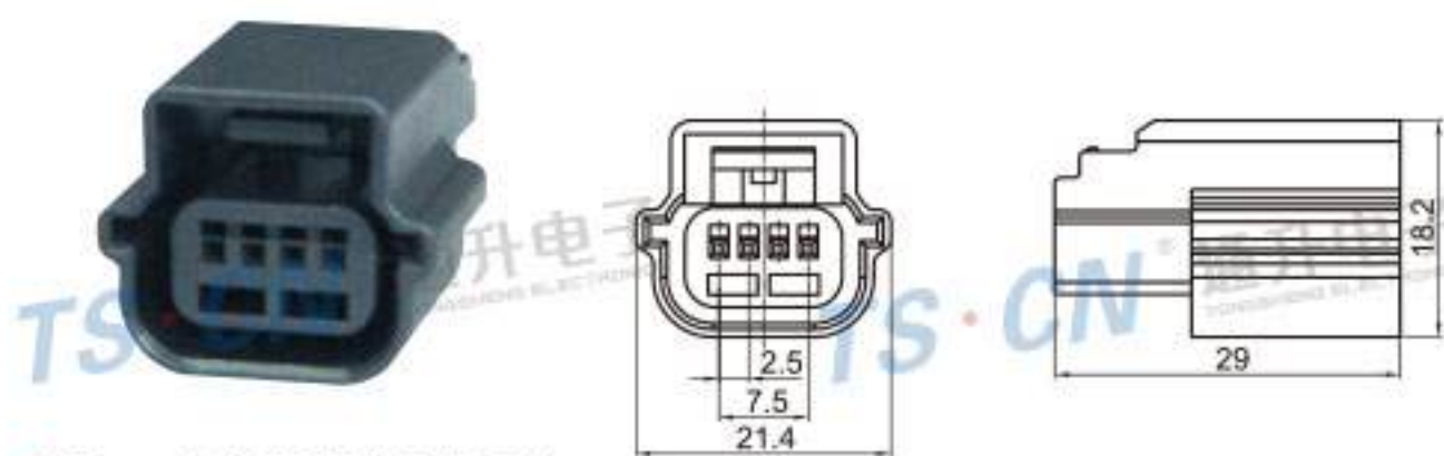
Type: TS30094-04P-21 Material: PA66 GF30% Matching Terminal: TSH143
