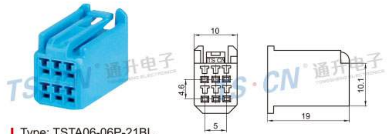
Type: TSTA06-06P-21BL Material: PA66 Matching Terminal: TSH076
