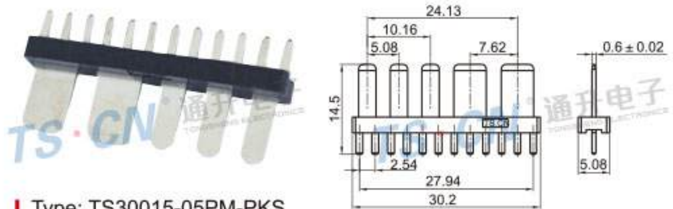
Type: TS30015-05PM-PKS Material: PA66 Matching Terminal: TSPM0155 / TSPM0156
