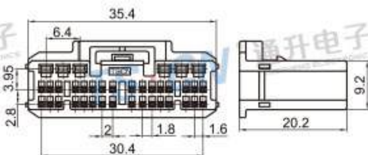
Type: TS30101-38P-21 Material: PA66 Matching Terminal: TSH593 / TSH600
