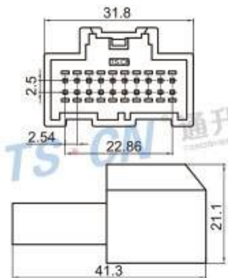
Type: TSGM20-20P-11-5 Material: PA66 GF30% Matching Terminal: TSZ208B
