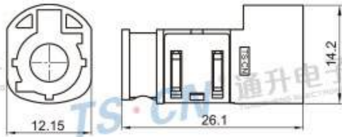
Type: TSVW10-04PM-AT-5WT-1 Material: PA66 GF15% Matching Terminal: TSPM0175 / TSTM0051
