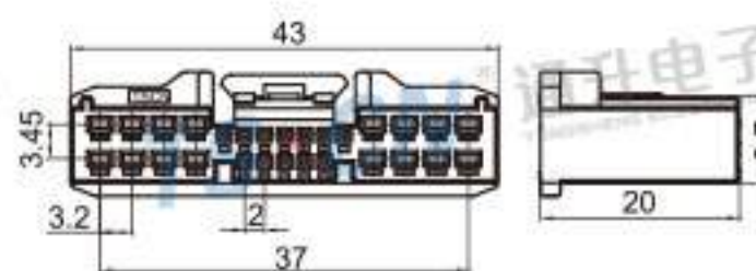
Type: TS30243-28P-21 Material: PA66 Matching Terminal: TSH593 / TSH606
