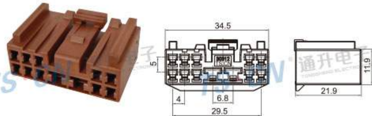
Type: TS30312-12P-21 Material: PBT Matching Terminal: TSH585 / TSH064
