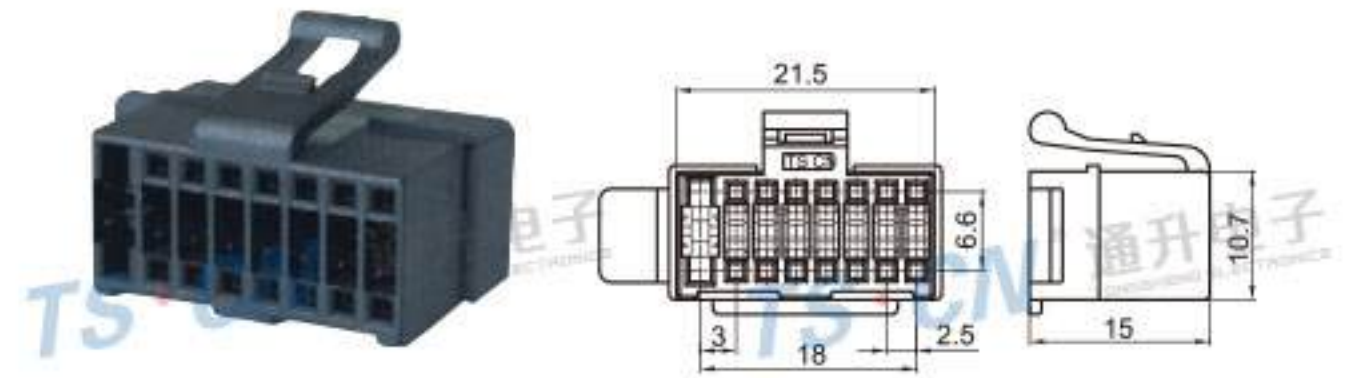
Type: TSPAN16E-16P-21 Material: PA66 GF30% Matching Terminal: TSH114 / TSH113
