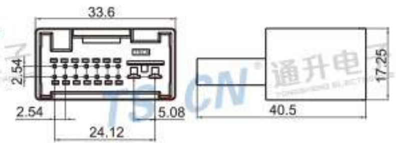
Type: TS30230-16P-11-2 Material: PBT Matching Terminal: TSZ024B / TSZ616
