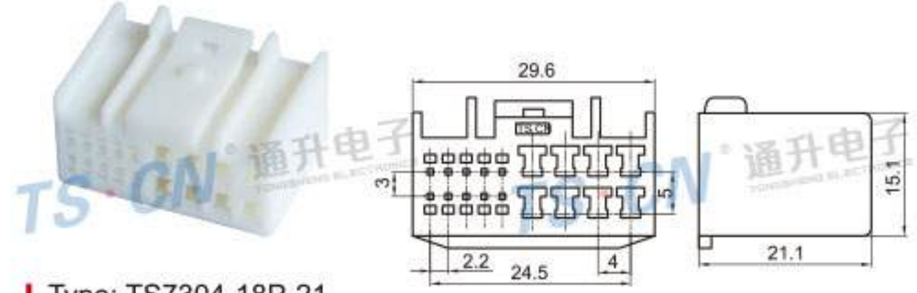
Type: TS7304-18P-21 Material: PA66 Matching Terminal: TSZ064 / TSH143
