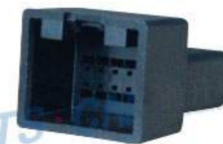
Type: TSGM12-12P-11-1 Material: PA66 GF30% Matching Terminal: TSZ208B
