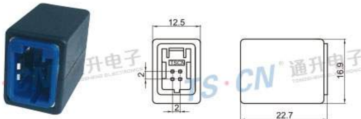
Type: TSMA04-04PM-AH-2 Material: PA66 GF30% Matching Terminal: TSAF0029 / TSPM0030
