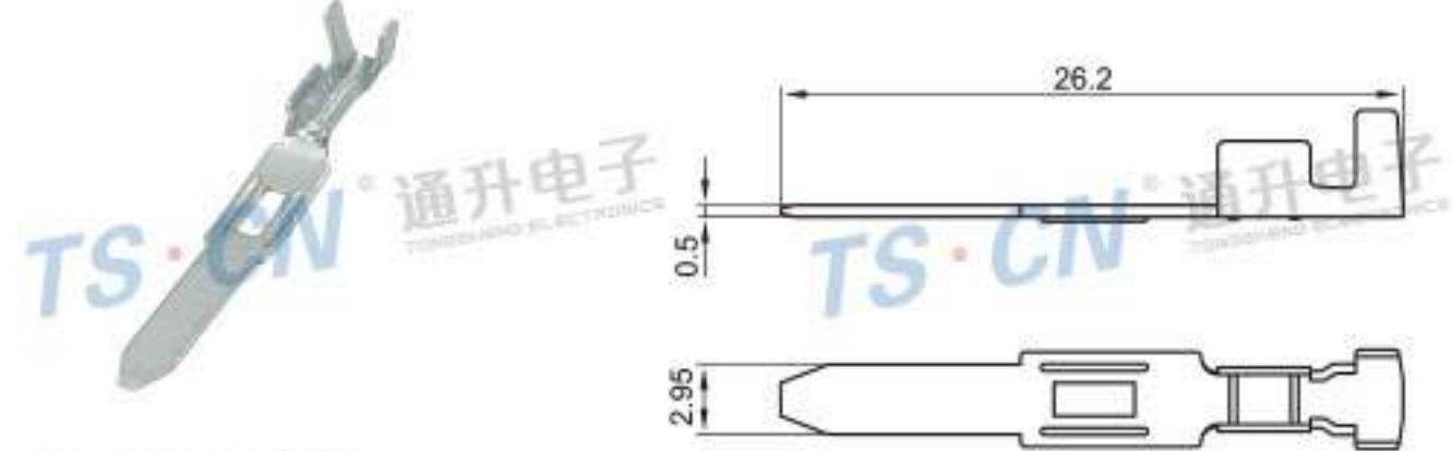
Type: TS1388 Material: Brass
