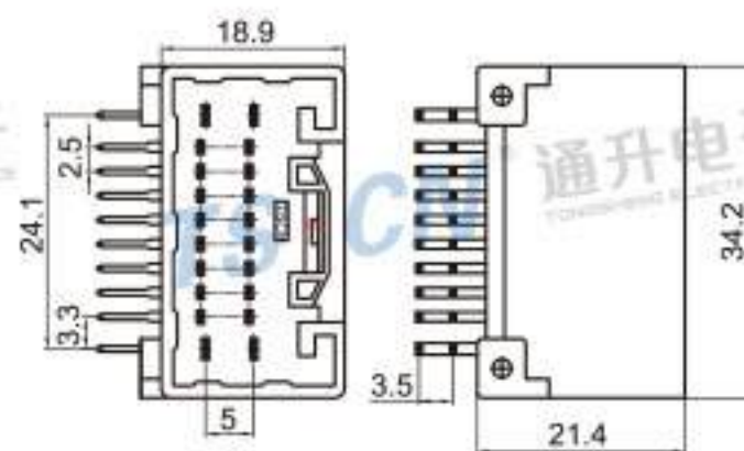
Type: TS8113-20PM-PKB Material: PA66 Matching Terminal: TSPM0001~TSPM0004
