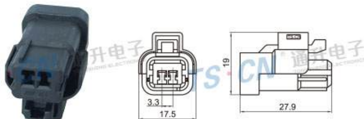
Type: TS30067-02P-21-1 Material: PA66 GF30% Matching Terminal: TSH047
