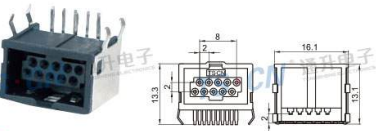
Type: TS3004-10PM-PKB Material: PA66 Matching Terminal: NIL
