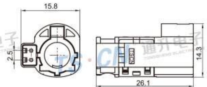
Type: TSVW10-06PM-AT-1VT Material: PBT GF15% Matching Terminal: TSPM0175 / TSTM0051 / TSZ208
