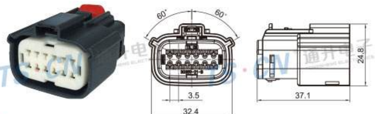
Type: TS30359-12P-21 Material: PA66 GF30% Matching Terminal: TSH047
