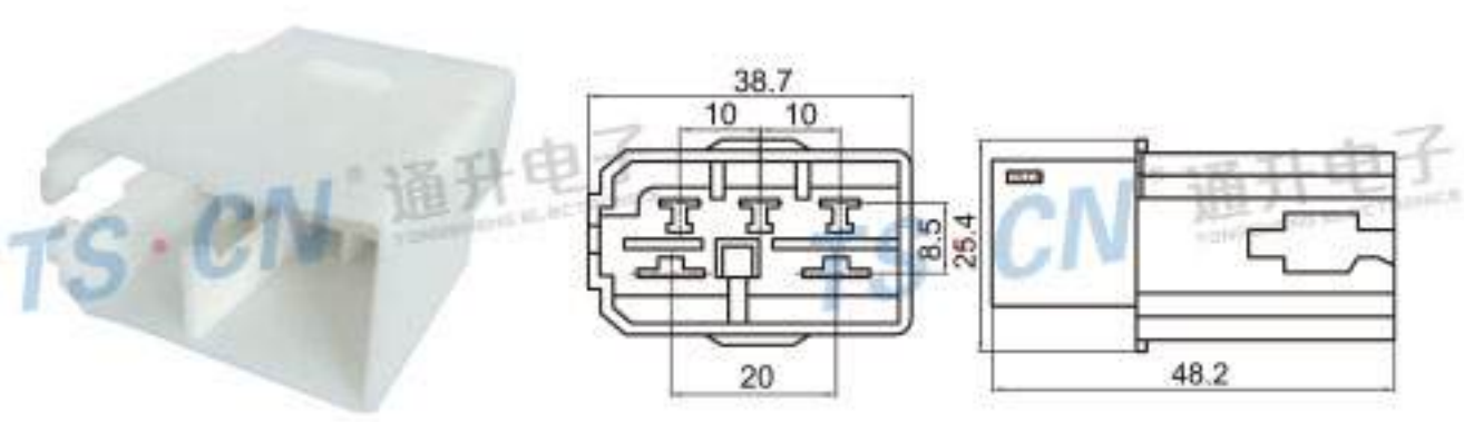
Type: TS30013-05P-11 Material: PBT Matching Terminal: TSZ552 / TSZ551
