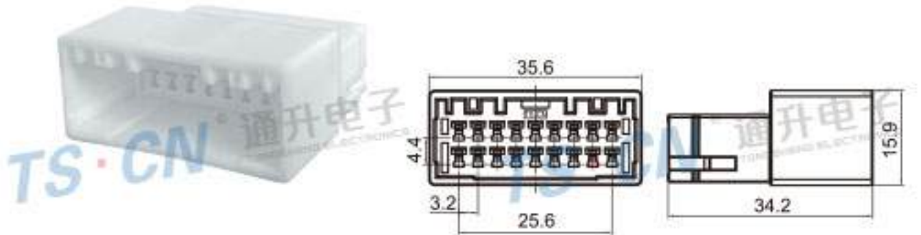
Type: TS30320-18P-11 Material: PBT Matching Terminal: TSZ619
