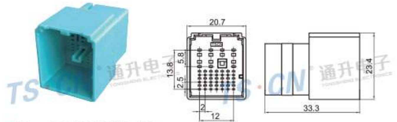
Type: TS30205-28P-11-2 Material: PA66 Matching Terminal: TSZ566 / TSZ561
