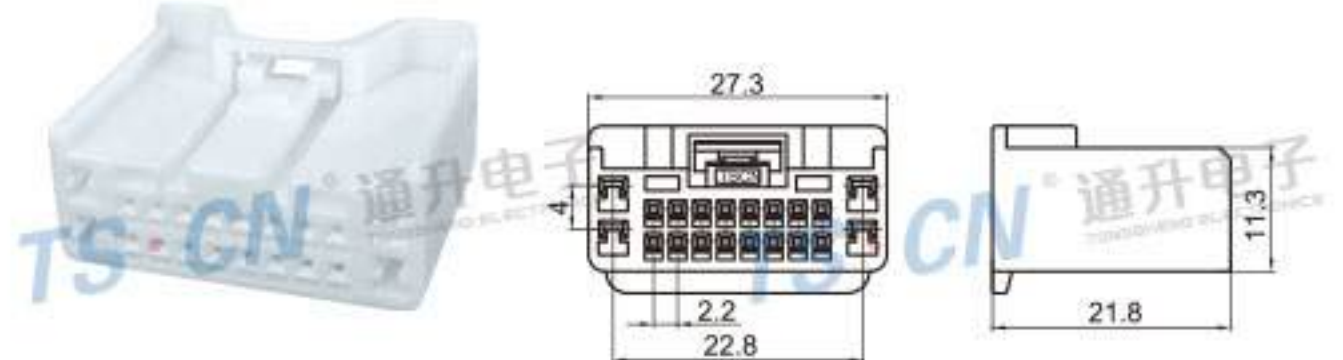
Type: TS30202-20P-21 Material: PA66 Matching Terminal: TSH541 / TSH143
