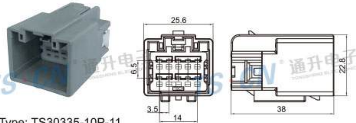
Type: TS30335-10P-11 Material: PBT GF15% Matching Terminal: TSZ144A
