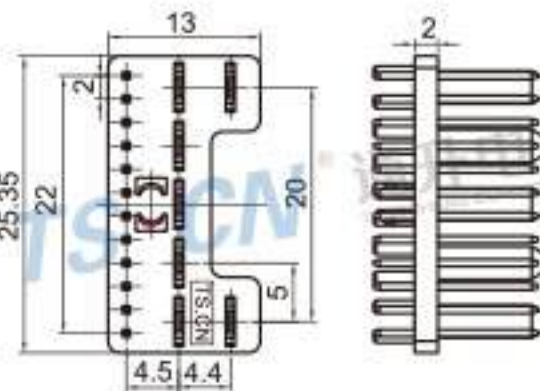
Type: TS30299-19PM-PKS Material: PA66 GF30% Matching Terminal: TSPM0154 / TSPM0299
