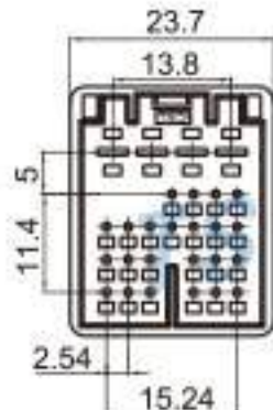
Type: TS30217-30P-11-5 Material: PBT GF15% Matching Terminal: TSDJ615B-2.8*0.8B / TSZ208
