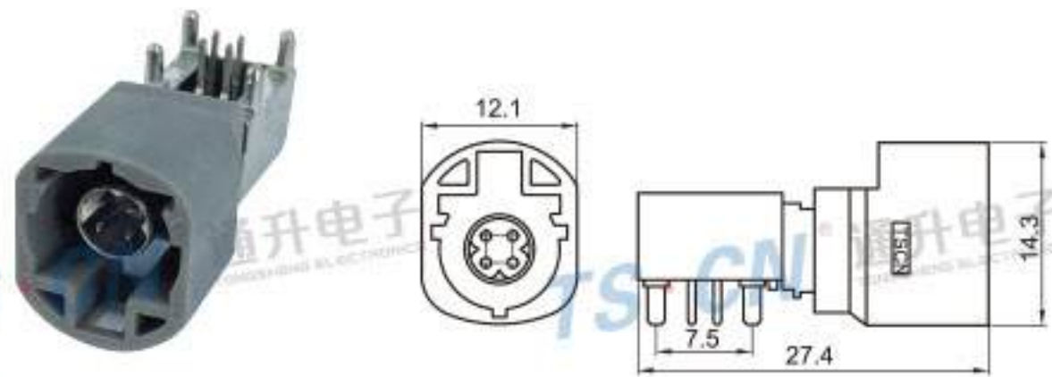
Type: TSVW10-04PM-AT-5GY Material: PA66 GF30% Matching Terminal: TSPM0021~TSPM0025
