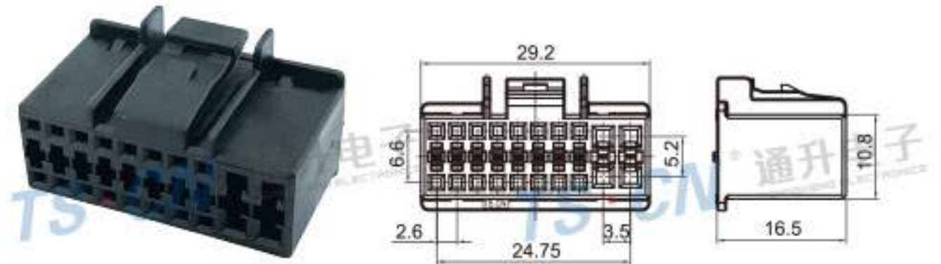
Type: TS30322-20P-21 Material: PA66 GF30% Matching Terminal: TSH032 / TSH031
