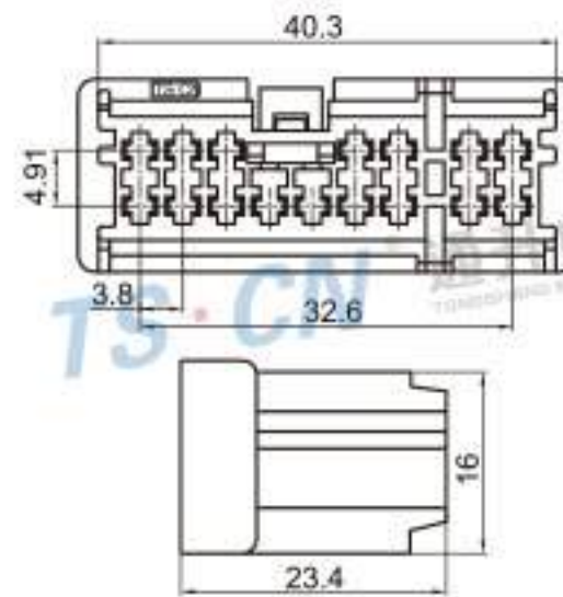
Type: TS7301A-16P-21-2 Material: PA66 Matching Terminal: TSH009
