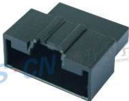
Type: TS5524-26P-11 Material: PA66 GF30% Matching Terminal: TSZ08B
