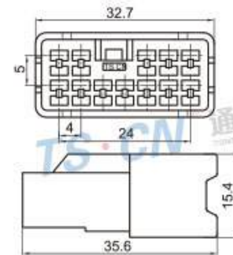
Type: TS7992-12P-11 Material: PA66 Matching Terminal: TSZ003
