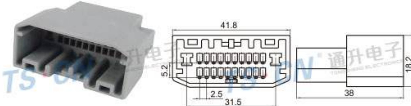
Type: TS6522-22P-11 Material: PA66 Matching Terminal: TSZ143 / TSZ145
