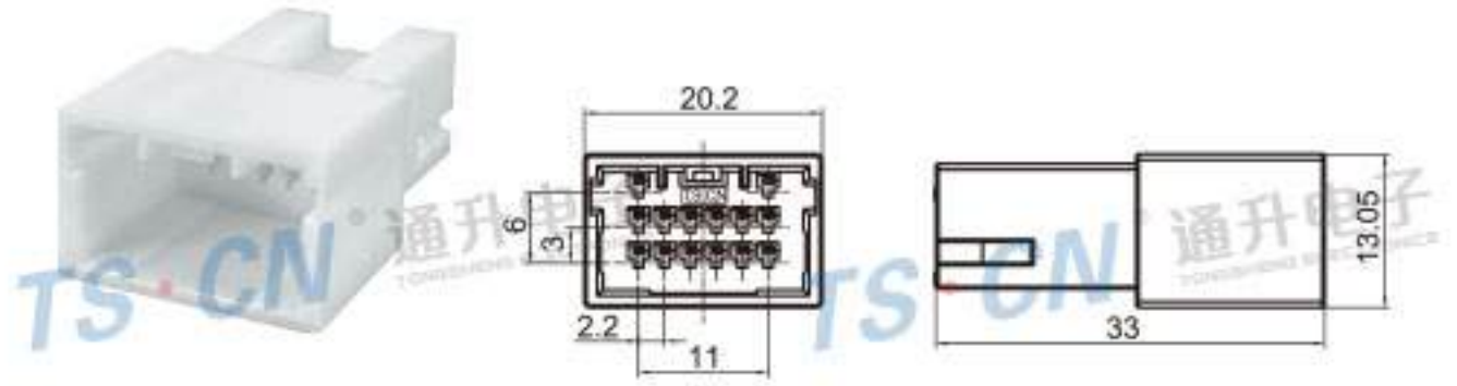
Type: TS30306-14P-11 Material: PA66 Matching Terminal: TSZ618
