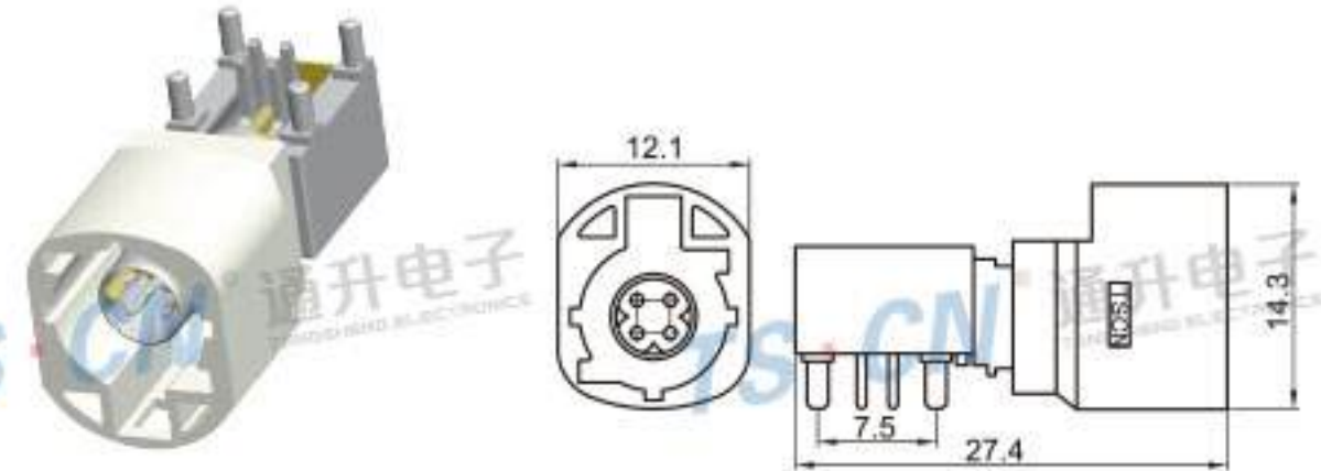
Type: TSVW10-04PM-AT-5WT Material: PA66 GF30% Matching Terminal: TSPM0021~TSPM0025
