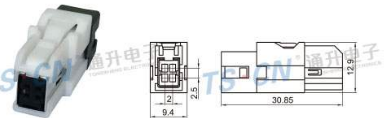
Type: TS30123-04PF-AH Material: PBT Matching Terminal: TSAF0032 / TSAF0033 / TSH600
