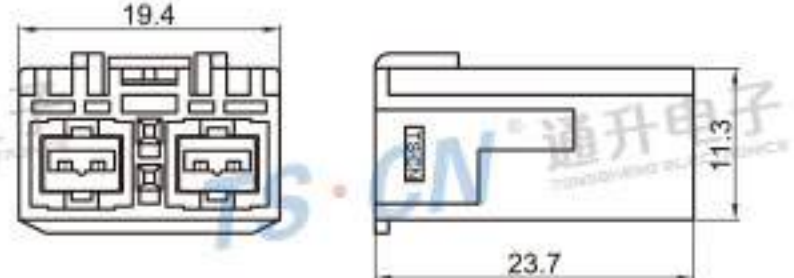
Type: TSNI06-06PF-AT Material: PA66 Matching Terminal: TSH143 / TSTF0006 / TSTF0020
