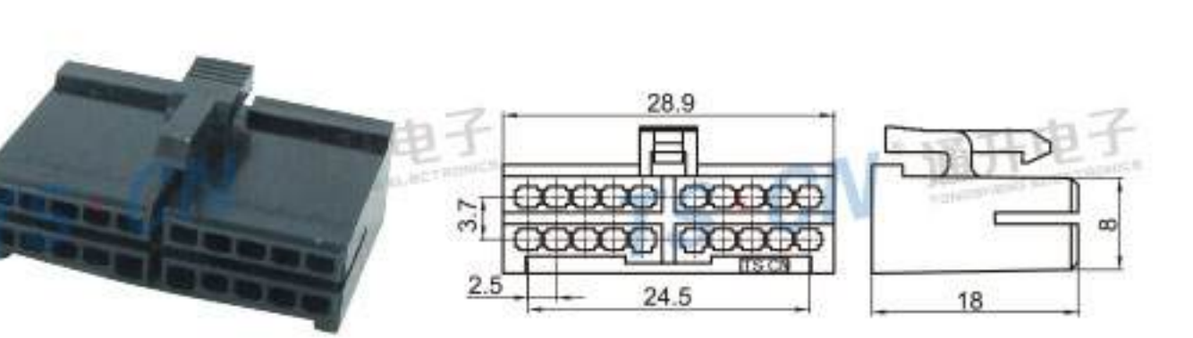
Type: TSJEN-20P-21-1 Material: PA66 GF15% Matching Terminal: TSH034 / TSH060
