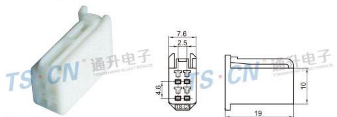
Type: TSTA04-04P-21 Material: PA66 Matching Terminal: TSH076
