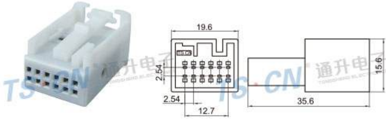
Type: TSVW12-12P-21WT Material: PA66 Matching Terminal: TSH143
