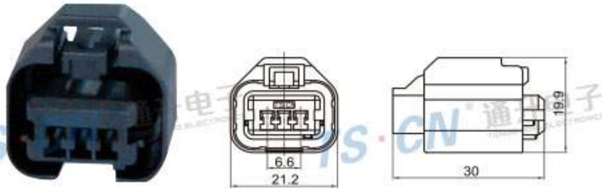
Type: TS30066-03P-21 Material: PA66 Matching Terminal: TSH047
