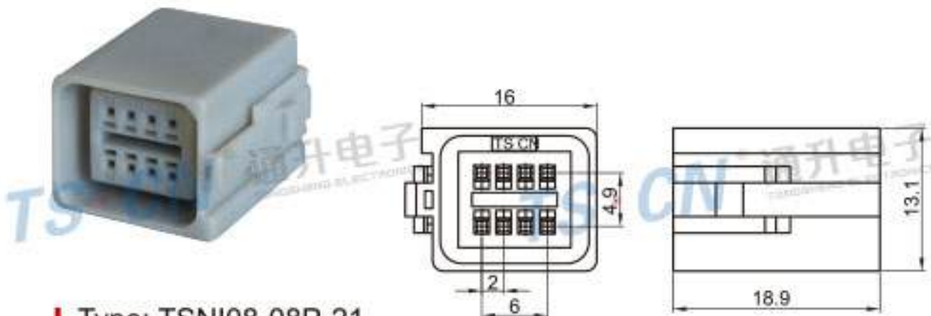
Type: TSNI08-08P-21 Material: PA66 GF30% Matching Terminal: TSHY66
