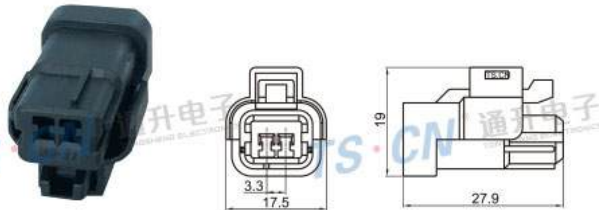
Type: TS30067-02P-21 Material: PA66 GF30% Matching Terminal: TSH047
