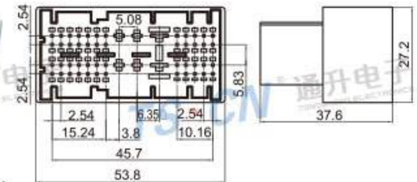
Type: TS30139-54P-11 Material: PBT GF15% Matching Terminal: TSZ028 / TSZ024B / TSZ208B
