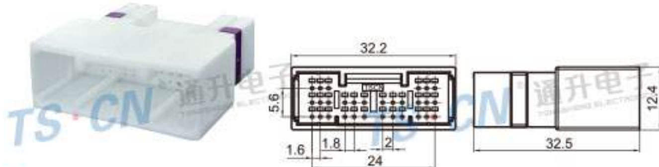
Type: TS30101-30P-11-5 Material: PA66 Matching Terminal: TSZ615
