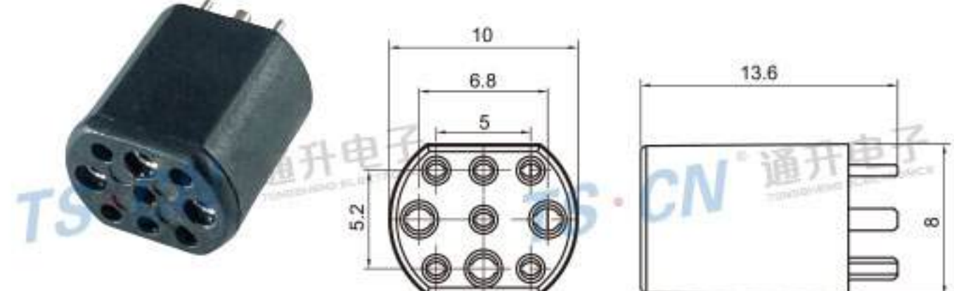
Type: TS30269-09PF-PKS Material: PA66 GF30% Matching Terminal: 0.9 母针 / 1.3 母针
