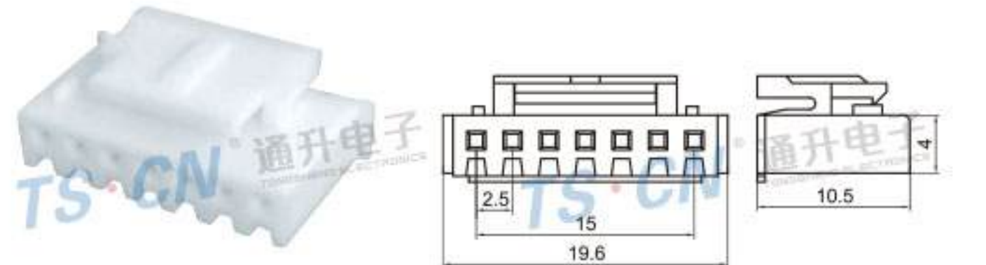
Type: TSHA-07P-21(02P-15P) Material: PA66 Matching Terminal: TSC3
