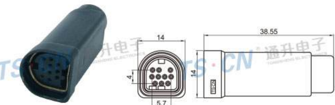
Type: TSALPH-10PF-AH-1 Material: PA66 Matching Terminal: NIL
