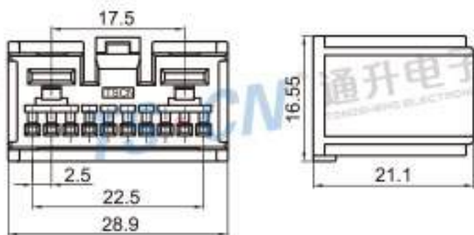
Type: TS30099-12P-21 Material: PA66 Matching Terminal: TSH585 / TSH076
