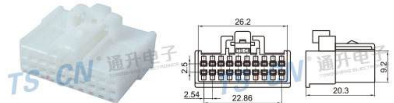
Type: TSPAN20-20P-21 Material: PA66 Matching Terminal: TSH053
