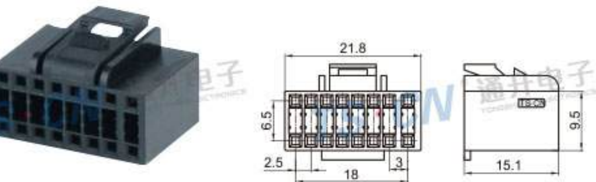
Type: TSALP16-16P-21-1 Material: PA66 GF30% Matching Terminal: TSH031B
