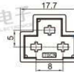
Type: TS30182-03P-11 Material: PA66 Matching Terminal: TSZ024
