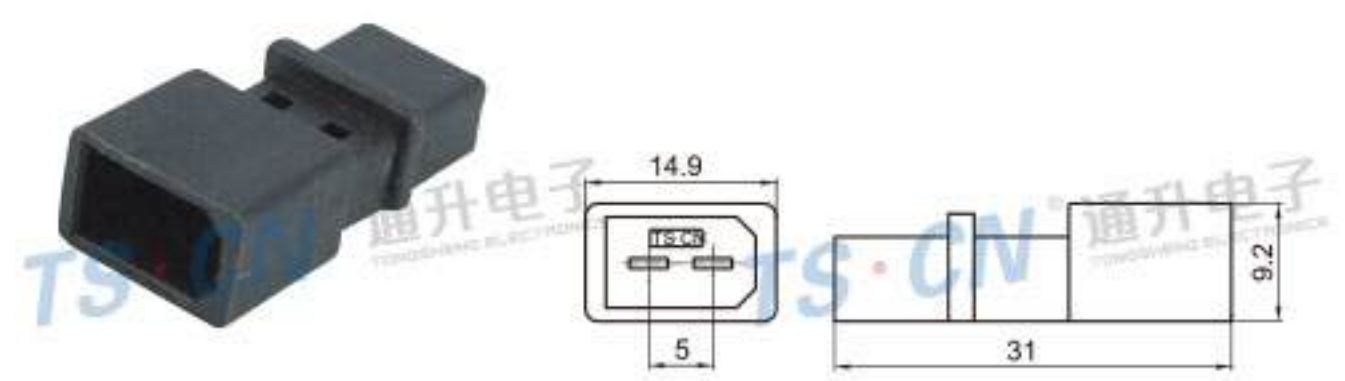
Type: TS7022-3.5-11 Material: PA66 Matching Terminal: NIL
