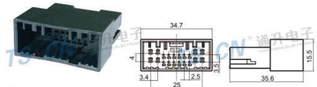
Type: TS30302-20P-11 Material: PBT Matching Terminal: TSZ040 / TSZ616
