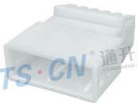
Type: TS30342-20P-11 Material: PA66 Matching Terminal: TSZ615
