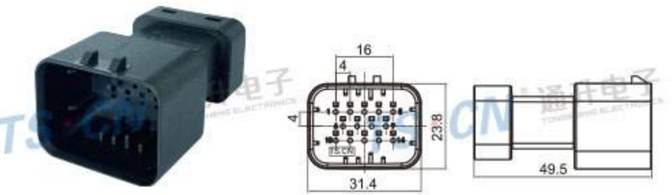
Type: TS30256-14P-11(TS3016) Material: PBT GF15% Matching Terminal: TSZ072
