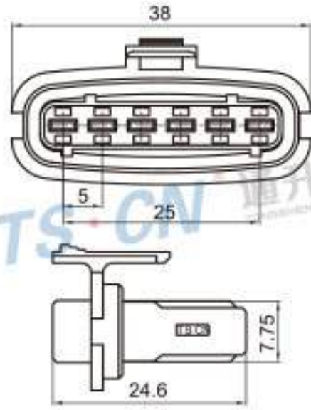
Type: TSBS06-06P-21 Material: PA66 GF30% Matching Terminal: TSH019
