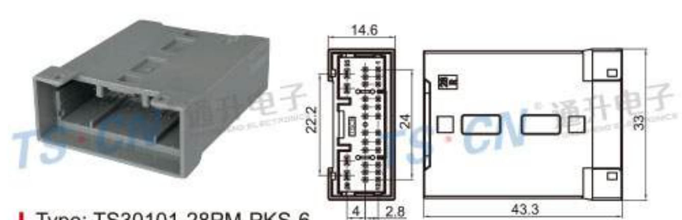
Type: TS30101-28PM-PKS-6 Material: PBT GF15% Matching Terminal: TSPM0331 / TSPM0305
