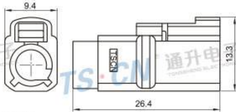
Type: TSVW20-01PF-AT-CU Material: PA66 GF30% Matching Terminal: TSTF0025 / TSTF0026
