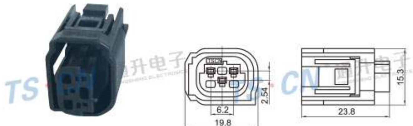
Type: TS30119-03P-21 Material: PBT Matching Terminal: TSH143
