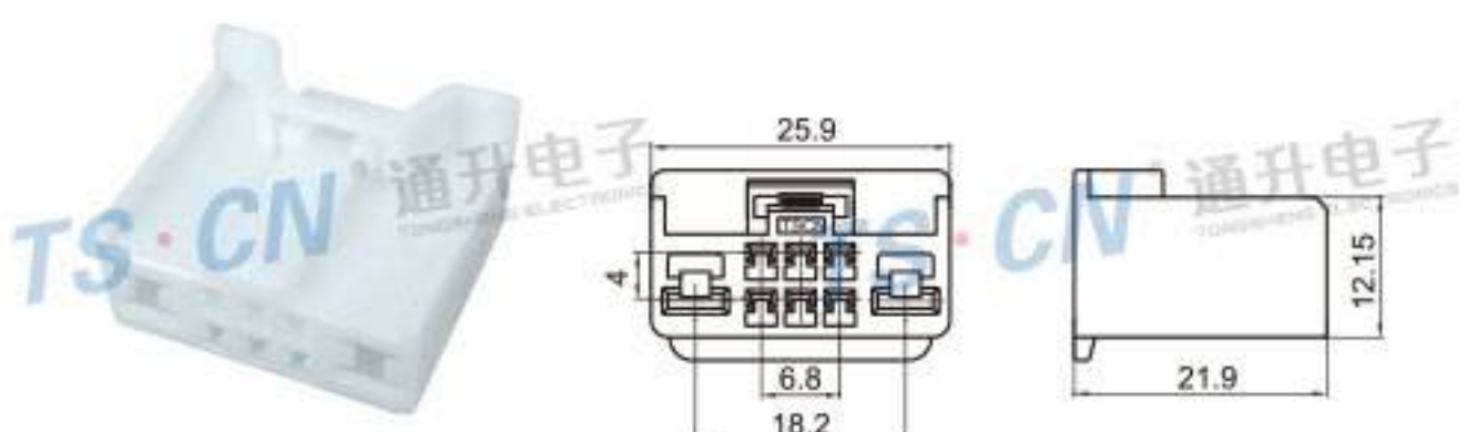
Type: TS30201-08P-21 Material: PA66 Matching Terminal: TSH541 / TSH585
