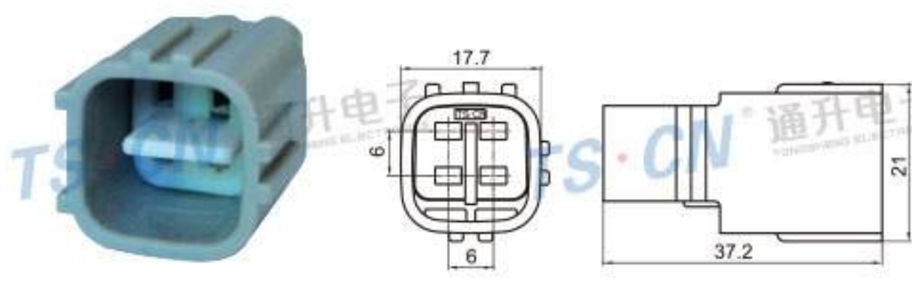
Type: TS1053-04P-11 Material: ABS Matching Terminal: TSZ045
