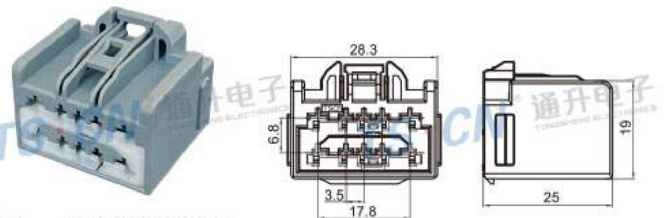
Type: TS30337-10P-21 Material: PBT GF15% Matching Terminal: TSH085 / TSH047
