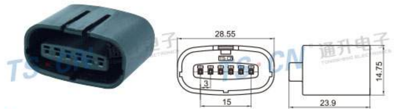
Type: TSTA06-06P-21-1 Material: PA66 GF30% Matching Terminal: TSH143
