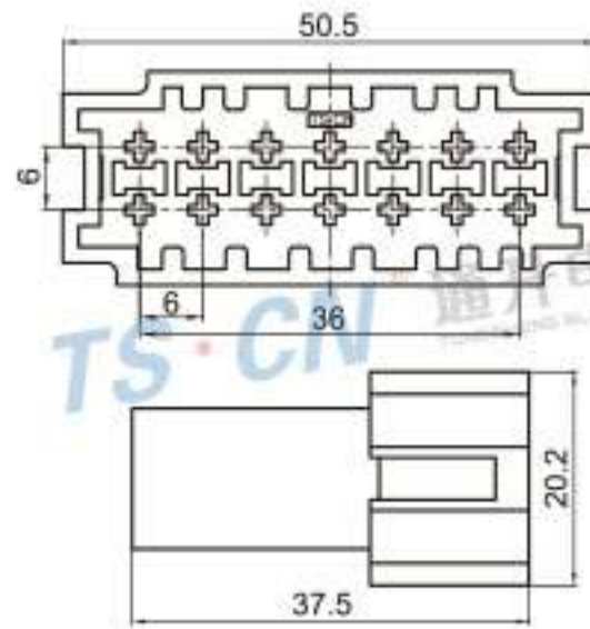
Type: TSBZ14-14P-11 Material: PA66 Matching Terminal: TSZ024
