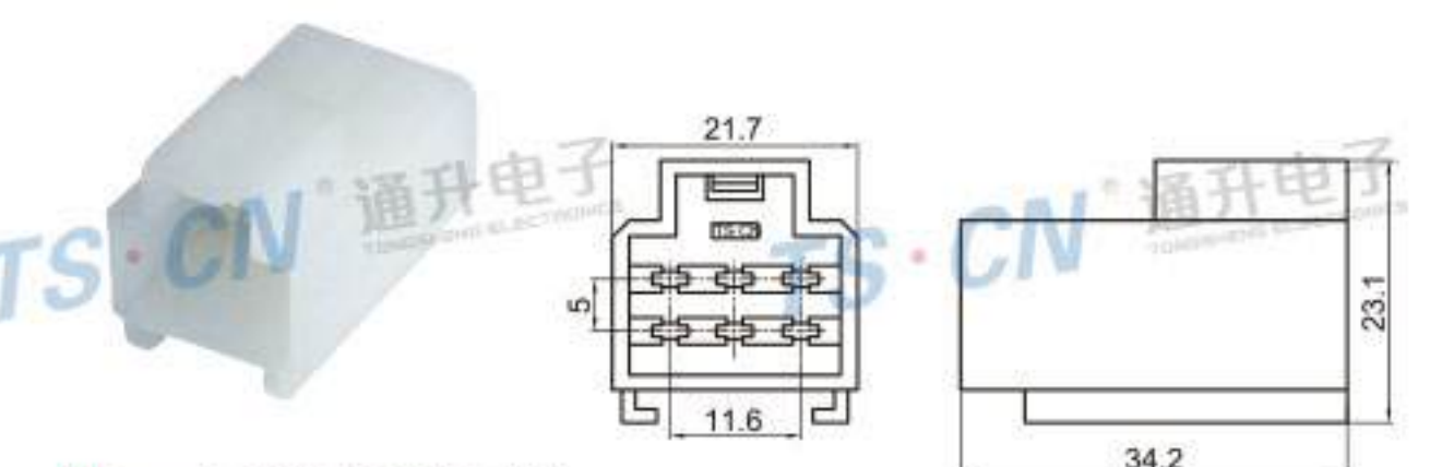
Type: TS1763-06P-11-1 Material: PA66 Matching Terminal: TSZ024
