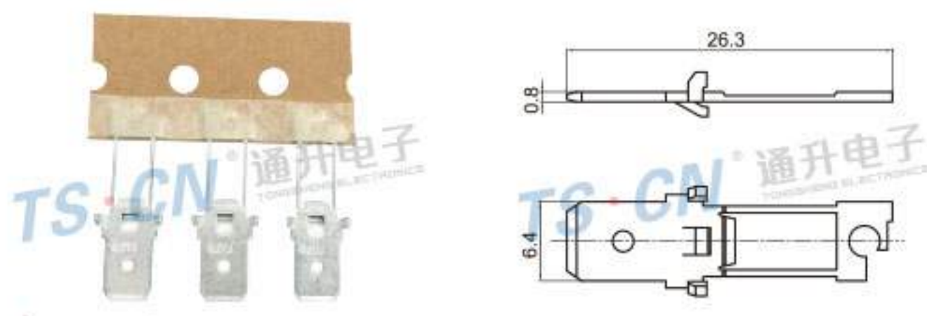
Type: TSZ569 Material: Brass
