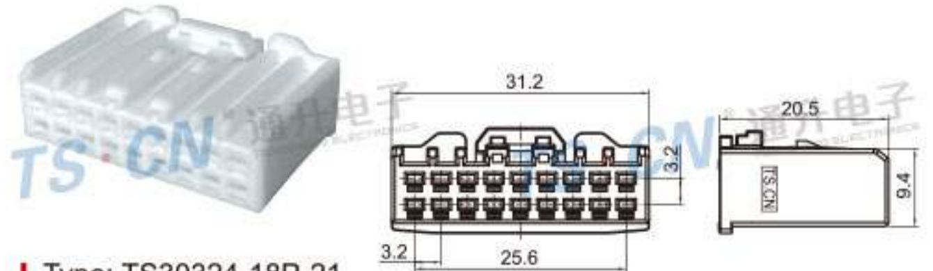
Type: TS30324-18P-21 Material: PBT Matching Terminal: TSH593
