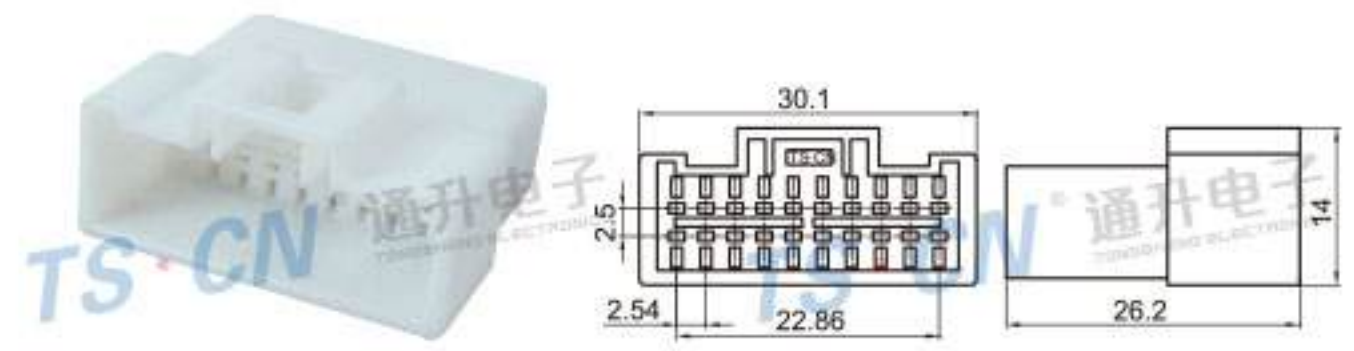
Type: TSPAN20-20P-11 Material: PA66 Matching Terminal: TSZ007B
