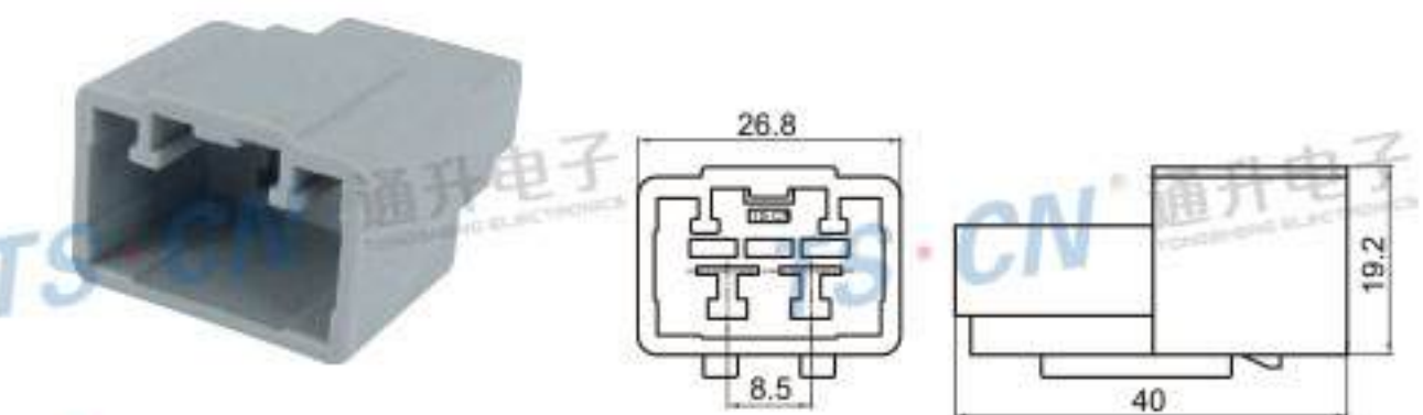
Type: TSVO02-02P-11 Material: PA66 Matching Terminal: TSZ539
