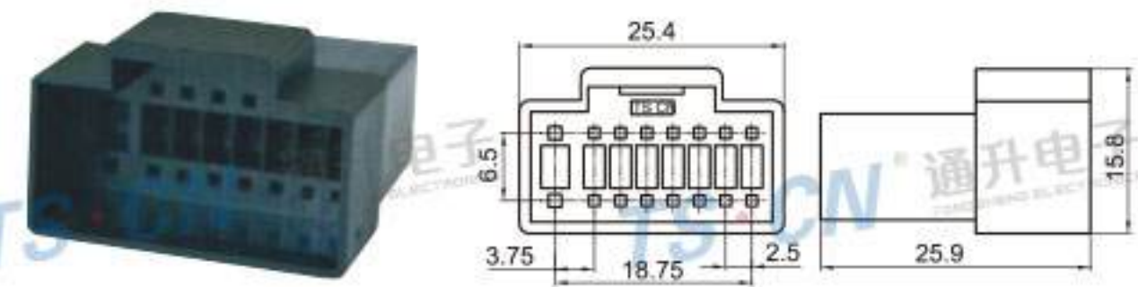
Type: TSALP04-16P-11 Material: PA66 GF30% Matching Terminal: TSZ532 / TSZ533
