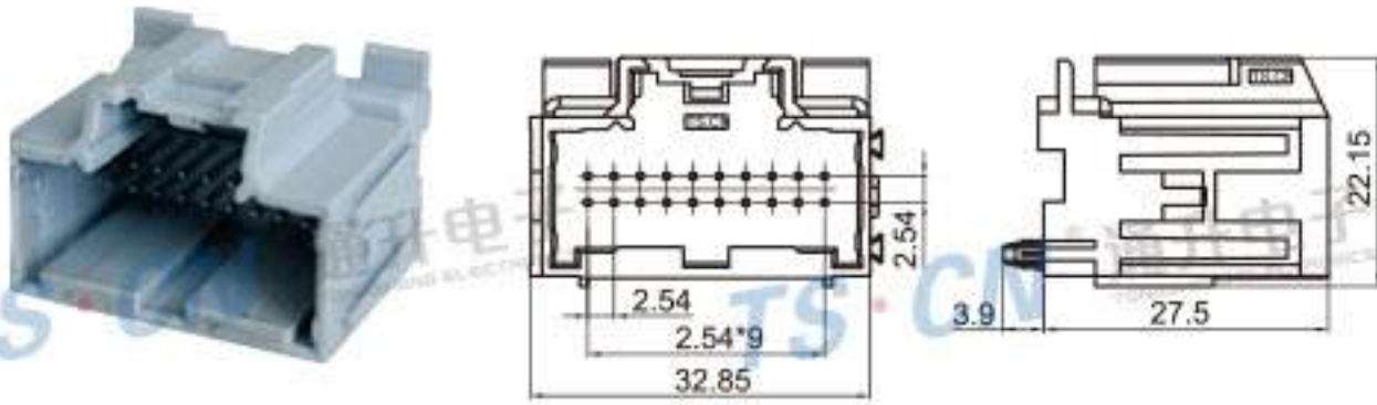
Type: TS30040-20PM-PKS Material: PBT GF15% Matching Terminal: TSPM0128
