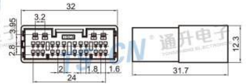
Type: TS30101-28P-11-1 Material: PA66 Matching Terminal: TSZ562 / TSZ556
