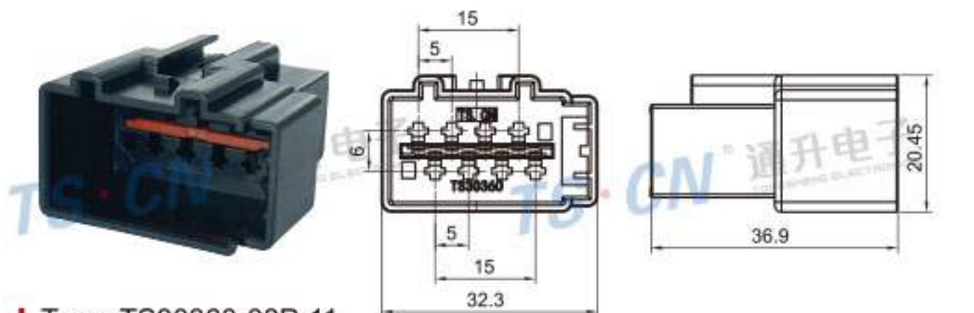
Type: TS30360-08P-11 Material: ABS Matching Terminal: TSZ143
