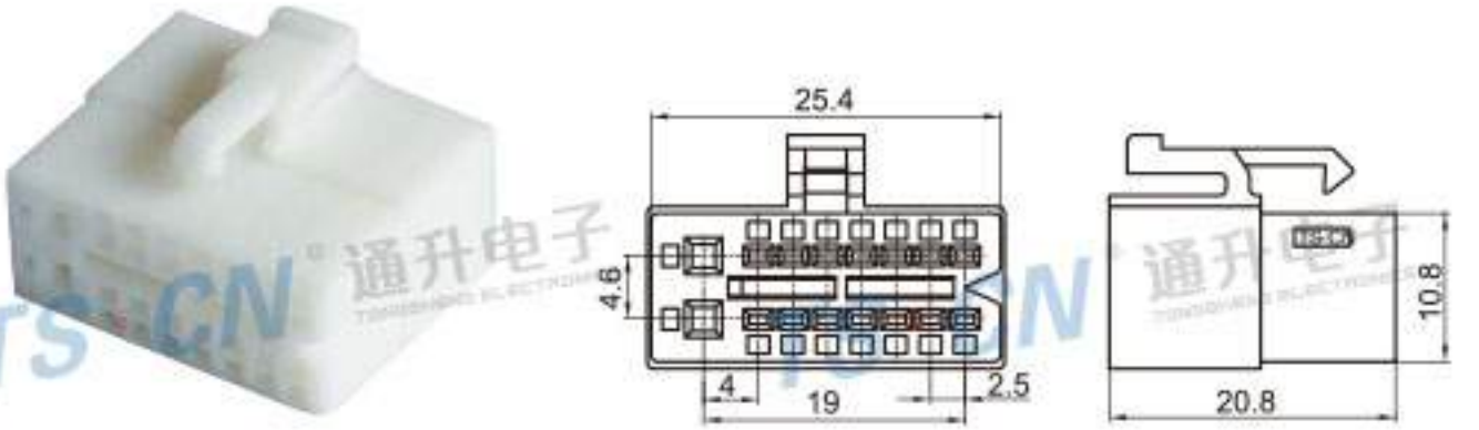
Type: TSCLR16-16P-21 Material: PA66 Matching Terminal: TSH052/TSH053
