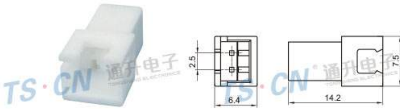
Type: TSXH-02R-11(02P-15P) Material: PA66 GF30% Matching Terminal: TSXH-RT
