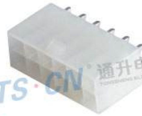
Type: TS5557-12PM-PKS(02P-24P) Material: PA66 Matching Terminal: TSPM0298
