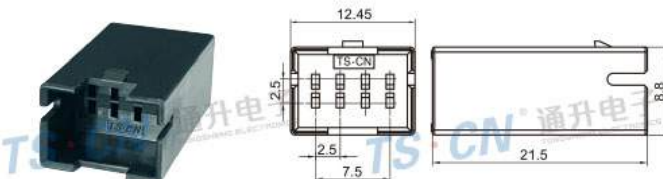
Type: TSPHC-08P-11 Material: PA66 Matching Terminal: TS25044-RT
