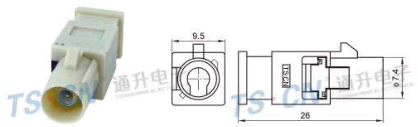
Type: TSVW10-01PM-AT-BE Material: PA66 Matching Terminal: TSTM0019 / TSTM0020
