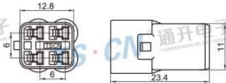
Type: TS30239-04P-21 Material: PBT Matching Terminal: TSDJ7045F-2.2-21
