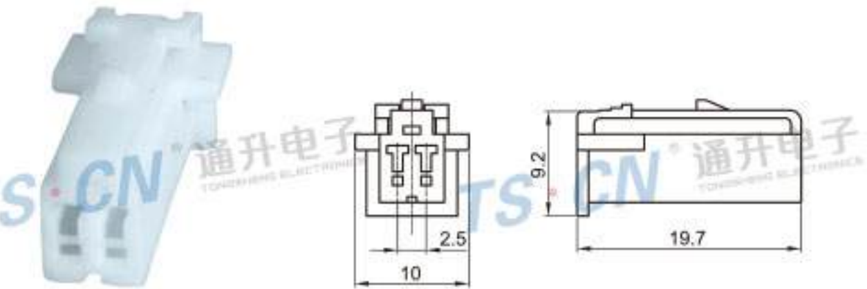
Type: TS30108-02P-21 Material: PBT Matching Terminal: TSH076
