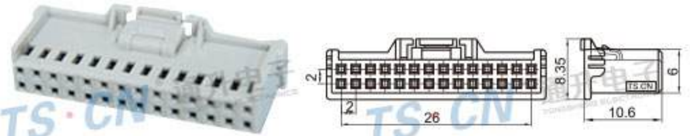
Type: TS30047-28P-21(QRA3) Material: PA66 GF15% Matching Terminal: TSPHB
