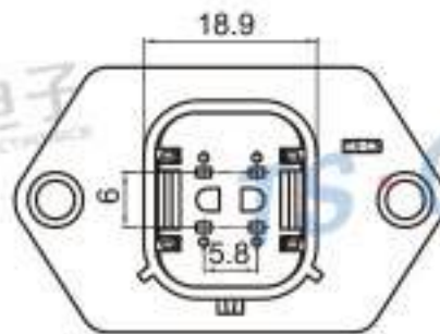
Type: TS02301-04P-11 Material: PBT GF15% Matching Terminal: TSZ144A
