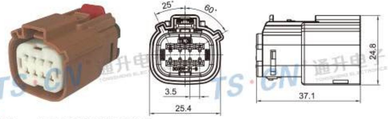
Type: TS30359-08P-21-2 Material: PA66 GF30% Matching Terminal: TSH047
