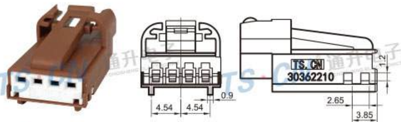
Type: TS30362-04P-21-2 Material: PA66 GF30% Matching Terminal: TSH006B
