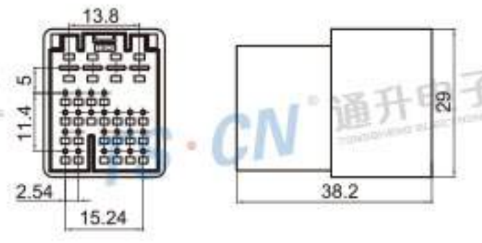
Type: TS30217-30P-11-2 Material: PBT GF15% Matching Terminal: TSDJ615B-2.8*0.8B / TSZ208
