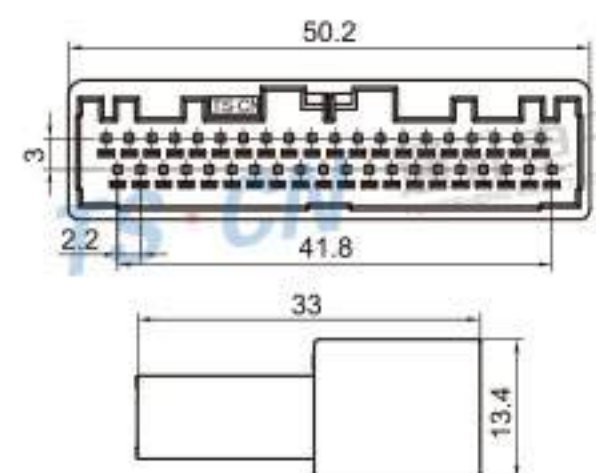
Type: TSCRV40-40P-11 Material: PA66 Matching Terminal: TSZ208B
