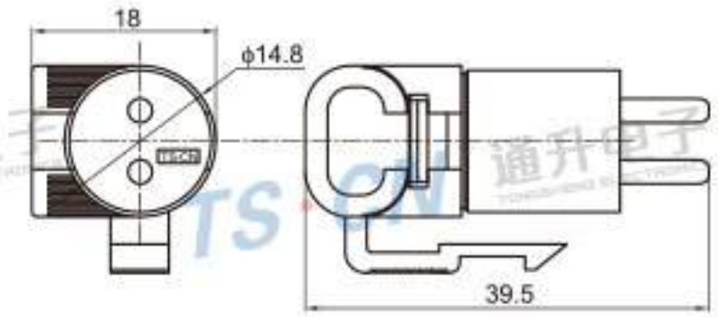
Type: TSNI02-02PF-AT Material: ABS Matching Terminal: TSTF0009 / TSTF0028
