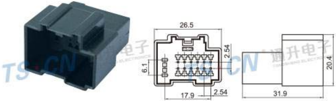
Type: TS2105-14P-11 Material: PA66 GF30% Matching Terminal: TSZ040 / TSZ018B
