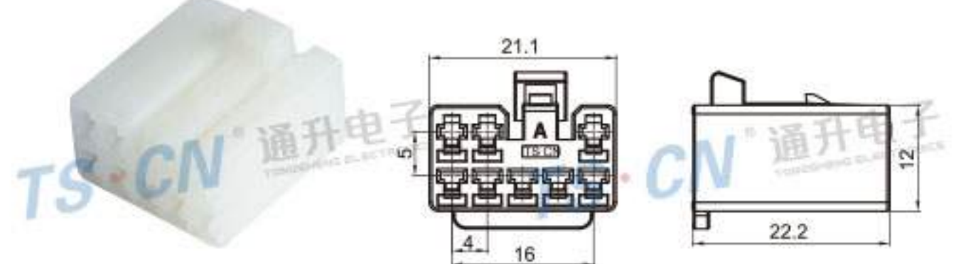
Type: TS1761-08P-21 Material: PA66 Matching Terminal: TSH009
