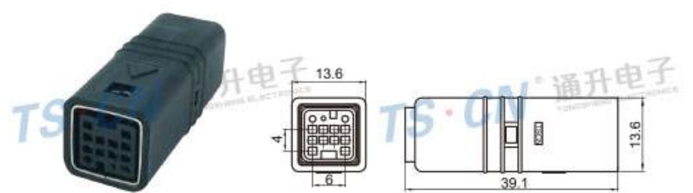
Type: TSCLR-13PF-AH Material: PA66 GF30% Matching Terminal: TSAF0017 / TSAF0018
