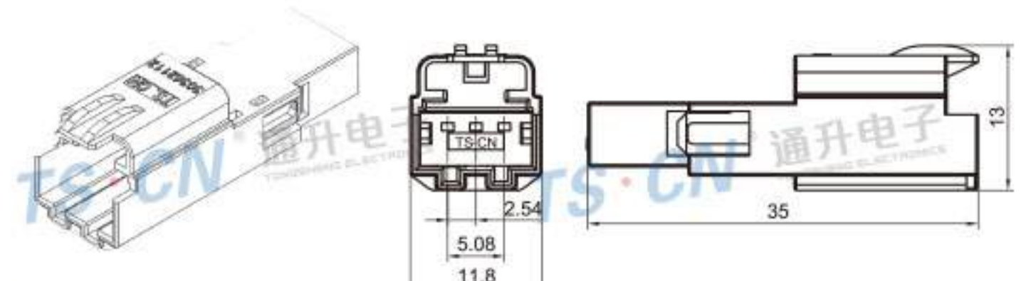
Type: TS30362-03P-11-2 Material: PA66 GF30% Matching Terminal: TSZ145
