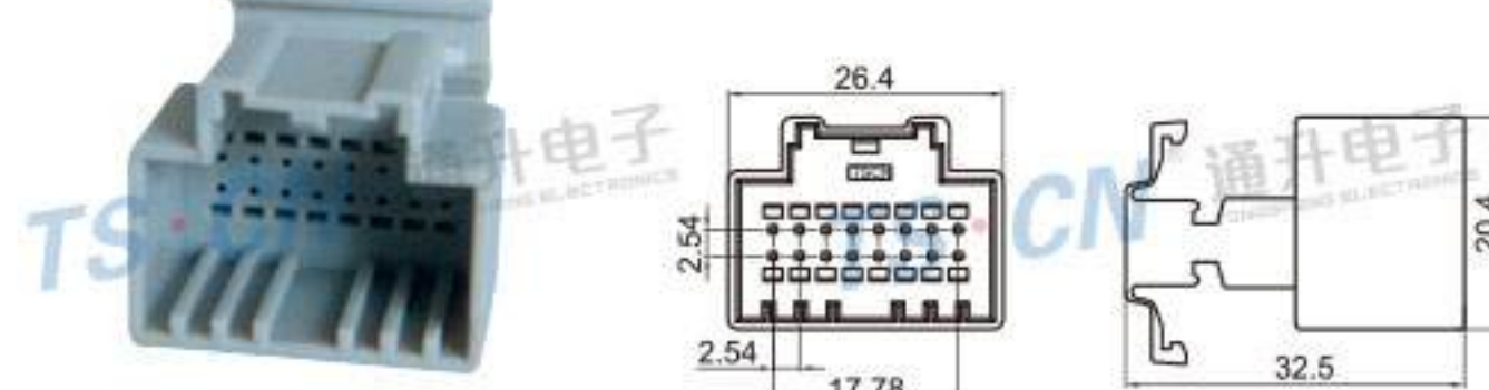
Type: TS30075-16P-11(2015) Material: PA66 GF15% Matching Terminal: TSZ208B
