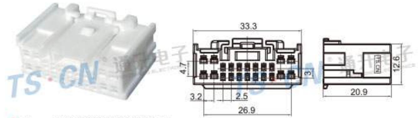
Type: TS30300-22P-21-1 Material: PBT Matching Terminal: TSH593 / TSH143
