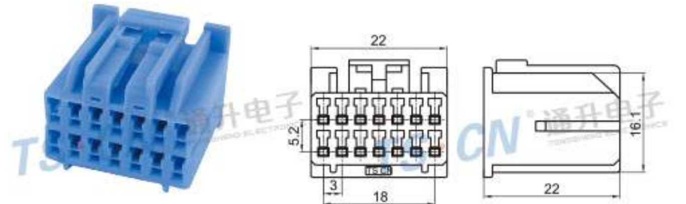
Type: TSHD14-14P-21 Material: PA66 Matching Terminal: TSH006
