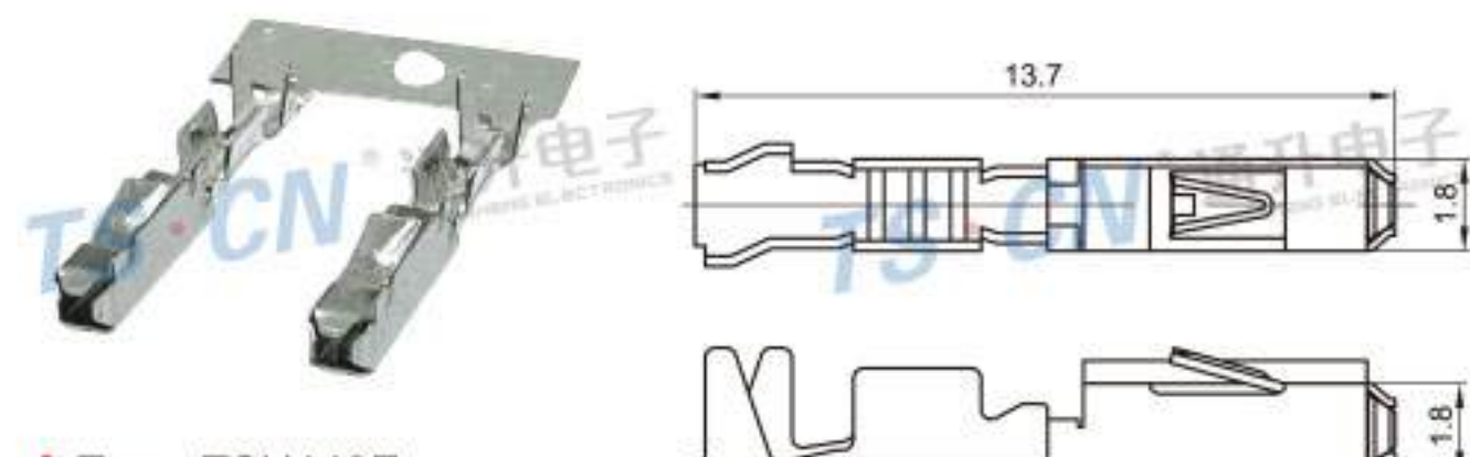
Type: TSH143E Material: Phos.bronze Applicable Thickness: 0.64
