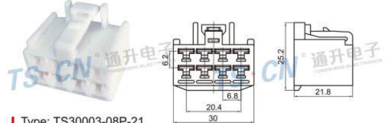
Type: TS30003-08P-21 Material: PBT Matching Terminal: TSH585
