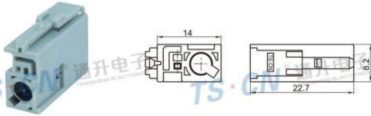
Type: TSHD21-02PF-AT-1 Material: PA66 Matching Terminal: TSH143 / TSTF0007 / TSTM0004
