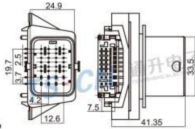
Type: TS30245-32PM-PKB-2 Material: GF30% PBT Matching Terminal: TSPM0289~TSPM0296
