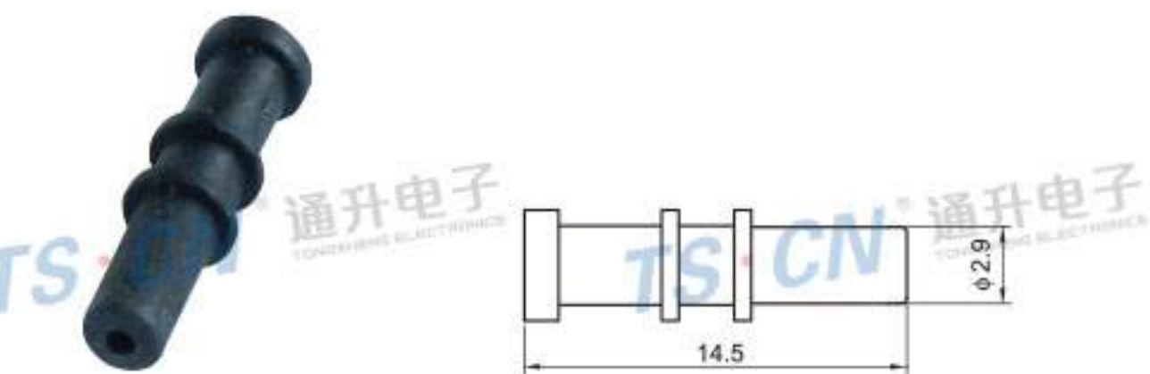
Type: TSBMGQ-B Material: PA66 GF30% Matching Terminal: NIL
