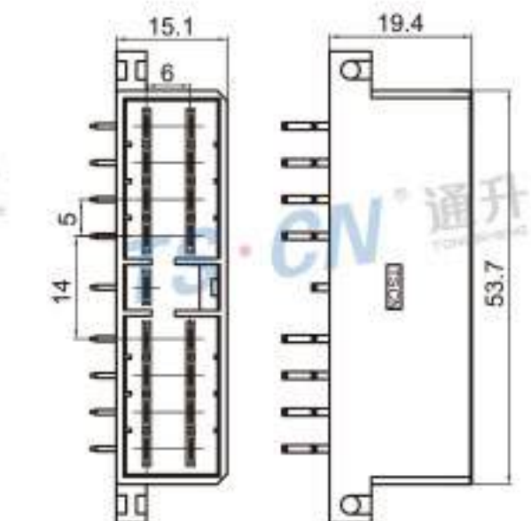
Type: TS1002-17PM-PKB Material: PA66 Matching Terminal: NIL
