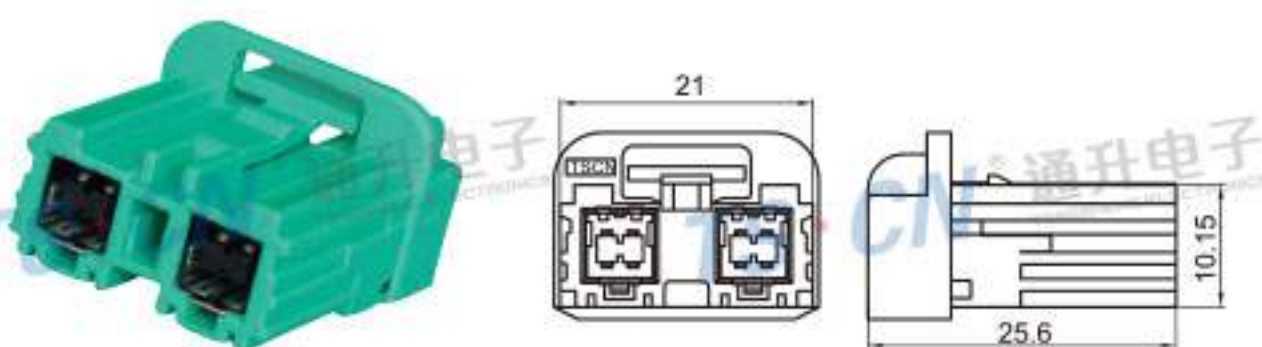
Type: TS1067-02PF-AT Material: PBT GF15% Matching Terminal: TSTF0008 / TSTF0010 / TSTF0011
