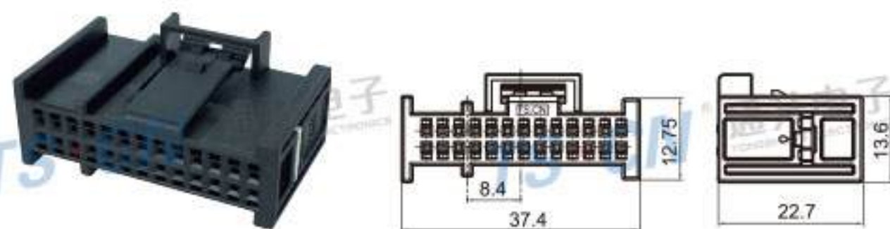
Type: TS30316-26P-21 Material: PA66 GF30% Matching Terminal: TSH624
