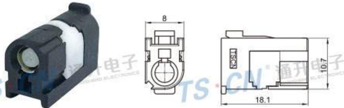
Type: TS1068-01PF-AT Material: PA66 Matching Terminal: TSTF0003 / TSTF0004
