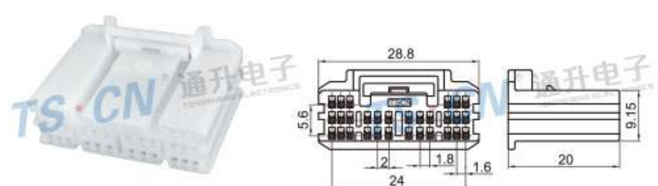
Type: TS30101-30P-21-1 Material: PA66 Matching Terminal: TSH600
