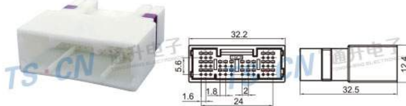
Type: TS30101-30P-11-6 Material: PA66 Matching Terminal: TSZ615
