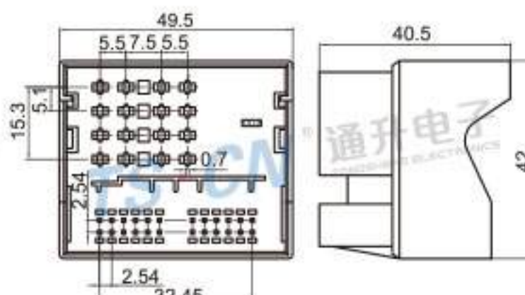
Type: TS9003-40P-11-7 Material: PA66 GF30% Matching Terminal: TSZ024B / TSZ208B
