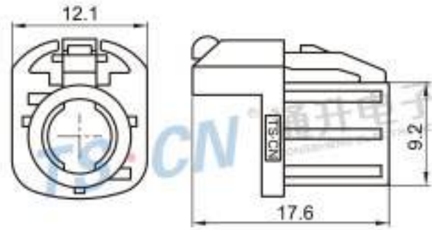
Type: TSVW20-04PF-AT-5PK Material: PA66 GF30% Matching Terminal: TSTF0048 / TSTF0049 / TSTF0050
