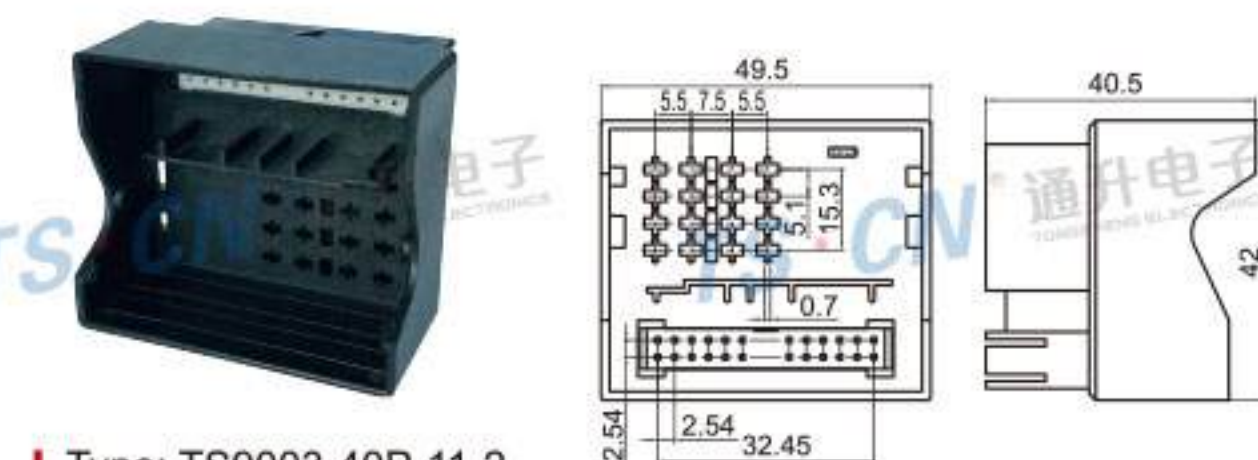
Type: TS9003-40P-11-2 Material: PA66 GF30% Matching Terminal: TSZ024B / TSZ208B
