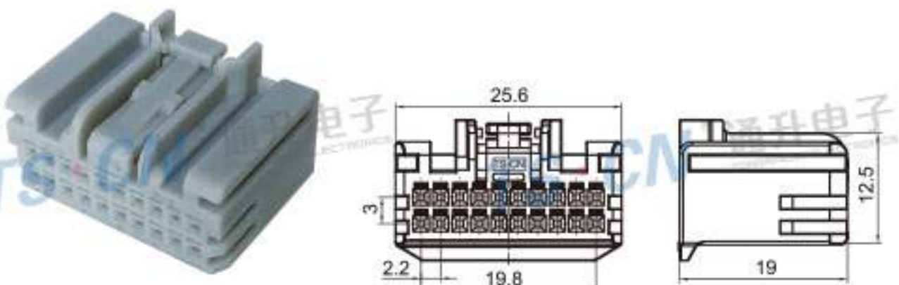
Type: TS30305-20P-21 Material: PA66 Matching Terminal: TSH143
