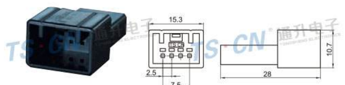
Type: TSTA04-04P-11-1 Material: PA66 Matching Terminal: TSZ208
