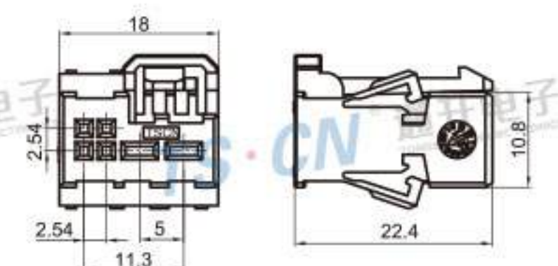
Type: TS30346-06P-21 Material: PA66 Matching Terminal: TSH091 / TSH624
