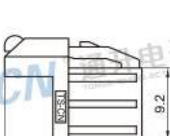
Type: TSVW20-04PF-AT-5BL Material: PA66 GF30% Matching Terminal: TSTF0048 / TSTF0049 / TSTF0050
