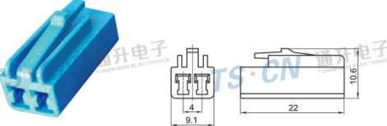
Type: TS30146-02P-21-2 Material: PA66 Matching Terminal: TSH009
