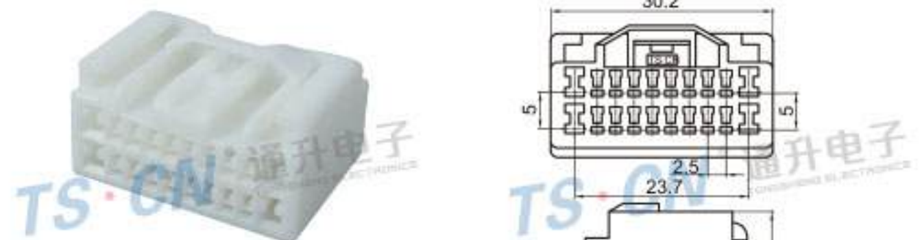
Type: TS8113-20P-21 Material: PA66 Matching Terminal: TSH009 / TSH006
