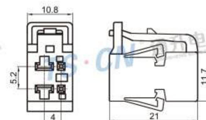
Type: TS30148-04P-21WT Material: PBT Matching Terminal: TSH091 / TSH092
