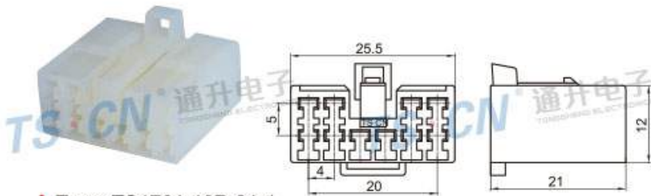
Type: TS1761-10P-21-1 Material: PA66 Matching Terminal: TSH009
