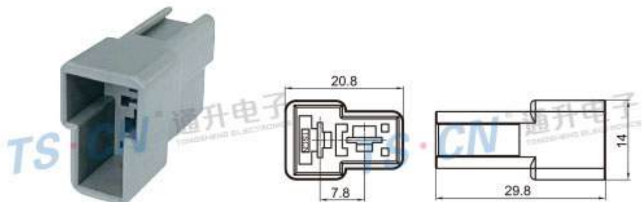
Type: TS30355-02P-11 Material: PBT Matching Terminal: TSZ538A
