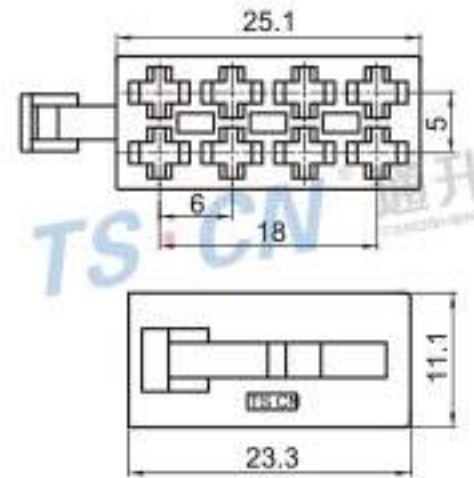
Type: TS1784A-08P-21-4BN Material: PA66 Matching Terminal: TSH019
