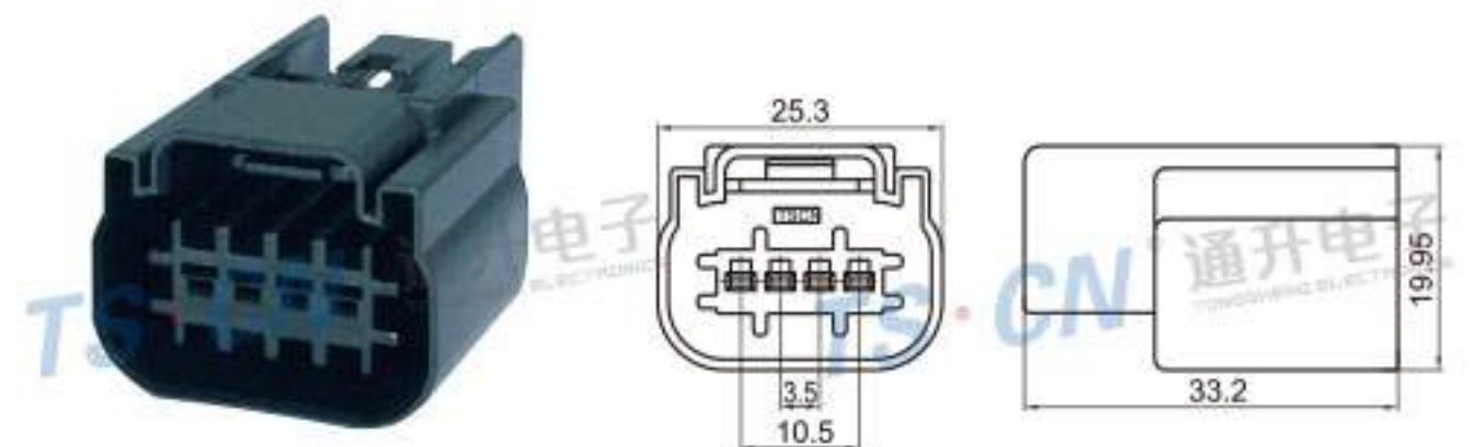
Type: TS30173-04P-21 Material: PBT Matching Terminal: TSH593
