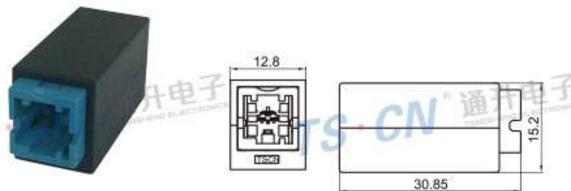
Type: TS30211-02PM-AT-1 Material: PBT GF15% Matching Terminal: TSTF0266~TSPM0269
