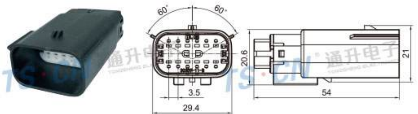
Type: TS30359-12P-11 Material: PA66 GF30% Matching Terminal: TSZ144A
