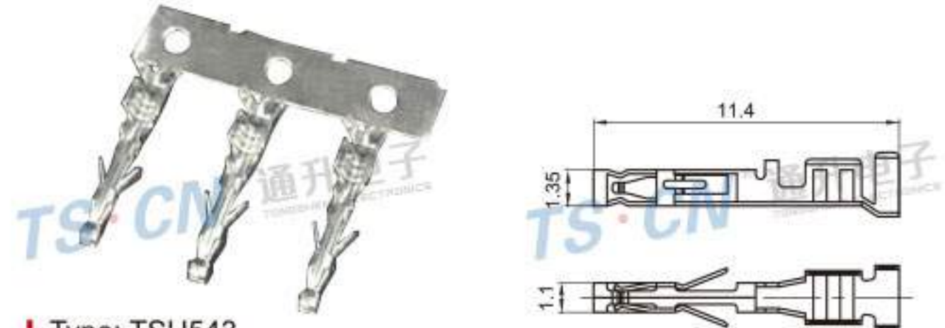
Type: TSH543 Material: Phos.bronze Applicable Thickness: 0.64
