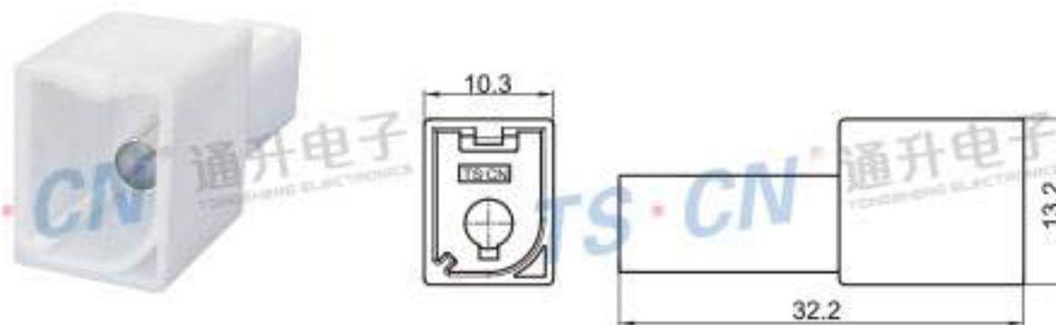
Type: TS1068-01PM-AT-2 Material: PA66 Matching Terminal: TSTM0003 / TSTM0004
