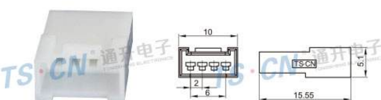
Type: TSPHD-04P-11(02P-10P) Material: PA66 Matching Terminal: TSHY-RT
