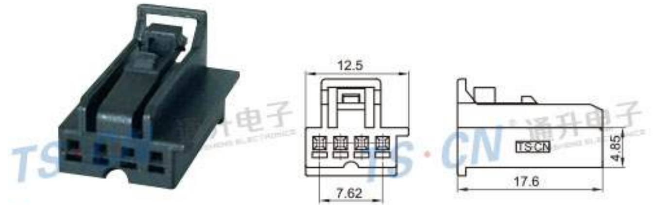
Type: TS30171-04P-21 Material: PA66 Matching Terminal: TSH143
