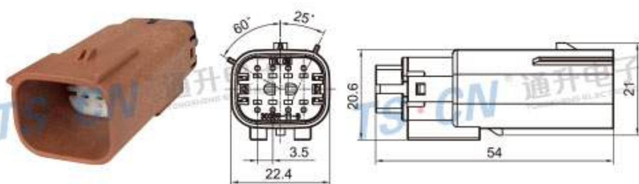
Type: TS30359-08P-11-2 Material: PA66 GF30% Matching Terminal: TSZ144A
