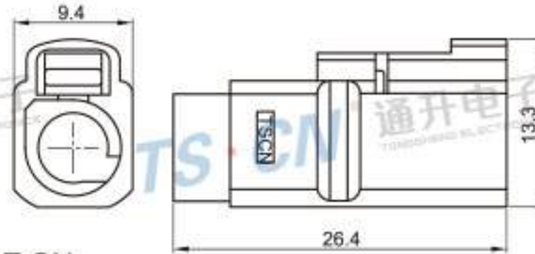
Type: TSVW20-01PF-AT-GN Material: PA66 GF30% Matching Terminal: TSTF0025 / TSTF0026
