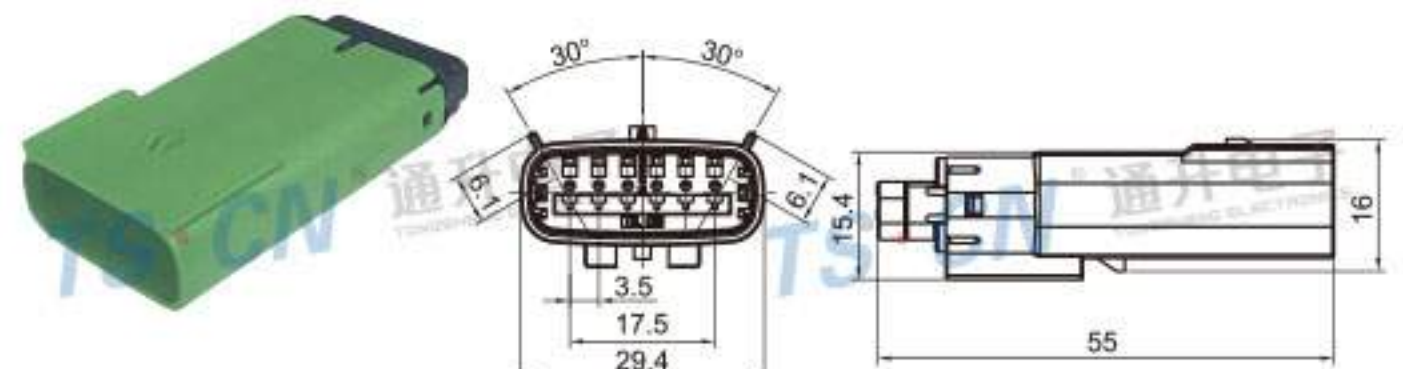
Type: TS30366-06P-11-3 Material: PA66 GF30% Matching Terminal: TSZ144A
