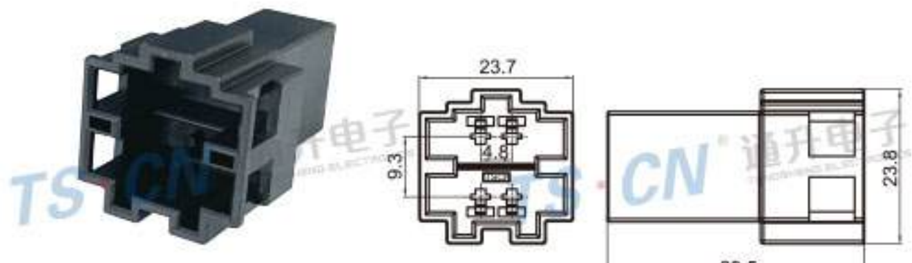
Type: TS30354-04P-11 Material: PBT Matching Terminal: TSZ006
