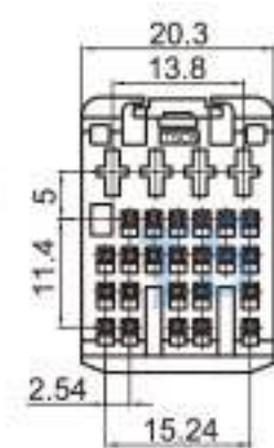
Type: TS30217-30P-21-6 Material: PBT GF10% Matching Terminal: TSH019 / TSH092
