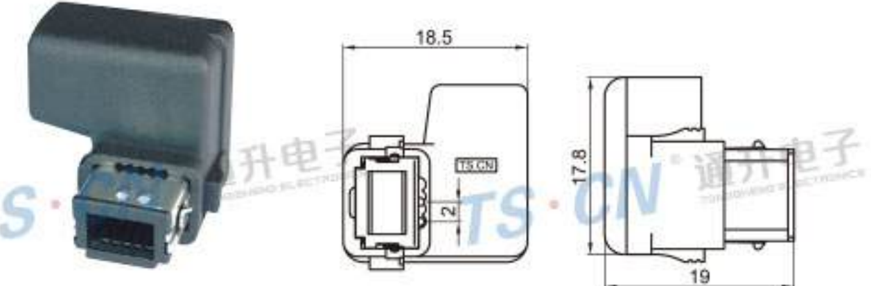
Type: TS30053-10PM-AH Material: PA66 GF30% Matching Terminal: TSAF0007 / TSAM0018 / TSAM0019
