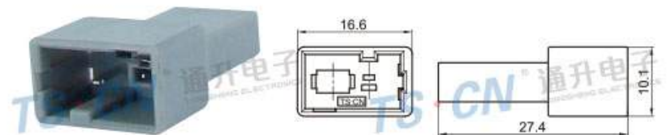
Type: TSHD10-02PM-AT Material: PA66 Matching Terminal: TSZ040 / TSTM0001 / TSTM0002
