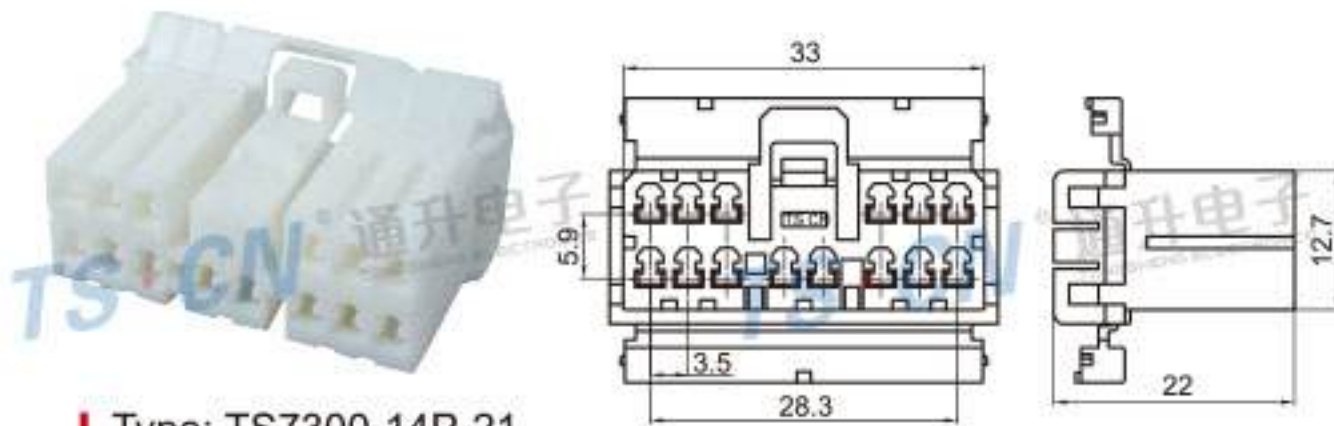
Type: TS7300-14P-21 Material: PA66 Matching Terminal: TSH016
