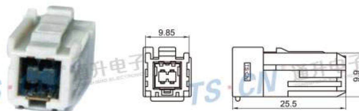
Type: TSTA04-04PF-AT Material: PA66 Matching Terminal: TSTF0008 / TSTF0010 / TSTF0011
