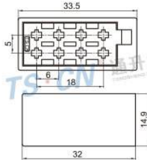
Type: TS1784A-08P-11BK Material: PA66 Matching Terminal: TSZ024
