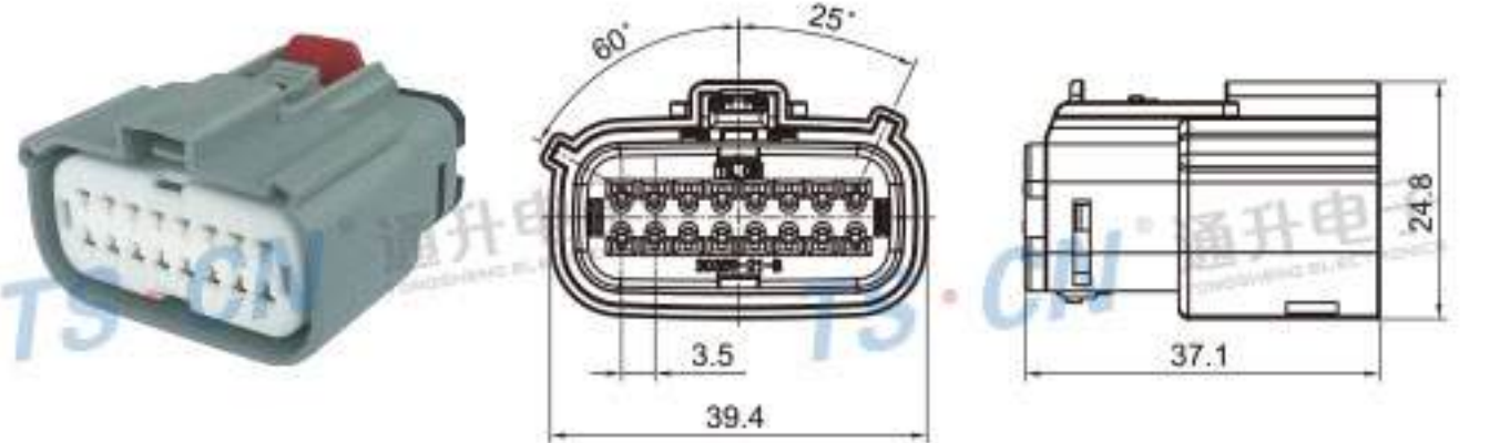
Type: TS30359-16P-21-1 Material: PA66 GF30% Matching Terminal: TSH047
