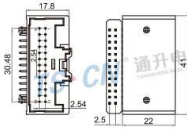
Type: TS5524-26PM-PKB Material: PA66 GF30% Matching Terminal: TSPM0085 / TSPM0122
