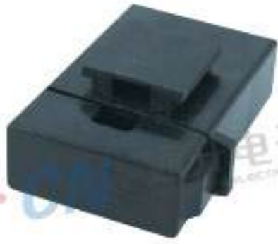
Type: TS BX01 Material: PA66 Matching Terminal: TSH033D
