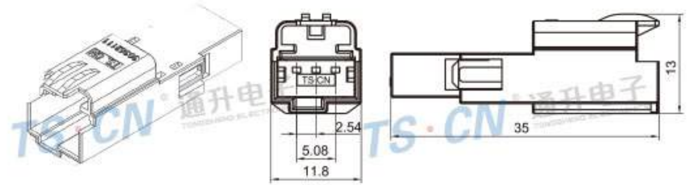
Type: TS30362-03P-11-1 Material: PA66 GF30% Matching Terminal: TSZ145
