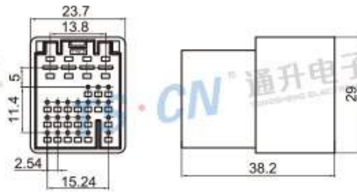
Type: TS30217-30P-11-3 Material: PBT GF15% Matching Terminal: TSDJ615B-2.8*0.8B / TSZ208
