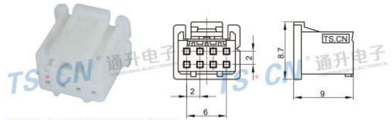
Type: TS30021-08P-21(10P) Material: PA66 Matching Terminal: TSH595
