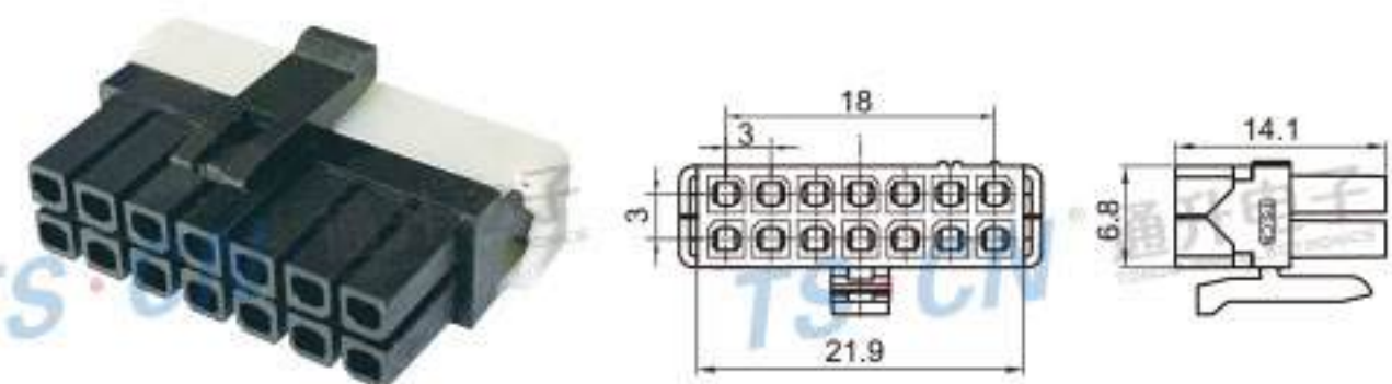
Type: TS43025-14P-21-3(04P-24P) Material: PA66 Matching Terminal: TSH035
