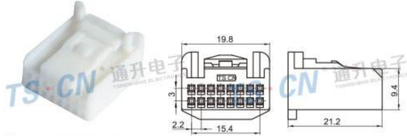
Type: TSTA16-16P-21 Material: PA66 Matching Terminal: TSH143
