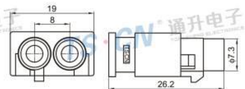
Type: TSVW10-02PM-AT-2 Material: PA66 Matching Terminal: TSTM0019 / TSTM0020
