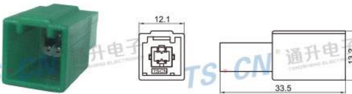
Type: TSTA04-04PM-AT-1 Material: PA66 GF30% Matching Terminal: TSTM0008-A / TSPM0218
