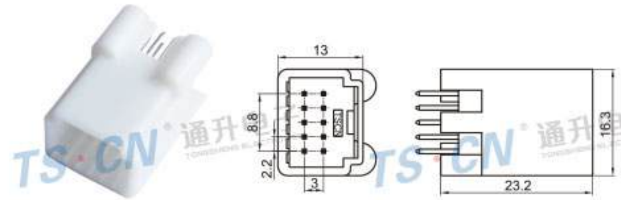
Type: TSTA10-10PM-PKS Material: PA66 Matching Terminal: TSPM0038
