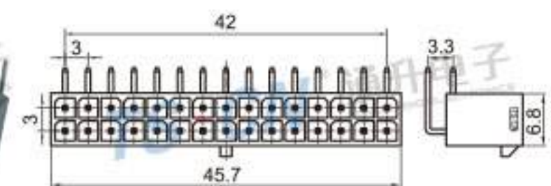
Type: TS43025-30PM-PKB Material: PA66 GF30% Matching Terminal: TSPM0066 / TSPM0121
