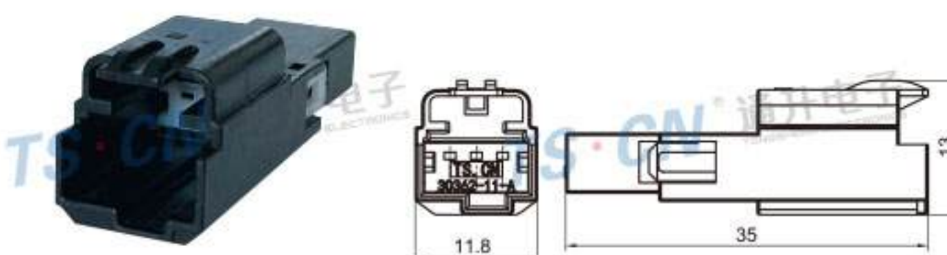
Type: TS30362-03P-11 Material: PA66 GF30% Matching Terminal: TSZ145
