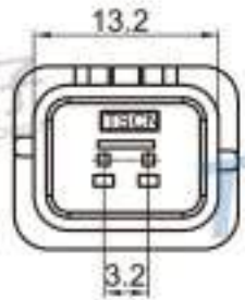
Type: TS30178-02P-11 Material: PA66 GF30% Matching Terminal: TSZ208
