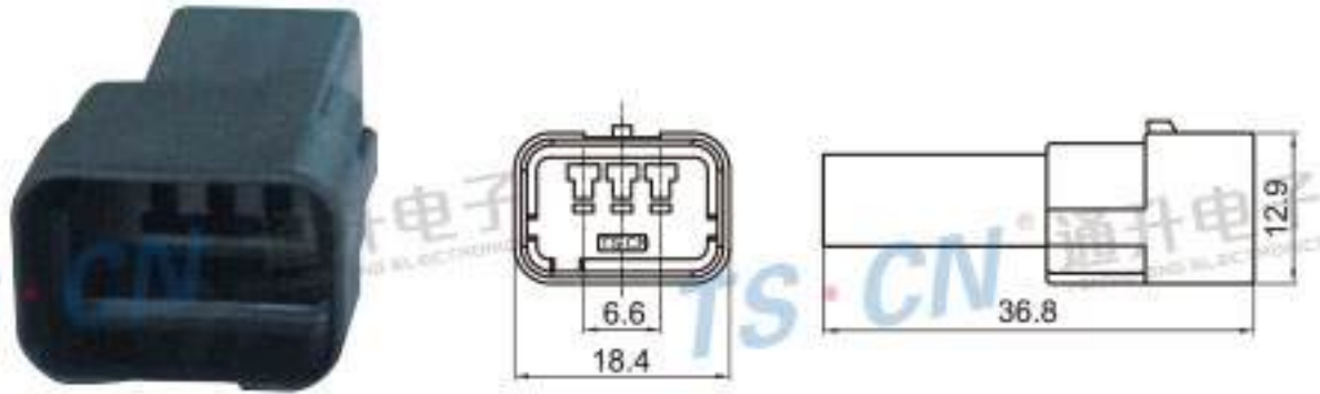
Type: TS30066-03P-11 Material: PA66 GF30% Matching Terminal: TSZ144
