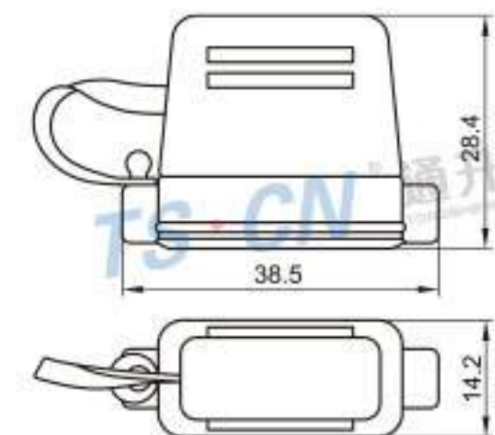
Type: TS BX10 Material: PA66 Matching Terminal: TSH587
