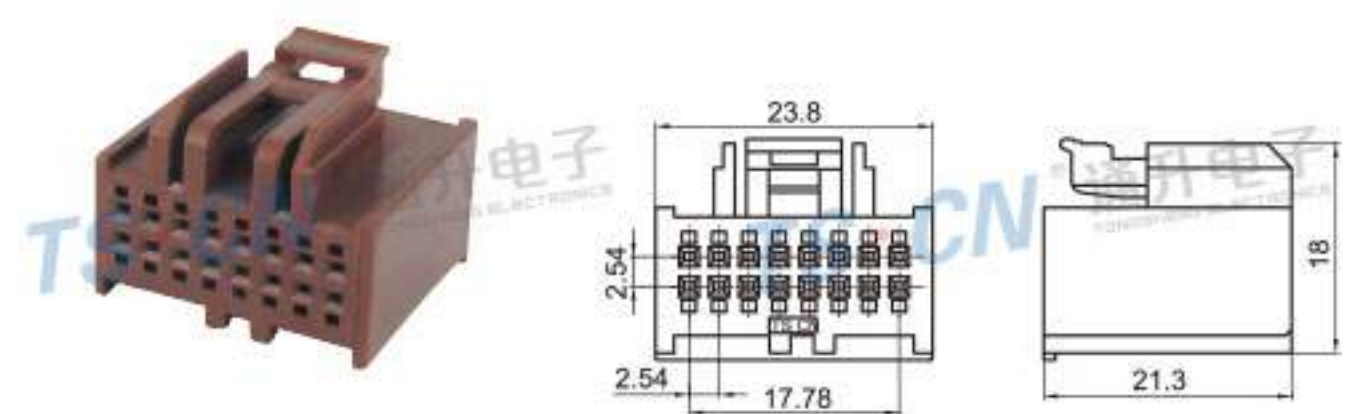
Type: TS2105-16P-21BN Material: PA66 Matching Terminal: TSH143B
