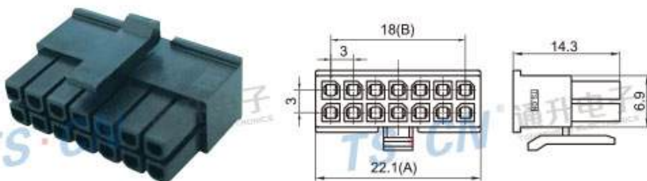
Type: TS43025-14P-21(02P-24P) Material: PA66 Matching Terminal: TSH035
