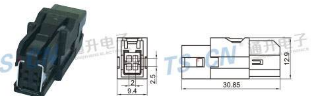
Type: TS30123-04PF-AH-1 Material: PBT Matching Terminal: TSAF0032 / TSAF0033 / TSH600
