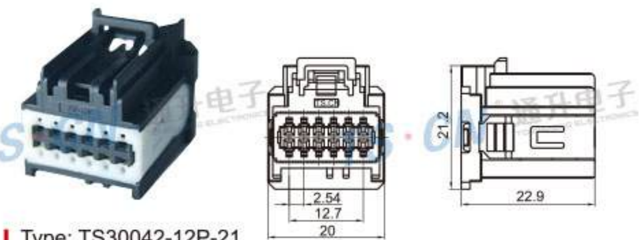
Type: TS30042-12P-21 Material: PA66 GF30% Matching Terminal: TSH006
