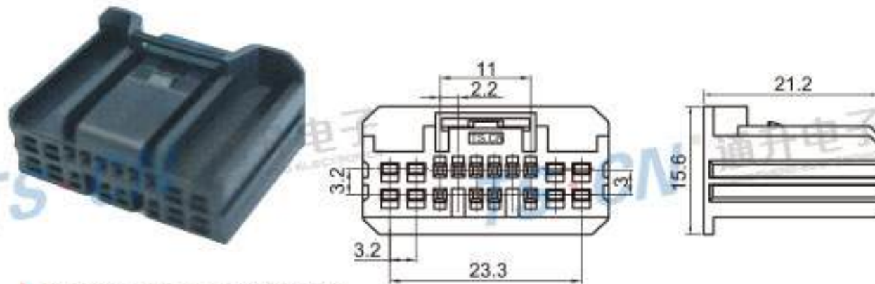
Type: TS30061-18P-21 Material: PA66 GF30% Matching Terminal: TSH593 / TSH143
