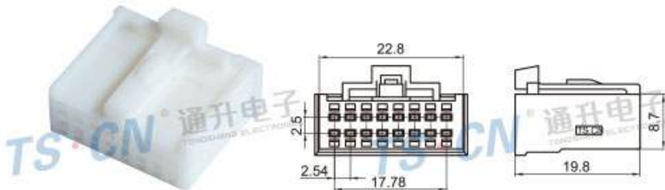
Type: TSPAN16-16P-21-1 Material: PA66 Matching Terminal: TSH053
