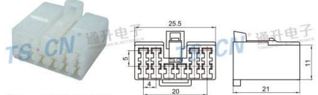
Type: TS1761-10P-21 Material: PA66 Matching Terminal: TSH009
