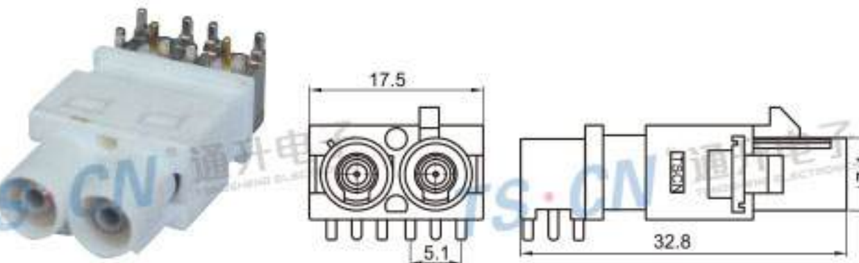
Type: TSVW10-02PM-AT-3 Material: PBT GF15% Matching Terminal: TSPM0169 / TSPM0172
