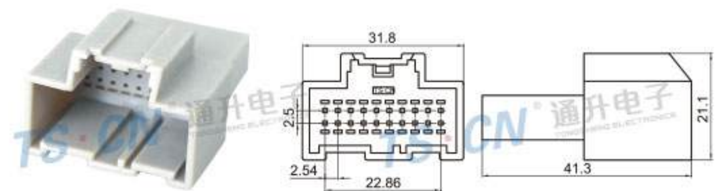
Type: TSGM20-20P-11-2 Material: PA66 GF30% Matching Terminal: TSZ208B
