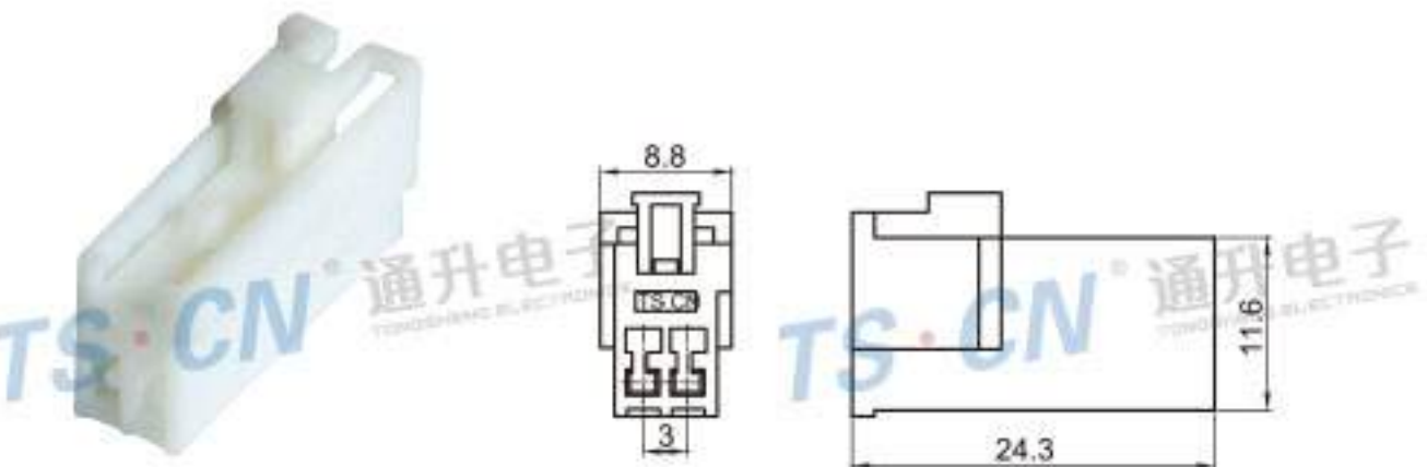
Type: TSLB08-02P-21 Material: PA66 Matching Terminal: NIL
