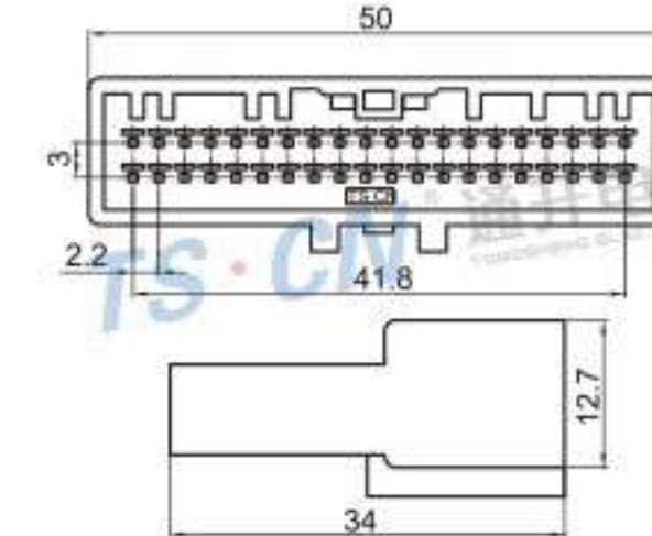
Type: TSTA40-40P-11-5 Material: PA66 Matching Terminal: TSZ208
