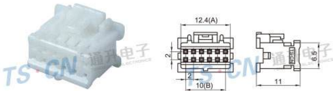
Type: TSPHS-12P-21(04P-24P) Material: PA66 Matching Terminal: TSPHS
