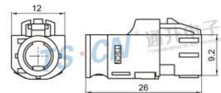
Type: TSVW20-04PF-AT-5BN-1 Material: PA66 GF30% Matching Terminal: TSTF0051 / TSTF0052
