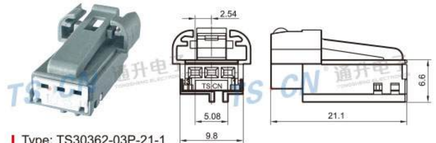
Type: TS30362-03P-21-1 Material: PA66 GF30% Matching Terminal: TSH006B
