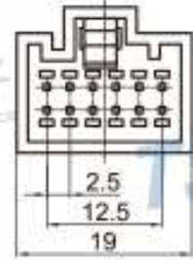
Type: TS30107-12P-11 Material: PA66 Matching Terminal: TSZ208B
