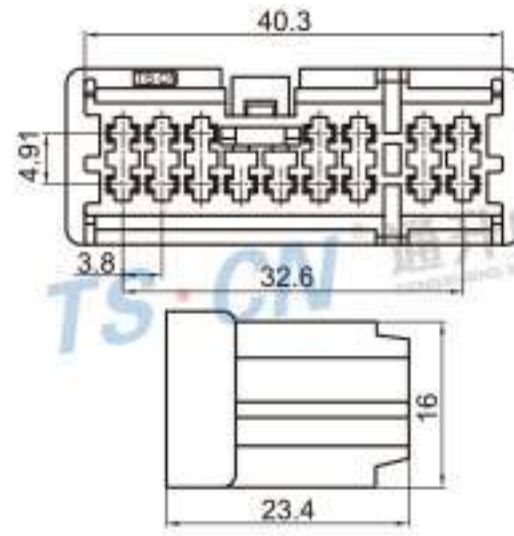
Type: TS7301A-16P-21-1 Material: PA66 Matching Terminal: TSH009
