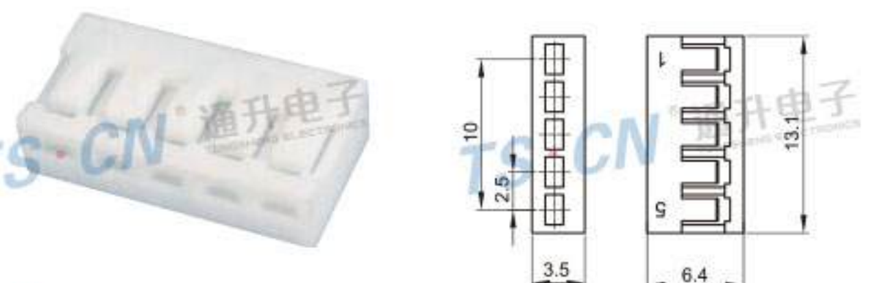
Type: TSJC25-05P-11(02P-15P) Material: PA66 Matching Terminal: JC25-T
