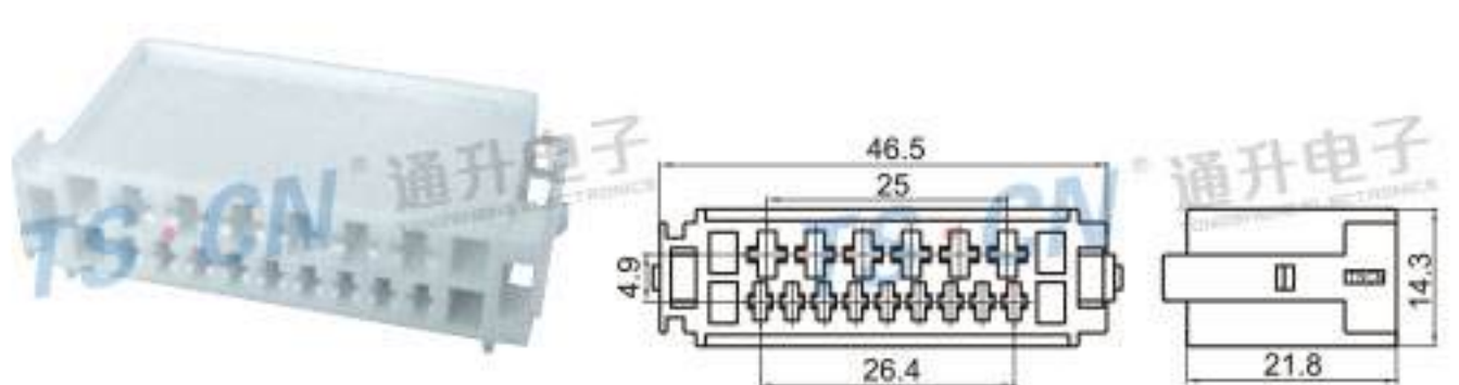
Type: TS30204-15P-21 Material: PA66 Matching Terminal: TSH019 / TSH054
