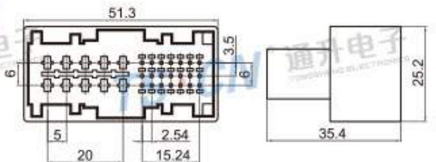
Type: TS30104-31P-11 Material: PBT GF15% Matching Terminal: TSZ024 / TSZ208
