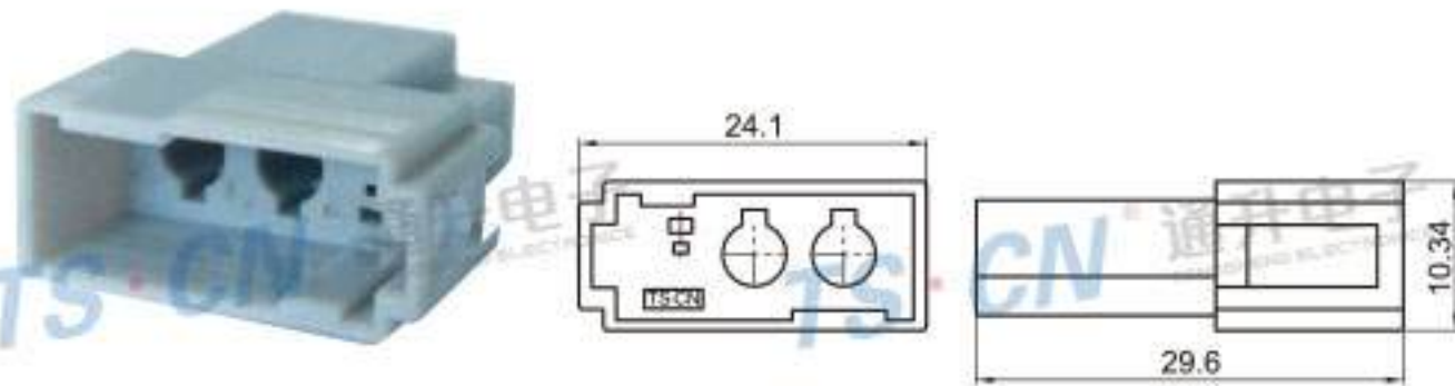
Type: TSHD11-03PM-AT Material: PA66 Matching Terminal: TSZ208 / TSTM0007 / TSTF0004
