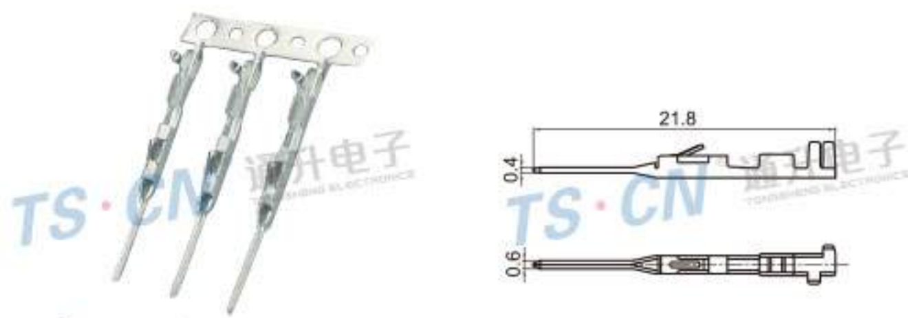
Type: TSZ561 Material: Brass
