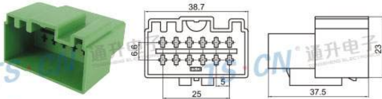
Type: TS9221-12P-11GN Material: PA66 Matching Terminal: TSZ024
