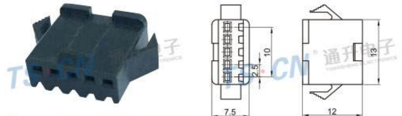
Type: TSSM-05P-21(02P-12P) Material: PA66 Matching Terminal: TSZSM
