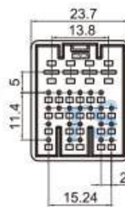
Type: TS30217-30P-11-6 Material: PBT GF15% Matching Terminal: TSDJ615B-2.8*0.8B / TSZ208
