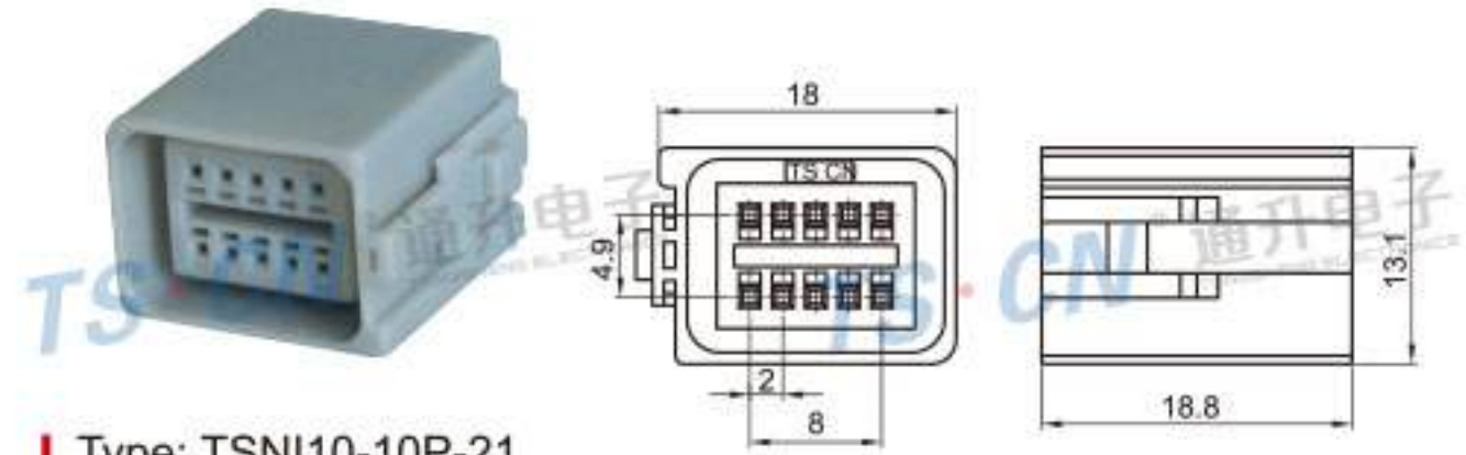
Type: TSNI10-10P-21 Material: PA66 GF30% Matching Terminal: TSHY66
