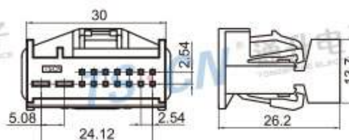
Type: TS30230-16P-21 Material: PBT Matching Terminal: TSH091 / TSH092
