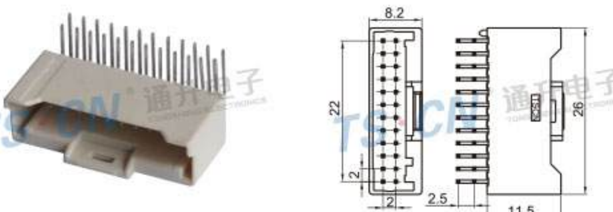
Type: TSQRA3-24PM-PKB(12P-28P) Material: PA66 GF15% Matching Terminal: TSPM0143 / TSPM0144
