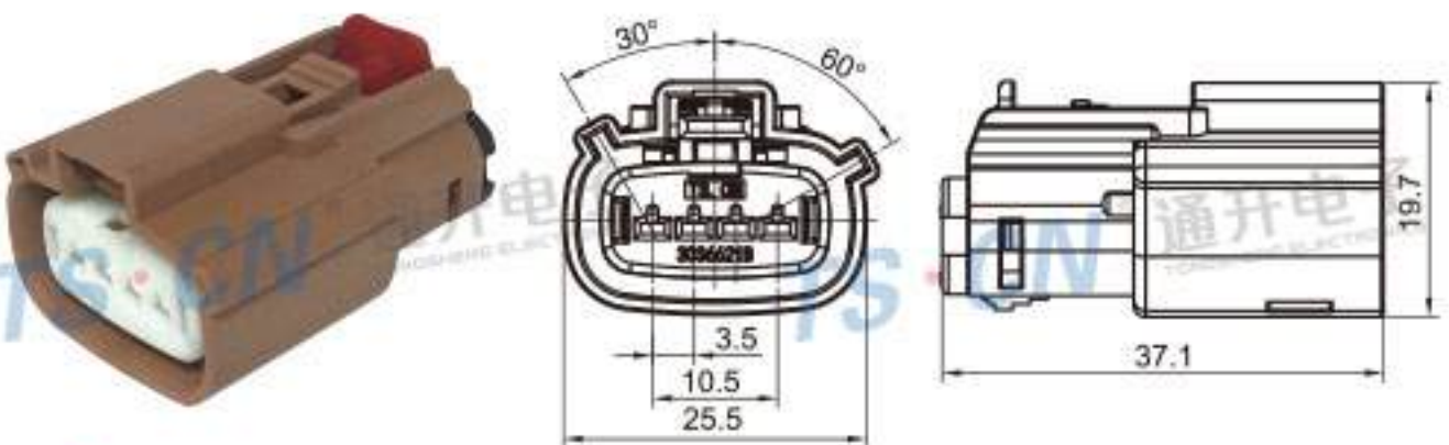
Type: TS30366-04P-21-2 Material: PA66 GF30% Matching Terminal: TSH047
