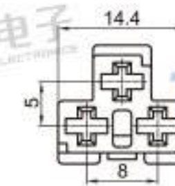
Type: TS30182-03P-21 Material: PA66 Matching Terminal: TSH019
