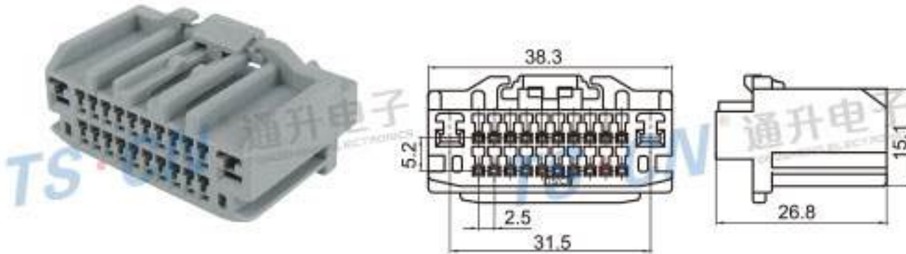
Type: TS6522-22P-21 Material: PA66 Matching Terminal: TSH085 / TSH006
