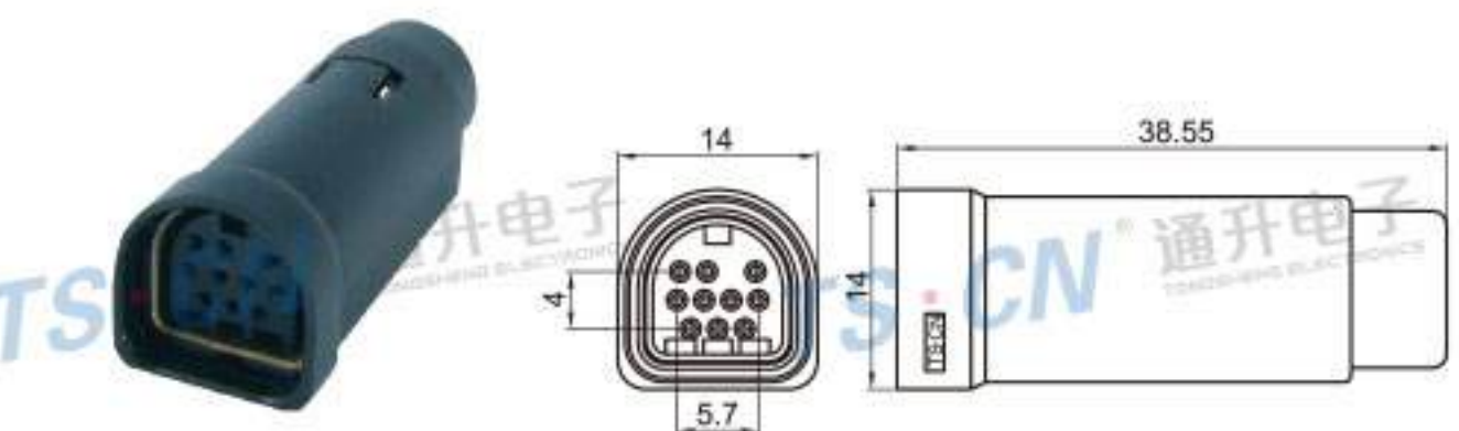
Type: TSALPH-10PF-AH Material: PA66 Matching Terminal: NIL
