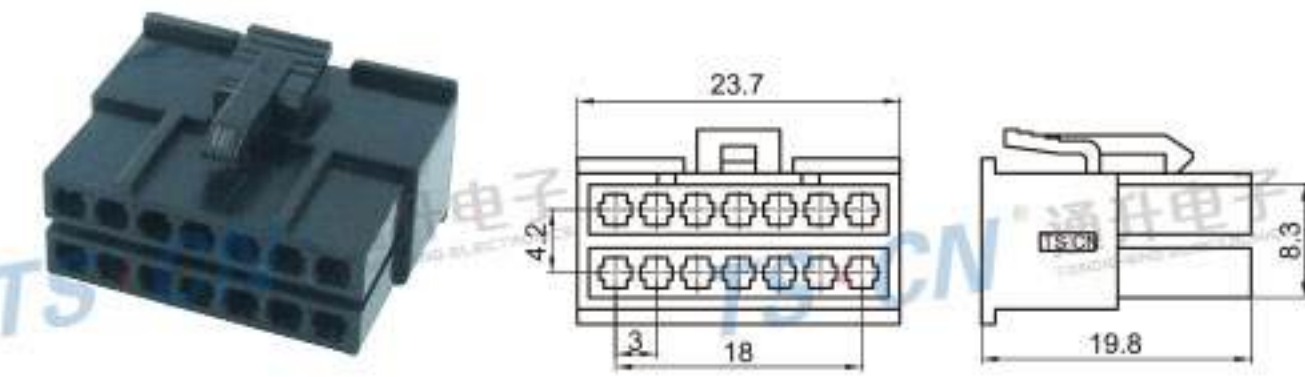
Type: TSLG14-14P-21 Material: PA66 Matching Terminal: TSH034
