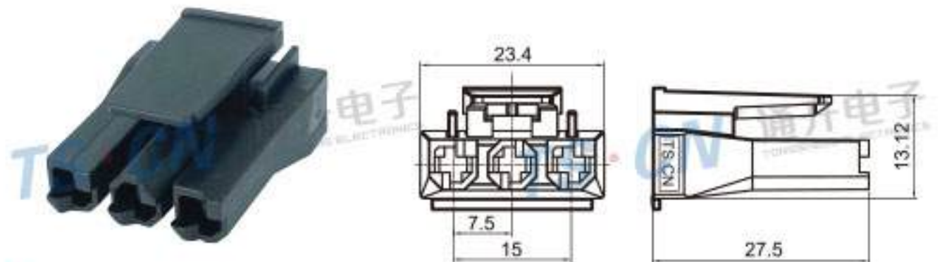
Type: TS30307-03P-21 Material: PA66 Matching Terminal: TSH630
