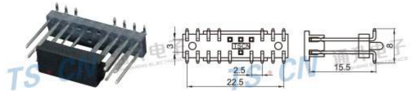
Type: TS57591-16PM-PKB Material: LCP GF30% Matching Terminal: TSPM0139
