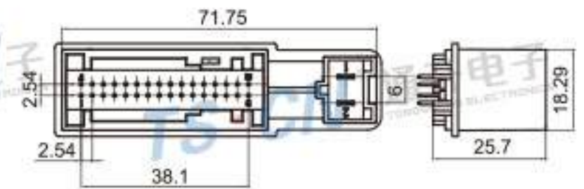
Type: TS30236-34PM-PKS Material: PBT GF15% Matching Terminal: TSPM0275 / TSPM0276
