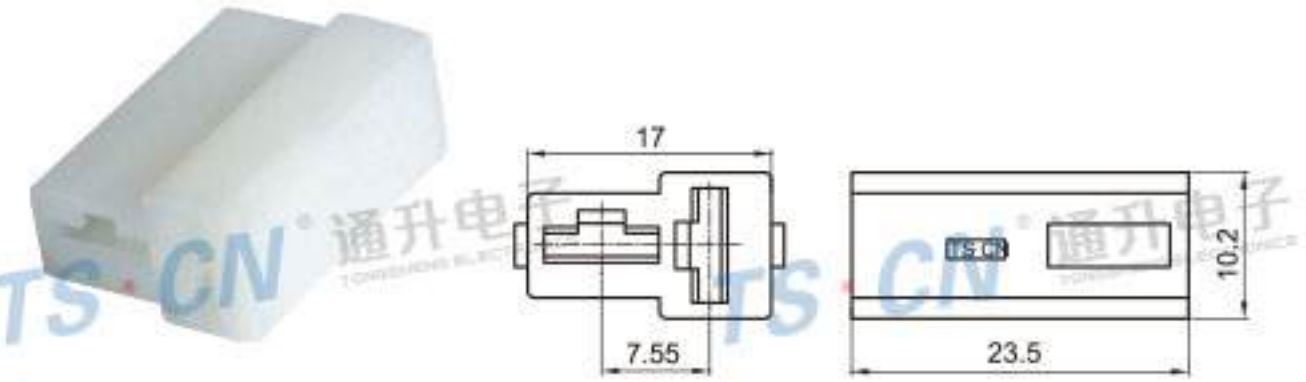
Type: TSLB05-02P-21 Material: PA66 Matching Terminal: TSH033
