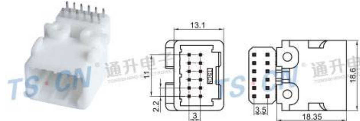
Type: TSTA12-12PM-PKB Material: PA66 Matching Terminal: TSPM0040 / TSPM0041
