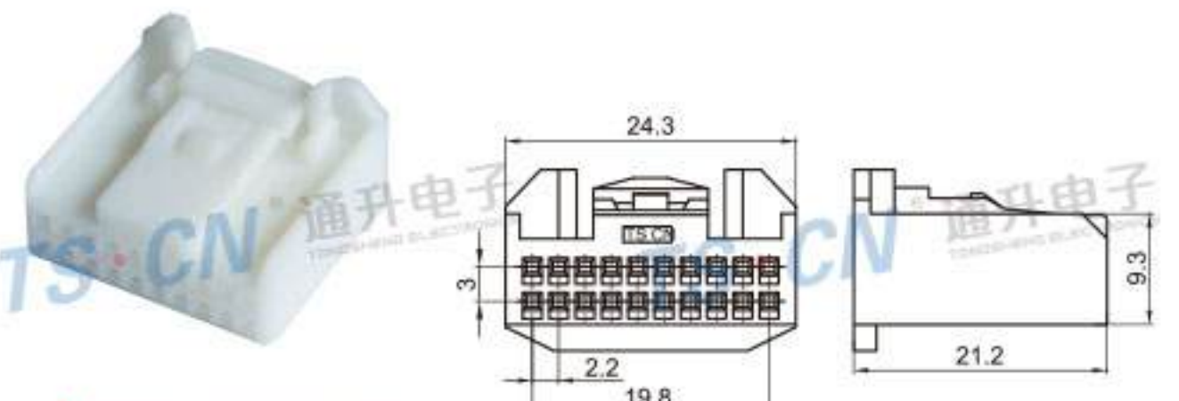
Type: TSTA20-20P-21 Material: PA66 Matching Terminal: TSH143
