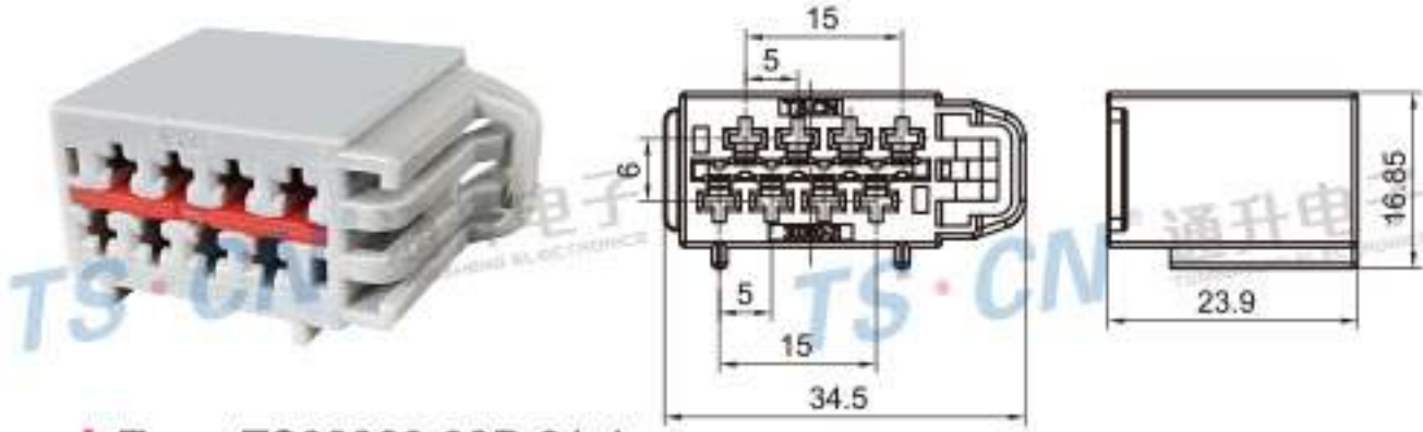
Type: TS30360-08P-21-1 Material: ABS Matching Terminal: TSH085
