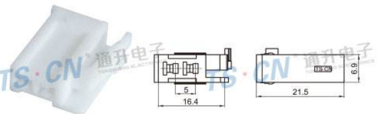
Type: TSLB10-02P-21 Material: PBT 1100 Matching Terminal: TSH064
