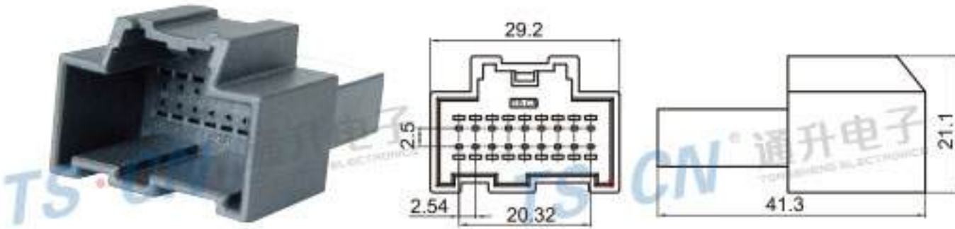
Type: TSGM18-18P-11 Material: PA66 GF30% Matching Terminal: TSZ208B
