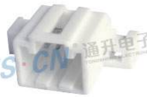
Type: TS30255-04PM-PKB Material: PBT GF15% Matching Terminal: TSPM0300
