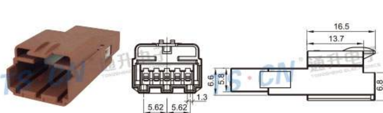
Type: TS30362-05P-11-2 Material: PA66 GF30% Matching Terminal: TSZ145
