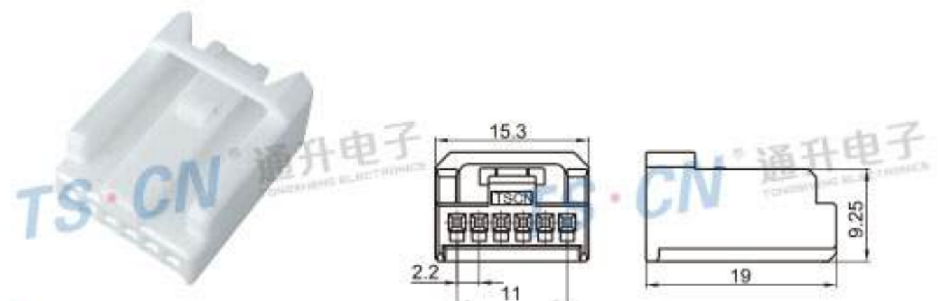
Type: TS30206-06P-21 Material: PBT GF15% Matching Terminal: TSH143
