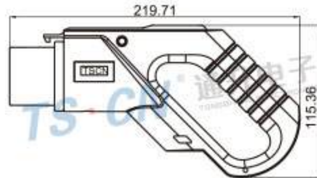
Type: TS 30247 (交流充电枪) Material: PA66 GF30% Matching Terminal: TS 30247-K / TS 30247-L / TS 30247-M
