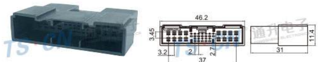
Type: TS30243-28P-11-8BK Material: PBT Matching Terminal: TSZ040 / TSZ561
