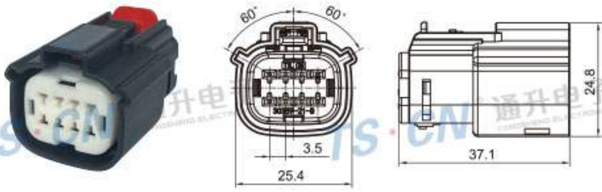
Type: TS30359-08P-21 Material: PA66 GF30% Matching Terminal: TSH047
