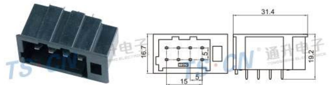
Type: TSABD-08PM-PKS-A Material: PA66 Matching Terminal: TSPM0127
