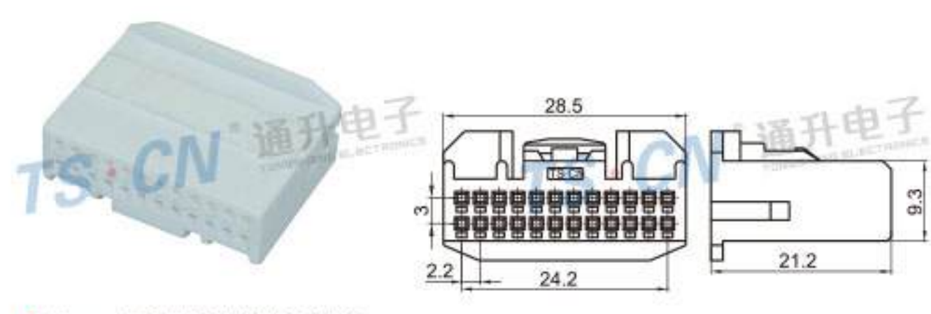
Type: TSTA24-24P-21-2 Material: PA66 Matching Terminal: TSH143D
