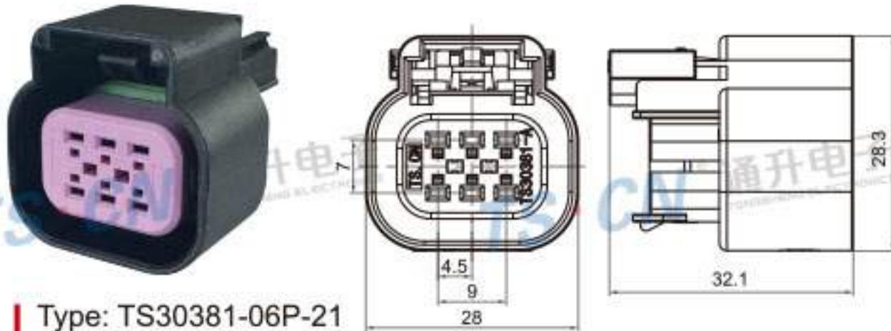
Type: TS30381-06P-21 Material: PA66 GF30% Matching Terminal: TSDJ625-F1.5A
