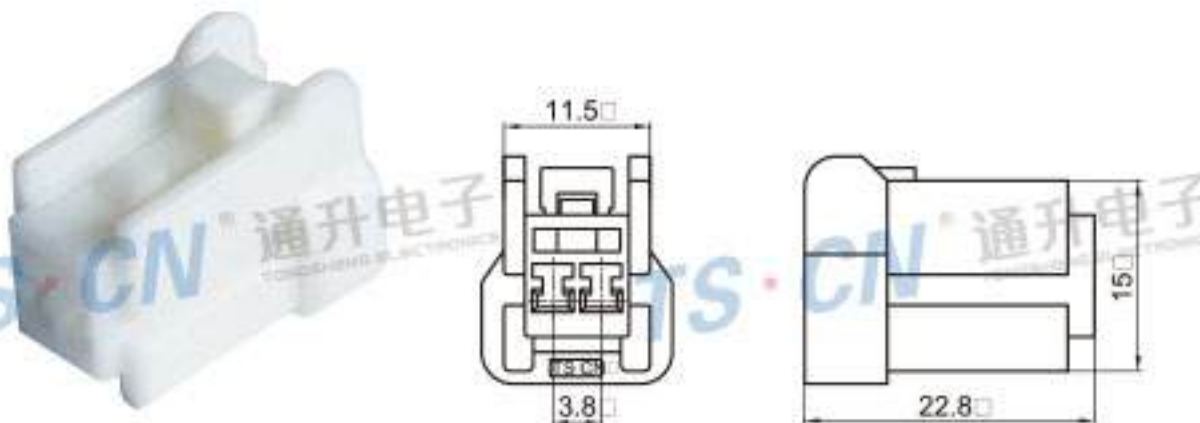
Type: TSLB03-02P-21 Material: PA66 Matching Terminal: TSH015
