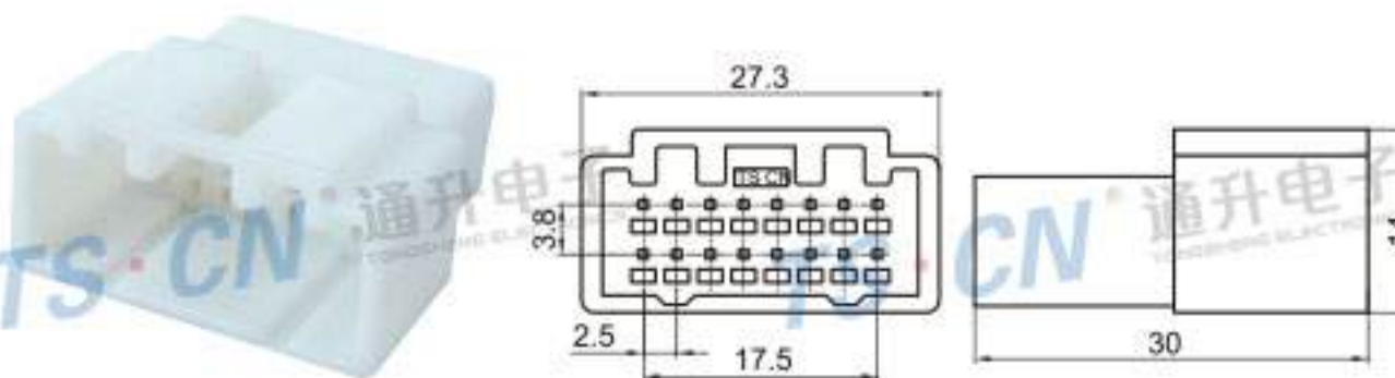
Type: TSMA16-16P-11 Material: PA66 Matching Terminal: TSZ208B
