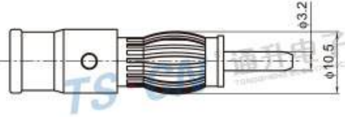
Type: TSAM-AT-2 Material: PA66 Matching Terminal: TSTM0030 / TSTM0030
