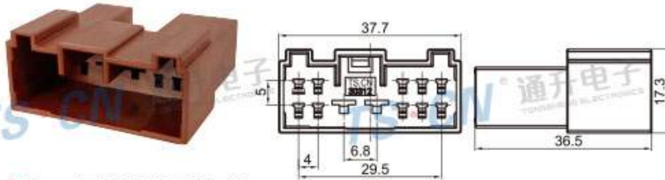
Type: TS30312-12P-11 Material: PBT Matching Terminal: TSZ028 / TSZ045
