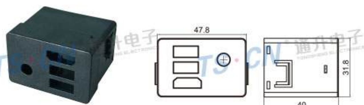
Type: TS30221 Material: PA66 GF30% Matching Terminal: TSHDMI-F / TSUSB-F / TS3.5-F
