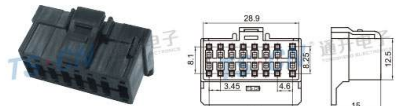
Type: TSPIO01A-16P-21 Material: PA66 GF30% Matching Terminal: TSH504 / TSH503
