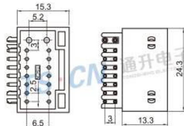
Type: TSKEN-16PM-PKB-2 Material: PA66 GF30% Matching Terminal: TSPM0103~TSPM0108
