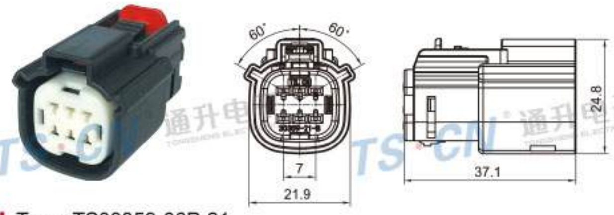
Type: TS30359-06P-21 Material: PA66 GF30% Matching Terminal: TSH047
