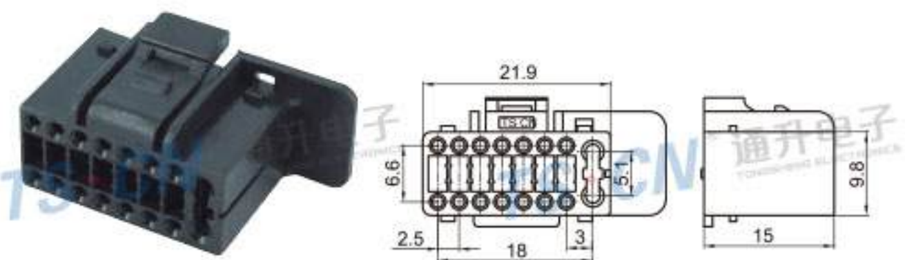
Type: TSKEN16-16P-21-1 Material: PA66 GF15% Matching Terminal: TSH032 / TSH031
