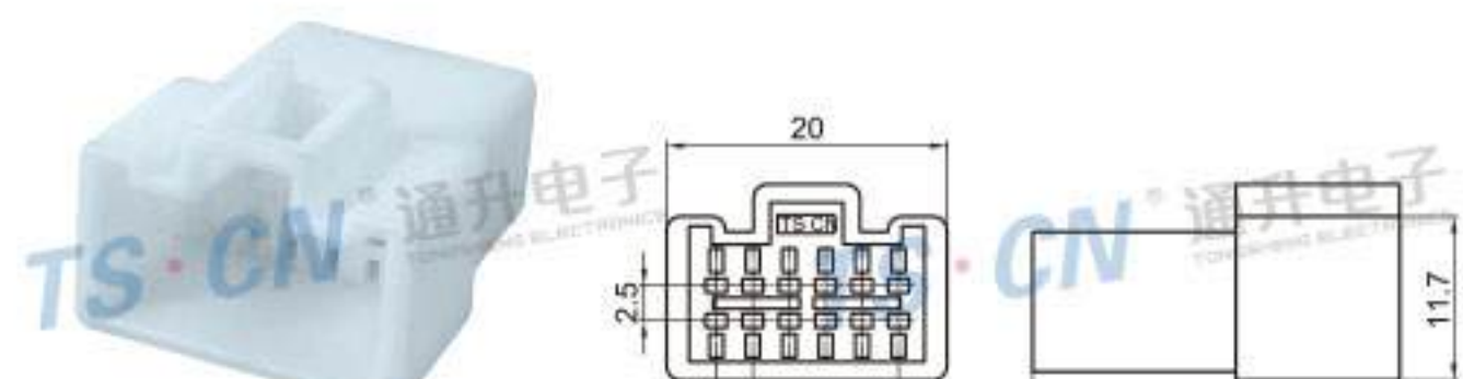
Type: TSPAN12-12P-11 Material: PA66 Matching Terminal: TSZ007B
