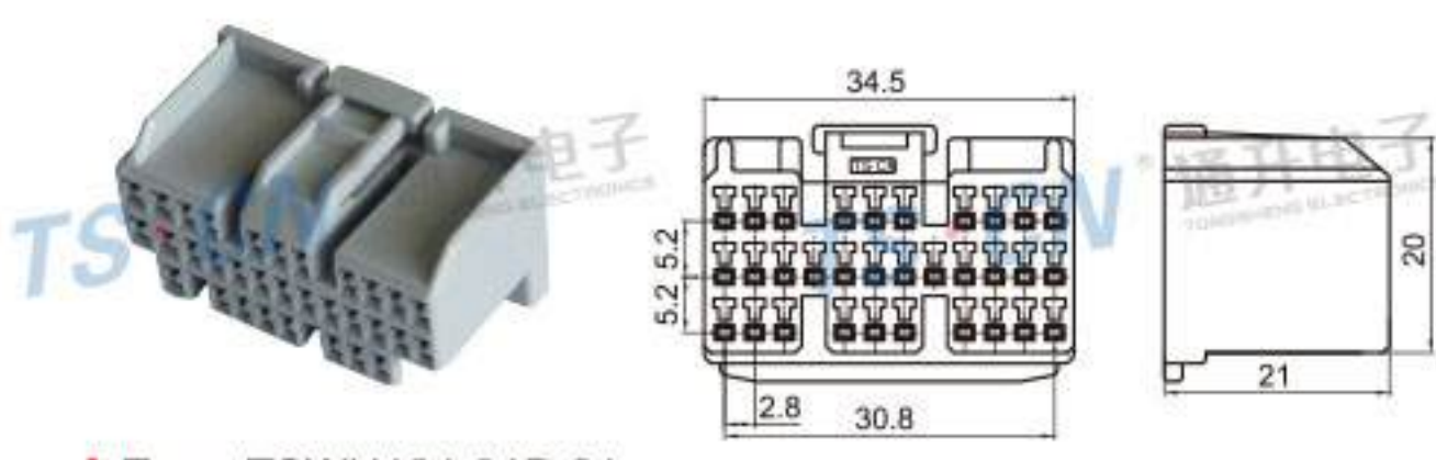
Type: TSWH104-31P-21 Material: PA66 Matching Terminal: TSH076
