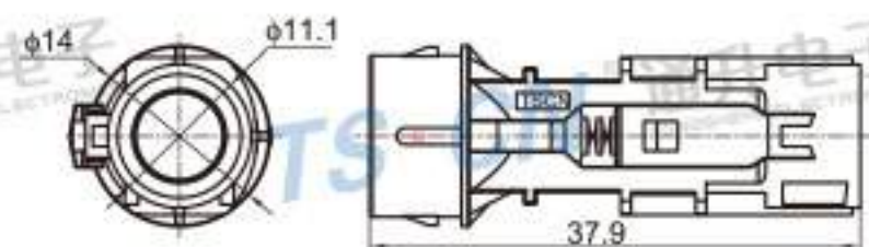
Type: TS30166-04PF-AT Material: PA66 GF30% Matching Terminal: TSTF0051-B / TSTF0052
