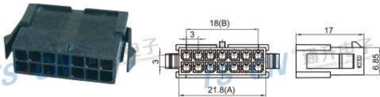
Type: TS43025-14P-11(02P-24P) Material: PA66 Matching Terminal: TSZ160
