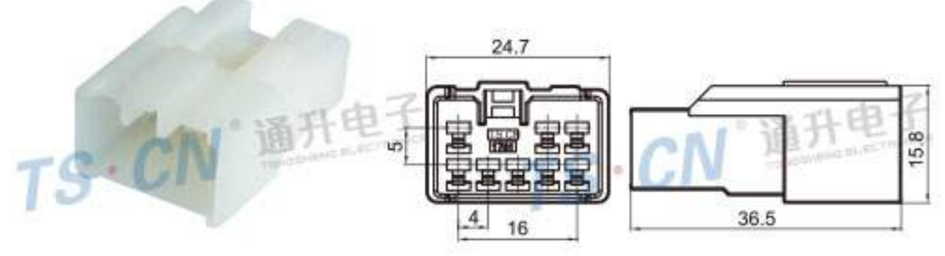
Type: TS1761-08P-11 Material: PA66 Matching Terminal: TSZ003
