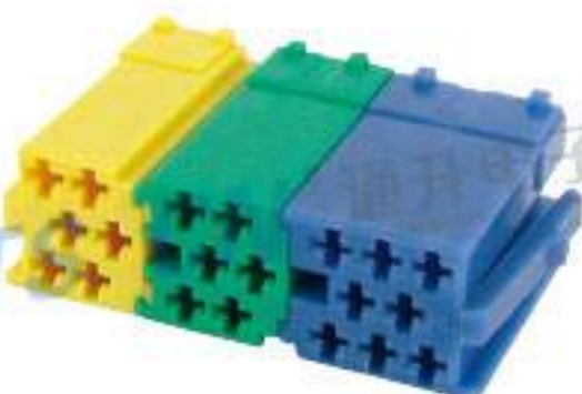
Type: TSAD20-20P-21 Material: PA66 Matching Terminal: TSH054
