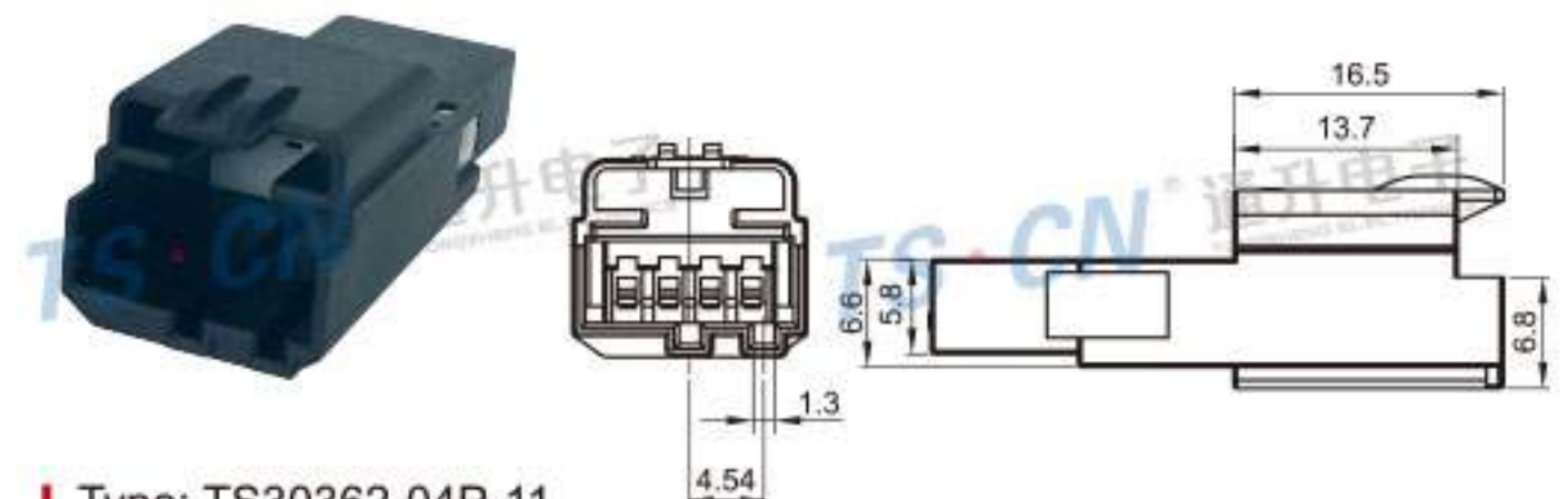
Type: TS30362-04P-11 Material: PA66 GF30% Matching Terminal: TSZ145
