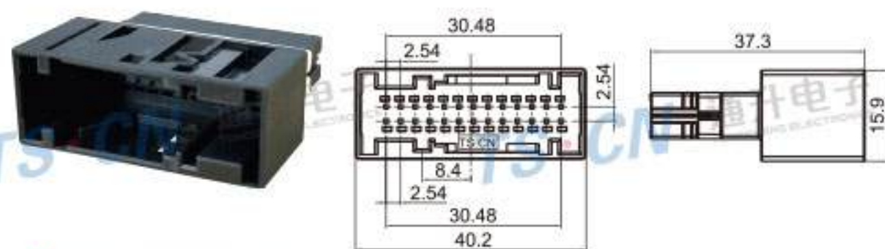
Type: TS30316-26P-11 Material: PA66 GF30% Matching Terminal: TSZ616
