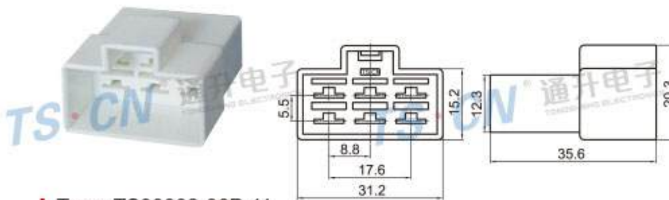
Type: TS30002-06P-11 Material: PBT GF15% Matching Terminal: TSZ538-A
