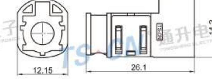
Type: TSVW10-04PM-AT-5LG-1 Material: PA66 GF15% Matching Terminal: TSPM0175 / TSTM0051
