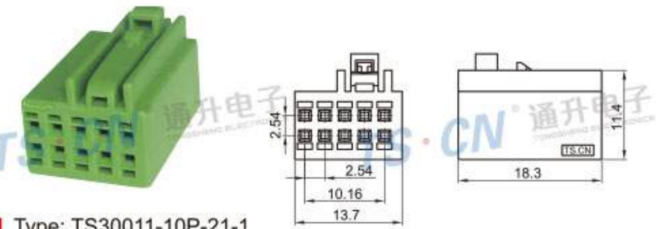
Type: TS30011-10P-21-1 Material: PBT GF15% Matching Terminal: TSH143
