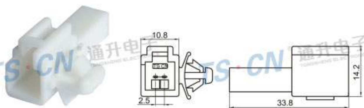
Type: TSLB04-02P-11 Material: PA66 Matching Terminal: TSZ145
