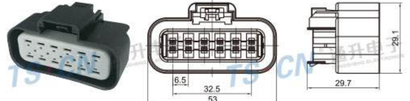
Type: TS30382-12P-21 Material: PA66 GF30% Matching Terminal: TSH645
