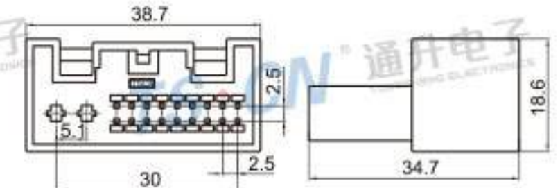
Type: TS30167-20P-11 Material: PA66 GF30% Matching Terminal: TSZ024 / TSZ208B
