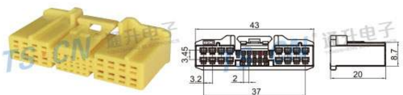
Type: TS30243-28P-21-6 Material: PA66 Matching Terminal: TSH593 / TSH606
