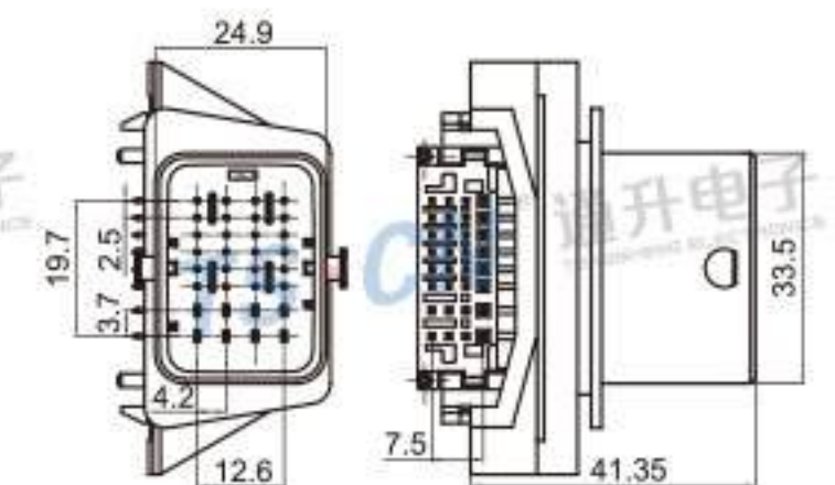
Type: TS30245-32PM-PKB Material: PA66 Matching Terminal: TSPM0289~TSPM0296
