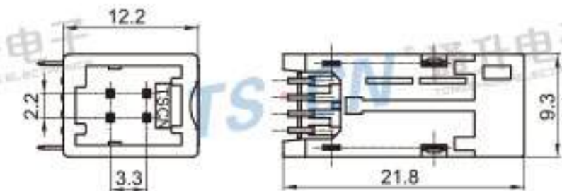
Type: TS30213-04PM-PKB Material: PBT GF15% Matching Terminal: TSPM0270~TSPM0274
