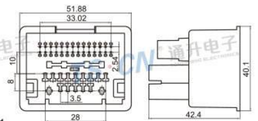
Type: TSKL44-44P-11-1 Material: PA66 GF30% Matching Terminal: TSZ024 / TSZ144 / TSZ208B
