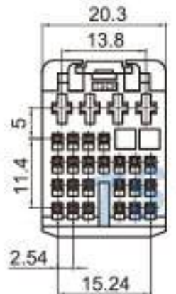
Type: TS30217-30P-21-5 Material: PBT GF10% Matching Terminal: TSH019 / TSH092
