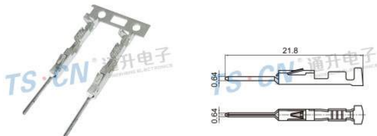
Type: TSZ616 Material: Brass
