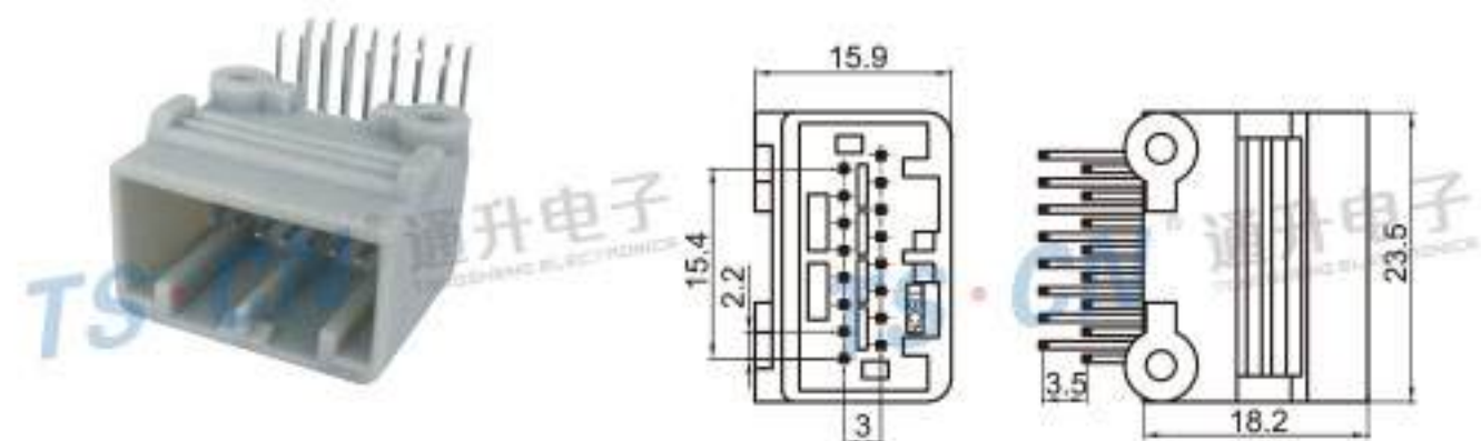
Type: TSCRV-16PM-PKB Material: PA66 Matching Terminal: TSPM0062 / TSPM0063
