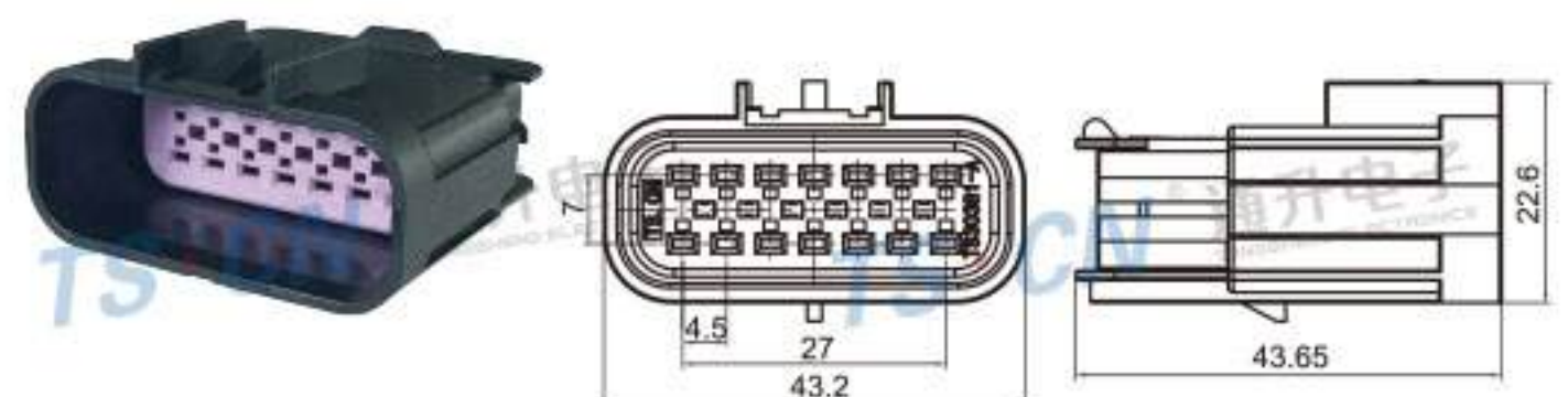
Type: TS30381-14P-11 Material: PA66 GF30% Matching Terminal: TS15326269
