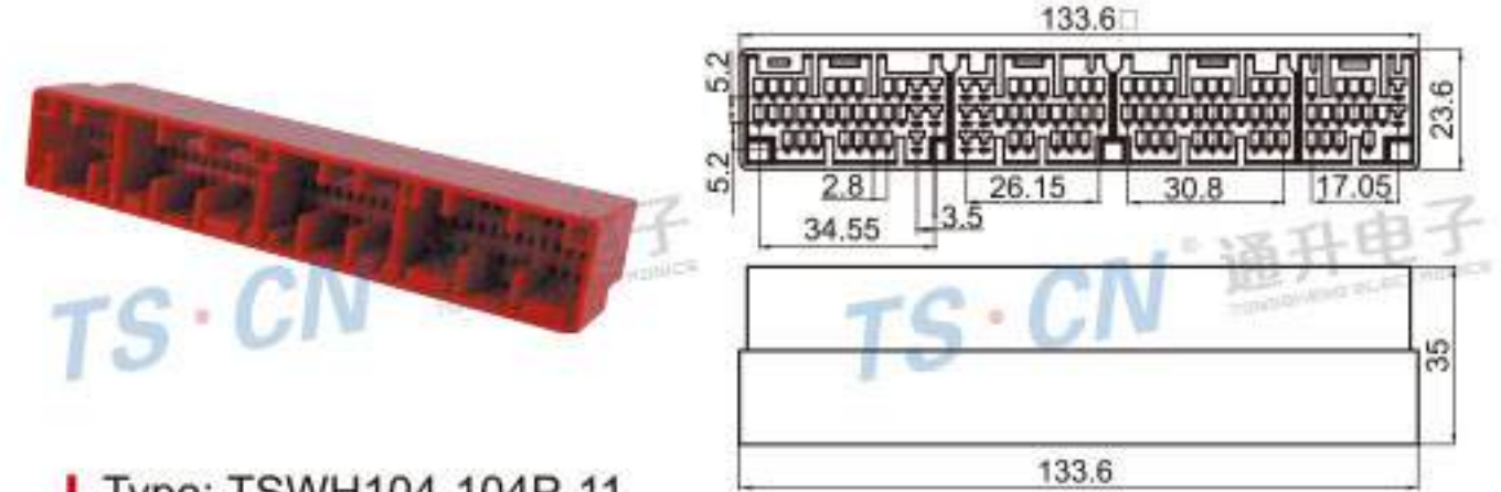
Type: TSWH104-104P-11 Material: PA66 Matching Terminal: TSZ007 / TSZ145
