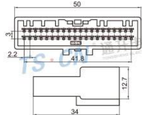
Type: TSTA40-40P-11-4 Material: PA66 Matching Terminal: TSZ208
