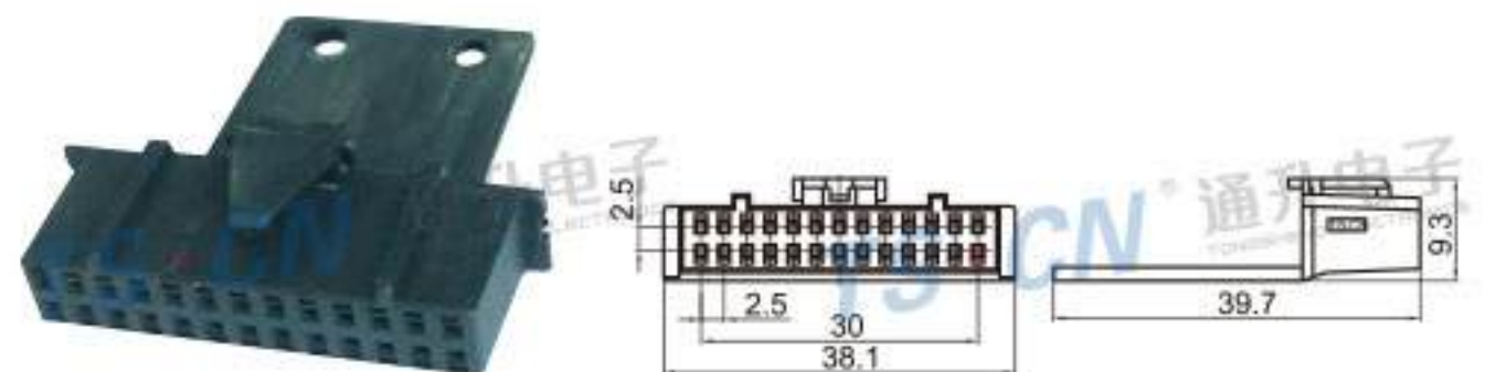
Type: TS30005-26P-21 Material: PA66 Matching Terminal: TSCH2.5A
