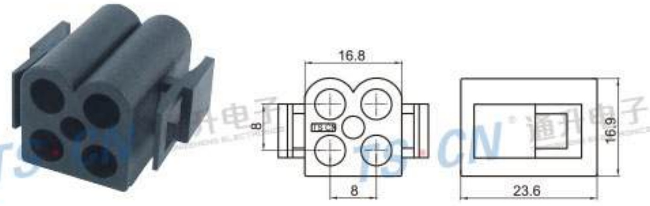
Type: TSVO04-04P-21 Material: PA66 GF15% Matching Terminal: TSH596
