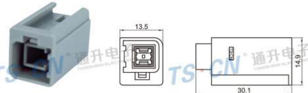
Type: TSFIAT10-01PM-AT-1 Material: PA66 Matching Terminal: TSTF0014/TSTF0015
