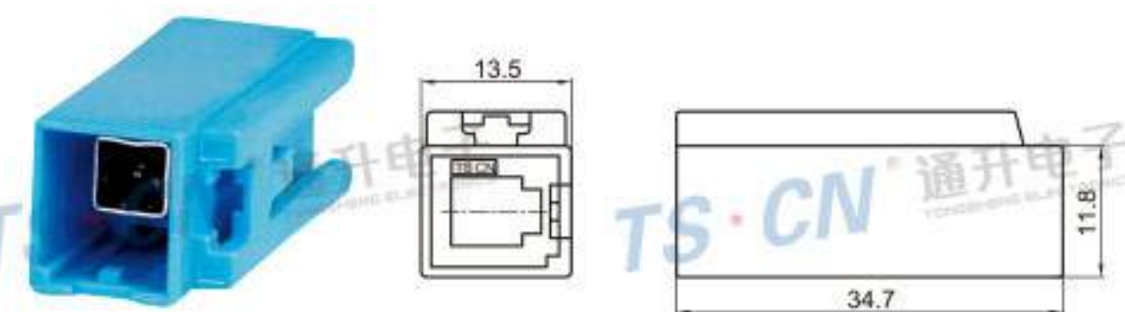
Type: TSTA10-01PM-AT-1 Material: PA66 Matching Terminal: TSPM0012 / TSPM0013
