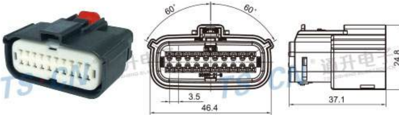
Type: TS30359-20P-21 Material: PA66 GF30% Matching Terminal: TSH047
