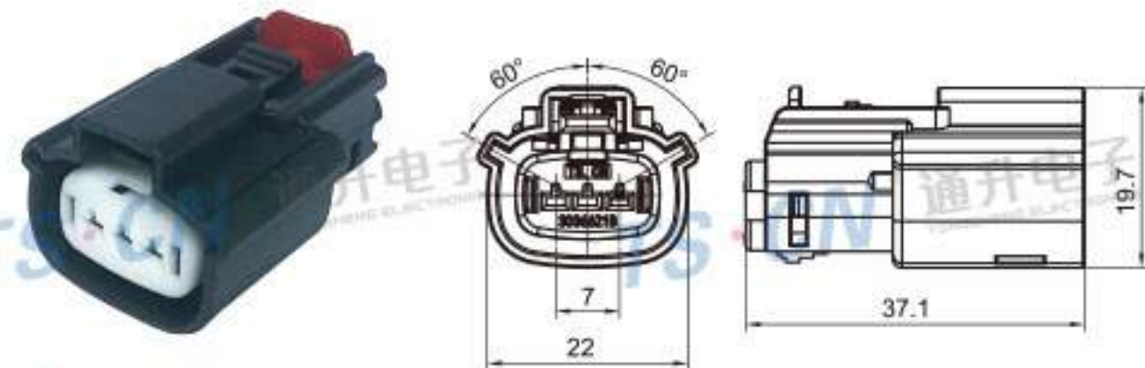
Type: TS30366-03P-21 Material: PA66 GF30% Matching Terminal: TSH047
