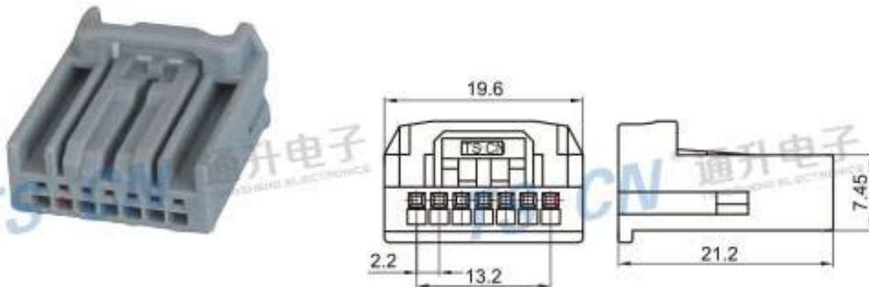
Type: TSCRV07-07P-21 Material: PBT Matching Terminal: TSH143D
