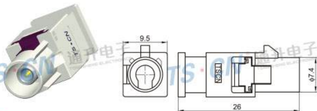
Type: TSVW10-01PM-AT-WT Material: PA66 Matching Terminal: TSTM0019 / TSTM0020
