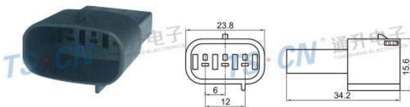
Type: TS30019-03P-11 Material: PA66 GF30% Matching Terminal: TSZ010B
