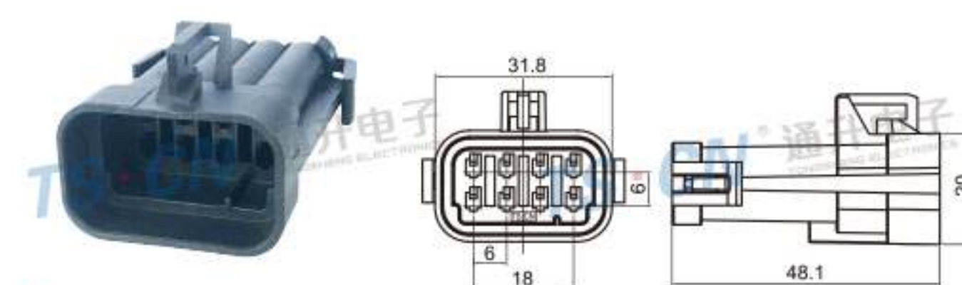
Type: TS30287-08P-11 Material: PBT GF30% Matching Terminal: TSZ614
