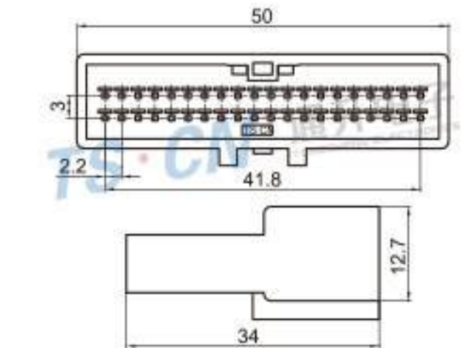
Type: TSTA40-40P-11-2 Material: PA66 Matching Terminal: TSZ208
