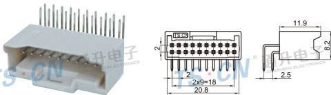
Type: TS30046-20PM-PKB(QRA3) Material: PA66 GF15% Matching Terminal: TSPM0143 / TSPM0144
