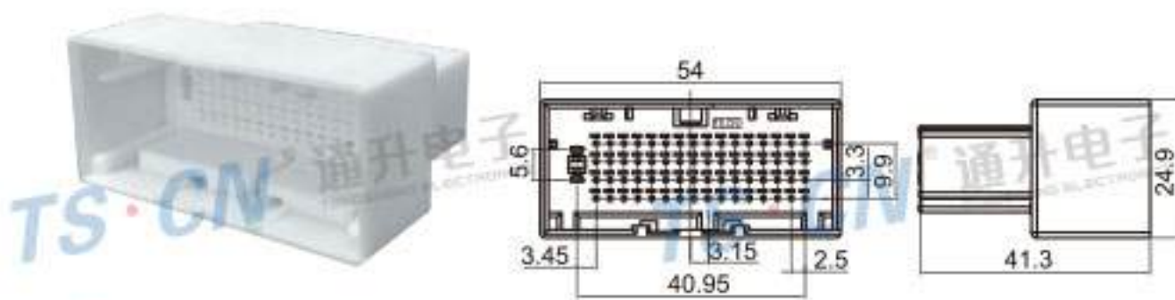
Type: TS30283-66P-11-2 Material: PBT Matching Terminal: TSZ045 / TSZ616
