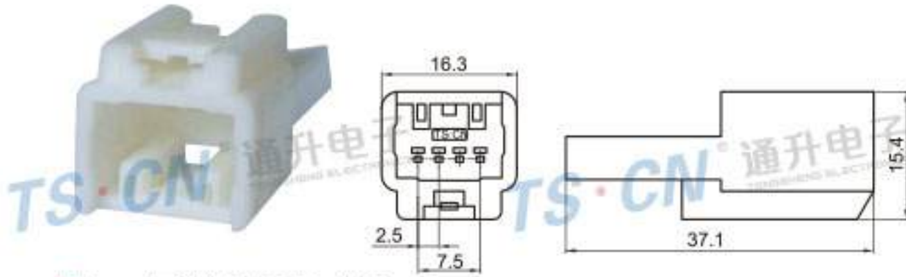
Type: TSTA04-04P-11-2 Material: PA66 Matching Terminal: TSZ208
