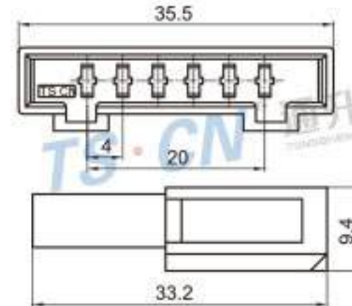
Type: TSVW06-06P-11-1 Material: PA66 GF15% Matching Terminal: TSZ040
