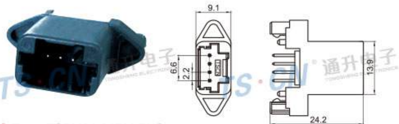
Type: TSBM04-04PM-PKS Material: PA66 GF15% Matching Terminal: TSPM0057
