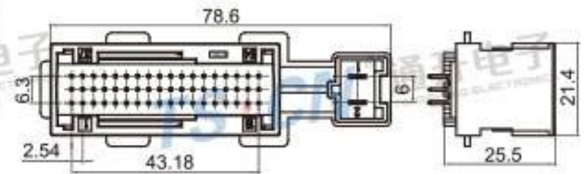
Type: TS30237-56PM-PKS Material: PBT GF15% Matching Terminal: TSPM0275 / TSPM0276
