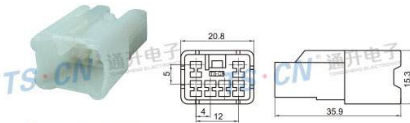
Type: TS1761-06P-11 Material: PA66 Matching Terminal: TSZ003
