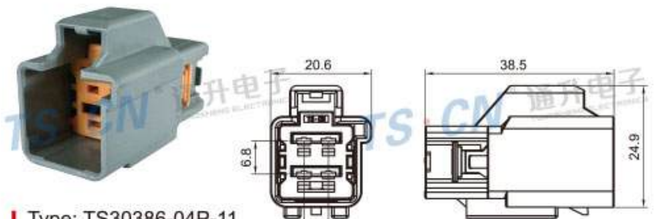
Type: TS30386-04P-11 Material: PA66 GF30% Matching Terminal: TSH650
