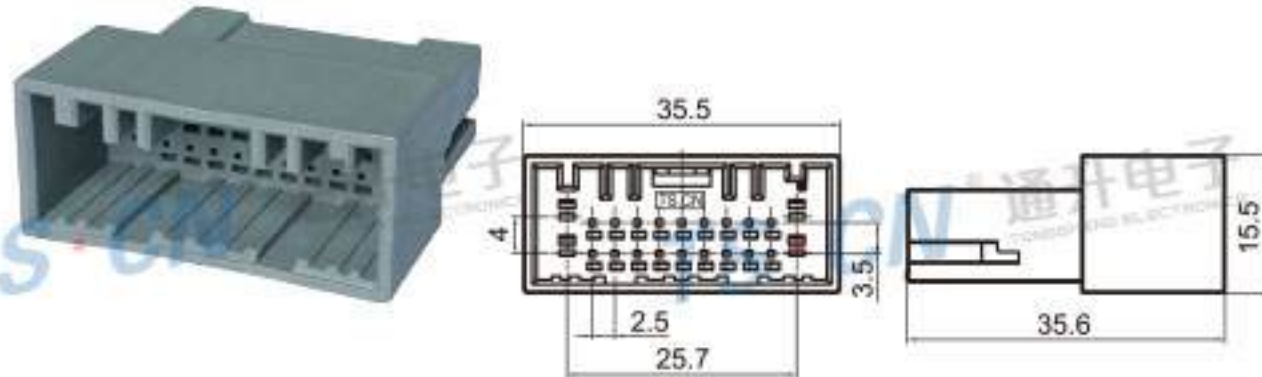
Type: TS30302-22P-11-1 Material: PBT Matching Terminal: TSZ040 / TSZ616
