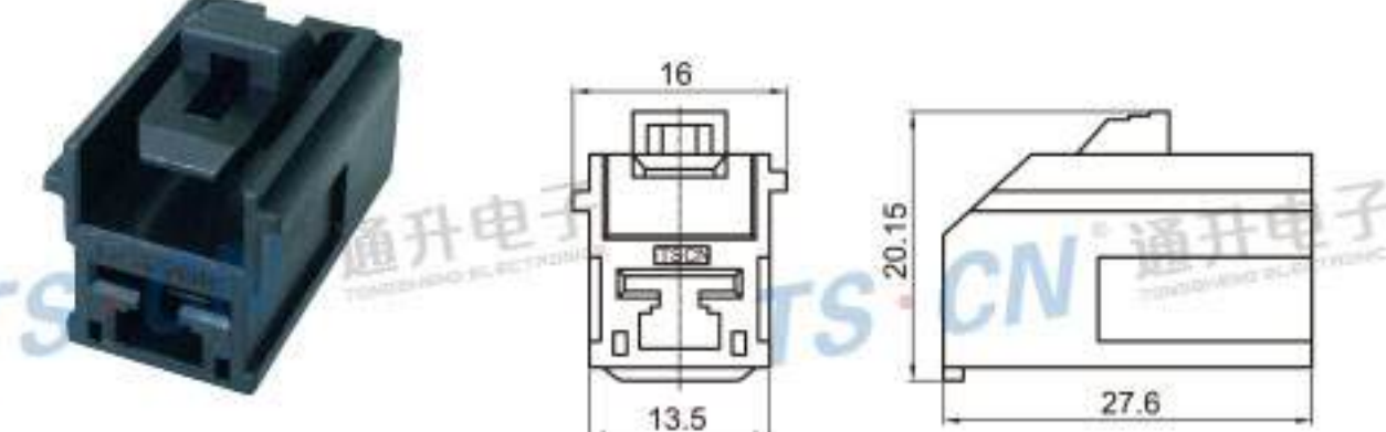
Type: TS30144-01P-21 Material: PA66 Matching Terminal: TSDJ625-7.8D
