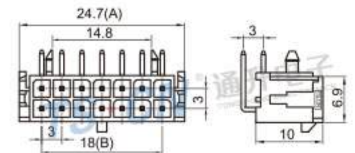
Type: TS43025-14PM-PKB(02P-24P) Material: PA66 GF30% Matching Terminal: TSPM0066 / TSPM0121
