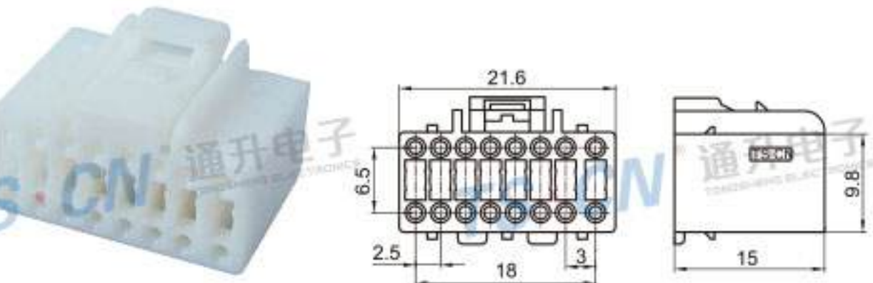
Type: TSALP16-16P-21 Material: PA66 Matching Terminal: TSH031
