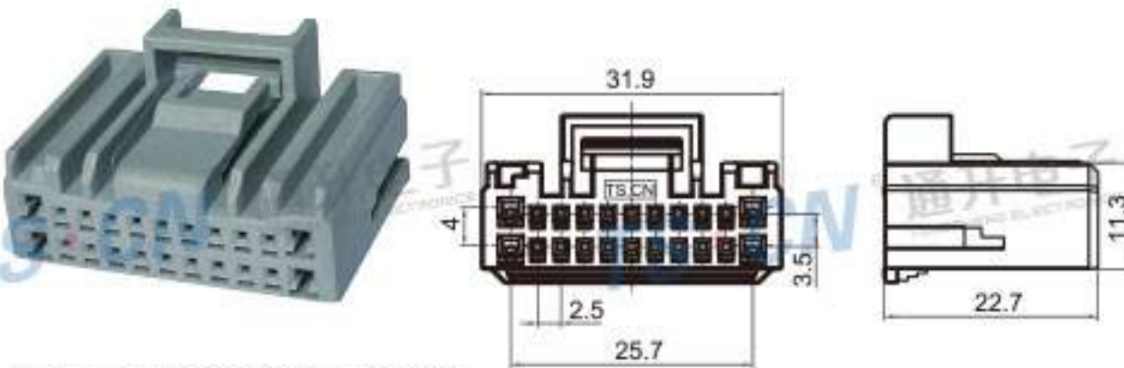
Type: TS30302-22P-21-1 Material: PBT Matching Terminal: TSH651 / TSH624
