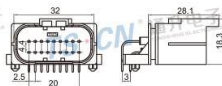
Type: TS30160-18PM-PKB Material: PBT GF30% Matching Terminal: TSPM0148 / TSPM0149
