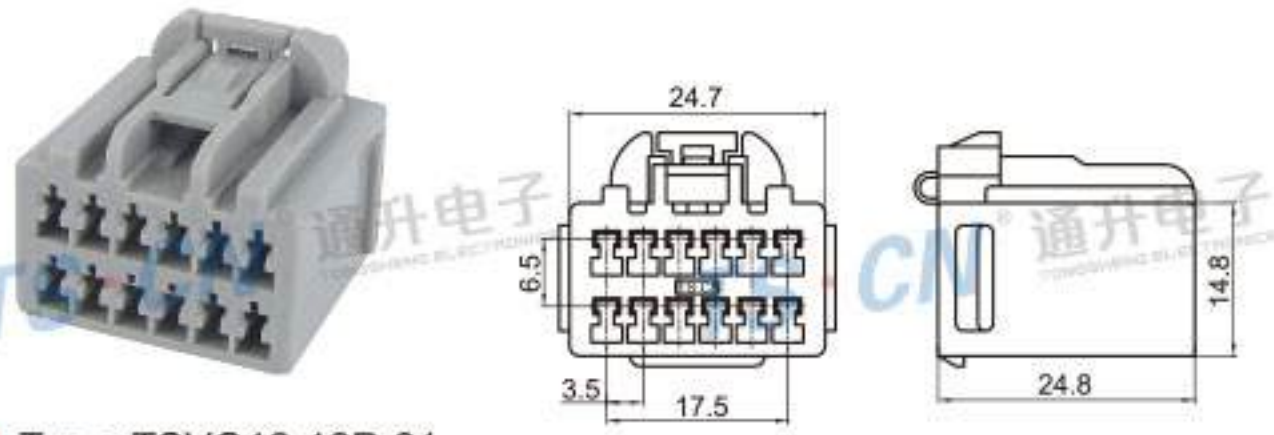
Type: TSVO12-12P-21 Material: PA66 Matching Terminal: TSH047
