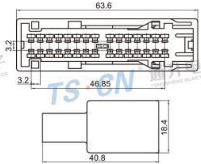
Type: TS1030-30P-11 Material: PA66 Matching Terminal: TSZ011
