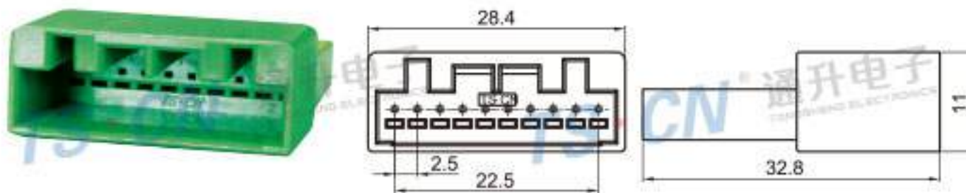
Type: TSHD10-10P-11 Material: PA66 Matching Terminal: TSZ208B
