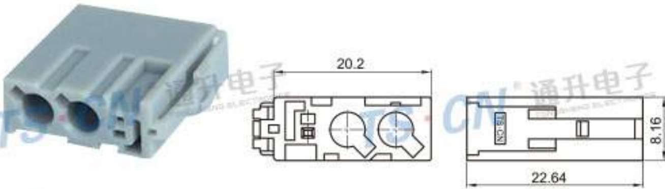
Type: TSHD21-03PF-AT Material: PA66 Matching Terminal: TSH143 / TSTF0007 / TSTM0004
