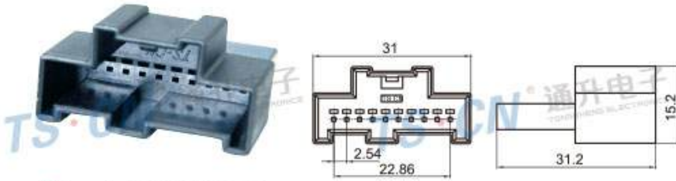
Type: TS2105-10P-11 Material: PA66 GF30% Matching Terminal: TSZ208B
