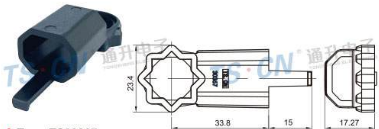
Type: TS30367 Material: PA66 GF30% Matching Terminal: NIL
