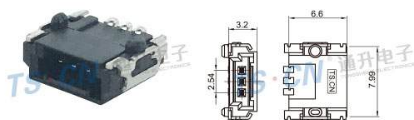
Type: TS30278-03PM-PKB Material: PPS Matching Terminal: TSPM0306 / TSPM0307
