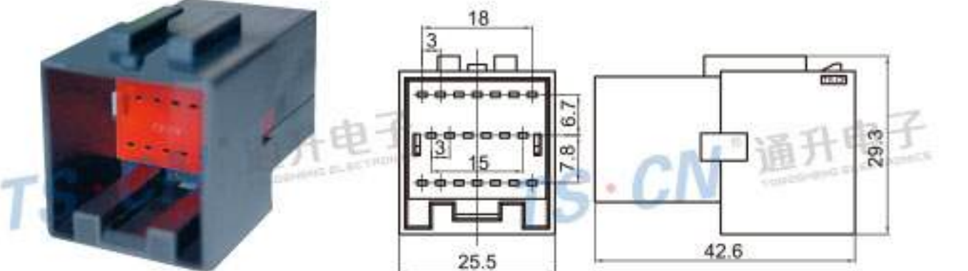
Type: TS30056-20P-11(5700) Material: PA66 Matching Terminal: TSZ185
