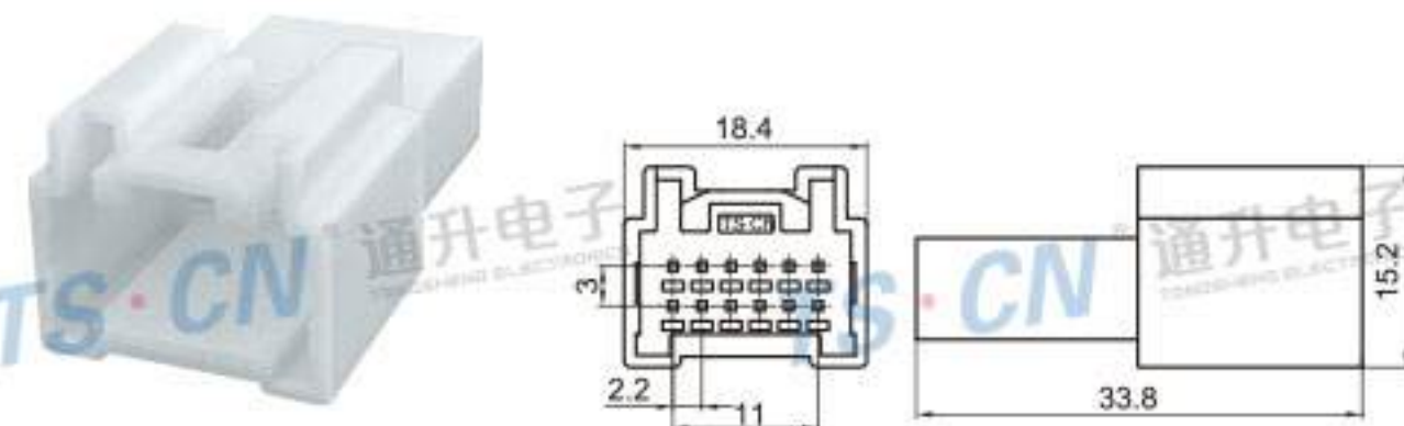
Type: TSMA12-12P-11 Material: PA66 Matching Terminal: TSZ208B
