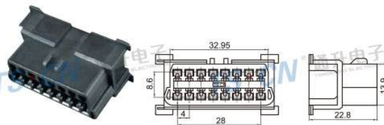
Type: TSOBD-16P-21-3 Material: PA66 GF30% Matching Terminal: TSH009
