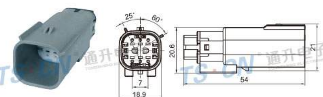
Type: TS30359-06P-11-1 Material: PA66 GF30% Matching Terminal: TSZ144A
