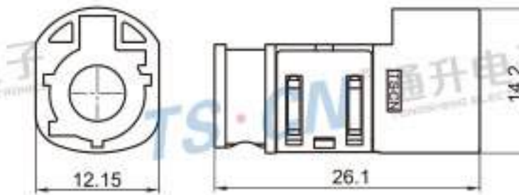
Type: TSVW10-04PM-AT-5PK-1 Material: PA66 GF15% Matching Terminal: TSPM0175 / TSTM0051
