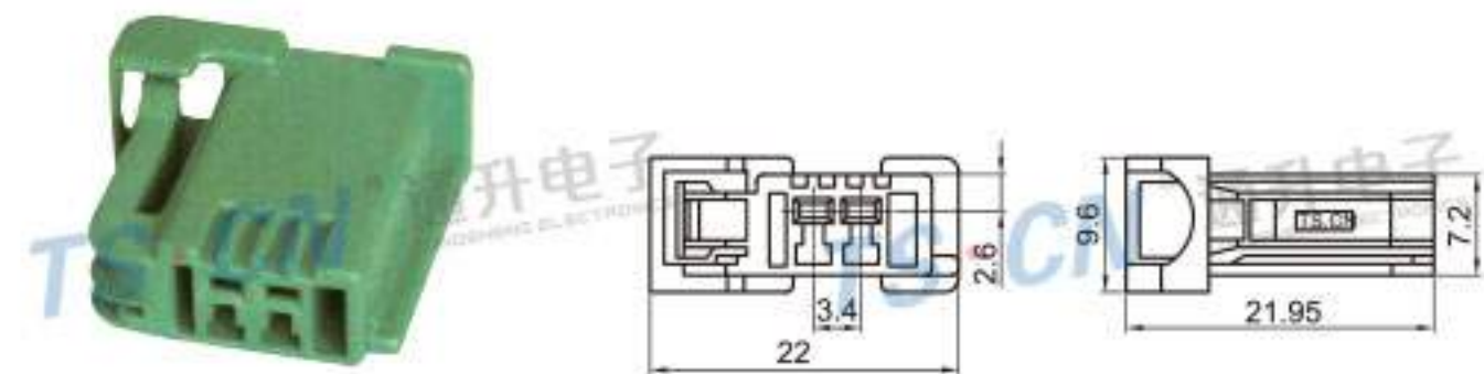
Type: TS30004-02P-21 Material: PBT GF15% Matching Terminal: TSH008
