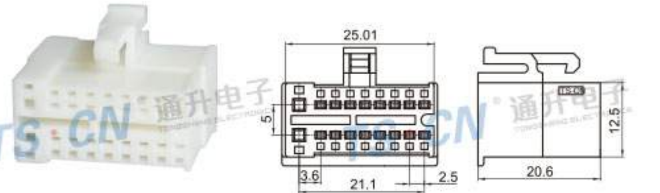
Type: TSCLR18-18P-21 Material: PA66 Matching Terminal: TSH052 / TSH053
