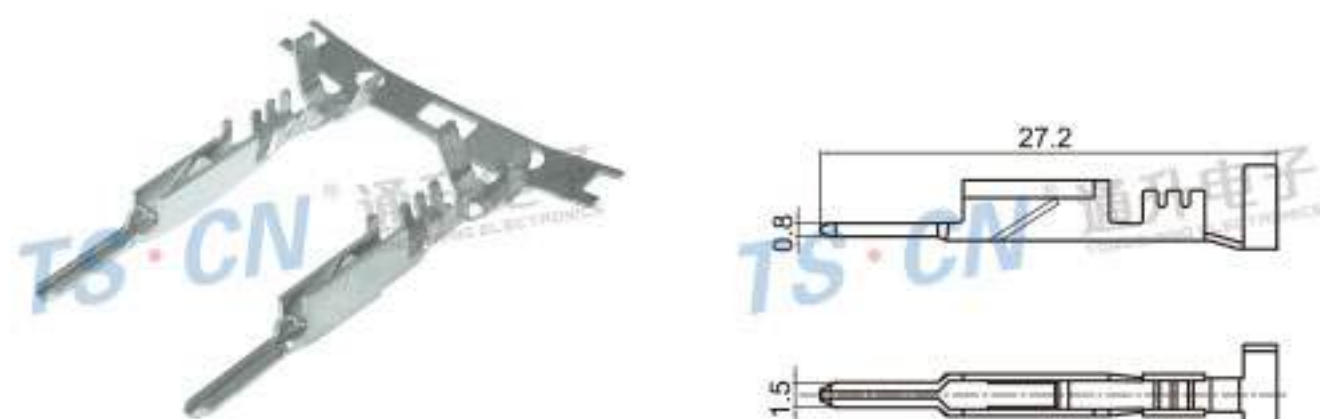
Type: TSZ614 Material: Brass
