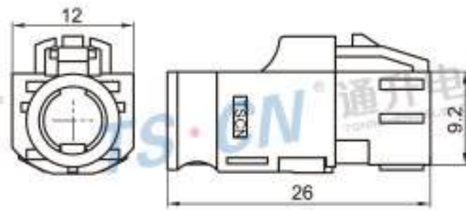
Type: TSVW20-04PF-AT-5LG-1 Material: PA66 GF30% Matching Terminal: TSTF0051 / TSTF0052
