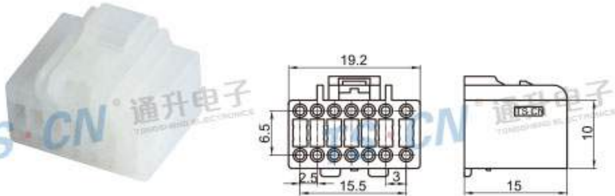
Type: TSALP14-14P-21 Material: PA66 Matching Terminal: TSH031
