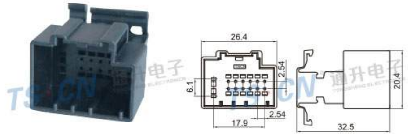
Type: TS30072-14P-11(2015) Material: PA66 GF15% Matching Terminal: TSZ040B / TSZ208B
