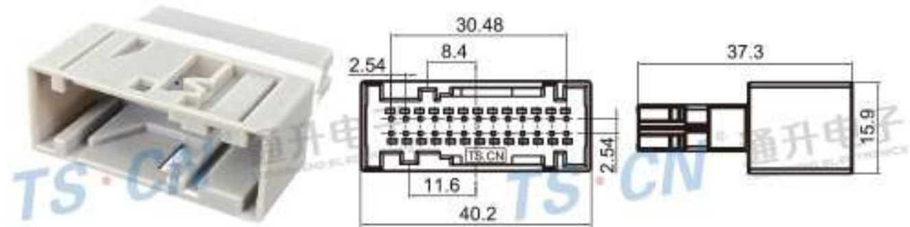
Type: TS30316-26P-11-2 Material: PA66 GF30% Matching Terminal: TSZ616
