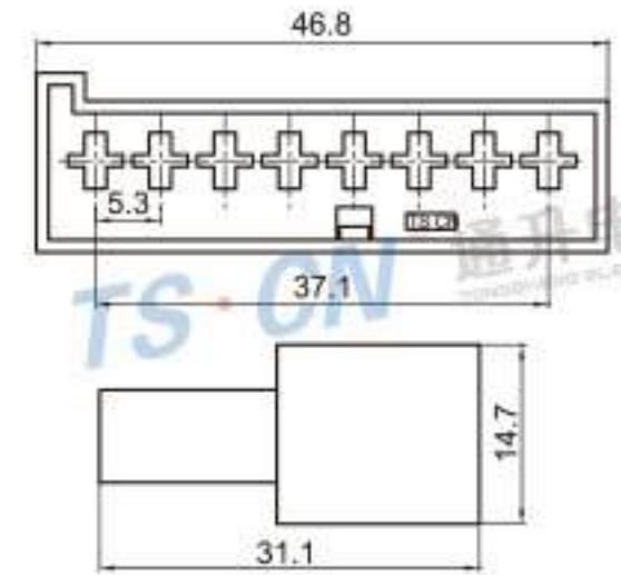
Type: TS1777-08P-11-1 Material: PA66 Matching Terminal: TSZ024
