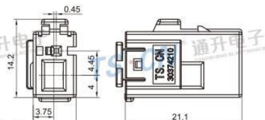
Type: TS30374-02PF-AT Material: PA66 Matching Terminal: TSTF0001/TSTF0002/TSTF6001
