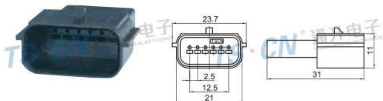
Type: TS30121-06P-11 Material: PA66 GF30% Matching Terminal: TSZ208B
