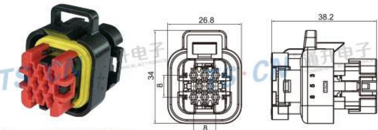
Type: TS30256-08P-21 Material: ABS+PC Matching Terminal: TSH640
