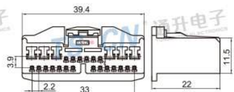
Type: TSTA26-26P-21 Material: PA66 Matching Terminal: TSH064 / TSH143
