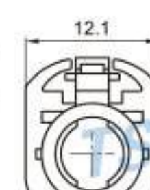
Type: TSVW20-04PF-AT-5BK Material: PA66 GF30% Matching Terminal: TSTF0048 / TSTF0049 / TSTF0050
