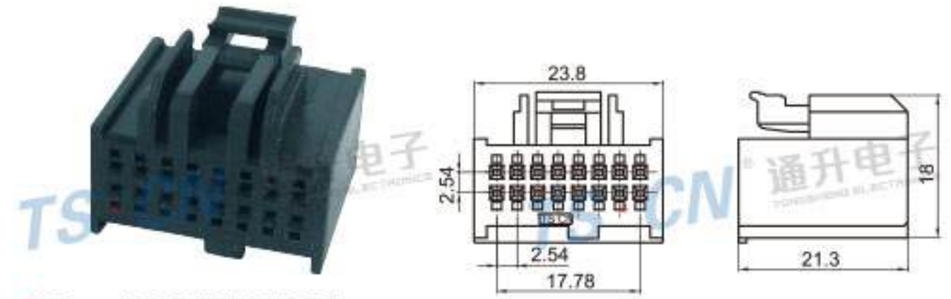
Type: TS2105-16P-21 Material: PA66 GF30% Matching Terminal: TSH143B
