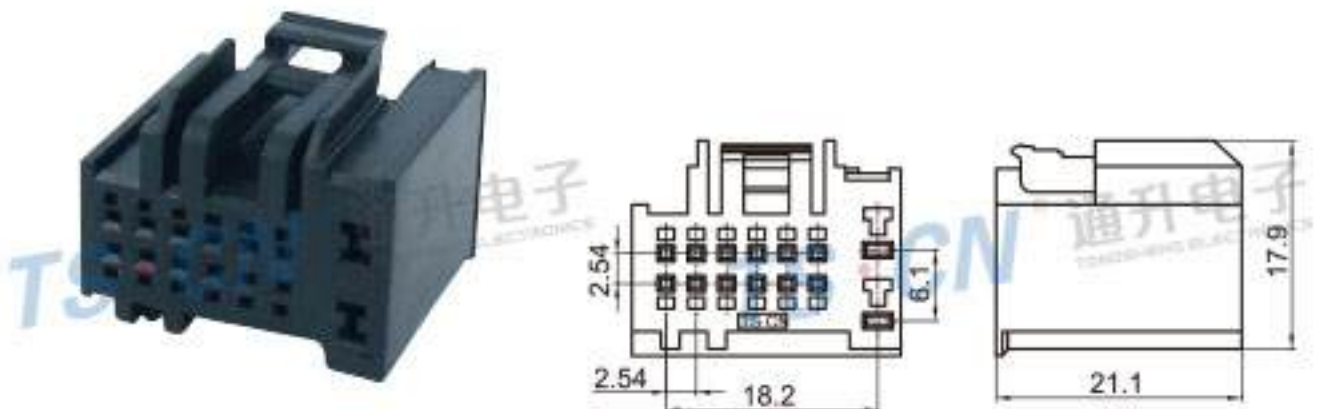
Type: TS2105-14P-21 Material: PA66 GF30% Matching Terminal: TSH008/TSH143B
