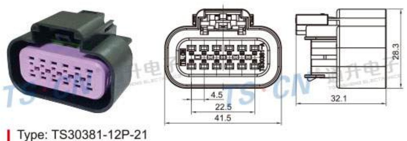
Type: TS30381-12P-21 Material: PA66 GF30% Matching Terminal: TSDJ625-F1.5A
