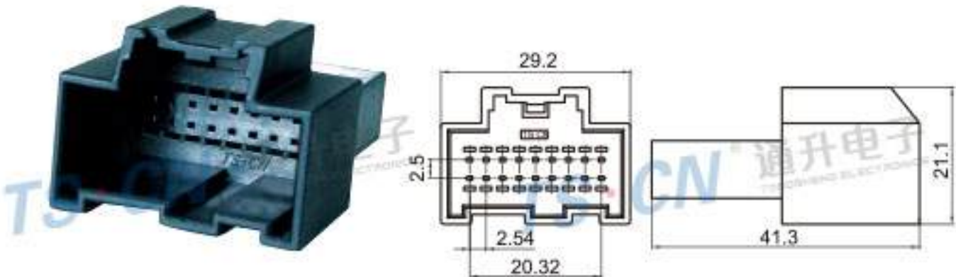
Type: TSGM18-18P-11-1 Material: PA66 GF30% Matching Terminal: TSZ208B
