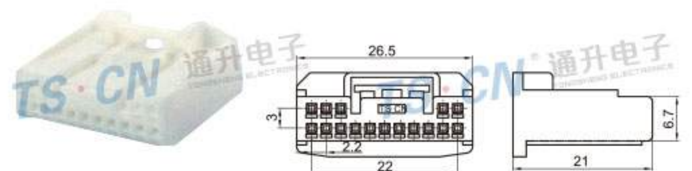
Type: TSHD16-16P-21-1 Material: PA66 Matching Terminal: TSH143
