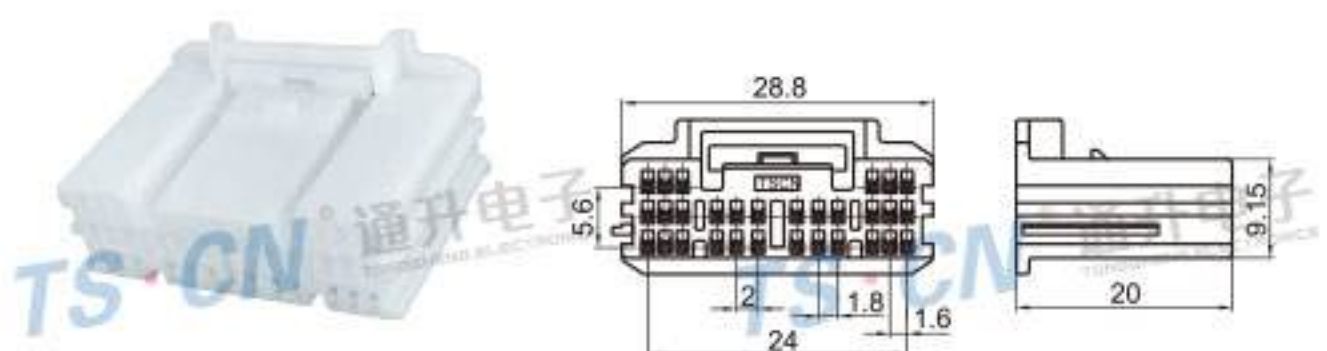
Type: TS30101-30P-21-2 Material: PA66 Matching Terminal: TSH600
