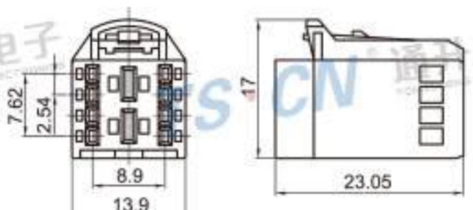
Type: TS30141-10P-21 Material: PBT GF15% Matching Terminal: TSH019/TSH092
