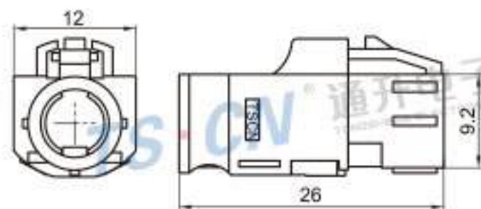
Type: TSVW20-04PF-AT-5VT-1 Material: PA66 GF30% Matching Terminal: TSTF0051 / TSTF0052
