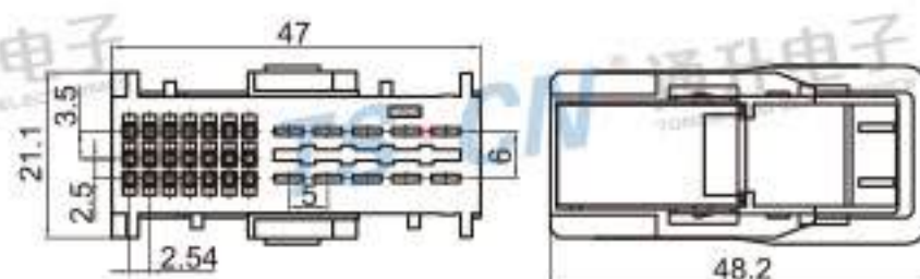
Type: TS30102-31P-21 Material: PBT GF15% Matching Terminal: TSH019/TSH143
