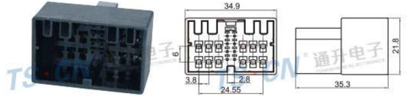
Type: TS30071-20P-11 Material: PA66 GF30% Matching Terminal: TSZ009 / TSZ208
