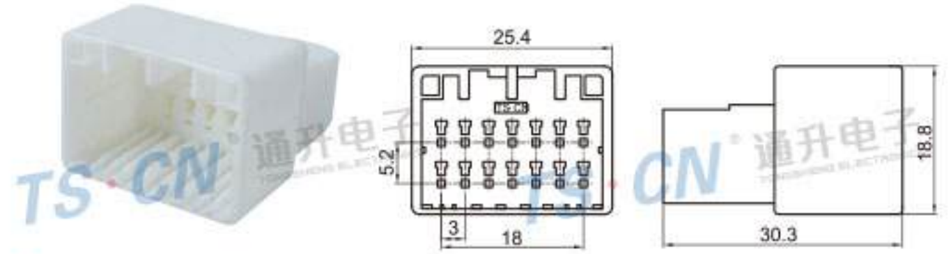
Type: TSHD14-14P-11 Material: PA66 Matching Terminal: TSZ018
