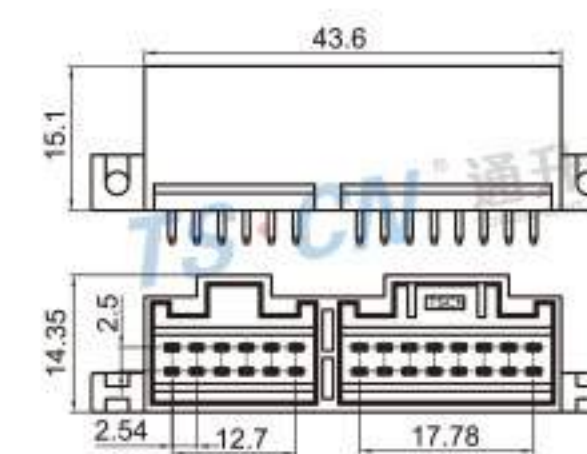
Type: TSPAN-28PM-PKB Material: PA66 Matching Terminal: TSPM0045 / TSPM0046
