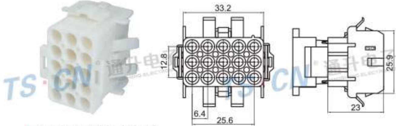
Type: TSPP15-15P-21 Material: PA66 GF15% Matching Terminal: TSH536
