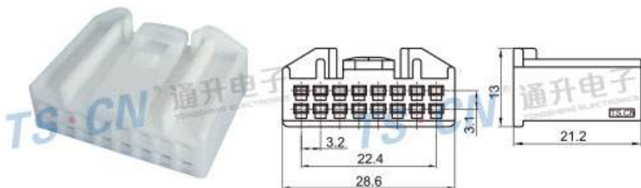
Type: TS30017-16PM-21 Material: PA66 Matching Terminal: TSH593
