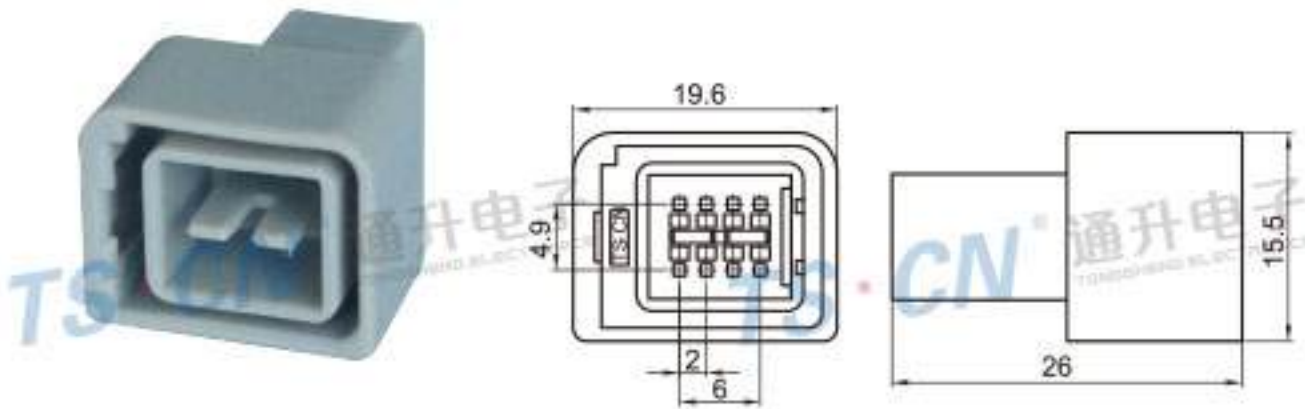
Type: TSNI08-08P-11 Material: PA66 GF30% Matching Terminal: TSZ540 / TSZ537
