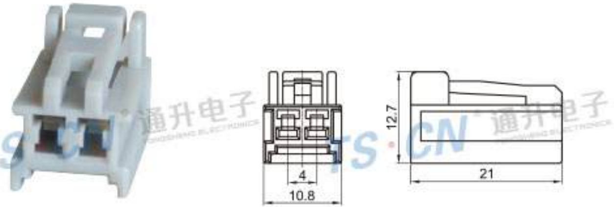
Type: TS30093-02P-21 Material: PA66 Matching Terminal: TSH009
