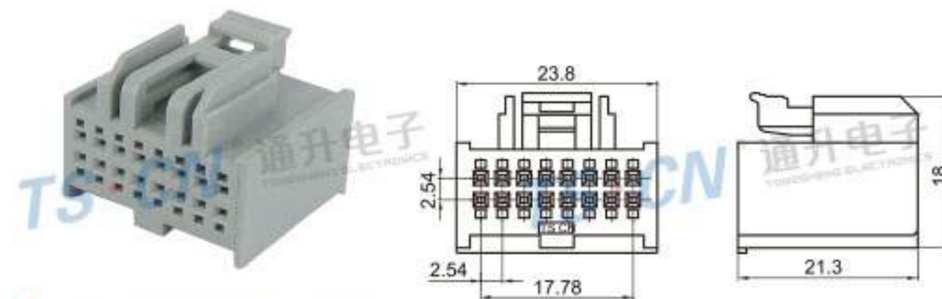
Type: TS2105-16P-21GY Material: PA66 Matching Terminal: TSH143B
