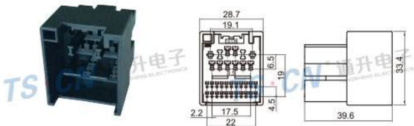
Type: TS30284-32P-11 Material: PA66 GF30% Matching Terminal: TSZ024 / TSZ144 / TSZ208B
