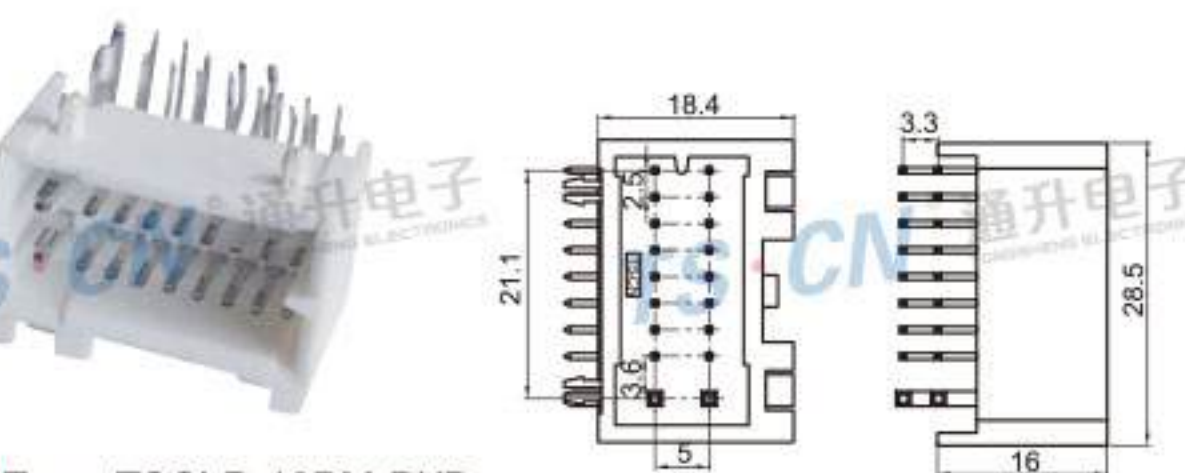
Type: TSCLR-18PM-PKB Material: PA66 Matching Terminal: TSPM0034~TSPM0037
