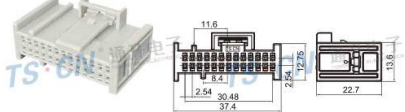
Type: TS30316-26P-21-2 Material: PA66 GF30% Matching Terminal: TSH624
