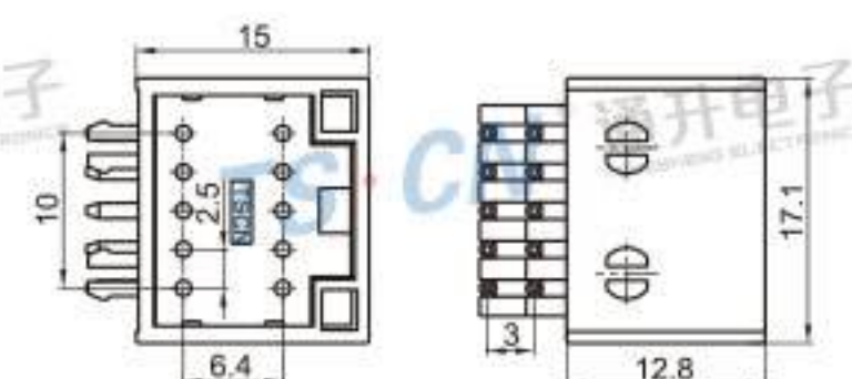
Type: TSKEN-10PM-PKB Material: PA66 GF30% Matching Terminal: TSPM0103 / TSPM0106
