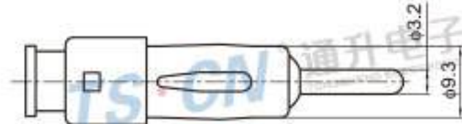
Type: TSAM-AT-1 Material: PA66 Matching Terminal: TSTM0009 / TSTM0010
