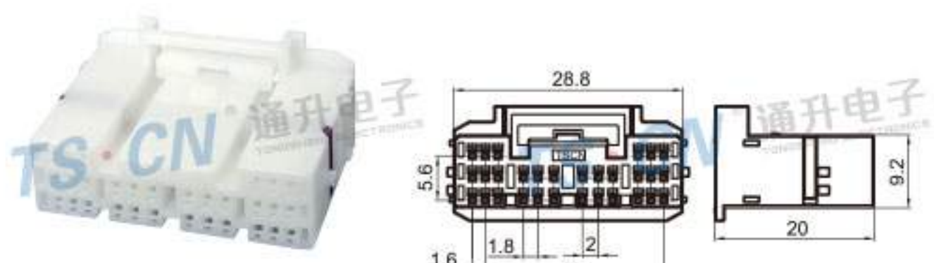
Type: TS30101-30P-21-7 Material: PA66 Matching Terminal: TSH600A
