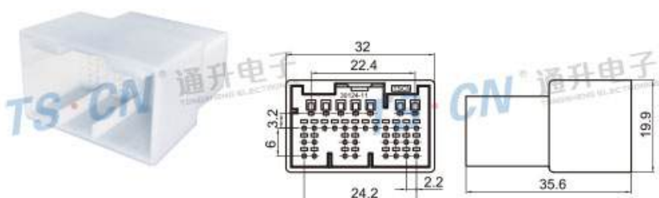
Type: TS30124-35P-11 Material: PA66 Matching Terminal: TSZ145 / TSZ208
