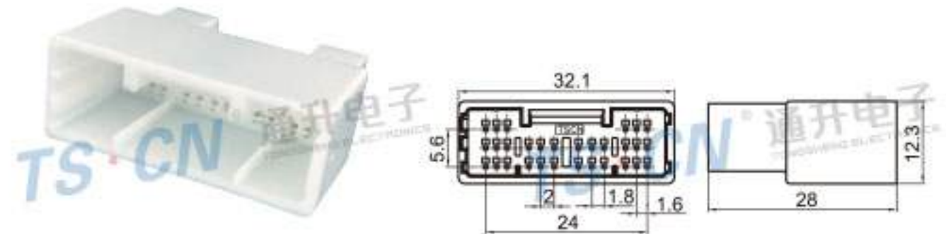
Type: TS30101-30P-11 Material: PA66 Matching Terminal: TSZ556
