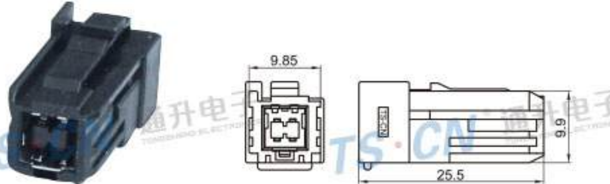
Type: TSTA04-04PF-AT-3 Material: PA66 Matching Terminal: TSTF0008 / TSTF0010 / TSTF0011
