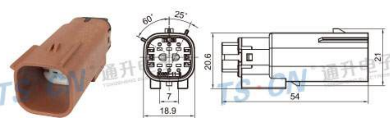
Type: TS30359-06P-11-2 Material: PA66 GF30% Matching Terminal: TSZ144A
