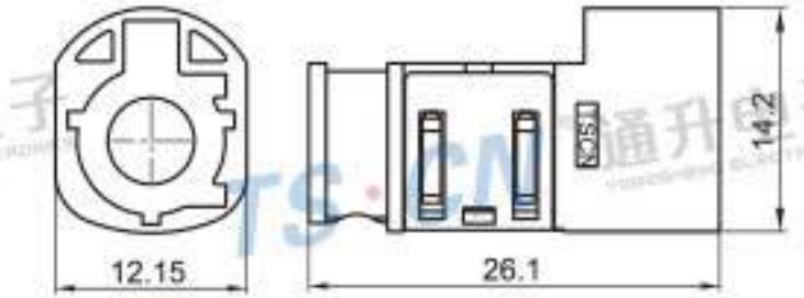
Type: TSVW10-04PM-AT-5OR-1 Material: PA66 GF15% Matching Terminal: TSPM0175 / TSTM0051
