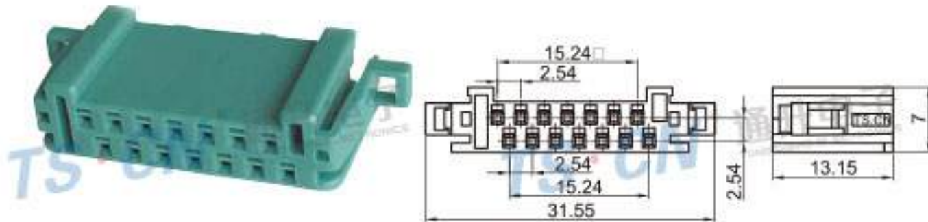
Type: TS30014-14P-21 Material: PBT GF15% Matching Terminal: TSPHB
