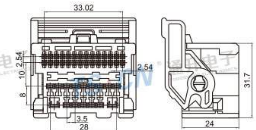
Type: TSKL44-44P-21 Material: PA66 GF30% Matching Terminal: TSH085 / TSH008 / TSH143
