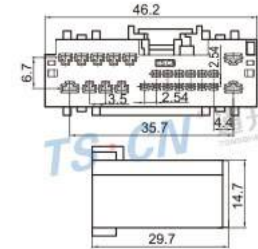
Type: TS5520-24P-11 Material: PA66 GF30% Matching Terminal: TSZ143 / TSZ144 / TSZ145
