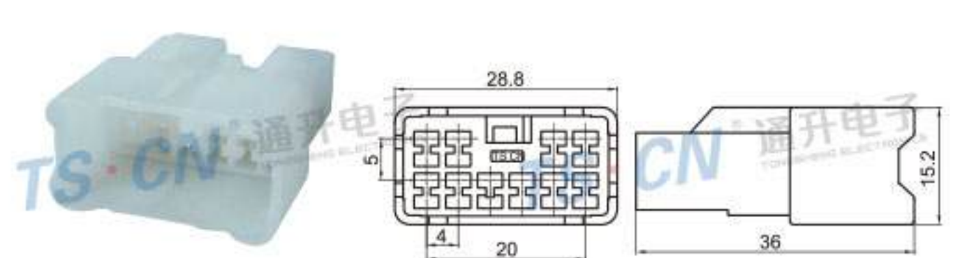
Type: TS1761-10P-11 Material: PA66 Matching Terminal: TSZ003
