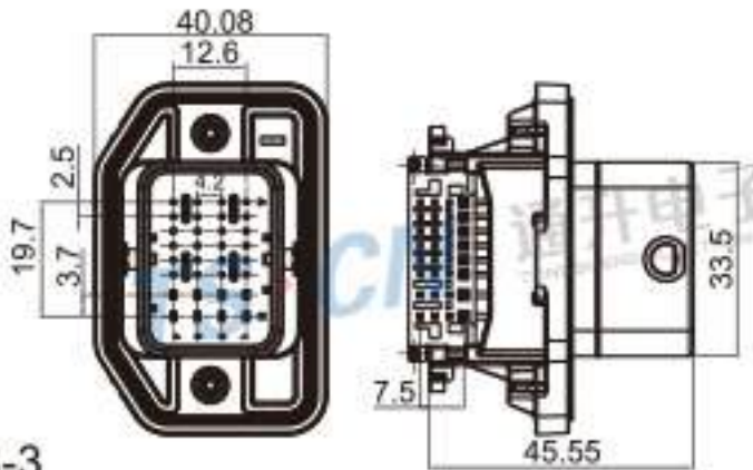
Type: TS30245-32PM-PKB-3 Material: GF30% PBT Matching Terminal: TSPM0289~TSPM0296
