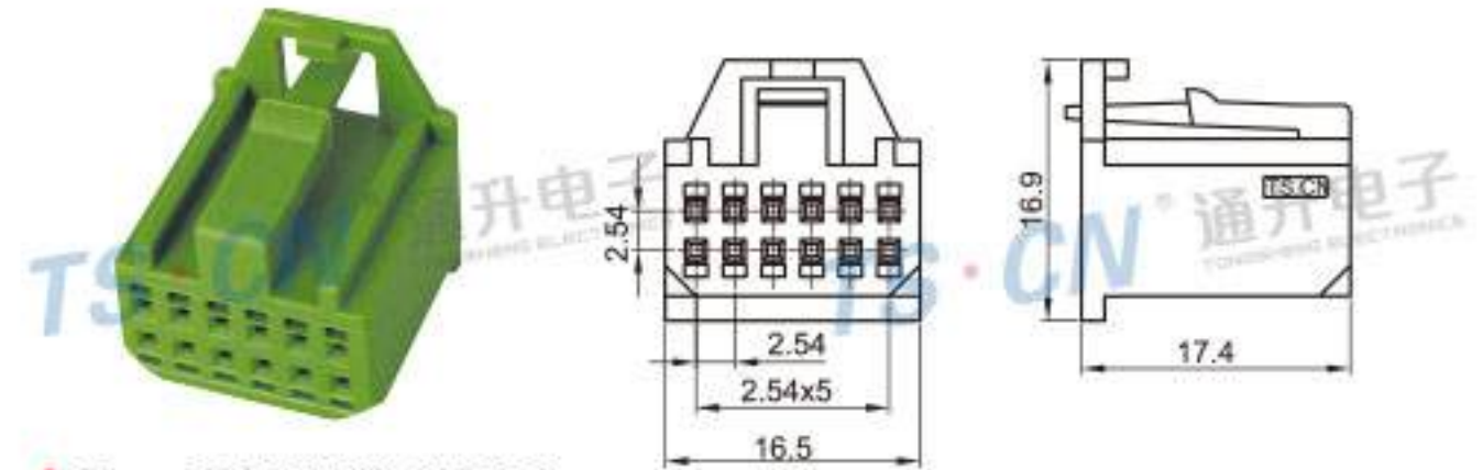
Type: TS30023-12P-21 Material: PBT Matching Terminal: TSH143
