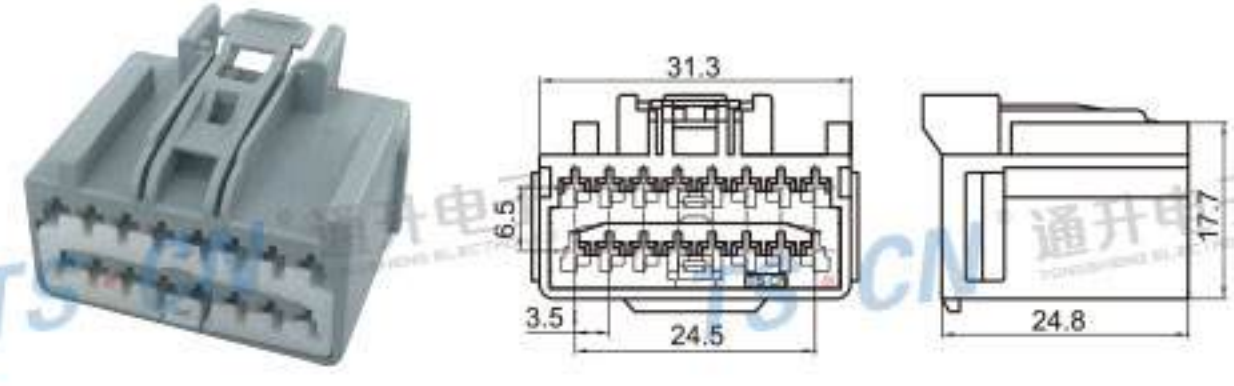
Type: TSVO16-16P-21-3 Material: PBT GF10% Matching Terminal: TSH047
