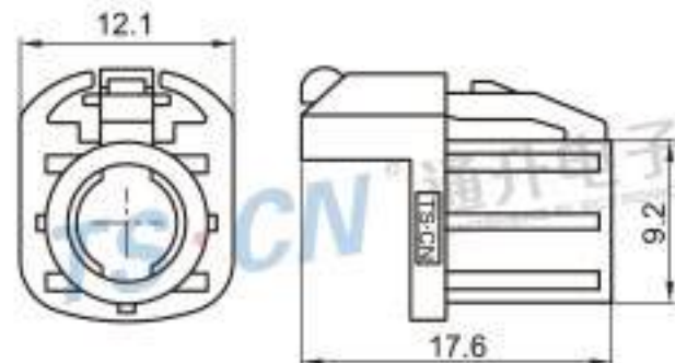
Type: TSVW20-04PF-AT-5WB Material: PA66 GF30% Matching Terminal: TSTF0048 / TSTF0049 / TSTF0050
