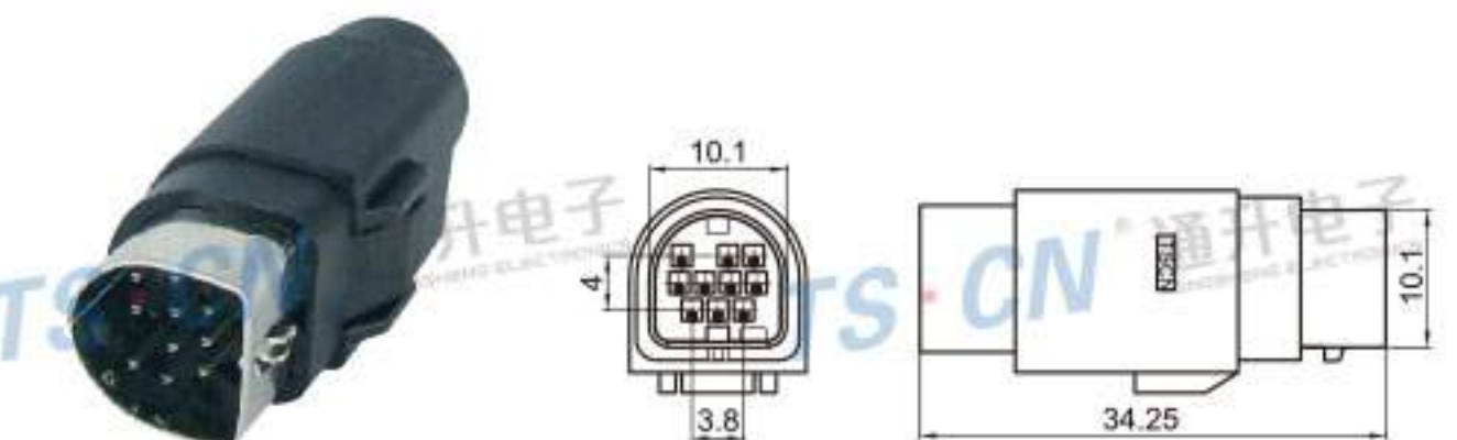
Type: TSALPH-10PM-AH-1 Material: PA66 Matching Terminal: TSAM0014 / TSAM0015 / TS0079
