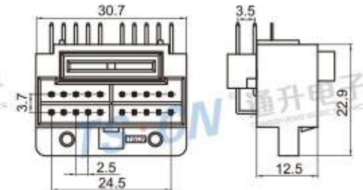
Type: TSJEN-20PM-PKB Material: PA66 GF30% Matching Terminal: TSPM0099 / TSPM00101 / TSPM0102
