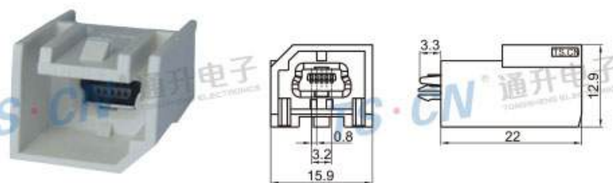
Type: TS30045-05PM-PKS Material: PA66 GF30% Matching Terminal: TSPM0205
