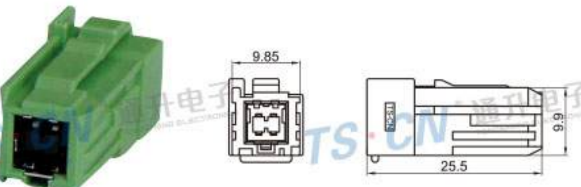
Type: TSTA04-04PF-AT-1 Material: PA66 Matching Terminal: TSTF0008 / TSTF0010 / TSTF0011
