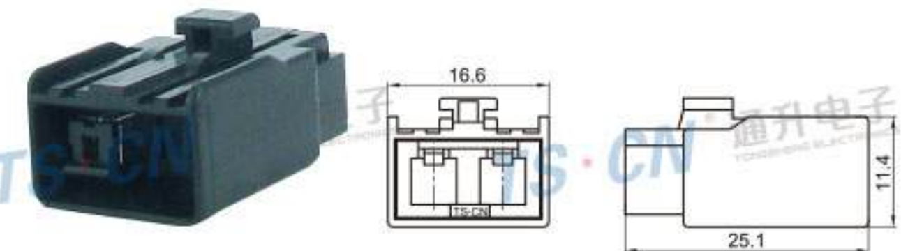
Type: TSVL20-02PF-AT Material: PA66 GF15% Matching Terminal: TSTF0014 / TF0015
