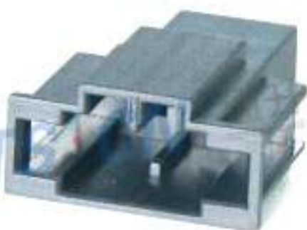
Type: TSVWLB32-02P-11 Material: PA66 GF30% Matching Terminal: TSZ024
