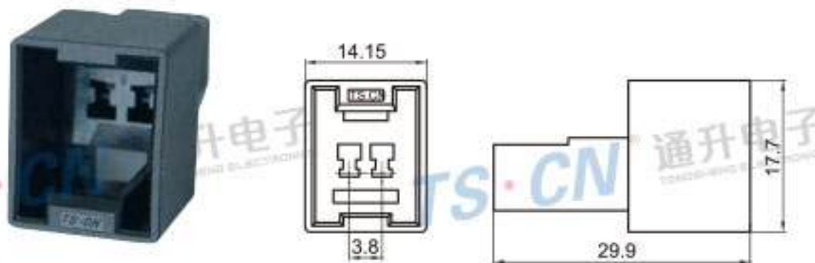
Type: TSLB03-02P-11 Material: PA66 GF30% Matching Terminal: TSZ011
