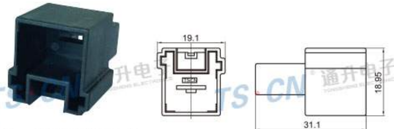
Type: TS30144-01P-11 Material: PA66 Matching Terminal: TSZ611
