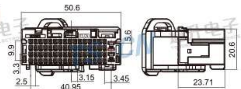
Type: TS30283-66P-21 Material: PBT Matching Terminal: TSH064 / TSH092
