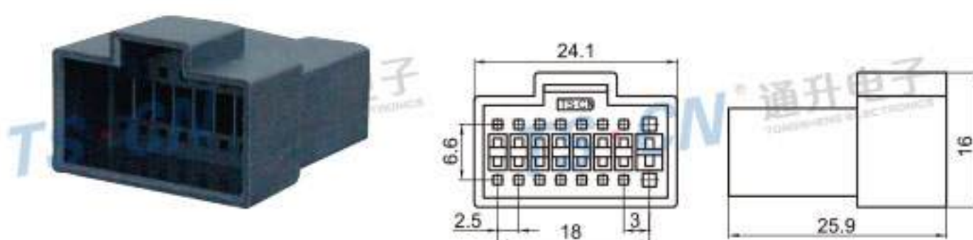
Type: TSPAN16E-16P-11 Material: PA66 GF30% Matching Terminal: TSZ532 / TSZ533
