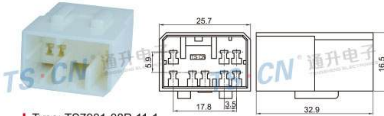
Type: TS7901-08P-11-1 Material: PA66 Matching Terminal: TSZ011
