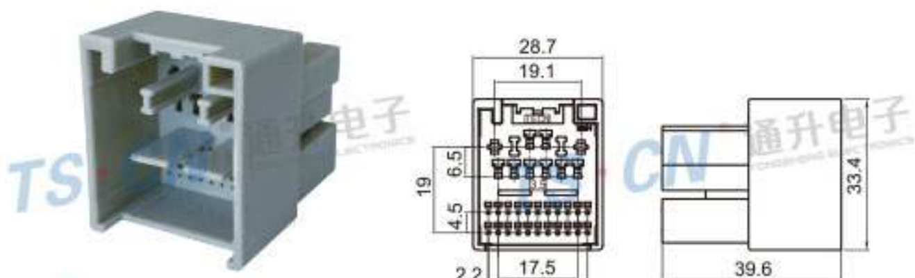
Type: TS30284-32P-11-1 Material: PA66 GF30% Matching Terminal: TSZ024 / TSZ144 / TSZ208B
