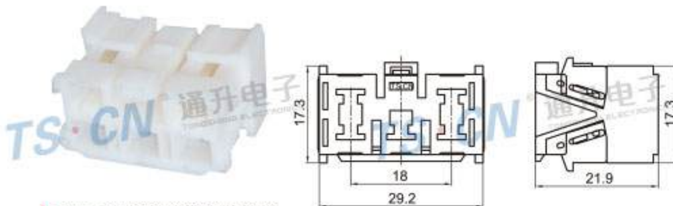
Type: TS30001-05P-21 Material: PBT Matching Terminal: TSH585
