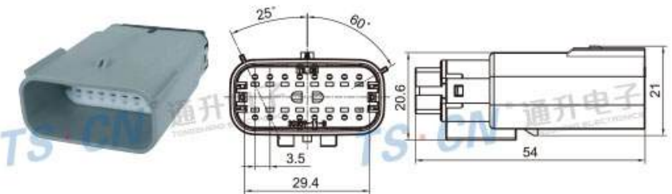
Type: TS30359-16P-11-1 Material: PA66 GF30% Matching Terminal: TSZ144A
