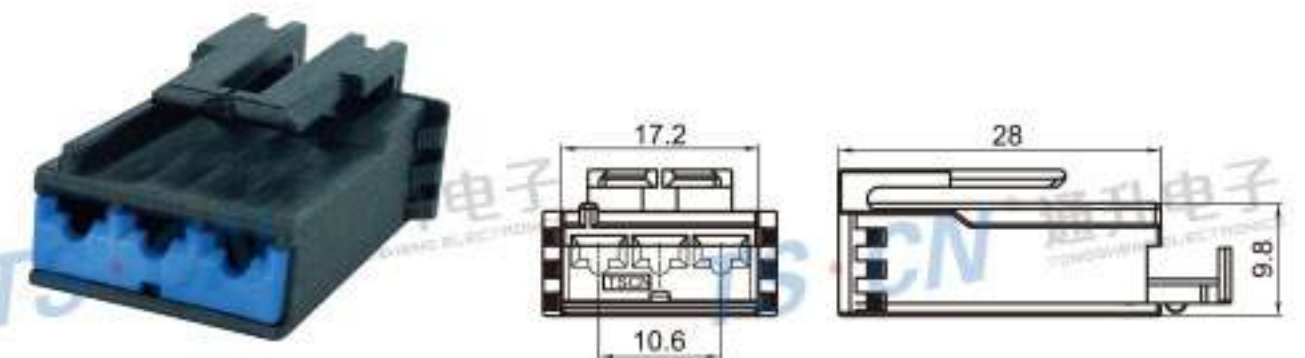
Type: TS30336-03P-21 Material: PA66 GF30% Matching Terminal: TSH085A
