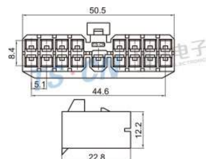
Type: TSHD17-17P-21 Material: PA66 Matching Terminal: TSH017
