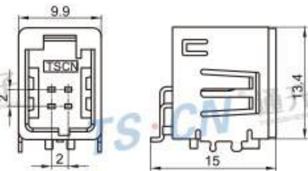
Type: TSMA04-04PM-PKB-2 Material: PA66 GF30% Matching Terminal: TSPM0029 / TSPM0031 / TSPM0032
