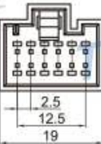
Type: TS30111-12P-11 Material: PA66 Matching Terminal: TSZ208B
