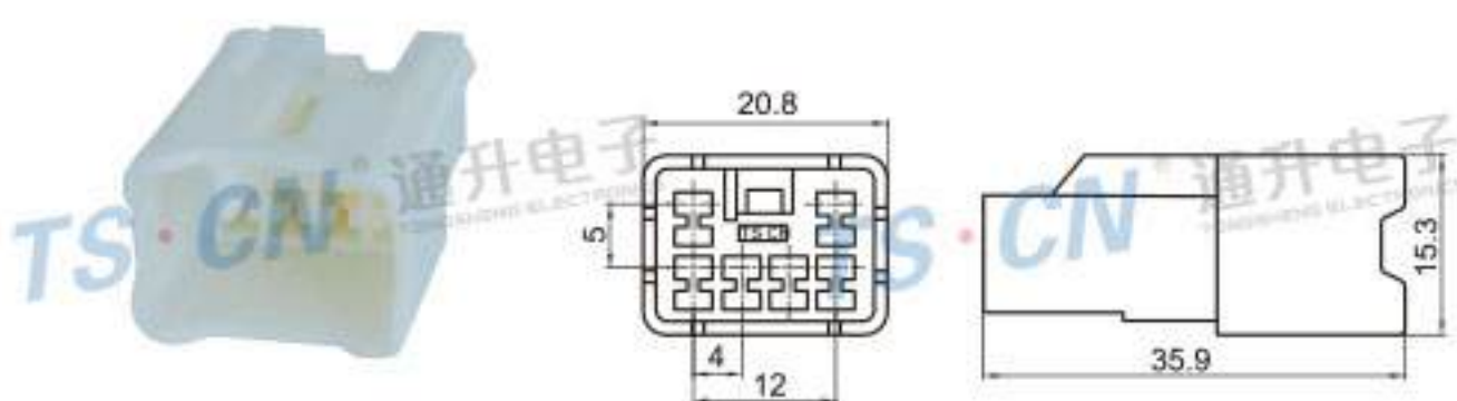
Type: TS1761-06P-11-1 Material: PA66 Matching Terminal: TSZ003
