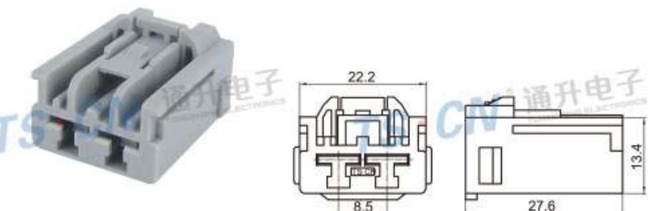
Type: TSVO02-02P-21 Material: PA66 Matching Terminal: TSH033B
