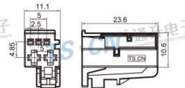
Type: TS30294-05P-21 Material: PBT Matching Terminal: TSH019C / TSH624
