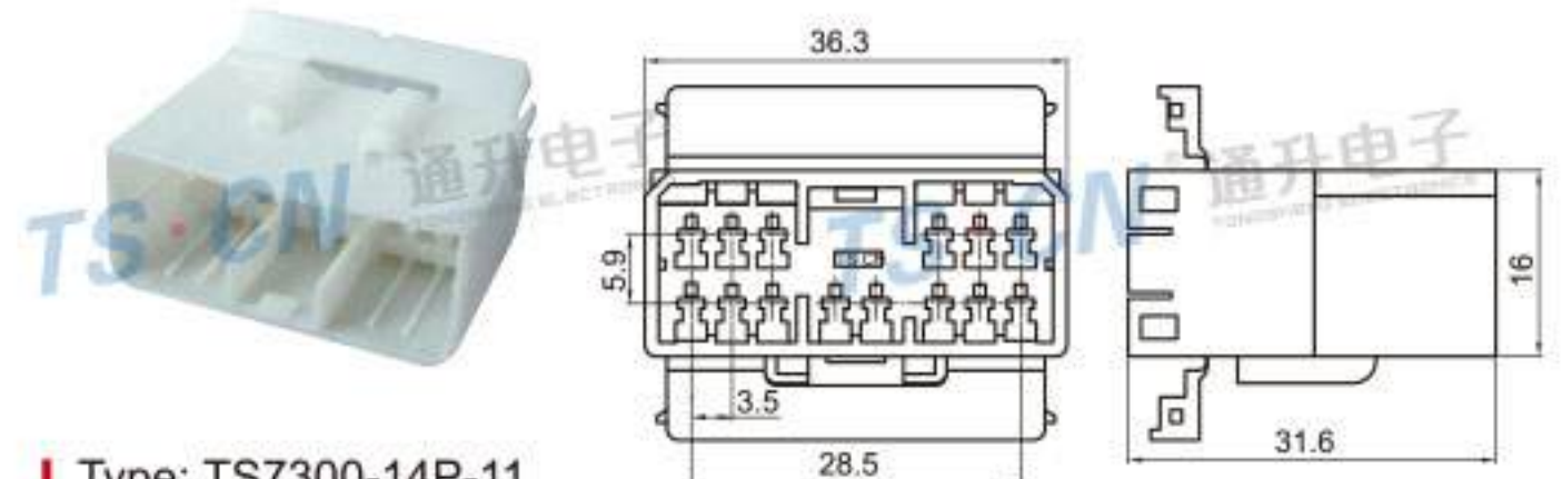
Type: TS7300-14P-11 Material: PA66 Matching Terminal: TSZ011
