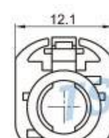
Type: TSVW20-04PF-AT-5BE Material: PA66 GF30% Matching Terminal: TSTF0048 / TSTF0049 / TSTF0050
