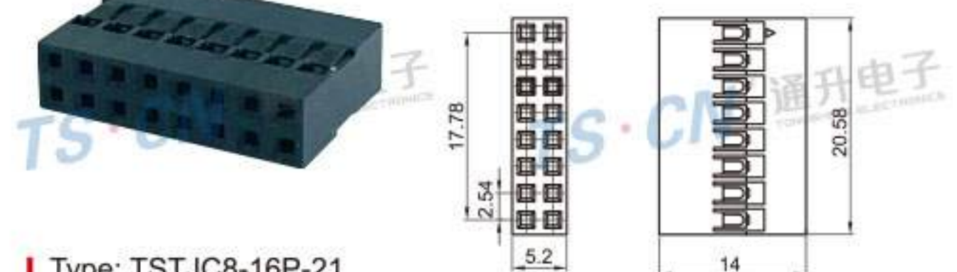
Type: TSTJC8-16P-21 Material: PA66 Matching Terminal: TS25402-PT
