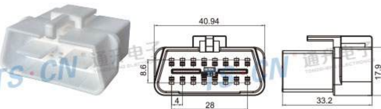
Type: TSOBD-16P-11-2 Material: PBT Matching Terminal: TSZ040B
