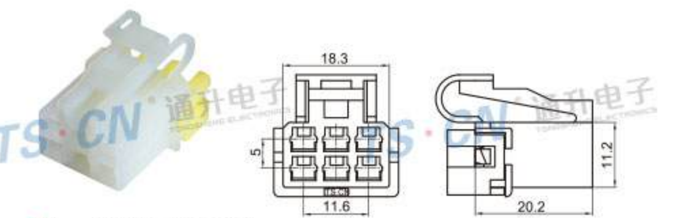
Type: TS1763-06P-21 Material: PA66 Matching Terminal: TSH011
