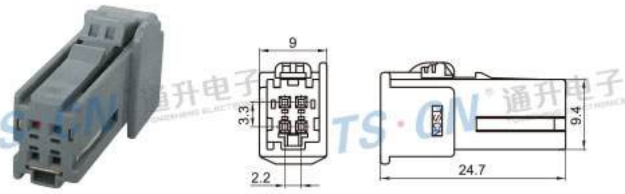
Type: TS30213-04PF-AT Material: PBT Matching Terminal: TSTF0058 / TSTF0059 / TSTF0006
