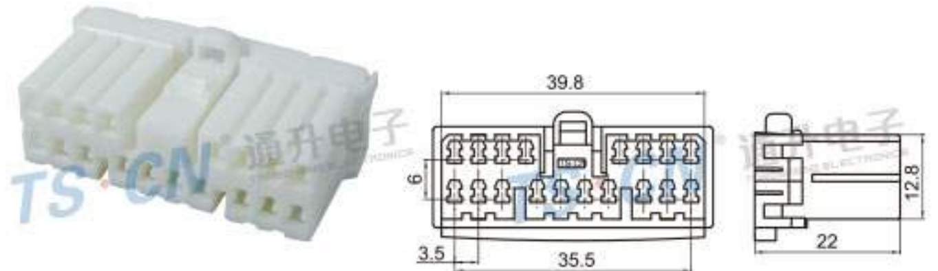
Type: TS8405-18P-21 Material: PA66 Matching Terminal: TSH016
