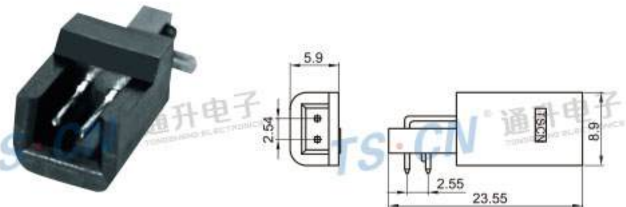
Type: TSBM02-02PM-PKB Material: PA66 GF15% Matching Terminal: TSPM0085 / TSPM0122
