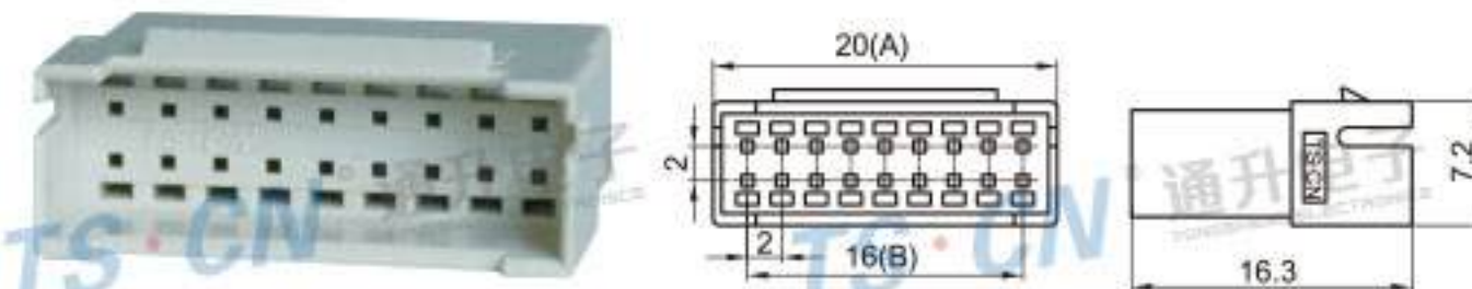
Type: TSPHB-18P-11(06P-20P) Material: PA66 GF15% Matching Terminal: TSZ210
