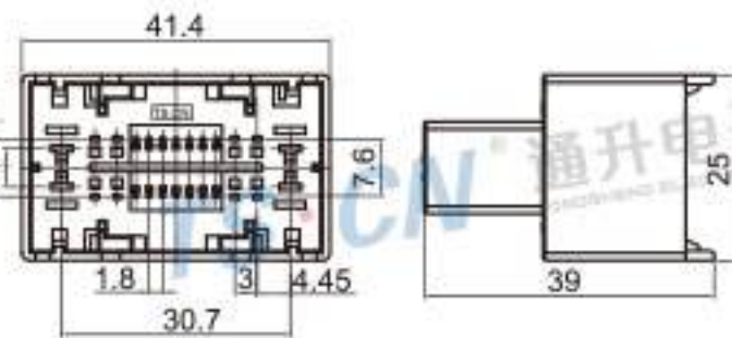
Type: TS30279-26P-11 Material: PA66 Matching Terminal: TSZ024 / TSZ566 / TSZ556
