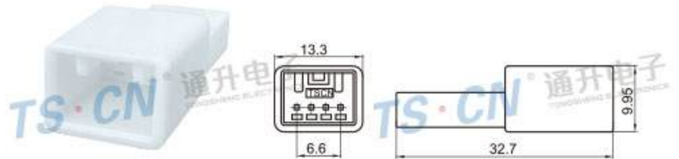
Type: TS30203-04P-11 Material: PA66 Matching Terminal: TSZ208
