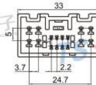
Type: TS30219-16P-11 Material: PA66 Matching Terminal: TSZ531/TSZ563
