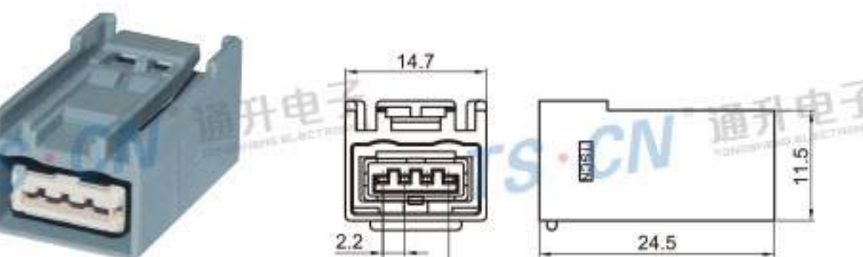
Type: TSTYUSB-04PF-AT Material: PA66 Matching Terminal: TSTF0021 / TSTF0006
