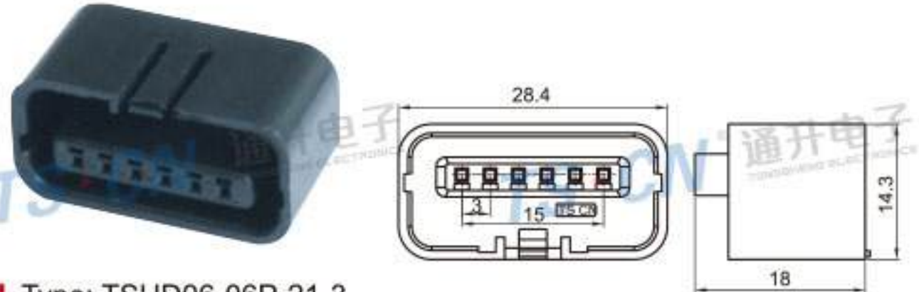
Type: TSHD06-06P-21-3 Material: PA66 Matching Terminal: TSH143
