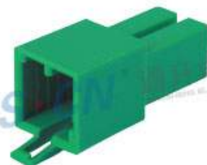
Type: TSVW06-06P-11GN Material: PA66 Matching Terminal: TSZ040
