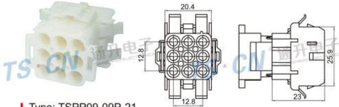
Type: TSPP09-09P-21 Material: PA66 GF15% Matching Terminal: TSH536
