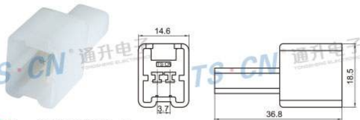
Type: TSLB28-02P-11 Material: PA66 Matching Terminal: TSZ045
