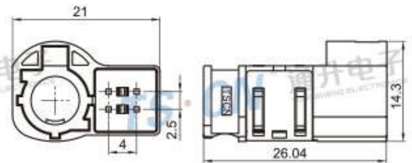
Type: TSVW10-08PM-AT-1BL Material: PBT GF15% Matching Terminal: TSPM0175 / TSTM0051 / TSZ208
