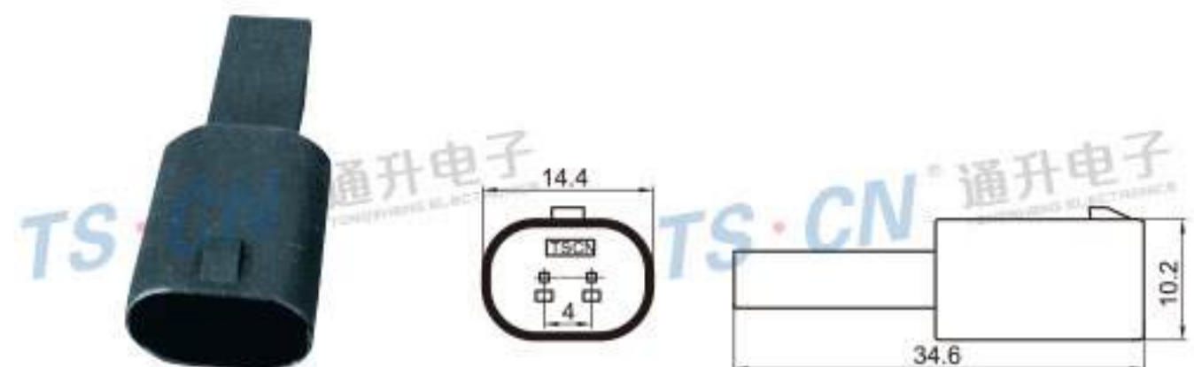
Type: TS30177-02P-11 Material: PA66 GF30% Matching Terminal: TSZ208
