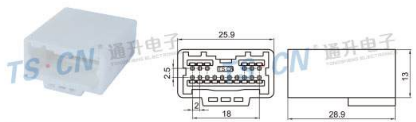
Type: TSNI16-16P-11 Material: PA66 Matching Terminal: TSZ050
