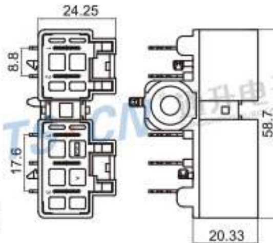
Type: TS30246-05PM-PKB-2(通孔) Material: PBT GF30% Matching Terminal: TSPM0150
