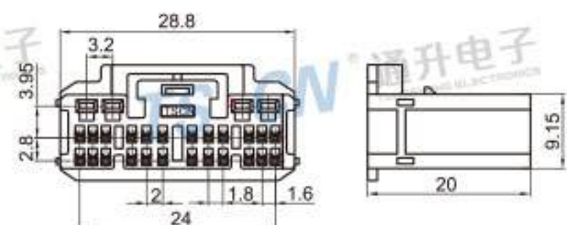
Type: TS30101-28P-21 Material: PA66 Matching Terminal: TSH593 / TSH600
