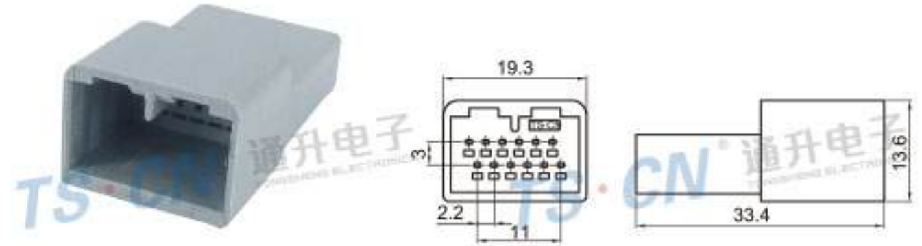
Type: TSCRV12-12P-11 Material: PA66 Matching Terminal: TSZ208B
