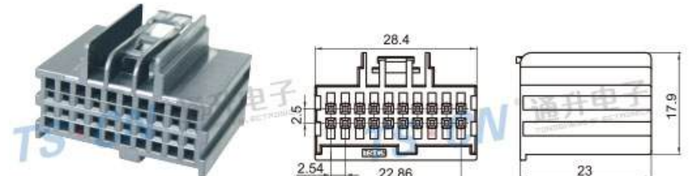
Type: TSGM20-20P-21-1 Material: PA66 GF30% Matching Terminal: TSH143
