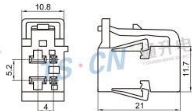
Type: TS30148-04P-21BK Material: PBT Matching Terminal: TSH091 / TSH092
