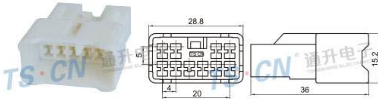
Type: TS1761-10P-11-1 Material: PA66 Matching Terminal: TSZ003
