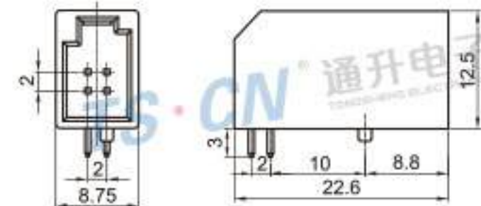
Type: TS30147-04PM-PKB-1 Material: PBT GF15% Matching Terminal: TSPM0140 / TSPM0077
