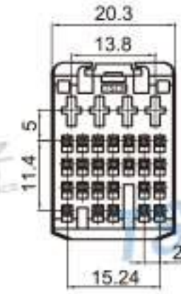
Type: TS30217-30P-21-7 Material: PBT GF10% Matching Terminal: TSH019 / TSH092
