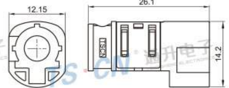
Type: TSVW10-04PM-AT-6BK-1 Material: PBT GF15% Matching Terminal: TSPM0175 / TSTM0051
