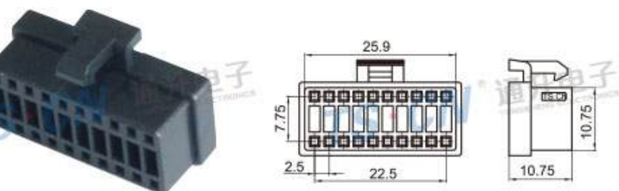
Type: TSALP20-20P-21 Material: PA66 GF15% Matching Terminal: TSH030
