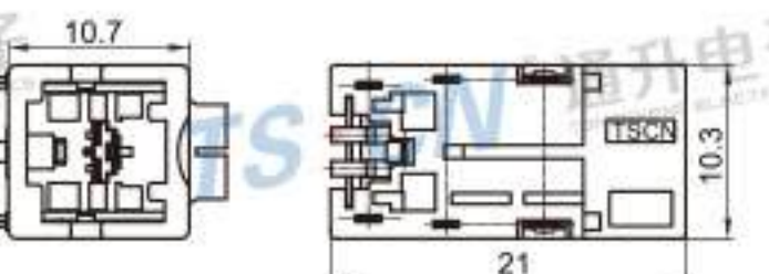
Type: TS30211-02PM-PKB-2 Material: PBT GF15% Matching Terminal: TSPM0266~TSPM0269
