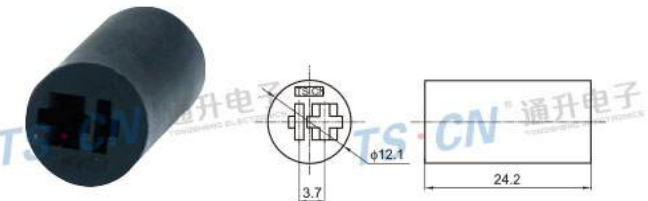
Type: TSLB09-02P-21 Material: PA66 Matching Terminal: TSH029
