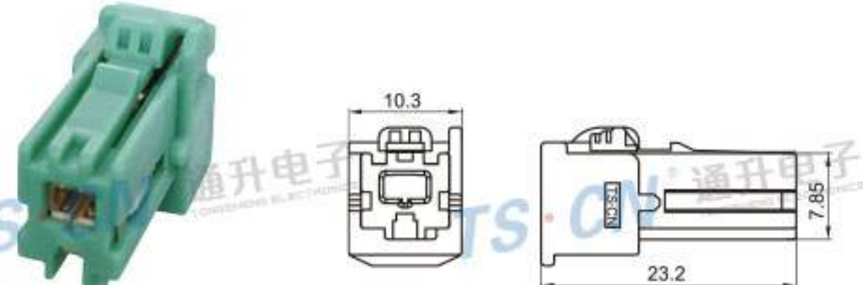
Type: TS30211-02PF-AT-2 Material: PBT Matching Terminal: TSTF0058 / TSTF0059 / TSTF0006
