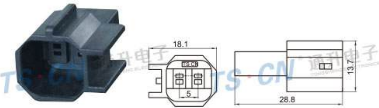
Type: TSLB38-02P-11 Material: PA66 GF15% Matching Terminal: TSZ040B
