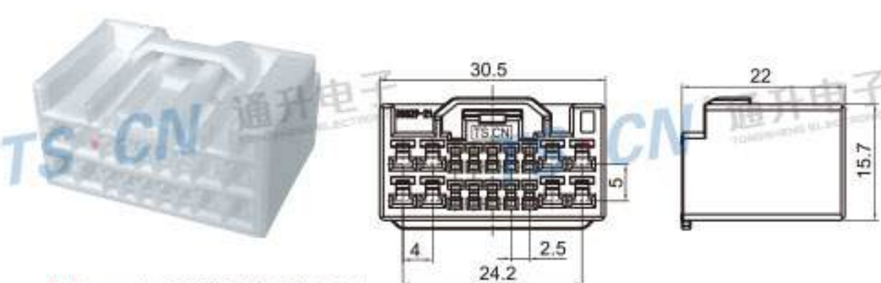
Type: TS30329-18P-21 Material: PBT Matching Terminal: TSH009 / TSH006
