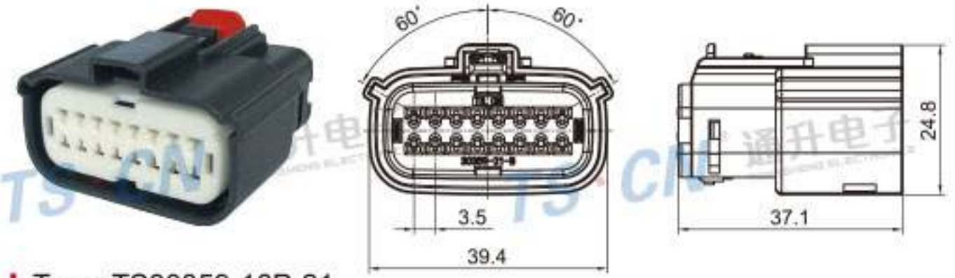
Type: TS30359-16P-21 Material: PA66 GF30% Matching Terminal: TSH047
