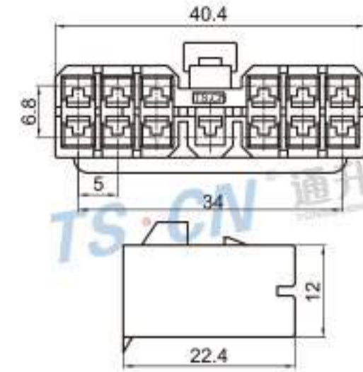
Type: TS1782-13P-21 Material: PA66 Matching Terminal: TSH017
