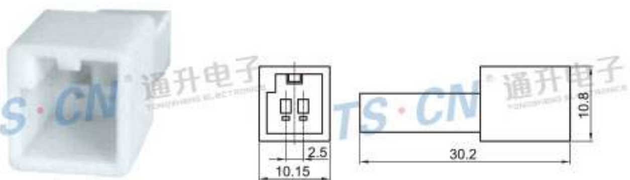
Type: TS30110-02P-11 Material: PBT Matching Terminal: TSZ145
