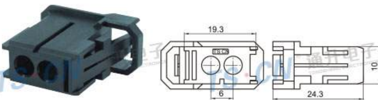
Type: TSBMGQ-02P-21 Material: PA66 Matching Terminal: NIL
