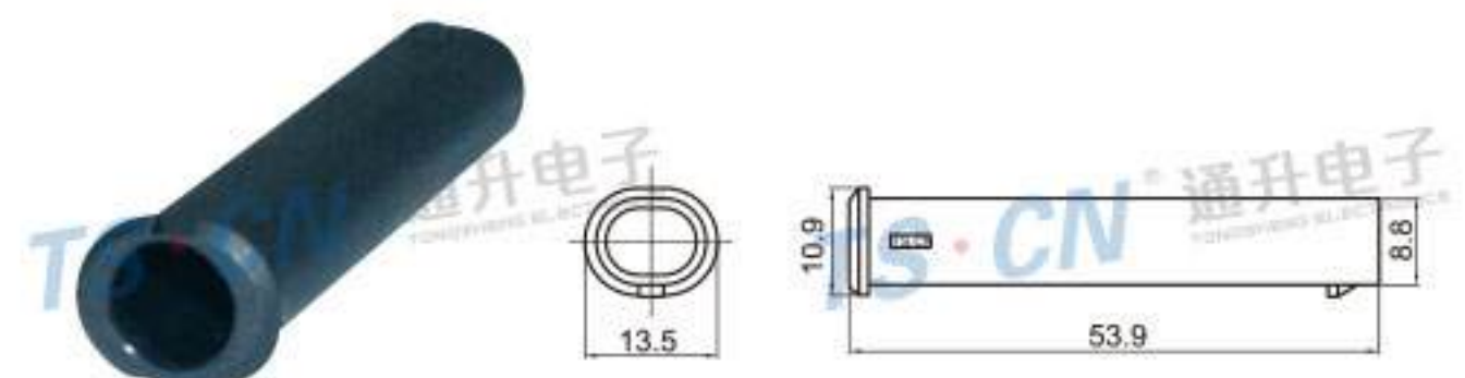
Type: TS30006-02P-11 Material: PA66 Matching Terminal: NIL
