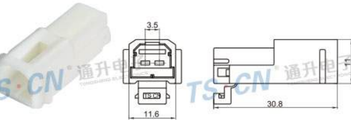
Type: TSLB27-02P-11 Material: PA66 Matching Terminal: TSZ011
