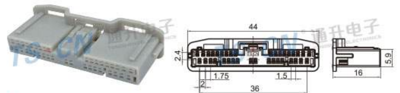
Type: TS30318-36P-21 Material: PA66 Matching Terminal: TSH600A
