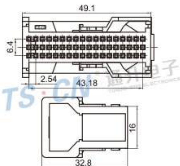
Type: TSAD54-54P-21 Material: PA66 GF15% Matching Terminal: TSHY66
