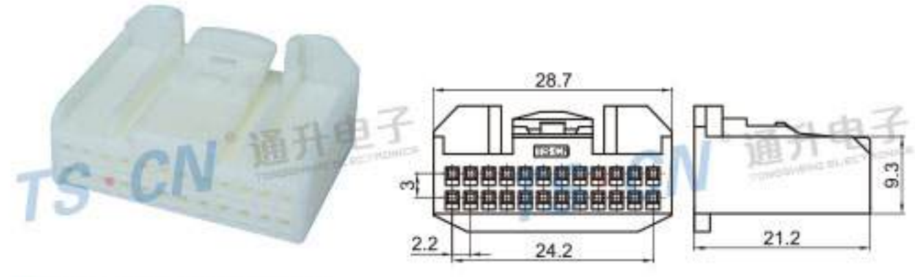
Type: TSTA24-24P-21 Material: PA66 Matching Terminal: TSH143
