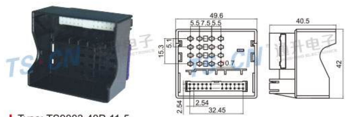
Type: TS9003-40P-11-5 Material: PA66 GF30% Matching Terminal: TSZ024B / TSZ208B
