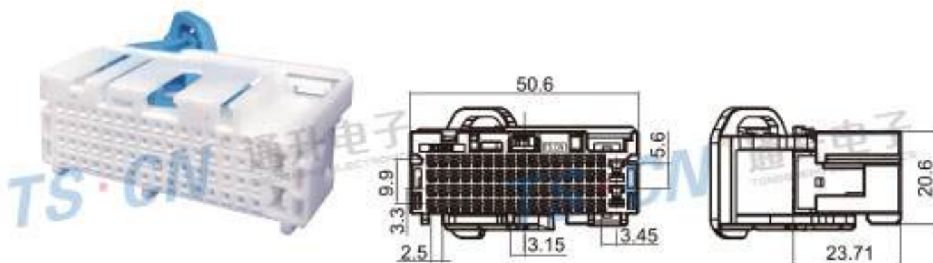
Type: TS30283-66P-21-2 Material: PBT Matching Terminal: TSH064 / TSH092
