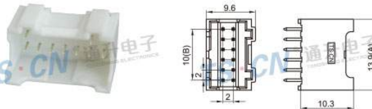
Type: TSPHS-14PM-PKB(10P-24P) Material: PBT GF15% Matching Terminal: TSPM0196 / TSPM0197
