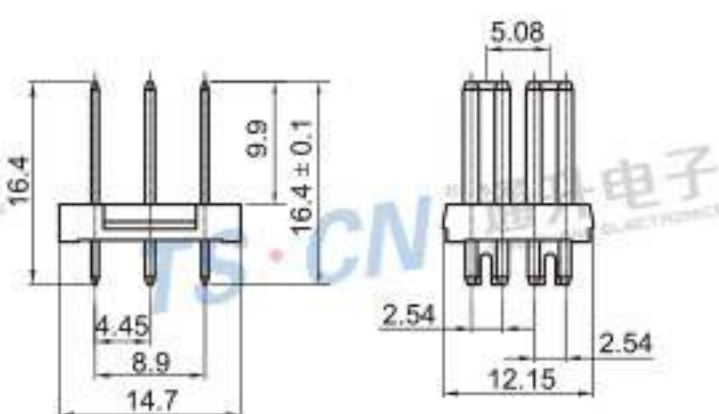
Type: TS30141-10PM-PKS Material: PBT GF15% Matching Terminal: TSPM0244 / TSPM0245
