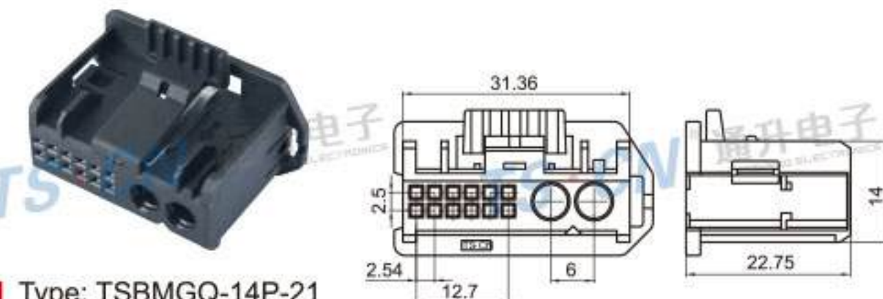
Type: TSBMGQ-14P-21 Material: PA66 GF30% Matching Terminal: TSH092
