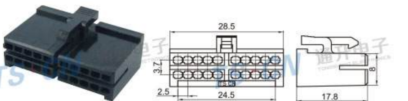
Type: TSJEN-20P-21 Material: PA66 GF15% Matching Terminal: TSH060
