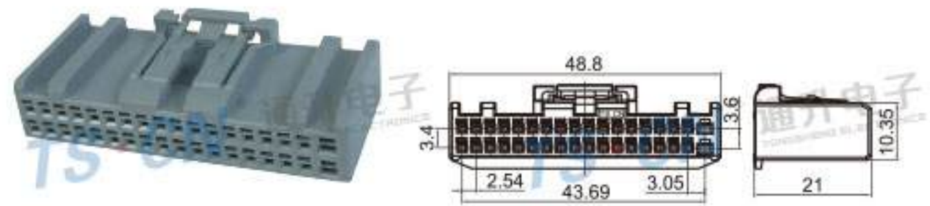
Type: TS30285-36P-21 Material: PBT GF15% Matching Terminal: TSH593 / TSH624
