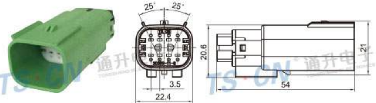
Type: TS30359-08P-11-3 Material: PA66 GF30% Matching Terminal: TSZ144A
