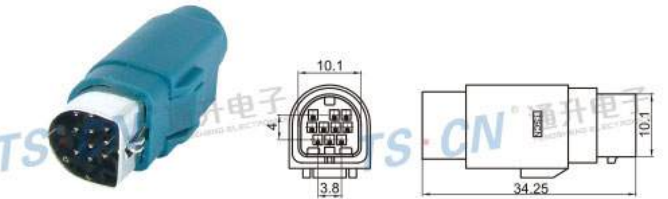
Type: TSALPH-10PM-AH Material: PA66 Matching Terminal: TSAM0014 / TSAM0015 / TS0079
