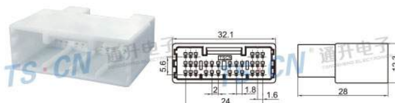
Type: TS30101-30P-11-3 Material: PA66 Matching Terminal: TSZ556
