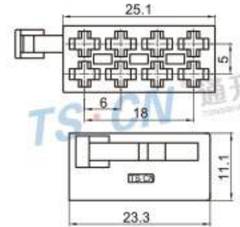
Type: TS1784A-08P-21-4BK Material: PA66 Matching Terminal: TSH019
