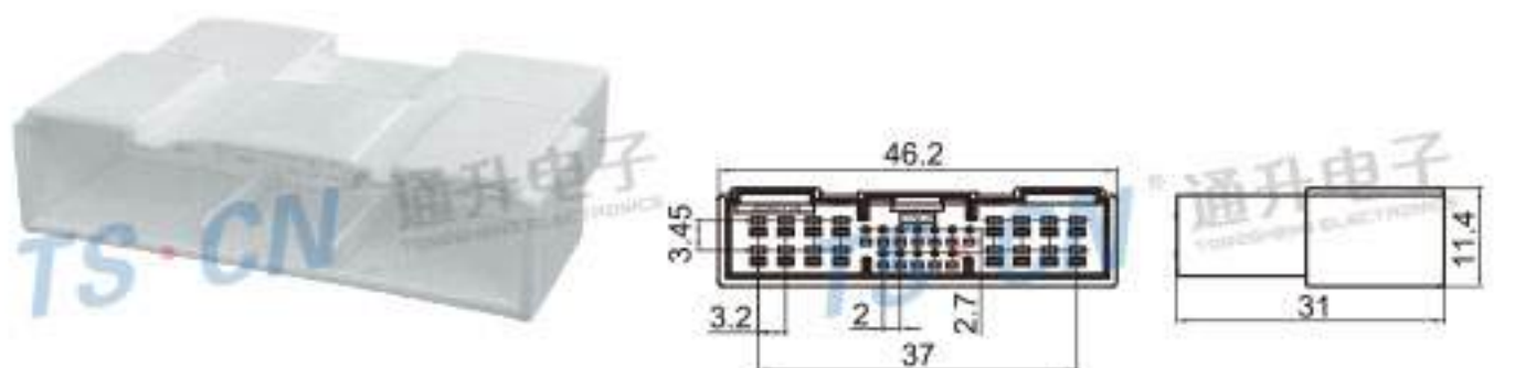
Type: TS30243-28P-11-8WT Material: PBT Matching Terminal: TSZ040 / TSZ561
