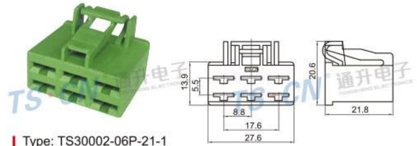
Type: TS30002-06P-21-1 Material: PBT Matching Terminal: TSH033A
