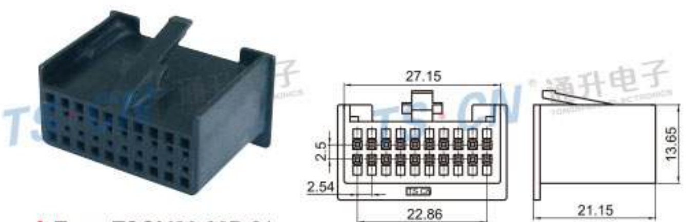
Type: TSGM20-20P-21 Material: PA66 GF30% Matching Terminal: TSH143
