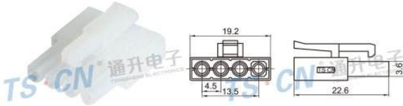
Type: TSOTP-04P-21 Material: PA66 Matching Terminal: NIL
