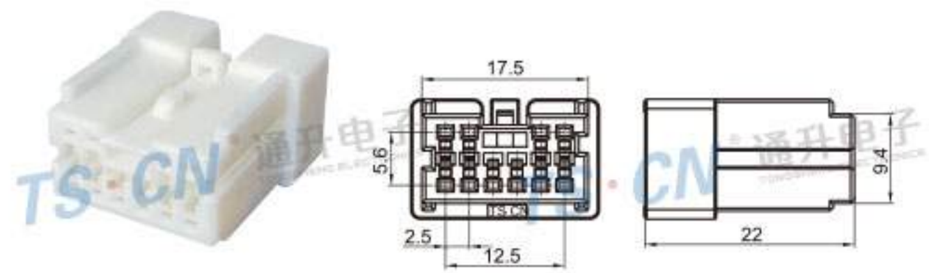
Type: TSNI10-10P-21-1 Material: PA66 Matching Terminal: TSH076
