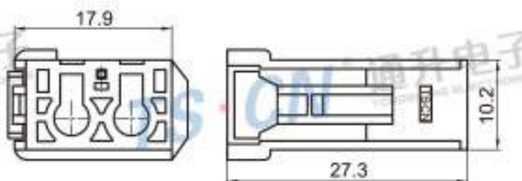
Type: TSLX21-03PF-AT Material: PA66 Matching Terminal: TSH143 / TSTF0003 / TSTF0004
