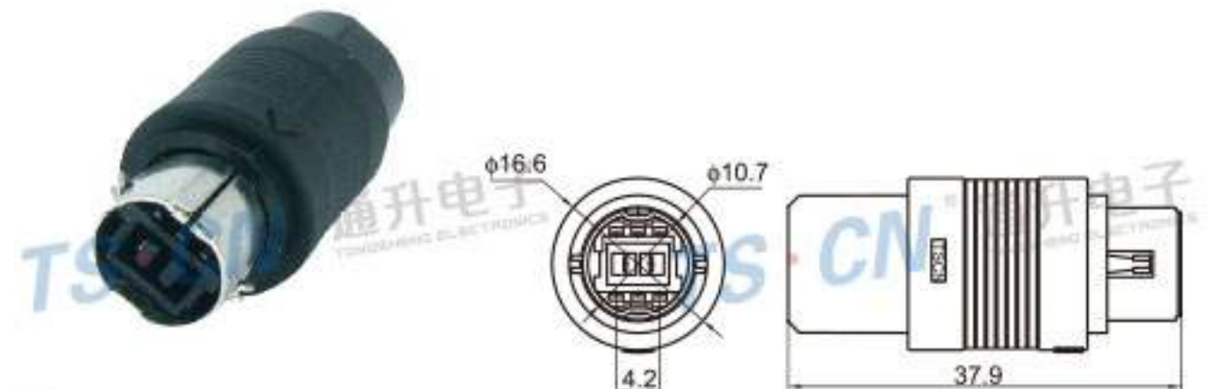
Type: TSSONY-08PF-AH-1 Material: PA66 GF30% Matching Terminal: TSAF0001 / TSH042 / TSH041
