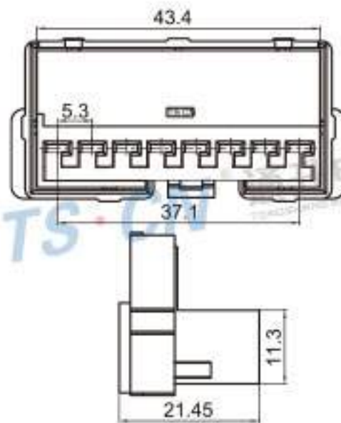
Type: TS1770-08P-21BK Material: ABS Matching Terminal: TSH007
