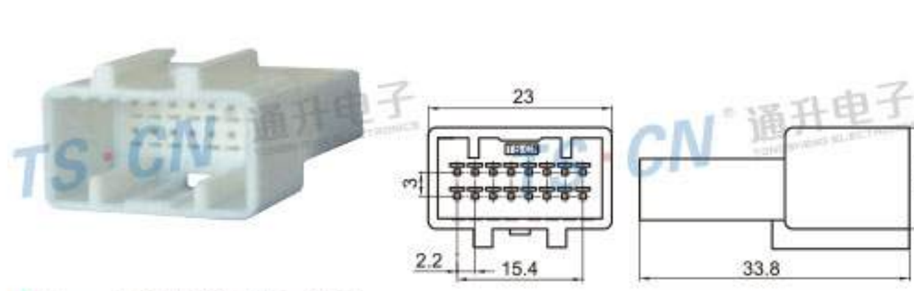
Type: TSTA16-16P-11-2 Material: PA66 Matching Terminal: TSZ208
