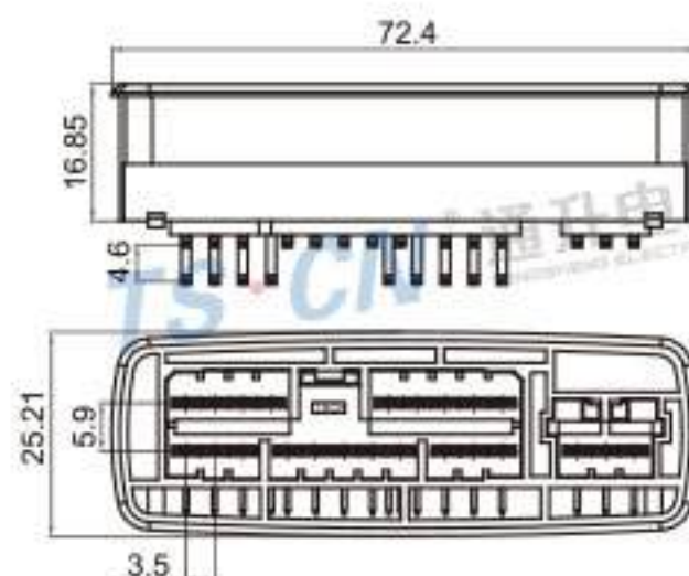
Type: TS8113-20PM-PKB Material: PA66 Matching Terminal: TSPM0001~TSPM0004
