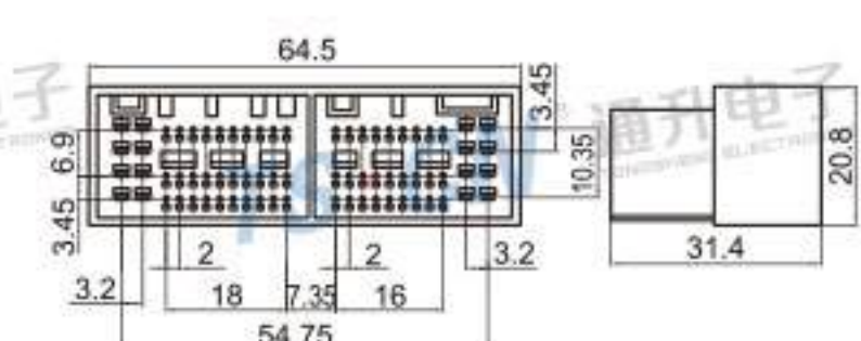
Type: TS30116-73P-11 Material: PA66 Matching Terminal: TSZ562 / TSZ561
