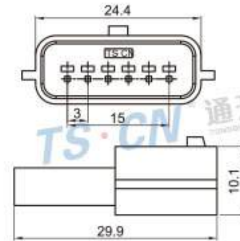
Type: TSNI06-06P-11-1 Material: PA66 GF30% Matching Terminal: TSZ208
