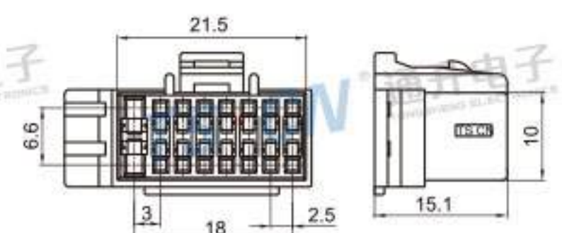
Type: TSSY16-16P-21 Material: PA66 GF30% Matching Terminal: TSH114 / TSH113
