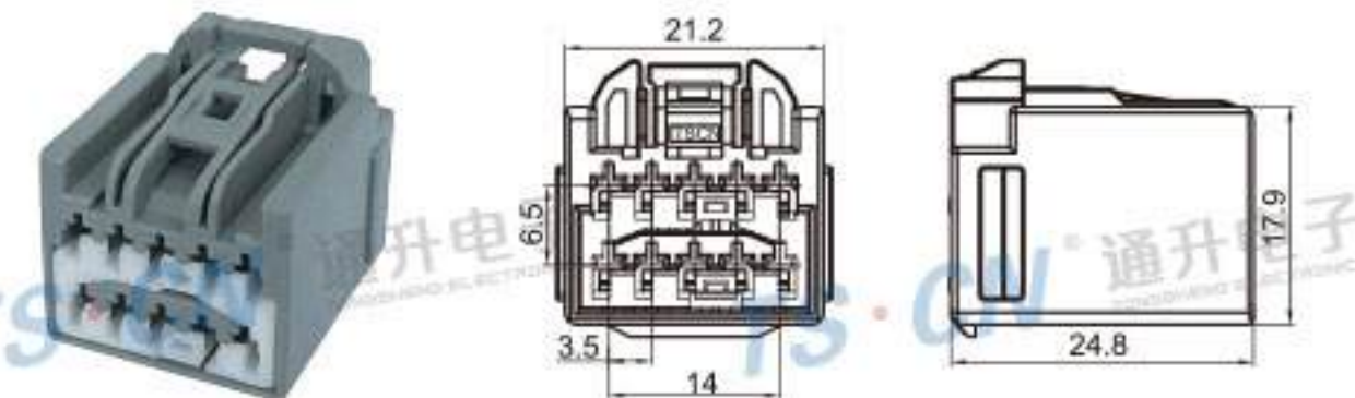
Type: TS30335-10P-21 Material: PBT GF15% Matching Terminal: TSH047
