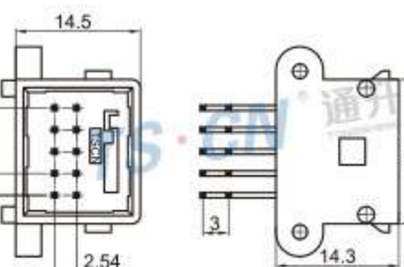
Type: TSROWE-10PM-PKB Material: PA66 Matching Terminal: TSPM0040 / TSPM0147
