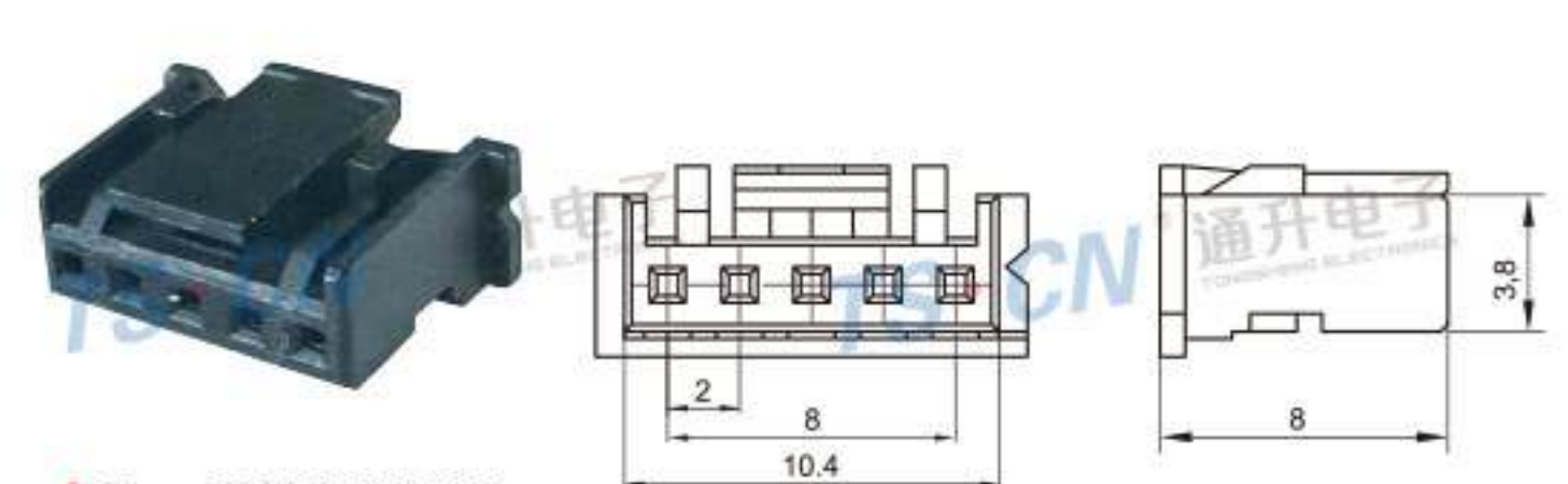
Type: TSPA-05P-21 Material: PA66 Matching Terminal: TSPA
