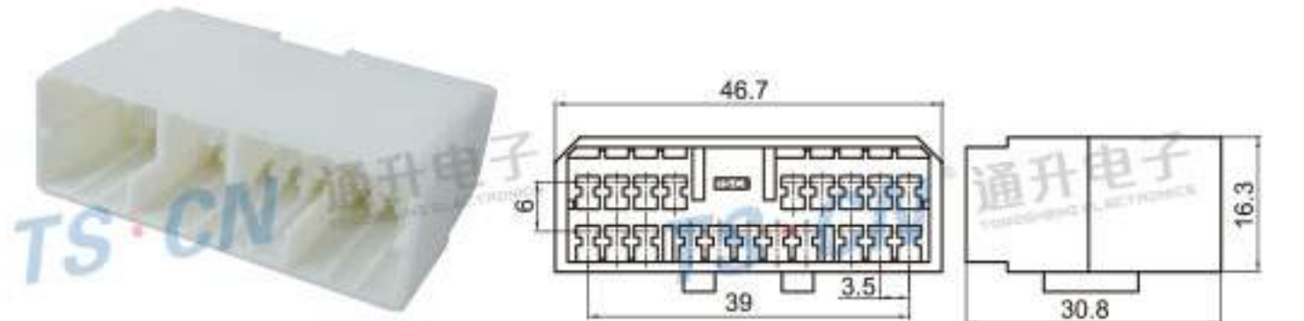
Type: TSDA20-20P-11 Material: PA66 Matching Terminal: TSZ011
