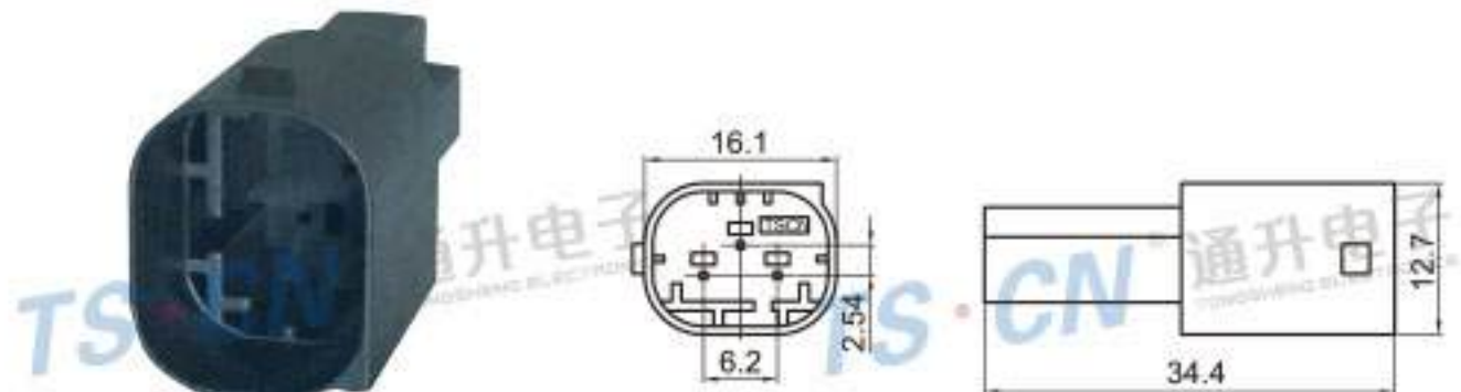
Type: TS30119-03P-11 Material: PA66 GF30% Matching Terminal: TSZ208
