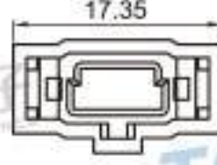
Type: TS1056-MINIUSB-21 Material: PA66 GF15% Matching Terminal: TSMINIUSB-F
