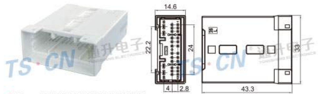
Type: TS30101-28PM-PKS-5 Material: PBT GF15% Matching Terminal: TSPM0331 / TSPM0305
