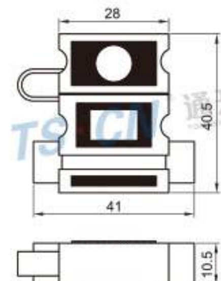
Type: TS BX12 Material: PBT Matching Terminal: TS7522-BS-2
