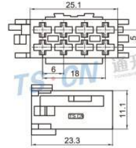
Type: TS1784A-08P-21-3BK Material: PA66 Matching Terminal: TSH019
