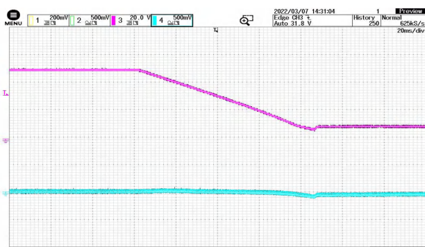
Figure 10 50V-9V Input Jump @ 10% Load CH3: VIN CH4: Vout
