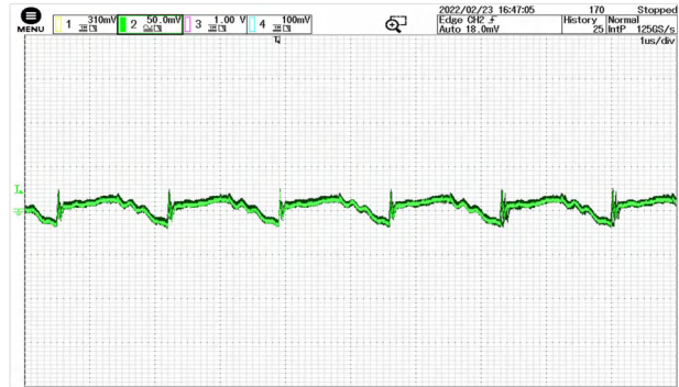
Figure 7 Output voltage ripple @ VIN=30V at full load
