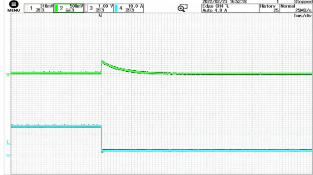
Figure 9 90% load -10% load jump @ VIN=30V CH2: Vout CH4: Io
