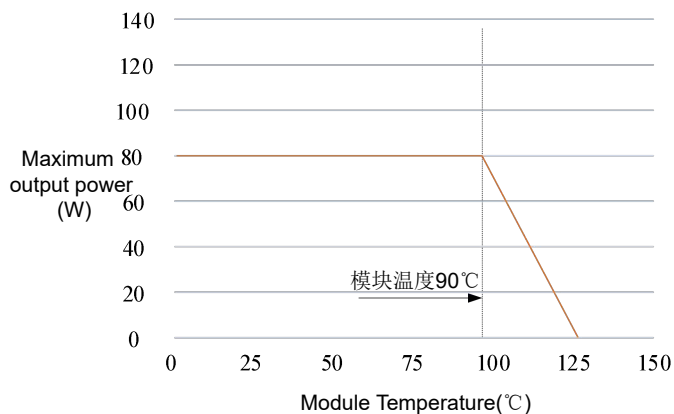
Figure 2 Loss Curve
