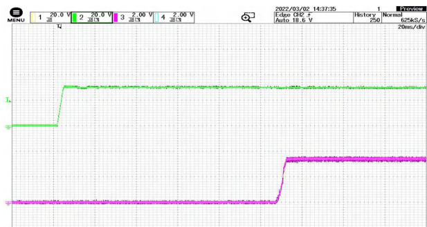
Figure 12 Output Downregulation CH2:VIN CH3:Vout Start Waveform @ VIN=30V
