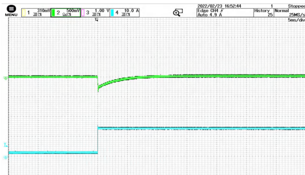
Figure 8 10% load -90% load jump @ VIN=30V CH2: Vout CH4: Io
