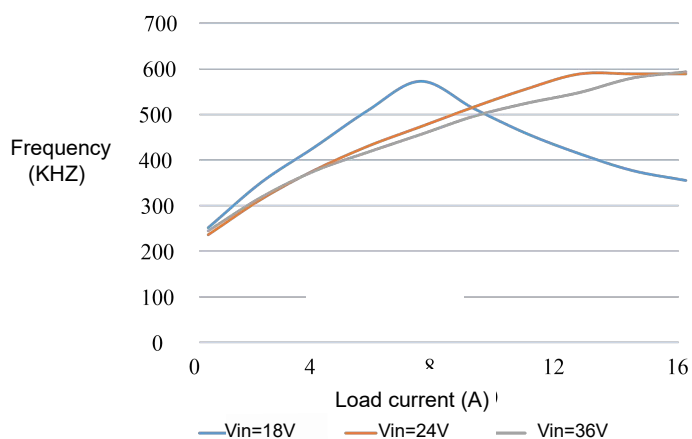
Figure 3 Frequency Curve
