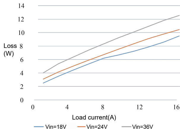
Figure 2 Loss Curve
