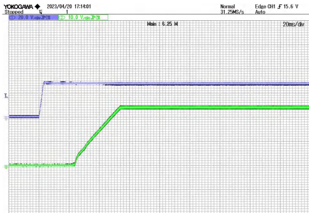
Figure 6 Start Waveform @ VIN=28V CH1: VIN CH2: Vout
