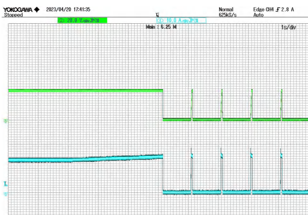
Figure 15 Overcurrent protection CH2: V out CH4:I out @ VIN=28V
