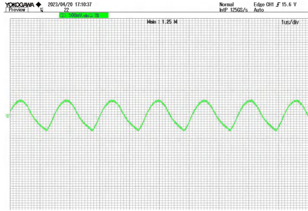
Figure 7 Output voltage ripple @ VIN=28V at full load
