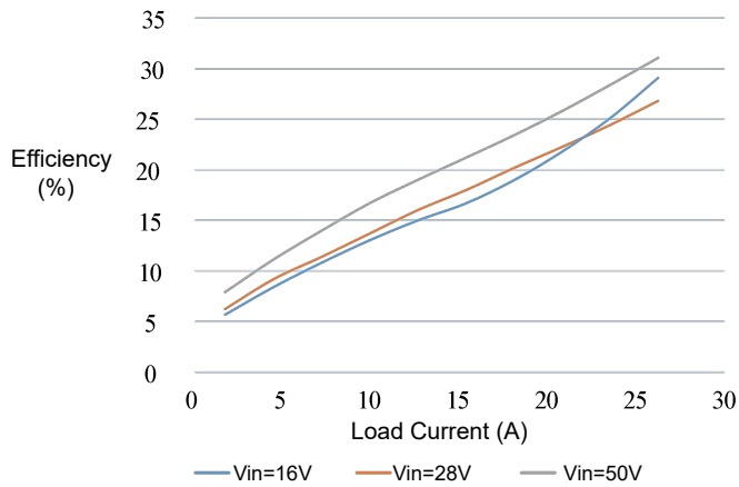
Figure 1 Efficiency Curve
