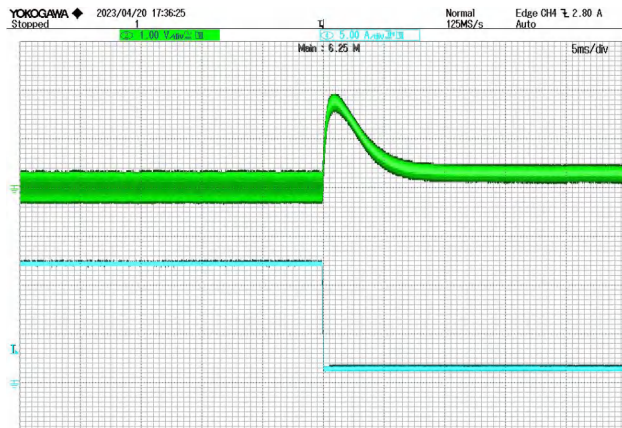
Figure 8 90% load -10% load jump @ VIN=28V CH2: Vout CH4: Io
