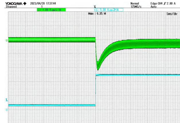
Figure 9 10% load -90% load jump @ VIN=28V CH2: Vout CH4: Io
