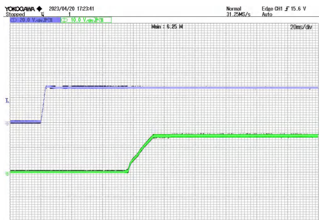
Figure 12 Output Downregulation CH1:V IN CH2:V out Start Waveform @ VIN=28V
