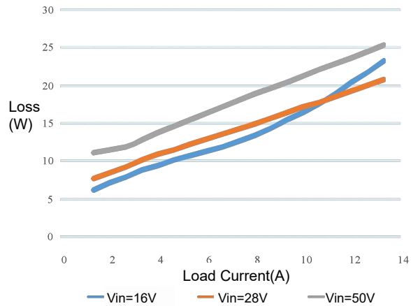
Figure 2 Loss Curve
