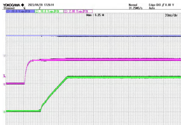
Figure 14 Start waveform CH2:V IN CH3:V out CH4:EN (enabled) @ VIN=28V
