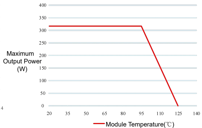
Figure 4 Temperature Derating Curve
