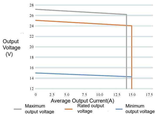
Figure 5 Safe Work Area
