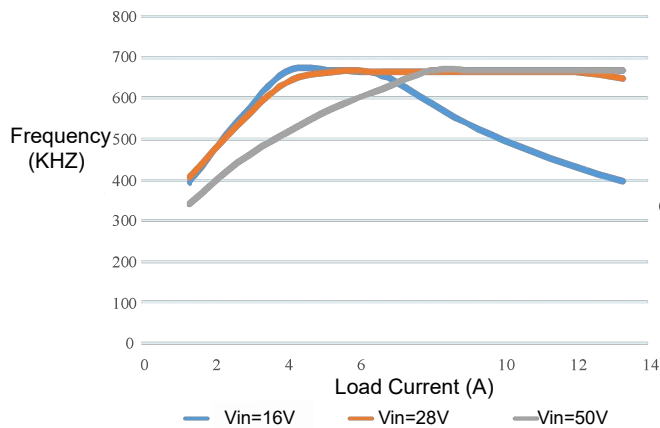
Figure 3 Frequency Curve
