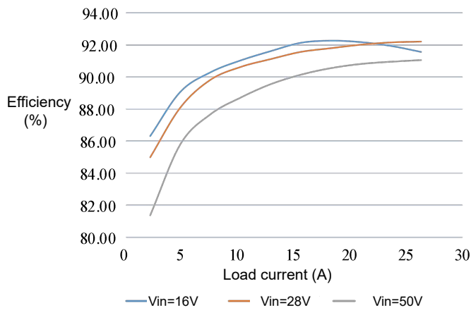
Figure 1 Efficiency curve
