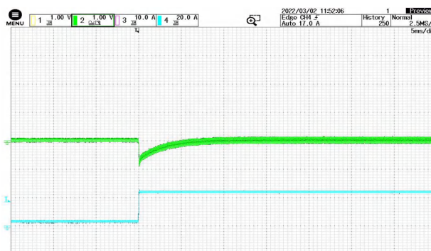
Figure 9 10% load -90% load jump @ VIN=28V CH2: Vout CH4: Io
