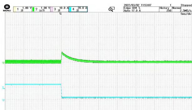
Figure 8 90% load -10% load jump @ VIN=28V CH2: Vout CH4: Io
