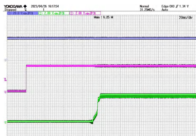
Figure 14 Start waveform CH2:VIN CH2:EN CH3:Vout (enabled) @ VIN=28V
