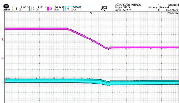
Figure 10 50V-16V Input Jump @ 10% Load CH3: VIN CH4: Vout
