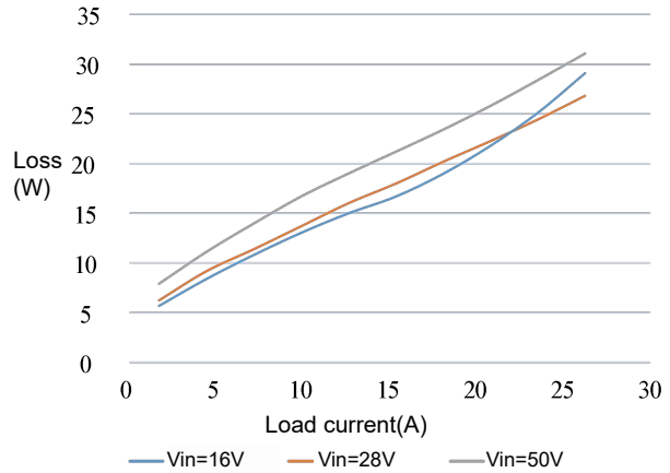
Figure 2 Loss Curve
