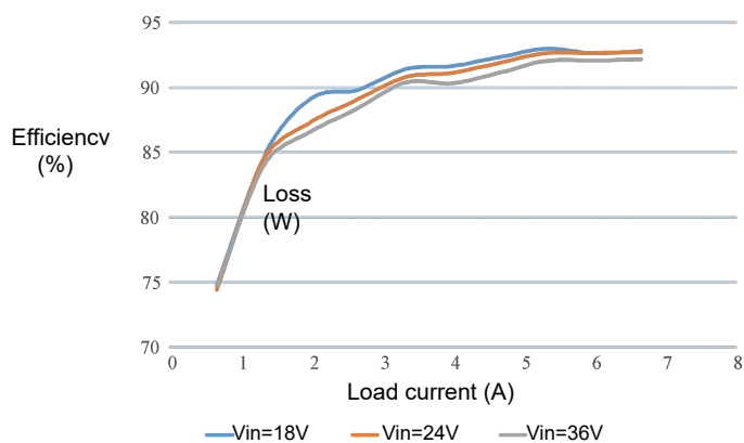
Figure 1 Efficiency curve
