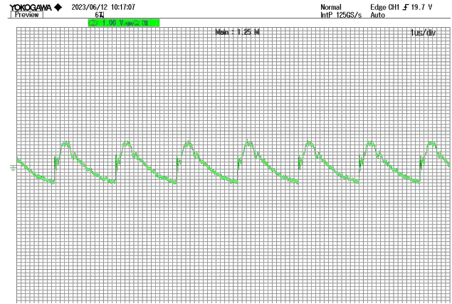
Figure 7 Output voltage ripple @ VIN=24V at full load
