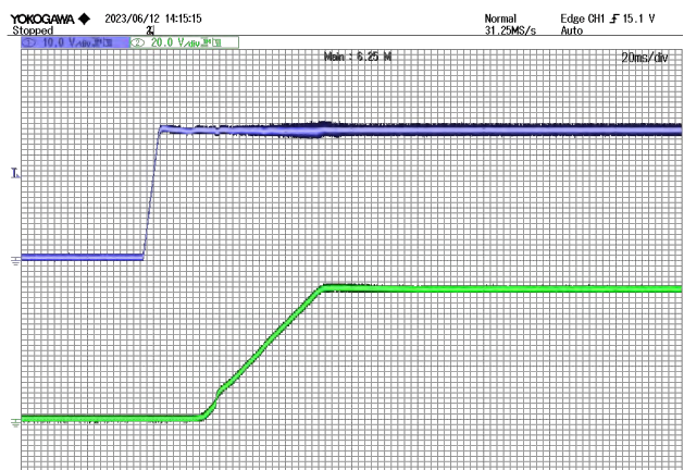
Figure 13 Output Upregulation CH1:VIN CH2:Vout Start Waveform @ VIN=24V
