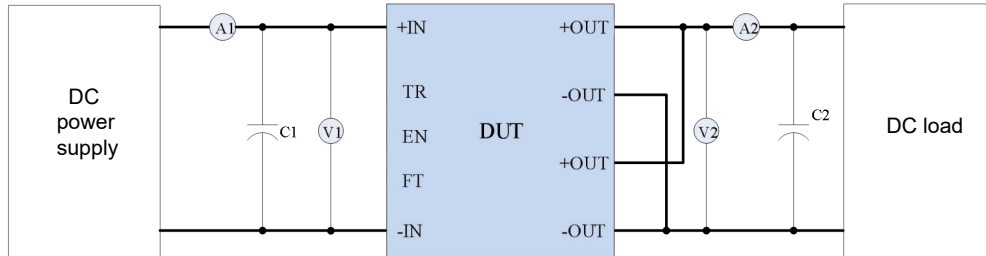
Figure 1 Electrical Test Circuit Connection Diagram
