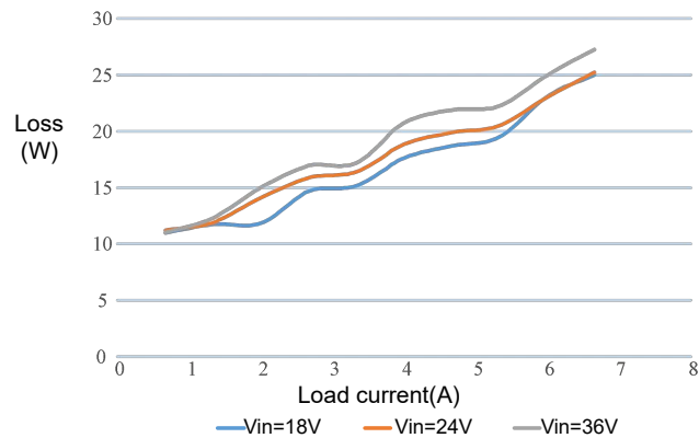
Figure 2 Loss Curve
