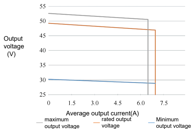
Figure 5 Safe Work Area
