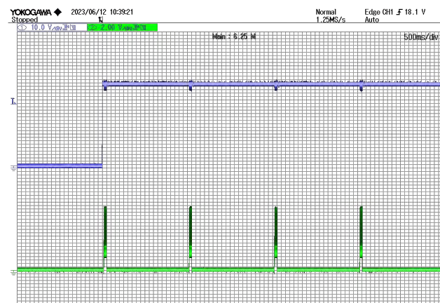
Figure 14 Short circuit startup waveform (enable) @ VIN=24V
