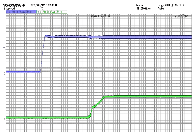
Figure 12 Output Downregulation CH1:VIN CH2:Vout Start Waveform @ VIN=24V
