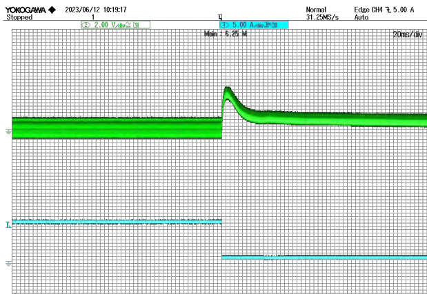
Figure 8 90% load -10% load jump @ VIN=24V CH2: Vout CH4: Io
