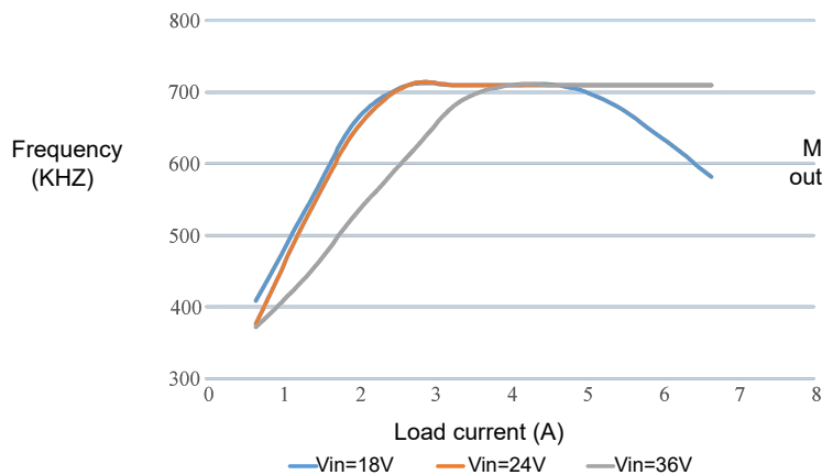
Figure 3 Frequency Curve
