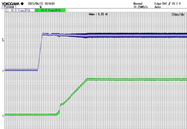
Figure 6 Start waveform @ VIN=24V CH1: VIN CH2: Vout
