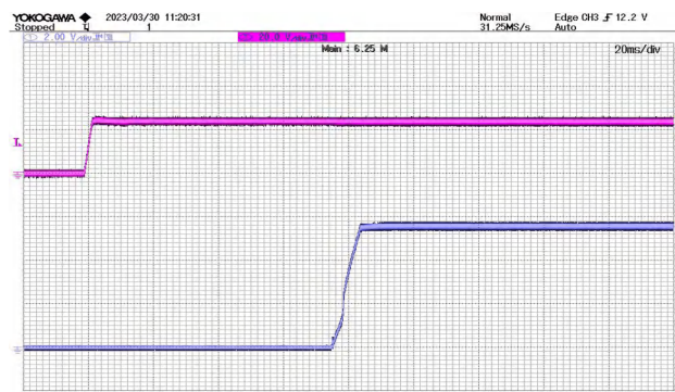
Figure 13 Output Upregulation CH3:VIN CH1:Vout Start Waveform @ VIN=24V
