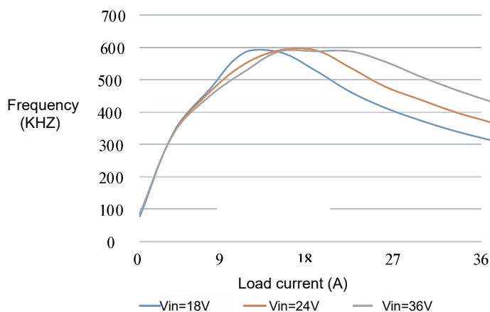
Figure 3 Frequency Curve
