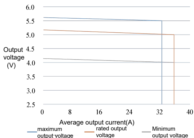
Figure 5 Safe Work Area
