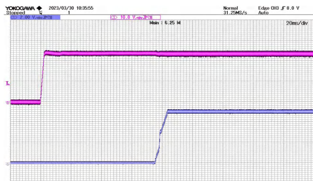
Figure 6 Start waveform @ VIN=24V CH3: VIN CH1: Vout
