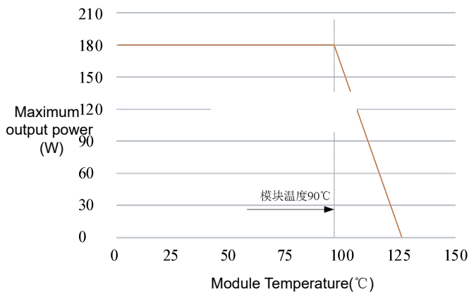
Figure 2 Loss Curve
