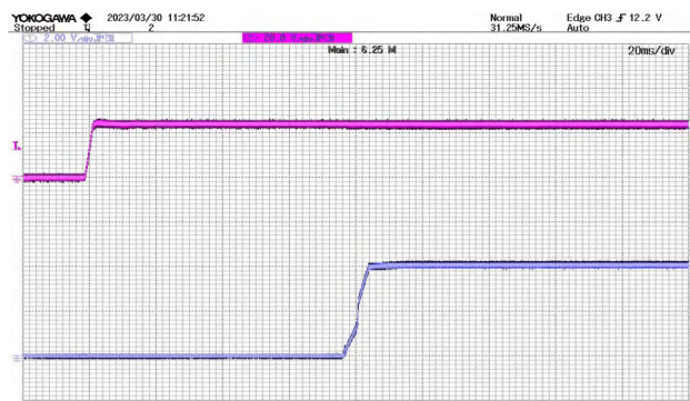
Figure 12 Output Downregulation CH3:VIN CH1:Vout Start Waveform @ VIN=24V
