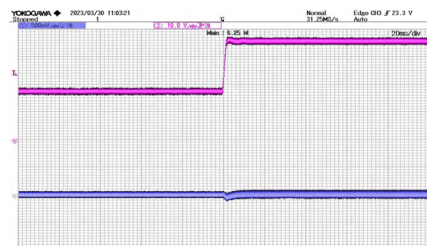
Figure 11 18V-36V Input Jump @ 10% Load CH3: VIN CH1: Vout
