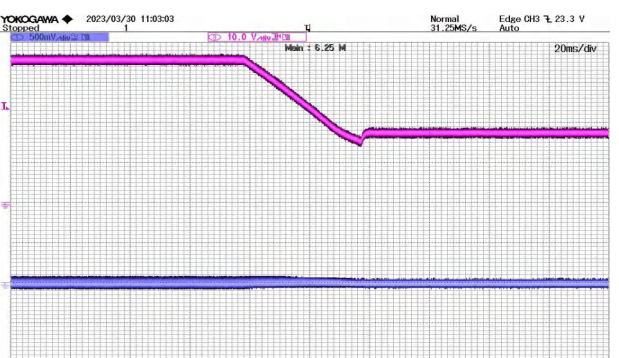
Figure 10 36V-18V Input Jump @ 10% Load CH3: VIN CH1: Vout
