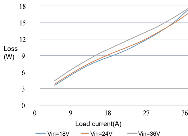
Figure 2 Loss Curve
