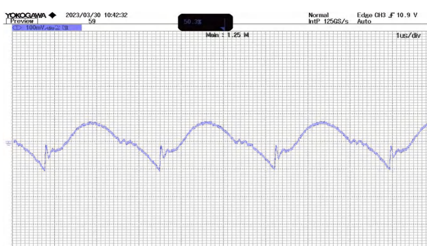
Figure 7 Output voltage ripple @ VIN=24V at full load
