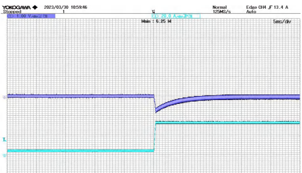
Figure 8 10% load -90% load jump @ VIN=24V CH1: Vout CH4: Io
