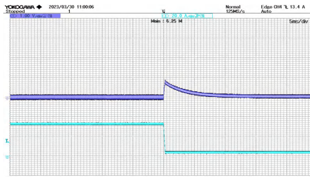
Figure 9 90% load -10% load jump @ VIN=24V CH1: Vout CH4: Io
