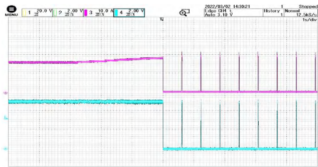
Figure 15 Overcurrent CH3: Iout CH4:Vout protection @ VIN=24V
