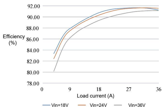
Figure 1 Efficiency curve
