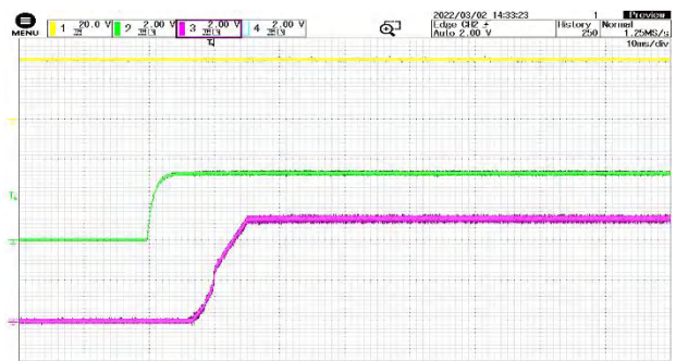
Figure 14 Start waveform CH1:VIN CH2:EN CH3:Vout (enabled) @ VIN=24V
