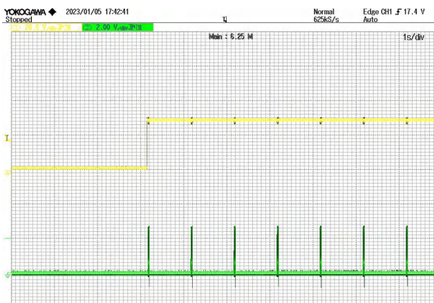
Figure 14 Start waveform CH3: V_{IN} (enabled) @ V_{IN}=28V
