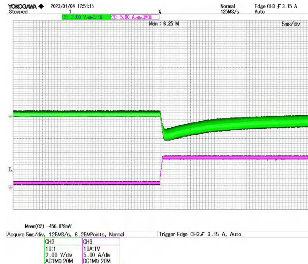
Figure 9 10% load -90% load jump @ VIN=28V CH2: Vout CH3: Io
