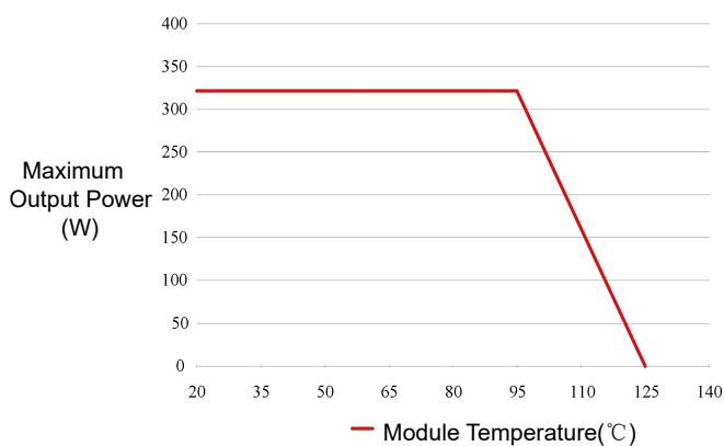
Figure 4 Temperature Derating Curve
