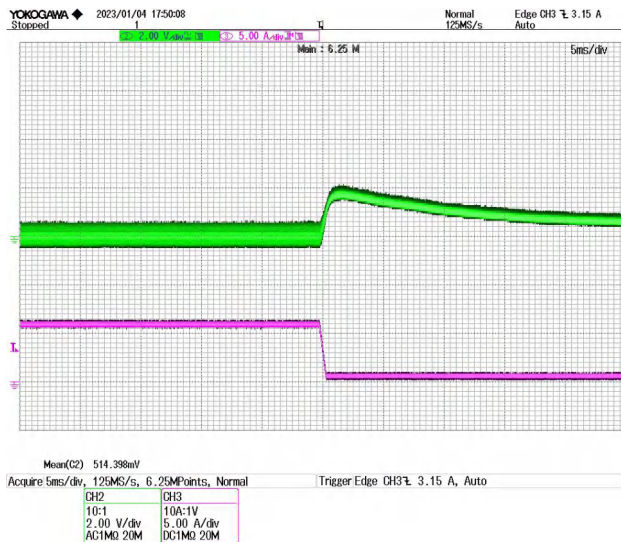
Figure 8 90% load -10% load jump @ VIN=28V CH2: Vout CH3: Io
