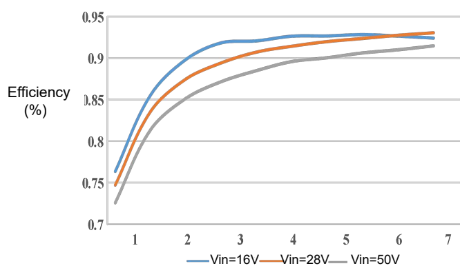
Figure 1 Efficiency Curve
