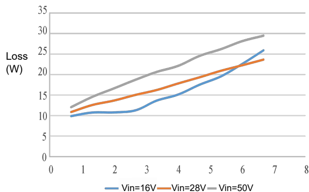
Figure 2 Loss Curve
