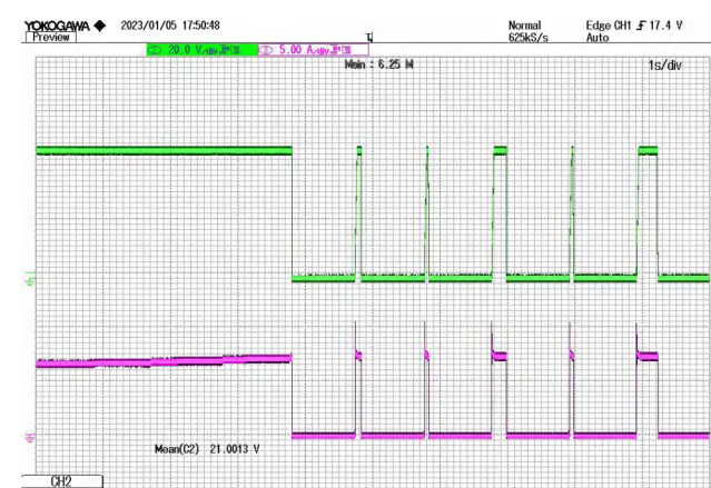
Figure 15 Overcurrent protection CH2: V_{out} CH4: I_{out} @ V_{IN}=28V
