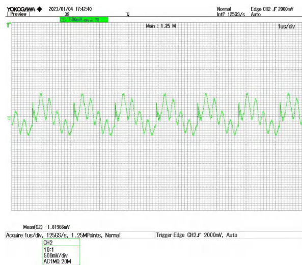
Figure 7 Output voltage ripple @ VIN=28V at full load
