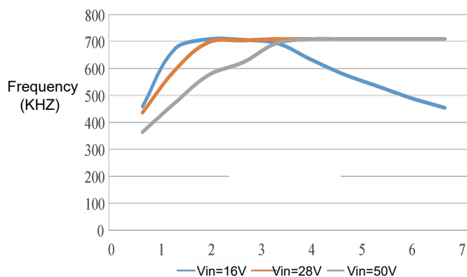
Figure 3 Frequency Curve
