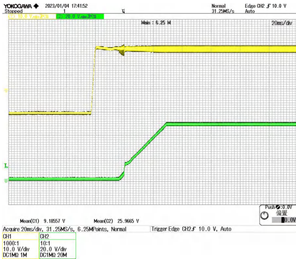
Figure 6 Start Waveform @ VIN=28V CH1: VIN CH2: Vout
