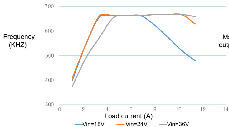
Figure 3 Frequency Curve
