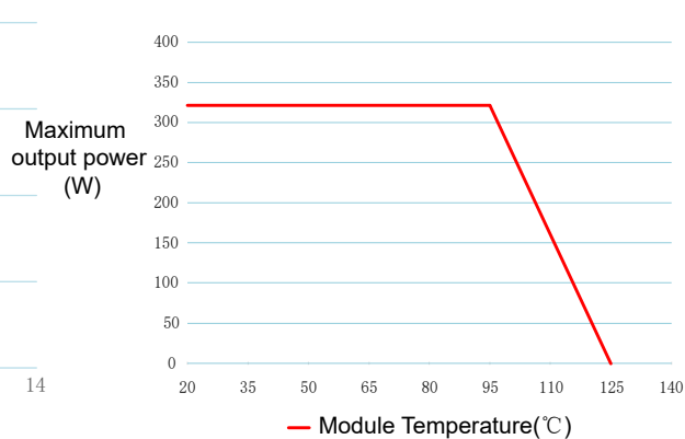
Figure 4 Temperature Derating Curve
