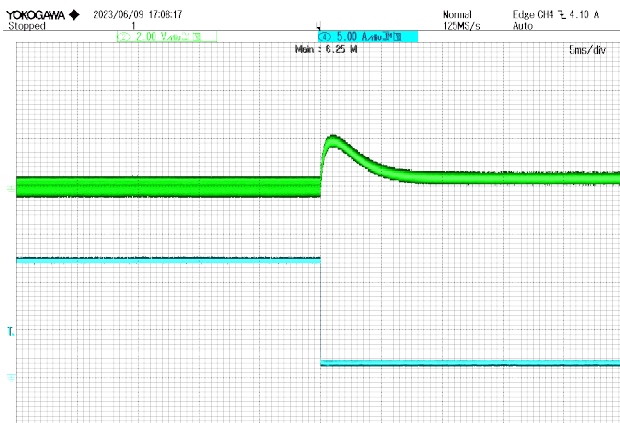
Figure 8 90% load -10% load jump @ VIN=24V CH2: V out CH4: I o
