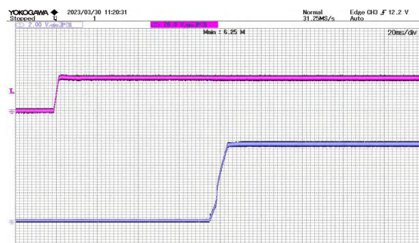
Figure 13 Output Upregulation Start Waveform @ VIN=24V CH1:VIN CH2:V out
