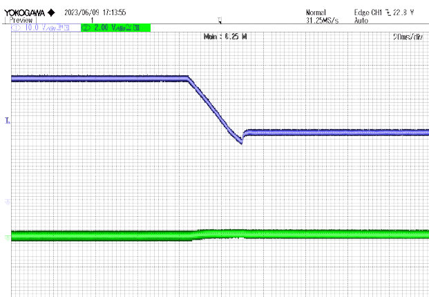
Figure 10 36V-18V Input Jump @ 10% Load CH1: V IN CH2: V out
