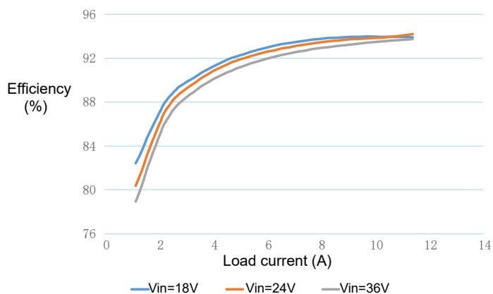
Figure 1 Efficiency curve
