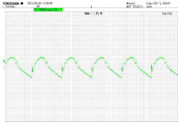
Figure 7 Output voltage ripple @ VIN=24V at full load
