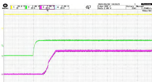
Figure 14 Start waveform (enabled) @ VIN=24V CH1:VIN CH2:V out CH3:EN
