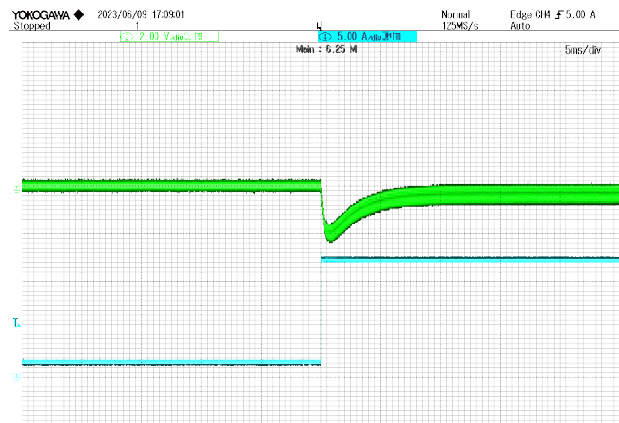
Figure 9 10% load -90% load jump @ VIN=24V CH2: V out CH4: I o
