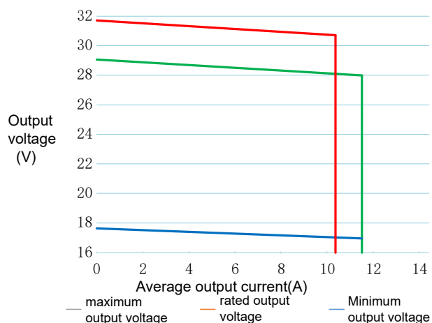
Figure 5 Safe Work Area
