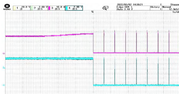
Figure 15 Overcurrent protection @ VIN=24V CH2: V out CH4:I out
