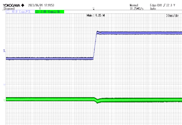
Figure 11 18V-36V Input Jump @ 10% Load CH1: V IN CH2: V out
