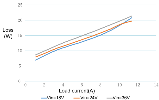
Figure 2 Loss Curve
