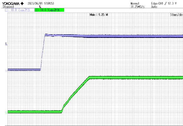
Figure 6 Start waveform @ VIN=24V CH1: V IN CH2: V out
