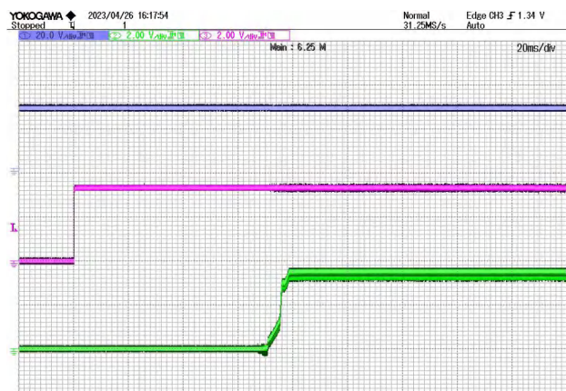
Figure 14 Start waveform CH1:VIN CH2: EN (enabled) @ VIN=28V
