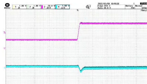
Figure 11 16V-50V Input Jump @ 10% Load CH3: V IN CH4: V out
