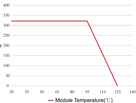
Figure 2 Loss Curve
