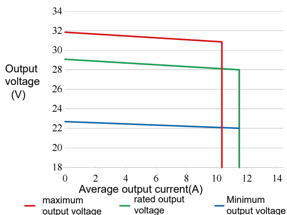
Figure 5 Safe Work Area
