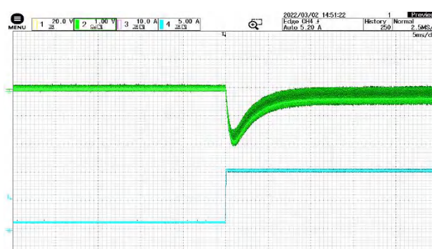
Figure 8 10% load -90% load jump @ VIN=28V CH2: V out CH4: I o
