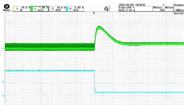
Figure 9 90% load -10% load jump @ VIN=28V CH2: V out CH4: I o
