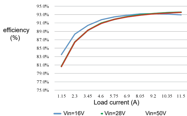
Figure 1 Efficiency curve
