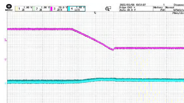
Figure 10 50V-16V Input Jump @ 10% Load CH3: V IN CH4: V out
