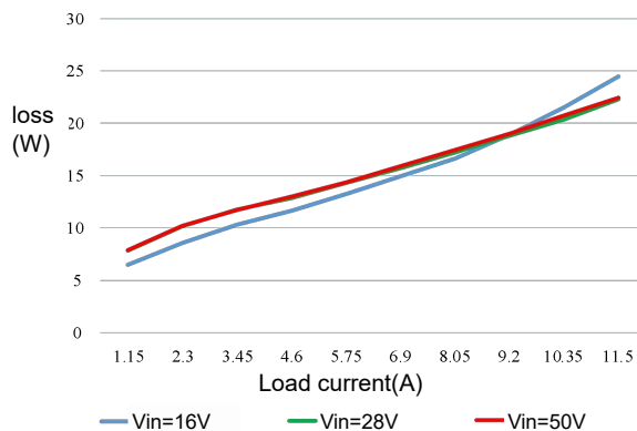
Figure 2 Loss Curve
