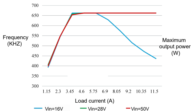
Figure 3 Frequency Curve
