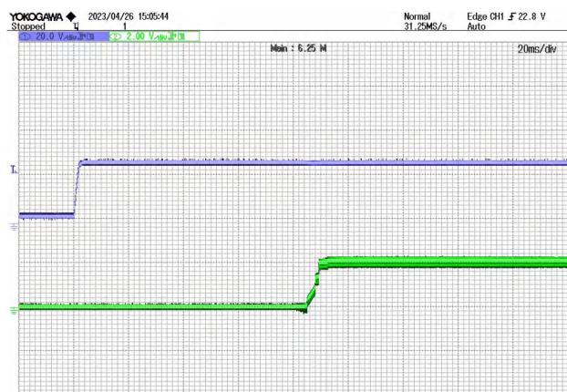
Figure 12 Output Downregulation CH2:VIN CH3:Vout Start Waveform @ VIN=28V
