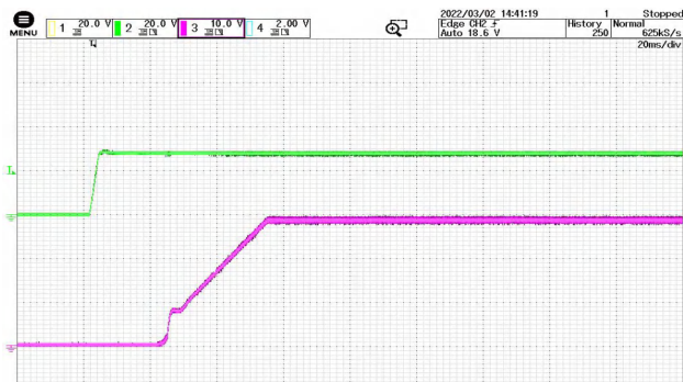
Figure 6 Start waveform @ VIN=28V CH2: VIN CH3: Vout
