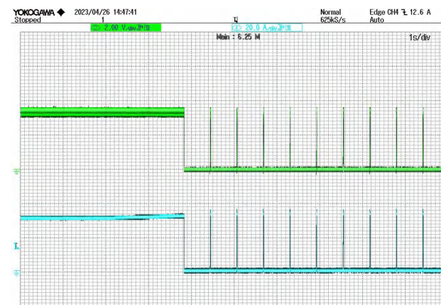
Figure 15 Overcurrent protection CH3: Iout CH4:Vout protection @ VIN=28V
