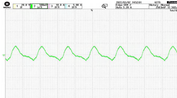
Figure 7 Output voltage ripple @ VIN=28V at full load
