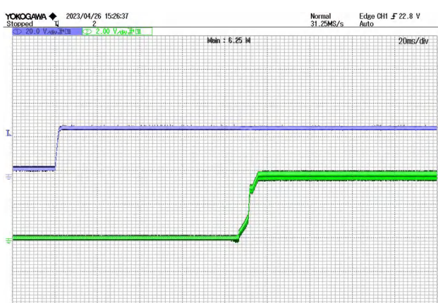
Figure 13 Output Upregulation CH2:VIN CH3:Vout Start Waveform @ VIN=28V
