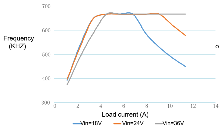
Figure 3 Frequency Curve
