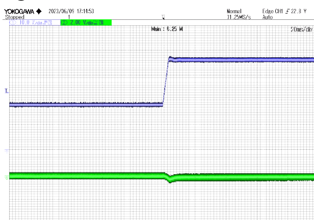
Figure 11 18V-36V Input Jump @ 10% Load CH1: VIN CH2: Vout
