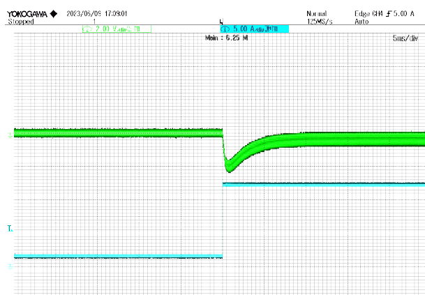
Figure 9 10% load -90% load jump @ VIN=24V CH2: Vout CH4: Io
