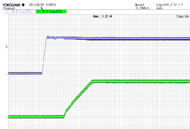
Figure 6 Start waveform @ VIN=24V CH1: VIN CH2: Vout
