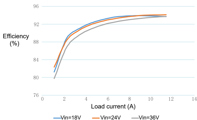
Figure 1 Efficiency curve
