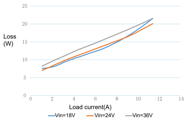
Figure 2 Loss Curve
