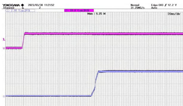
Figure 12 Output Downregulation Start Waveform @ VIN=24V CH1:VIN CH2:V out
