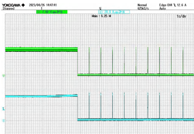
Figure 15 Overcurrent CH2: Vout CH4:Iout protection @ VIN=28V
