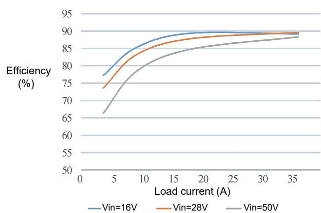
Figure 1 Efficiency curve
