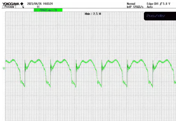
Figure 7 Output voltage ripple @ VIN=28V at full load
