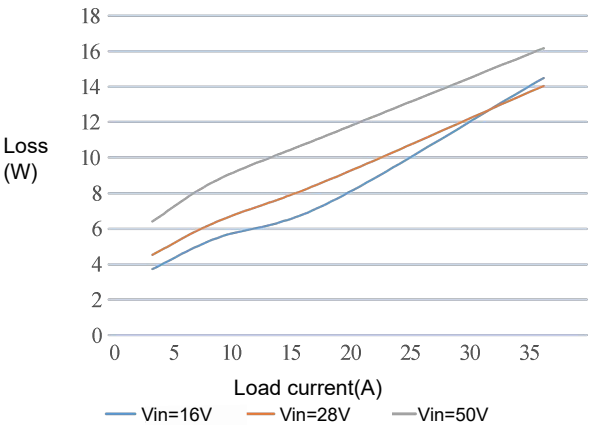
Figure 2 Loss Curve
