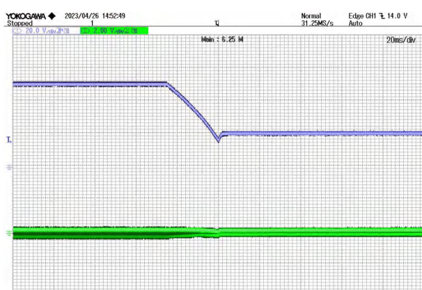
Figure 10 50V-16V Input Jump @ 10% Load CH1: VIN CH2: Vout
