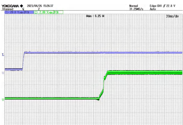
Figure 13 Output Upregulation CH1:VIN CH2:Vout Start Waveform @ VIN=28V
