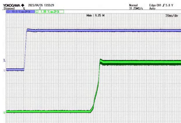
Figure 6 Start waveform @ VIN=28V CH1: VIN CH2: Vout
