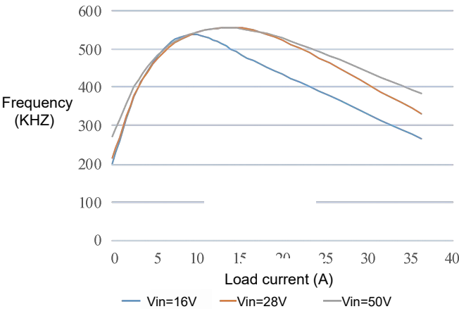
Figure 3 Frequency Curve
