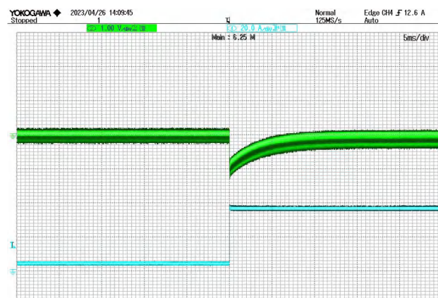
Figure 8 90% load -10% load jump @ VIN=28V CH2: Vout CH4: Io
