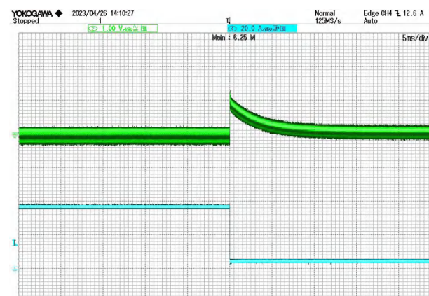
Figure 9 10% load -90% load jump @ VIN=28V CH2: Vout CH4: Io
