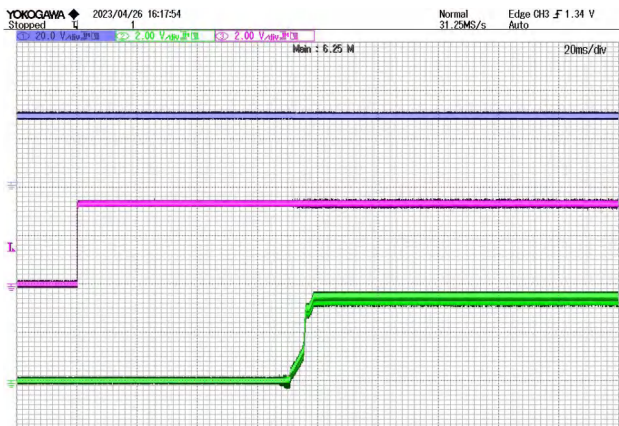
Figure 14 Start waveform CH1:VIN CH2:Vout CH3:EN (enabled) @ VIN=28V
