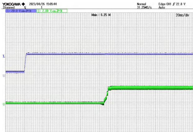
Figure 12 Output Downregulation CH1:VIN CH2:Vout Start Waveform @ VIN=28V
