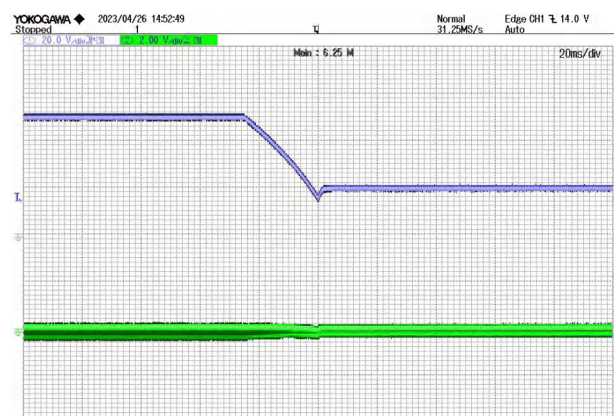
Figure 10 50V-16V Input Jump @ 10% Load CH1: VIN CH2: Vout
