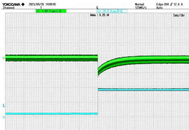
Figure 8 10% load -90% load jump @ VIN=28V CH2: Vout CH4: Io
