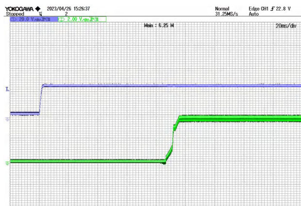
Figure 13 Output Upregulation Start Waveform @ VIN=28V CH1:V IN CH2:V out
