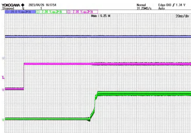
Figure 14 Start waveform (enabled) @ VIN=28V CH1:V IN CH3: EN CH2:V out
