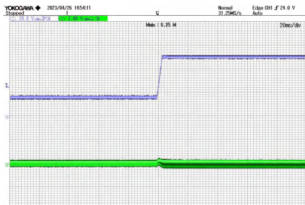
Figure 11 16V-50V Input Jump @ 10% Load CH1: VIN CH2: Vout
