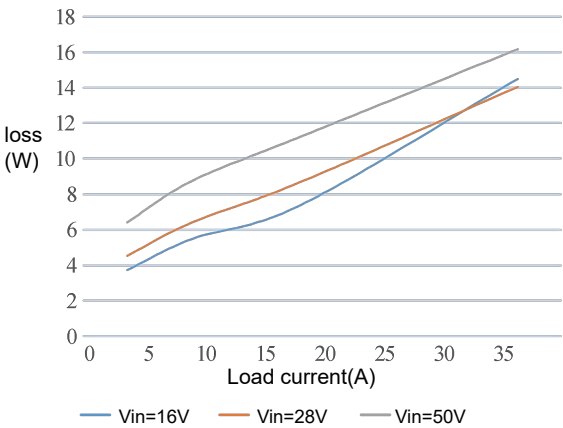
Figure 2 Loss Curve
