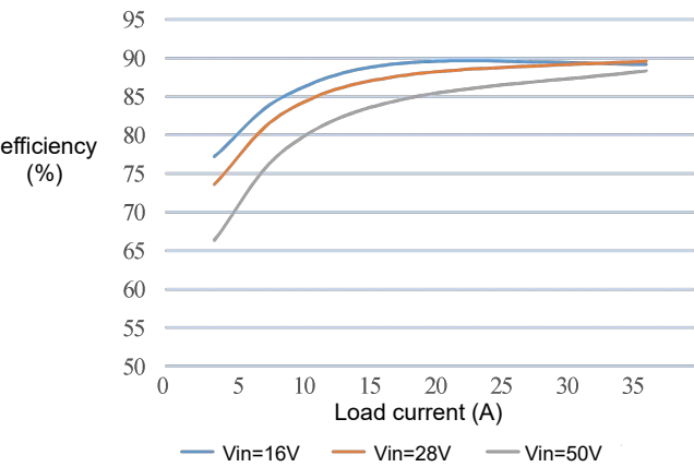
Figure 1 Efficiency curve
