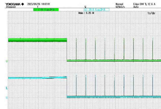
Figure 15 Overcurrent protection @ VIN=28V CH2: V out CH4: I out
