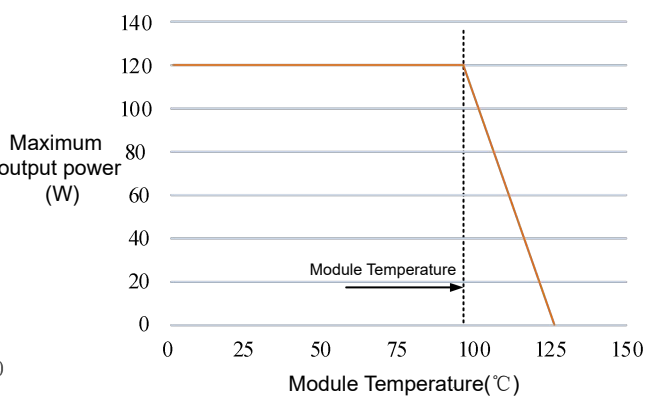
Figure 2 Loss Curve
