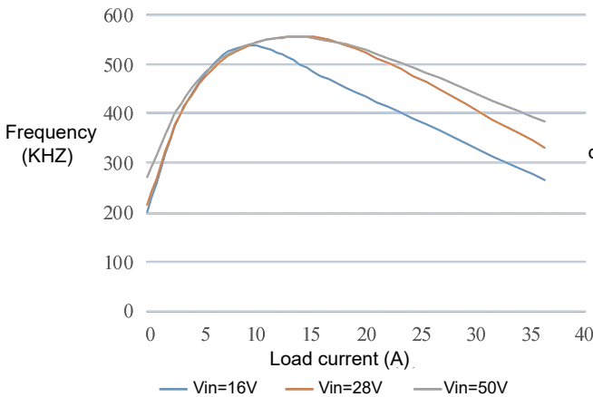
Figure 3 Frequency Curve
