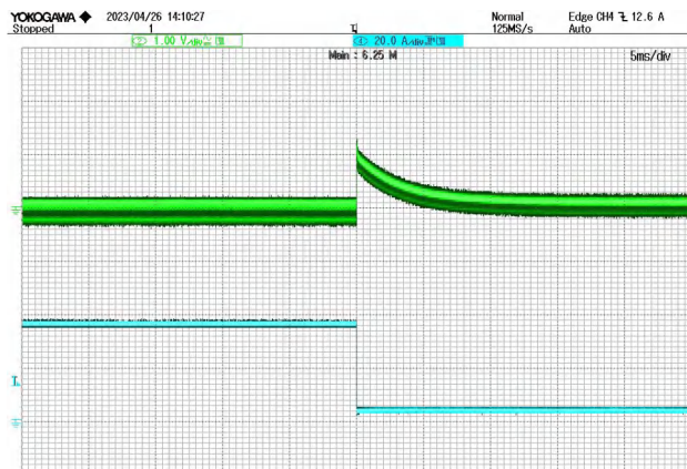
Figure 9 90% load -10% load jump @ VIN=28V CH2: Vout CH4: Io
