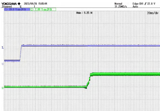
Figure 12 Output Downregulation Start Waveform @ VIN=28V CH1:V IN CH2:V out
