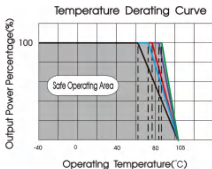
CFDQR75-110S12 temperature derating curve(Vin=110V)
