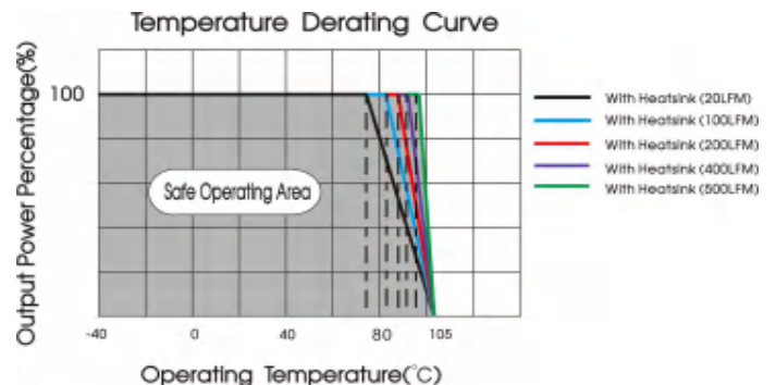
CFDQR75-110S12 temperature derating curve(Vin=110V)
