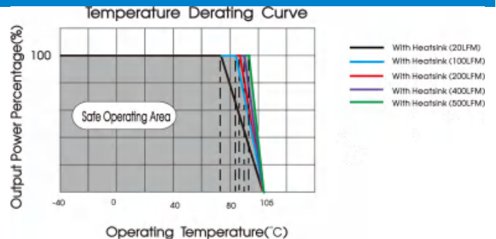
CFDQR75-110S05S temperature derating curve(Vin=110V)
