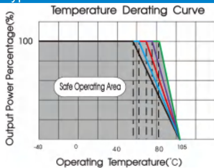
CFDQR75-110S05S temperature derating curve(Vin=110V)
