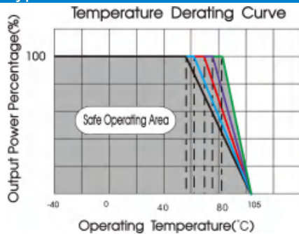
CFDQR50-110S05S temperature derating curve(Vin=110V)
