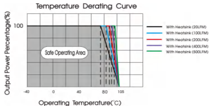
CFDQR50-110S12 temperature derating curve(Vin=110V)
