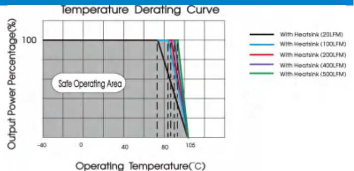
CFDQR50-110S05S temperature derating curve(Vin=110V)
