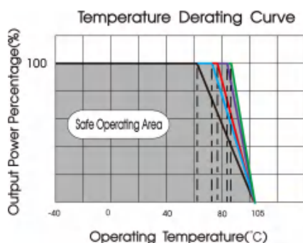
CFDQR50-110S12 temperature derating curve(Vin=110V)
