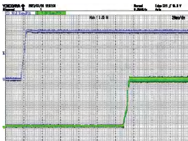
Figure 12 Output Downregulation Start Waveform @ VIN=30V CH1:V IN CH2:V out
