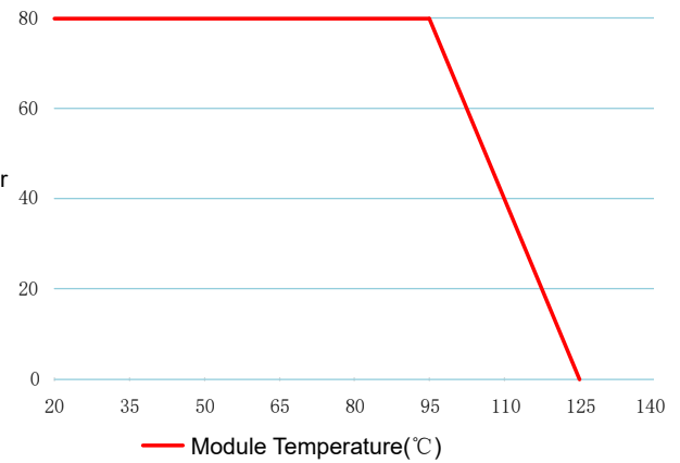
Figure 4 Temperature Derating Curve
