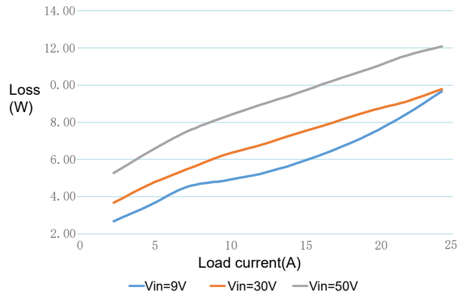
Figure 2 Loss Curve
