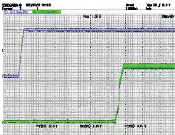
Figure 13 Output Upregulation Start Waveform @ VIN=30V CH1:V IN CH2:V out
