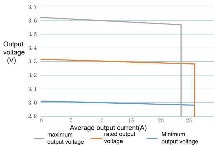
Figure 5 Safe Work Area
