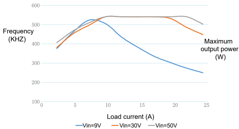
Figure 3 Frequency Curve
