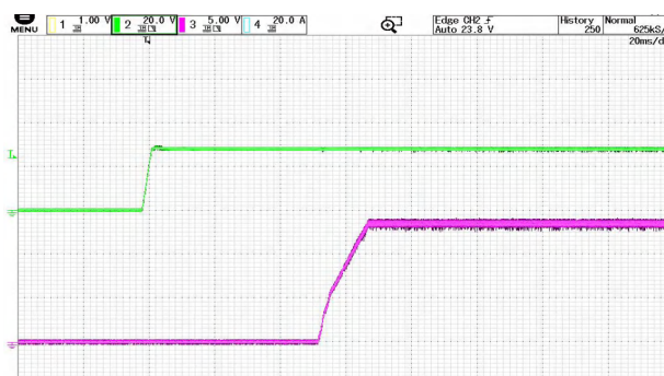
Figure 13 Output Upregulation Start Waveform @ VIN=30V CH2:VIN CH3:Vout
