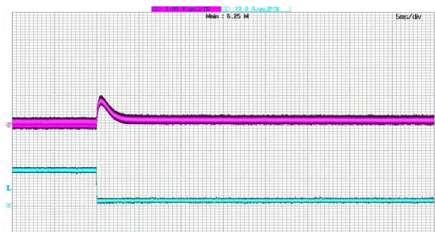
Figure 9 90% load -10% load jump @ VIN=30V CH3: Vout CH4: Io
