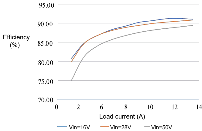
Figure 1 Efficiency curve
