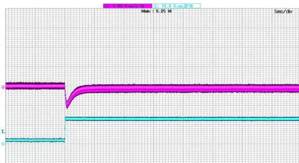
Figure 8 10% load -90% load jump @ VIN=30V CH3: Vout CH4: Io
