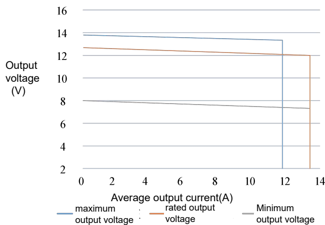
Figure 5 Safe Work Area
