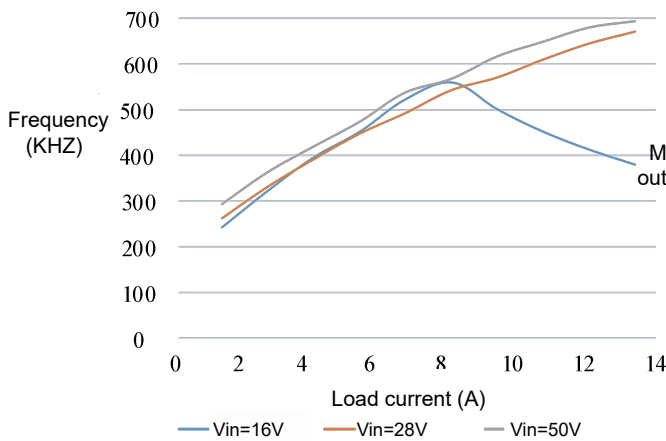
Figure 3 Frequency Curve
