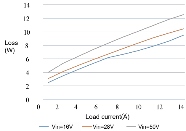
Figure 2 Loss Curve
