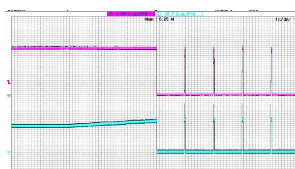
Figure 15 Overcurrent protection @ VIN=30V CH3: Iout CH4:Vout
