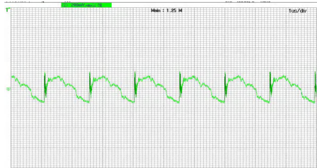
Figure 7 Output voltage ripple @ VIN=30V at full load
