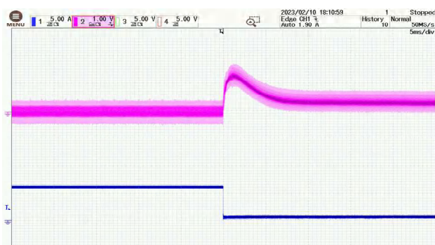
Figure 8 90% load -10% load jump @ VIN=30V CH2: Vout CH1: Io
